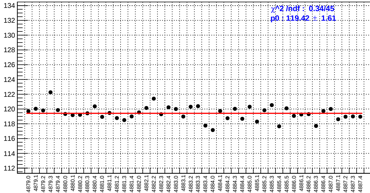
slug89: reg_asym_right_avg.rms/ppm
