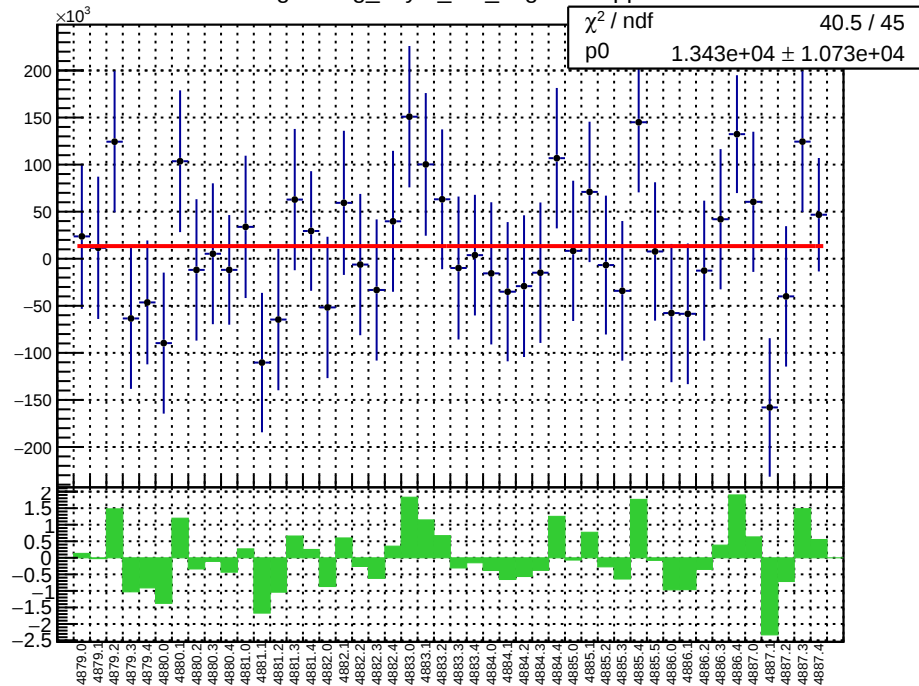
slug89: reg_asym_at2_avg.mean/ppb
