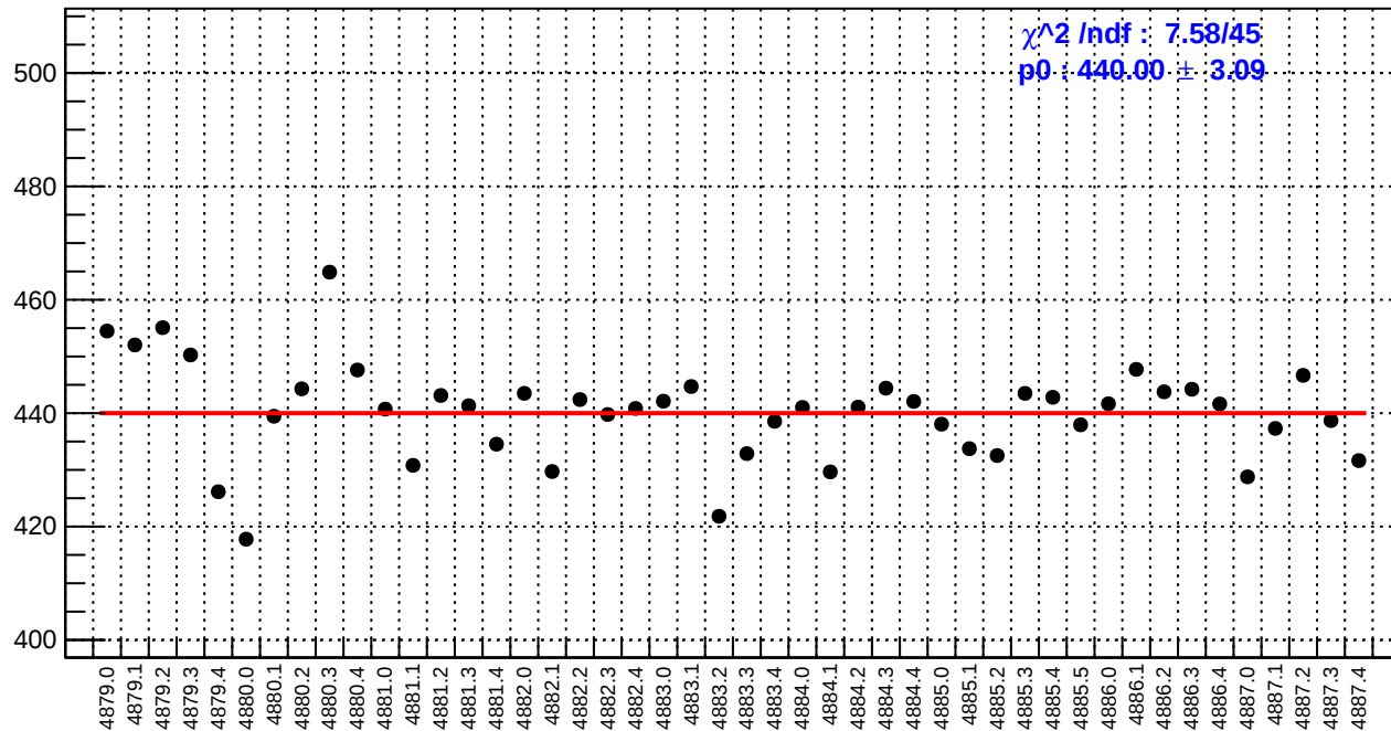
slug89: reg_asym_sam8.rms/ppm
