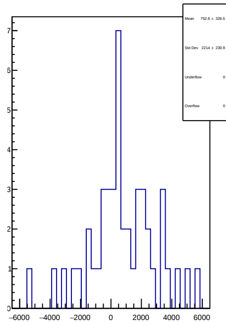
slug89: 1D Corr asym_at2_avg.mean/ppb-reg_asym_at2_avg.mean/ppb
