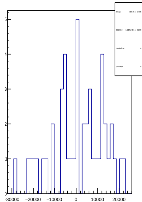
slug89: 1D Corr asym_sam6.mean/ppb-reg_asym_sam6.mean/ppb
