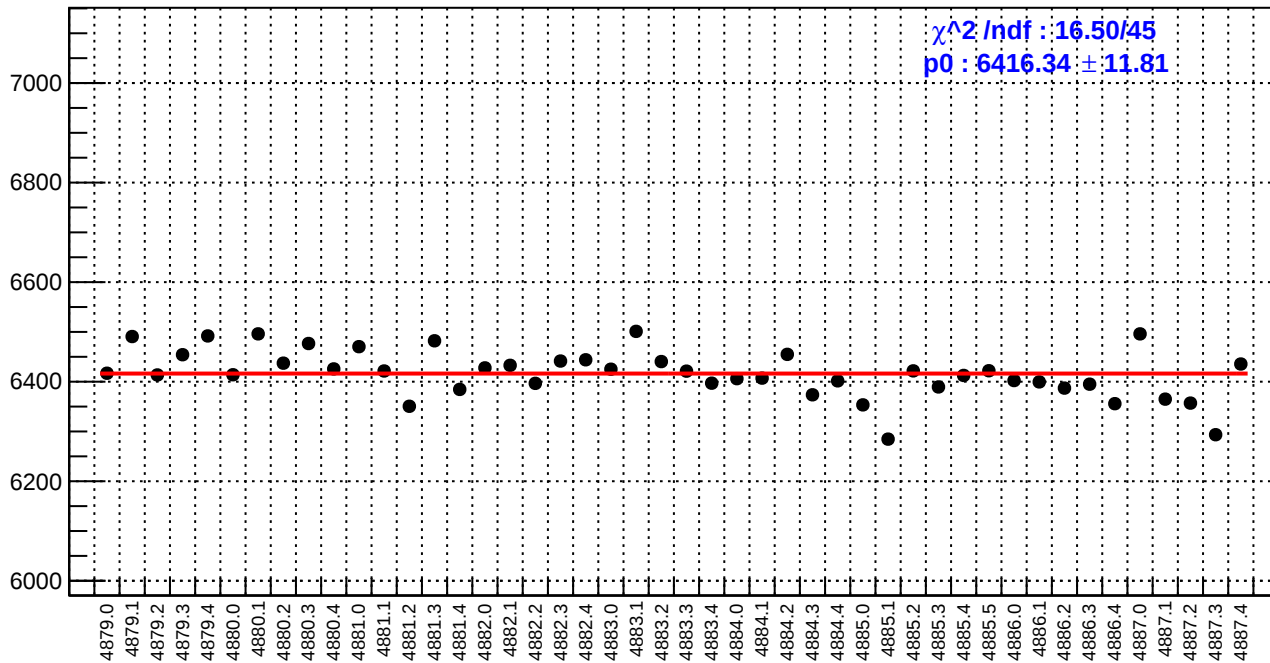
slug89: reg_asym_atl1r2_dd.rms/ppm
