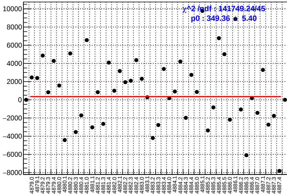
slug89: asym_atr_avg.mean/ppb-reg_asym_atr_avg.mean/ppb
