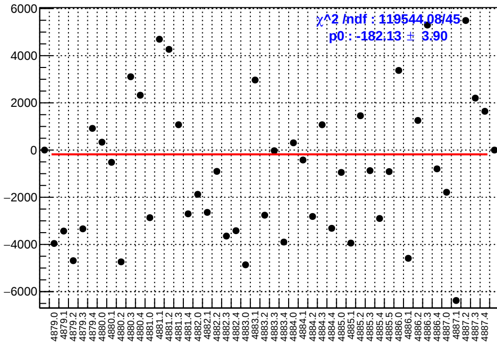
slug89: asym_atl1.mean/ppb-reg_asym_atl1.mean/ppb
