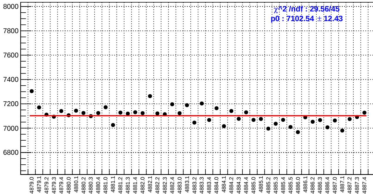
slug89: reg_asym_at2_avg.rms/ppm
