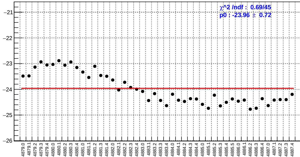
slug89: us_avg_bpm4eX/(ppb/nm)
