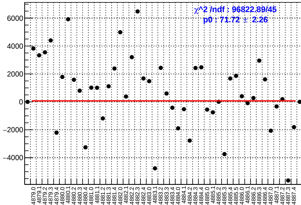
slug89: asym_us_avg.mean/ppb-reg_asym_us_avg.mean/ppb
