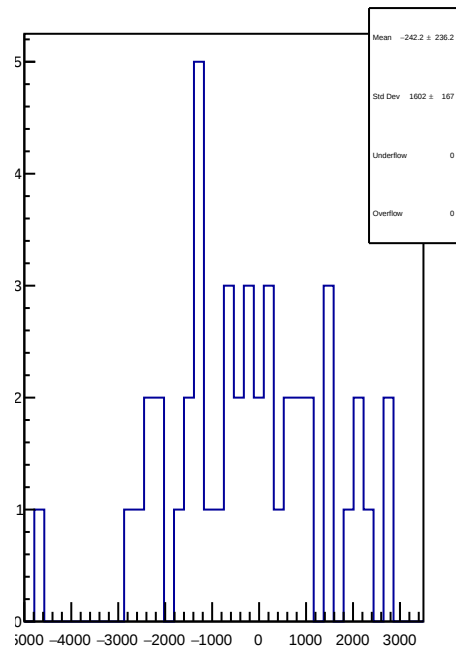
slug89: 1D Corr asym_at1_avg.mean/ppb-reg_asym_at1_avg.mean/ppb
