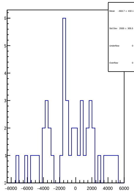
slug89: 1D Corr asym_ds_dd.mean/ppb-reg_asym_ds_dd.mean/ppb
