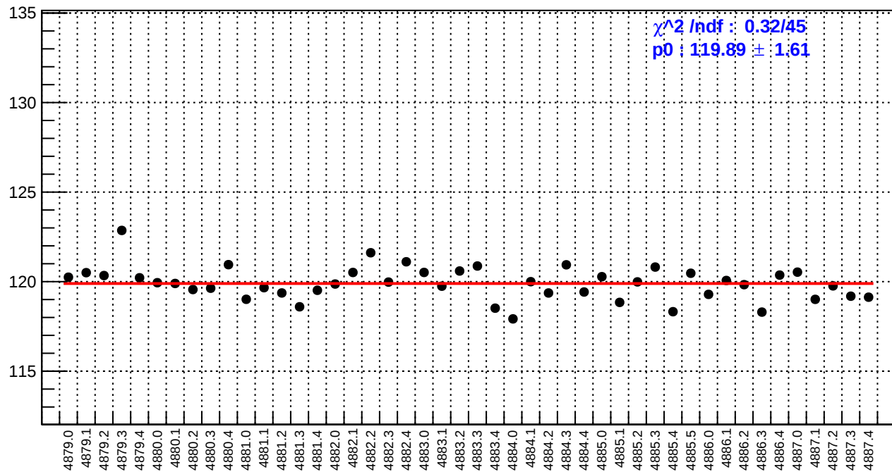
slug89: reg_asym_usr.rms/ppm
