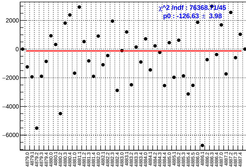
slug89: asym_atr_dd.mean/ppb-reg_asym_atr_dd.mean/ppb
