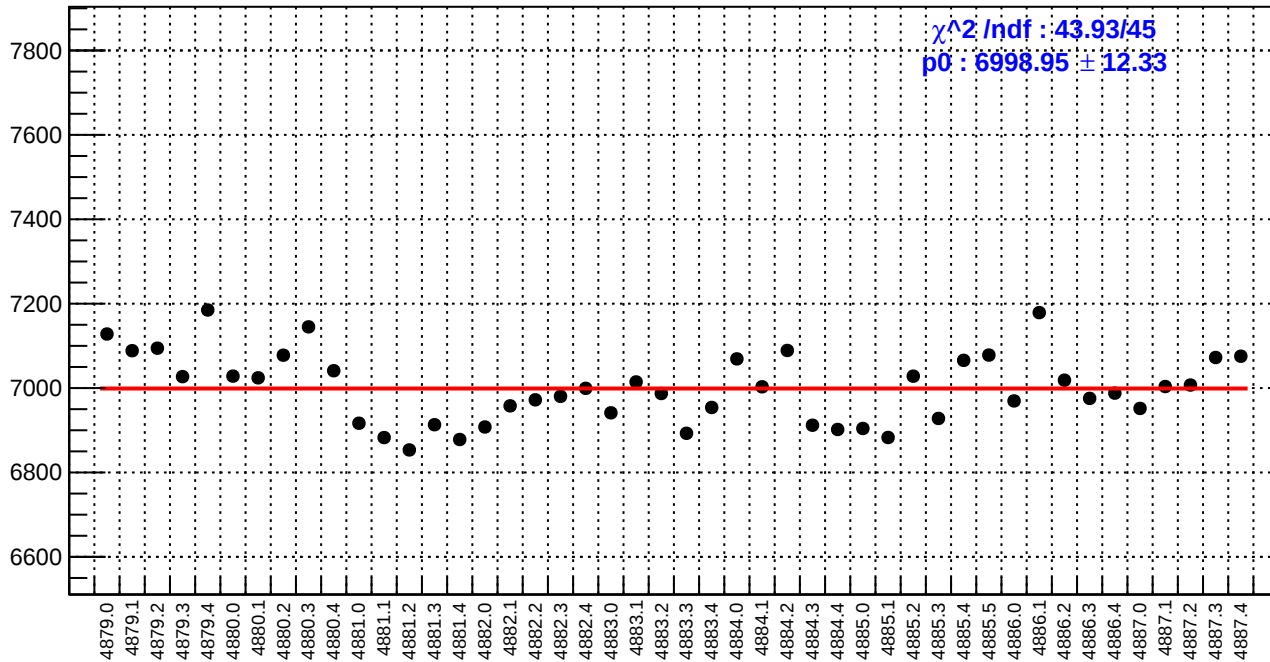
slug89: diff_bpm4eX.rms/nm
