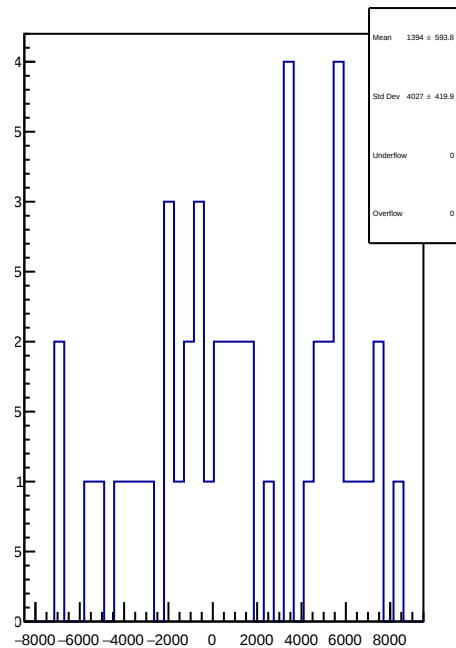
slug89: 1D Corr asym_usr.mean/ppb-reg_asym_usr.mean/ppb
