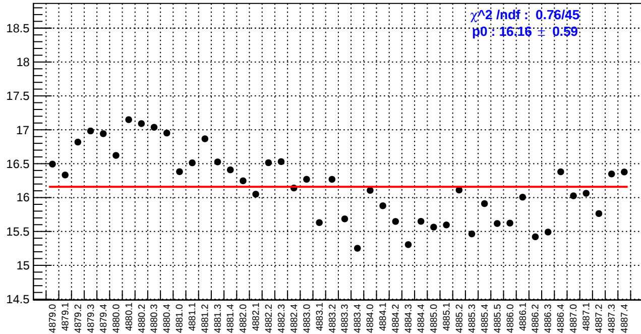
slug89: right_avg_bpm4eX/(ppb/nm)
