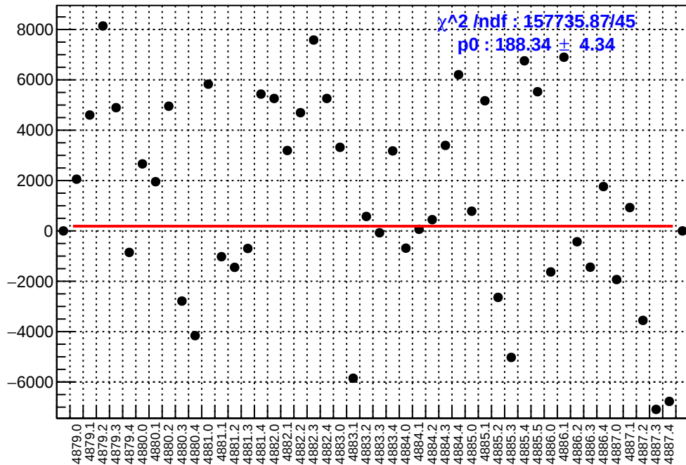
slug89: asym_right_avg.mean/ppb-reg_asym_right_avg.mean/ppb
