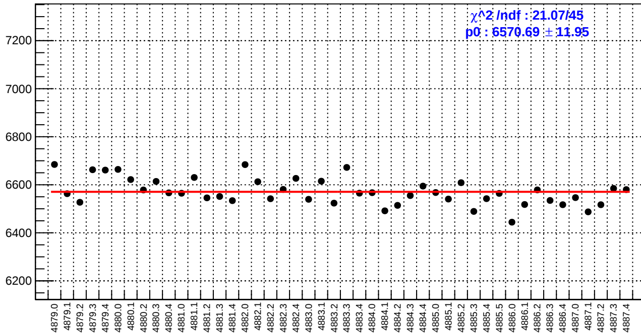
slug89: reg_asym_atr1l2_avg.rms/ppm
