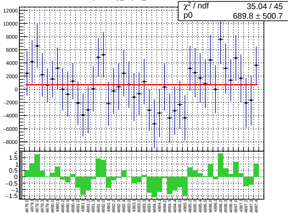
slug89: reg_asym_sam7.mean/ppb
