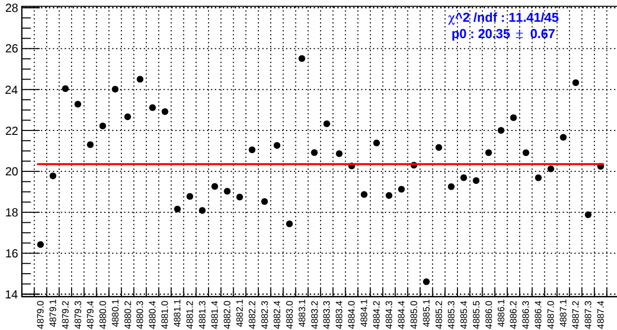
slug89: usl_bpm4eY/(ppb/nm)
