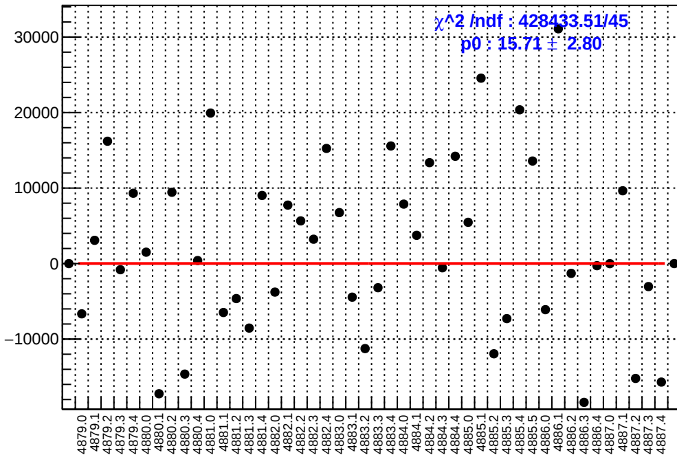
slug89: asym_sam8.mean/ppb-reg_asym_sam8.mean/ppb
