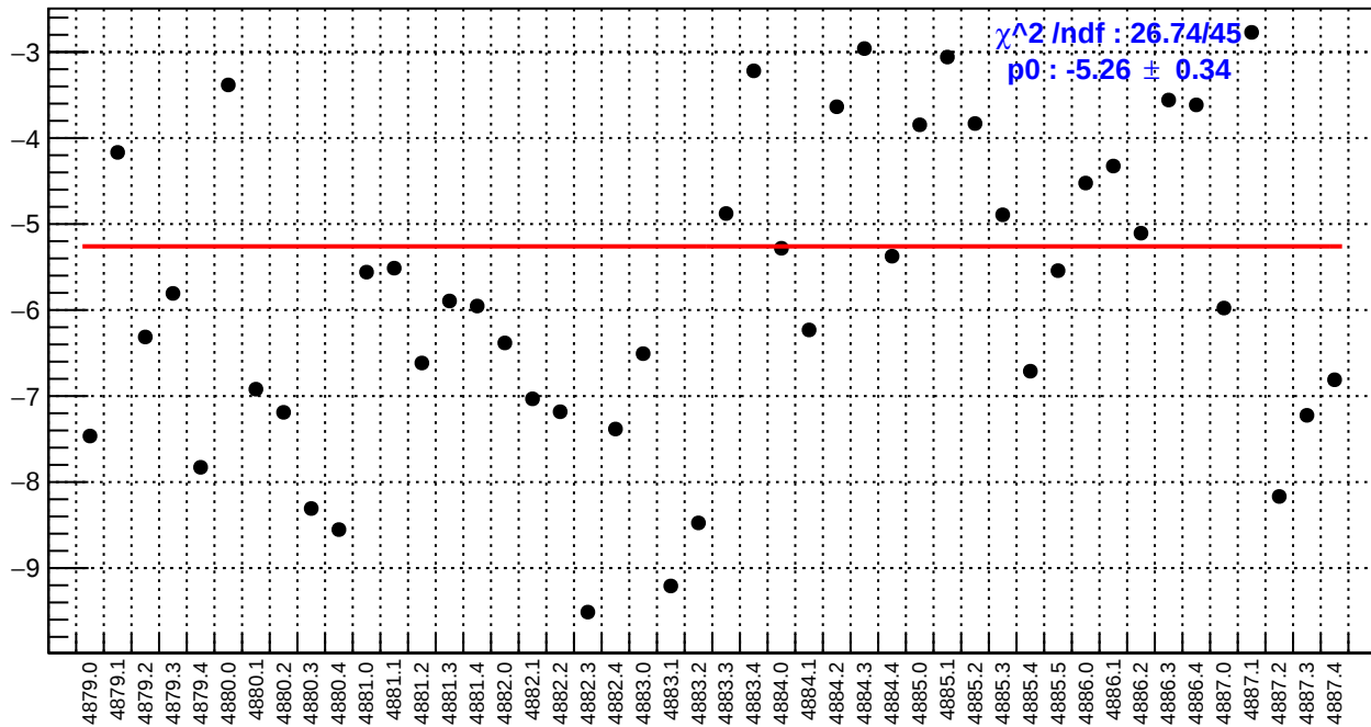
slug89: right_avg_bpm4aX/(ppb/nm)
