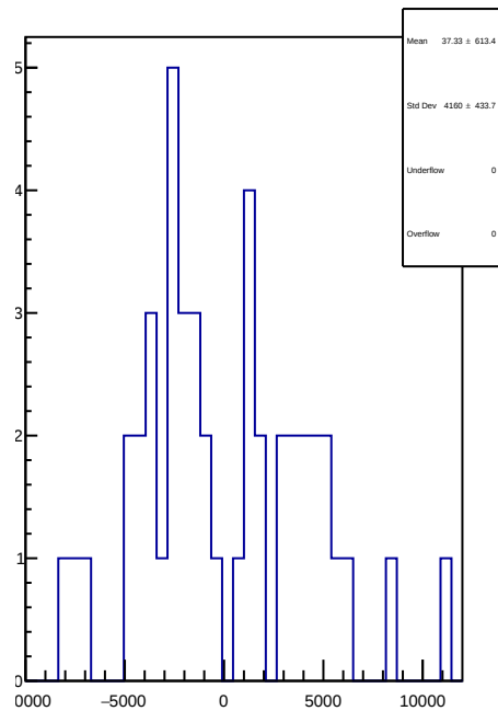
slug89: 1D Corr asym_dsl.mean/ppb-reg_asym_dsl.mean/ppb
