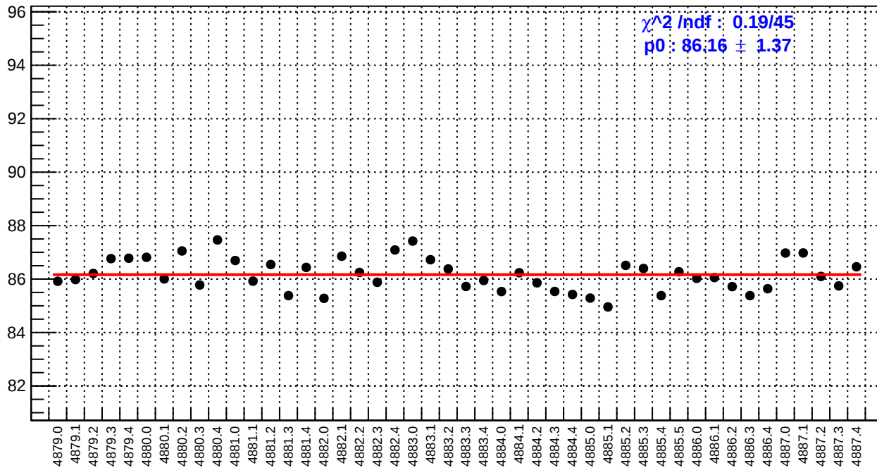
slug89: reg_asym_ds_dd.rms/ppm
