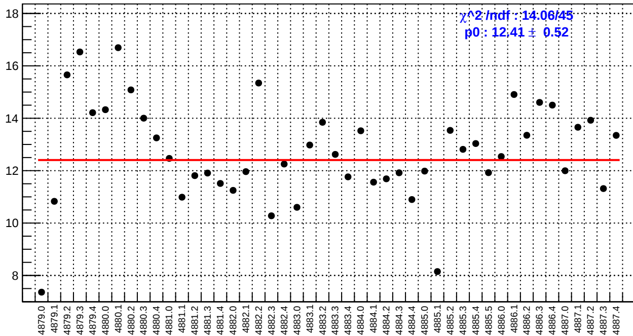
slug89: us_avg_bpm4eY/(ppb/nm)
