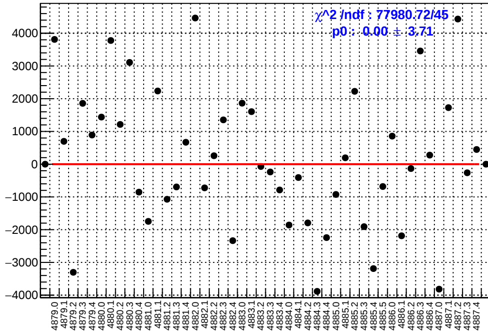
slug89: asym_atr1l2_avg.mean/ppb-reg_asym_atr1l2_avg.mean/ppb
