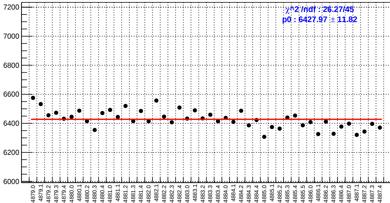
slug89: reg_asym_atl1r2_avg.rms/ppm
