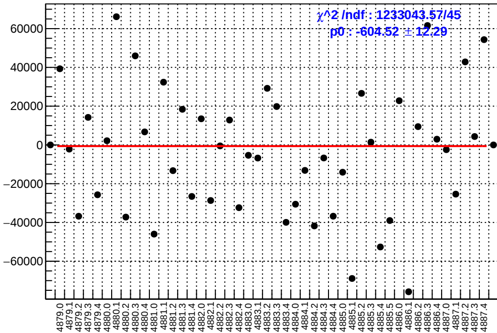
slug89: asym_sam2.mean/ppb-reg_asym_sam2.mean/ppb
