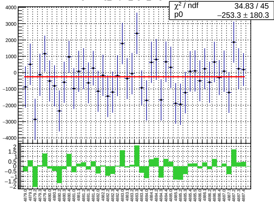
slug89: reg_asym_right_avg.mean/ppb
