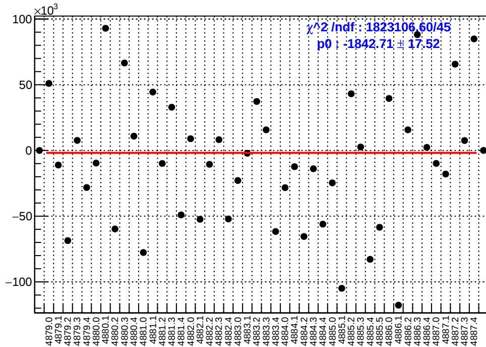
slug89: asym_sam3.mean/ppb-reg_asym_sam3.mean/ppb
