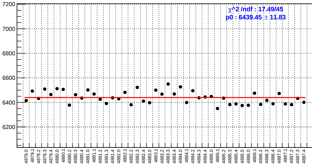
slug89: reg_asym_atl_avg.rms/ppm
