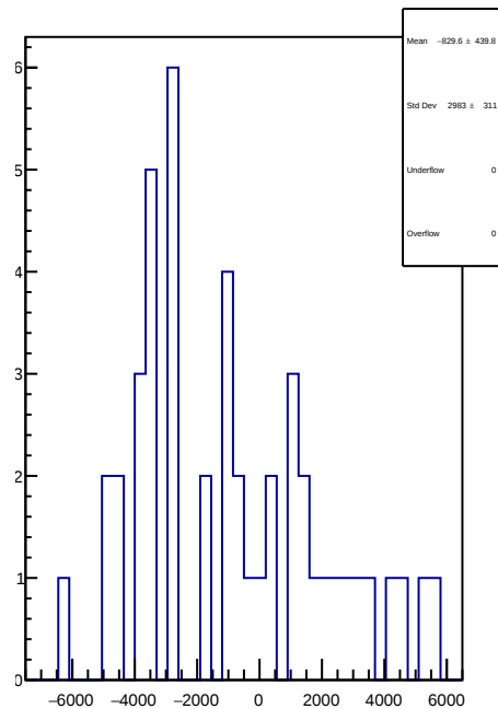
slug89: 1D Corr asym_atl1.mean/ppb-reg_asym_atl1.mean/ppb
