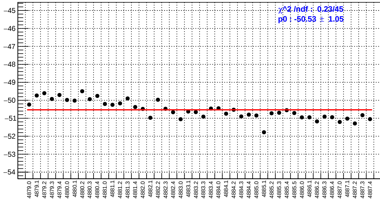
slug89: ds_avg_bpm12X/(ppb/nm)
