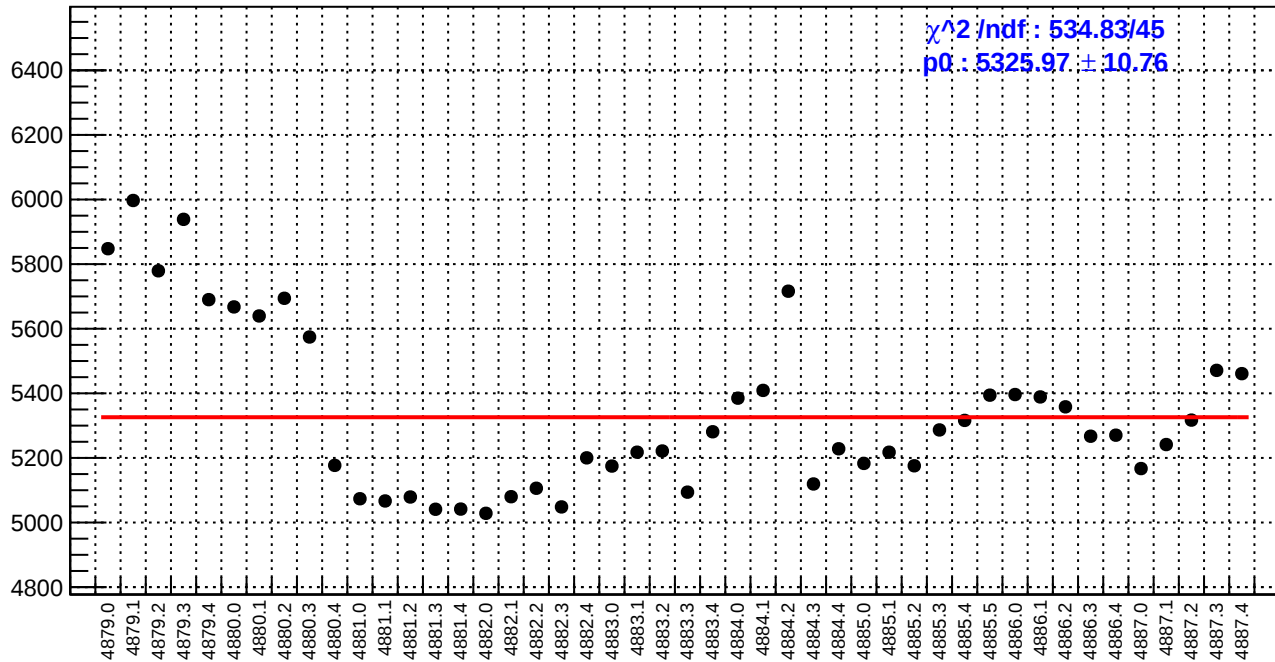
slug89: diff_bpm11X.rms/nm
