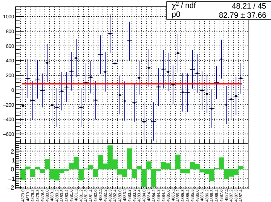
slug89: reg_asym_right_dd.mean/ppb
