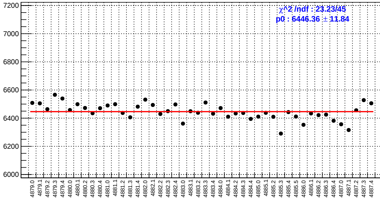
slug89: reg_asym_atl_dd.rms/ppm
