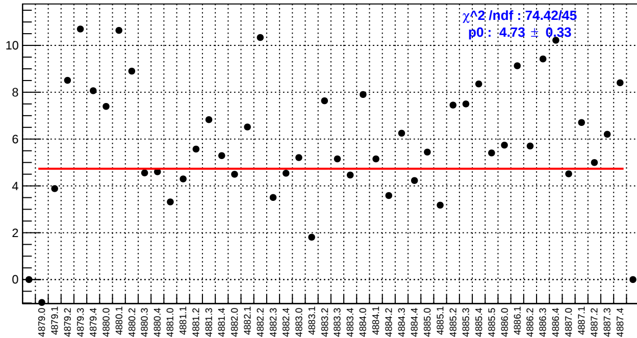
slug89: right_avg_bpm4eY/(ppb/nm)
