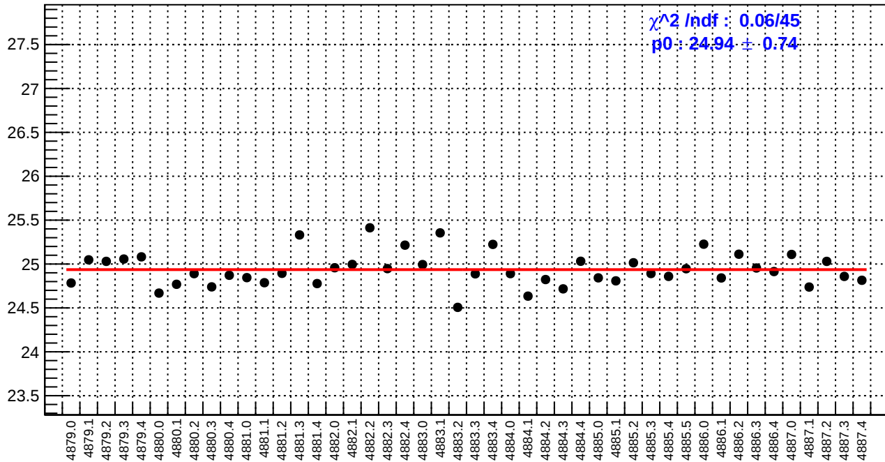
slug89: reg_asym_right_dd.rms/ppm
