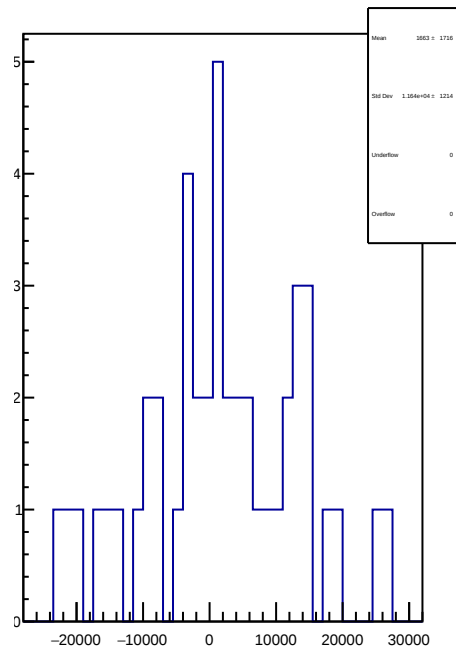
slug89: 1D Corr asym_sam7.mean/ppb-reg_asym_sam7.mean/ppb
