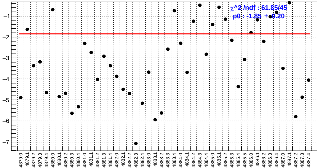
slug89: dsr_bpm4aX/(ppb/nm)
