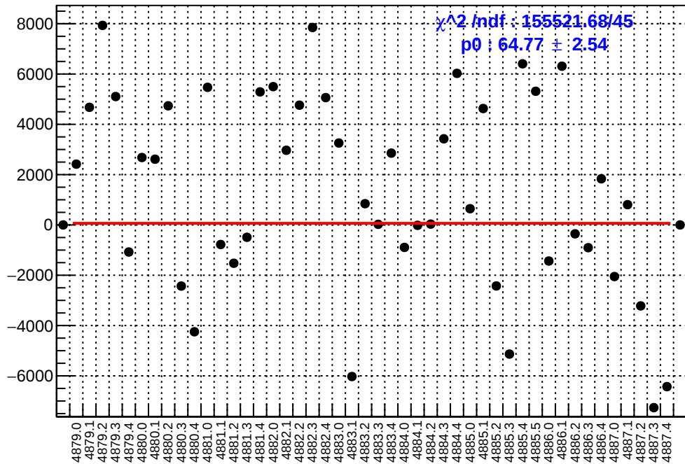
slug89: asym_dsr.mean/ppb-reg_asym_dsr.mean/ppb
