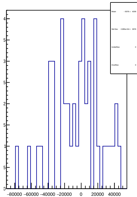
slug89: 1D Corr asym_sam4.mean/ppb-reg_asym_sam4.mean/ppb
