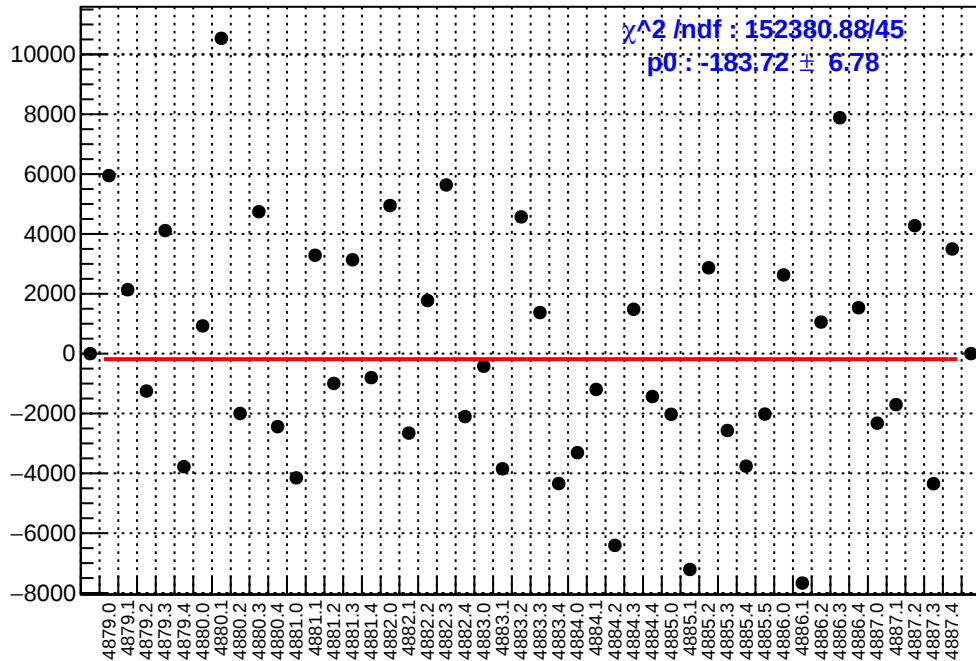
slug89: asym_usl.mean/ppb-reg_asym_usl.mean/ppb
