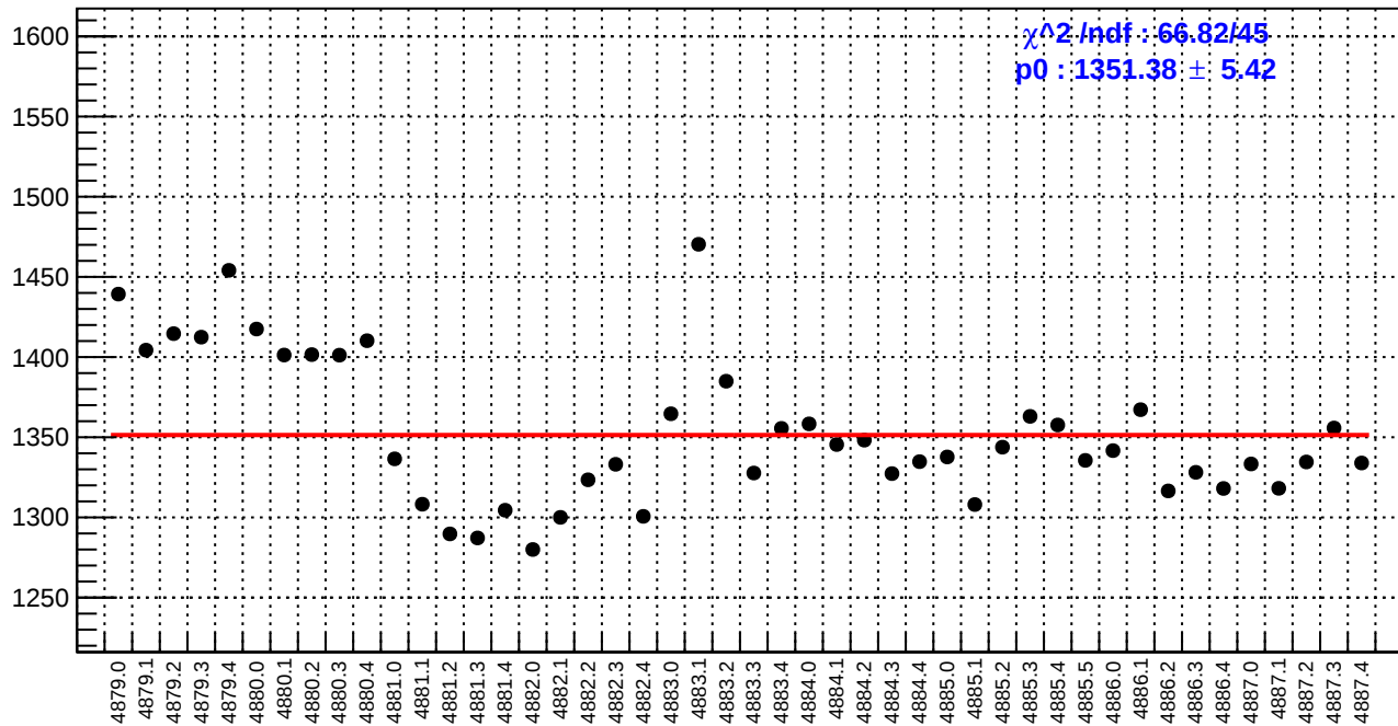
slug89: diff_bpm4aX.rms/nm
