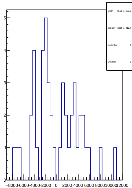
slug89: 1D Corr asym_usl.mean/ppb-reg_asym_usl.mean/ppb
