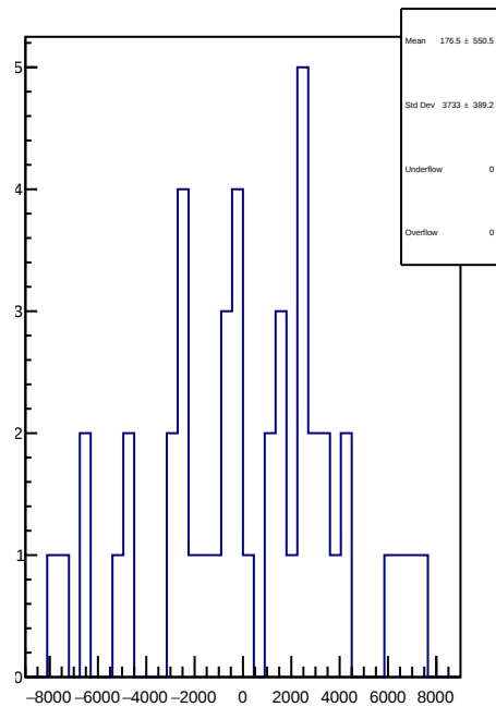
slug89: 1D Corr asym_atr1l2_dd.mean/ppb-reg_asym_atr1l2_dd.mean/ppb
