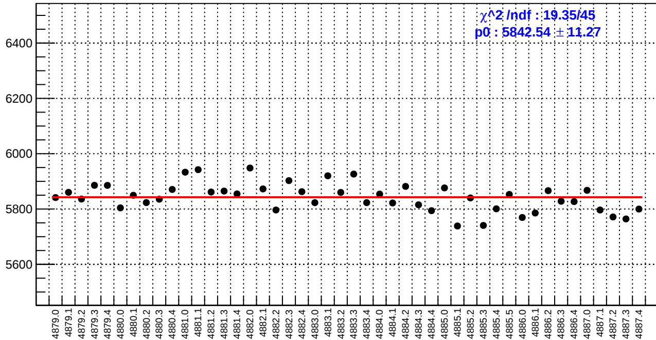
slug89: reg_asym_at1_avg.rms/ppm
