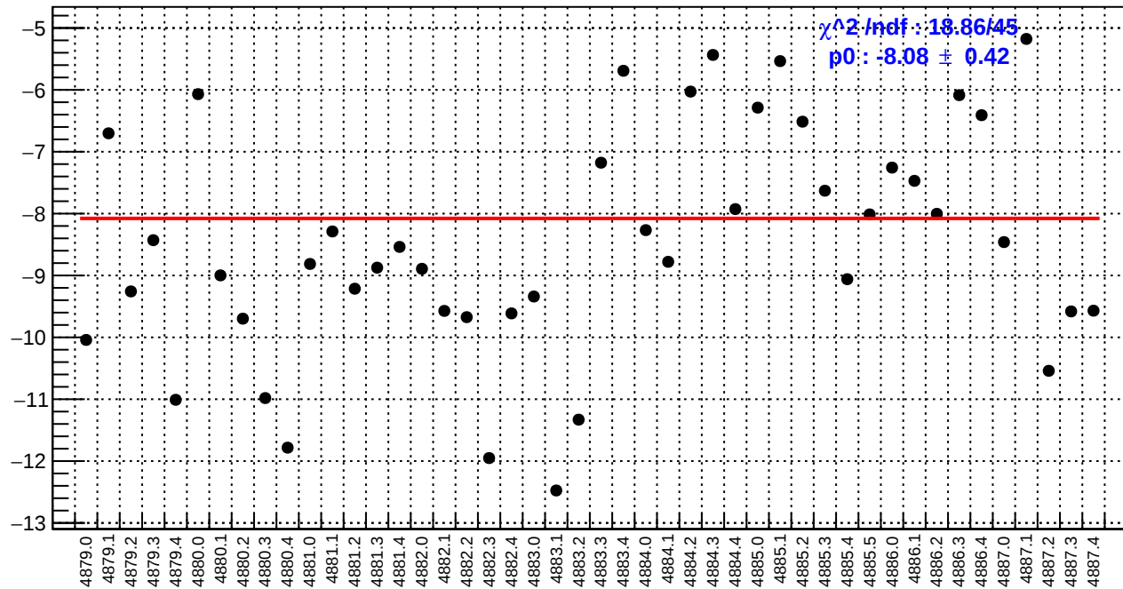
slug89: usr_bpm4aX/(ppb/nm)
