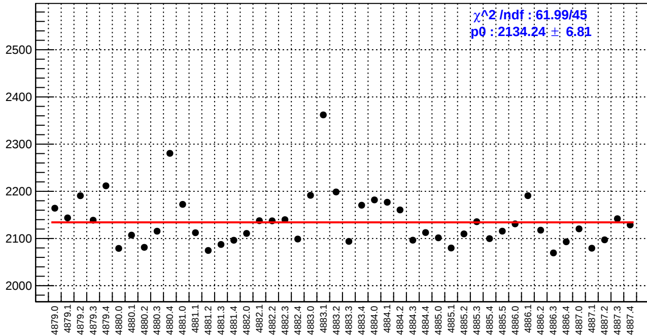
slug89: diff_bpm4eY.rms/nm
