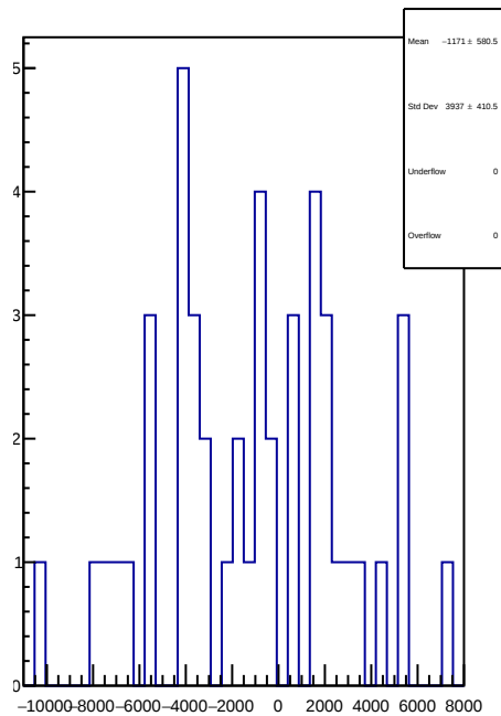
slug89: 1D Corr asym_atl1r2_dd.mean/ppb-reg_asym_atl1r2_dd.mean/ppb
