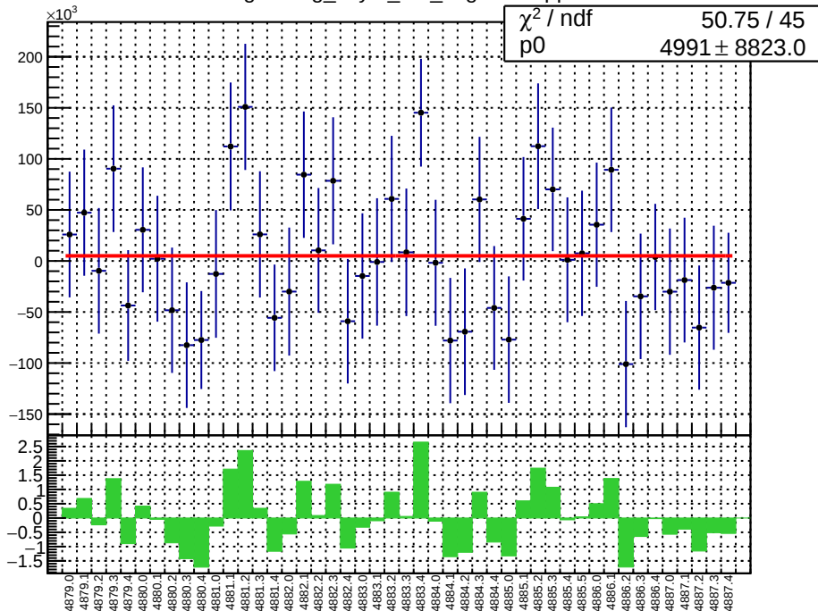
slug89: reg_asym_at1_avg.mean/ppb
