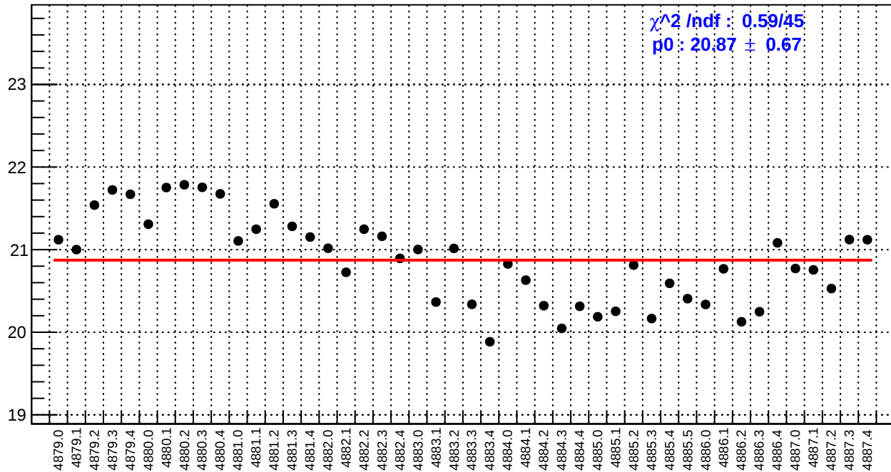
slug89: usr_bpm4eX/(ppb/nm)
