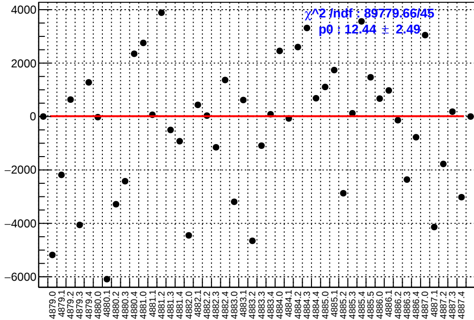
slug89: asym_atl_dd.mean/ppb-reg_asym_atl_dd.mean/ppb
