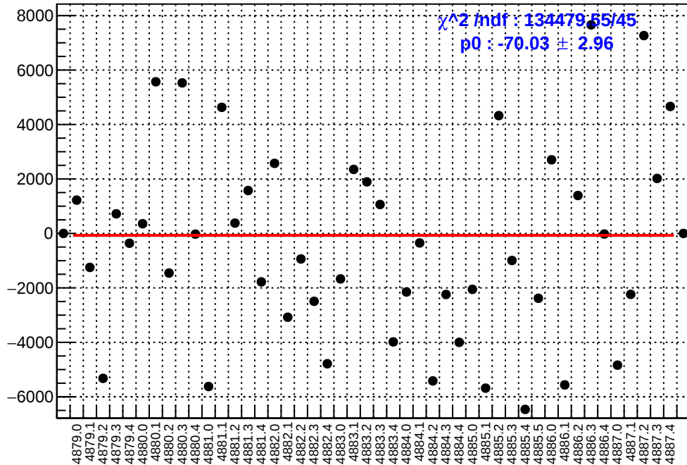
slug89: asym_atl_avg.mean/ppb-reg_asym_atl_avg.mean/ppb
