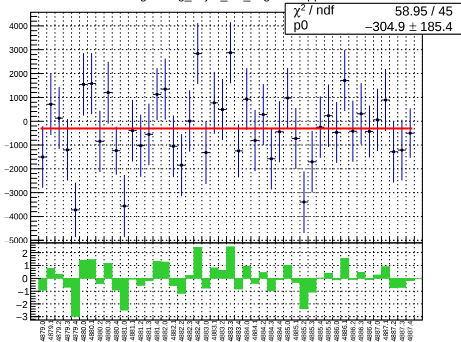
slug89: reg_asym_left_avg.mean/ppb
