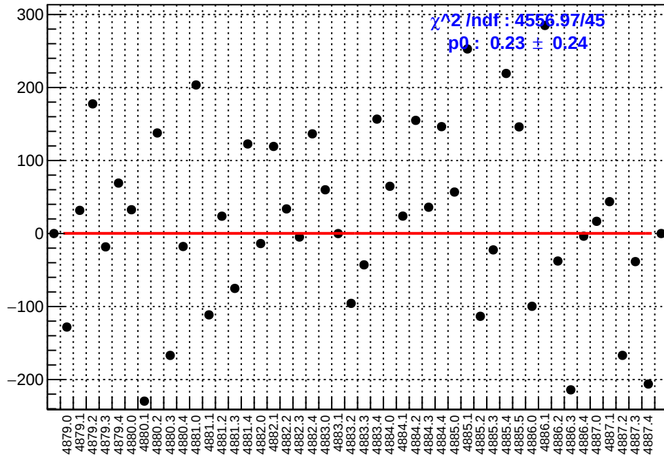
slug89: asym_left_dd.mean/ppb-reg_asym_left_dd.mean/ppb
