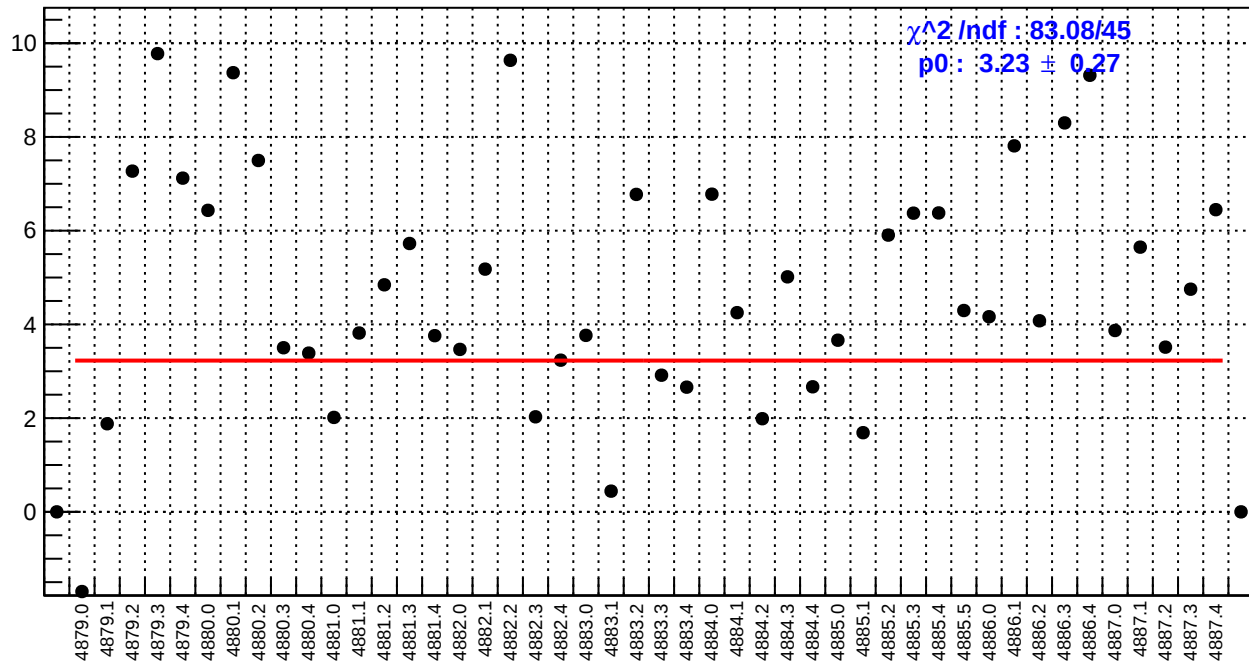
slug89: usr_bpm4eY/(ppb/nm)
