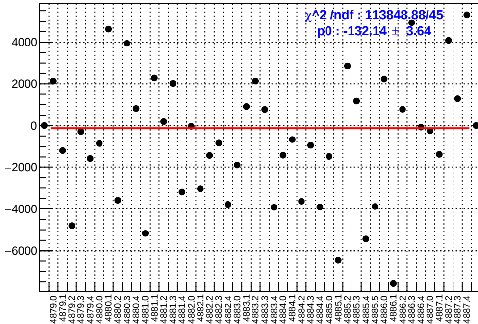
slug89: asym_us_dd.mean/ppb-reg_asym_us_dd.mean/ppb
