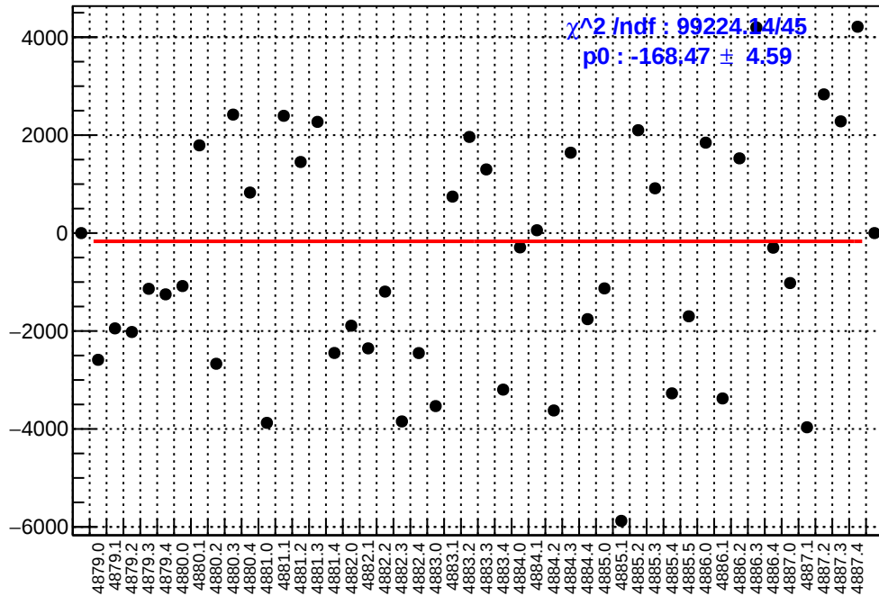
slug89: asym_at1_dd.mean/ppb-reg_asym_at1_dd.mean/ppb
