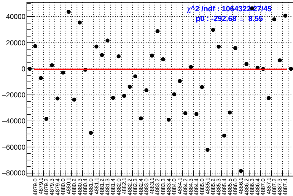
slug89: asym_sam4.mean/ppb-reg_asym_sam4.mean/ppb
