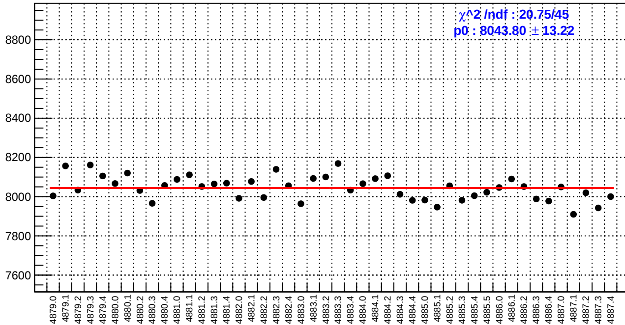
slug89: reg_asym_atl1.rms/ppm
