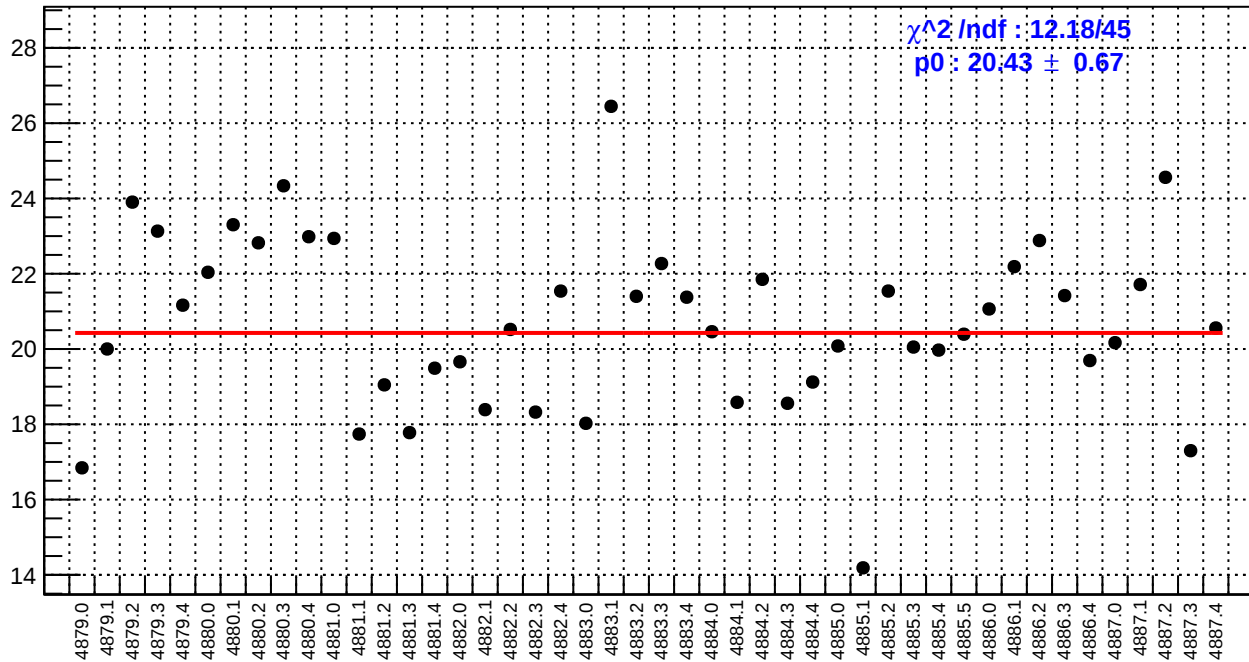
slug89: left_avg_bpm4eY/(ppb/nm)
