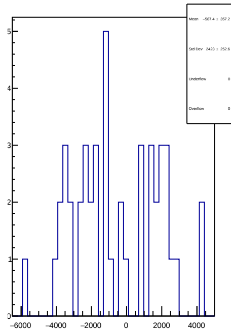
slug89: 1D Corr asym_at1_dd.mean/ppb-reg_asym_at1_dd.mean/ppb
