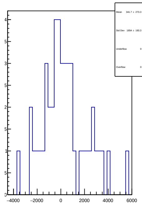
slug89: 1D Corr asym_atl1r2_avg.mean/ppb-reg_asym_atl1r2_avg.mean/ppb
