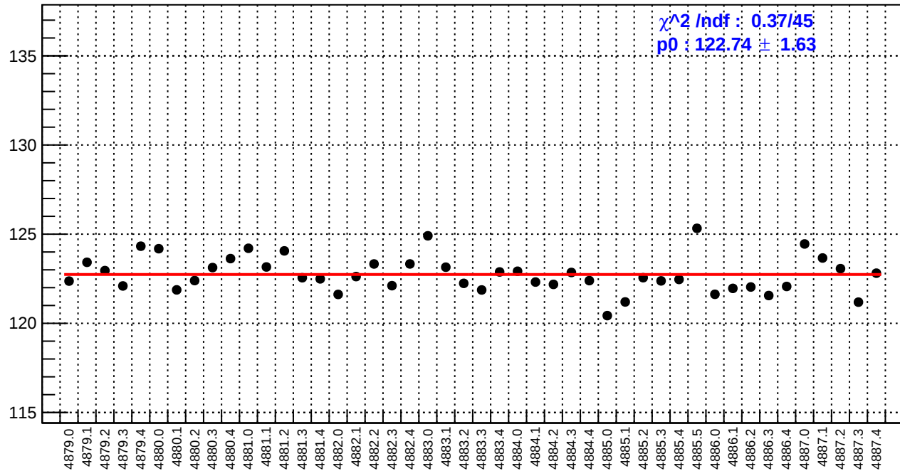
slug89: reg_asym_left_avg.rms/ppm
