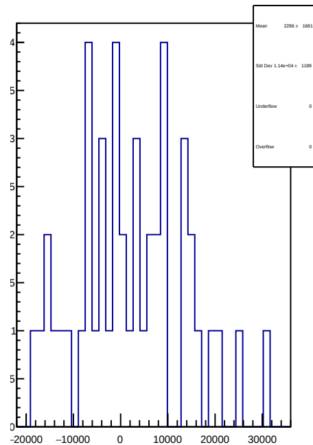
slug89: 1D Corr asym_sam8.mean/ppb-reg_asym_sam8.mean/ppb
