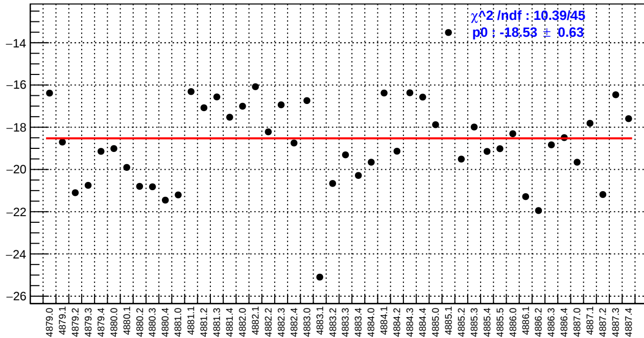
slug89: left_avg_bpm4aY/(ppb/nm)
