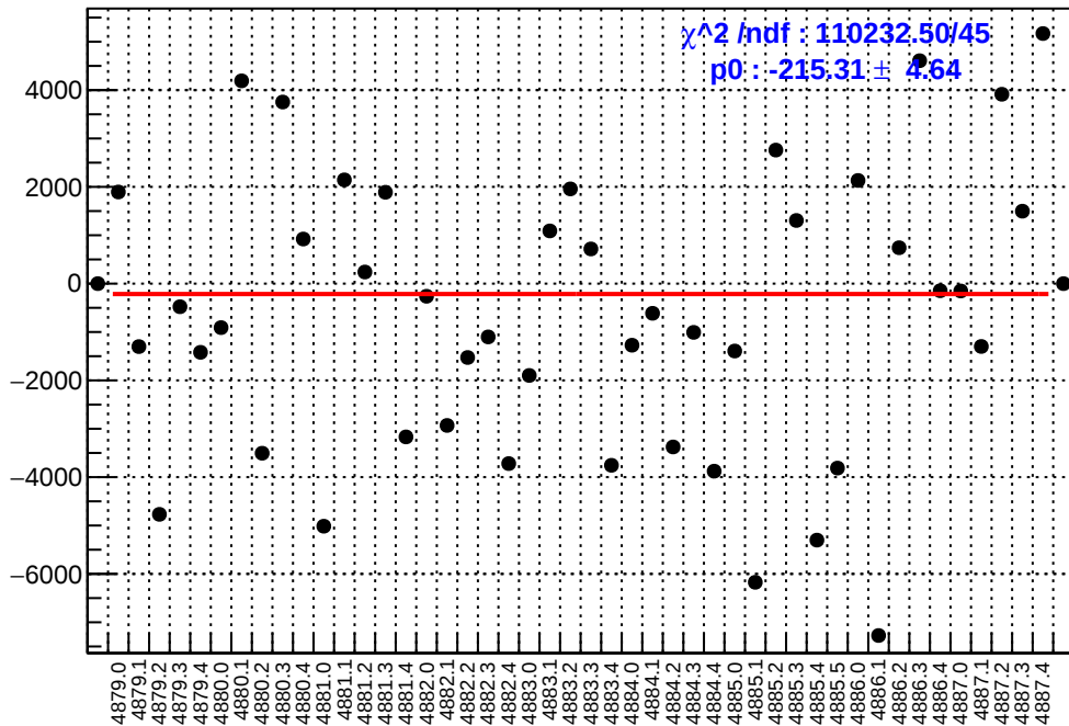
slug89: asym_ds_dd.mean/ppb-reg_asym_ds_dd.mean/ppb
