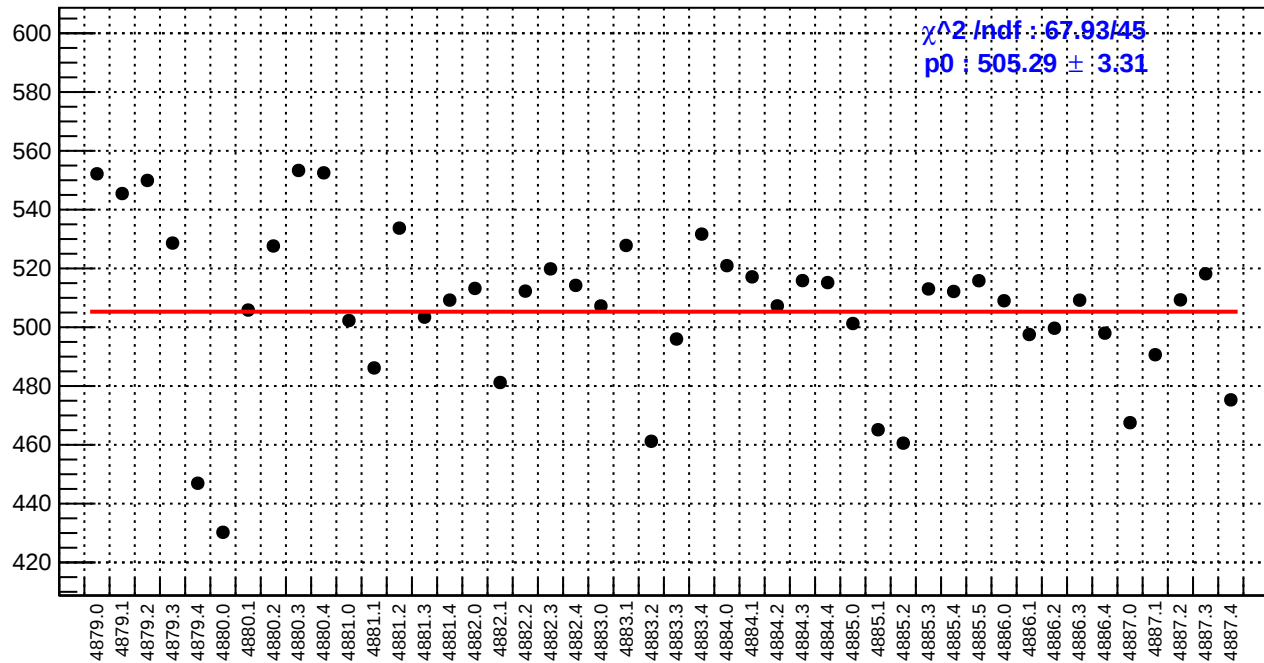
slug89: reg_asym_sam6.rms/ppm
