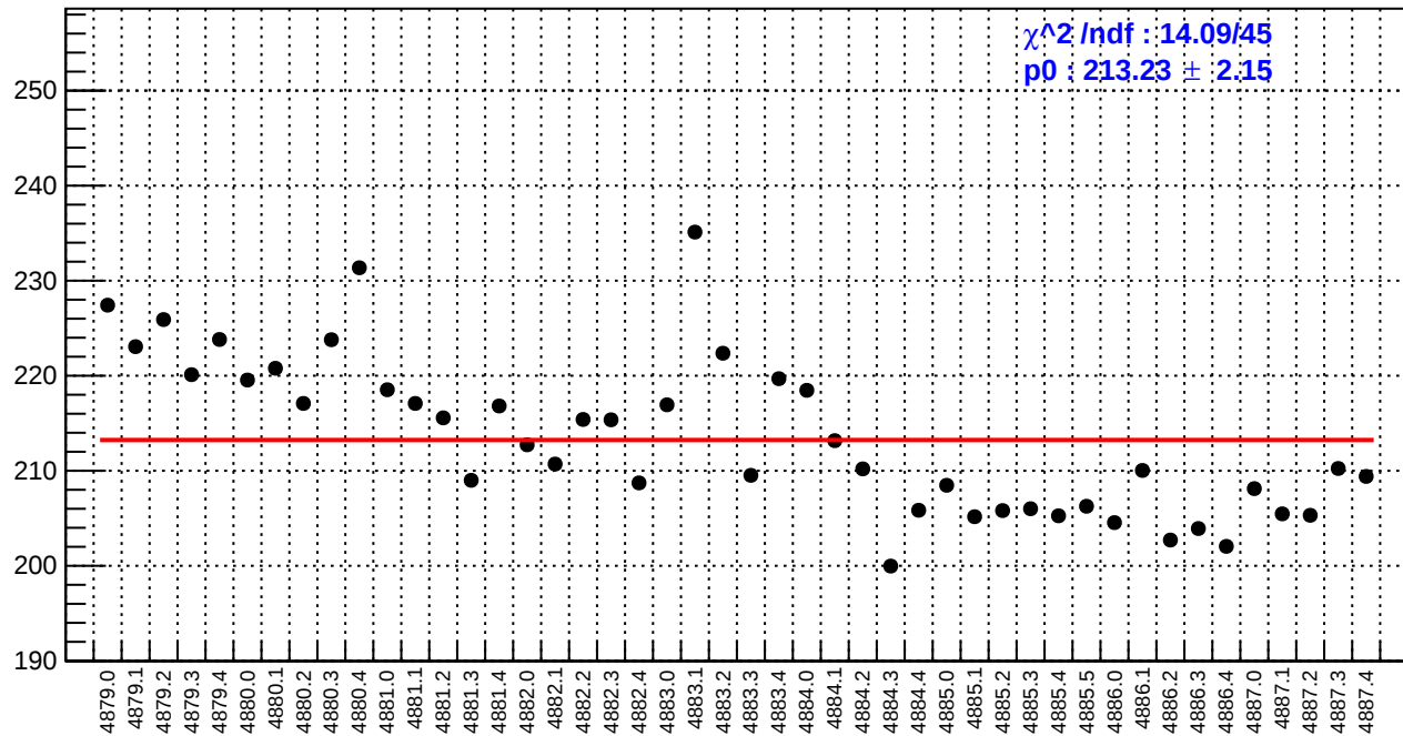
slug89: reg_asym_sam1.rms/ppm
