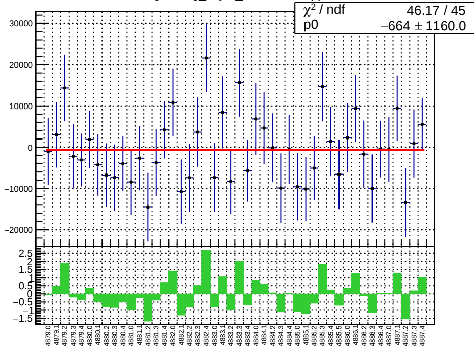
slug89: reg_asym_sam3.mean/ppb
