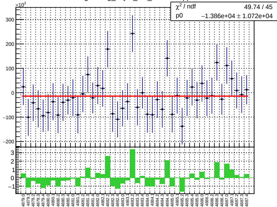
slug89: reg_asym_at2_dd.mean/ppb
