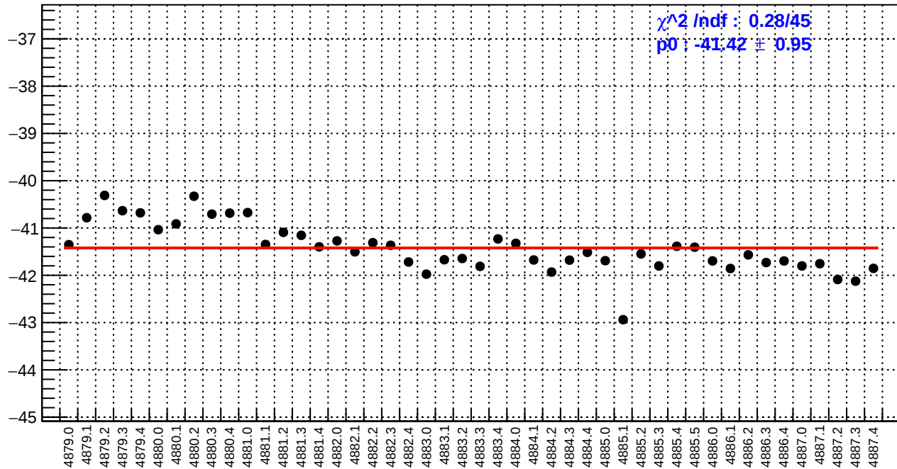
slug89: left_avg_bpm12X/(ppb/nm)
