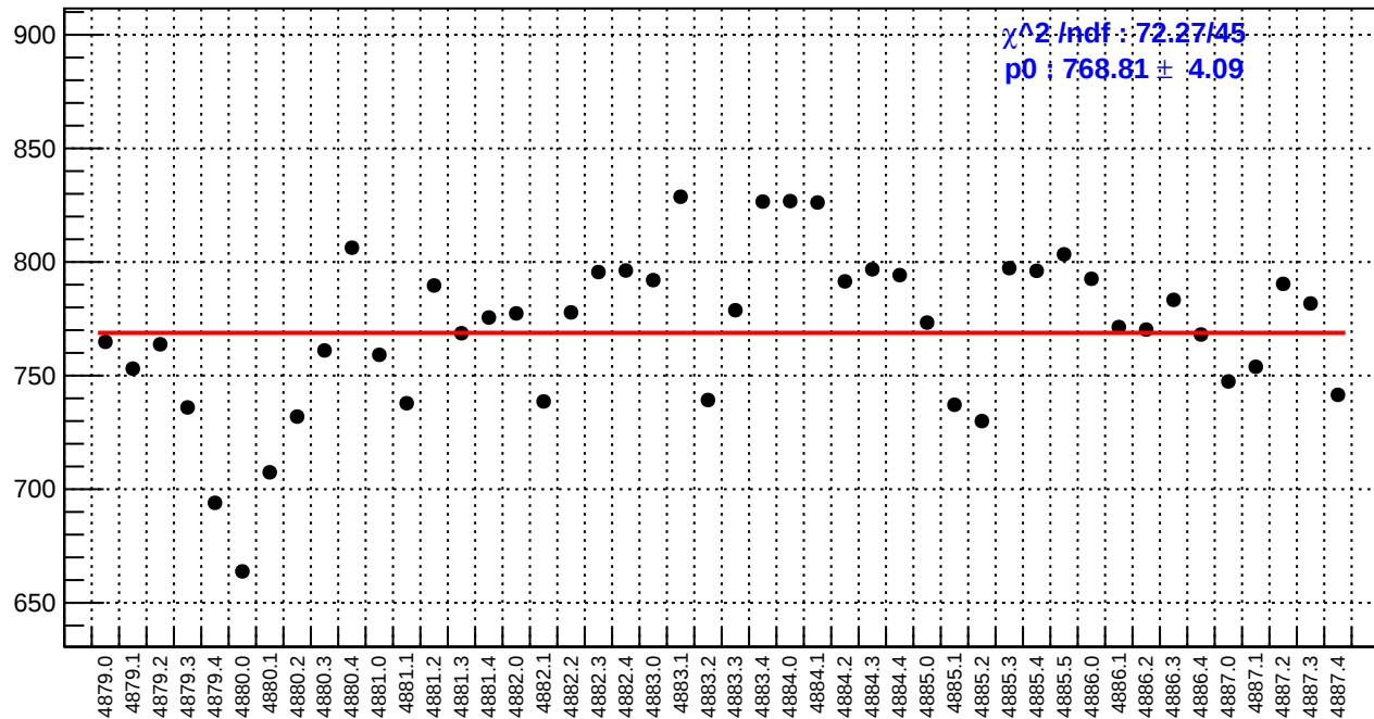
slug89: reg_asym_sam3.rms/ppm
