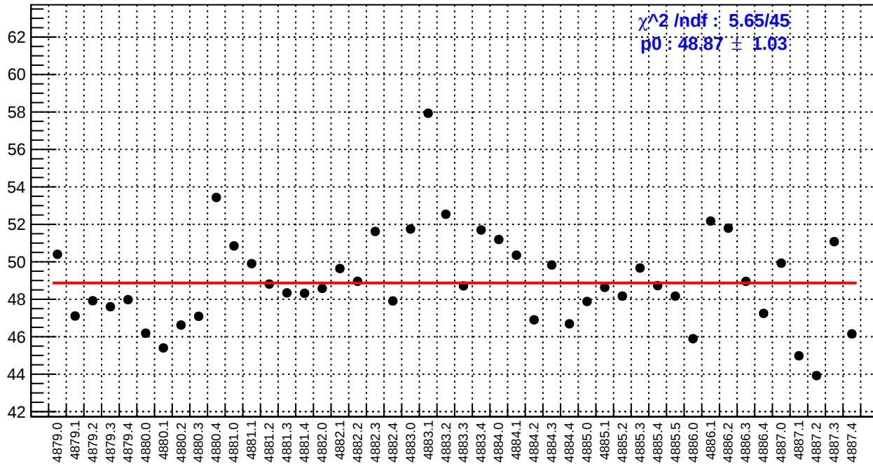
slug89: left_avg_bpm4aX/(ppb/nm)
