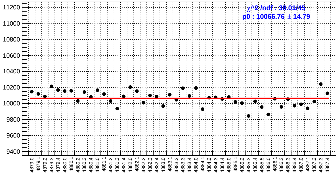
slug89: reg_asym_atl2.rms/ppm
