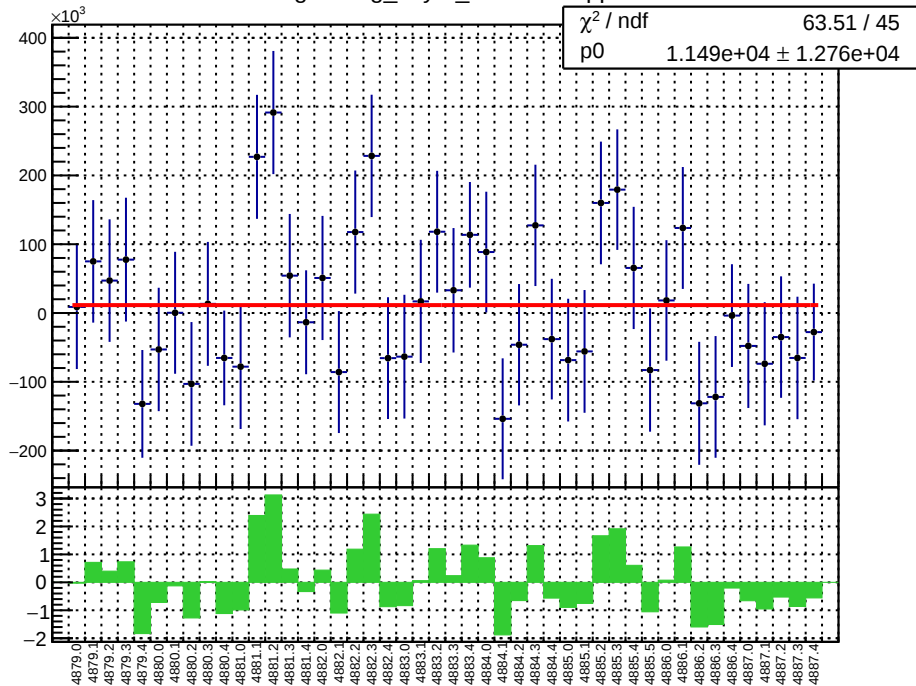
slug89: reg_asym_atr1.mean/ppb
