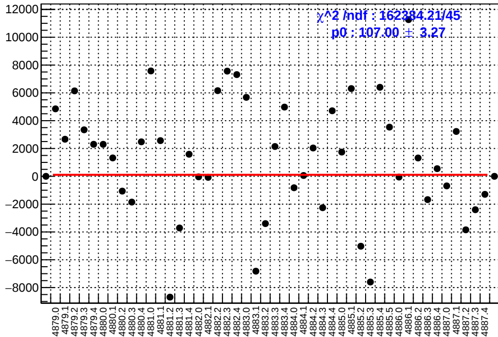
slug89: asym_sam1.mean/ppb-reg_asym_sam1.mean/ppb
