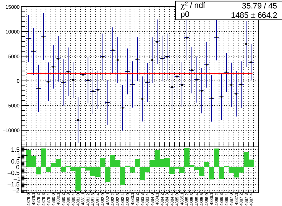
slug89: reg_asym_sam8.mean/ppb
