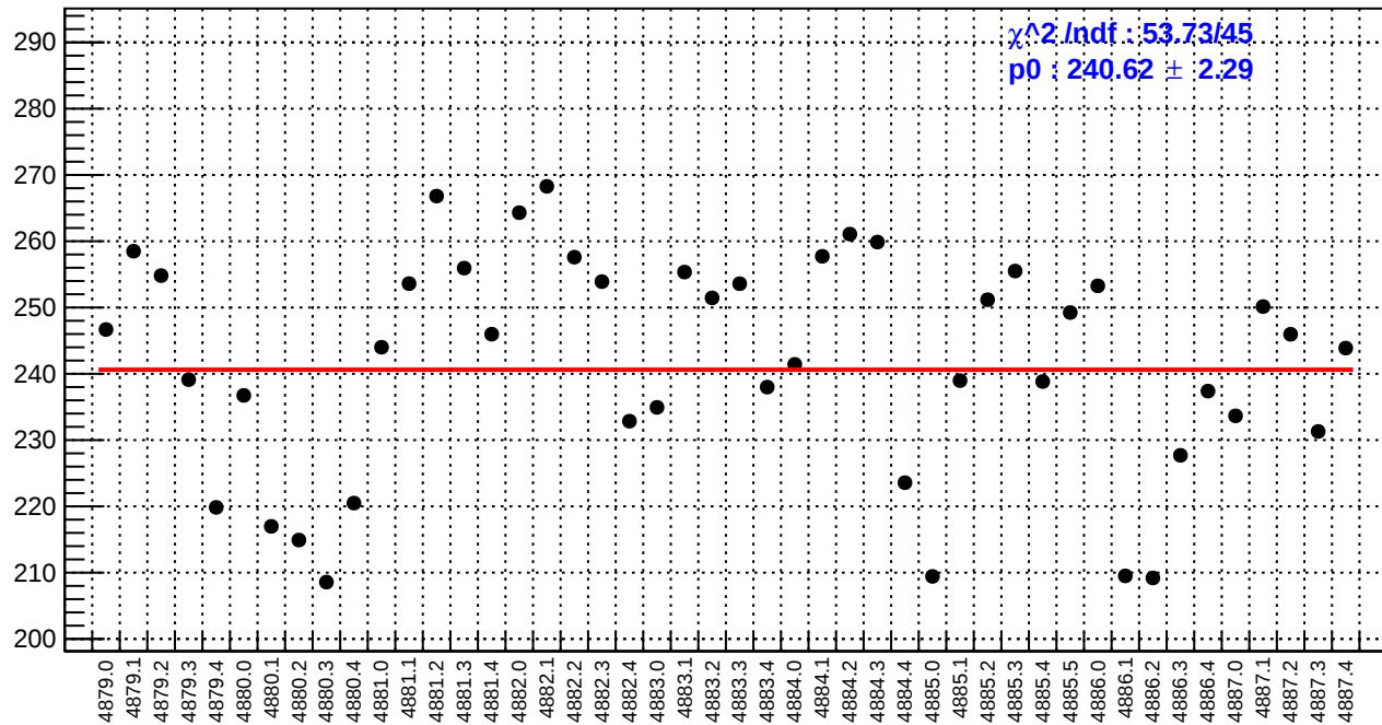
slug89: asym_bcm_an_ds.rms/ppm
