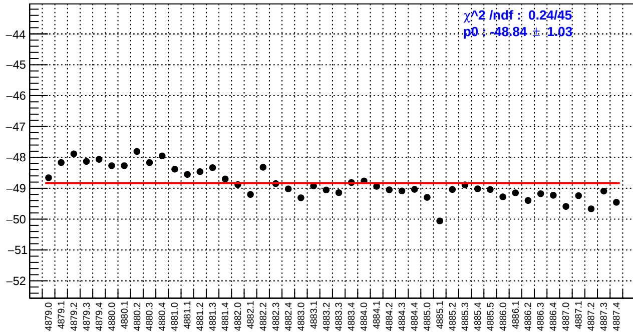
slug89: us_avg_bpm12X/(ppb/nm)
