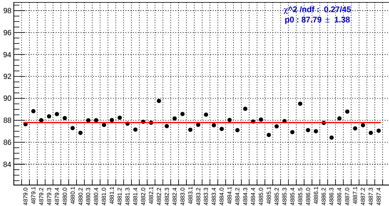
slug89: reg_asym_us_avg.rms/ppm
