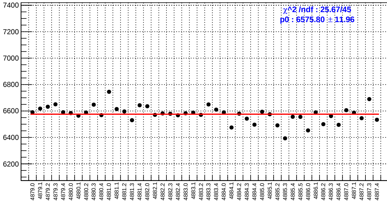
slug89: reg_asym_atr1l2_dd.rms/ppm
