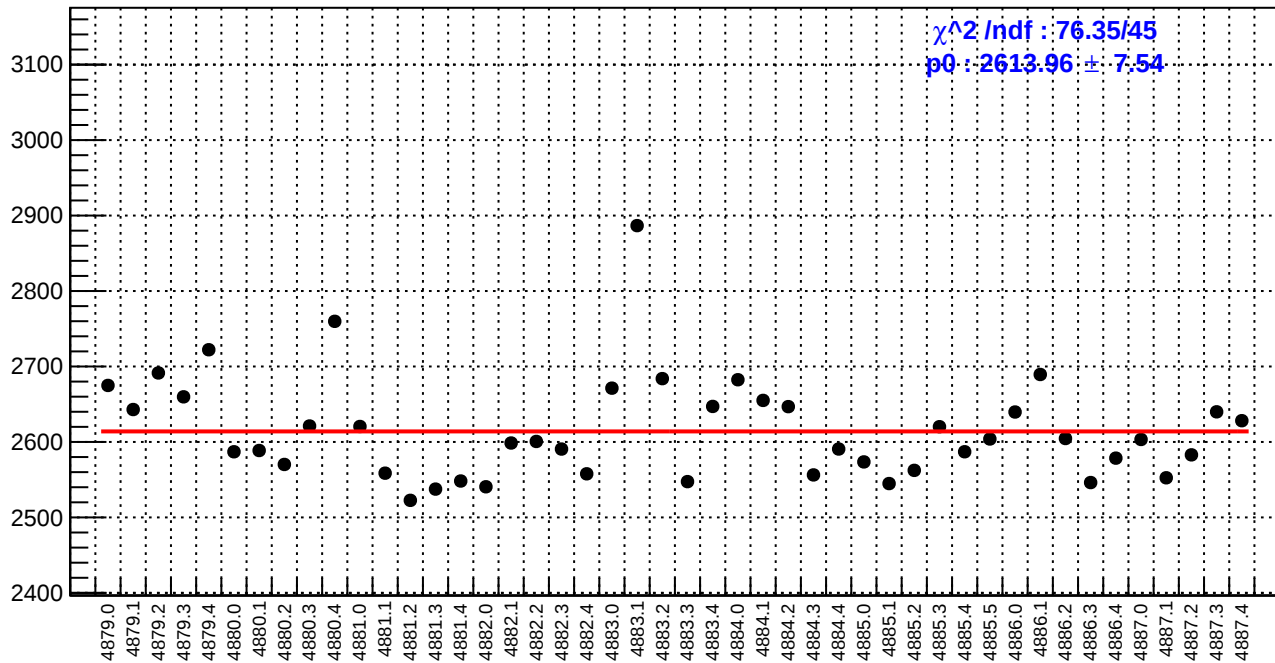
slug89: diff_bpm4aY.rms/nm
