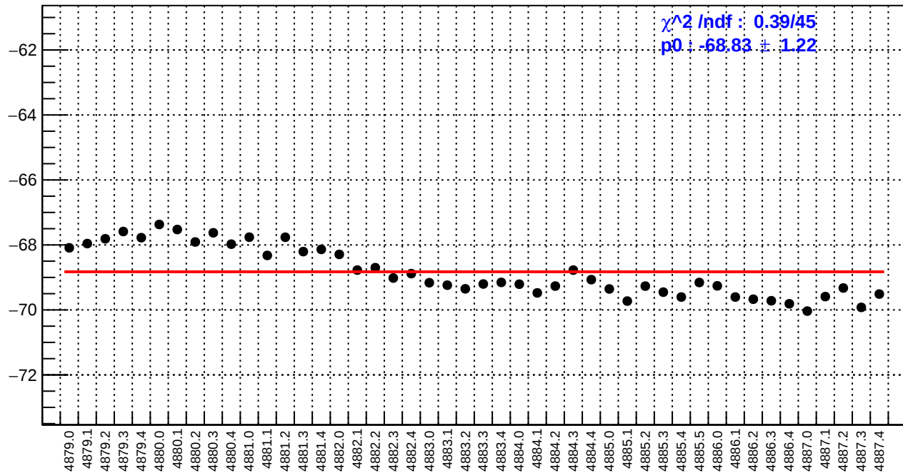
slug89: usl_bpm4eX/(ppb/nm)
