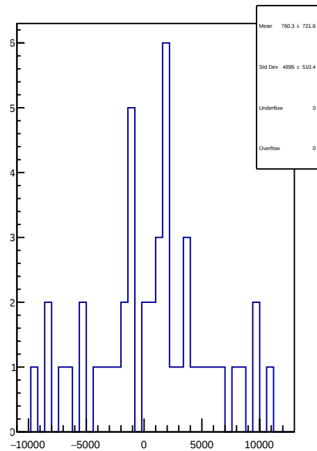
slug89: 1D Corr asym_at2_dd.mean/ppb-reg_asym_at2_dd.mean/ppb
