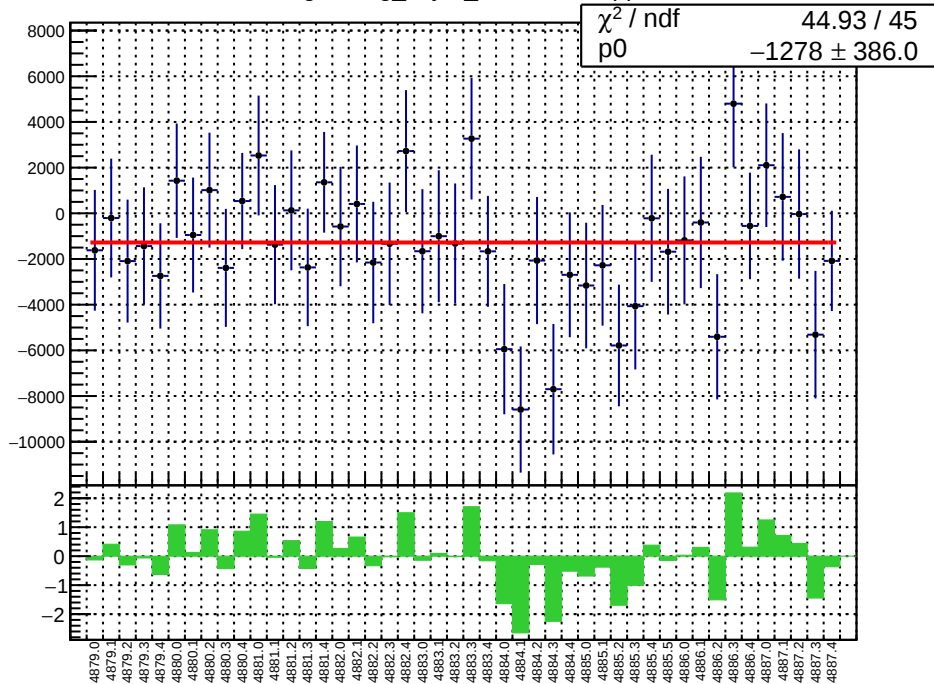
slug89: reg_asym_sam5.mean/ppb
