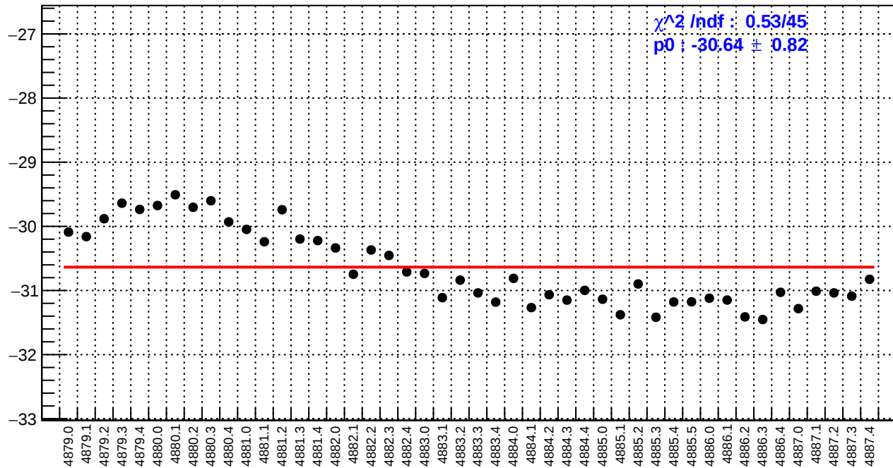
slug89: ds_avg_bpm4eX/(ppb/nm)
