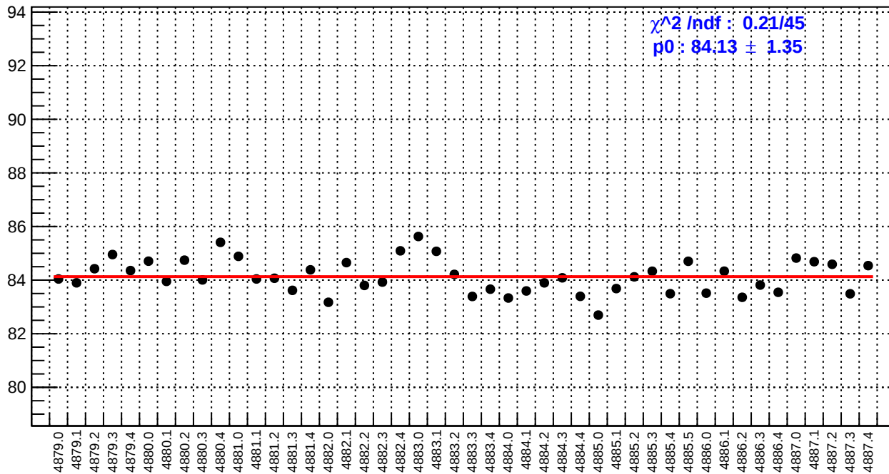
slug89: reg_asym_us_dd.rms/ppm
