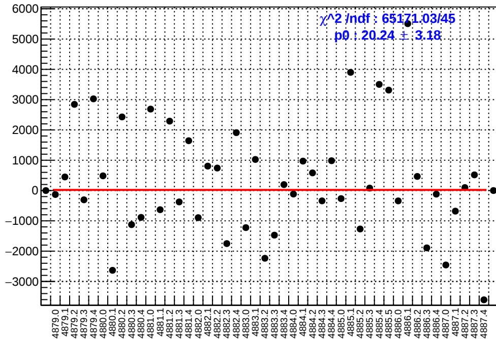
slug89: asym_atl1r2_avg.mean/ppb-reg_asym_atl1r2_avg.mean/ppb
