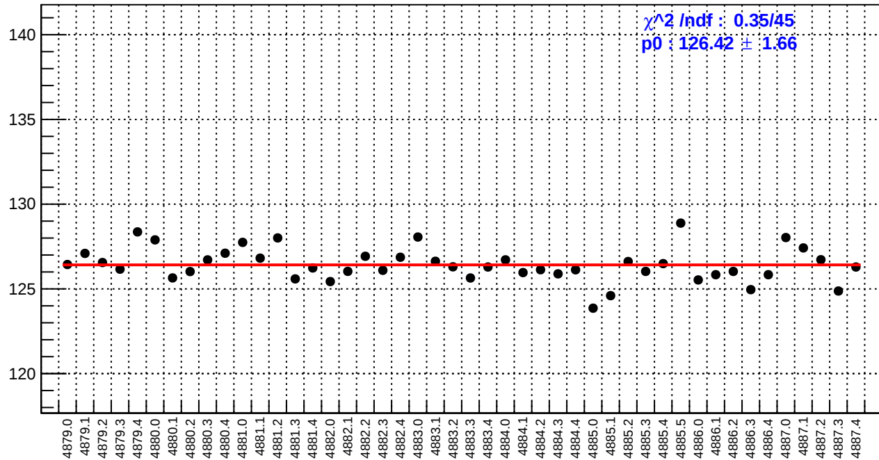
slug89: reg_asym_dsl.rms/ppm
