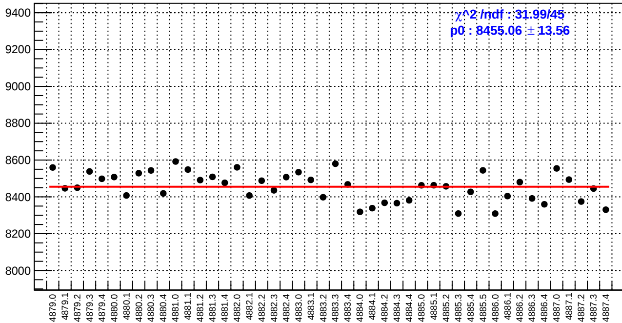
slug89: reg_asym_atr1.rms/ppm
