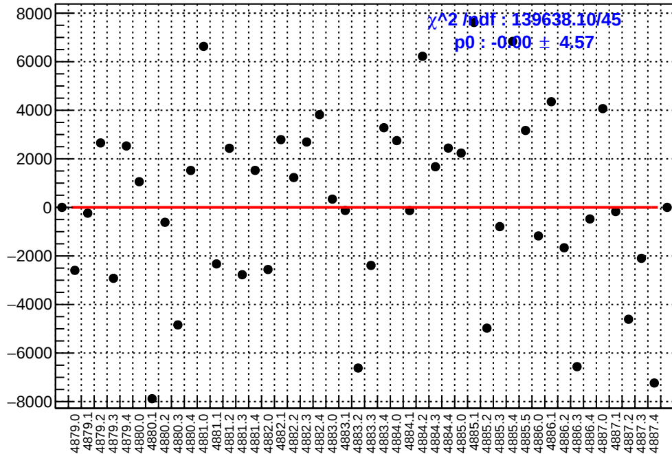
slug89: asym_atr1l2_dd.mean/ppb-reg_asym_atr1l2_dd.mean/ppb
