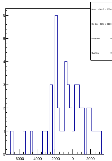
slug89: 1D Corr asym_atr_dd.mean/ppb-reg_asym_atr_dd.mean/ppb
