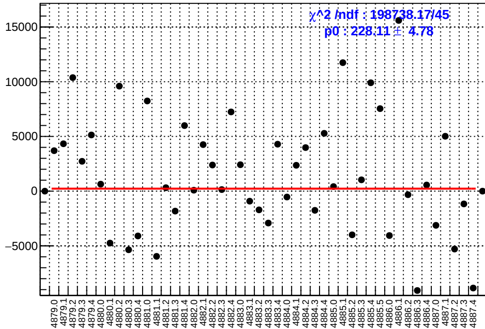
slug89: asym_atr2.mean/ppb-reg_asym_atr2.mean/ppb
