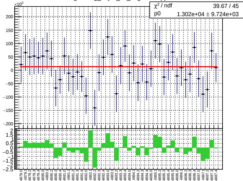
slug89: reg_asym_atl_avg.mean/ppb
