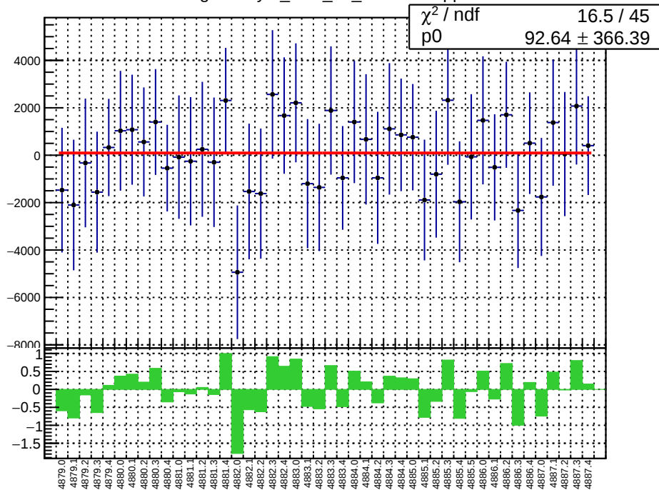
slug89: asym_bcm_an_ds3.mean/ppb
