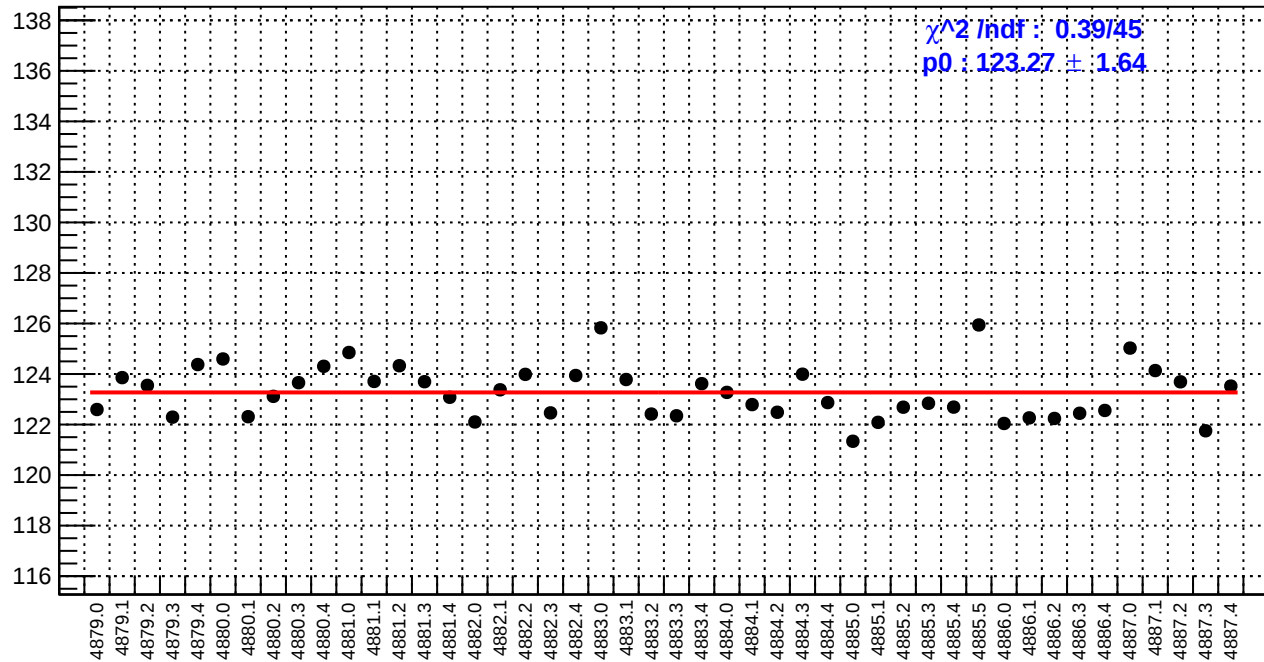
slug89: reg_asym_usl.rms/ppm
