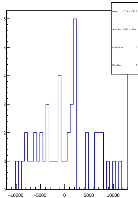
slug89: 1D Corr asym_atl2.mean/ppb-reg_asym_atl2.mean/ppb
