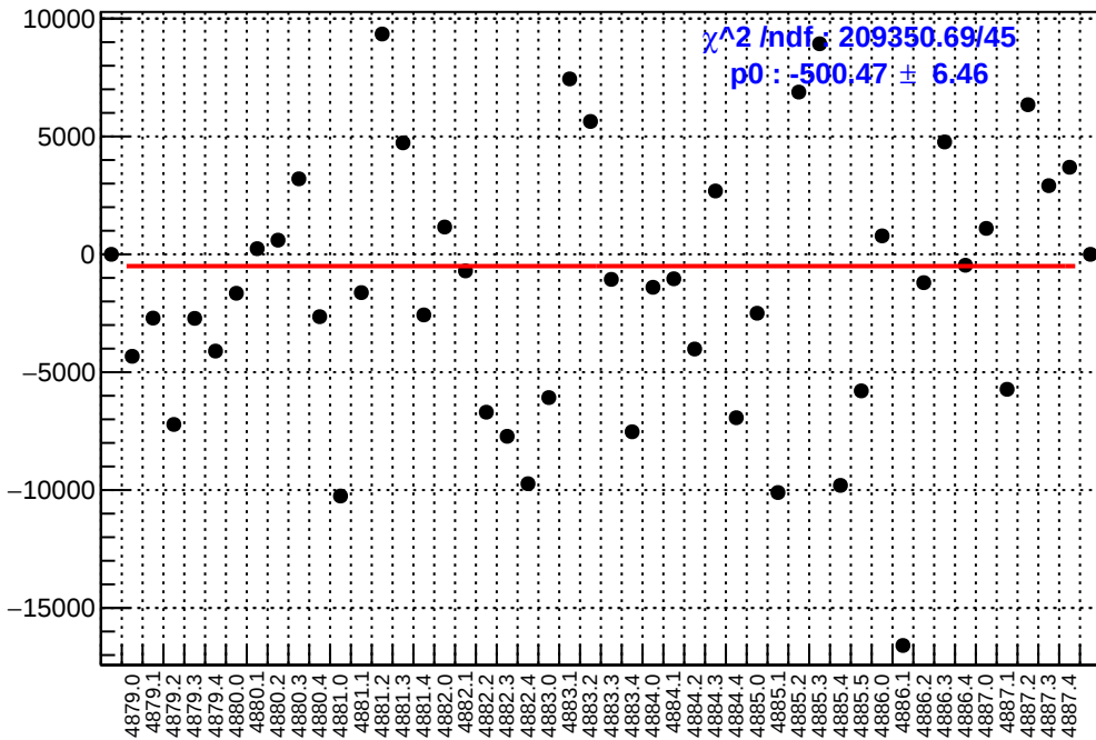
slug89: asym_sam5.mean/ppb-reg_asym_sam5.mean/ppb
