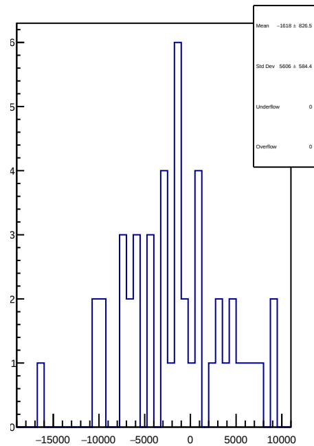
slug89: 1D Corr asym_sam5.mean/ppb-reg_asym_sam5.mean/ppb
