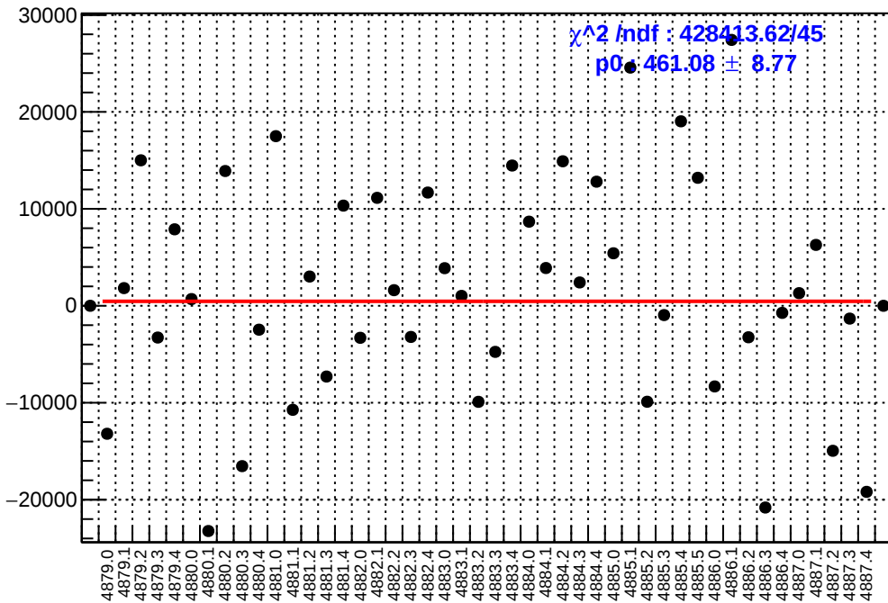
slug89: asym_sam7.mean/ppb-reg_asym_sam7.mean/ppb
