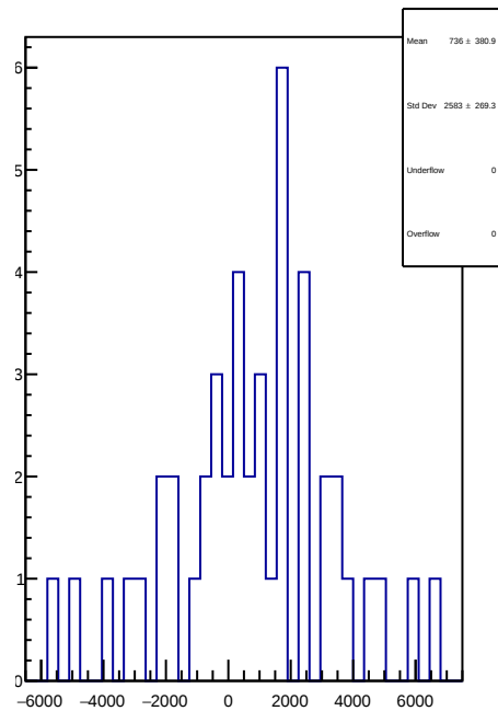
slug89: 1D Corr asym_us_avg.mean/ppb-reg_asym_us_avg.mean/ppb
