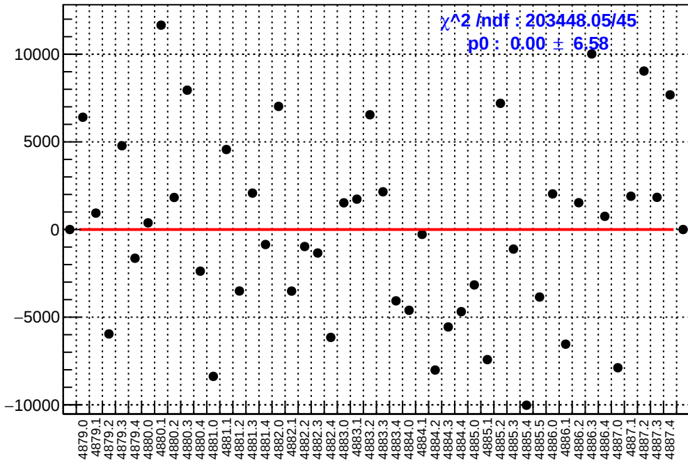
slug89: asym_atl2.mean/ppb-reg_asym_atl2.mean/ppb
