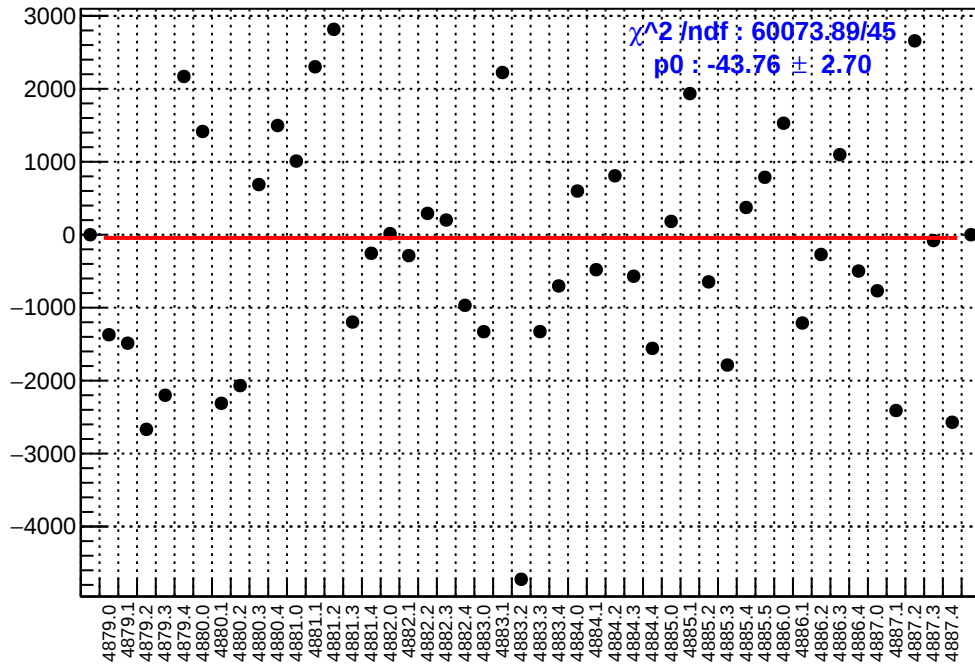
slug89: asym_at1_avg.mean/ppb-reg_asym_at1_avg.mean/ppb
