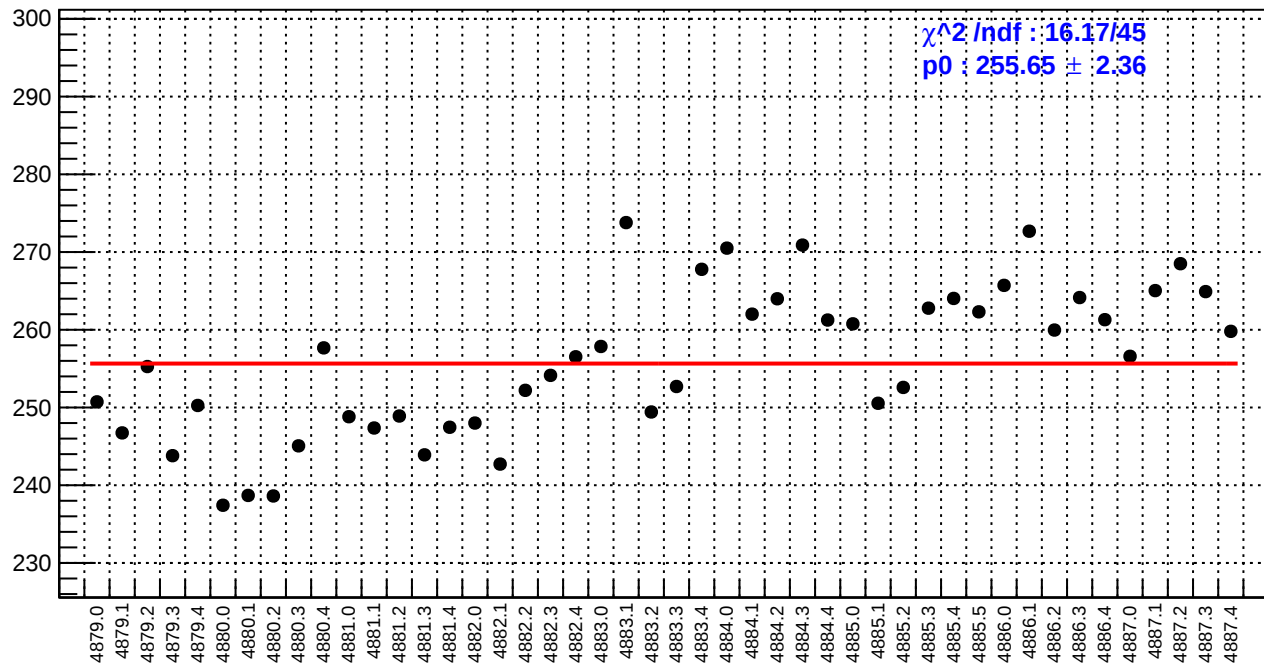
slug89: reg_asym_sam5.rms/ppm
