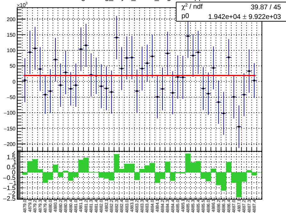
slug89: reg_asym_atr1l2_avg.mean/ppb
