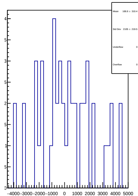
slug89: 1D Corr asym_atr1l2_avg.mean/ppb-reg_asym_atr1l2_avg.mean/ppb
