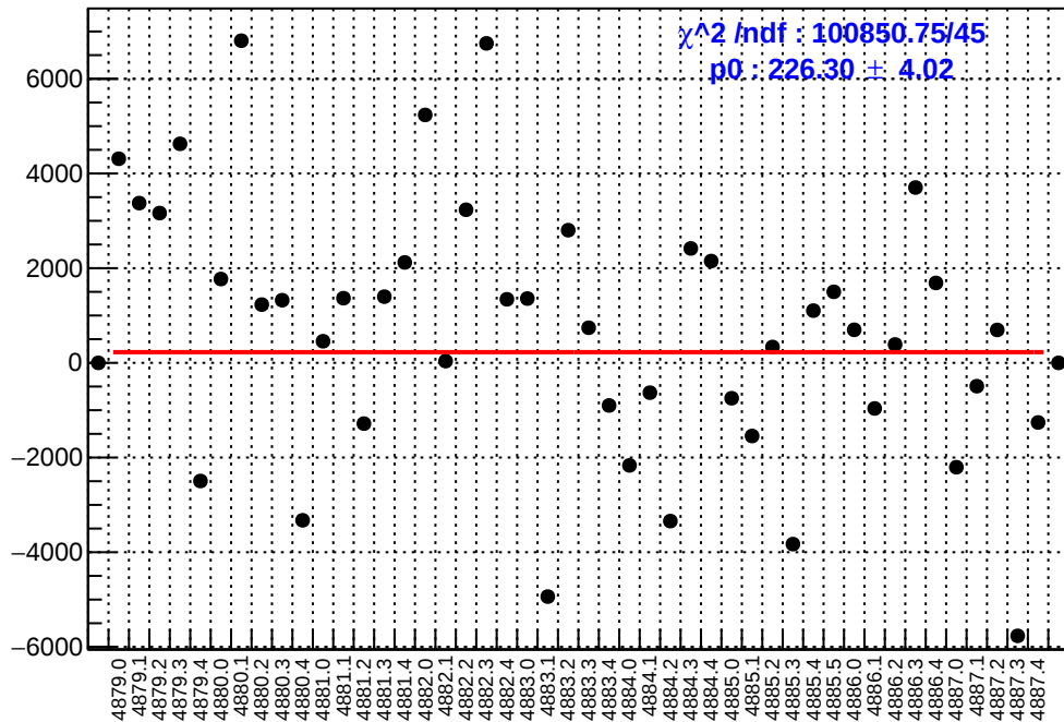
slug89: asym_ds_avg.mean/ppb-reg_asym_ds_avg.mean/ppb
