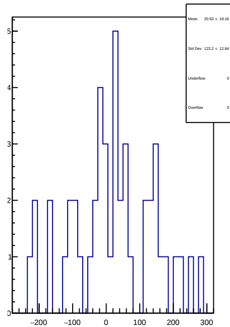
slug89: 1D Corr asym_left_dd.mean/ppb-reg_asym_left_dd.mean/ppb
