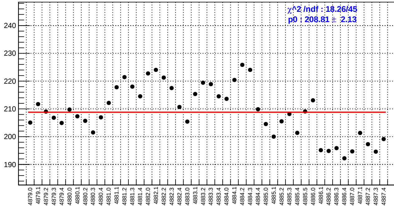
slug89: asym_bcm_an_us.rms/ppm
