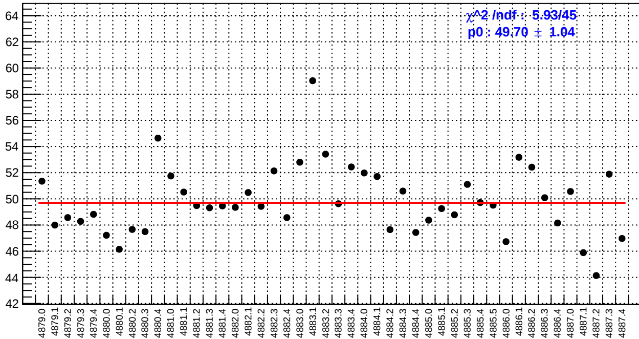
slug89: dsl_bpm4aX/(ppb/nm)
