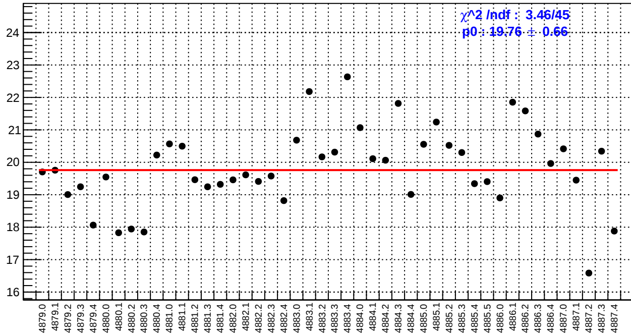
slug89: us_avg_bpm4aX/(ppb/nm)
