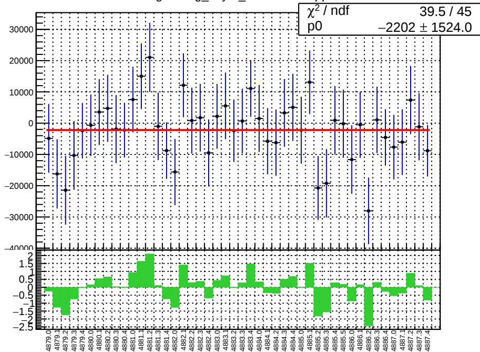
slug89: reg_asym_sam4.mean/ppb
