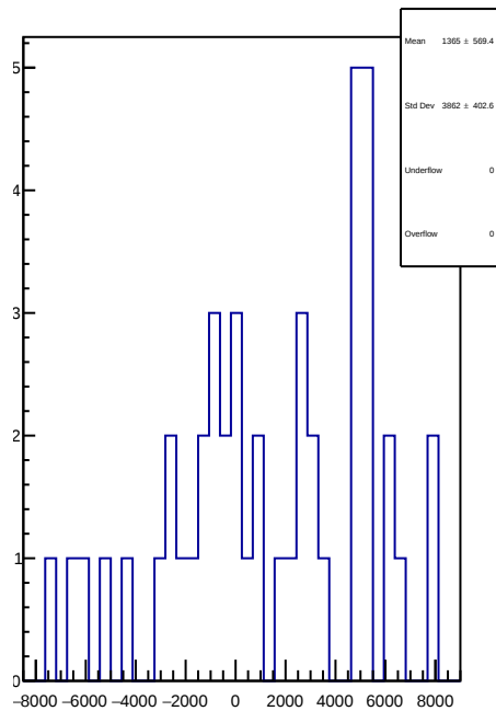
slug89: 1D Corr asym_dsr.mean/ppb-reg_asym_dsr.mean/ppb
