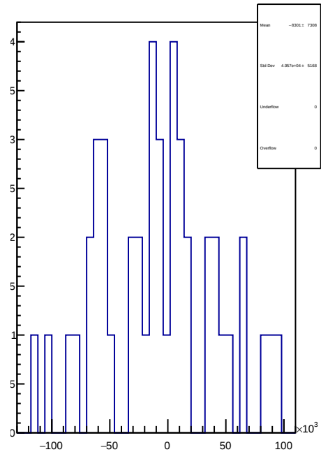
slug89: 1D Corr asym_sam3.mean/ppb-reg_asym_sam3.mean/ppb
