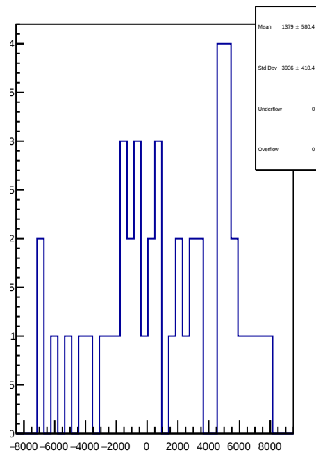
slug89: 1D Corr asym_right_avg.mean/ppb-reg_asym_right_avg.mean/ppb
