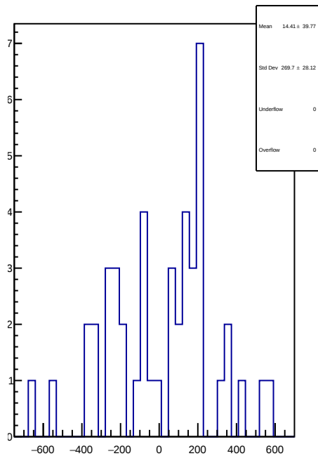
slug89: 1D Corr asym_right_dd.mean/ppb-reg_asym_right_dd.mean/ppb
