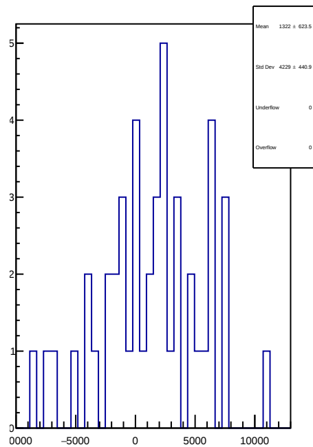
slug89: 1D Corr asym_sam1.mean/ppb-reg_asym_sam1.mean/ppb
