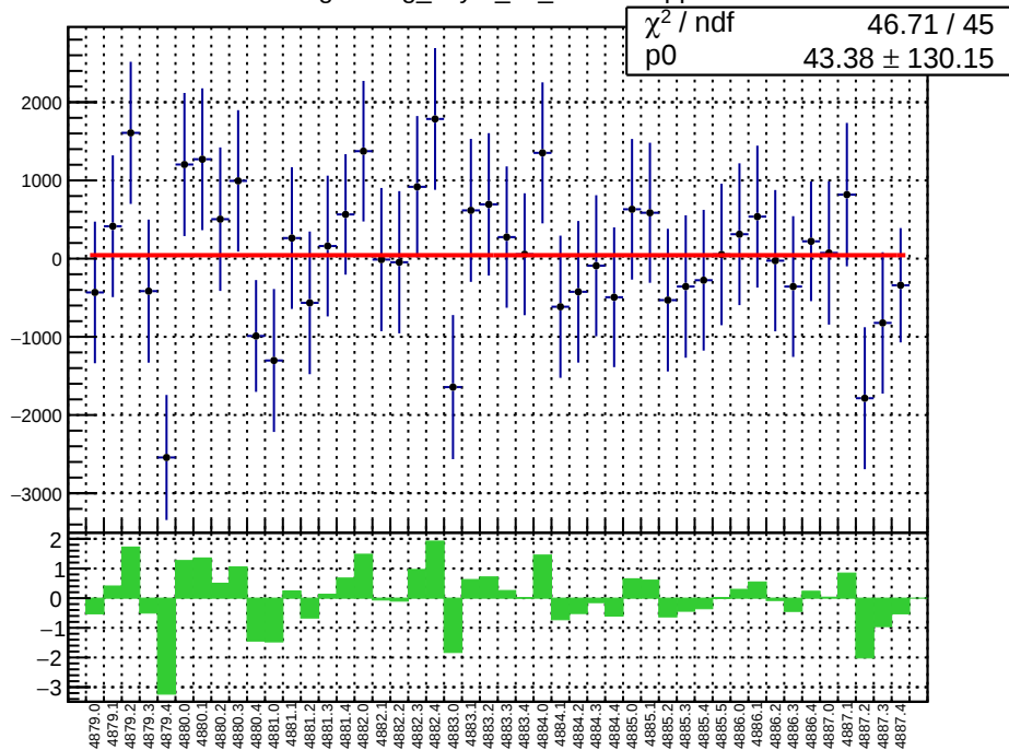
slug89: reg_asym_ds_dd.mean/ppb
