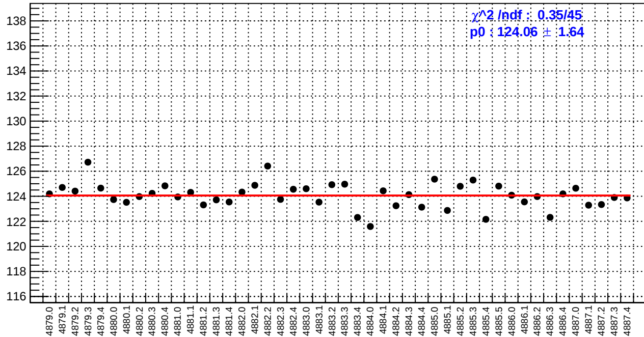
slug89: reg_asym_dsr.rms/ppm
