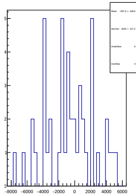
slug89: 1D Corr asym_us_dd.mean/ppb-reg_asym_us_dd.mean/ppb
