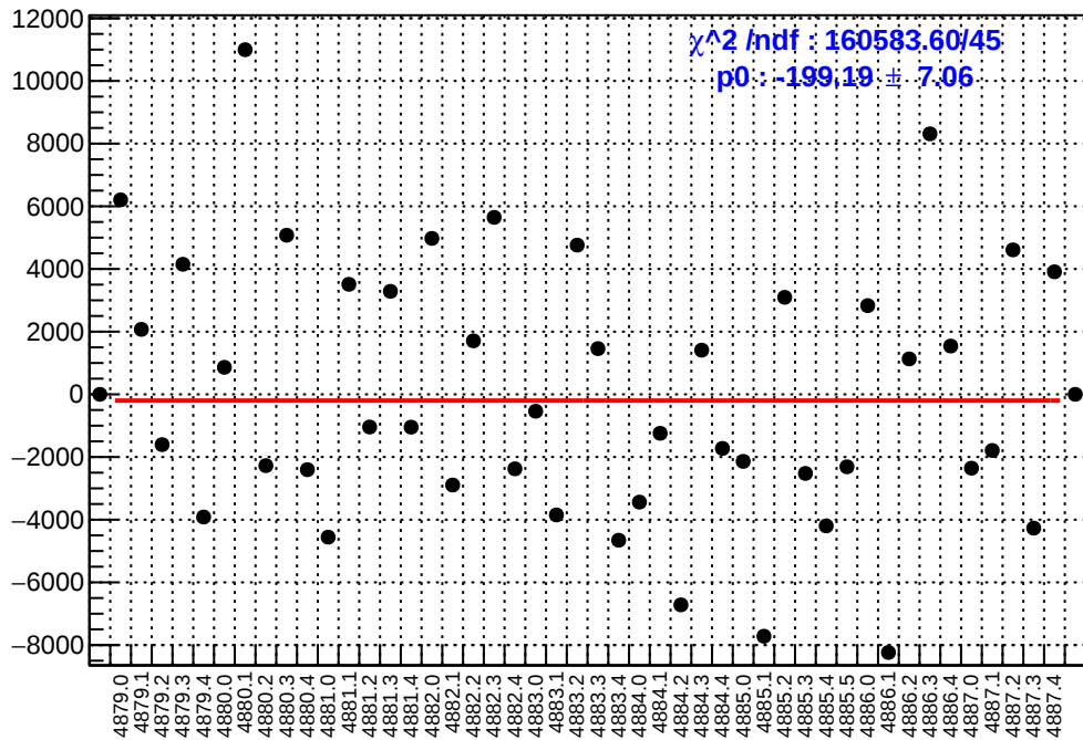
slug89: asym_dsl.mean/ppb-reg_asym_dsl.mean/ppb
