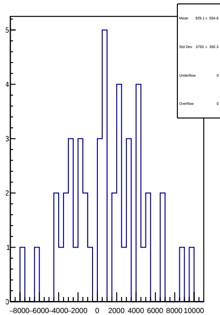
slug89: 1D Corr asym_atr_avg.mean/ppb-reg_asym_atr_avg.mean/ppb
