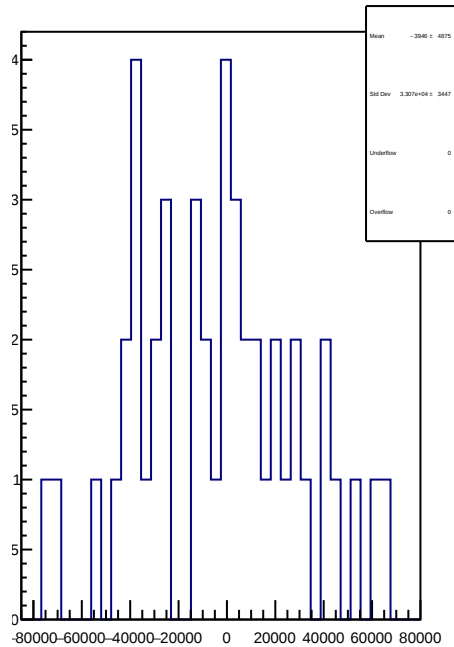
slug89: 1D Corr asym_sam2.mean/ppb-reg_asym_sam2.mean/ppb
