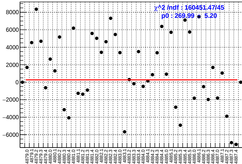
slug89: asym_usr.mean/ppb-reg_asym_usr.mean/ppb
