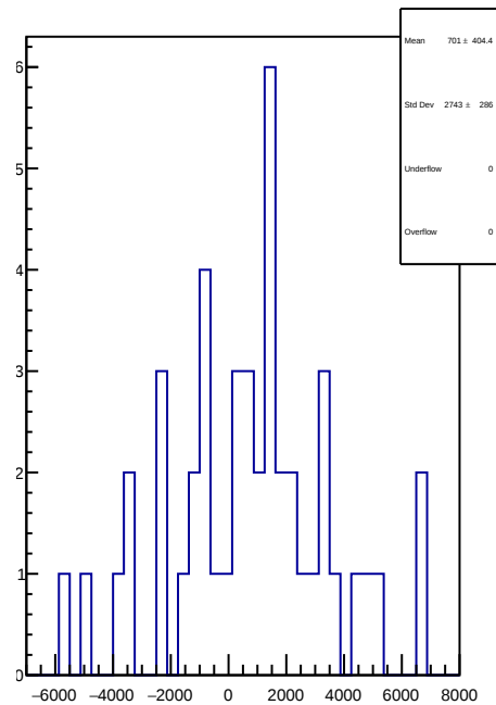
slug89: 1D Corr asym_ds_avg.mean/ppb-reg_asym_ds_avg.mean/ppb
