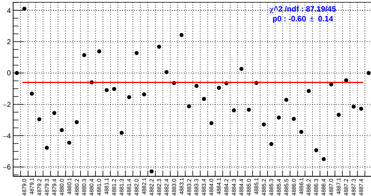
slug89: right_avg_bpm4aY/(ppb/nm)
