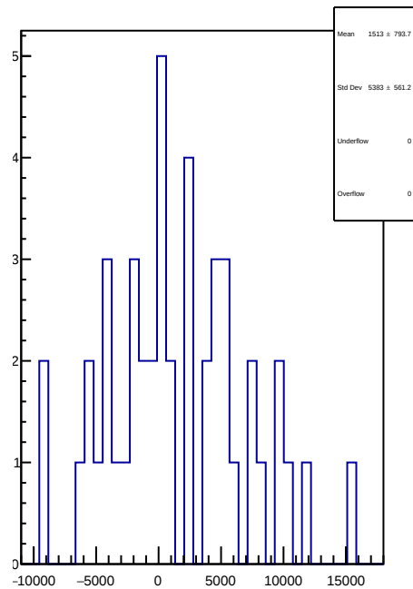
slug89: 1D Corr asym_atr2.mean/ppb-reg_asym_atr2.mean/ppb
