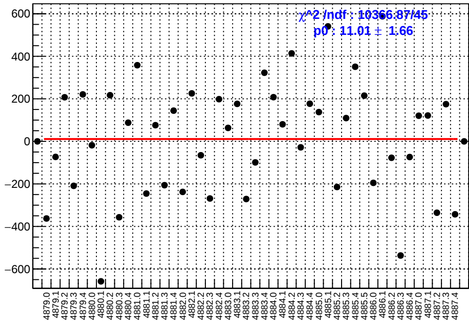
slug89: asym_right_dd.mean/ppb-reg_asym_right_dd.mean/ppb
