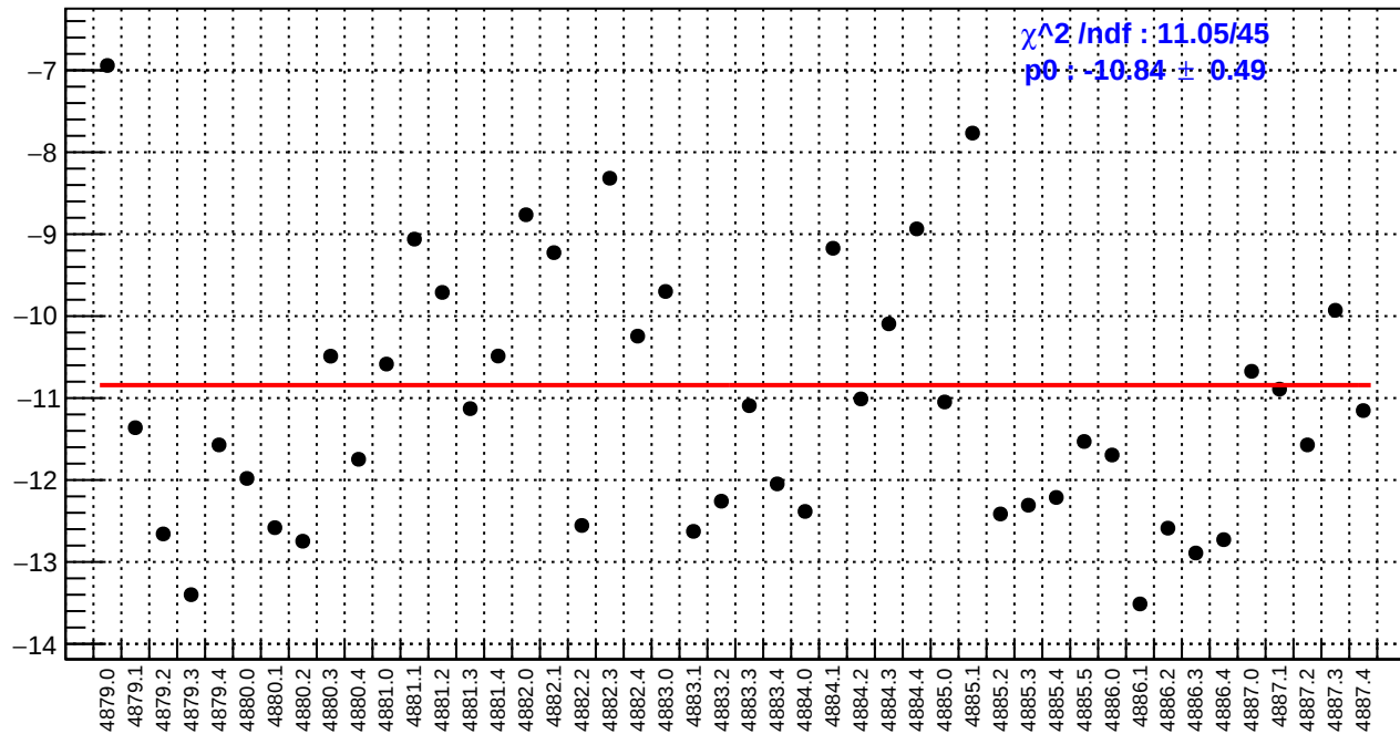
slug89: ds_avg_bpm4aY/(ppb/nm)
