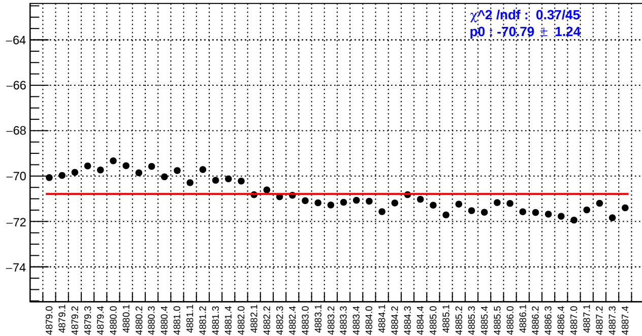
slug89: left_avg_bpm4eX/(ppb/nm)
