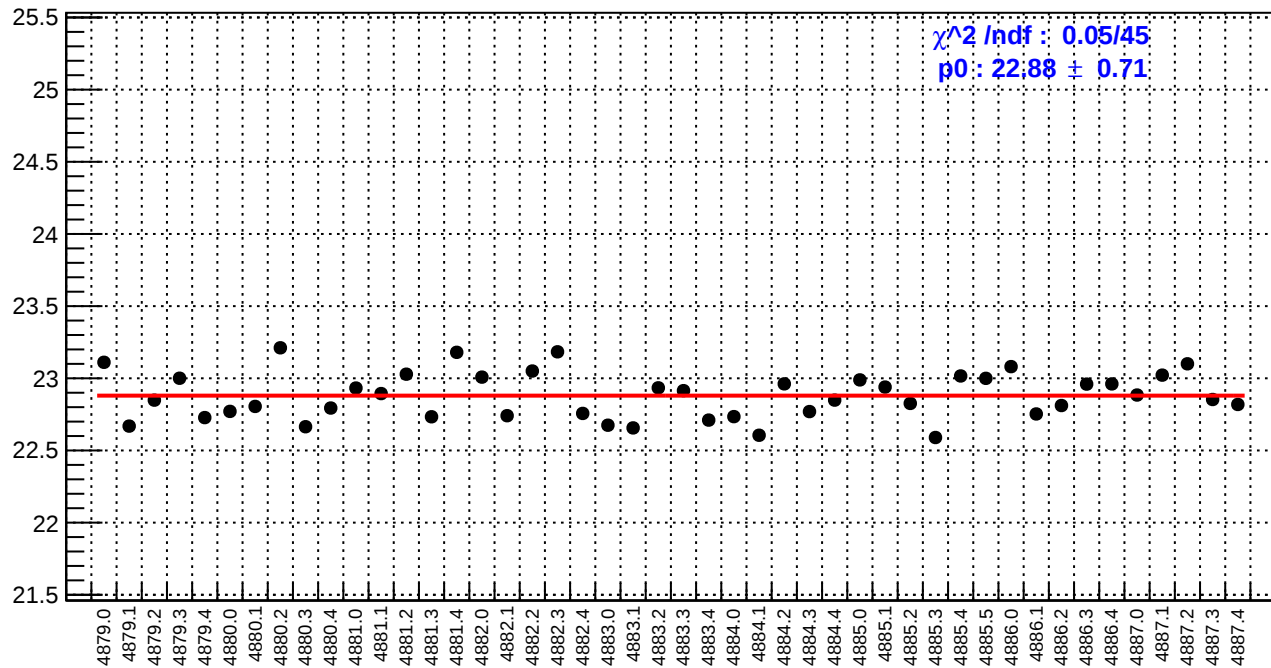
slug89: reg_asym_left_dd.rms/ppm
