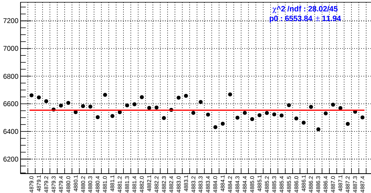
slug89: reg_asym_atr_dd.rms/ppm
