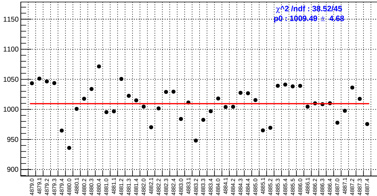
slug89: reg_asym_sam4.rms/ppm
