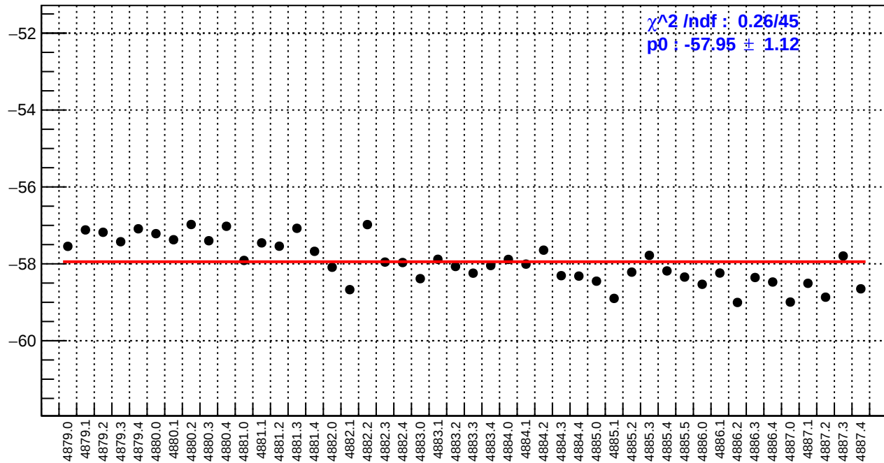
slug89: right_avg_bpm12X/(ppb/nm)
