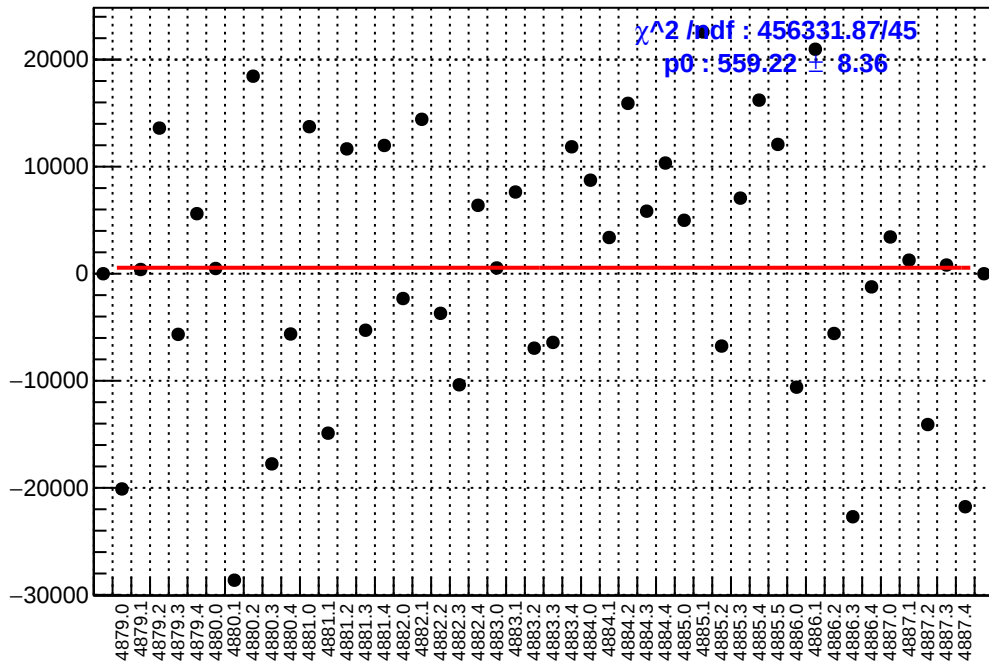
slug89: asym_sam6.mean/ppb-reg_asym_sam6.mean/ppb
