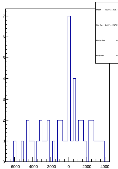
slug89: 1D Corr asym_atl_dd.mean/ppb-reg_asym_atl_dd.mean/ppb
