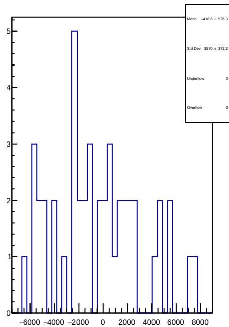
slug89: 1D Corr asym_atl_avg.mean/ppb-reg_asym_atl_avg.mean/ppb
