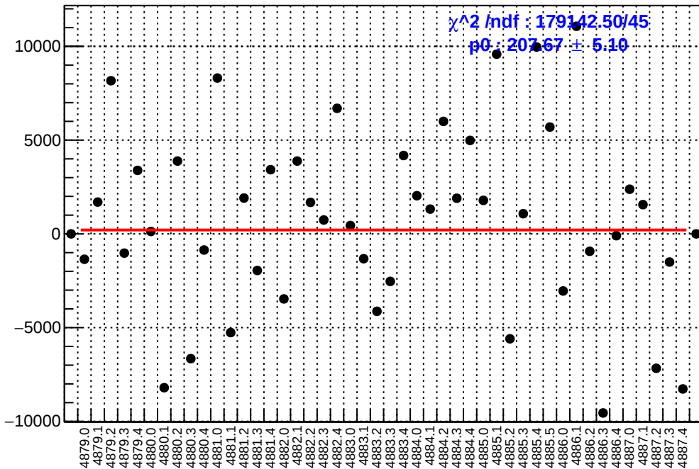
slug89: asym_at2_dd.mean/ppb-reg_asym_at2_dd.mean/ppb
