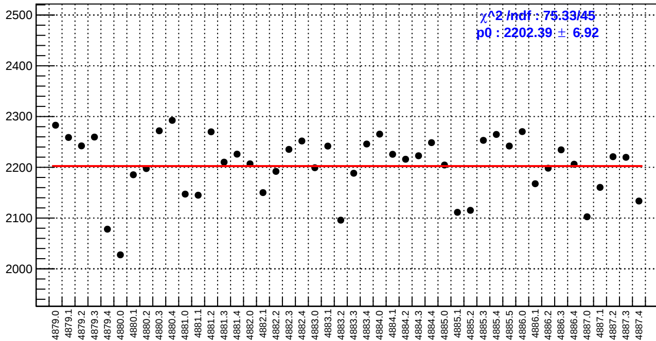
slug89: reg_asym_sam2.rms/ppm
