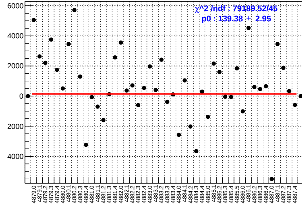
slug89: asym_at2_avg.mean/ppb-reg_asym_at2_avg.mean/ppb
