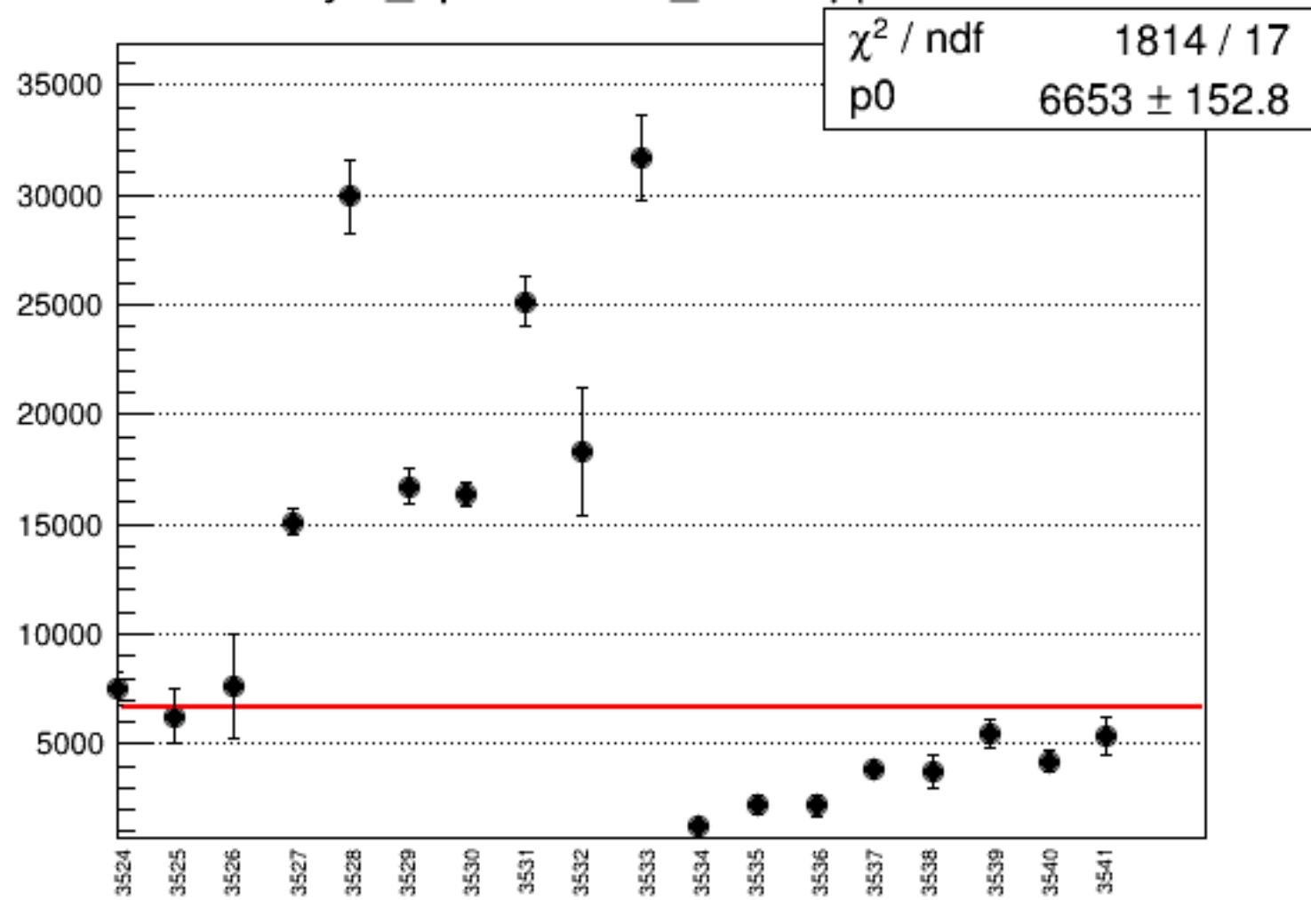
asym_bpm2i01WS_mean/ppb vs run
