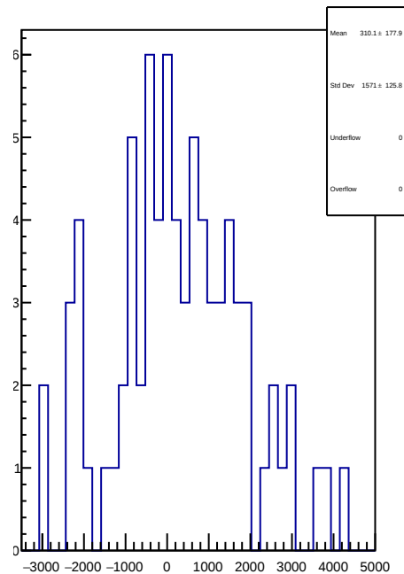
slug9-Left: 1D Corr asym_ds_dd.mean/ppb-reg_asym_ds_dd.mean/ppb
