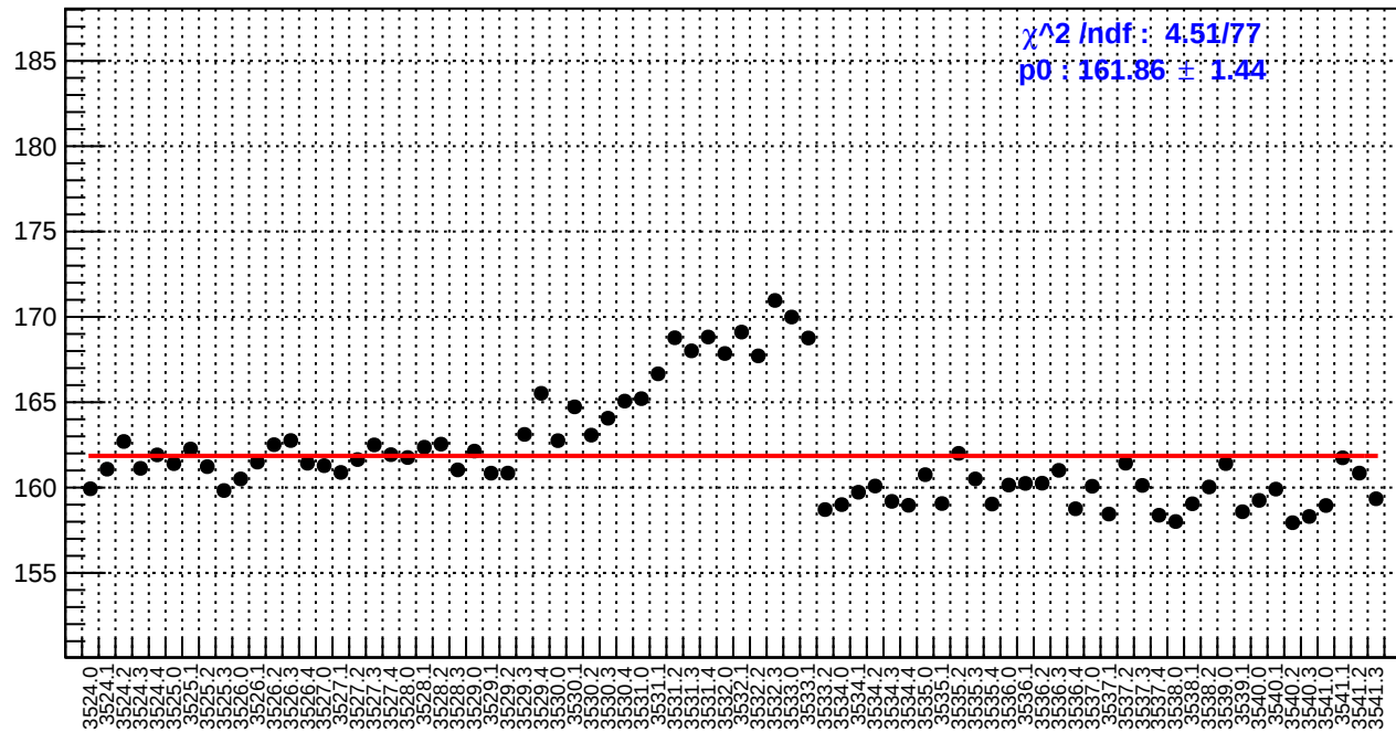
slug9-Left: reg_asym_usl.rms/ppm
