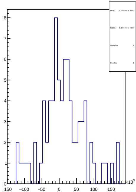
slug9-Left: 1D Corr asym_sam2.mean/ppb-reg_asym_sam2.mean/ppb
