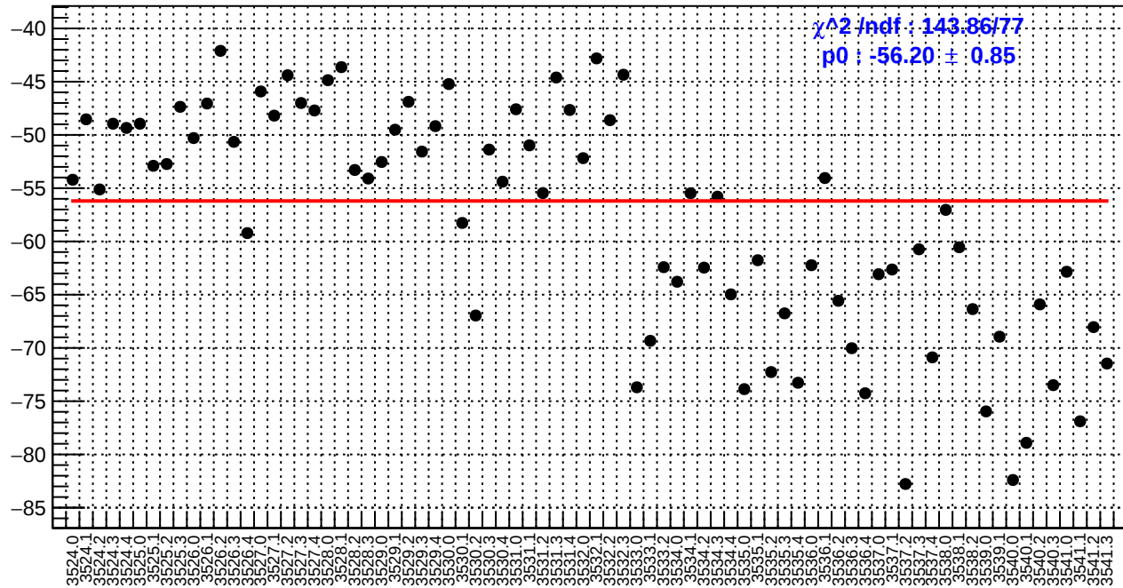
slug9-Left: dsr_bpm4eX/(ppb/nm)
