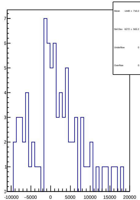
slug9-Left: 1D Corr asym_dsl.mean/ppb-reg_asym_dsl.mean/ppb
