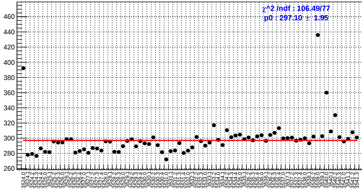
slug9-Left: reg_asym_sam7.rms/ppm
