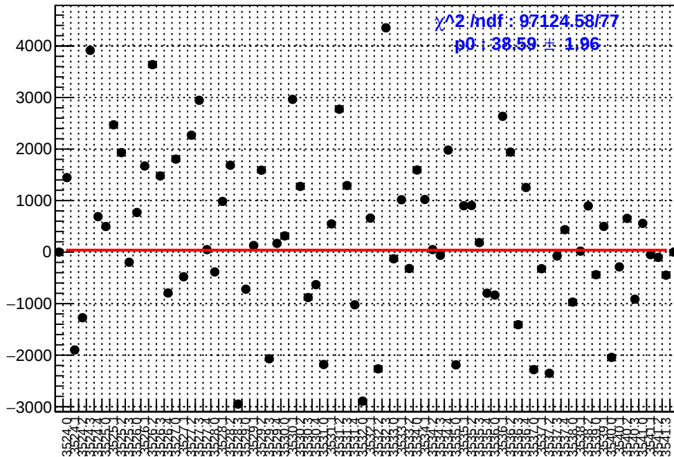
slug9-Left: asym_ds_dd.mean/ppb-reg_asym_ds_dd.mean/ppb
