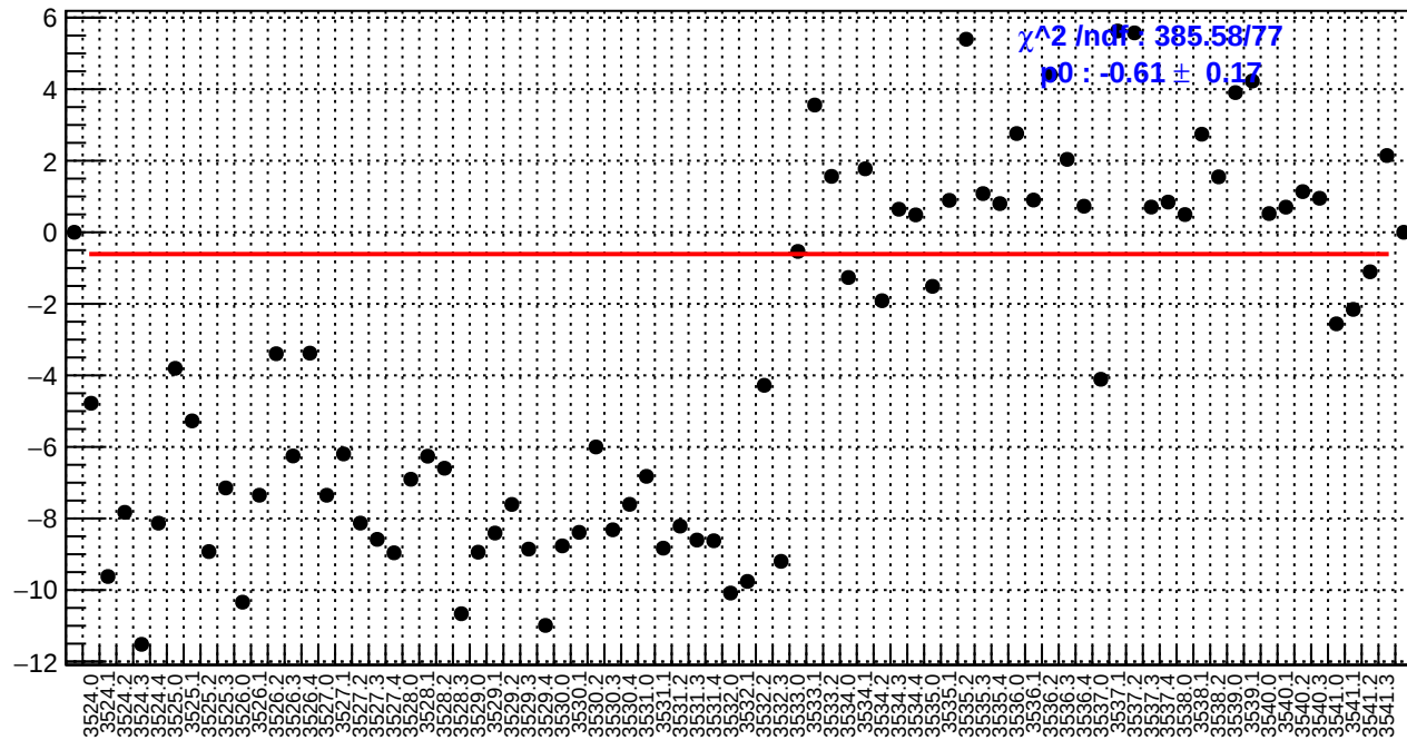
slug9-Left: usr_bpm12X/(ppb/nm)
