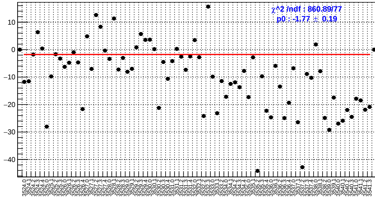
slug9-Left: usr_bpm4aX/(ppb/nm)
