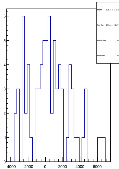
slug9-Left: 1D Corr asym_us_avg.mean/ppb-reg_asym_us_avg.mean/ppb
