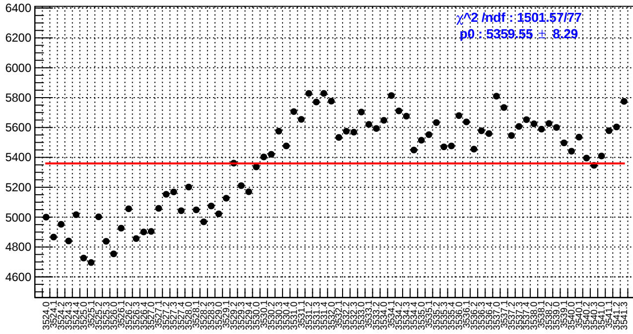
slug9-Left: diff_bpm12X.rms/nm
