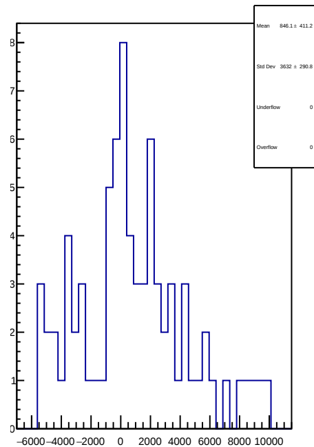
slug9-Left: 1D Corr asym_us_dd.mean/ppb-reg_asym_us_dd.mean/ppb
