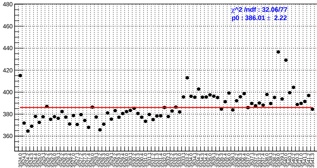
slug9-Left: reg_asym_sam8.rms/ppm
