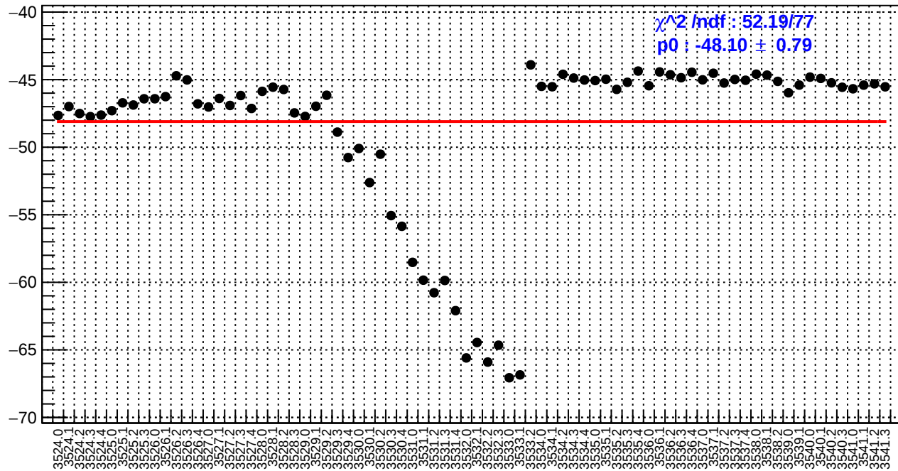
slug9-Left: dsl_bpm12X/(ppb/nm)
