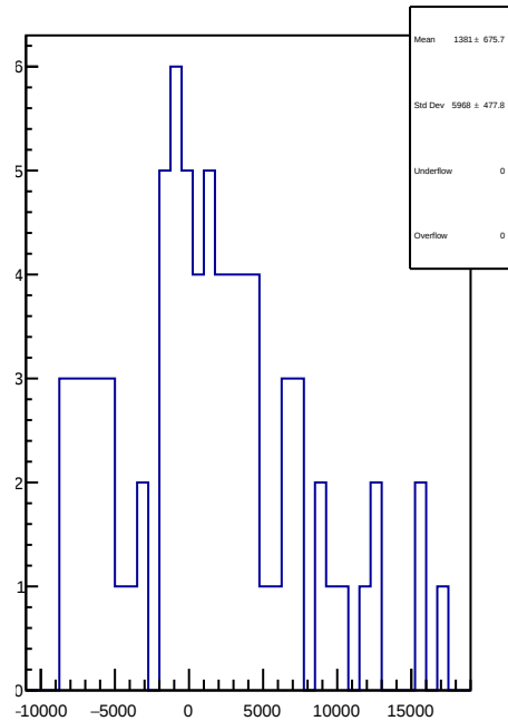
slug9-Left: 1D Corr asym_usl.mean/ppb-reg_asym_usl.mean/ppb
