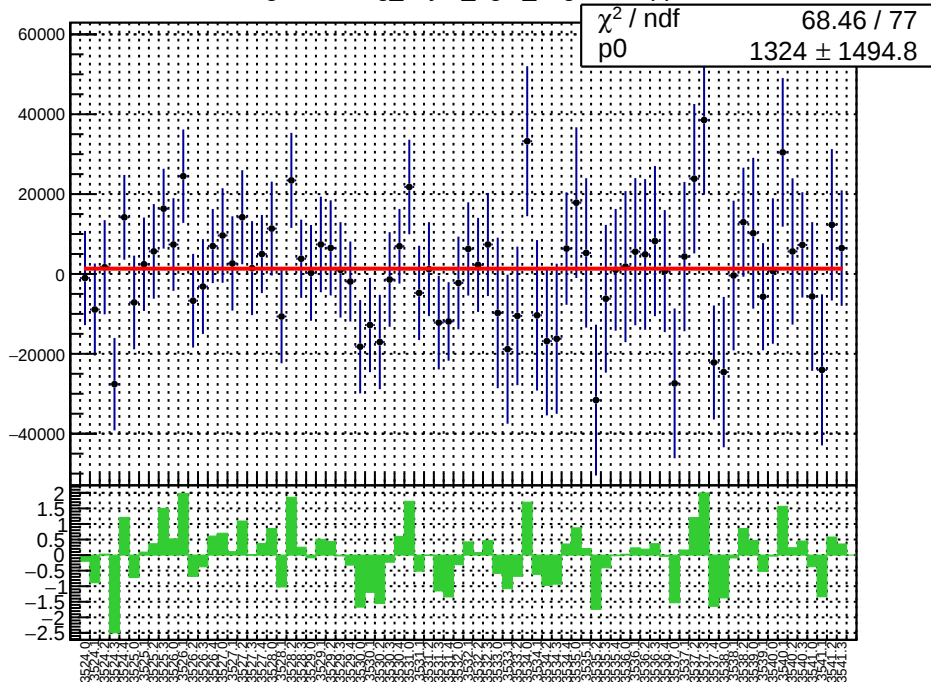
slug9-Left: reg_asym_right_avg.mean/ppb
