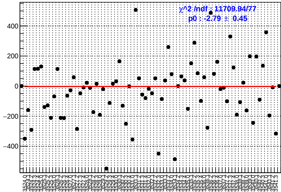
slug9-Left: asym_left_dd.mean/ppb-reg_asym_left_dd.mean/ppb
