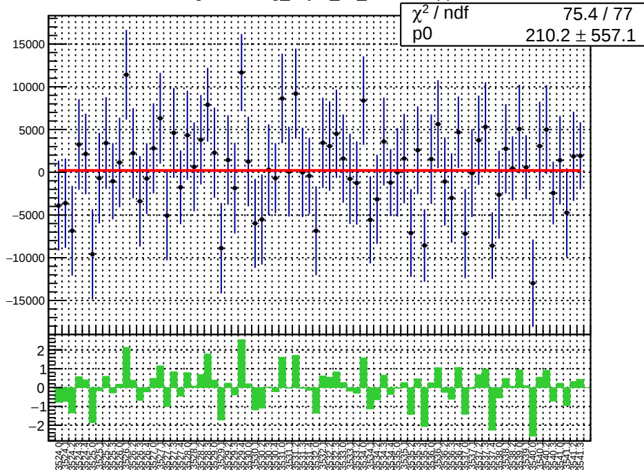
slug9-Left: reg_asym_us_dd.mean/ppb
