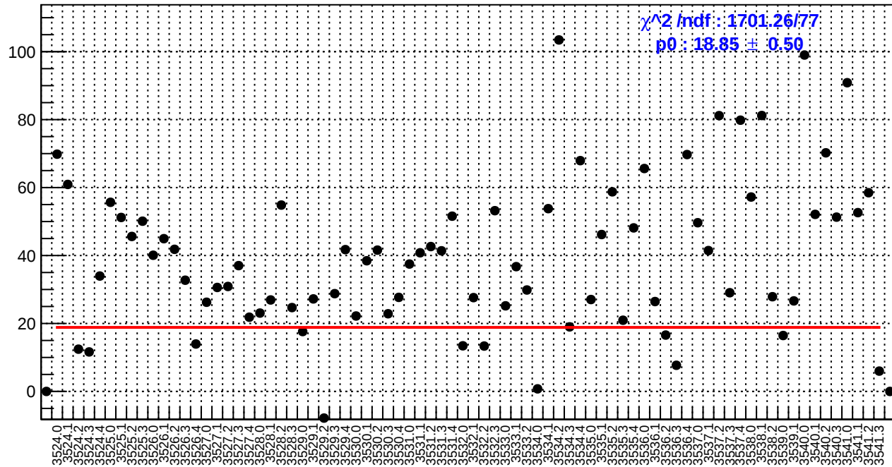
slug9-Left: dsr_bpm4eY/(ppb/nm)
