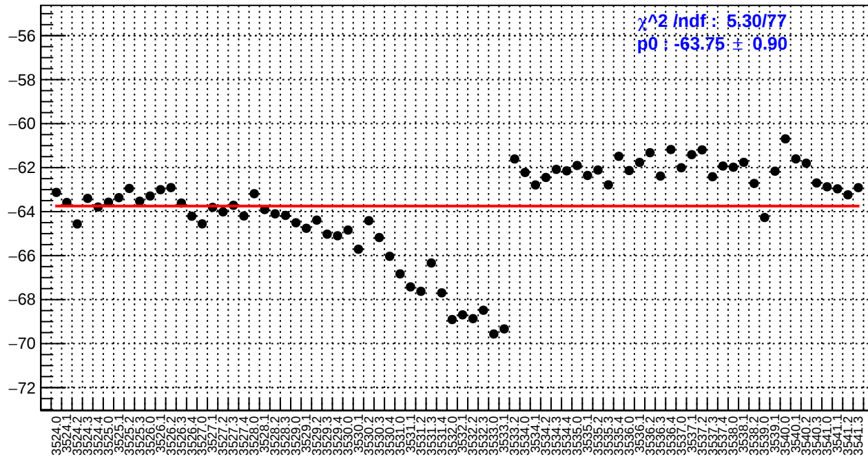
slug9-Left: usl_bpm4eX/(ppb/nm)
