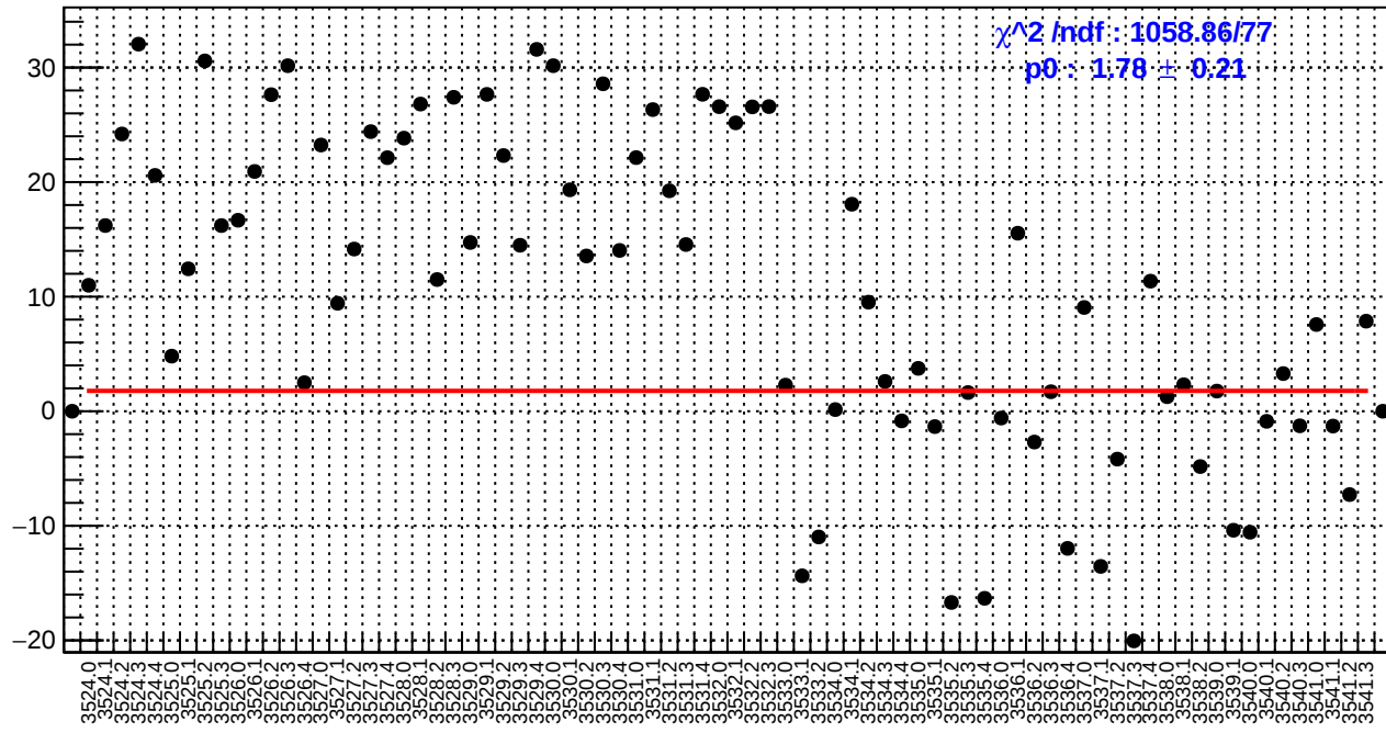
slug9-Left: dsr_bpm12X/(ppb/nm)
