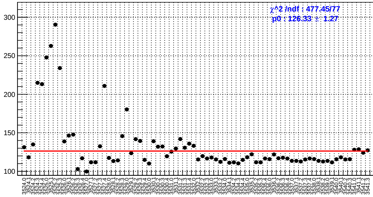
slug9-Left: asym_bcm_an_ds3.rms/ppm
