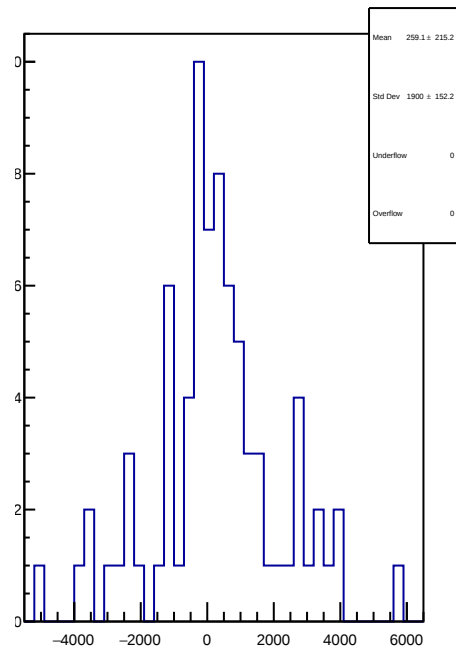
slug9-Left: 1D Corr asym_right_avg.mean/ppb-reg_asym_right_avg.mean/ppb
