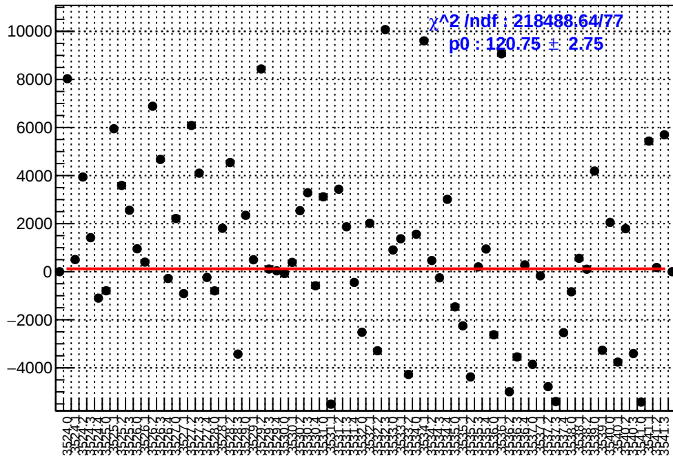
slug9-Left: asym_us_dd.mean/ppb-reg_asym_us_dd.mean/ppb
