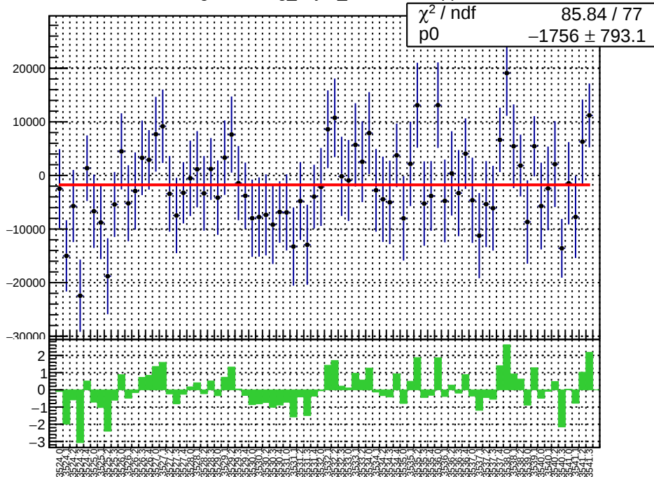
slug9-Left: reg_asym_sam6.mean/ppb
