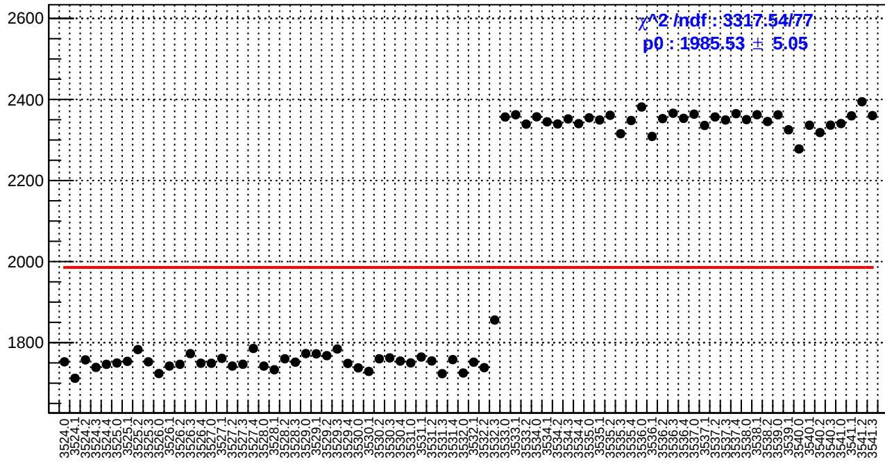
slug9-Left: reg_asym_right_dd.rms/ppm
