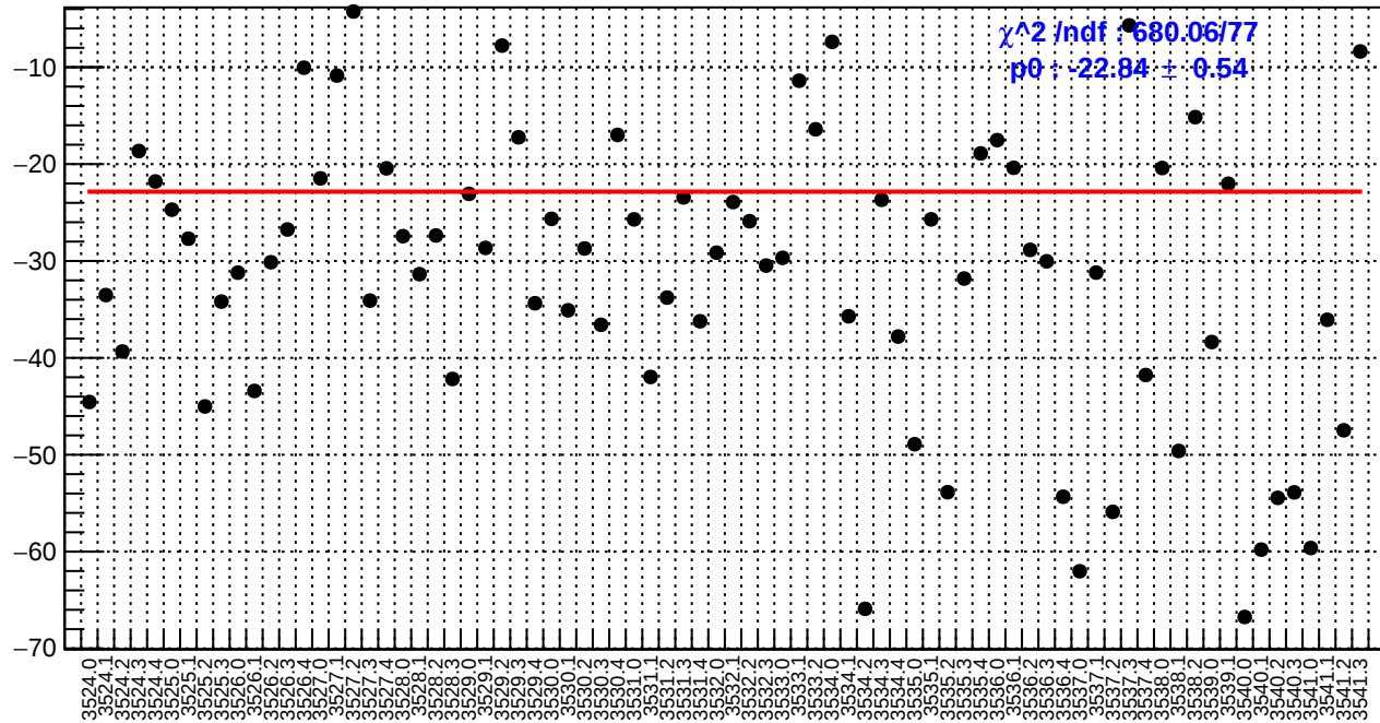
slug9-Left: ds_avg_bpm4aY/(ppb/nm)
