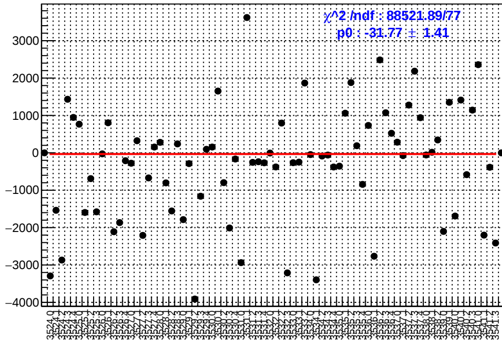
slug9-Left: asym_usr.mean/ppb-reg_asym_usr.mean/ppb
