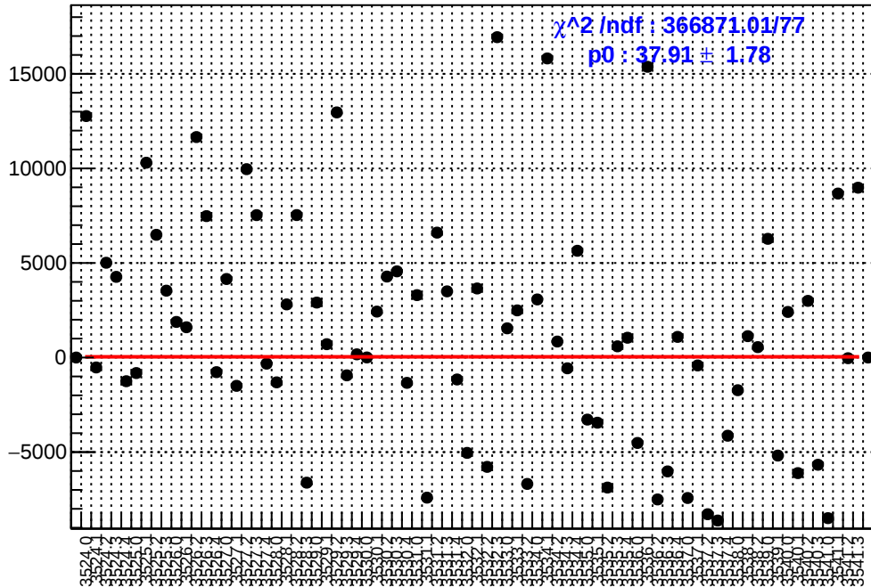
slug9-Left: asym_usl.mean/ppb-reg_asym_usl.mean/ppb
