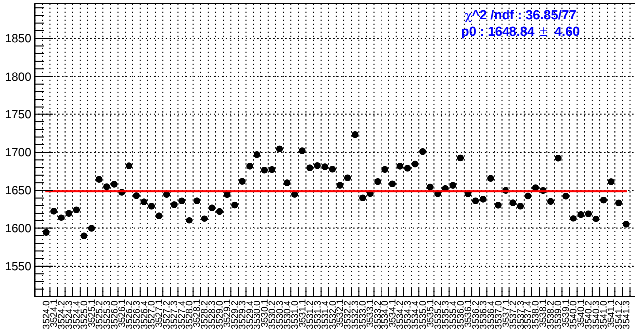
slug9-Left: reg_asym_sam2.rms/ppm
