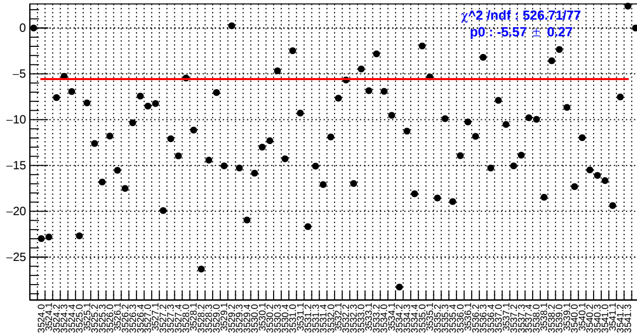
slug9-Left: usr_bpm4eY/(ppb/nm)
