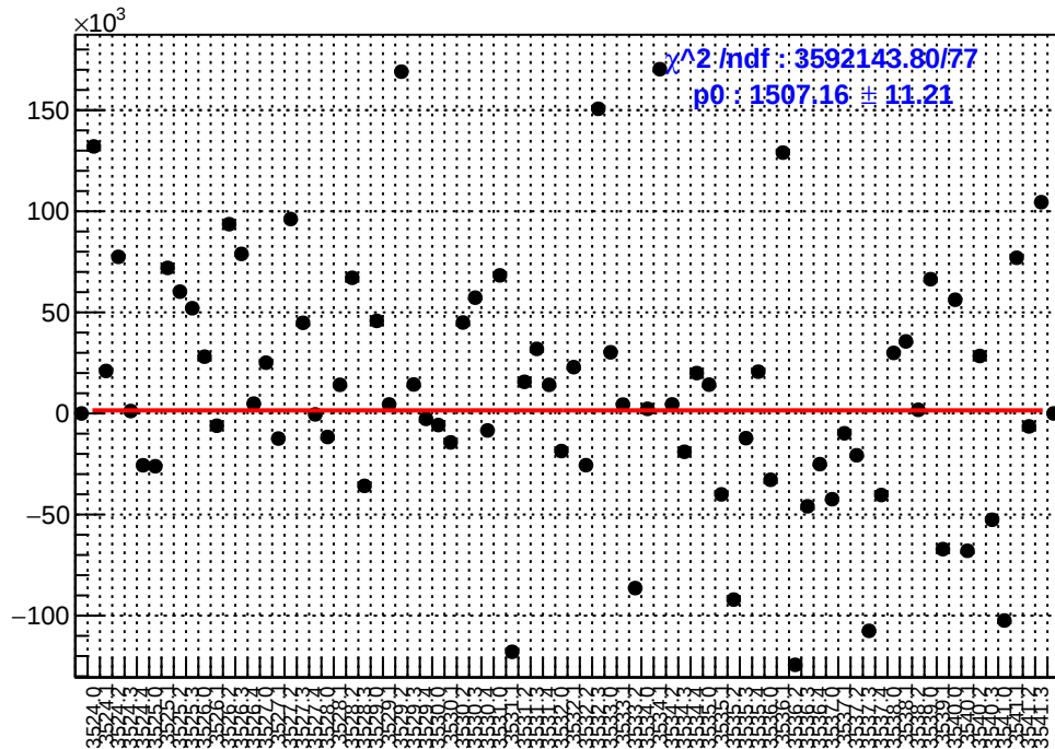
slug9-Left: asym_sam2.mean/ppb-reg_asym_sam2.mean/ppb
