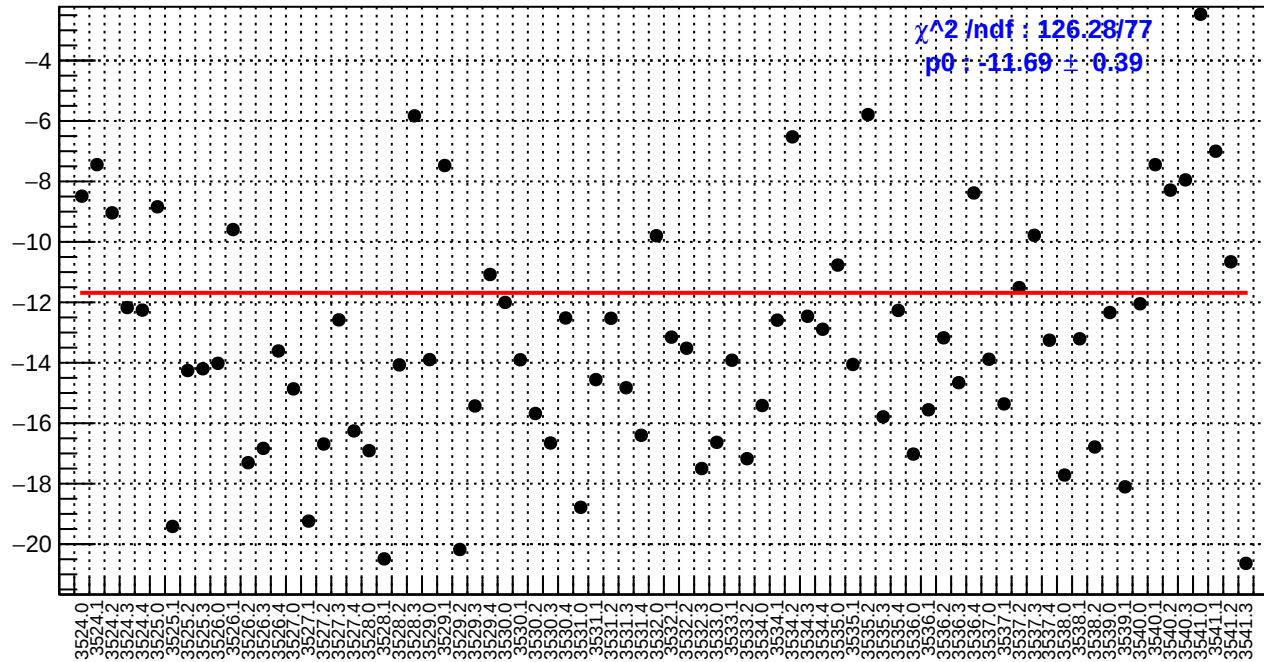
slug9-Left: us_avg_bpm4aY/(ppb/nm)
