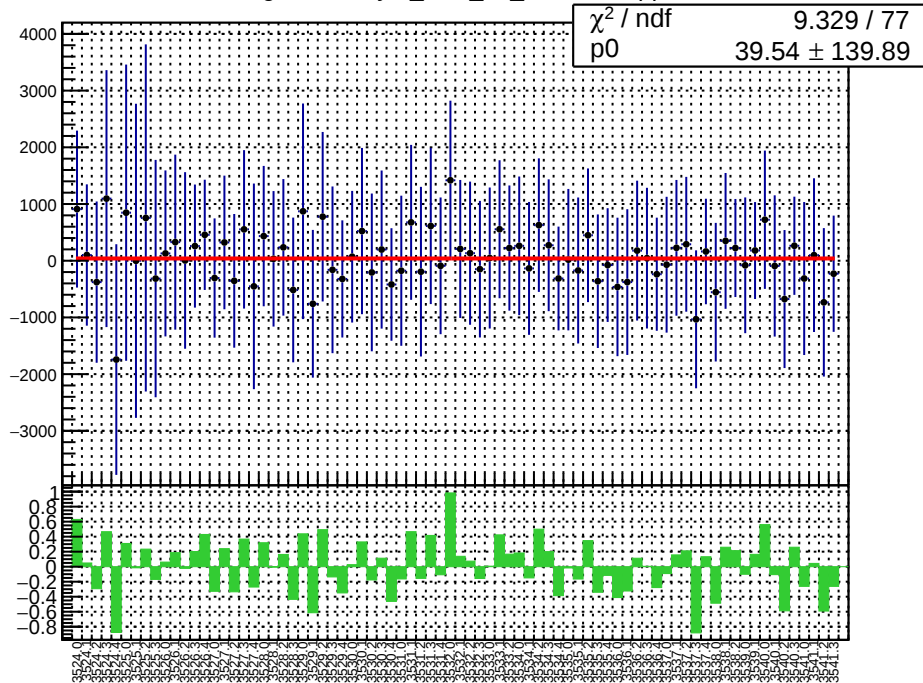
slug9-Left: asym_bcm_an_ds3.mean/ppb
