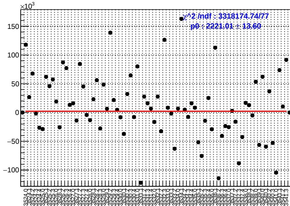
slug9-Left: asym_sam4.mean/ppb-reg_asym_sam4.mean/ppb
