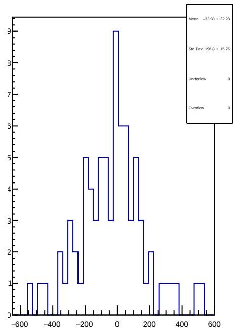
slug9-Left: 1D Corr asym_left_dd.mean/ppb-reg_asym_left_dd.mean/ppb
