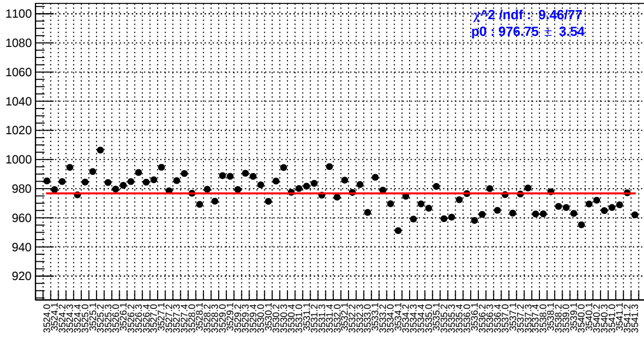
slug9-Left: reg_asym_usr.rms/ppm
