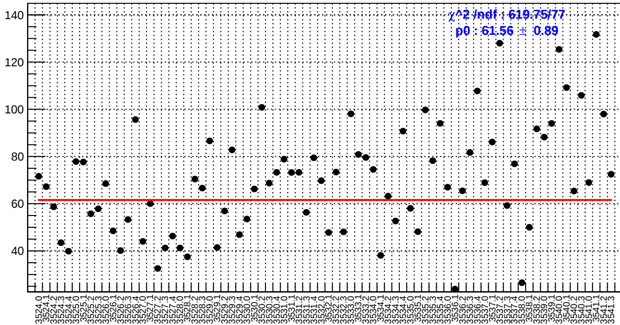
slug9-Left: ds_avg_bpm4aX/(ppb/nm)
