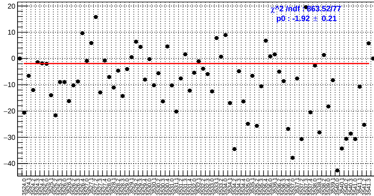
slug9-Left: right_avg_bpm4aY/(ppb/nm)
