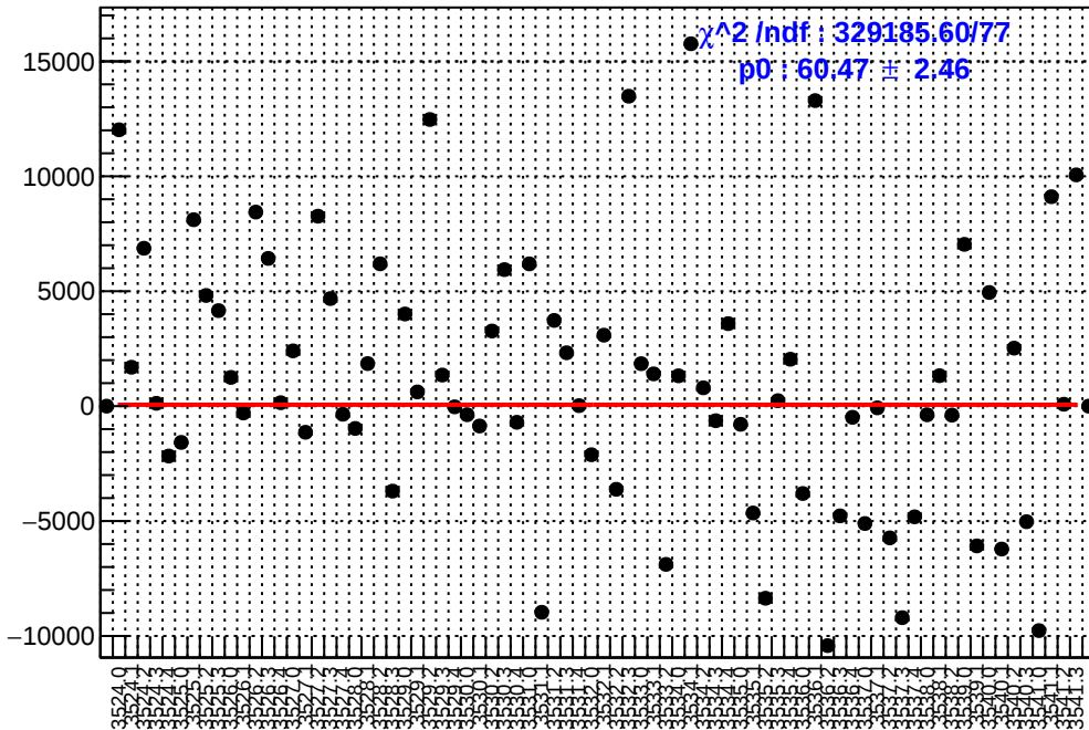
slug9-Left: asym_ds_avg.mean/ppb-reg_asym_ds_avg.mean/ppb
