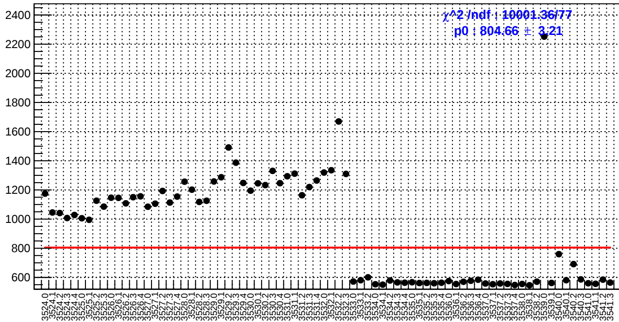
slug9-Left: reg_asym_sam3.rms/ppm
