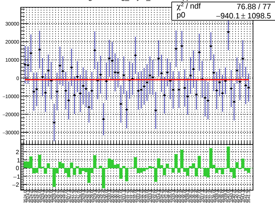
slug9-Left: reg_asym_usr.mean/ppb
