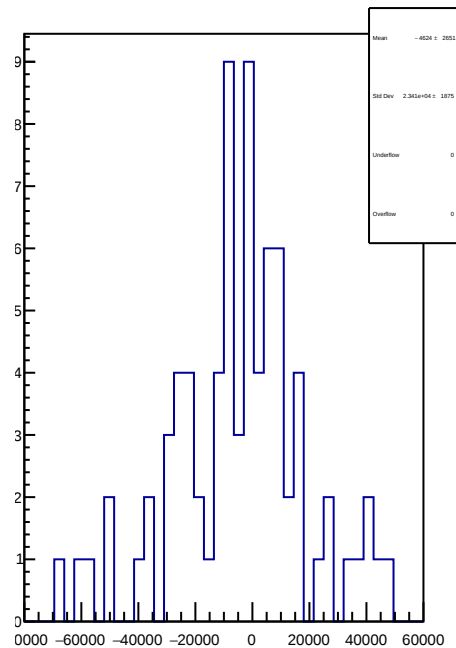
slug9-Left: 1D Corr asym_sam7.mean/ppb-reg_asym_sam7.mean/ppb
