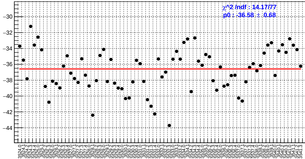
slug9-Left: dsl_bpm4aY/(ppb/nm)
