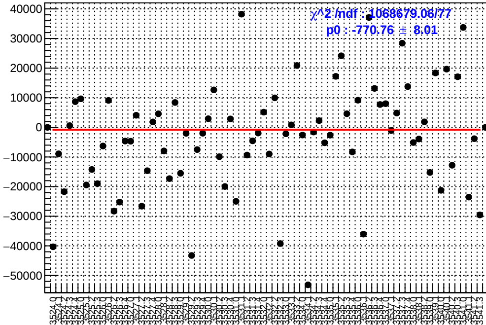
slug9-Left: asym_sam8.mean/ppb-reg_asym_sam8.mean/ppb
