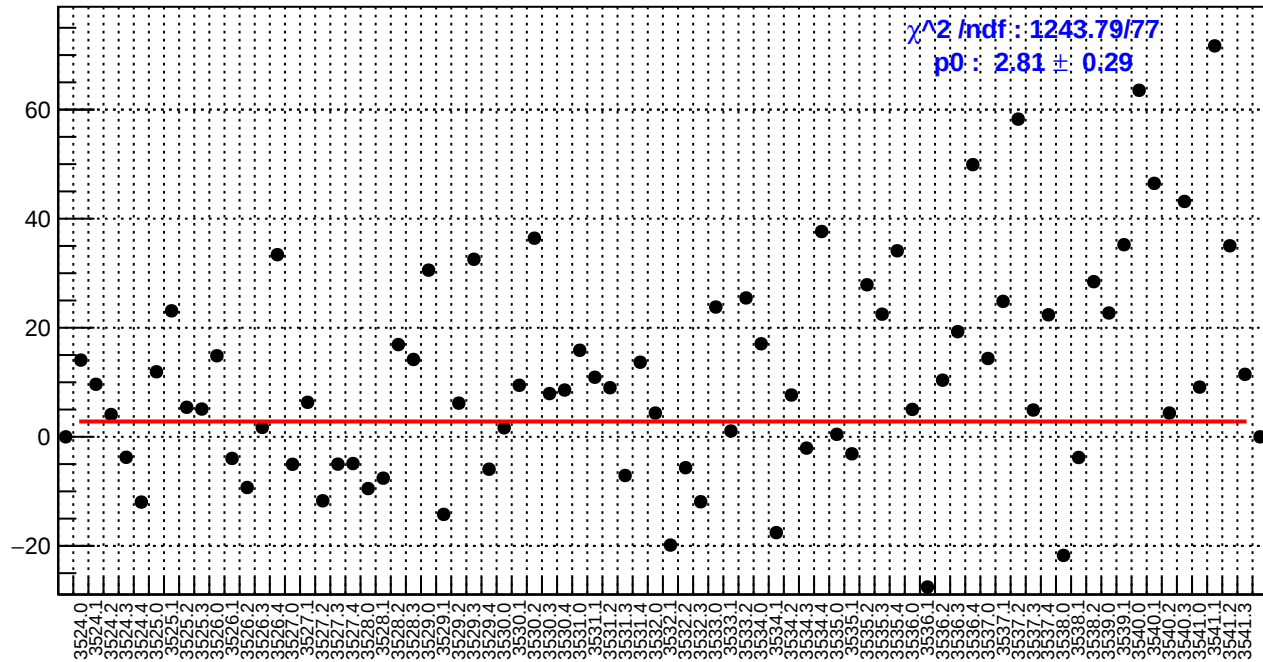
slug9-Left: right_avg_bpm4aX/(ppb/nm)
