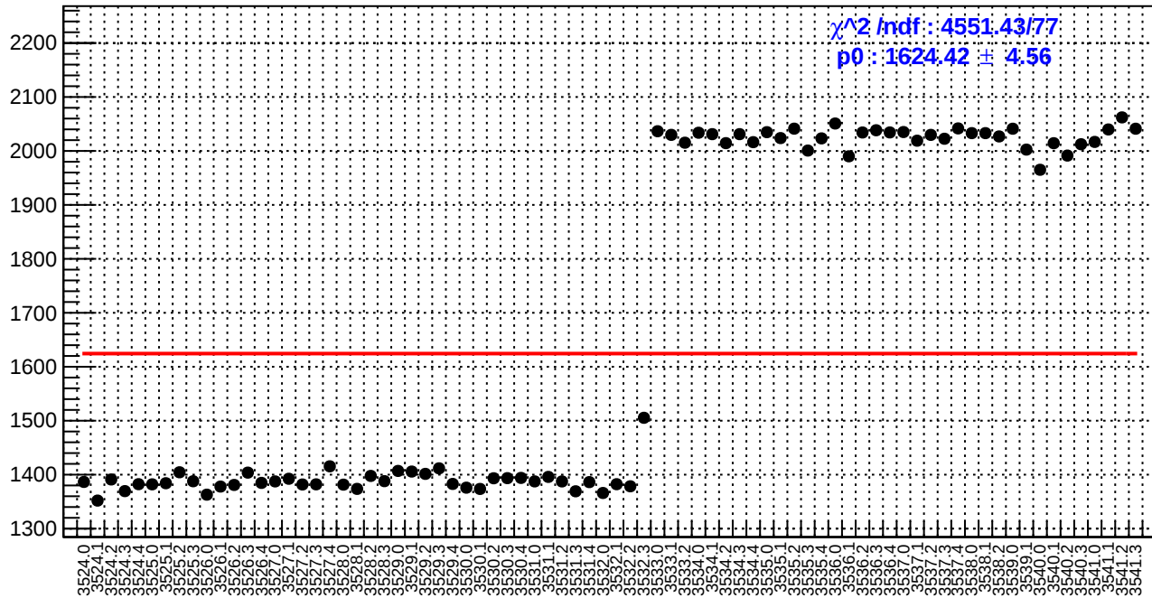
slug9-Left: reg_asym_ds_dd.rms/ppm
