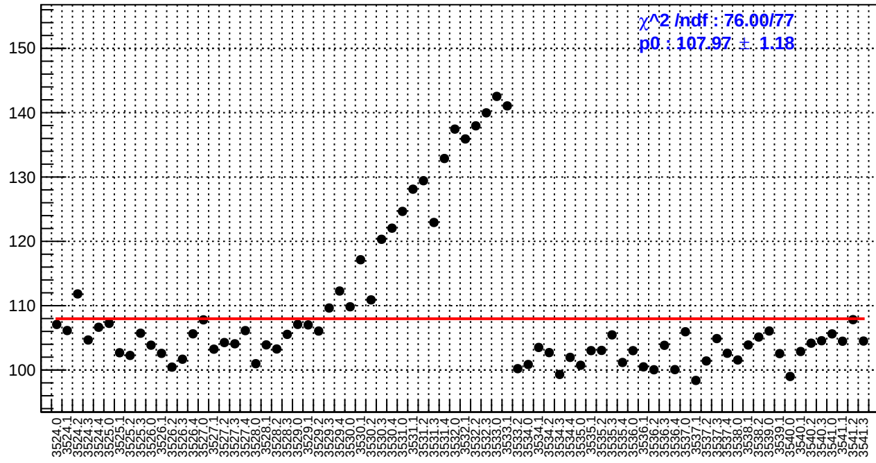
slug9-Left: usl_bpm4aX/(ppb/nm)
