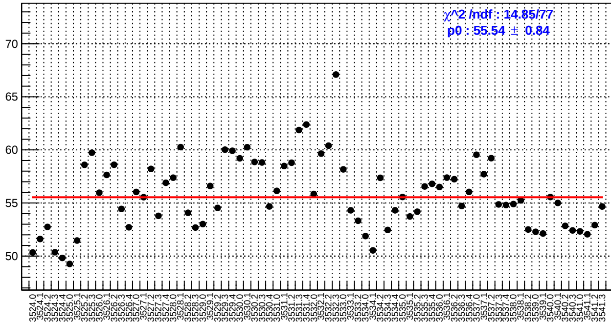
slug9-Left: dsl_bpm4eY/(ppb/nm)
