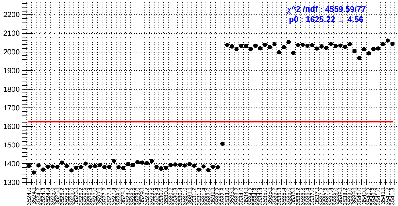
slug9-Left: reg_asym_ds_avg.rms/ppm
