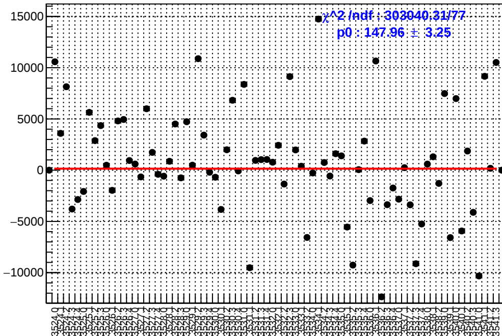
slug9-Left: asym_dsr.mean/ppb-reg_asym_dsr.mean/ppb
