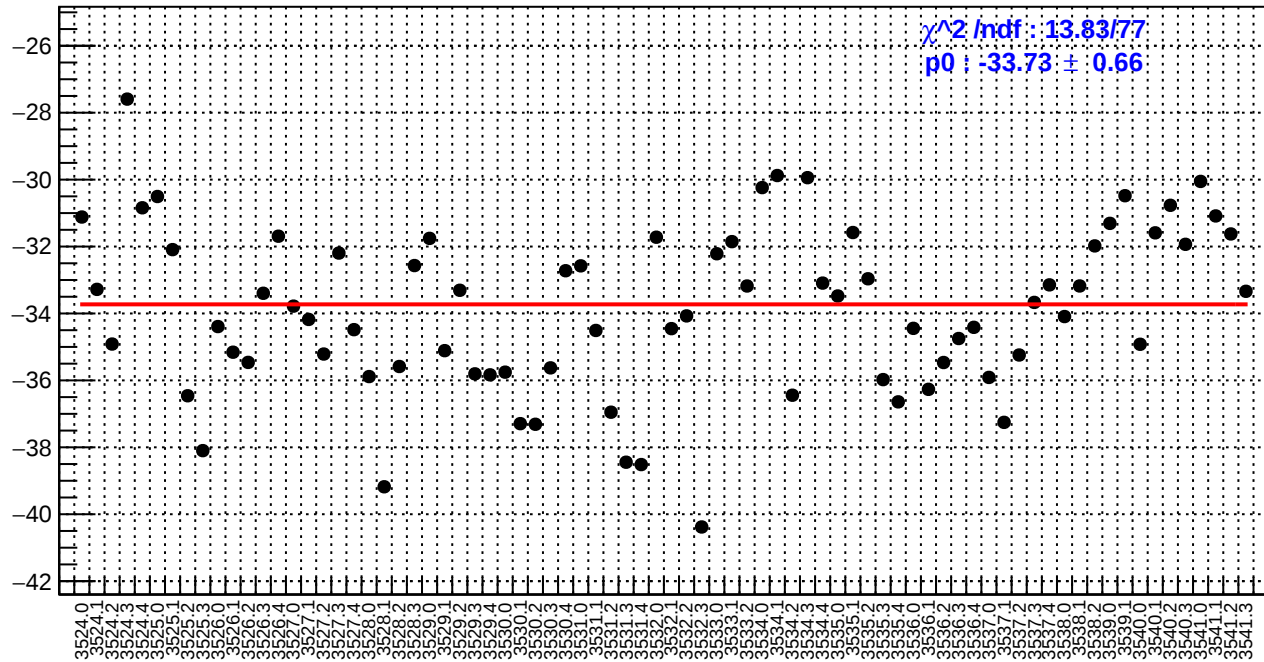
slug9-Left: usl_bpm4aY/(ppb/nm)
