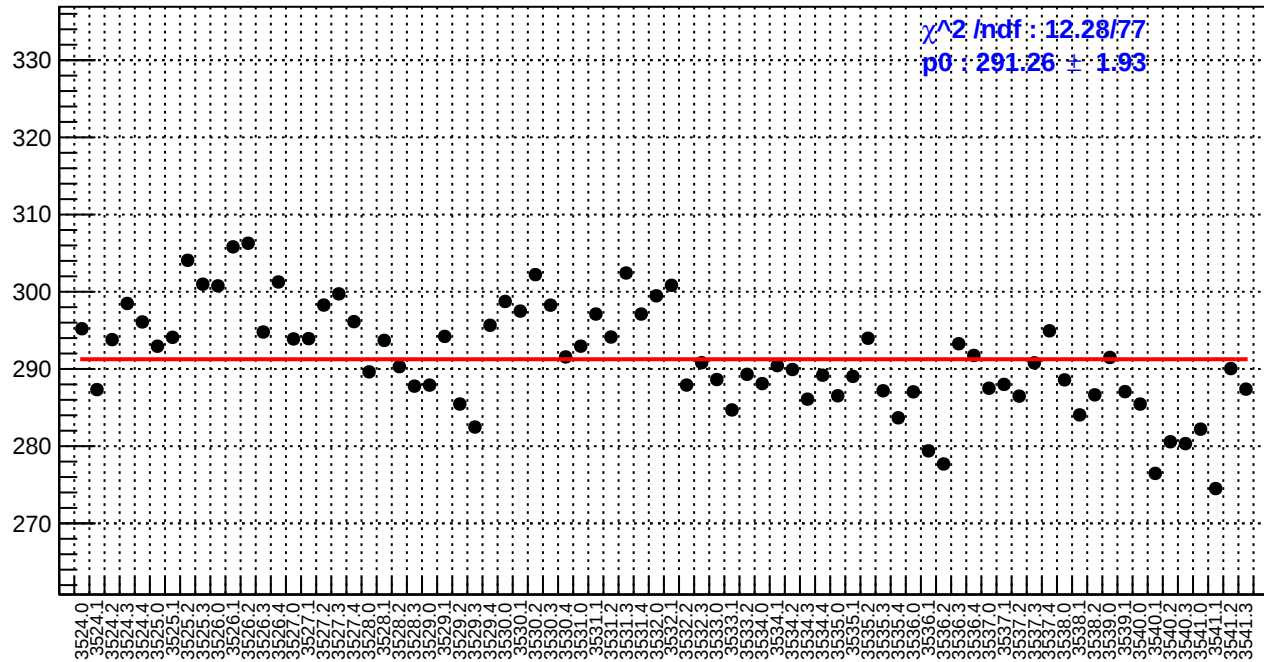
slug9-Left: reg_asym_sam1.rms/ppm
