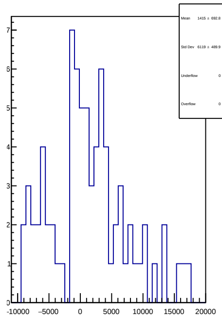
slug9-Left: 1D Corr asym_left_avg.mean/ppb-reg_asym_left_avg.mean/ppb
