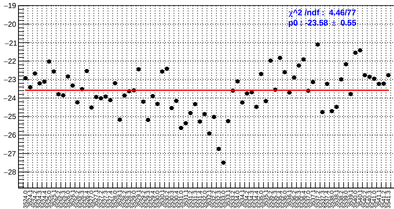
slug9-Left: us_avg_bpm4eX/(ppb/nm)
