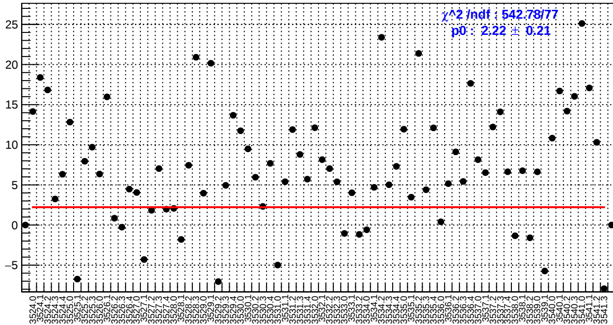
slug9-Left: usr_bpm4aY/(ppb/nm)
