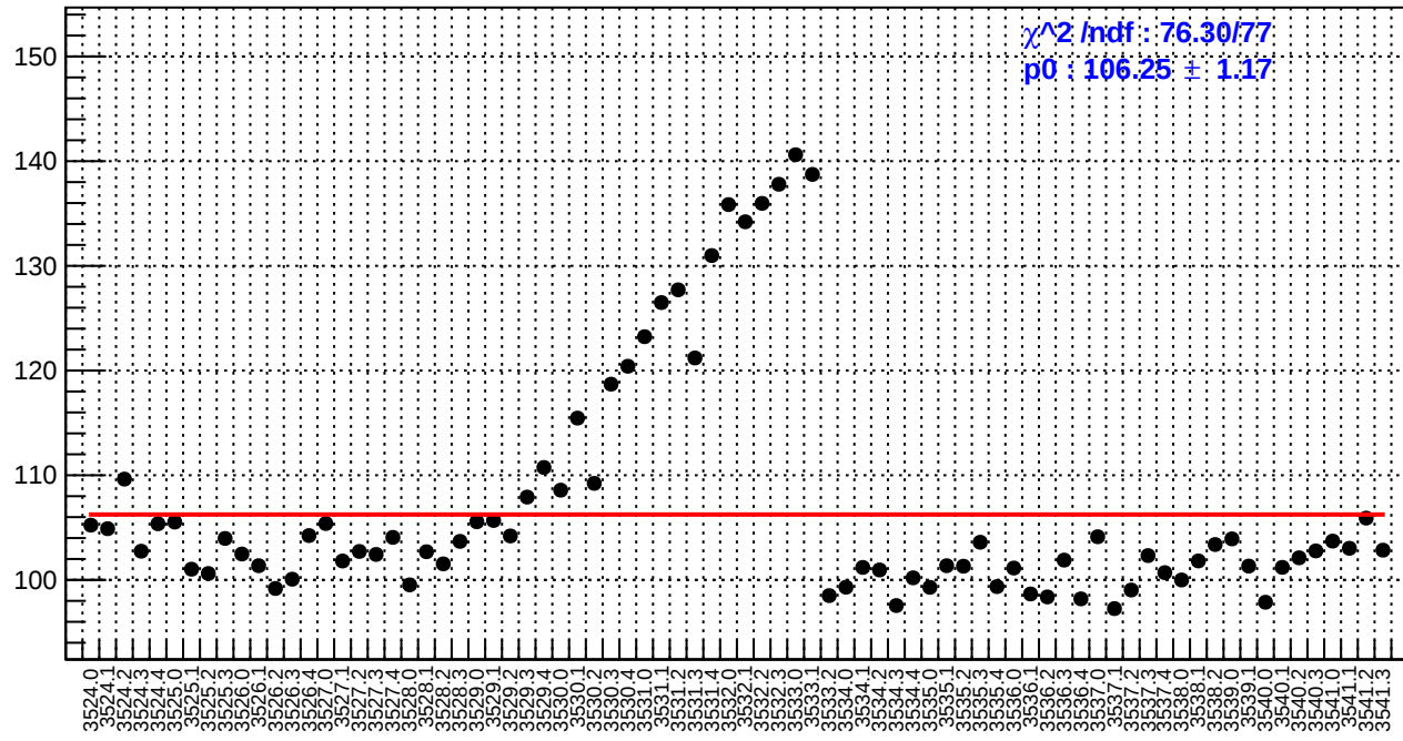
slug9-Left: left_avg_bpm4aX/(ppb/nm)
