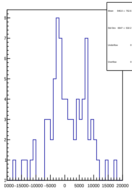
slug9-Left: 1D Corr asym_sam5.mean/ppb-reg_asym_sam5.mean/ppb
