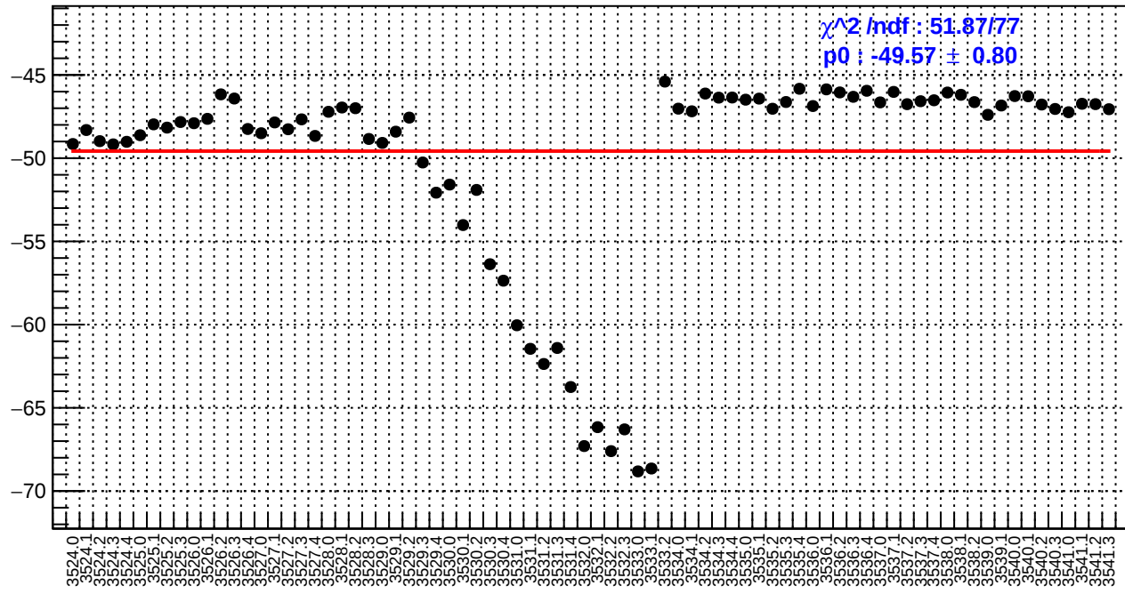
slug9-Left: left_avg_bpm12X/(ppb/nm)
