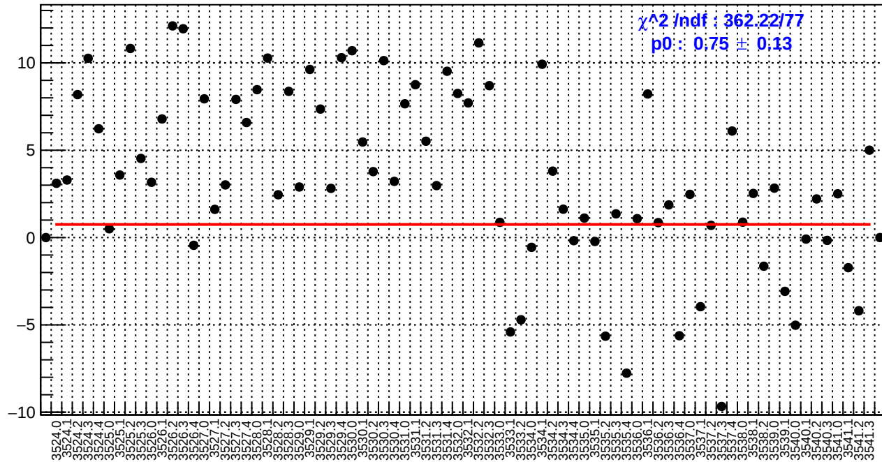
slug9-Left: right_avg_bpm12X/(ppb/nm)
