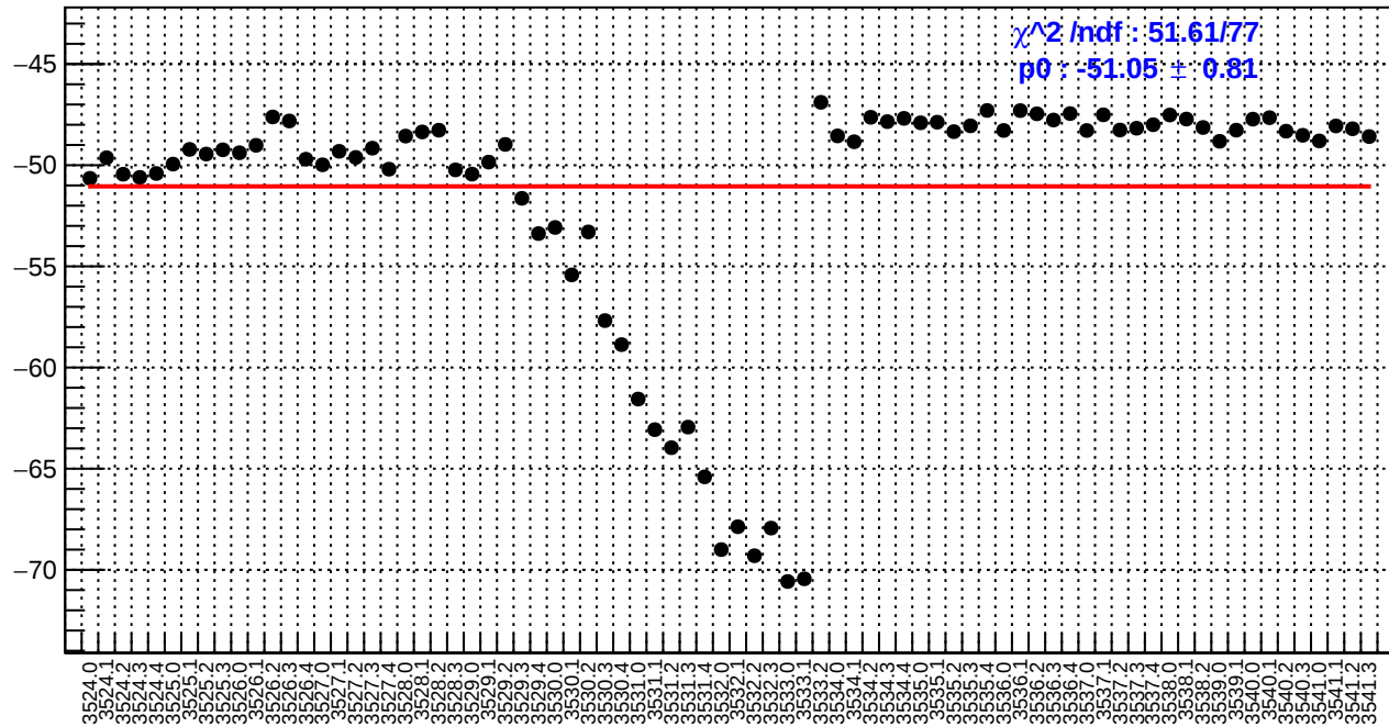
slug9-Left: usl_bpm12X/(ppb/nm)
