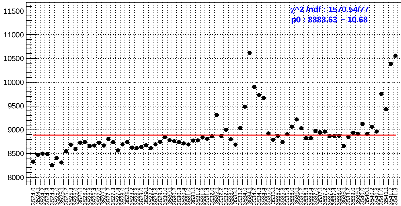
slug9-Left: diff_bpm4eX.rms/nm
