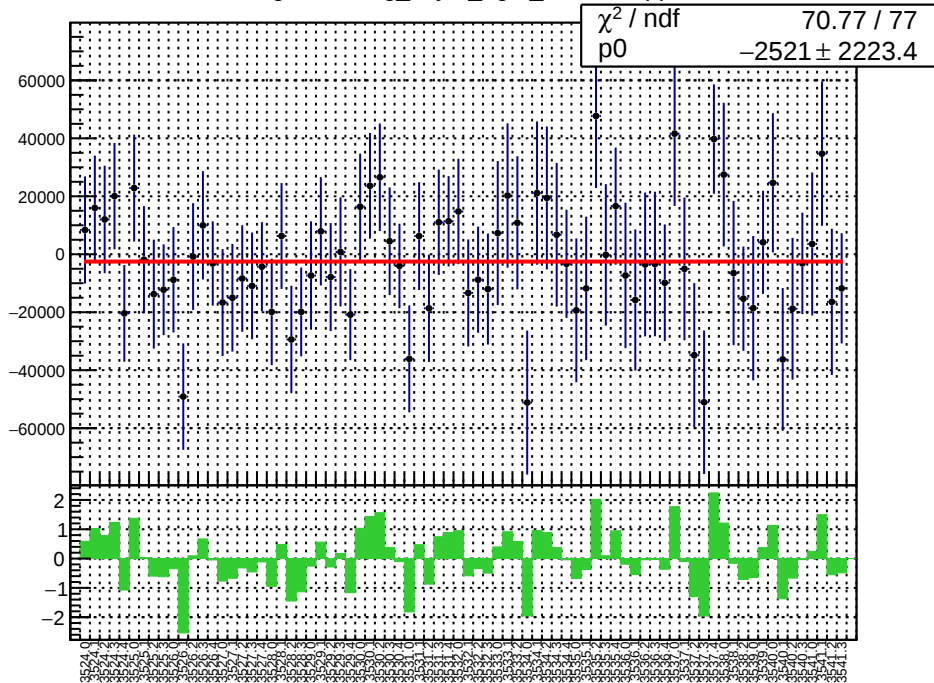
slug9-Left: reg_asym_right_dd.mean/ppb
