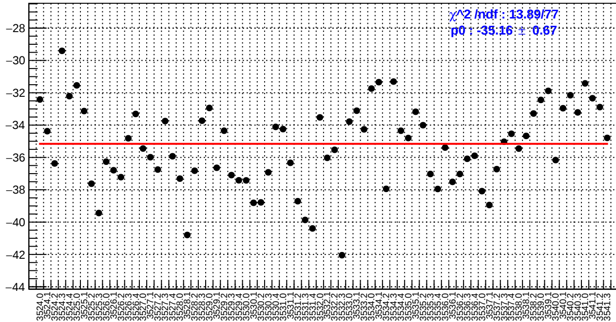
slug9-Left: left_avg_bpm4aY/(ppb/nm)
