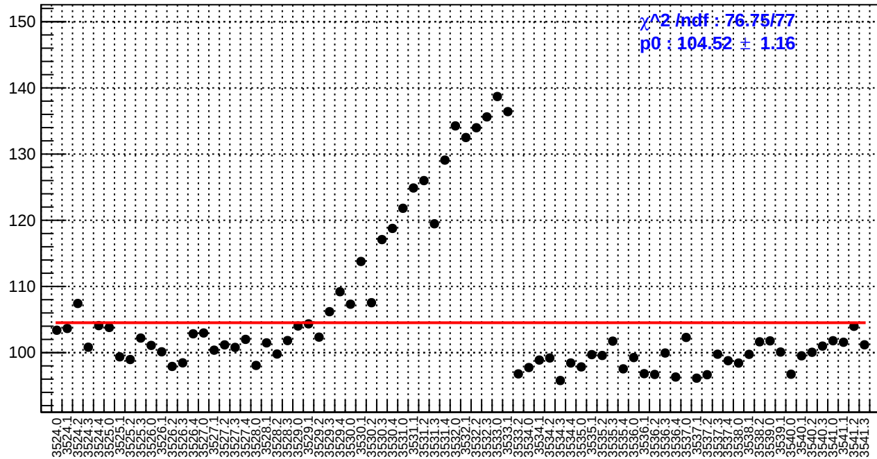
slug9-Left: dsl_bpm4aX/(ppb/nm)
