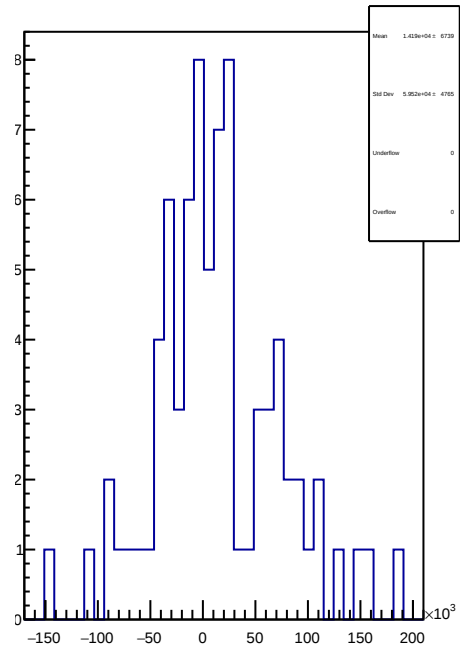
slug9-Left: 1D Corr asym_sam3.mean/ppb-reg_asym_sam3.mean/ppb
