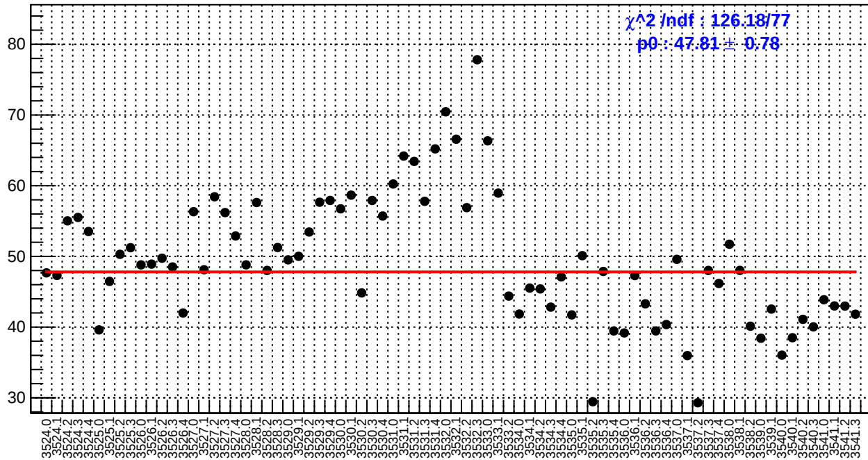
slug9-Left: us_avg_bpm4aX/(ppb/nm)
