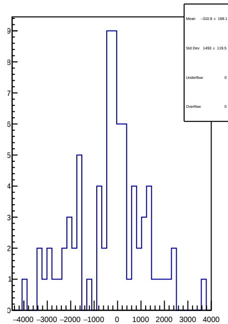
slug9-Left: 1D Corr asym_usr.mean/ppb-reg_asym_usr.mean/ppb
