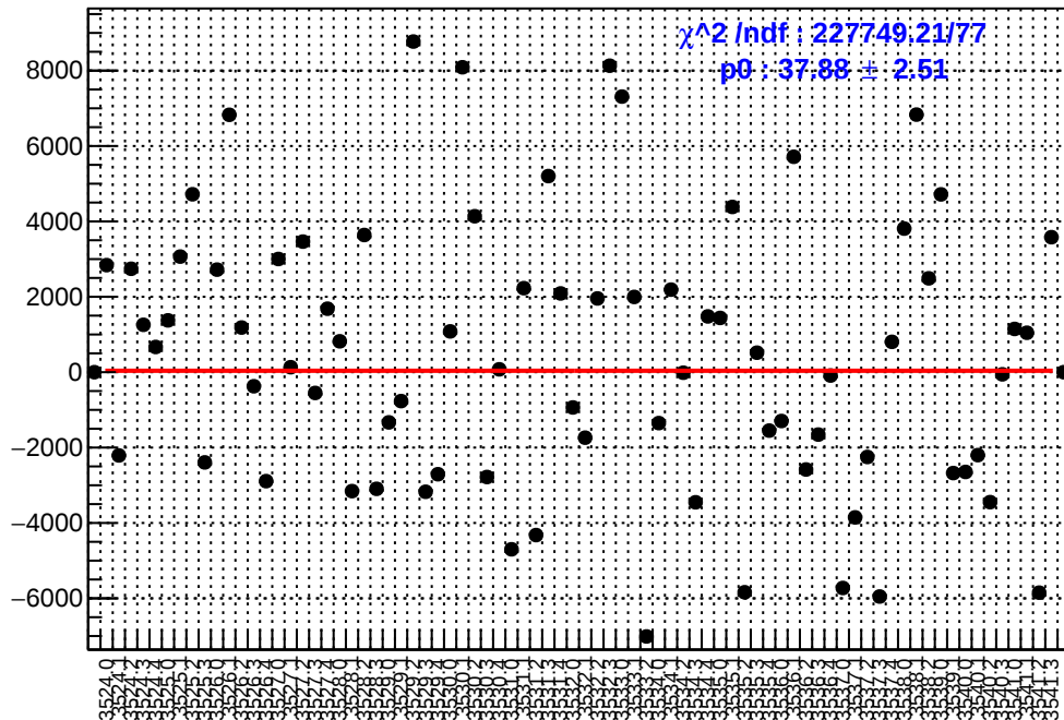
slug9-Left: asym_sam1.mean/ppb-reg_asym_sam1.mean/ppb
