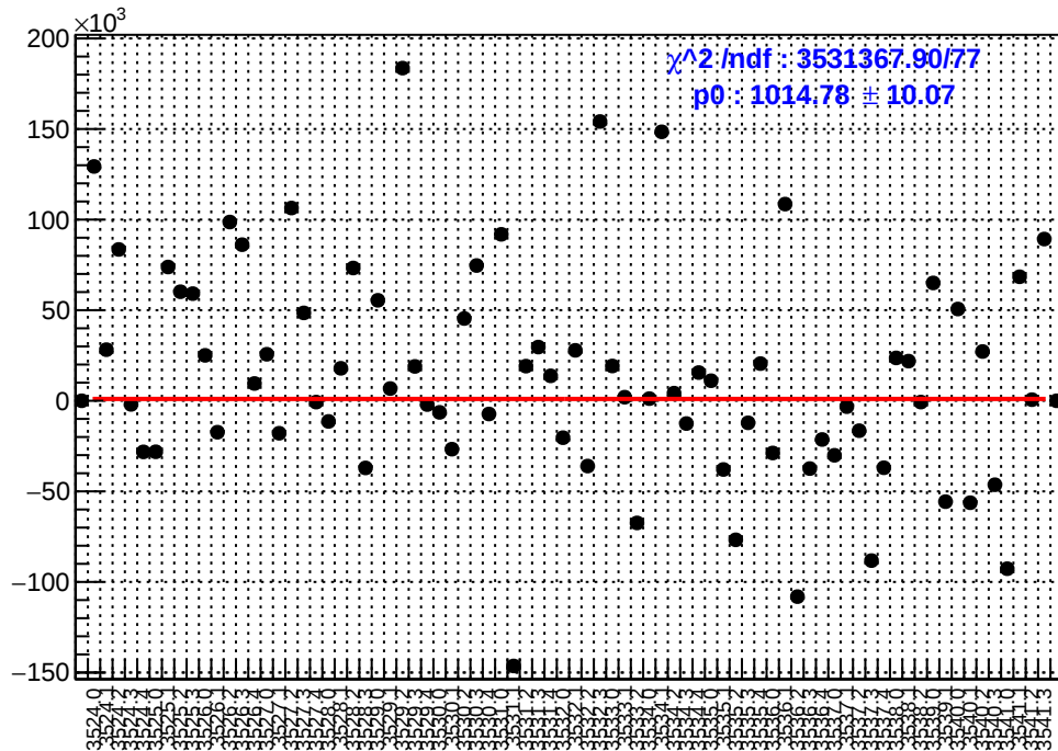
slug9-Left: asym_sam3.mean/ppb-reg_asym_sam3.mean/ppb
