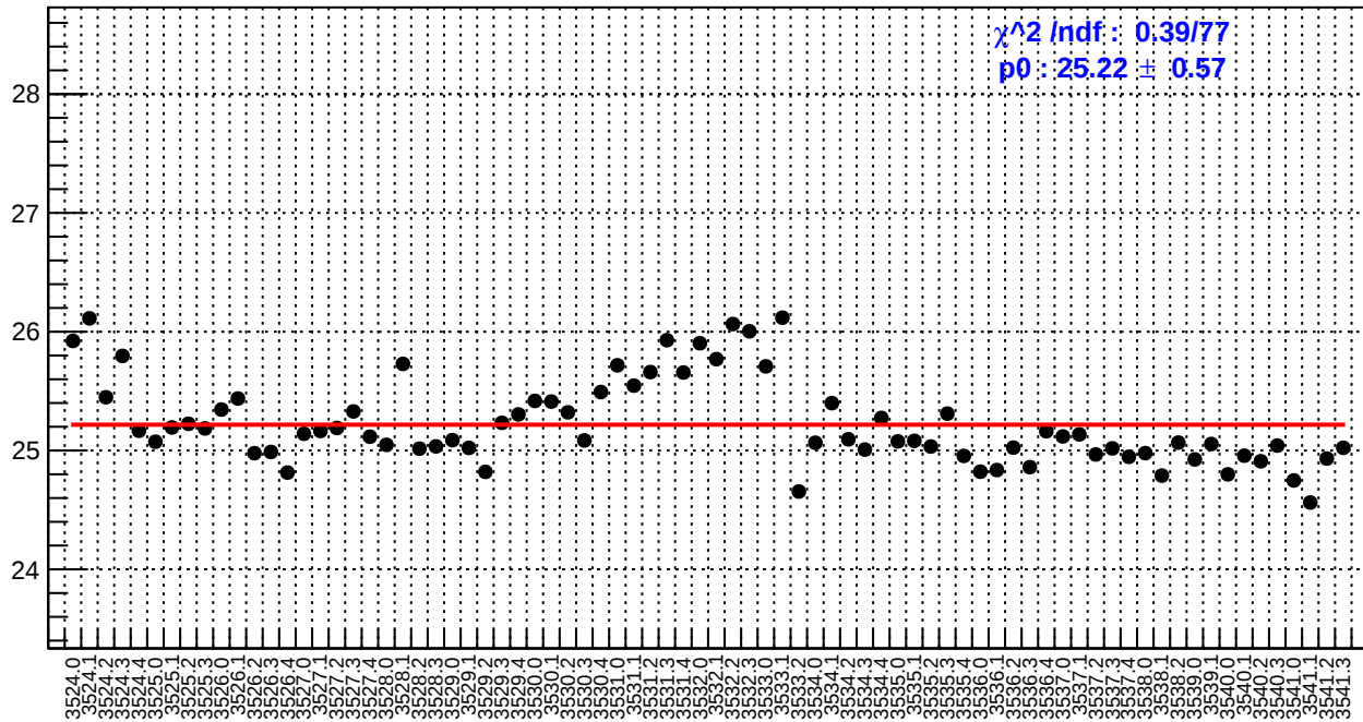
slug9-Left: reg_asym_left_dd.rms/ppm
