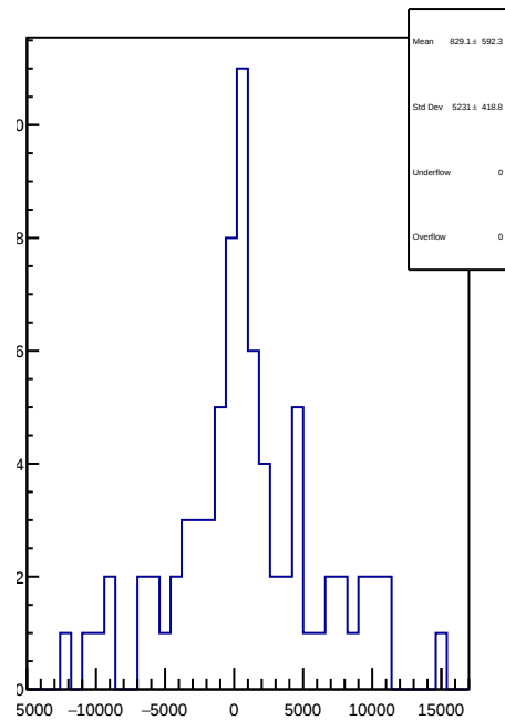
slug9-Left: 1D Corr asym_dsr.mean/ppb-reg_asym_dsr.mean/ppb
