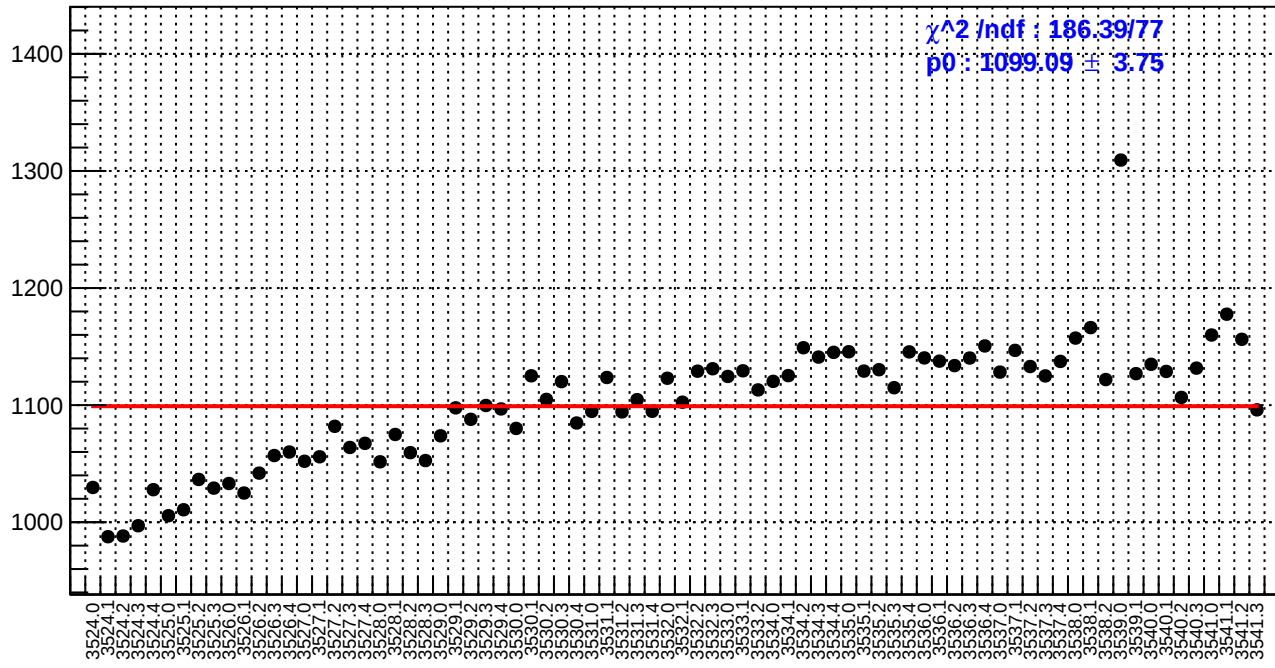
slug9-Left: reg_asym_sam4.rms/ppm
