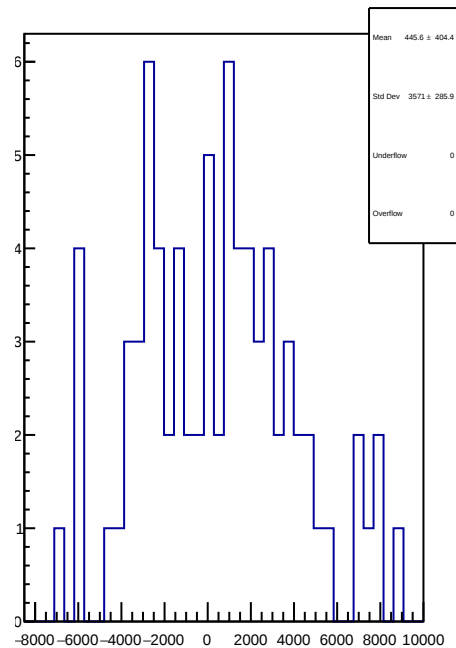
slug9-Left: 1D Corr asym_sam1.mean/ppb-reg_asym_sam1.mean/ppb
