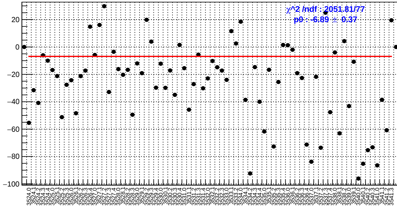
slug9-Left: dsr_bpm4aY/(ppb/nm)
