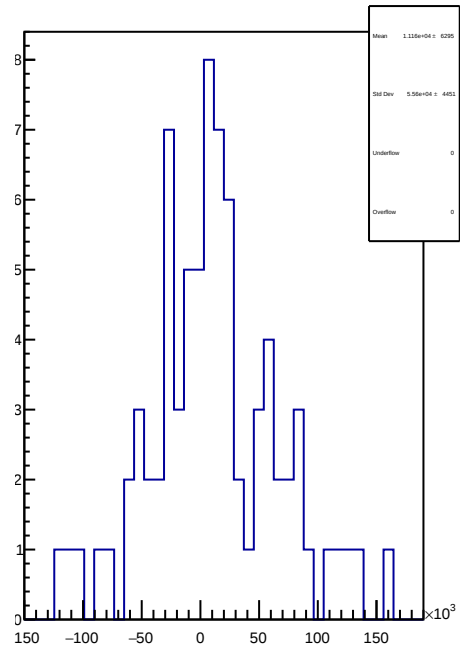
slug9-Left: 1D Corr asym_sam4.mean/ppb-reg_asym_sam4.mean/ppb
