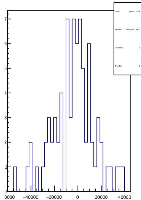
slug9-Left: 1D Corr asym_sam8.mean/ppb-reg_asym_sam8.mean/ppb
