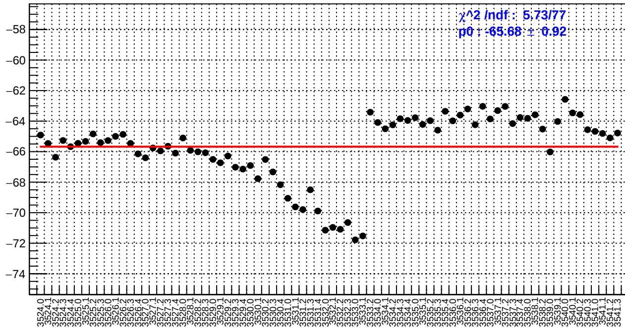
slug9-Left: left_avg_bpm4eX/(ppb/nm)
