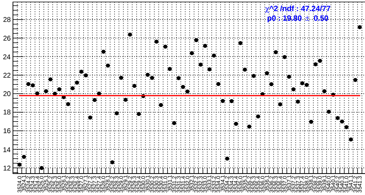
slug9-Left: us_avg_bpm4eY/(ppb/nm)
