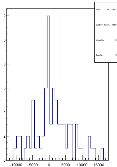
slug9-Left: 1D Corr asym_ds_avg.mean/ppb-reg_asym_ds_avg.mean/ppb
