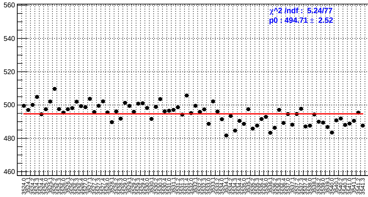
slug9-Left: reg_asym_us_avg.rms/ppm
