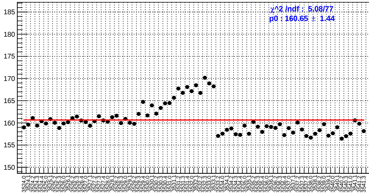
slug9-Left: reg_asym_left_avg.rms/ppm
