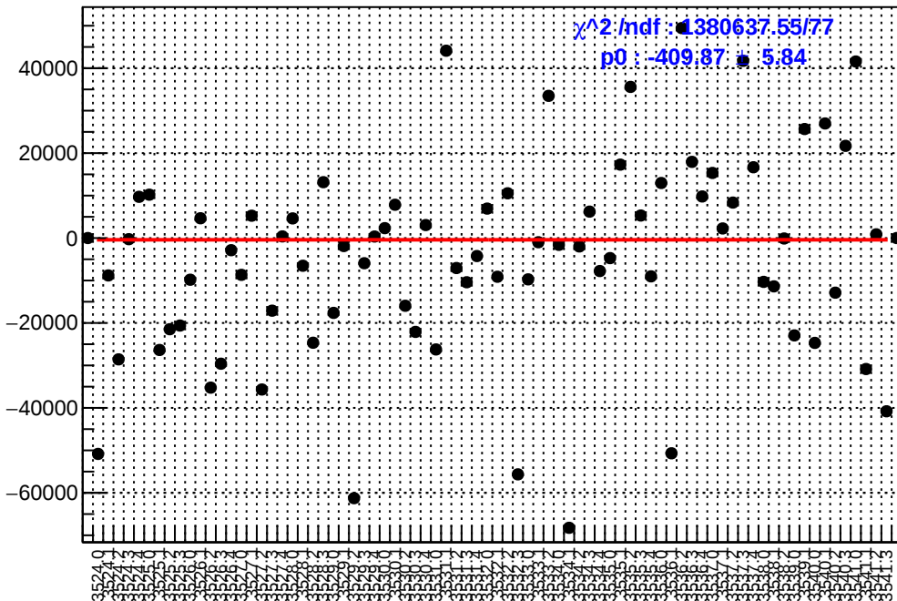
slug9-Left: asym_sam7.mean/ppb-reg_asym_sam7.mean/ppb
