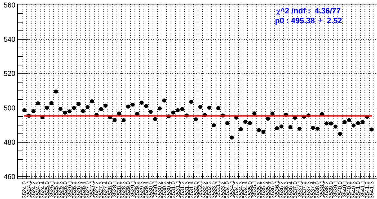
slug9-Left: reg_asym_us_dd.rms/ppm
