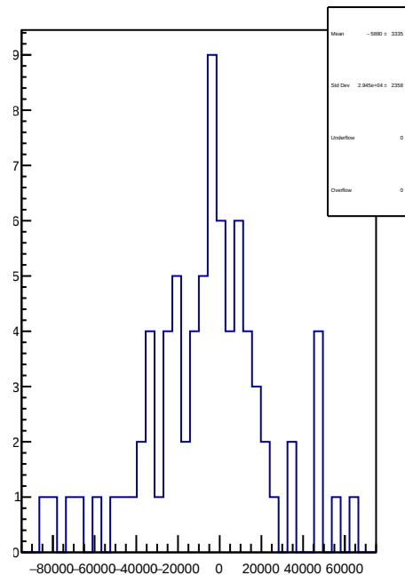
slug9-Left: 1D Corr asym_sam6.mean/ppb-reg_asym_sam6.mean/ppb
