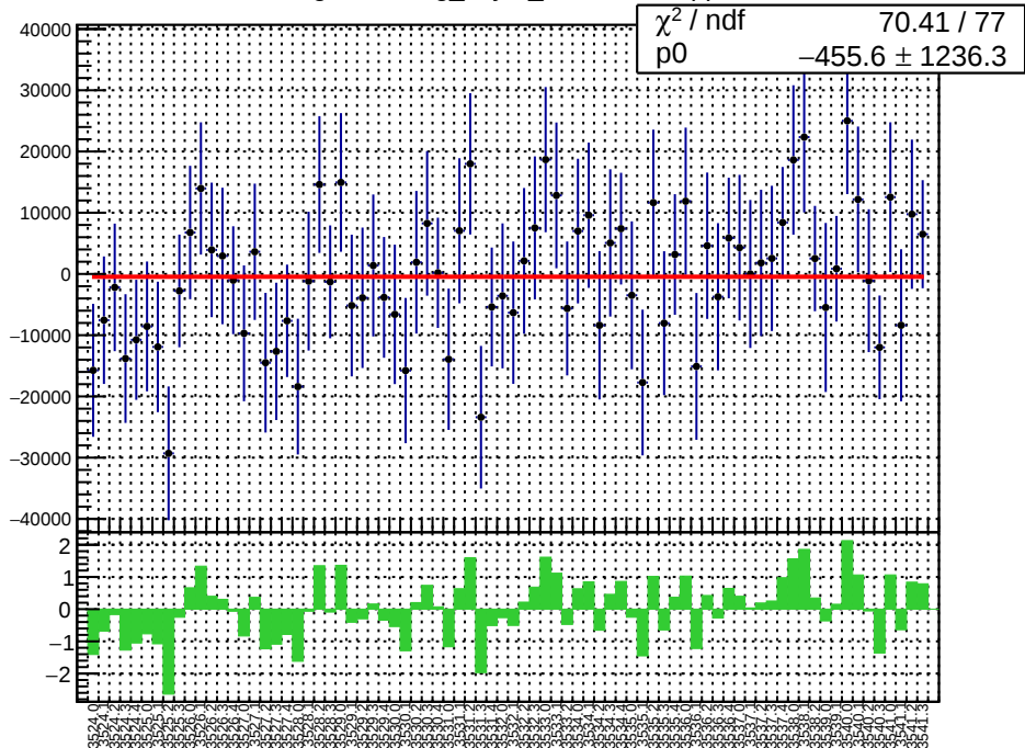
slug9-Left: reg_asym_sam4.mean/ppb
