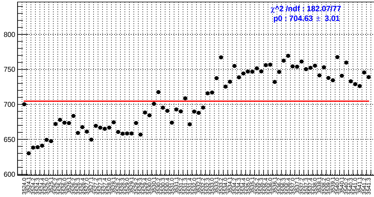
slug9-Left: reg_asym_sam6.rms/ppm
