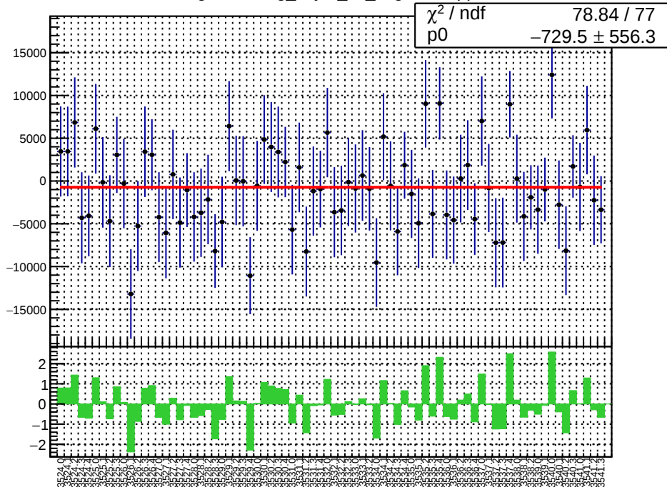
slug9-Left: reg_asym_us_avg.mean/ppb
