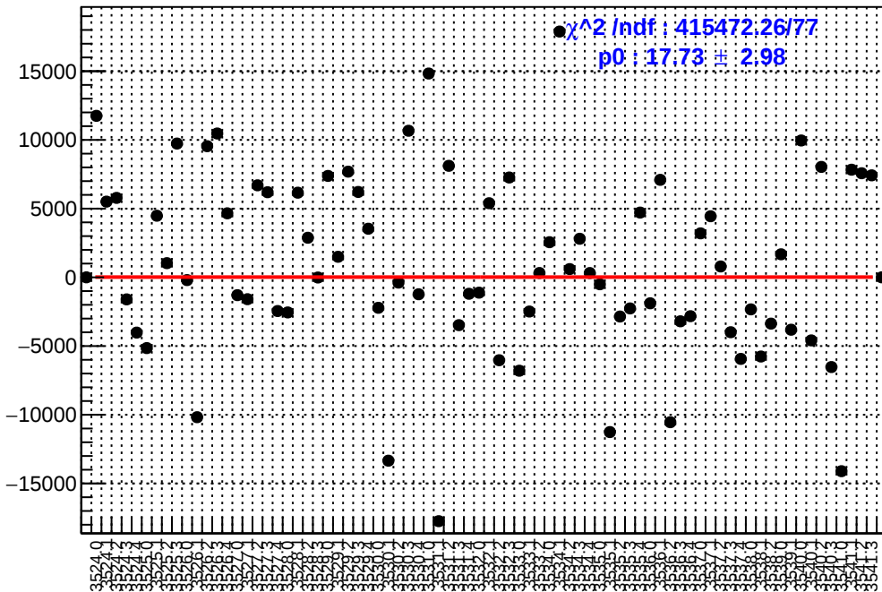
slug9-Left: asym_sam5.mean/ppb-reg_asym_sam5.mean/ppb
