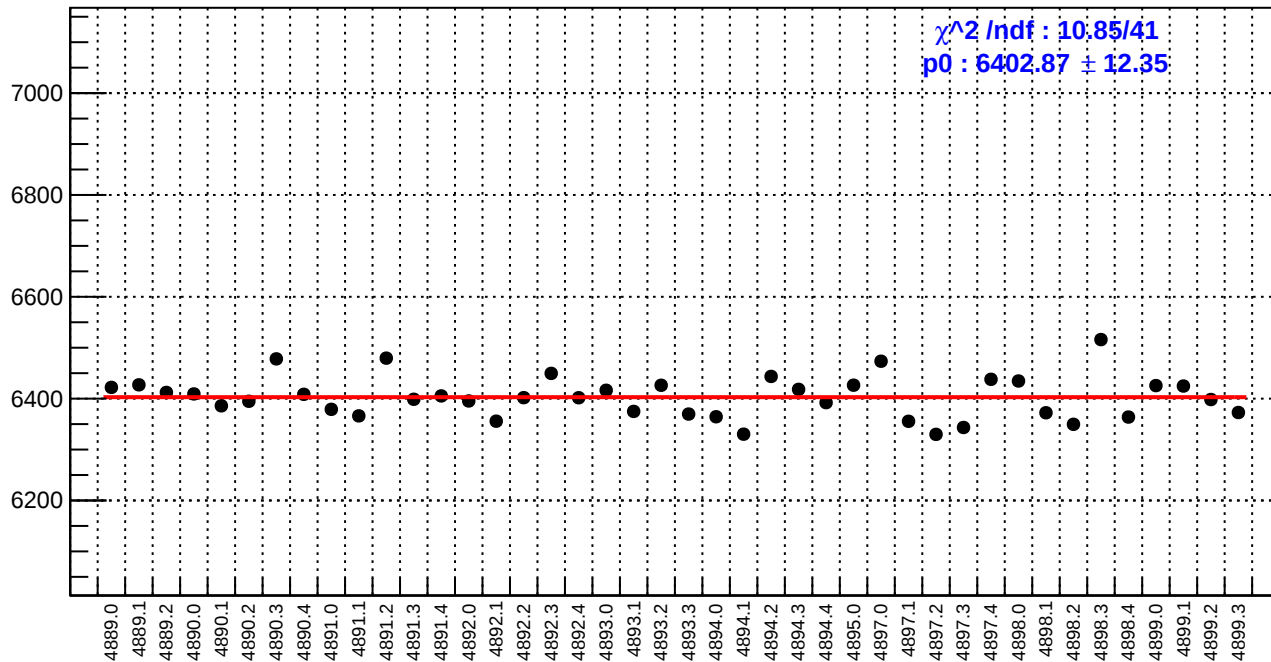
slug90: reg_asym_atl_dd.rms/ppm
