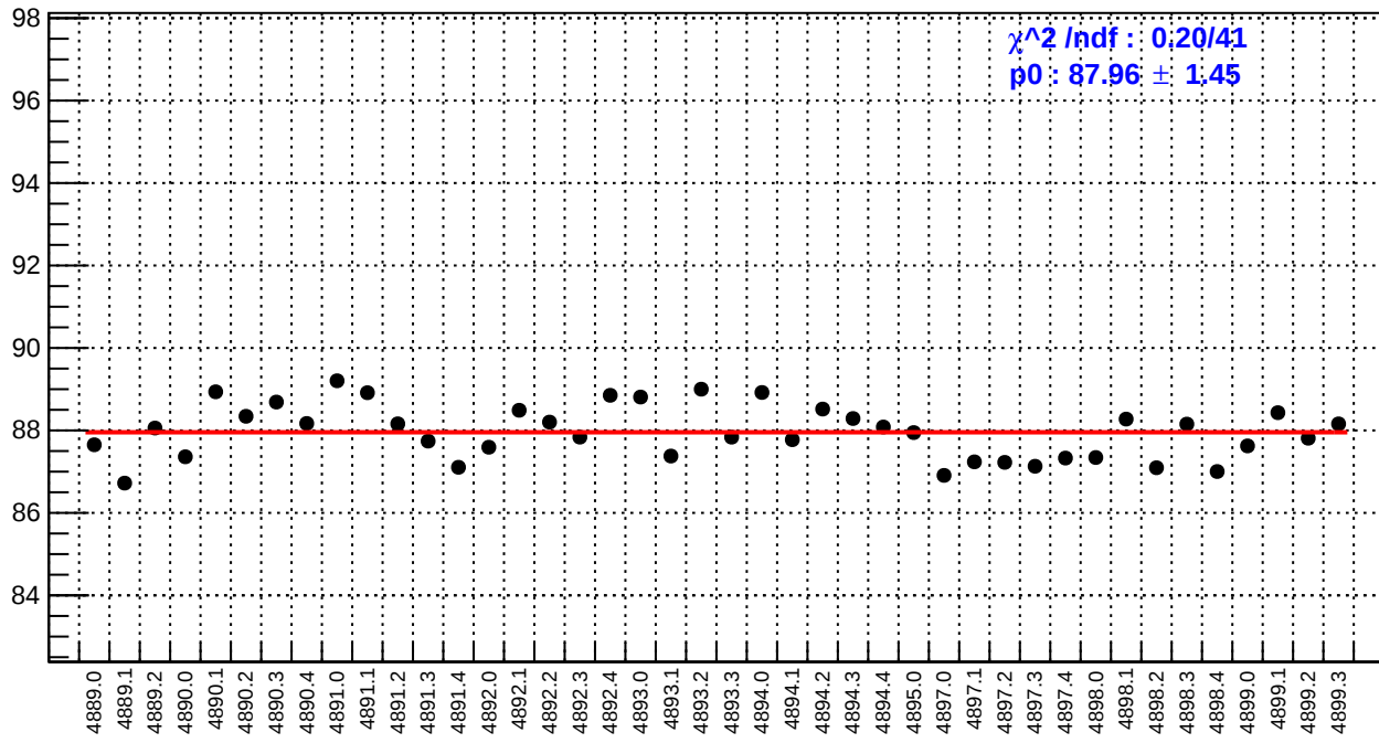
slug90: reg_asym_us_avg.rms/ppm
