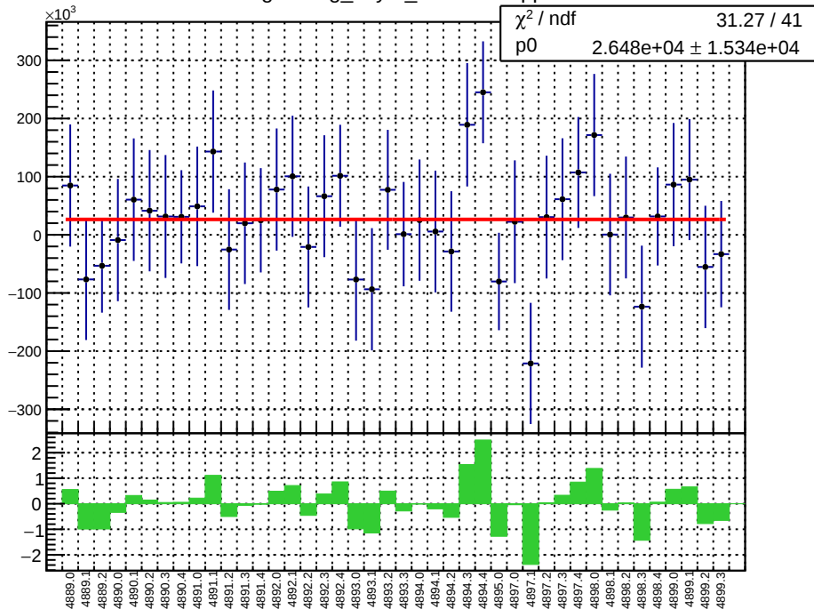
slug90: reg_asym_atr2.mean/ppb
