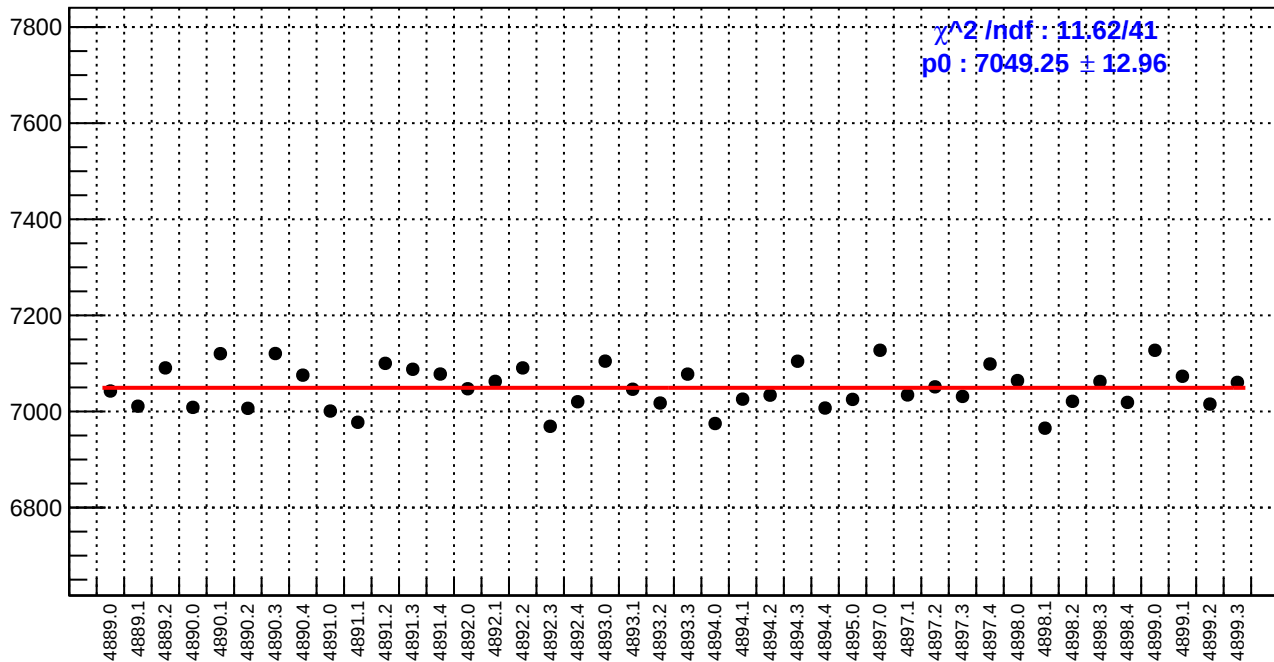
slug90: reg_asym_at2_avg.rms/ppm
