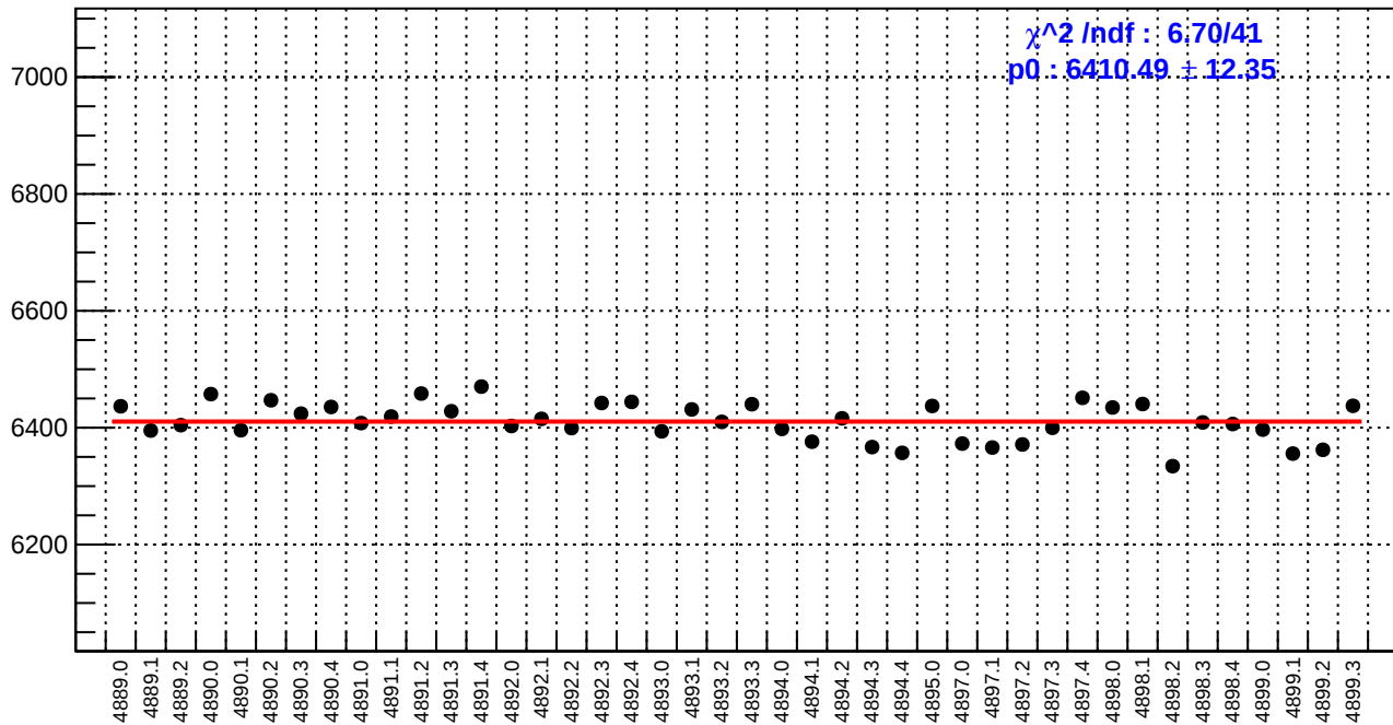
slug90: reg_asym_atl_avg.rms/ppm
