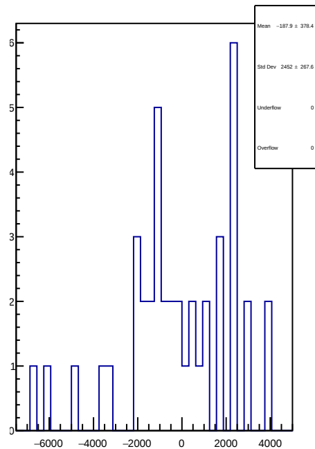
slug90: 1D Corr asym_atl1.mean/ppb-reg_asym_atl1.mean/ppb
