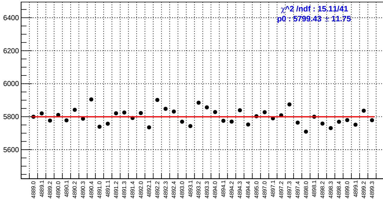
slug90: reg_asym_at1_dd.rms/ppm
