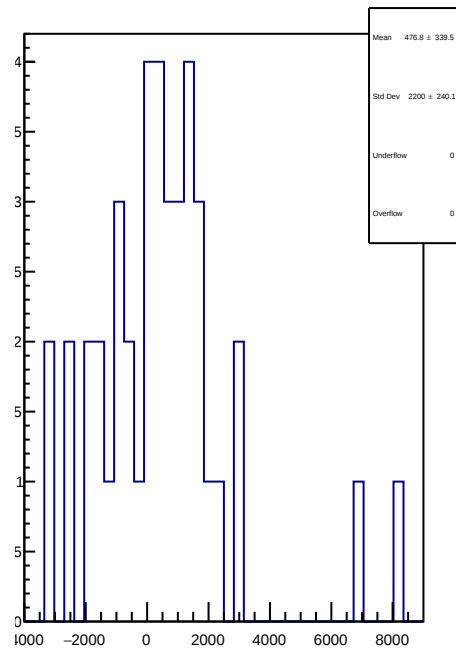
slug90: 1D Corr asym_at2_avg.mean/ppb-reg_asym_at2_avg.mean/ppb
