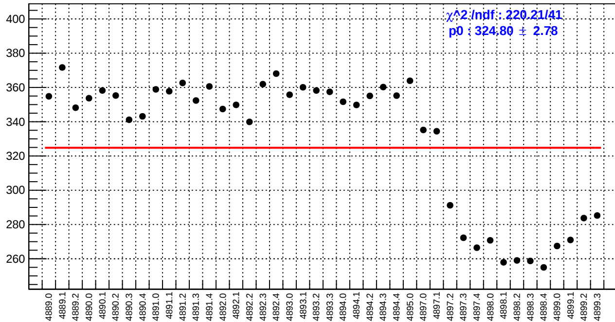
slug90: reg_asym_sam7.rms/ppm
