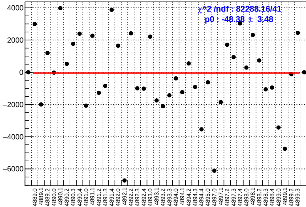
slug90: asym_atl1.mean/ppb-reg_asym_atl1.mean/ppb
