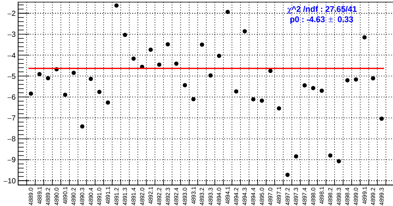
slug90: right_avg_bpm4aX/(ppb/nm)
