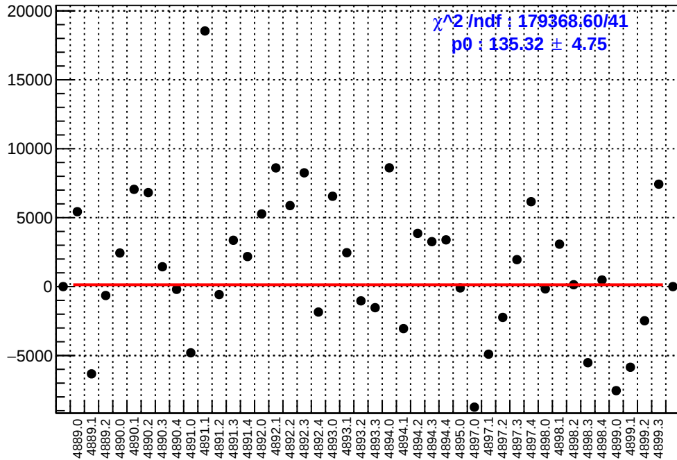
slug90: asym_left_avg.mean/ppb-reg_asym_left_avg.mean/ppb
