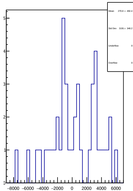
slug90: 1D Corr asym_atl1r2_dd.mean/ppb-reg_asym_atl1r2_dd.mean/ppb
