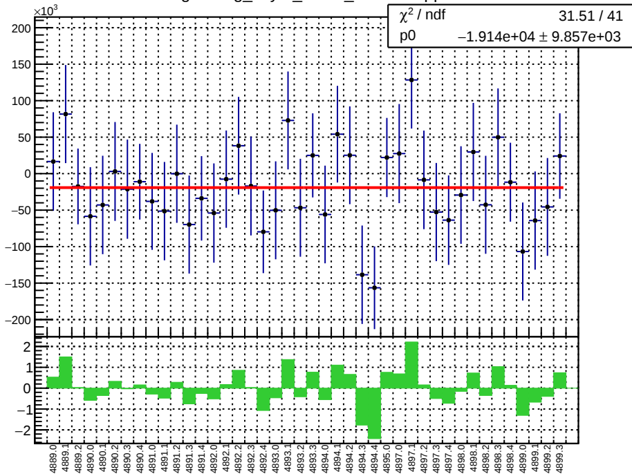
slug90: reg_asym_atl1r2_dd.mean/ppb
