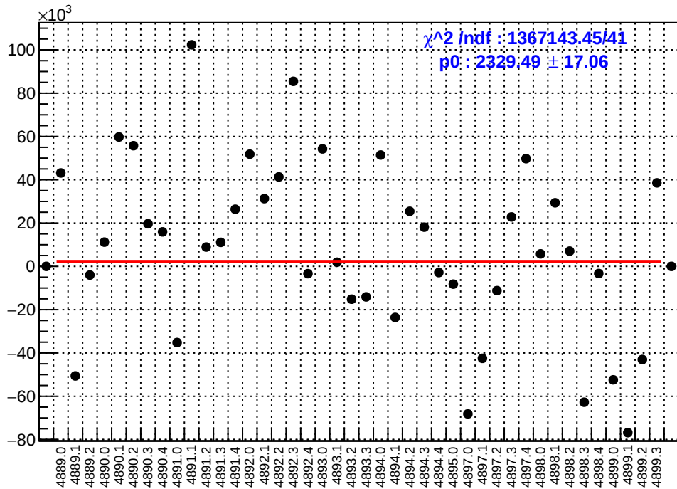
slug90: asym_sam2.mean/ppb-reg_asym_sam2.mean/ppb
