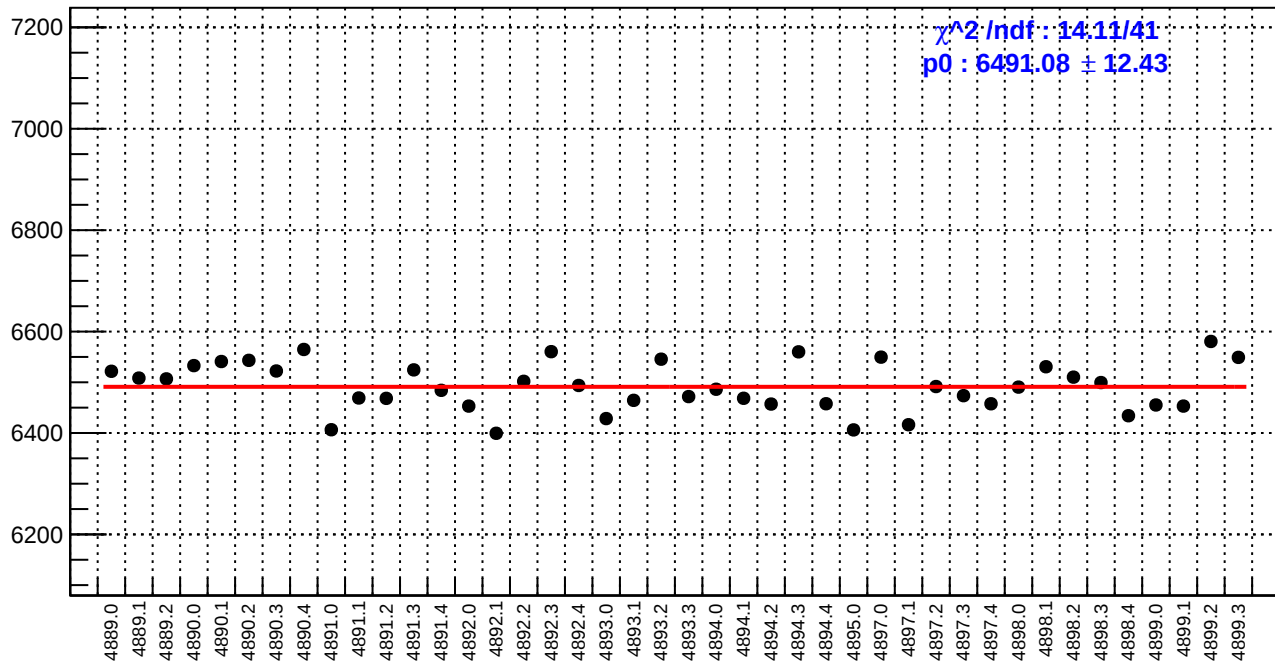
slug90: reg_asym_atr_dd.rms/ppm
