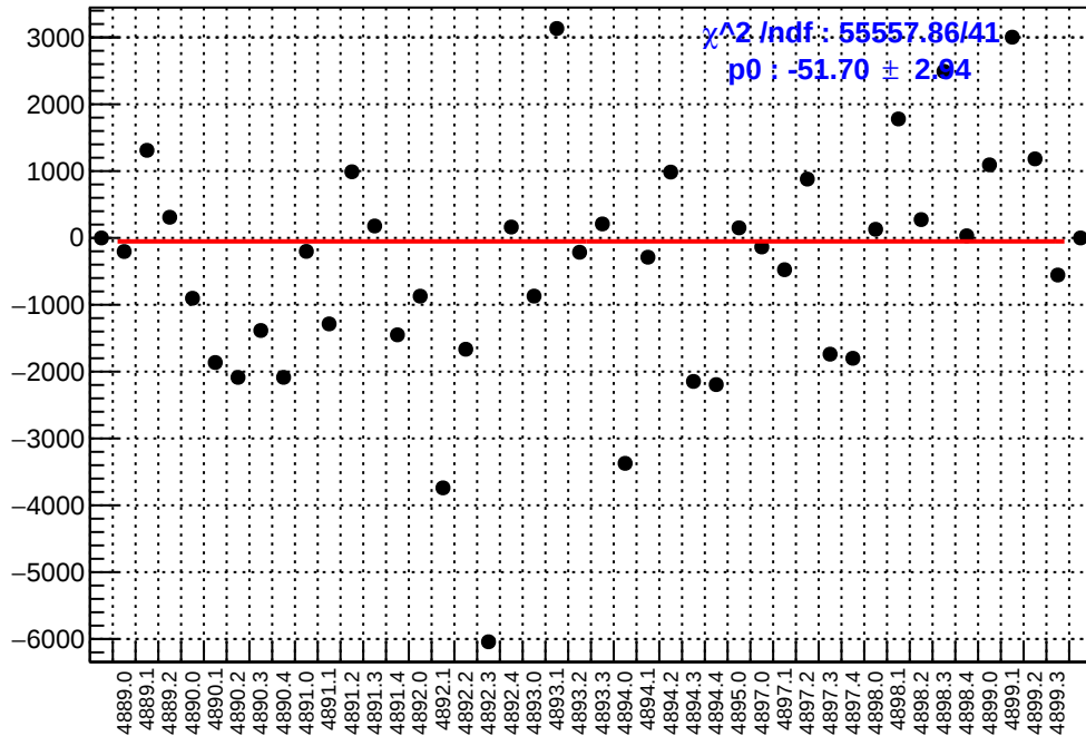
slug90: asym_atl1r2_avg.mean/ppb-reg_asym_atl1r2_avg.mean/ppb
