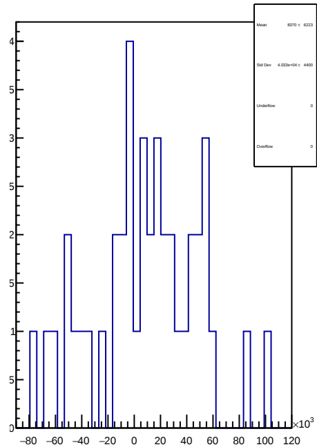
slug90: 1D Corr asym_sam2.mean/ppb-reg_asym_sam2.mean/ppb
