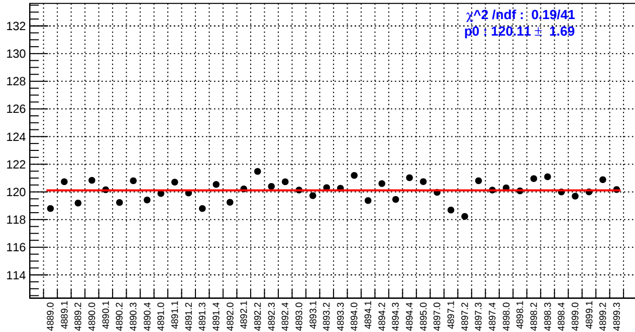
slug90: reg_asym_usr.rms/ppm
