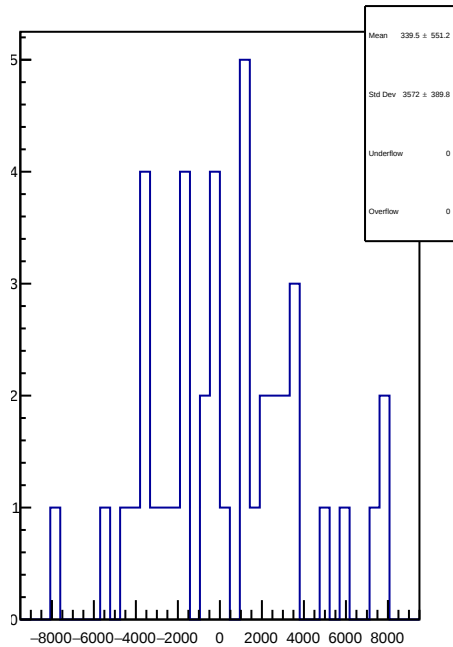
slug90: 1D Corr asym_sam1.mean/ppb-reg_asym_sam1.mean/ppb
