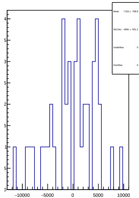
slug90: 1D Corr asym_sam5.mean/ppb-reg_asym_sam5.mean/ppb
