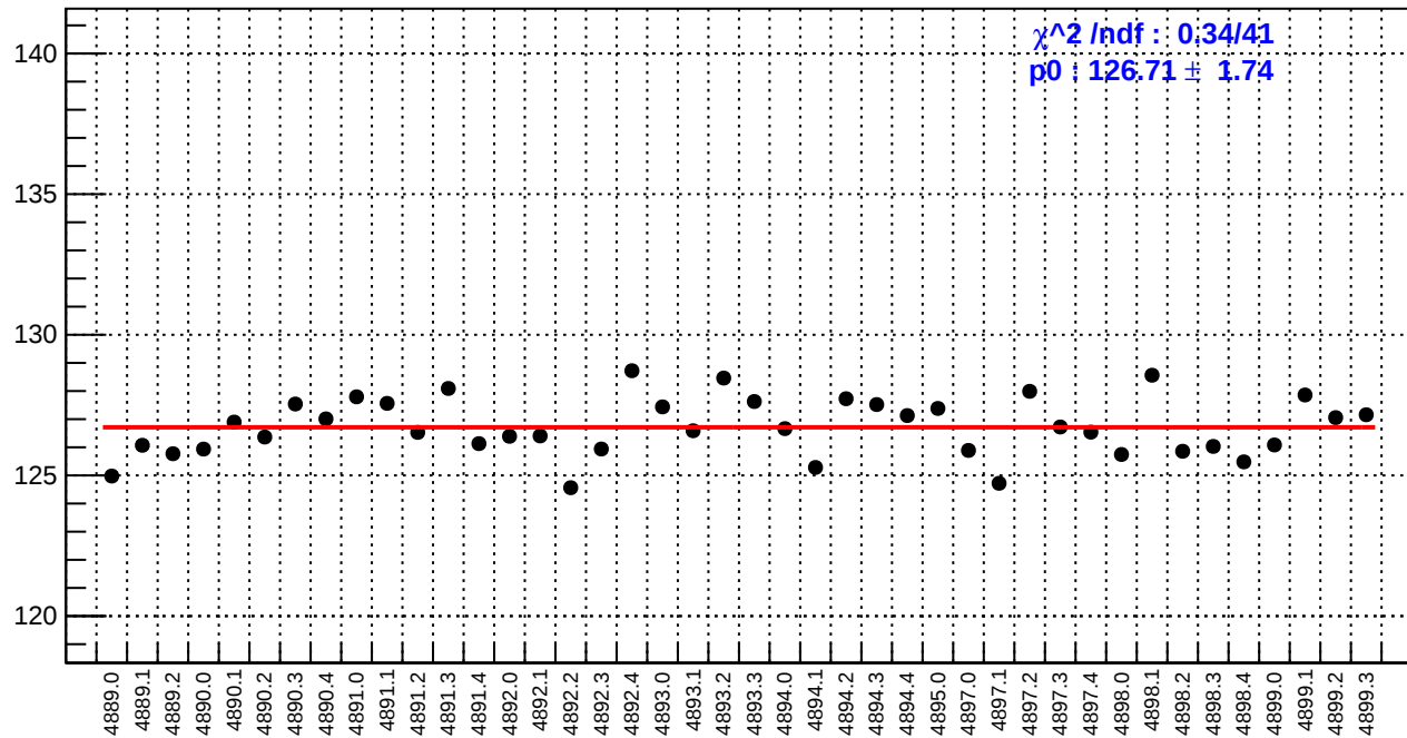
slug90: reg_asym_dsl.rms/ppm
