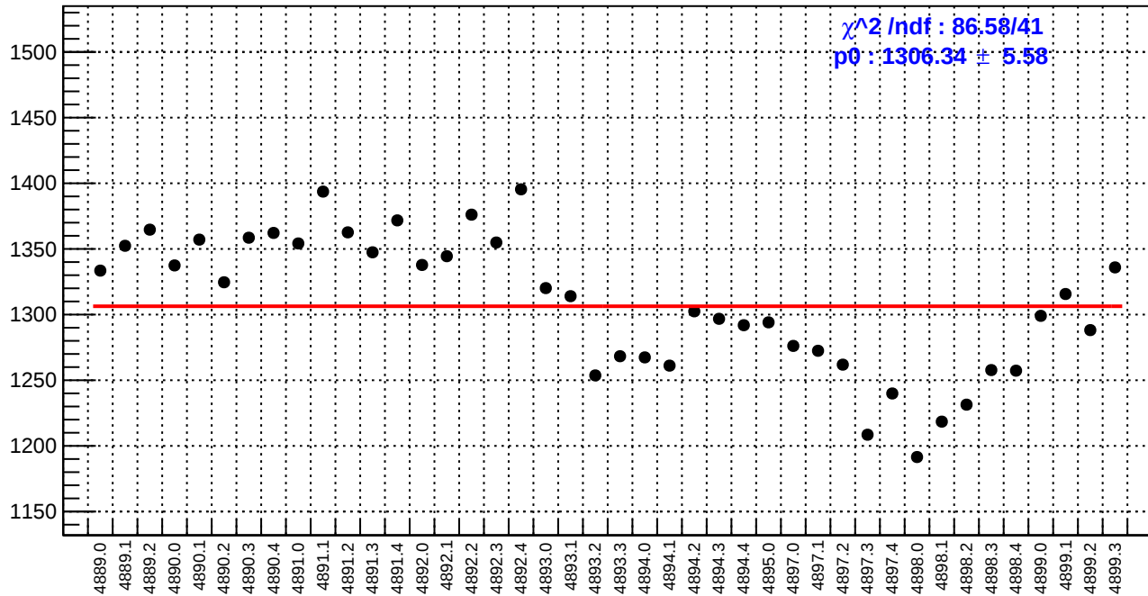
slug90: diff_bpm4aX.rms/nm
