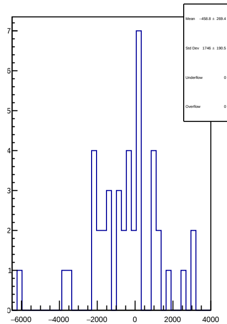
slug90: 1D Corr asym_atl1r2_avg.mean/ppb-reg_asym_atl1r2_avg.mean/ppb
