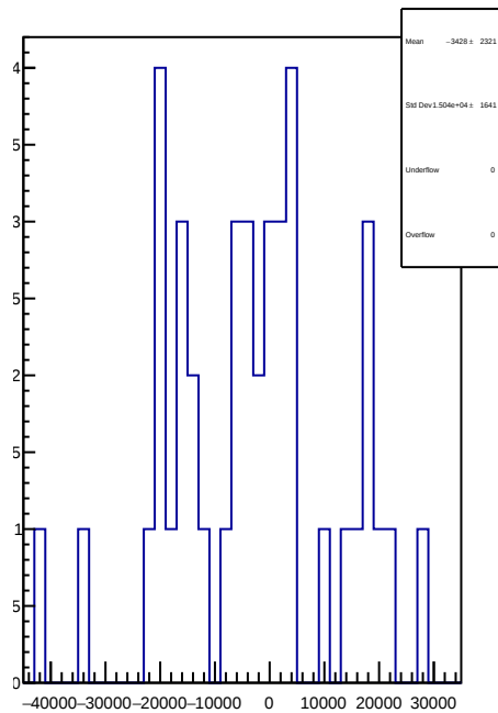
slug90: 1D Corr asym_sam6.mean/ppb-reg_asym_sam6.mean/ppb
