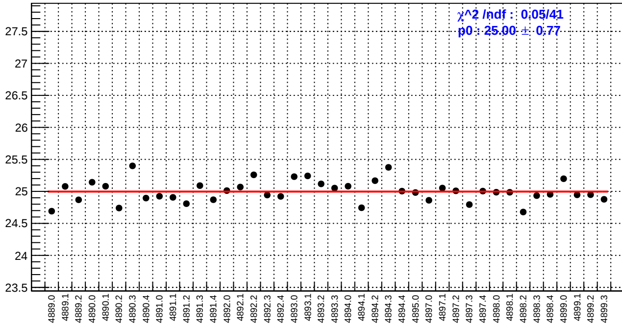
slug90: reg_asym_right_dd.rms/ppm
