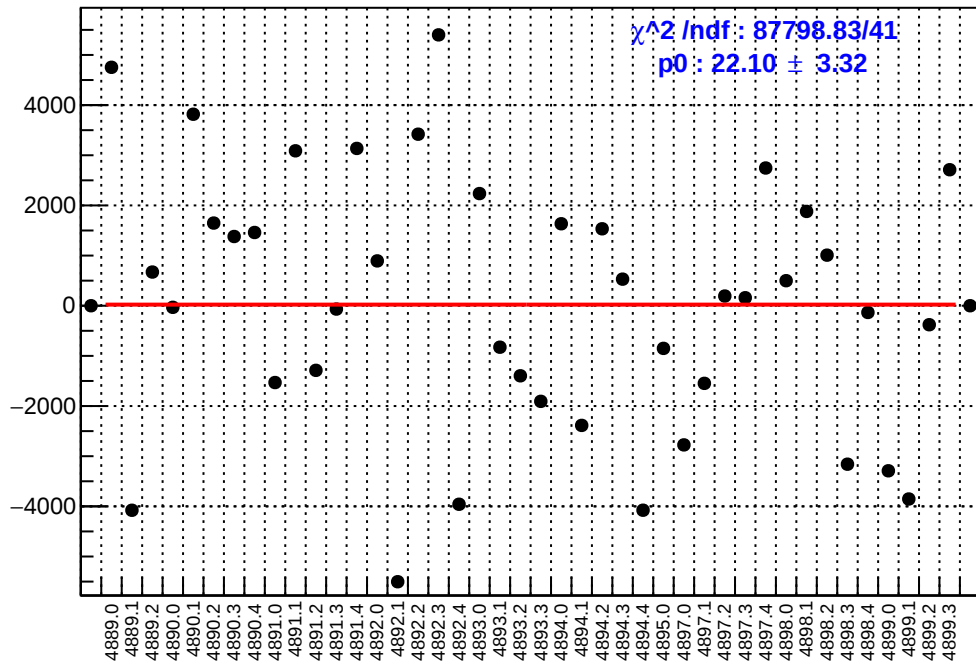
slug90: asym_at1_dd.mean/ppb-reg_asym_at1_dd.mean/ppb
