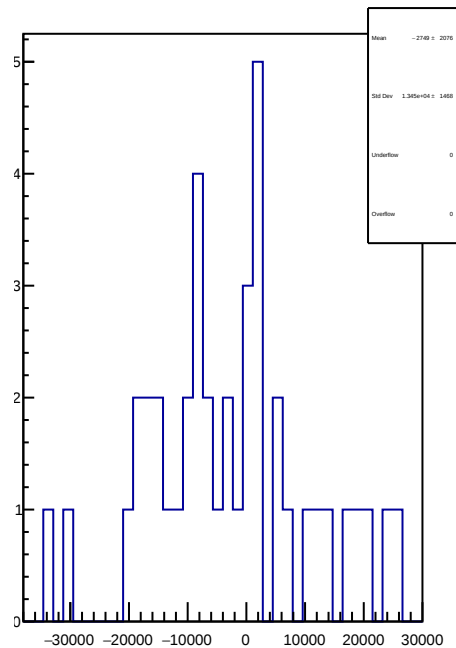
slug90: 1D Corr asym_sam7.mean/ppb-reg_asym_sam7.mean/ppb
