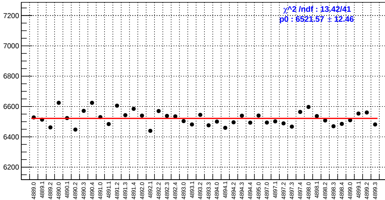
slug90: reg_asym_atr1l2_avg.rms/ppm
