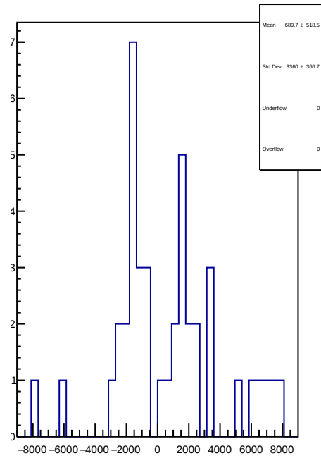
slug90: 1D Corr asym_right_avg.mean/ppb-reg_asym_right_avg.mean/ppb
