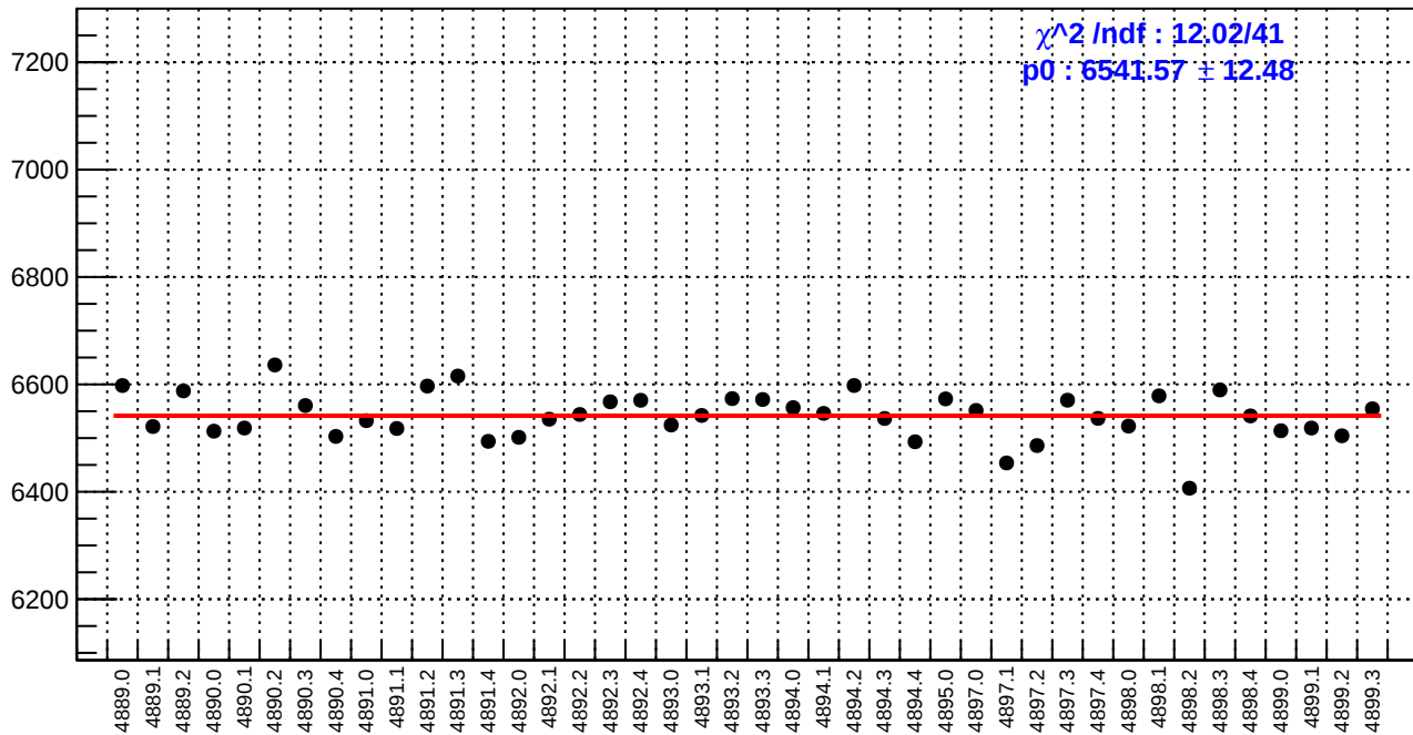
slug90: reg_asym_atr1l2_dd.rms/ppm
