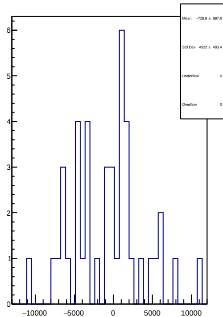
slug90: 1D Corr asym_atr2.mean/ppb-reg_asym_atr2.mean/ppb
