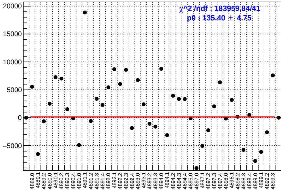
slug90: asym_dsl.mean/ppb-reg_asym_dsl.mean/ppb
