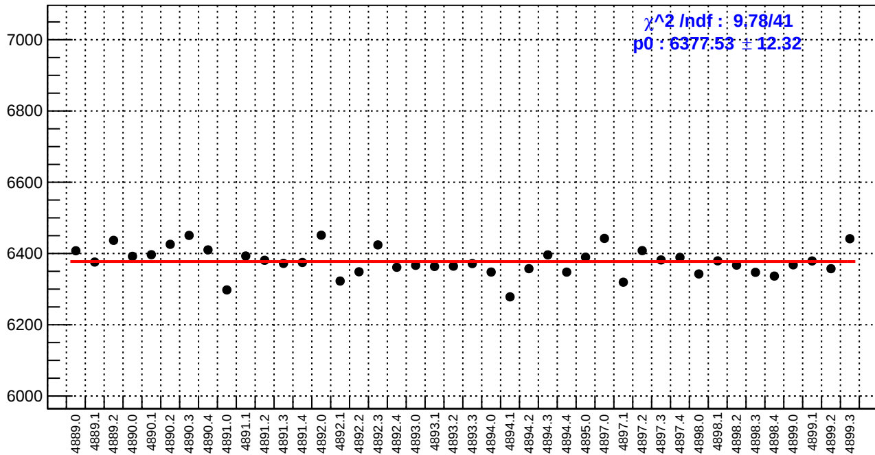
slug90: reg_asym_atl1r2_dd.rms/ppm
