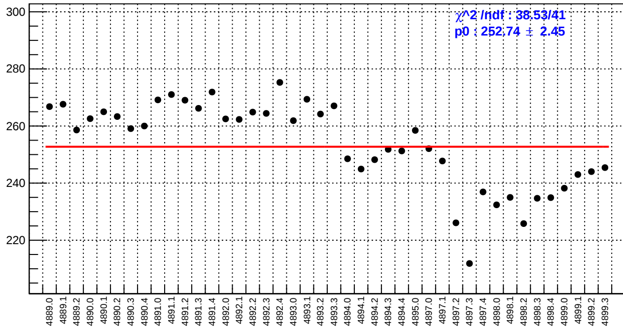
slug90: reg_asym_sam5.rms/ppm
