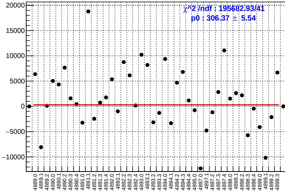
slug90: asym_atl2.mean/ppb-reg_asym_atl2.mean/ppb
