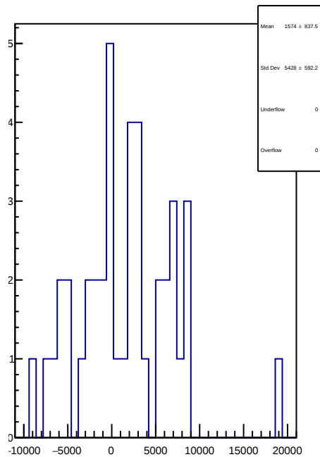
slug90: 1D Corr asym_dsl.mean/ppb-reg_asym_dsl.mean/ppb
