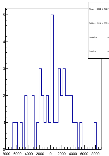
slug90: 1D Corr asym_ds_dd.mean/ppb-reg_asym_ds_dd.mean/ppb
