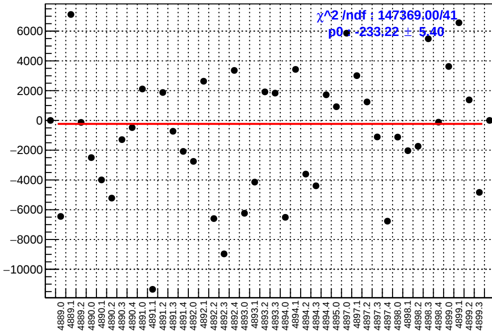
slug90: asym atr1l2 dd.mean/ppb-reg asym atr1l2 dd.mean/ppb
