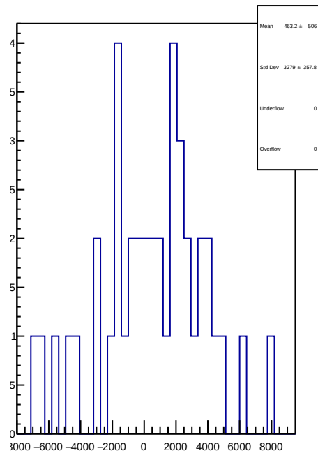
slug90: 1D Corr asym_us_dd.mean/ppb-reg_asym_us_dd.mean/ppb
