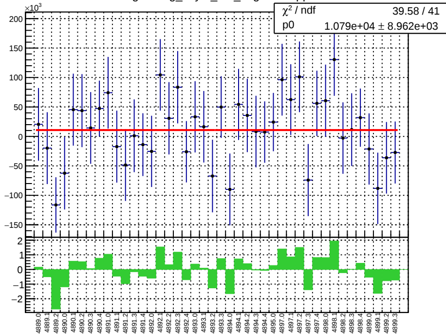
slug90: reg_asym_at1_avg.mean/ppb
