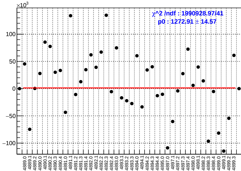
slug90: asym_sam3.mean/ppb-reg_asym_sam3.mean/ppb
