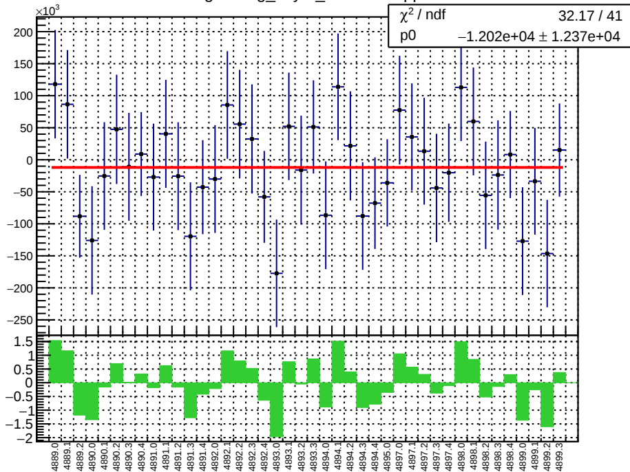
slug90: reg_asym_atl1.mean/ppb
