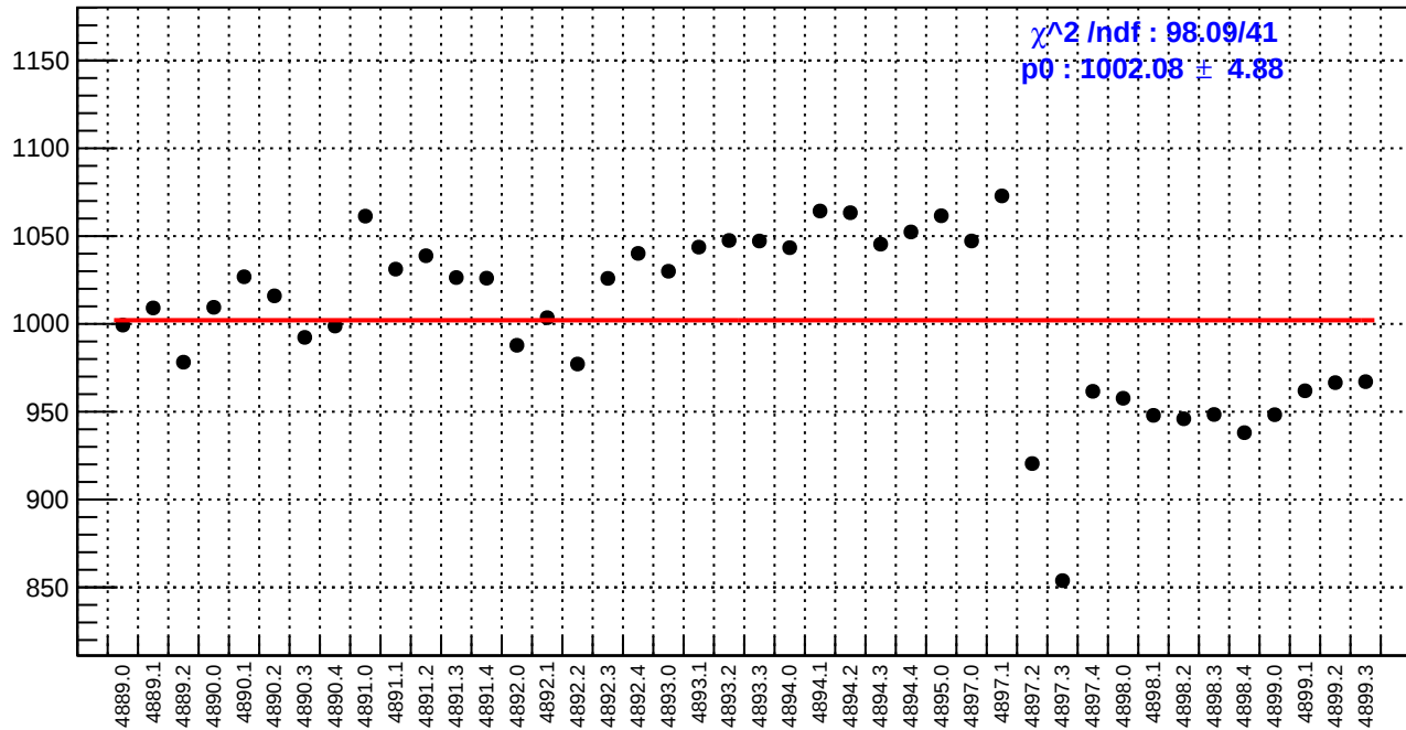
slug90: reg_asym_sam4.rms/ppm
