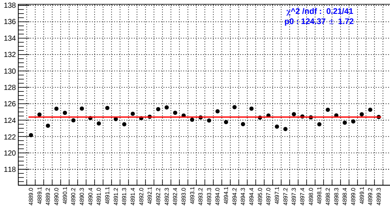
slug90: reg_asym_dsr.rms/ppm
