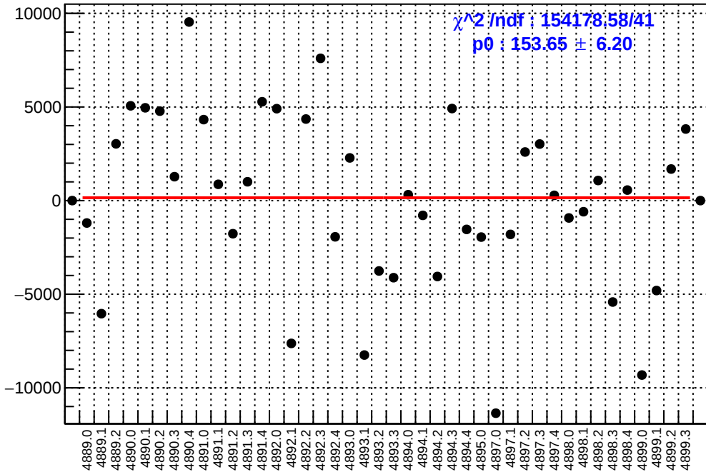
slug90: asym_sam5.mean/ppb-reg_asym_sam5.mean/ppb
