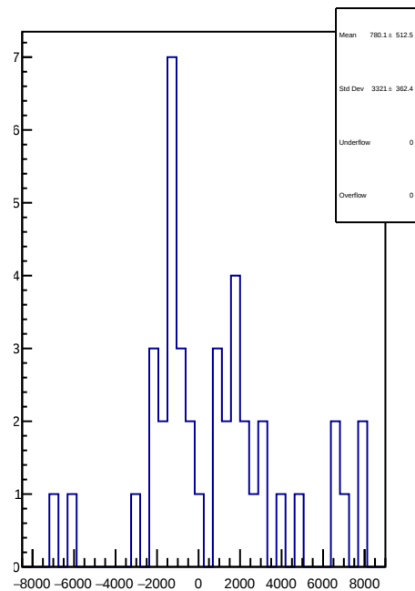
slug90: 1D Corr asym_dsr.mean/ppb-reg_asym_dsr.mean/ppb
