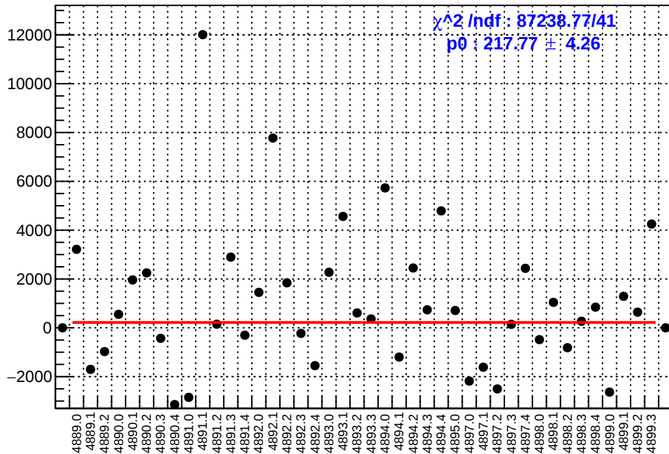
slug90: asym_us_avg.mean/ppb-reg_asym_us_avg.mean/ppb
