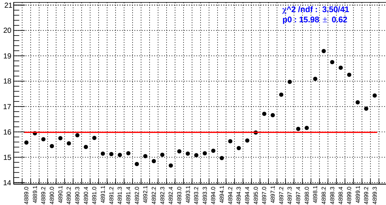
slug90: right_avg_bpm4eX/(ppb/nm)
