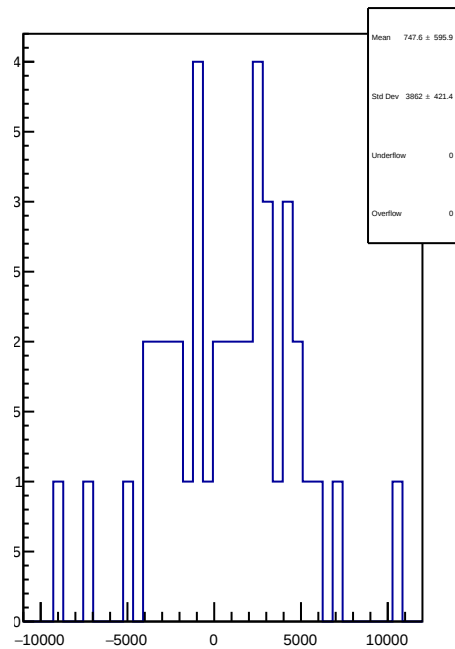
slug90: 1D Corr asym_atl_avg.mean/ppb-reg_asym_atl_avg.mean/ppb
