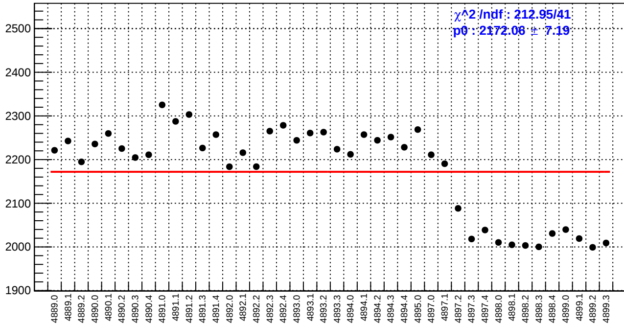
slug90: reg_asym_sam2.rms/ppm
