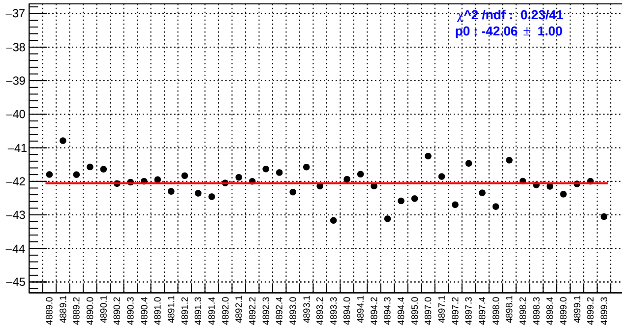
slug90: left_avg_bpm12X/(ppb/nm)
