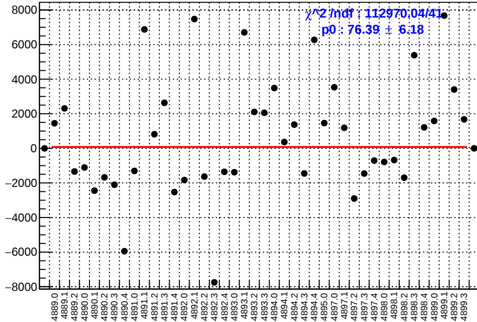
slug90: asym_right_avg.mean/ppb-reg_asym_right_avg.mean/ppb
