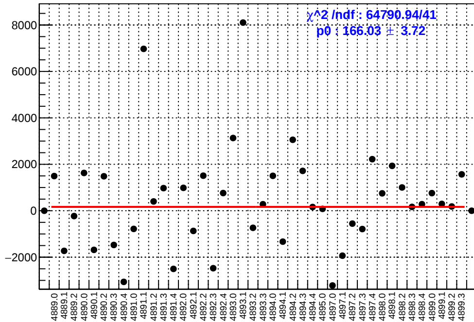
slug90: asym_at2_avg.mean/ppb-reg_asym_at2_avg.mean/ppb
