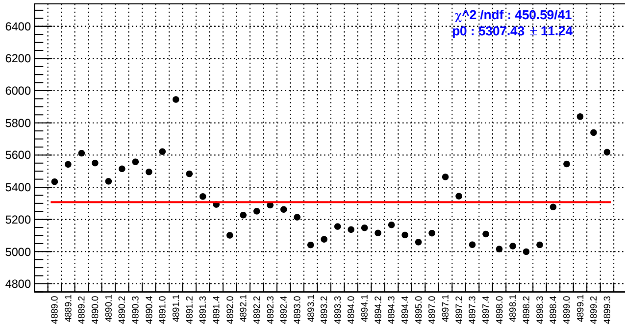
slug90: diff_bpm11X.rms/nm
