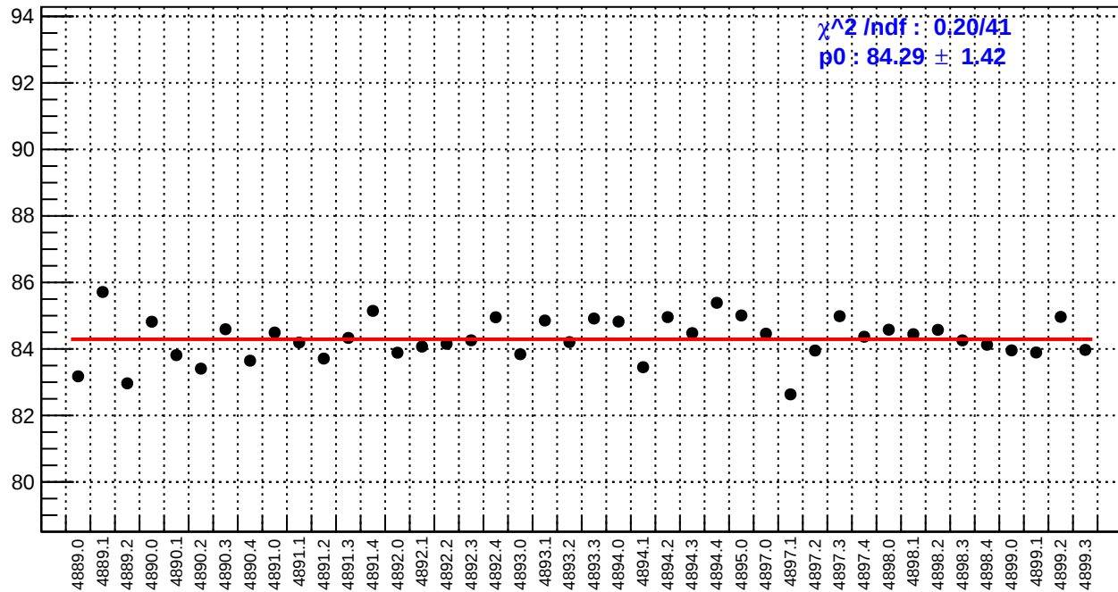
slug90: reg_asym_us_dd.rms/ppm
