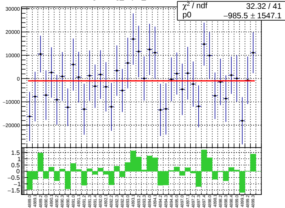
slug90: reg_asym_sam4.mean/ppb
