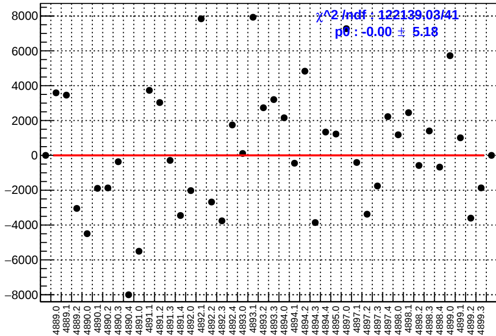
slug90: asym_sam1.mean/ppb-reg_asym_sam1.mean/ppb
