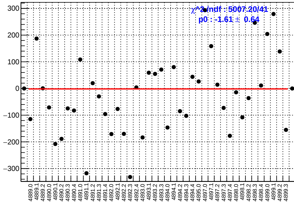
slug90: asym_left_dd.mean/ppb-reg_asym_left_dd.mean/ppb
