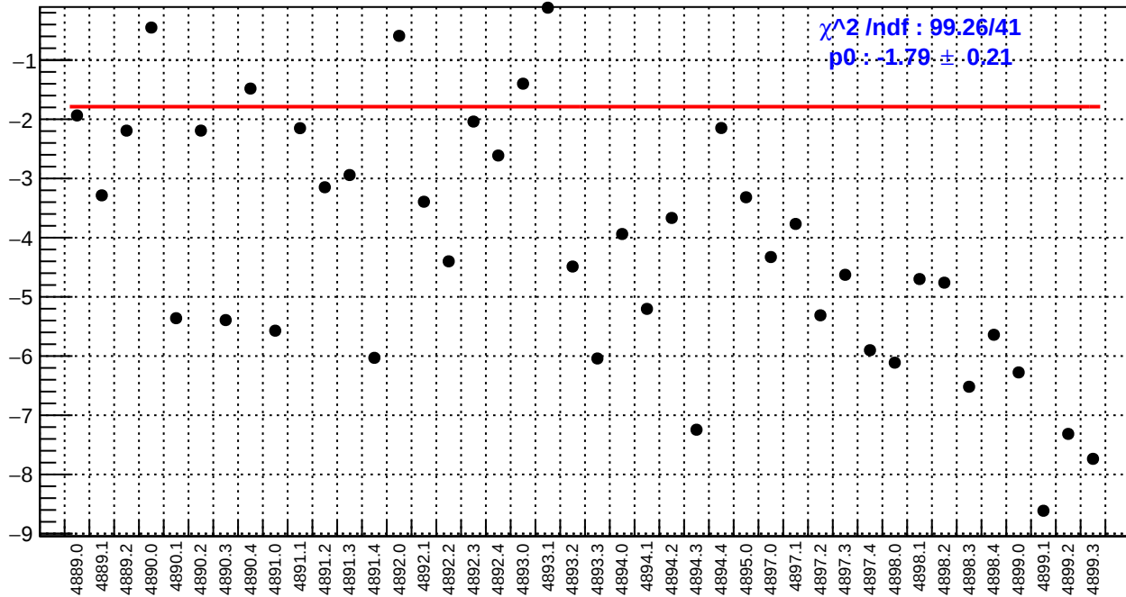
slug90: dsr_bpm4aY/(ppb/nm)
