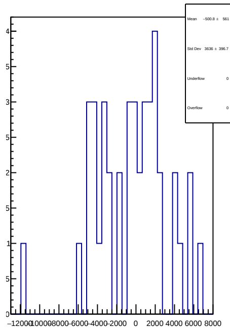
slug90: 1D Corr asym_atr_avg.mean/ppb-reg_asym_atr_avg.mean/ppb
