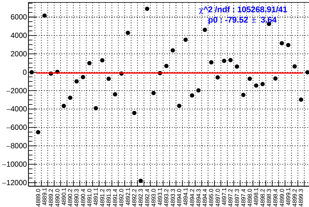
slug90: asym_atr1.mean/ppb-reg_asym_atr1.mean/ppb
