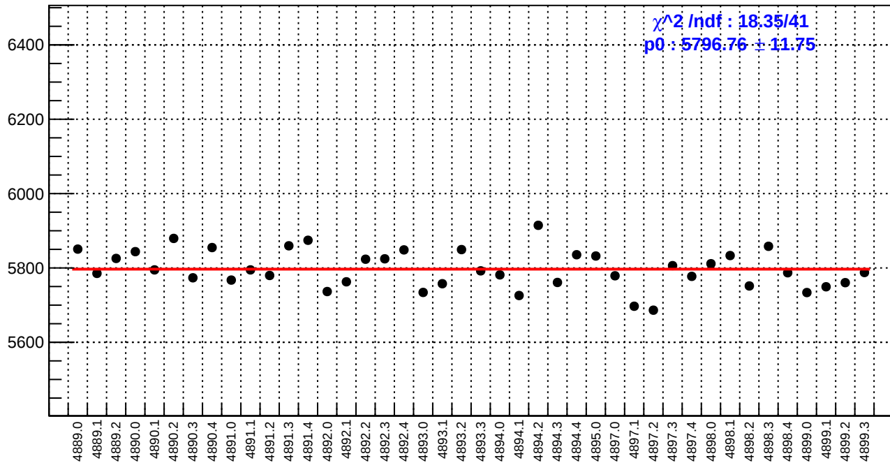
slug90: reg_asym_at1_avg.rms/ppm
