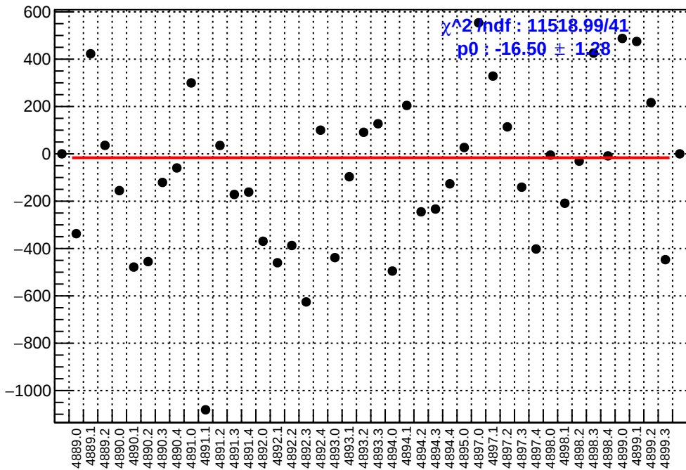
slug90: asym_right_dd.mean/ppb-reg_asym_right_dd.mean/ppb
