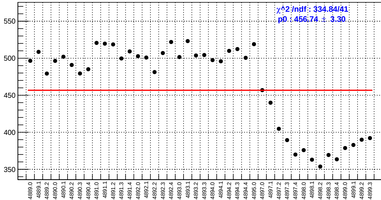
slug90: reg_asym_sam6.rms/ppm
