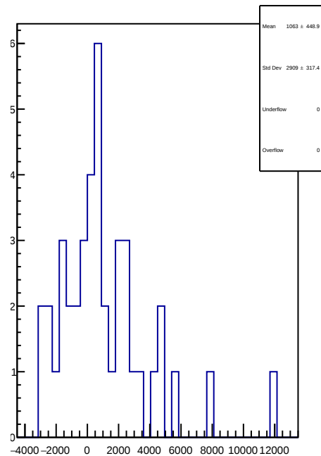
slug90: 1D Corr asym_us_avg.mean/ppb-reg_asym_us_avg.mean/ppb
