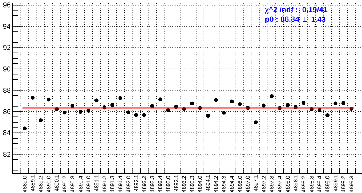
slug90: reg_asym_ds_dd.rms/ppm
