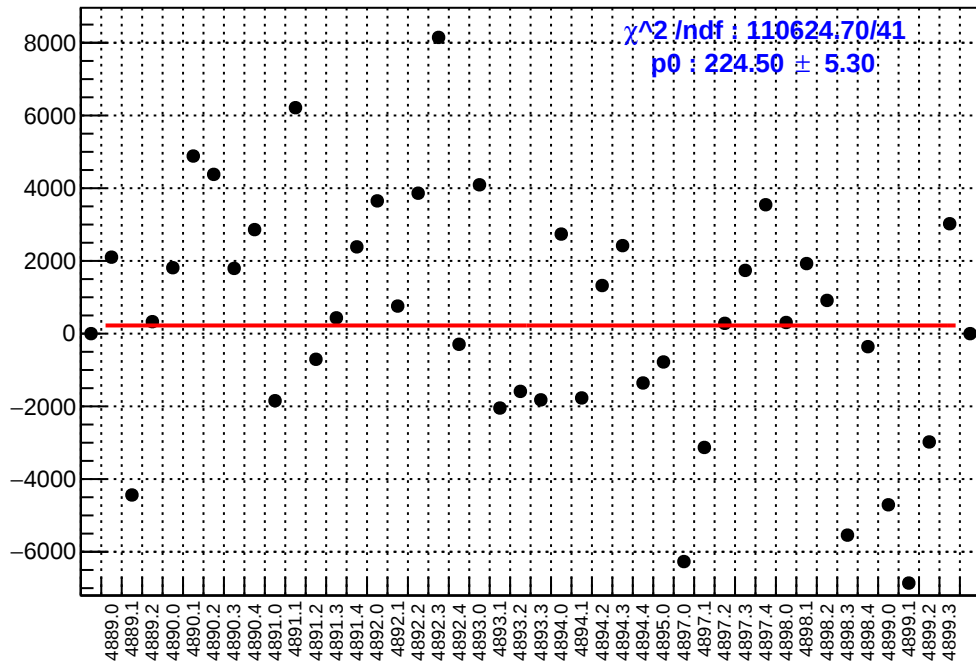
slug90: asym_us_dd.mean/ppb-reg_asym_us_dd.mean/ppb
