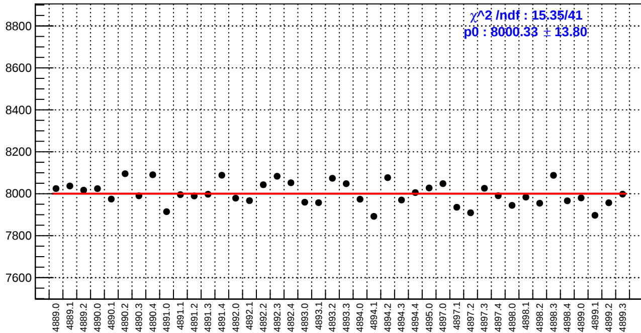
slug90: reg_asym_atl1.rms/ppm
