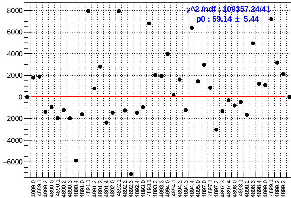
slug90: asym_dsr.mean/ppb-reg_asym_dsr.mean/ppb
