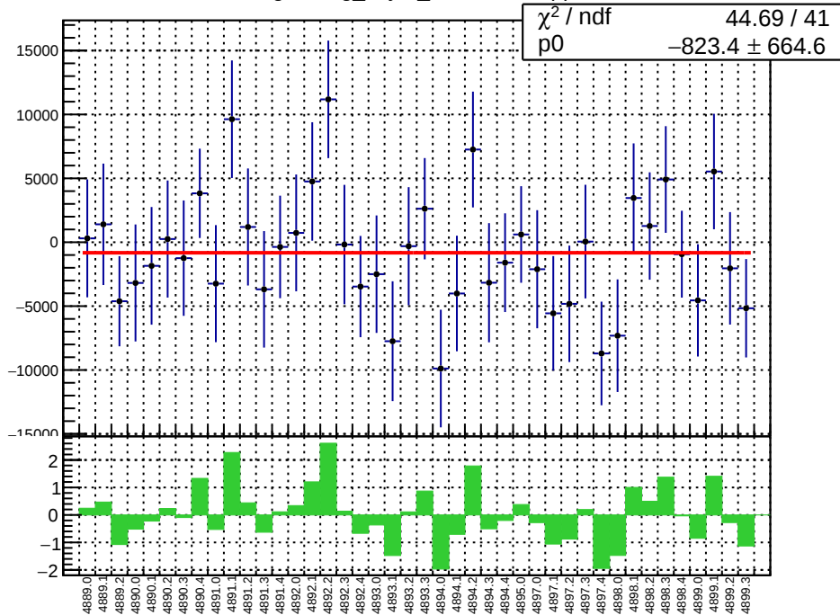
slug90: reg_asym_sam8.mean/ppb
