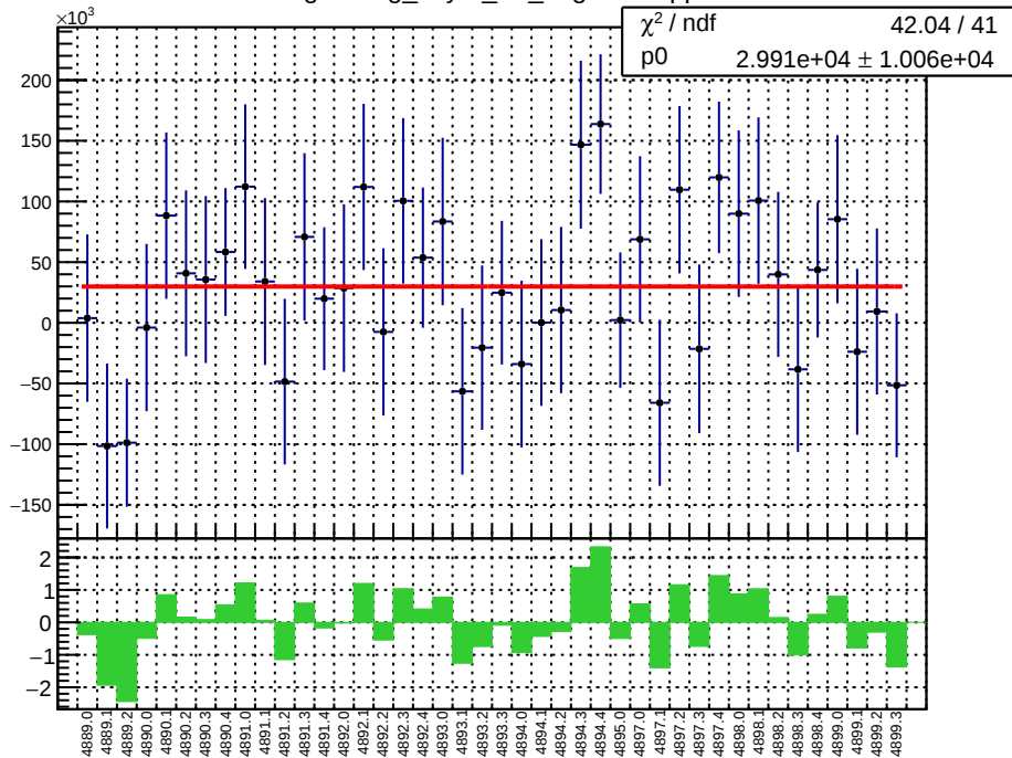
slug90: reg_asym_atr_avg.mean/ppb
