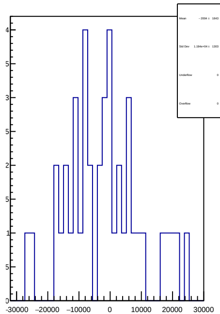
slug90: 1D Corr asym_sam8.mean/ppb-reg_asym_sam8.mean/ppb
