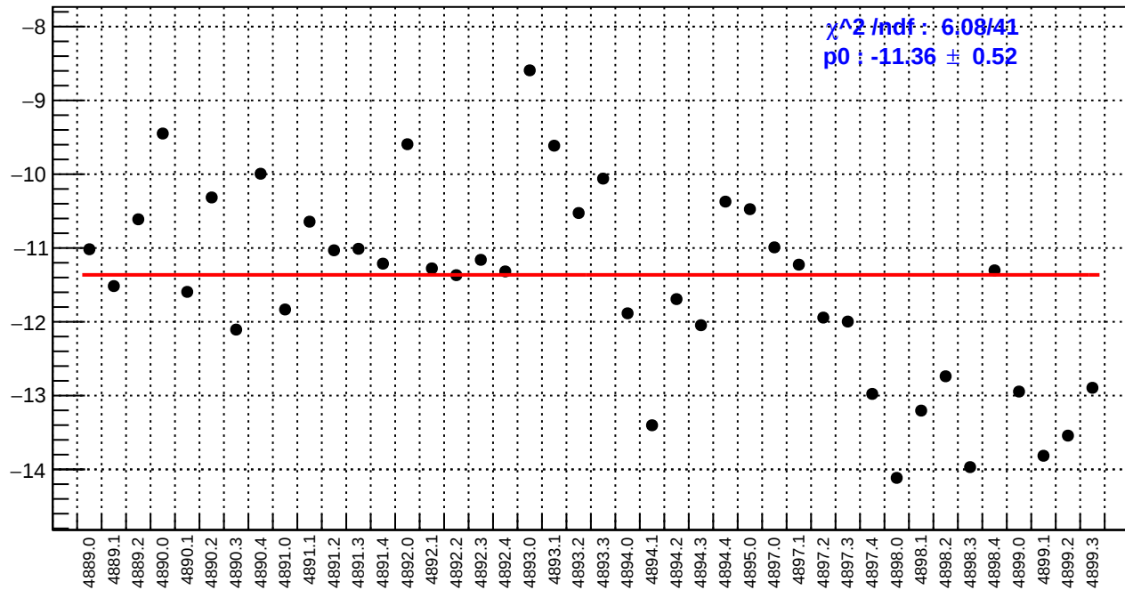
slug90: ds_avg_bpm4aY/(ppb/nm)
