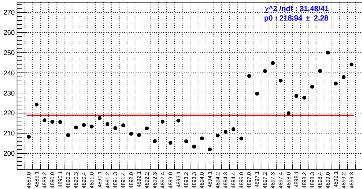
slug90: reg_asym_sam1.rms/ppm
