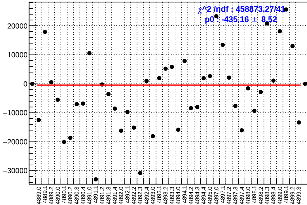
slug90: asym_sam7.mean/ppb-reg_asym_sam7.mean/ppb
