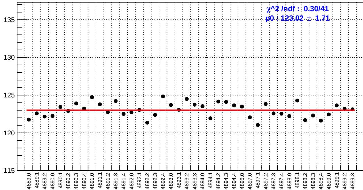
slug90: reg_asym_left_avg.rms/ppm
