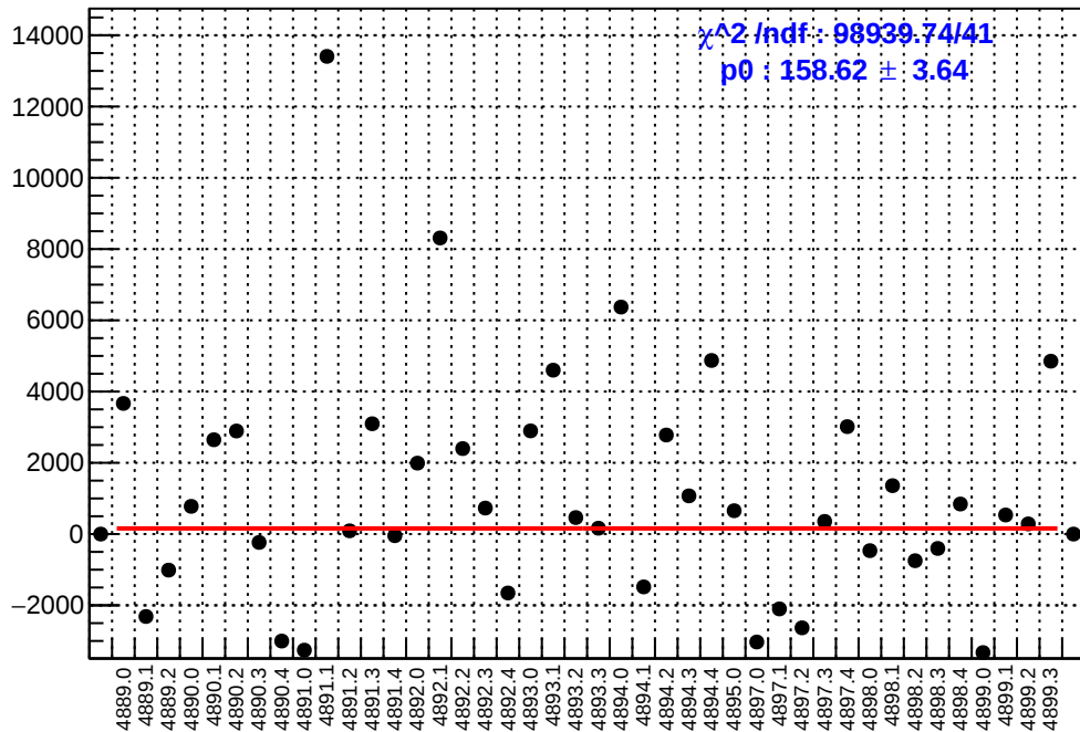
slug90: asym_ds_avg.mean/ppb-reg_asym_ds_avg.mean/ppb
