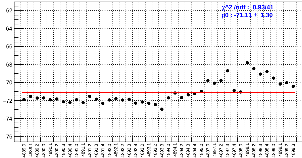
slug90: left_avg_bpm4eX/(ppb/nm)
