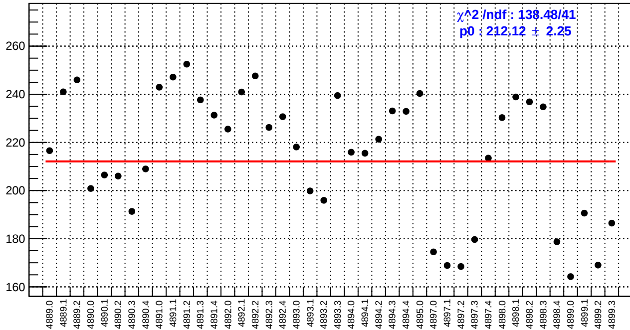
slug90: asym_bcm_an_ds3.rms/ppm
