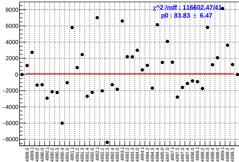
slug90: asym_usr.mean/ppb-reg_asym_usr.mean/ppb
