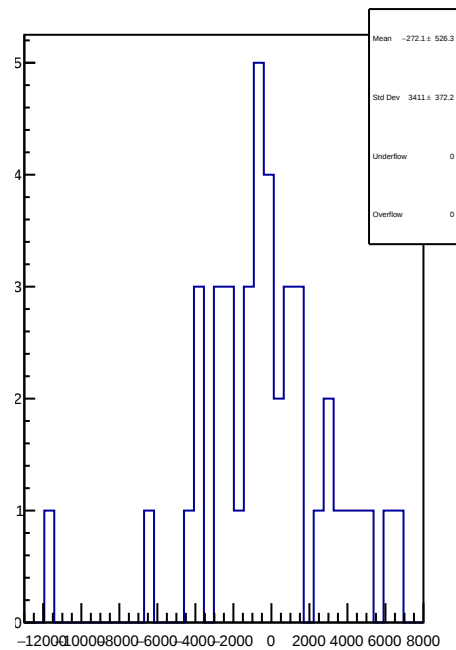
slug90: 1D Corr asym_atr1.mean/ppb-reg_asym_atr1.mean/ppb
