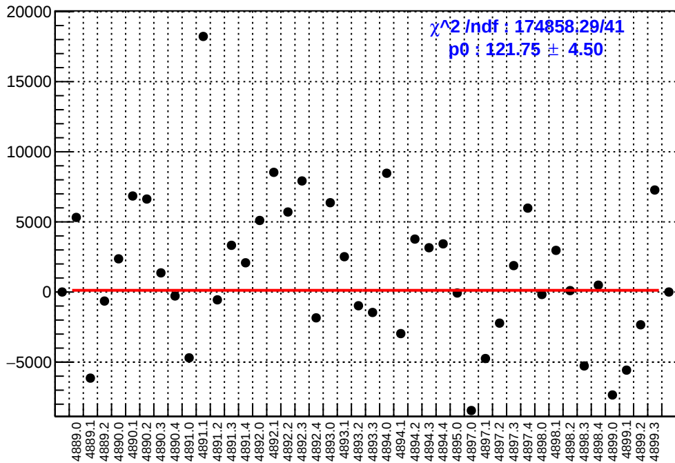
slug90: asym_usl.mean/ppb-reg_asym_usl.mean/ppb
