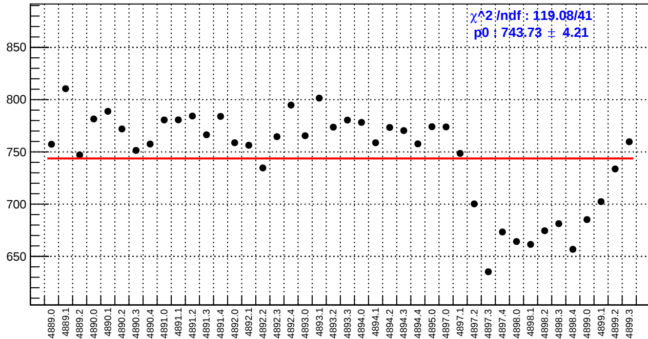
slug90: reg_asym_sam3.rms/ppm
