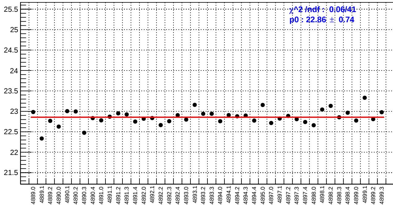
slug90: reg_asym_left_dd.rms/ppm
