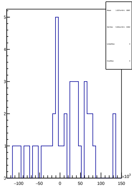
slug90: 1D Corr asym_sam3.mean/ppb-reg_asym_sam3.mean/ppb
