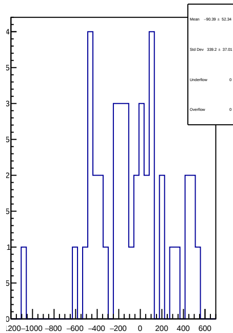
slug90: 1D Corr asym_right_dd.mean/ppb-reg_asym_right_dd.mean/ppb
