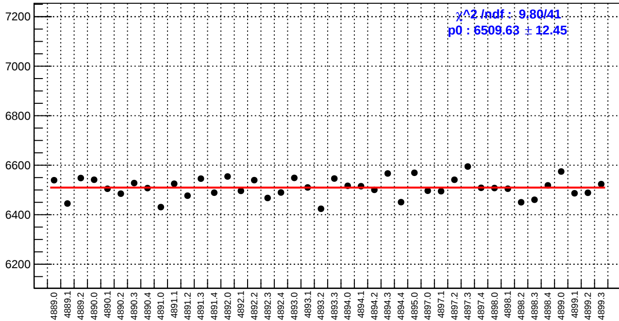
slug90: reg_asym_atr_avg.rms/ppm
