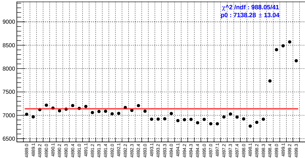
slug90: diff_bpm4eX.rms/nm
