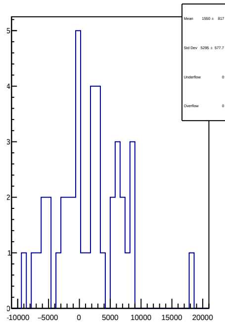
slug90: 1D Corr asym_left_avg.mean/ppb-reg_asym_left_avg.mean/ppb
