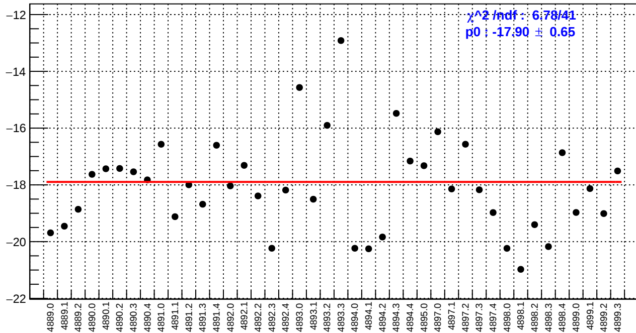
slug90: usl_bpm4aY/(ppb/nm)
