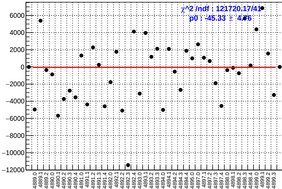
slug90: asym_atr_avg.mean/ppb-reg_asym_atr_avg.mean/ppb
