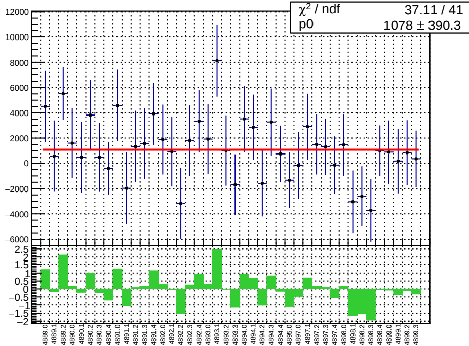
slug90: reg_asym_sam5.mean/ppb
