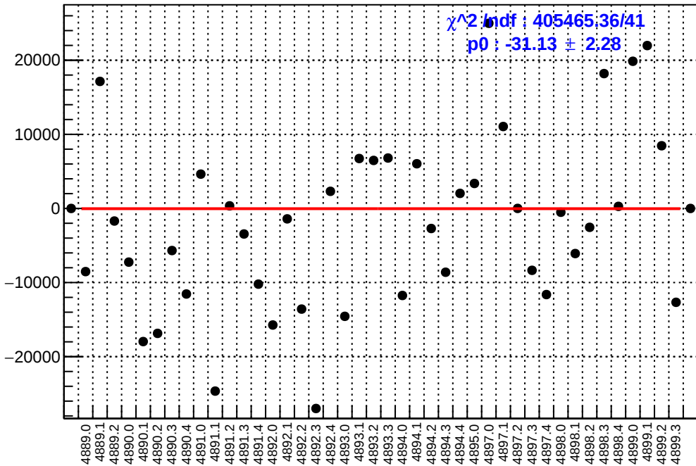
slug90: asym_sam8.mean/ppb-reg_asym_sam8.mean/ppb
