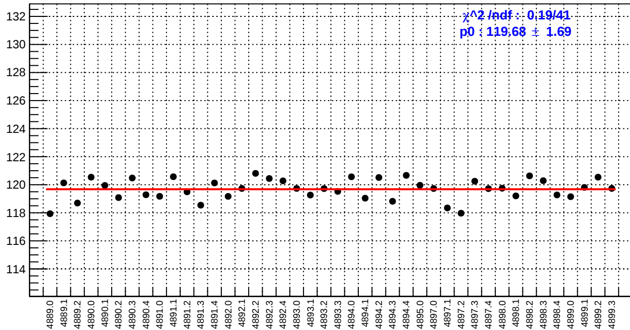
slug90: reg_asym_right_avg.rms/ppm
