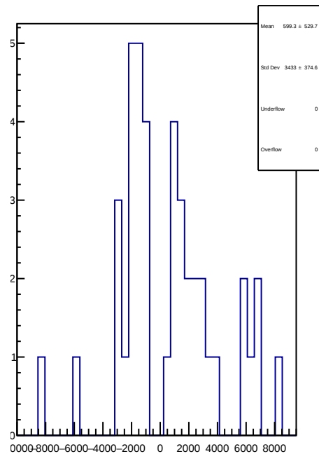
slug90: 1D Corr asym_usr.mean/ppb-reg_asym_usr.mean/ppb
