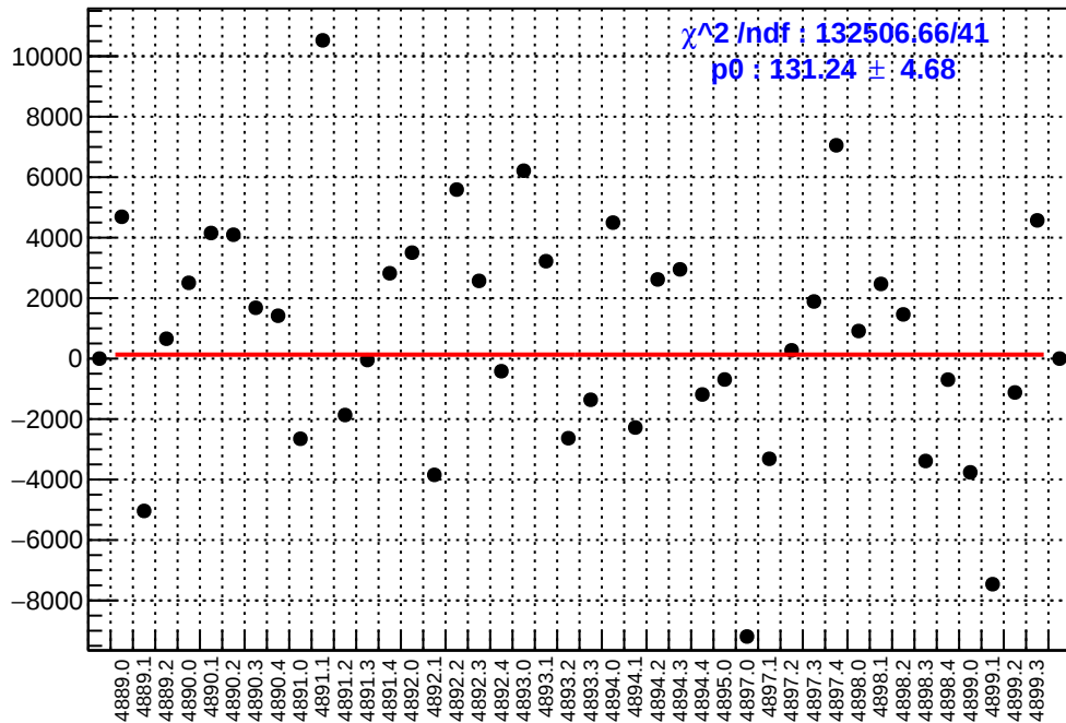
slug90: asym_atl_avg.mean/ppb-reg_asym_atl_avg.mean/ppb
