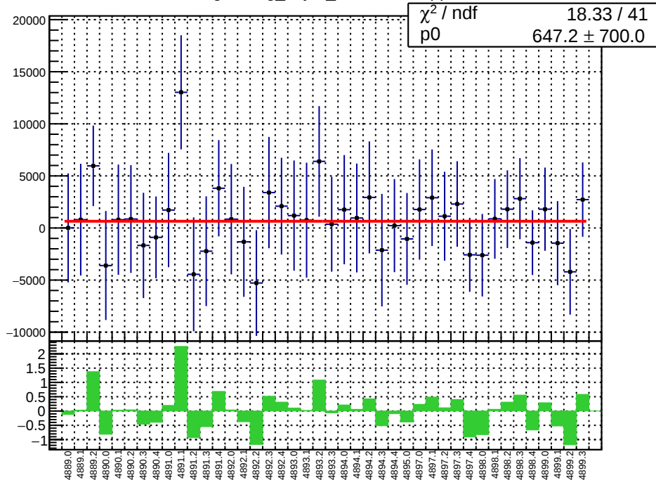
slug90: reg_asym_sam6.mean/ppb
