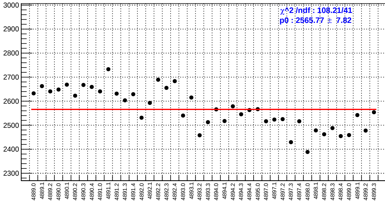
slug90: diff_bpm4aY.rms/nm
