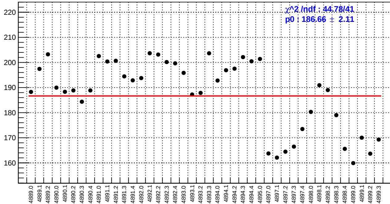
slug90: asym_bcm_an_us.rms/ppm
