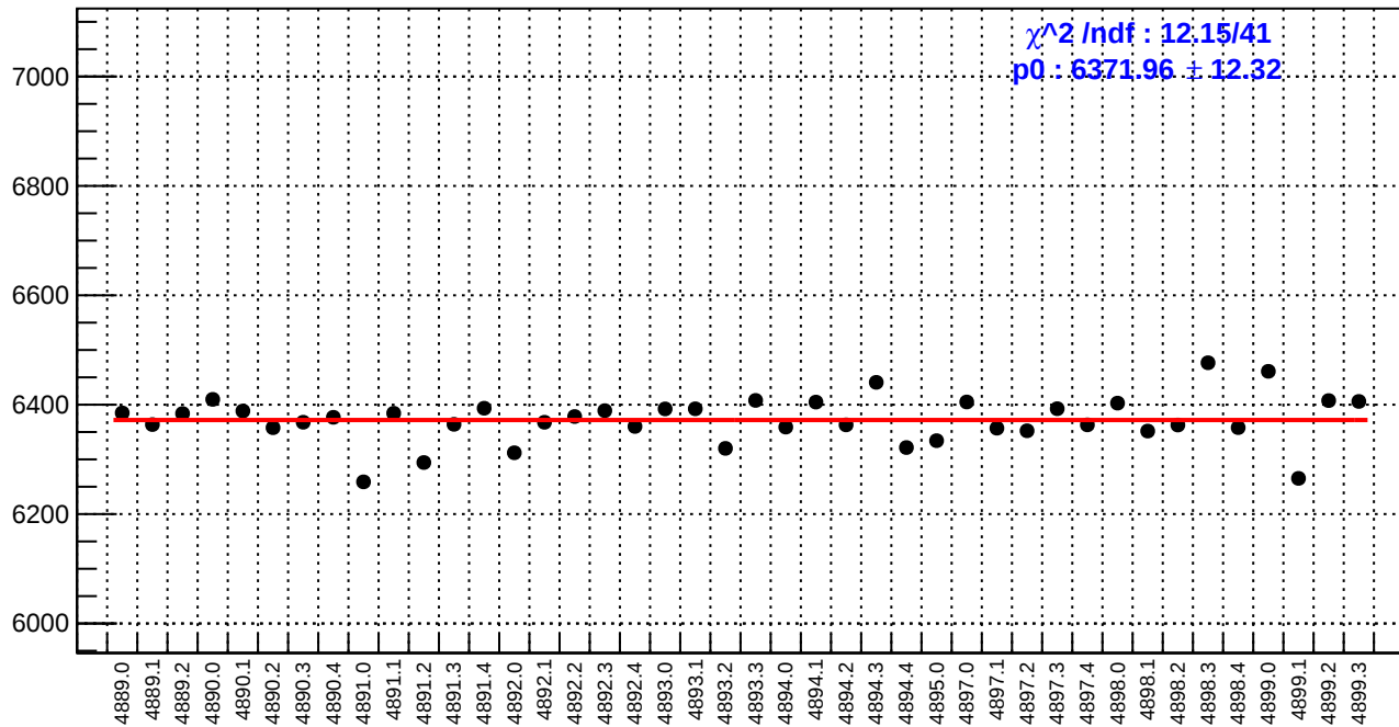
slug90: reg_asym_atl1r2_avg.rms/ppm
