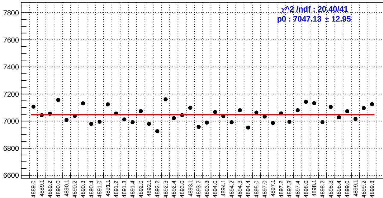
slug90: reg_asym_at2_dd.rms/ppm
