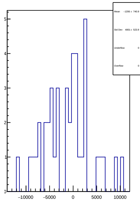
slug90: 1D Corr asym_at2_dd.mean/ppb-reg_asym_at2_dd.mean/ppb
