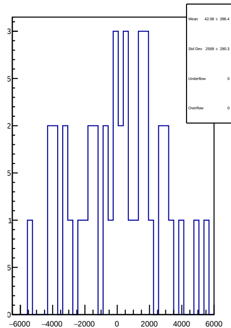
slug90: 1D Corr asym_at1_dd.mean/ppb-reg_asym_at1_dd.mean/ppb
