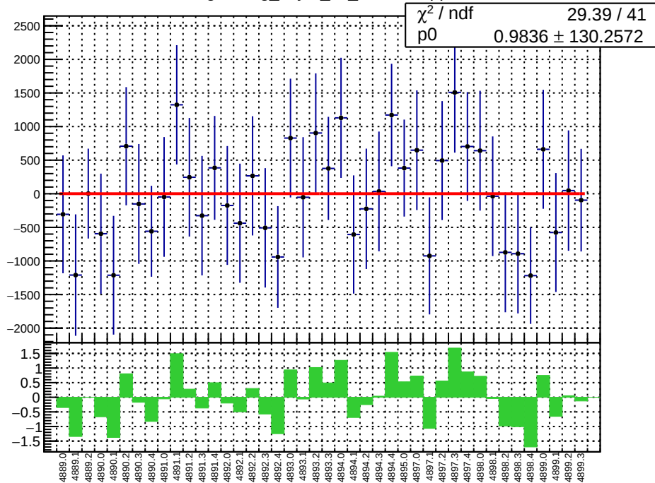
slug90: reg_asym_us_dd.mean/ppb
