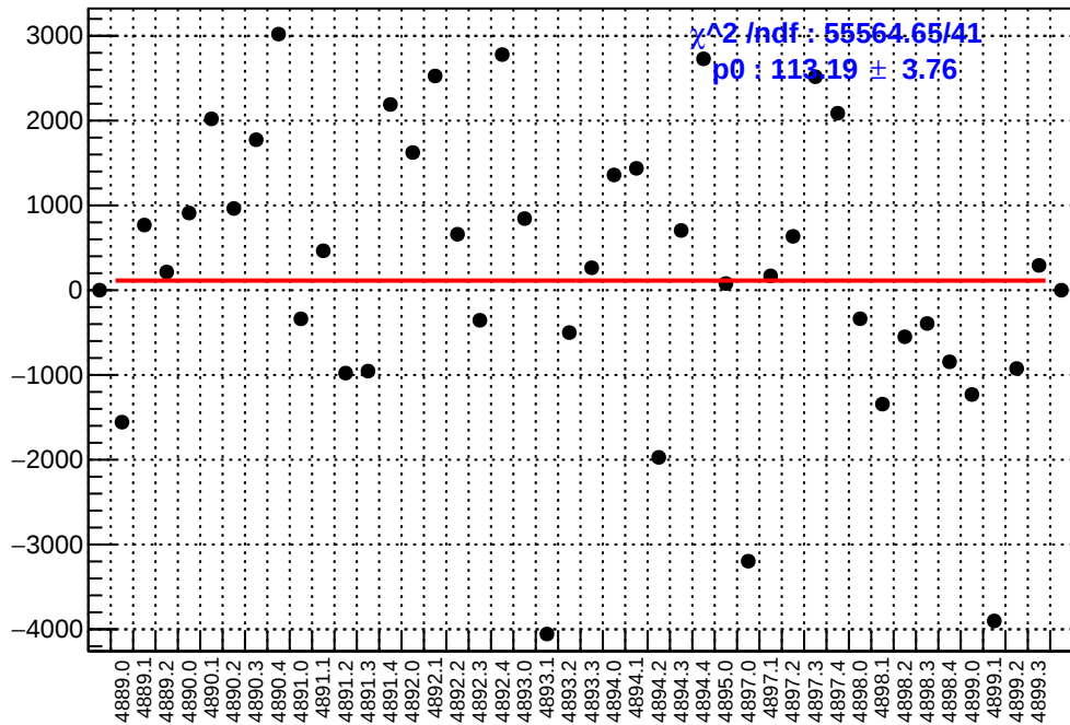
slug90: asym_atr_dd.mean/ppb-reg_asym_atr_dd.mean/ppb
