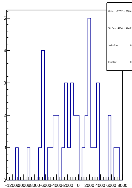
slug90: 1D Corr asym_atr1l2_dd.mean/ppb-reg_asym_atr1l2_dd.mean/ppb
