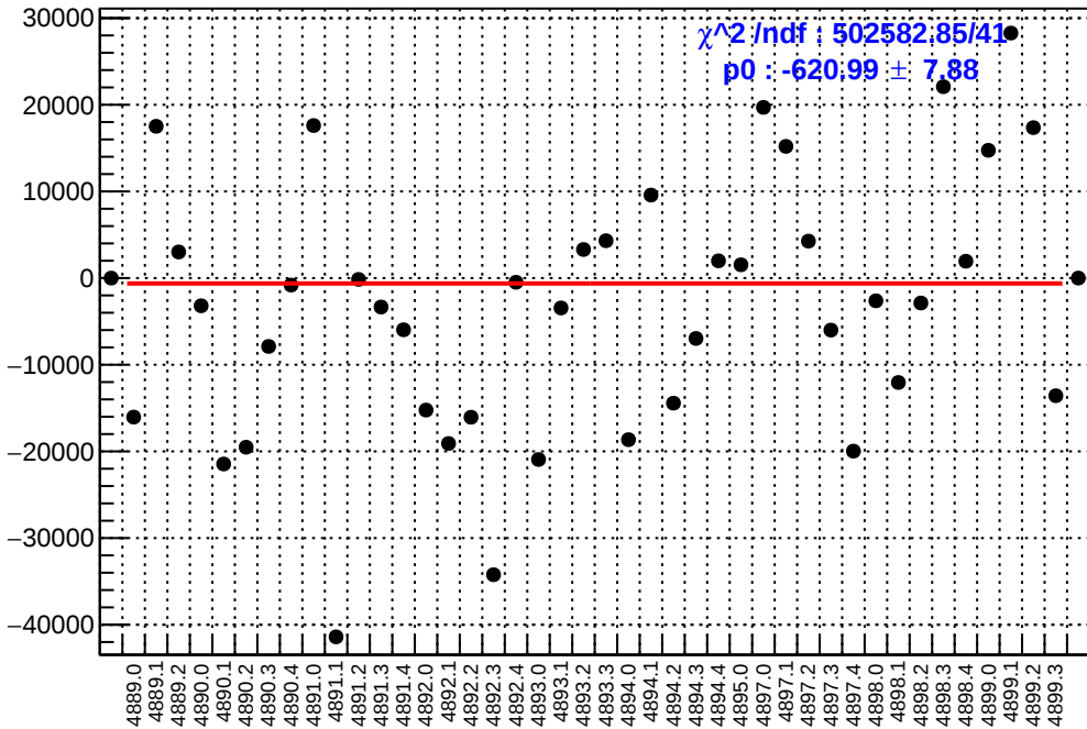
slug90: asym_sam6.mean/ppb-reg_asym_sam6.mean/ppb
