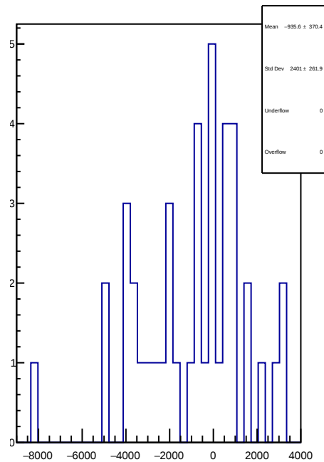
slug90: 1D Corr asym_atl_dd.mean/ppb-reg_asym_atl_dd.mean/ppb
