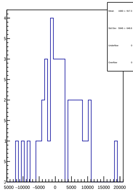
slug90: 1D Corr asym_atl2.mean/ppb-reg_asym_atl2.mean/ppb
