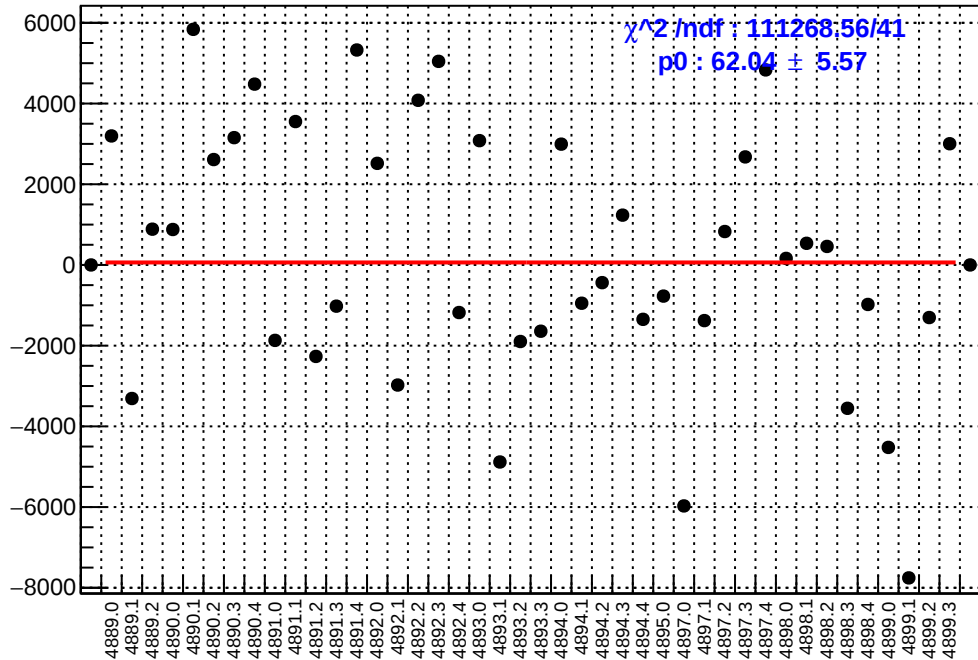
slug90: asym_atl1r2_dd.mean/ppb-reg_asym_atl1r2_dd.mean/ppb
