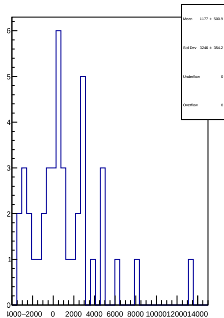
slug90: 1D Corr asym_ds_avg.mean/ppb-reg_asym_ds_avg.mean/ppb
