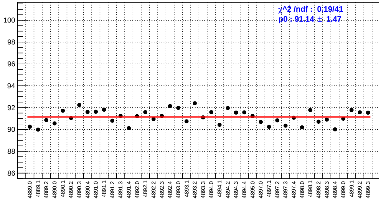
slug90: reg_asym_ds_avg.rms/ppm
