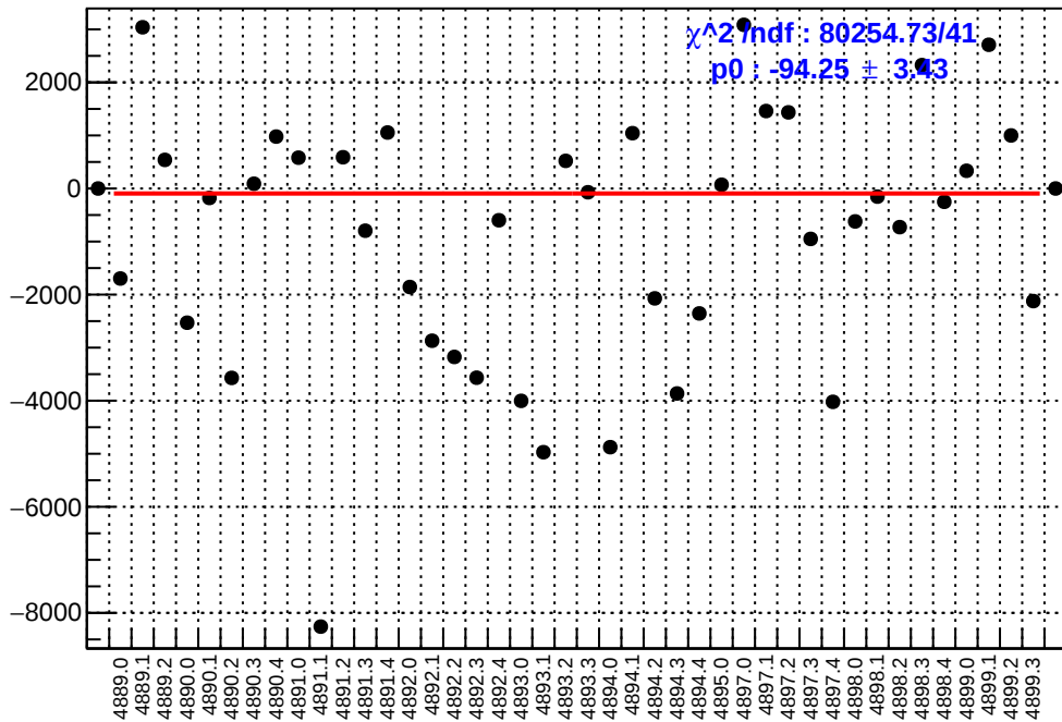
slug90: asym_atl_dd.mean/ppb-reg_asym_atl_dd.mean/ppb
