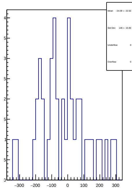
slug90: 1D Corr asym_left_dd.mean/ppb-reg_asym_left_dd.mean/ppb
