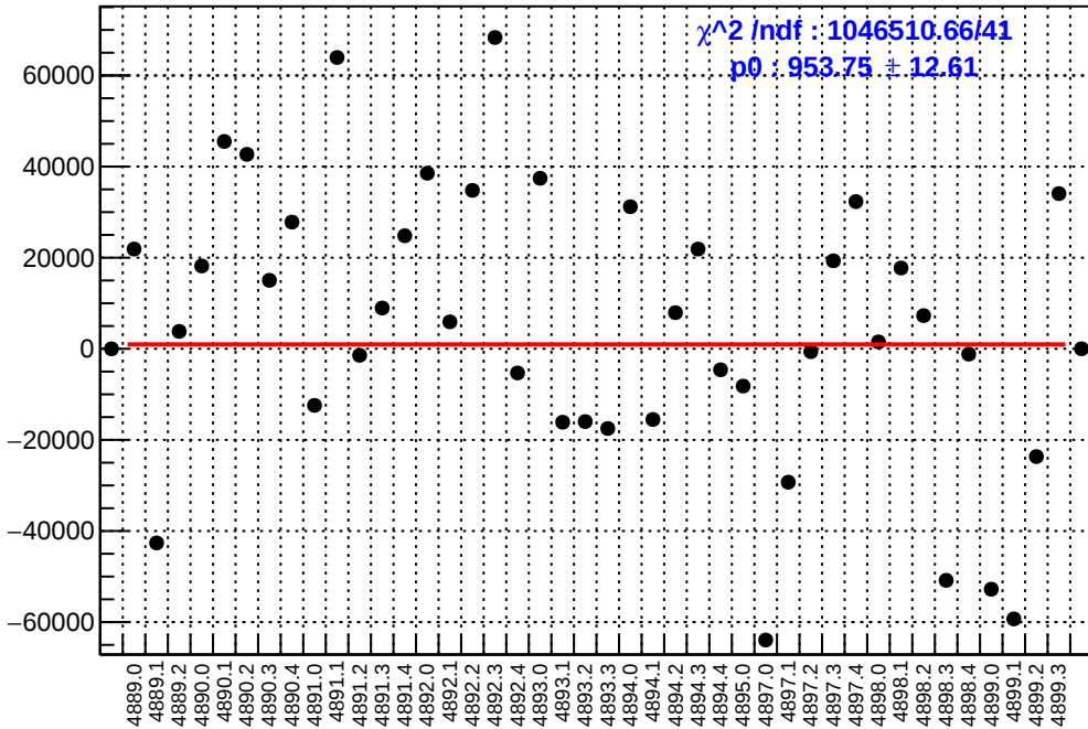
slug90: asym_sam4.mean/ppb-reg_asym_sam4.mean/ppb
