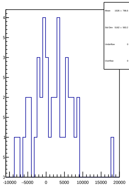
slug90: 1D Corr asym_usl.mean/ppb-reg_asym_usl.mean/ppb
