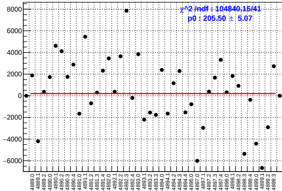
slug90: asym_ds_dd.mean/ppb-reg_asym_ds_dd.mean/ppb
