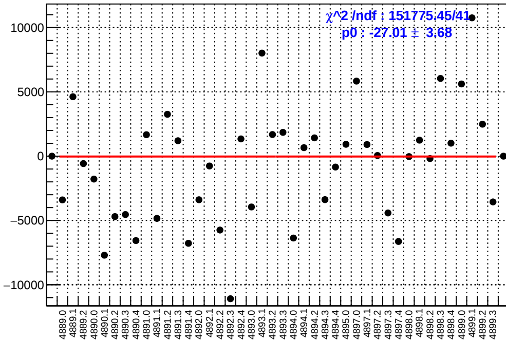
slug90: asym_atr2.mean/ppb-reg_asym_atr2.mean/ppb
