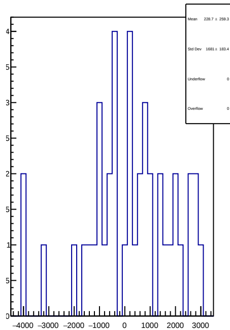
slug90: 1D Corr asym_atr_dd.mean/ppb-reg_asym_atr_dd.mean/ppb
