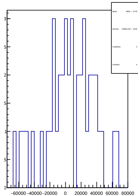
slug90: 1D Corr asym_sam4.mean/ppb-reg_asym_sam4.mean/ppb
