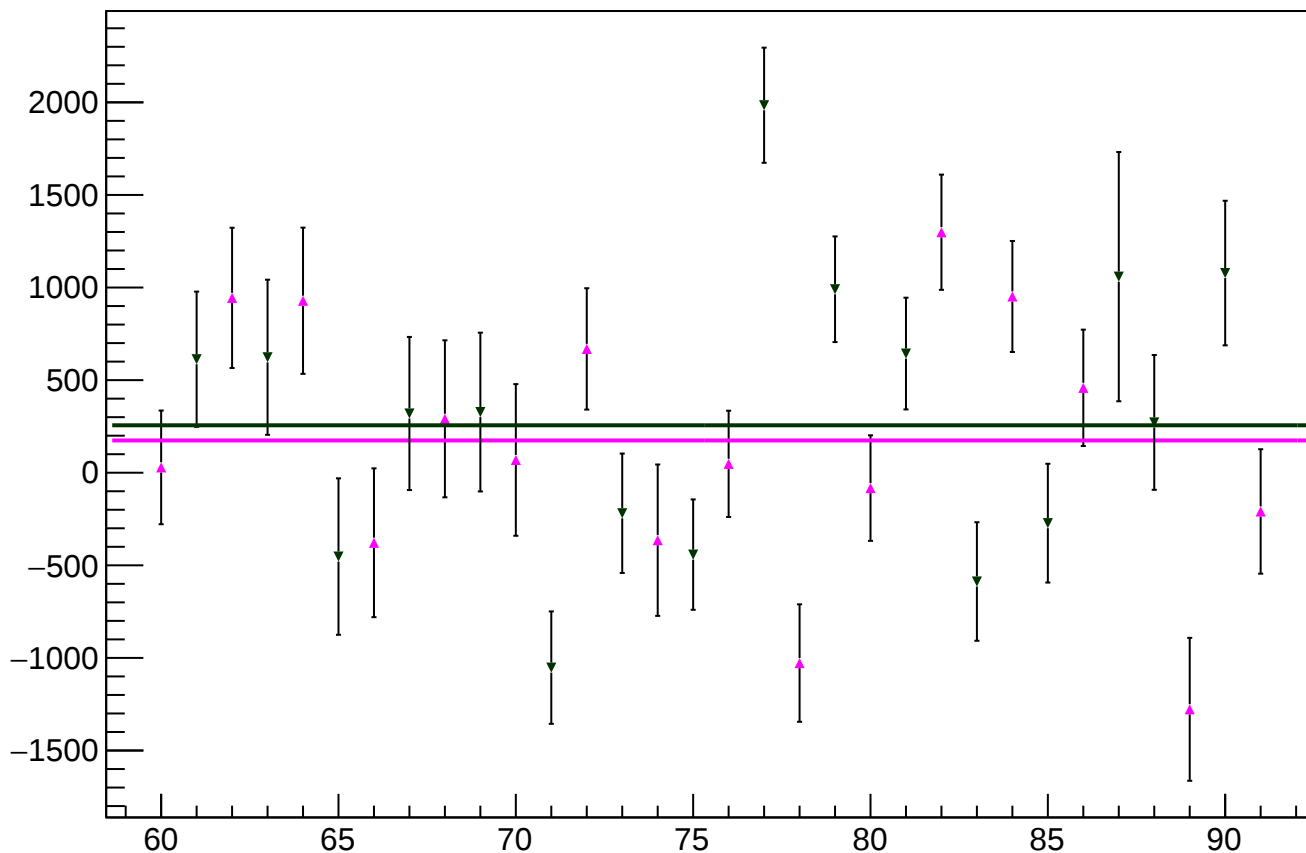
reg_asym_sam5_mean vs slug
