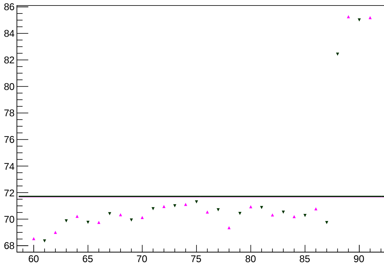
yield_cav4cQ_mean vs slug
