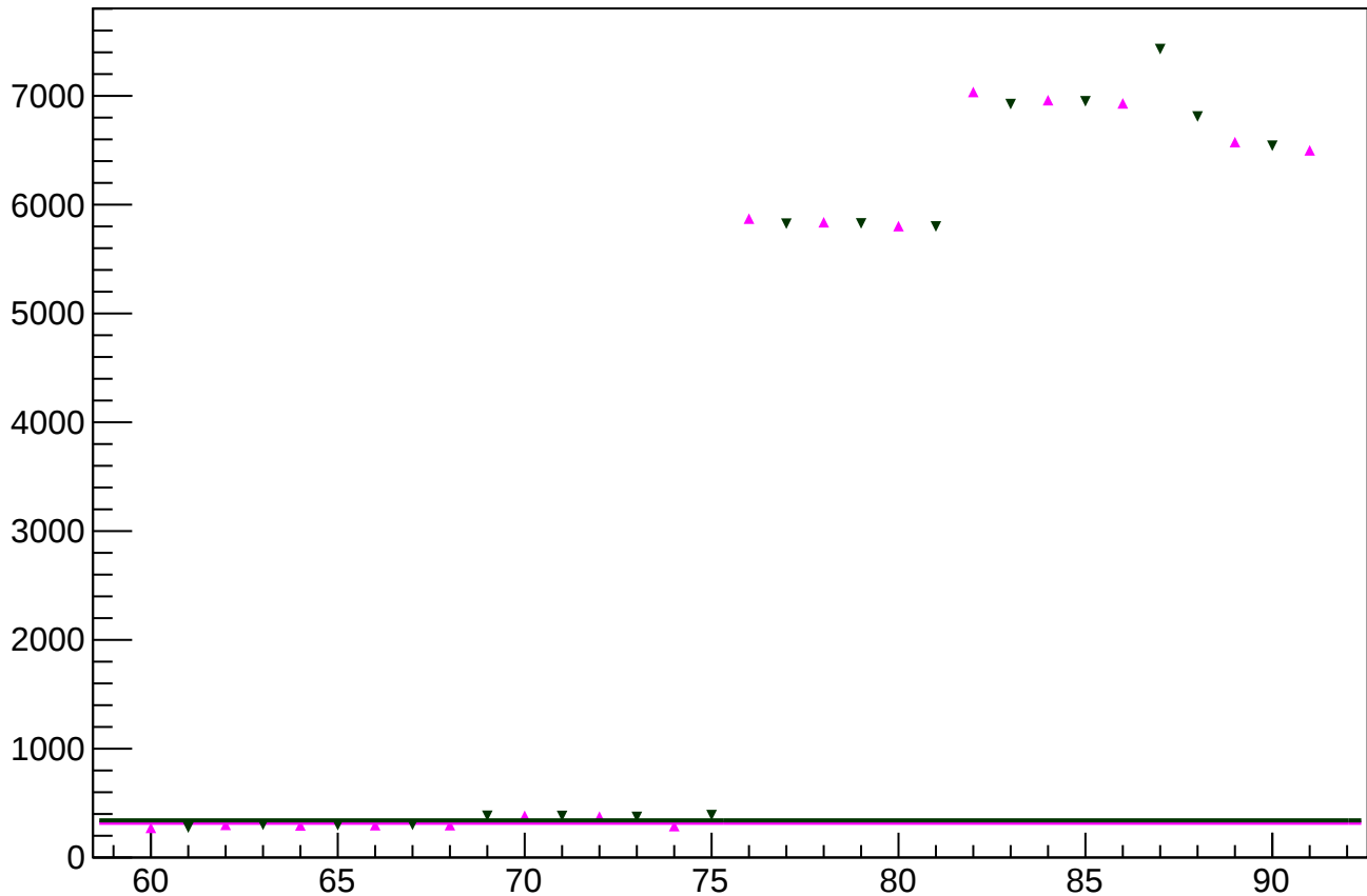
reg_asym_atr1l2_dd_rms vs slug
