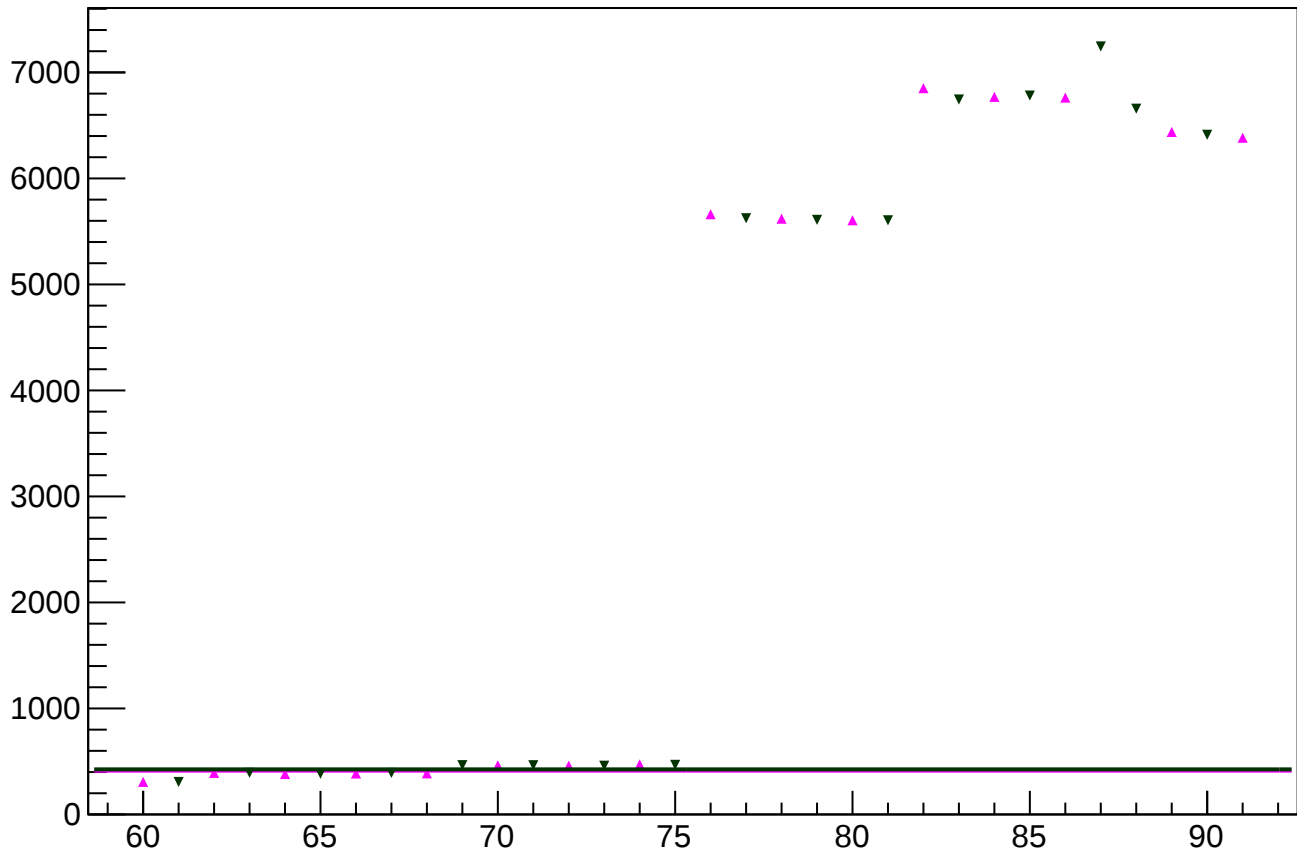
reg_asym_atl_avg_rms vs slug
