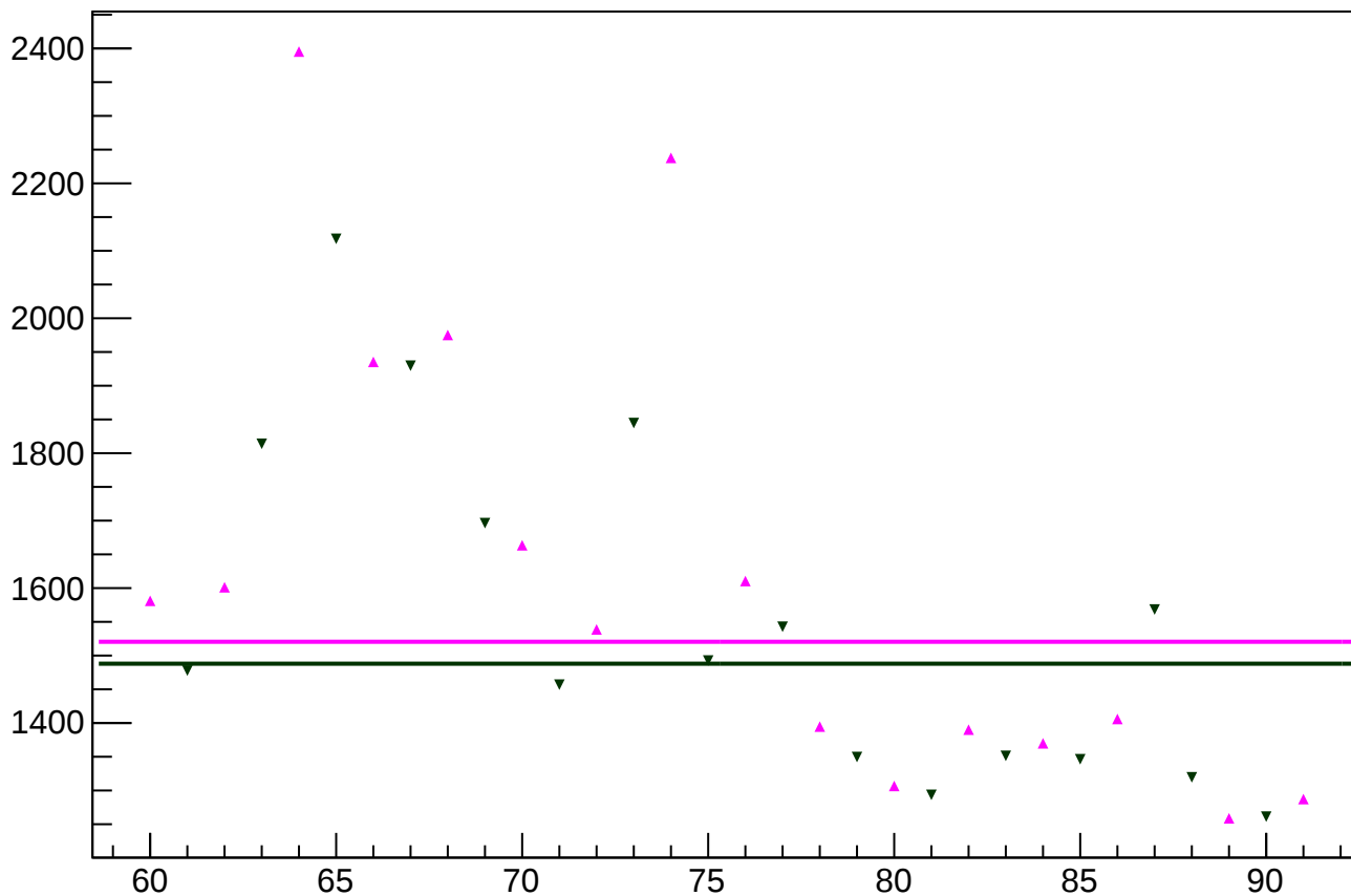
asym_sam8_rms vs slug
