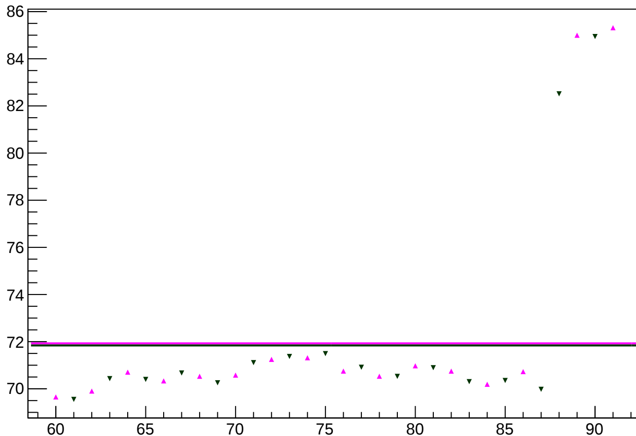
yield_bcm_dg_us_mean vs slug
