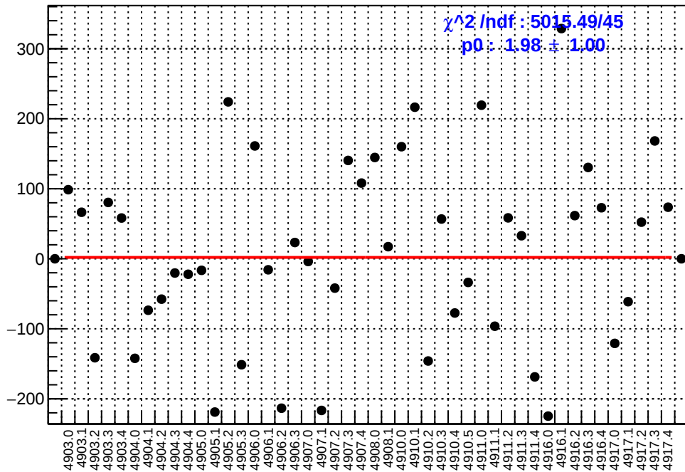
slug91: asym_left_dd.mean/ppb-reg_asym_left_dd.mean/ppb
