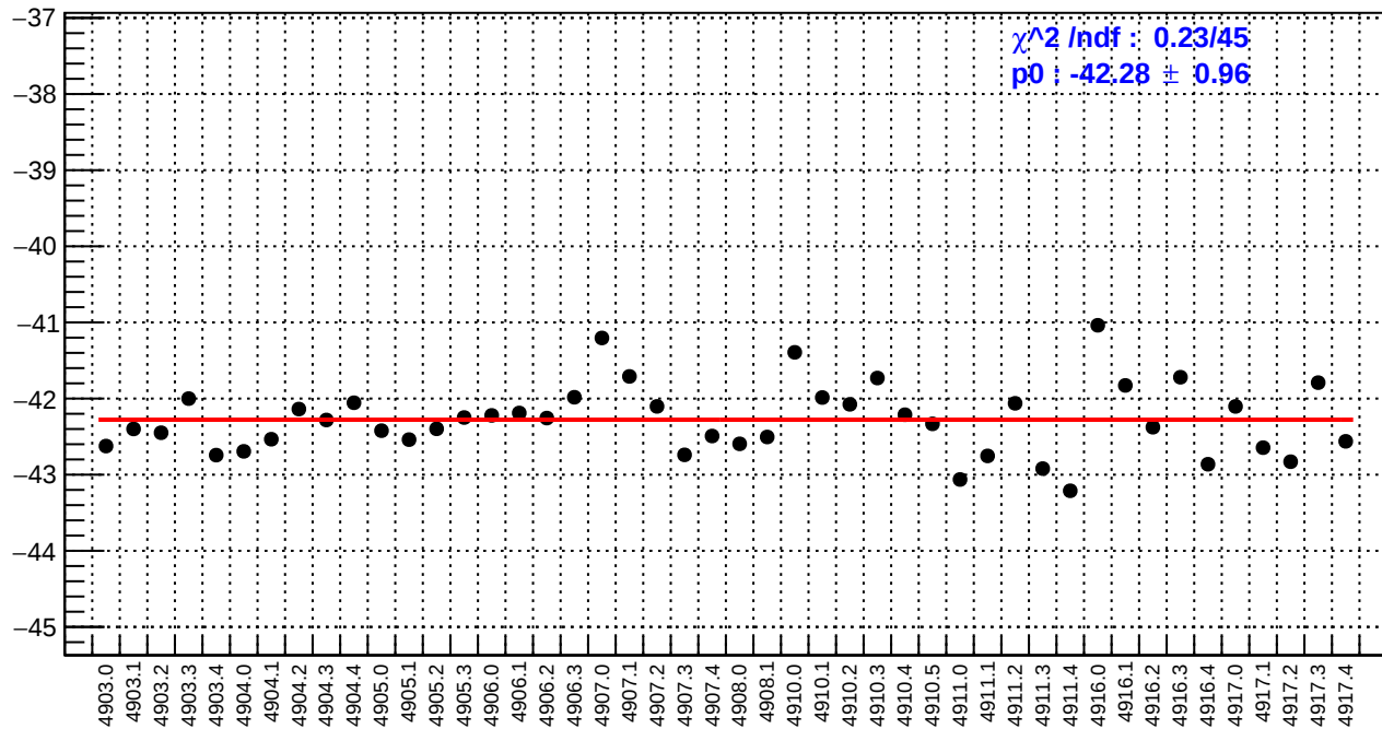
slug91: usl_bpm12X/(ppb/nm)
