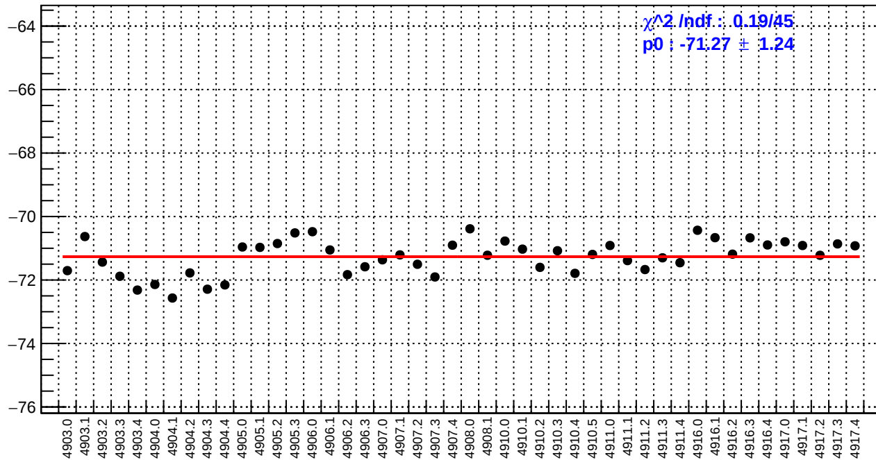
slug91: left_avg_bpm4eX/(ppb/nm)
