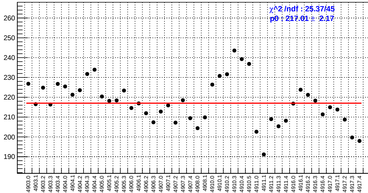
slug91: reg_asym_sam1.rms/ppm
