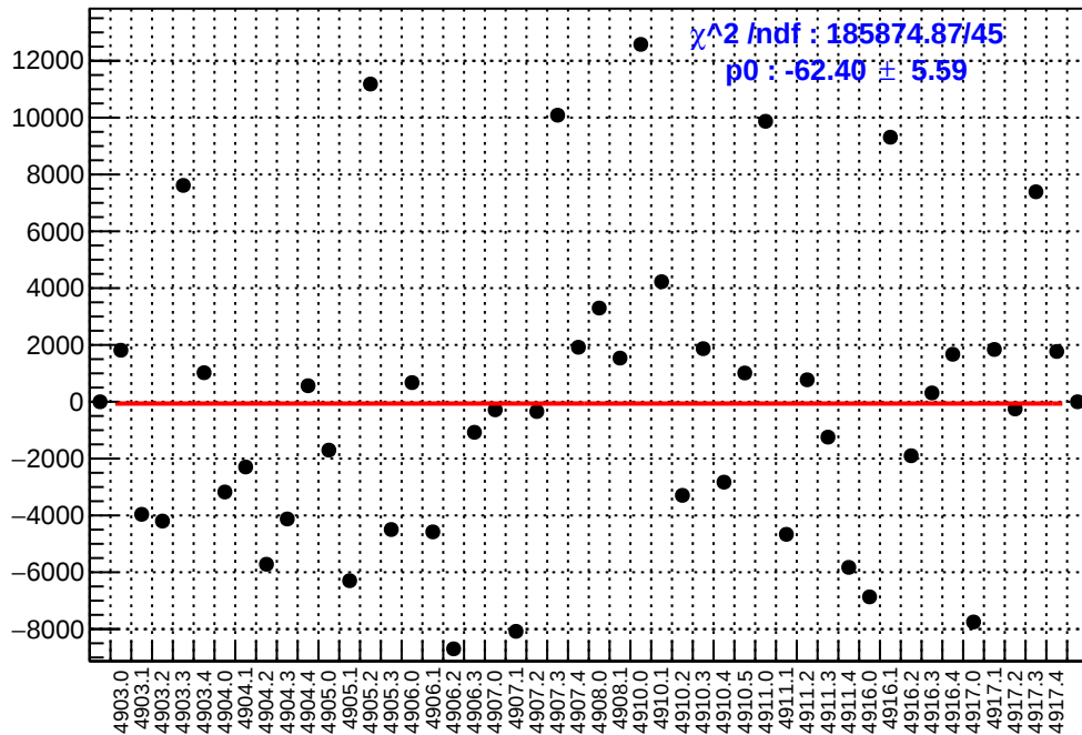
slug91: asym_atr2.mean/ppb-reg_asym_atr2.mean/ppb
