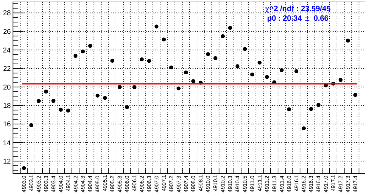
slug91: dsl_bpm4eY/(ppb/nm)
