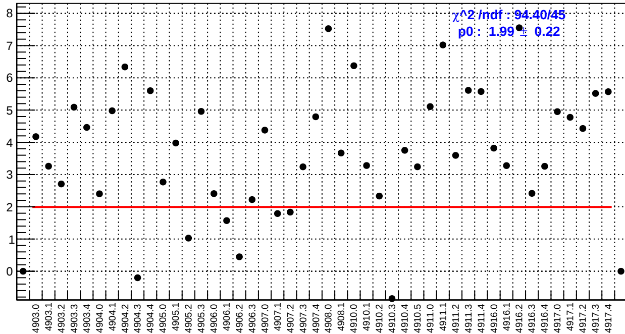
slug91: usr_bpm4eY/(ppb/nm)
