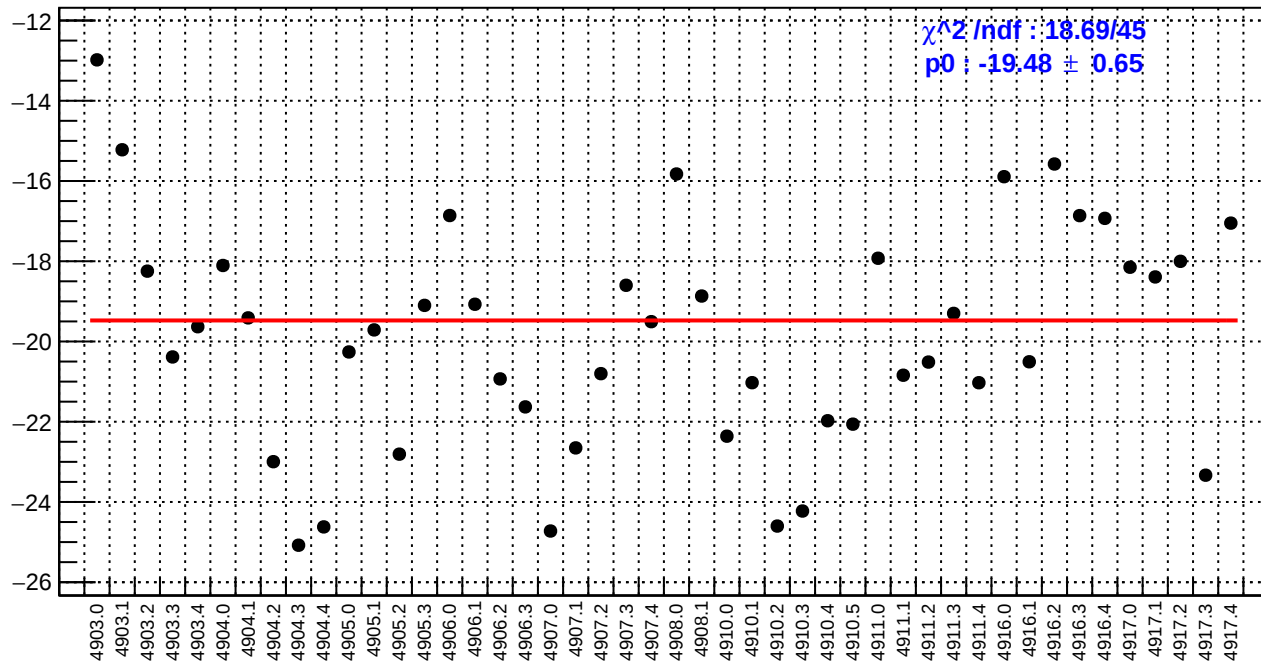
slug91: left_avg_bpm4aY/(ppb/nm)
