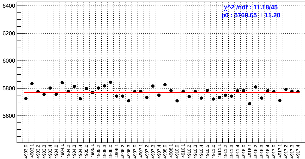
slug91: reg_asym_at1_dd.rms/ppm
