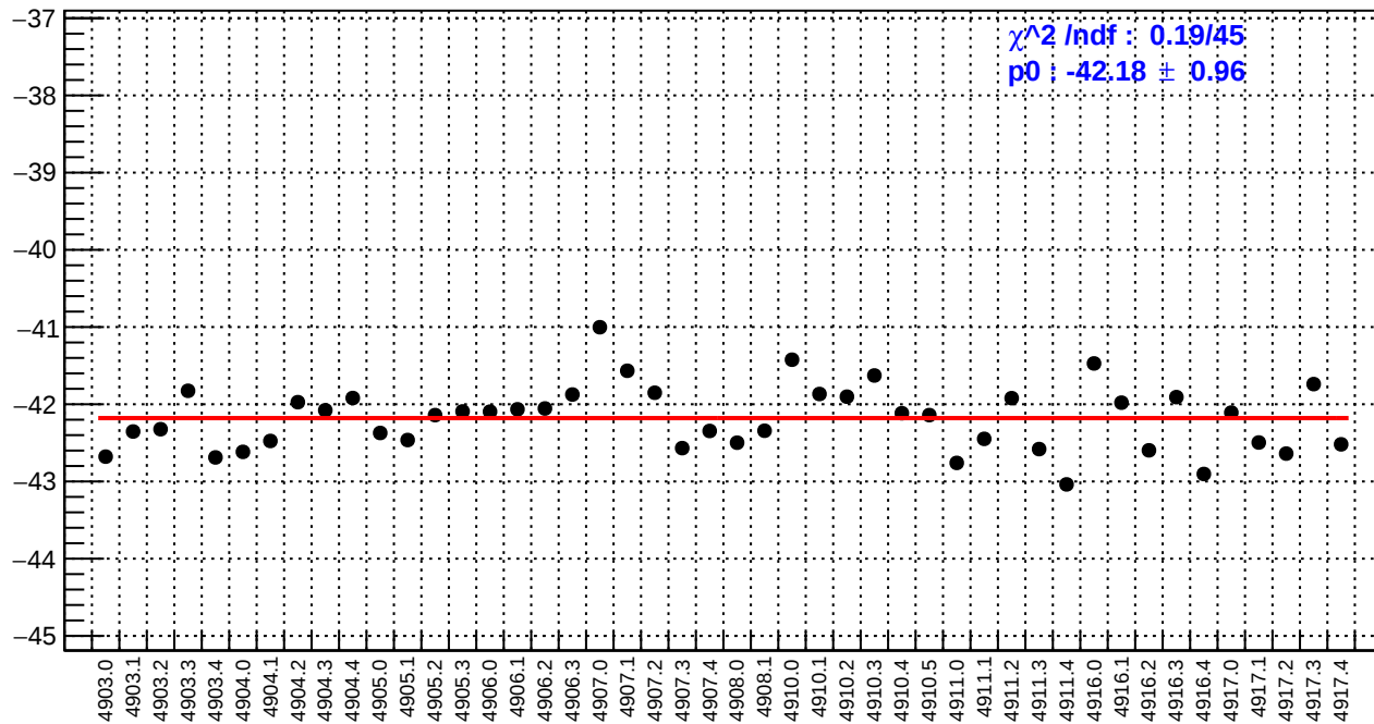
slug91: left_avg_bpm12X/(ppb/nm)
