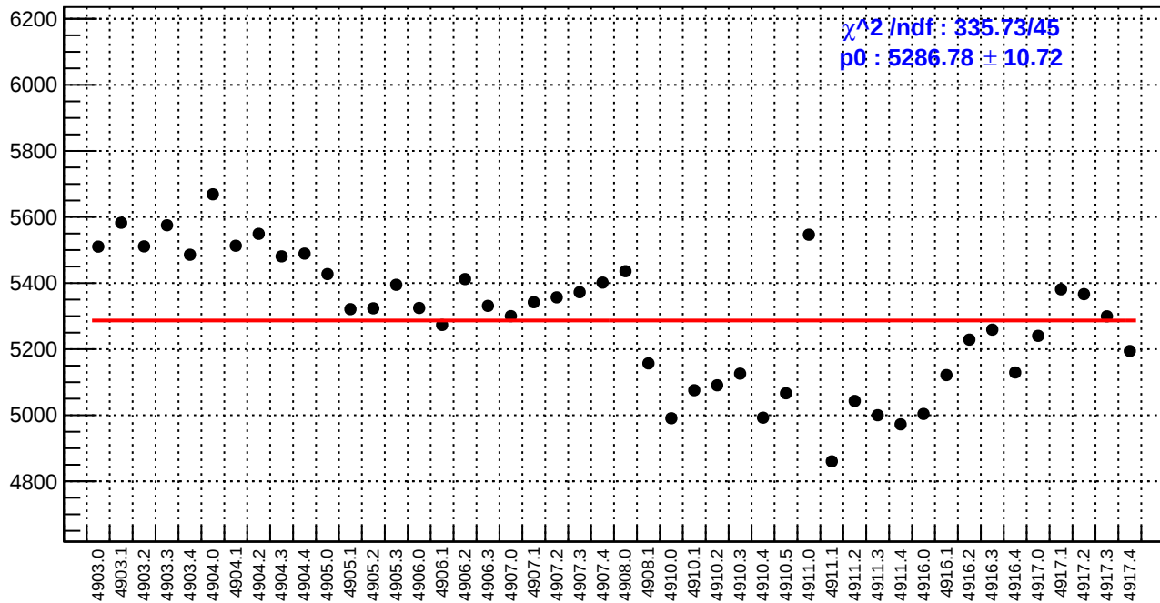
slug91: diff_bpm11X.rms/nm
