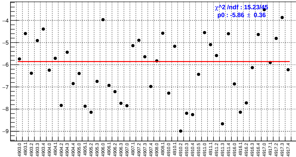
slug91: right_avg_bpm4aX/(ppb/nm)
