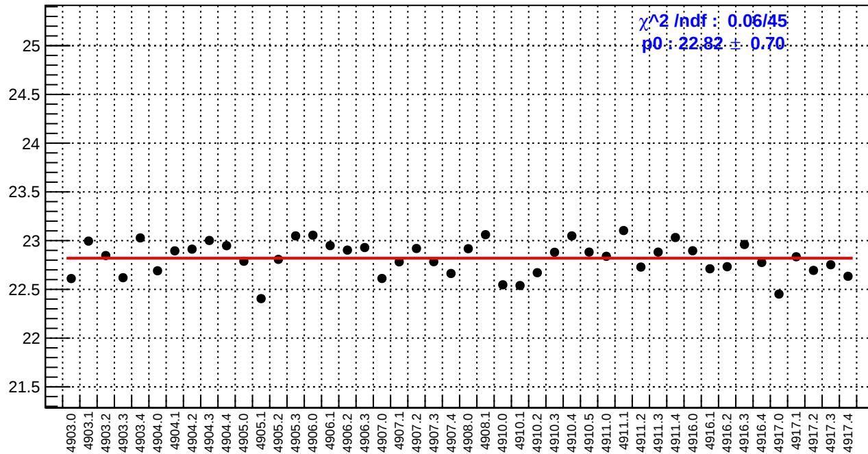
slug91: reg_asym_left_dd.rms/ppm
