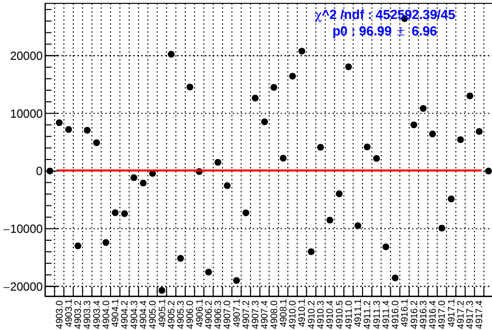
slug91: asym_sam7.mean/ppb-reg_asym_sam7.mean/ppb
