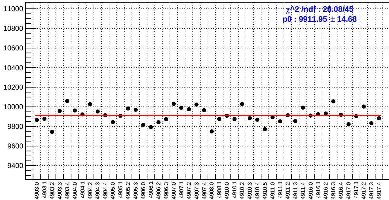
slug91: reg_asym_atr2.rms/ppm
