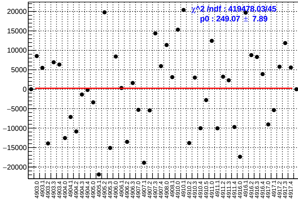
slug91: asym_sam8.mean/ppb-reg_asym_sam8.mean/ppb
