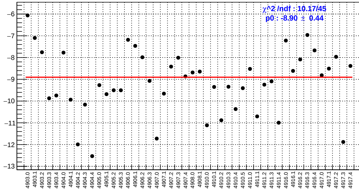
slug91: us_avg_bpm4aY/(ppb/nm)
