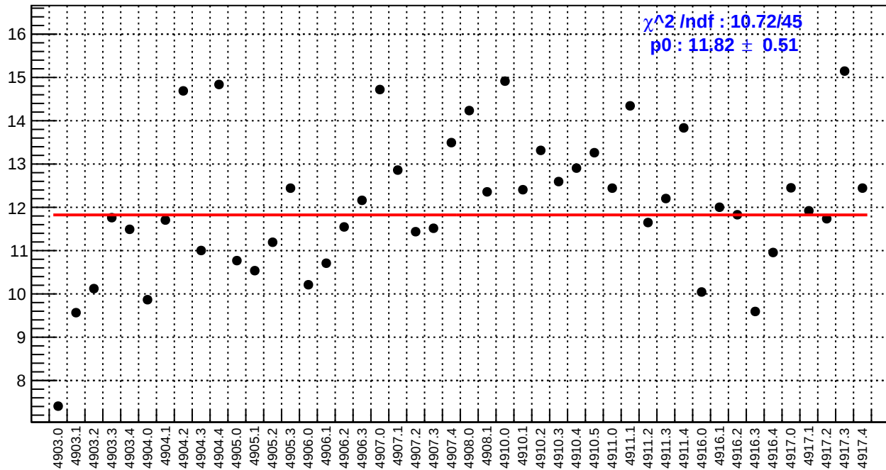
slug91: us_avg_bpm4eY/(ppb/nm)
