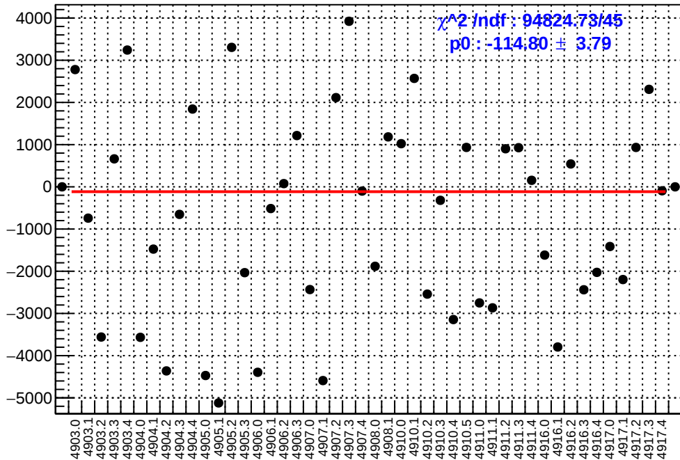
slug91: asym_sam1.mean/ppb-reg_asym_sam1.mean/ppb
