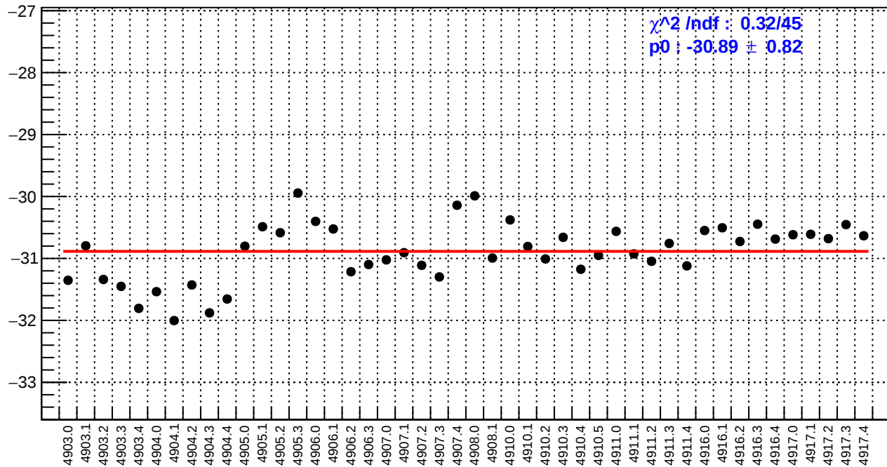
slug91: ds_avg_bpm4eX/(ppb/nm)
