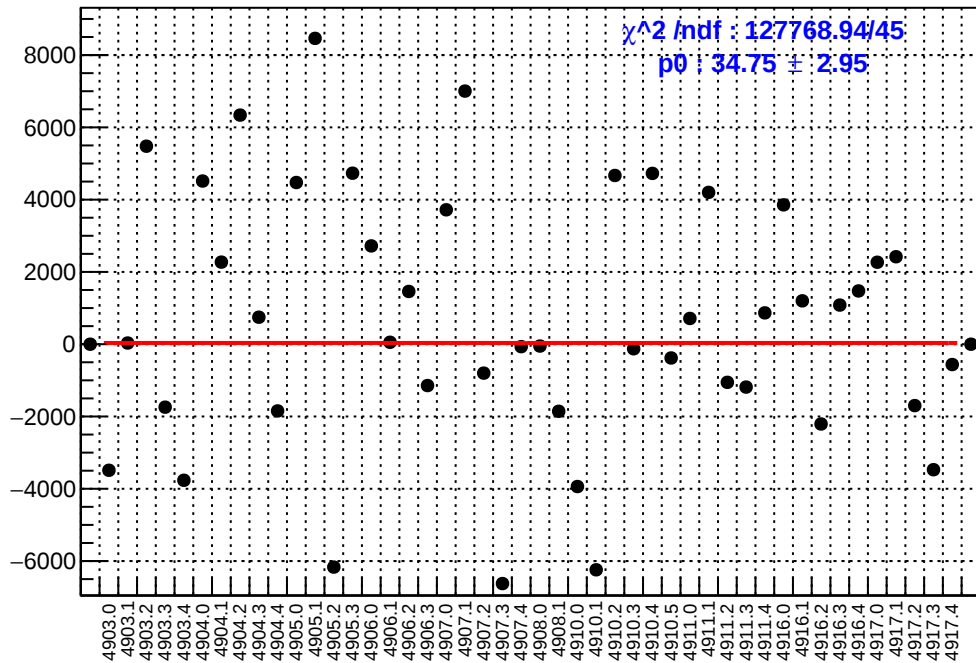
slug91: asym_sam5.mean/ppb-reg_asym_sam5.mean/ppb
