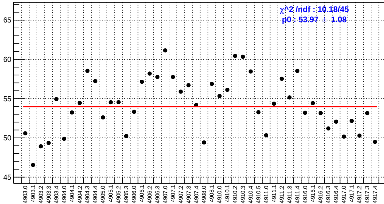
slug91: left_avg_bpm4aX/(ppb/nm)
