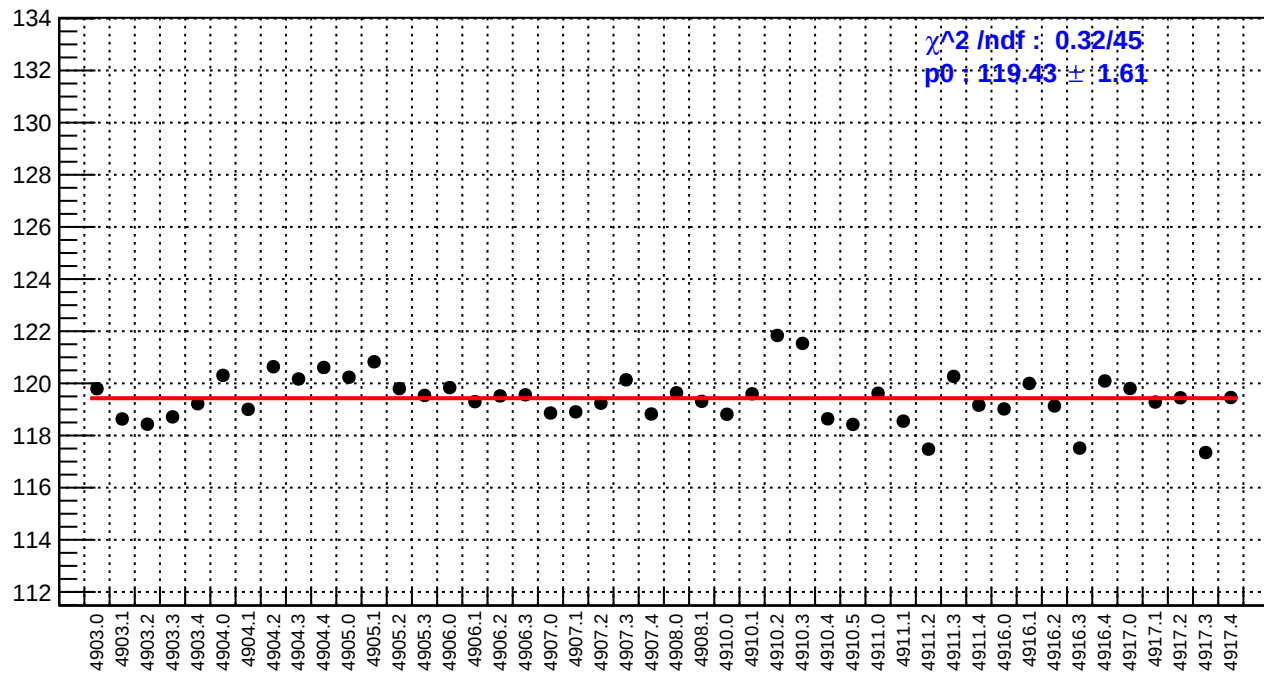
slug91: reg_asym_usr.rms/ppm
