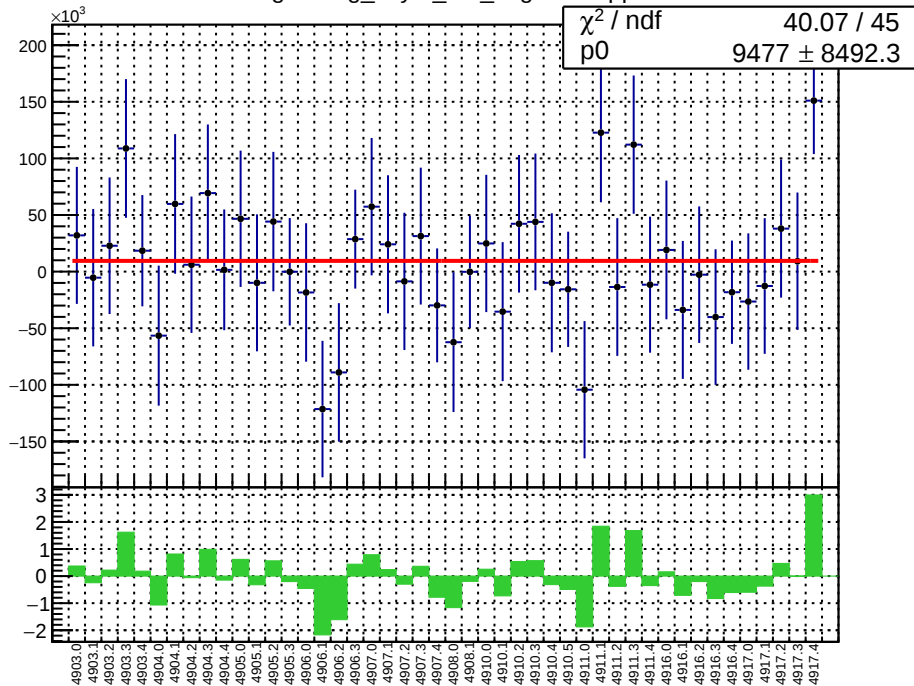
slug91: reg_asym_at1_avg.mean/ppb
