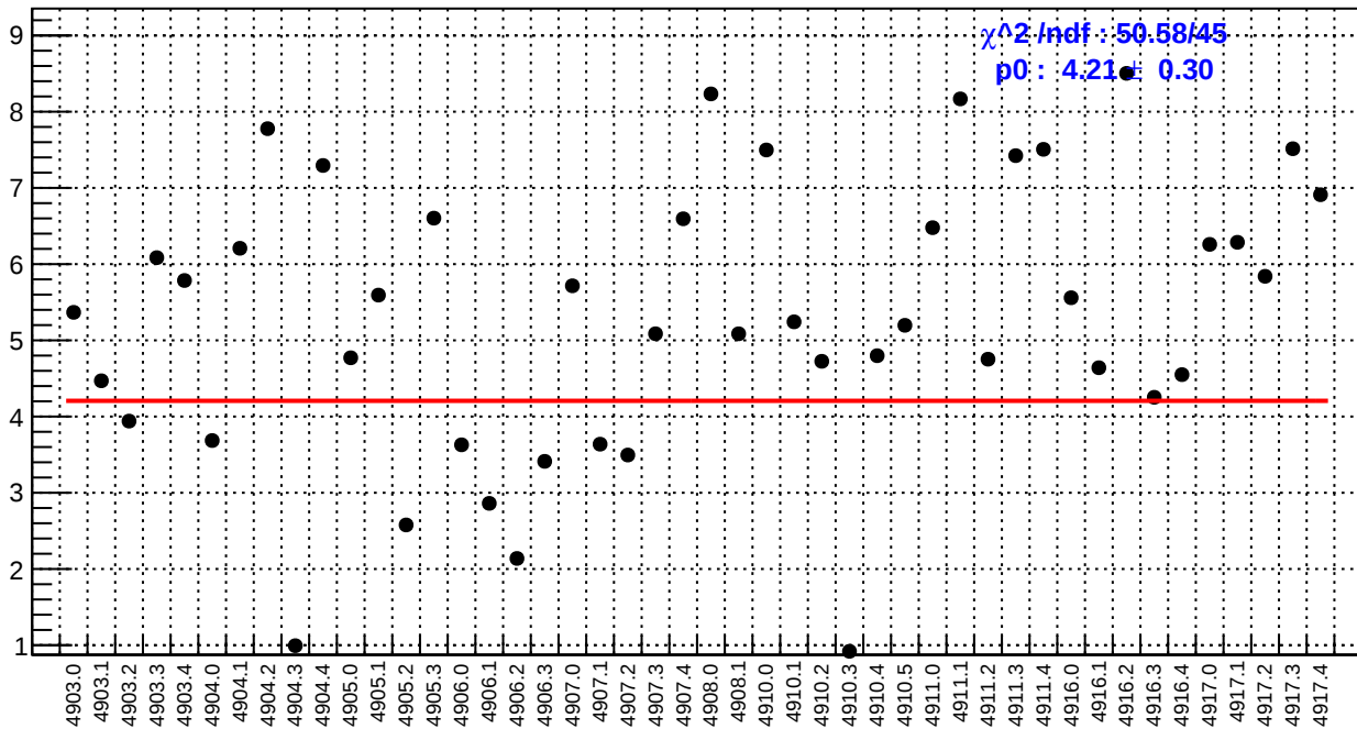
slug91: right_avg_bpm4eY/(ppb/nm)
