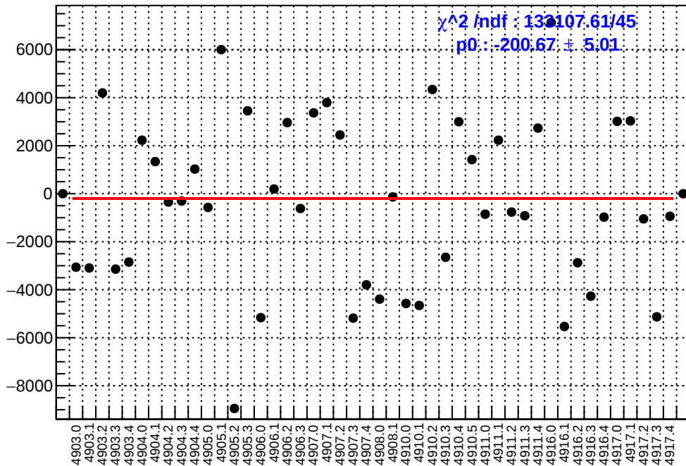
slug91: asym_atl_avg.mean/ppb-reg_asym_atl_avg.mean/ppb
