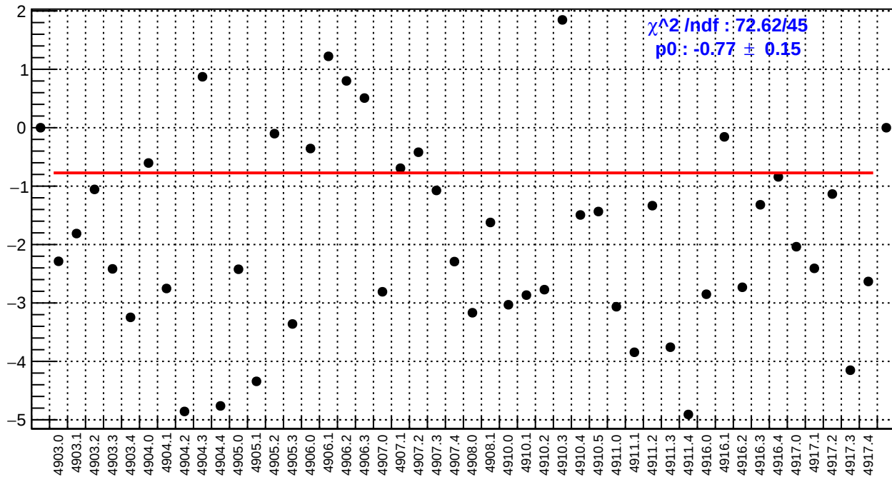
slug91: dsr_bpm4aY/(ppb/nm)
