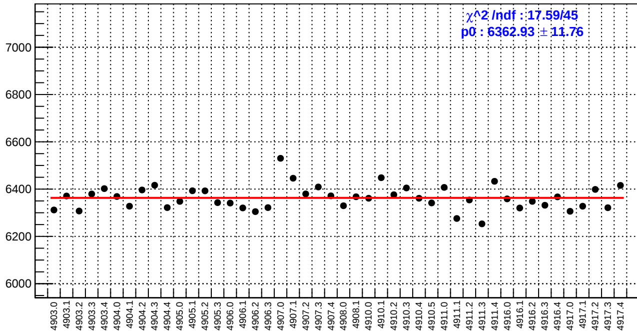
slug91: reg_asym_atl1r2_avg.rms/ppm
