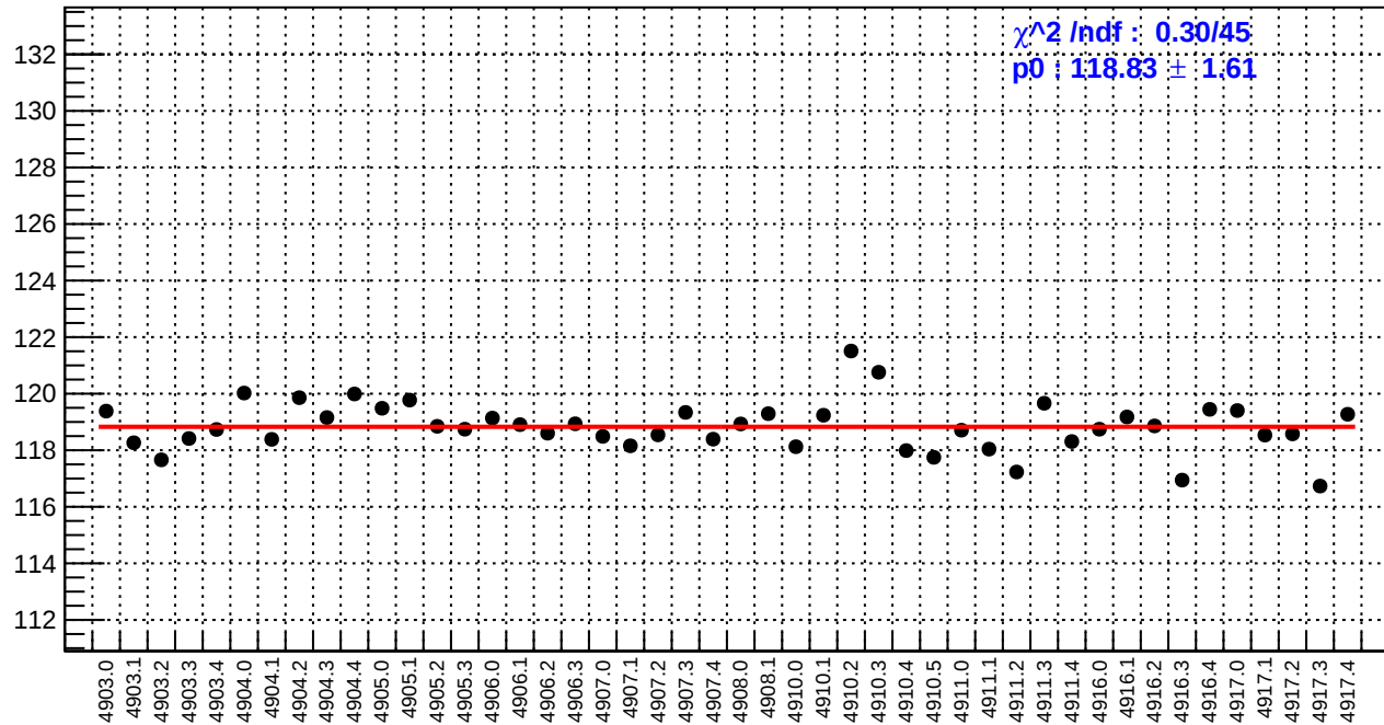
slug91: reg_asym_right_avg.rms/ppm
