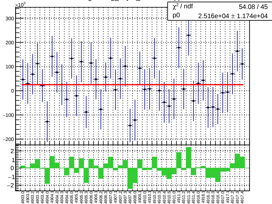
slug91: reg_asym_atl1.mean/ppb
