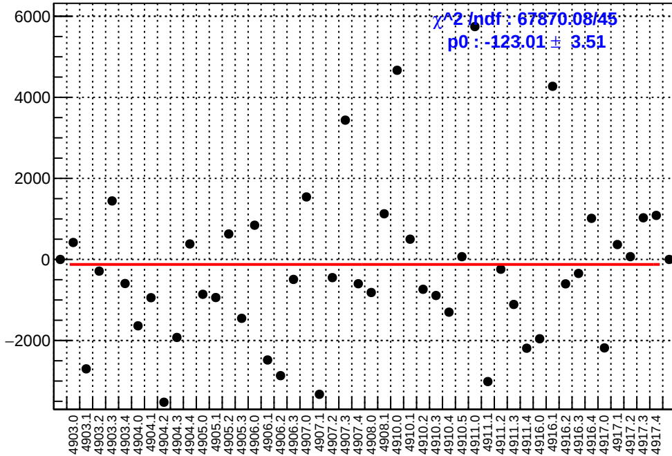
slug91: asym_atl1r2_avg.mean/ppb-reg_asym_atl1r2_avg.mean/ppb
