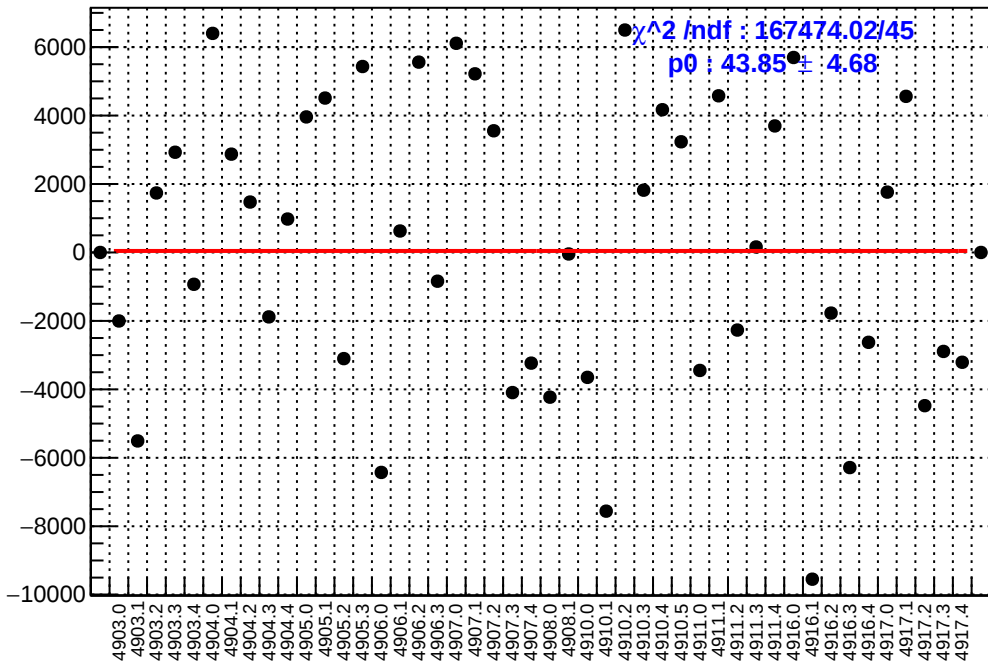
slug91: asym_dsl.mean/ppb-reg_asym_dsl.mean/ppb
