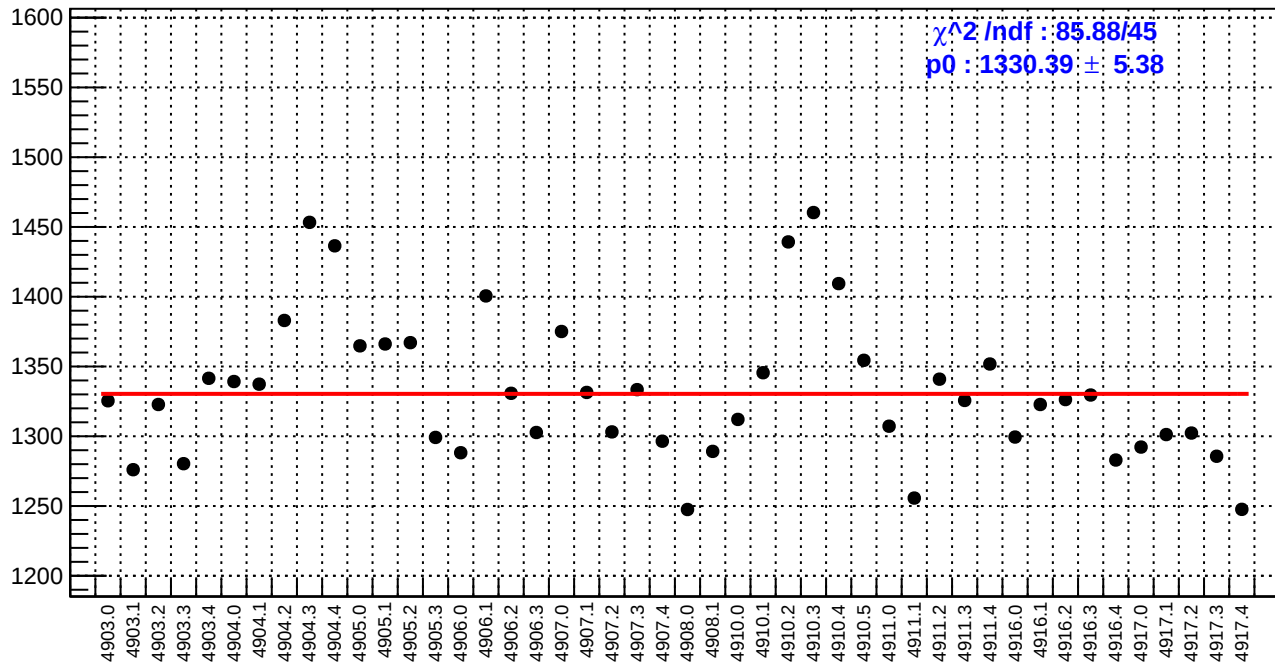
slug91: diff_bpm4aX.rms/nm
