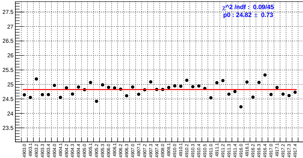
slug91: reg_asym_right_dd.rms/ppm
