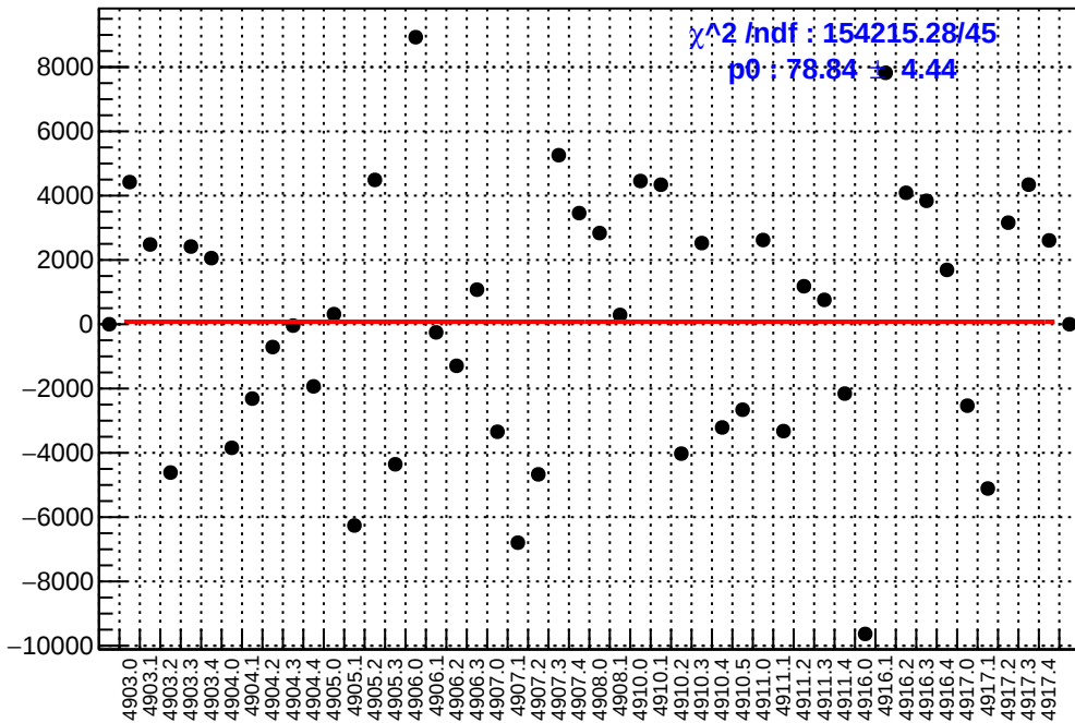
slug91: asym_atr1l2_dd.mean/ppb-reg_asym_atr1l2_dd.mean/ppb
