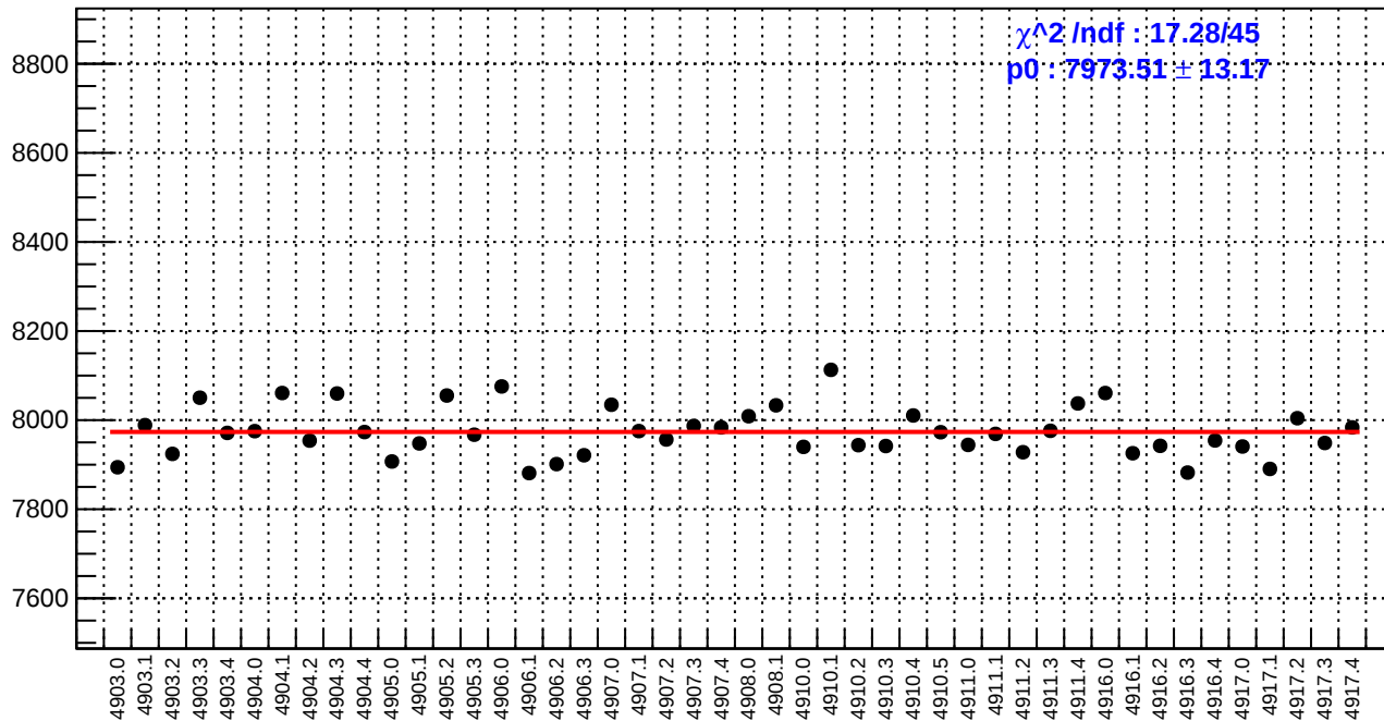
slug91: reg_asym_atl1.rms/ppm
