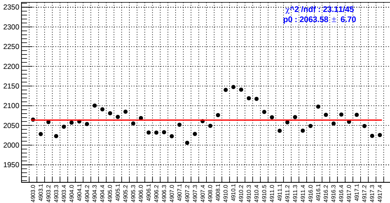
slug91: reg_asym_sam2.rms/ppm
