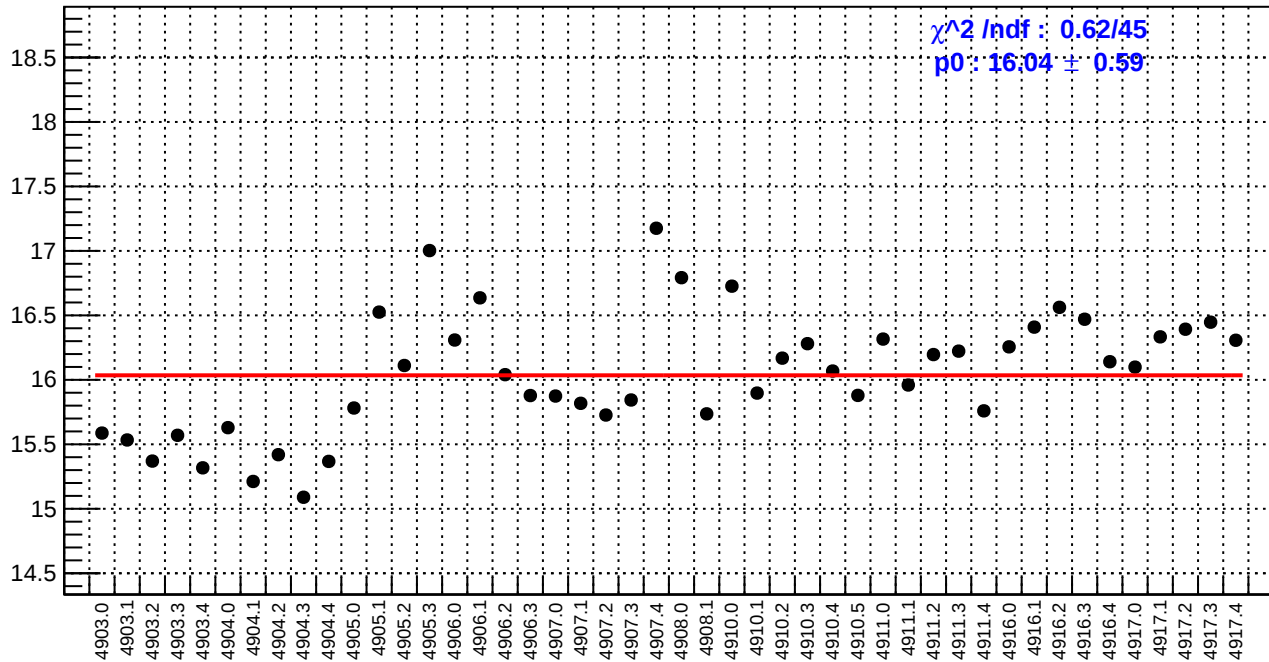
slug91: right_avg_bpm4eX/(ppb/nm)
