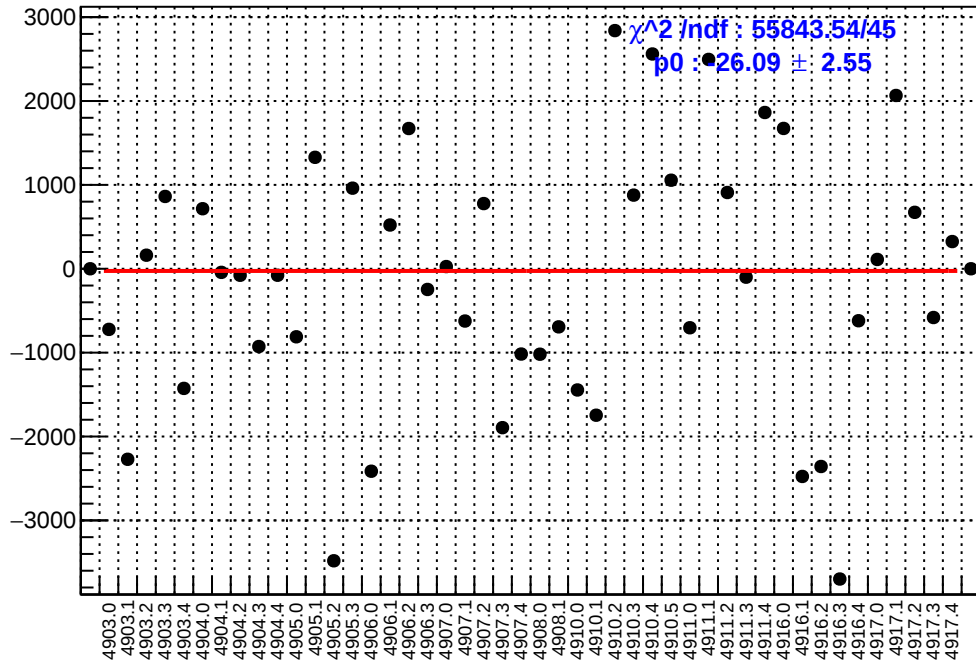
slug91: asym_atr1l2_avg.mean/ppb-reg_asym_atr1l2_avg.mean/ppb
