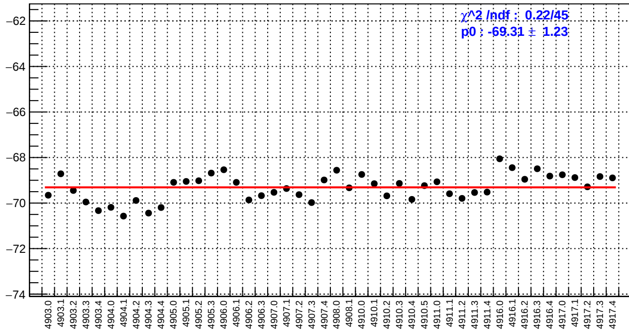
slug91: usl_bpm4eX/(ppb/nm)
