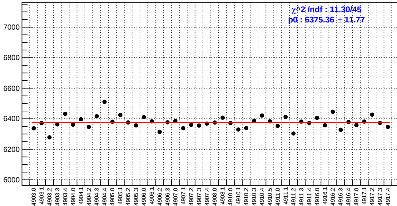
slug91: reg_asym_atl_dd.rms/ppm
