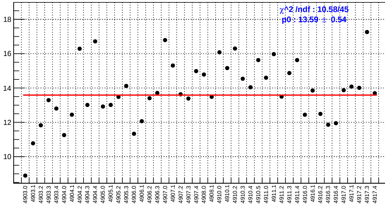
slug91: ds_avg_bpm4eY/(ppb/nm)
