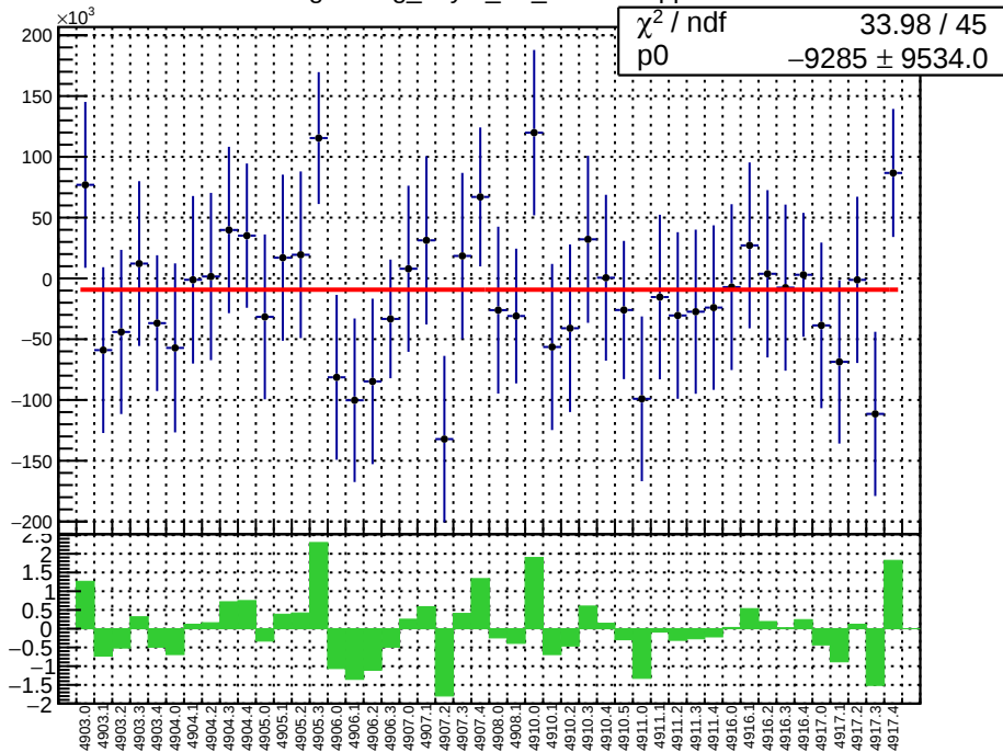
slug91: reg_asym_atr_dd.mean/ppb
