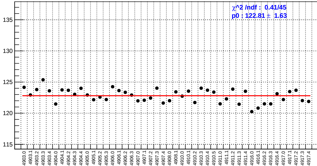
slug91: reg_asym_usl.rms/ppm
