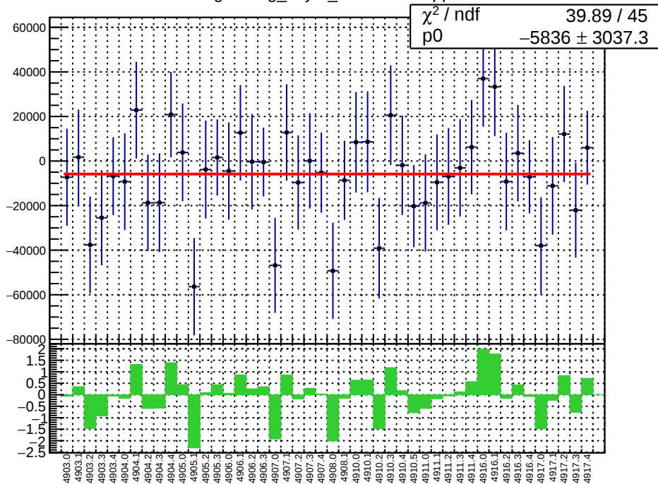
slug91: reg_asym_sam2.mean/ppb
