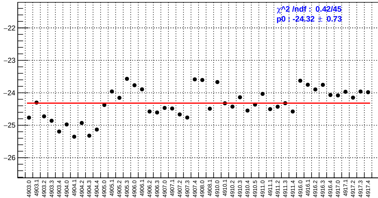
slug91: us_avg_bpm4eX/(ppb/nm)
