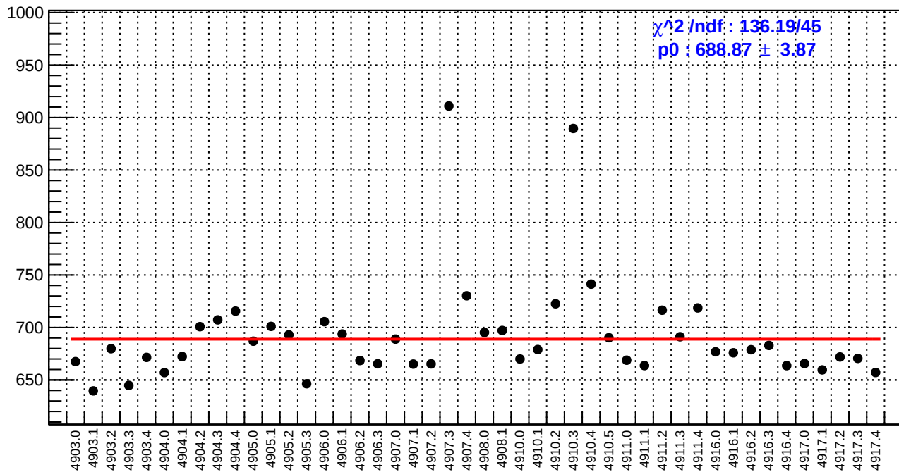
slug91: reg_asym_sam3.rms/ppm
