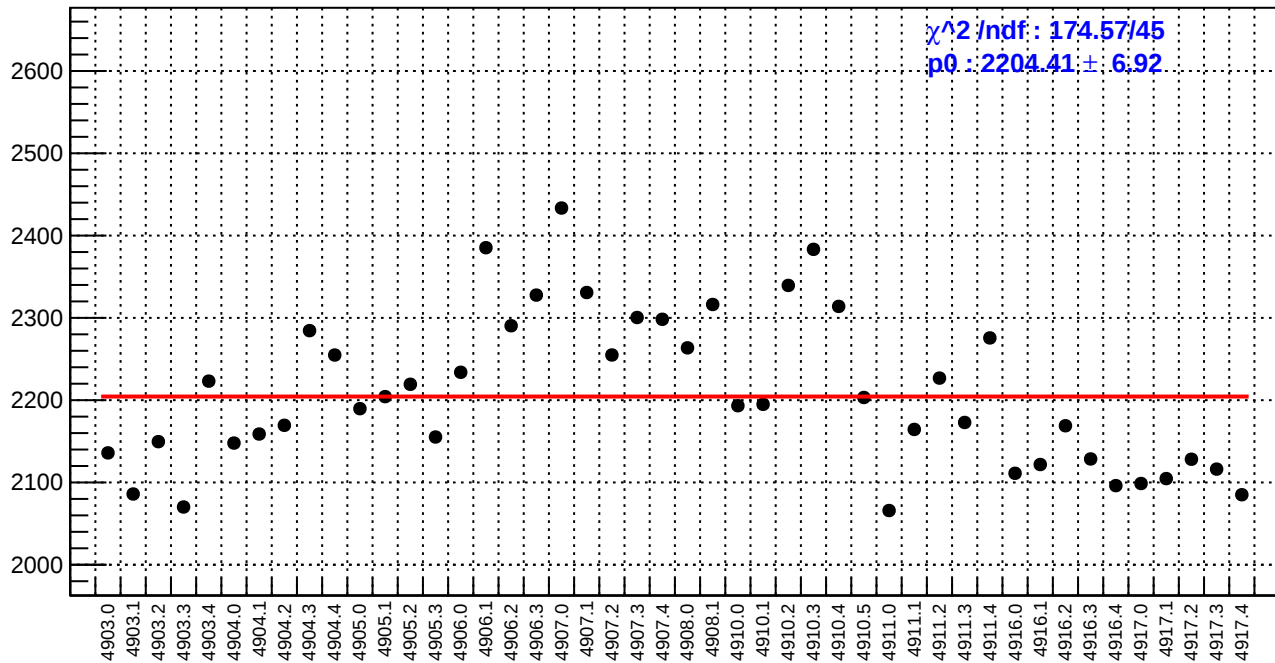
slug91: diff_bpm4eY.rms/nm
