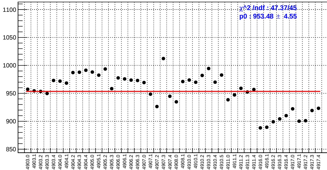
slug91: reg_asym_sam4.rms/ppm
