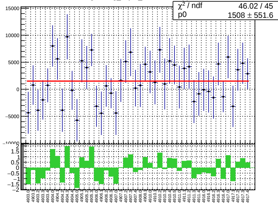
slug91: reg_asym_sam6.mean/ppb
