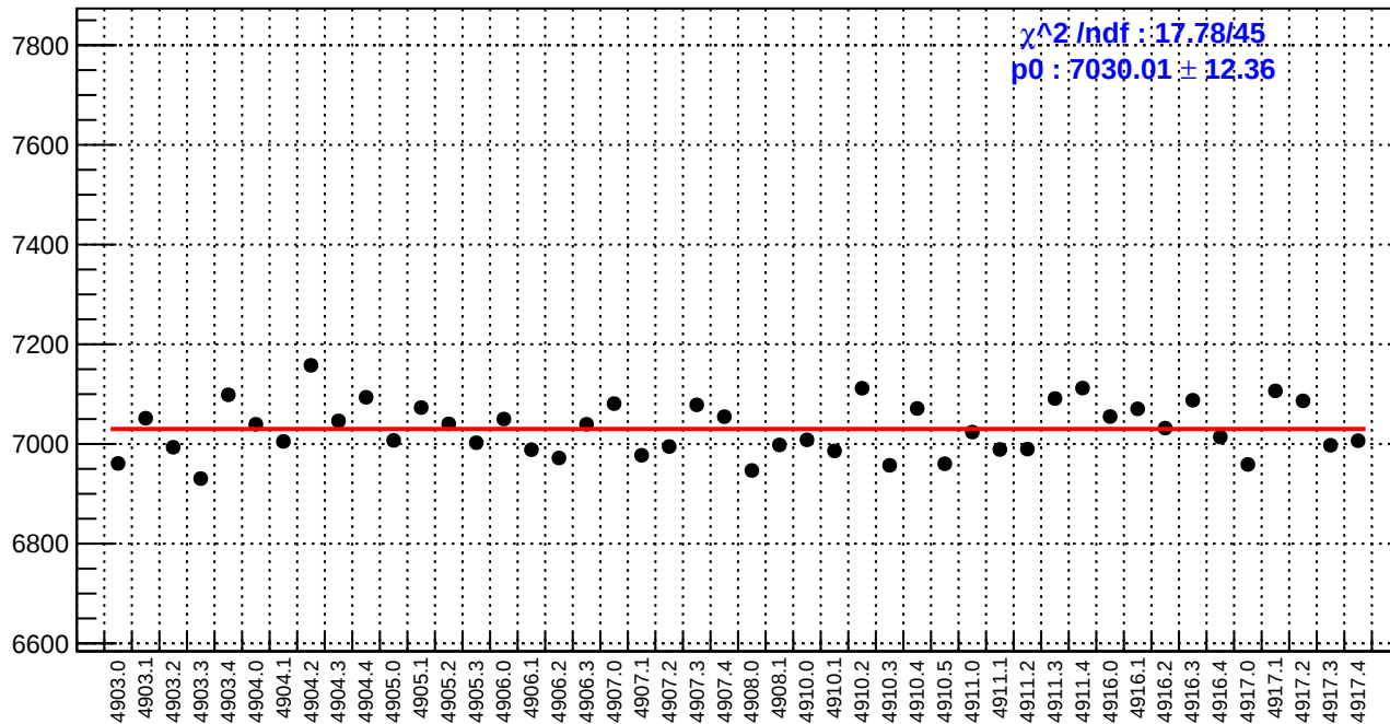
slug91: reg_asym_at2_dd.rms/ppm
