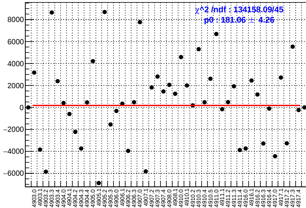
slug91: asym_dsr.mean/ppb-reg_asym_dsr.mean/ppb
