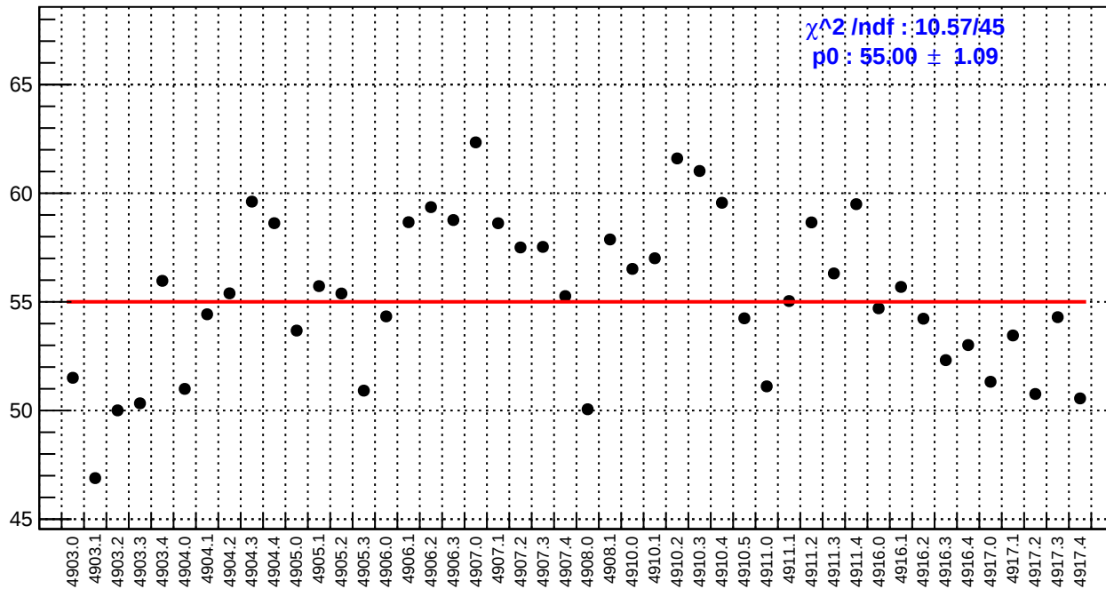
slug91: dsl_bpm4aX/(ppb/nm)
