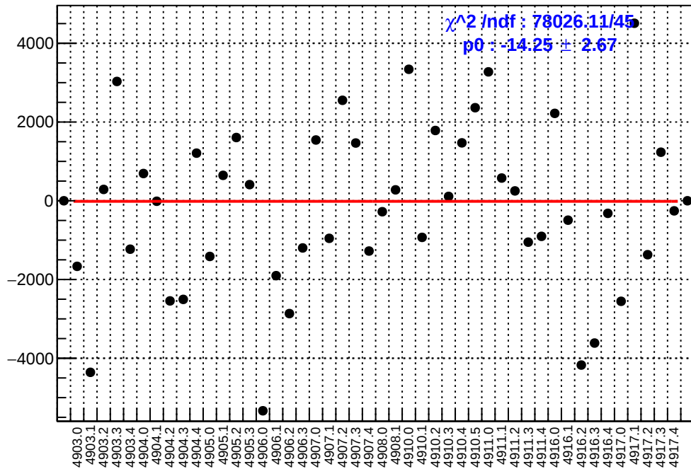
slug91: asym_at2_avg.mean/ppb-reg_asym_at2_avg.mean/ppb
