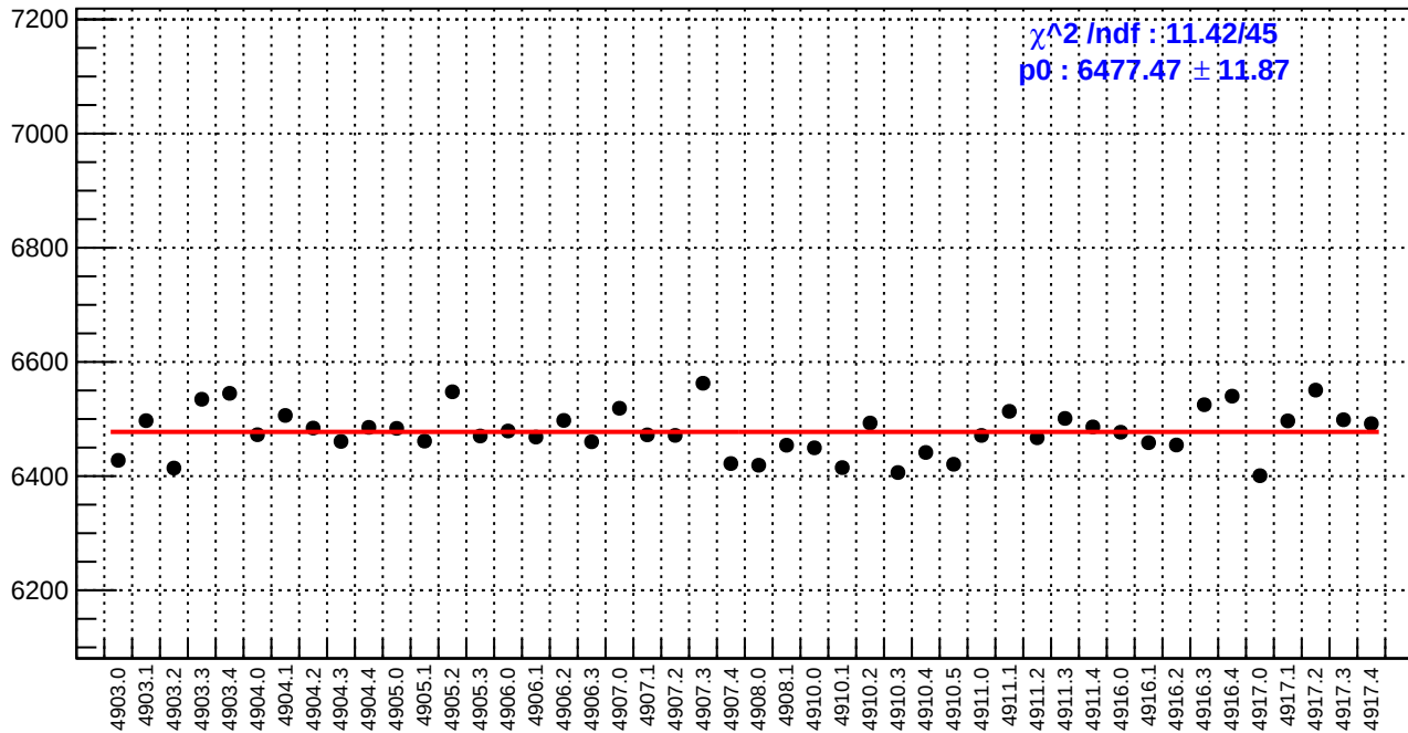
slug91: reg_asym_atr_avg.rms/ppm
