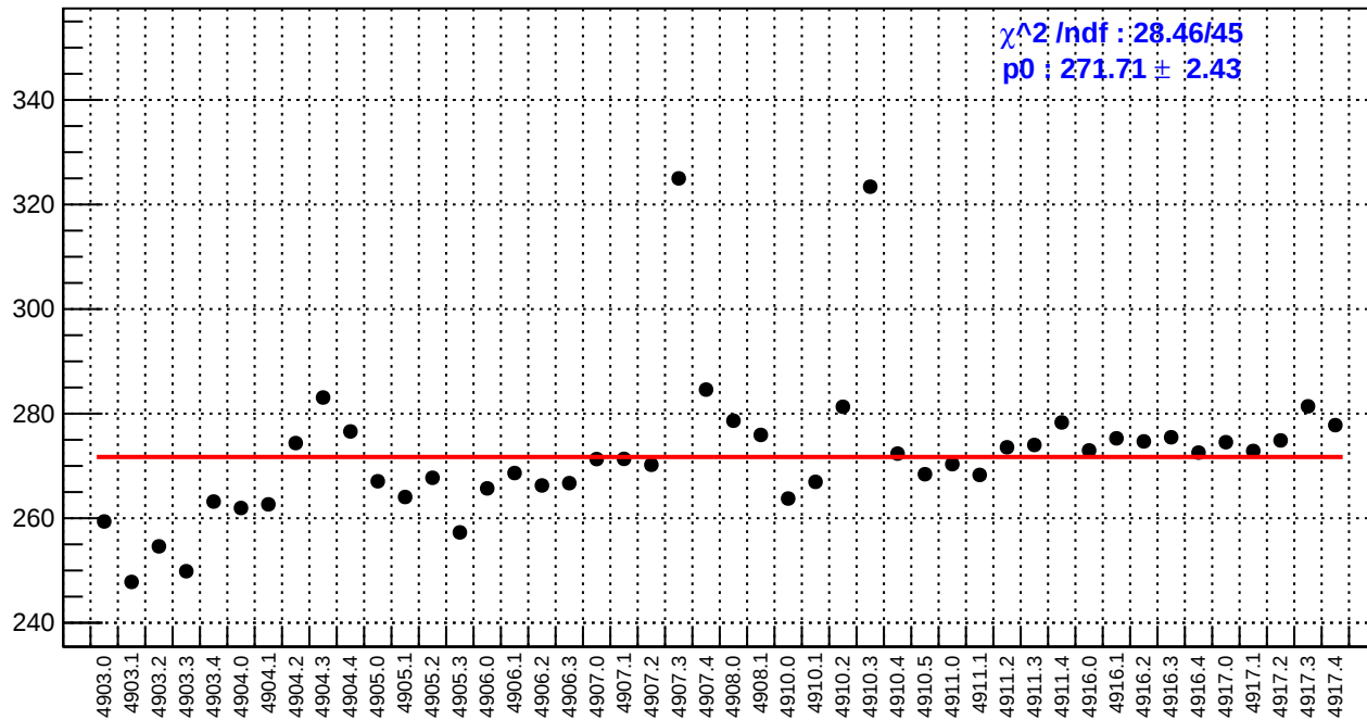
slug91: reg_asym_sam7.rms/ppm
