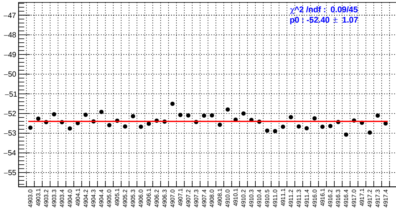
slug91: ds_avg_bpm12X/(ppb/nm)
