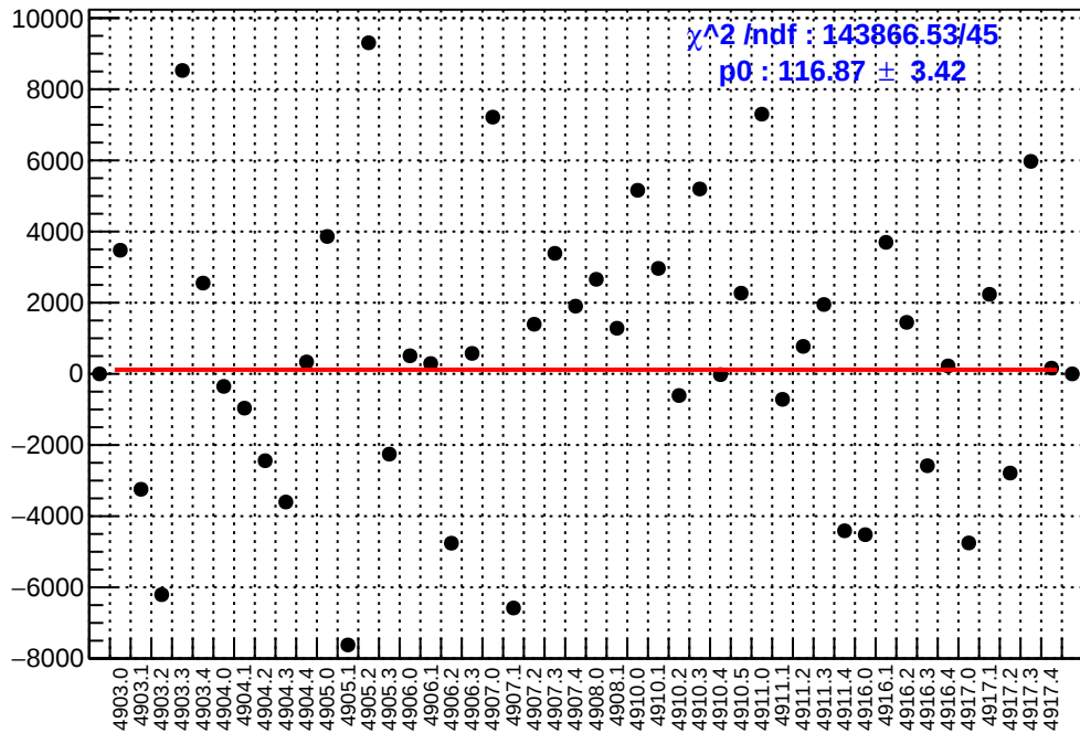
slug91: asym_usr.mean/ppb-reg_asym_usr.mean/ppb
