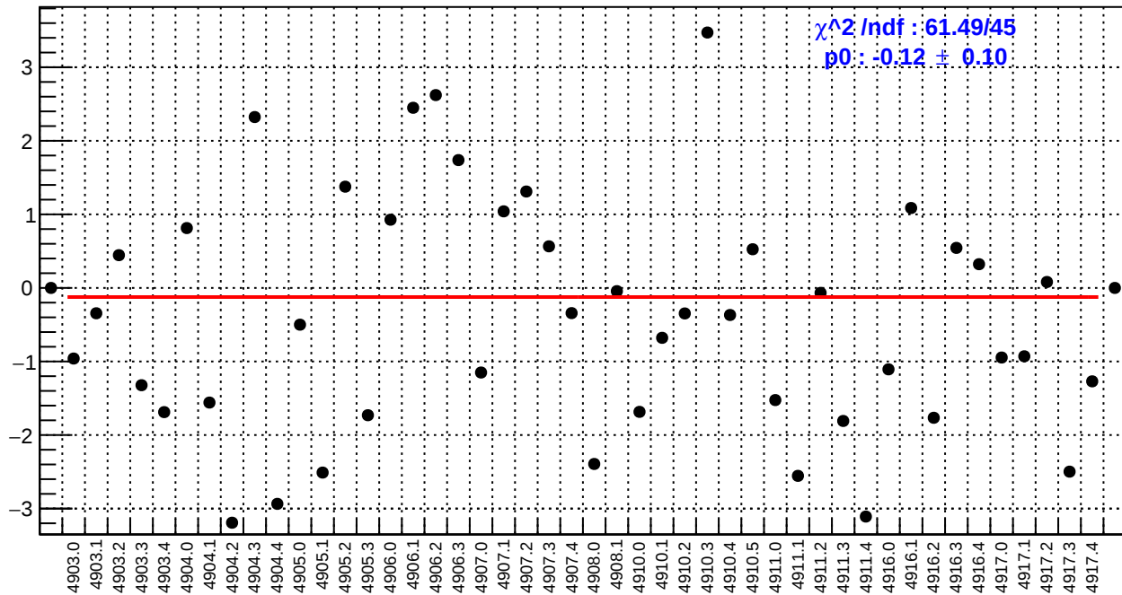
slug91: right_avg_bpm4aY/(ppb/nm)
