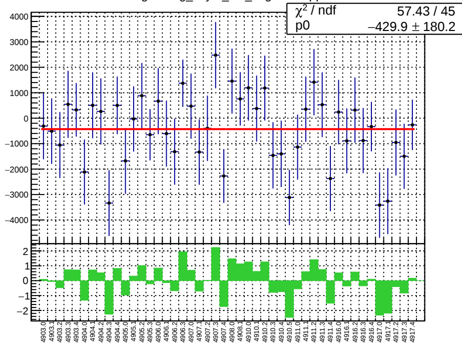
slug91: reg_asym_left_avg.mean/ppb
