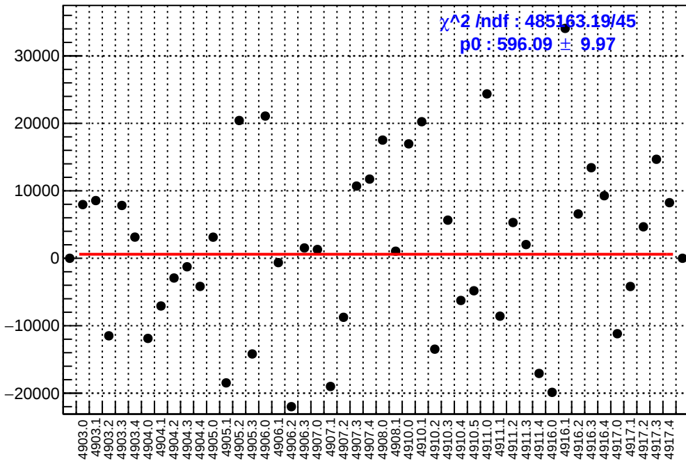
slug91: asym_sam6.mean/ppb-reg_asym_sam6.mean/ppb
