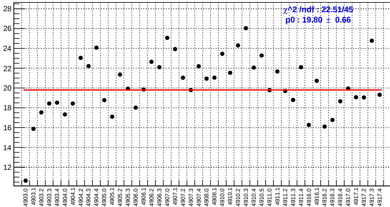
slug91: usl_bpm4eY/(ppb/nm)
