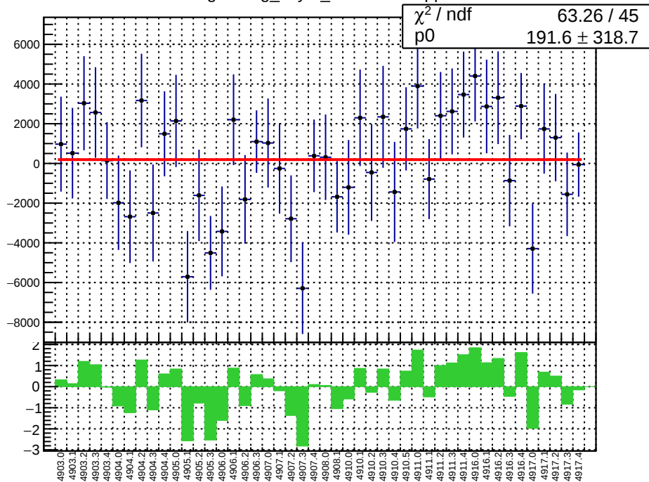
slug91: reg_asym_sam1.mean/ppb
