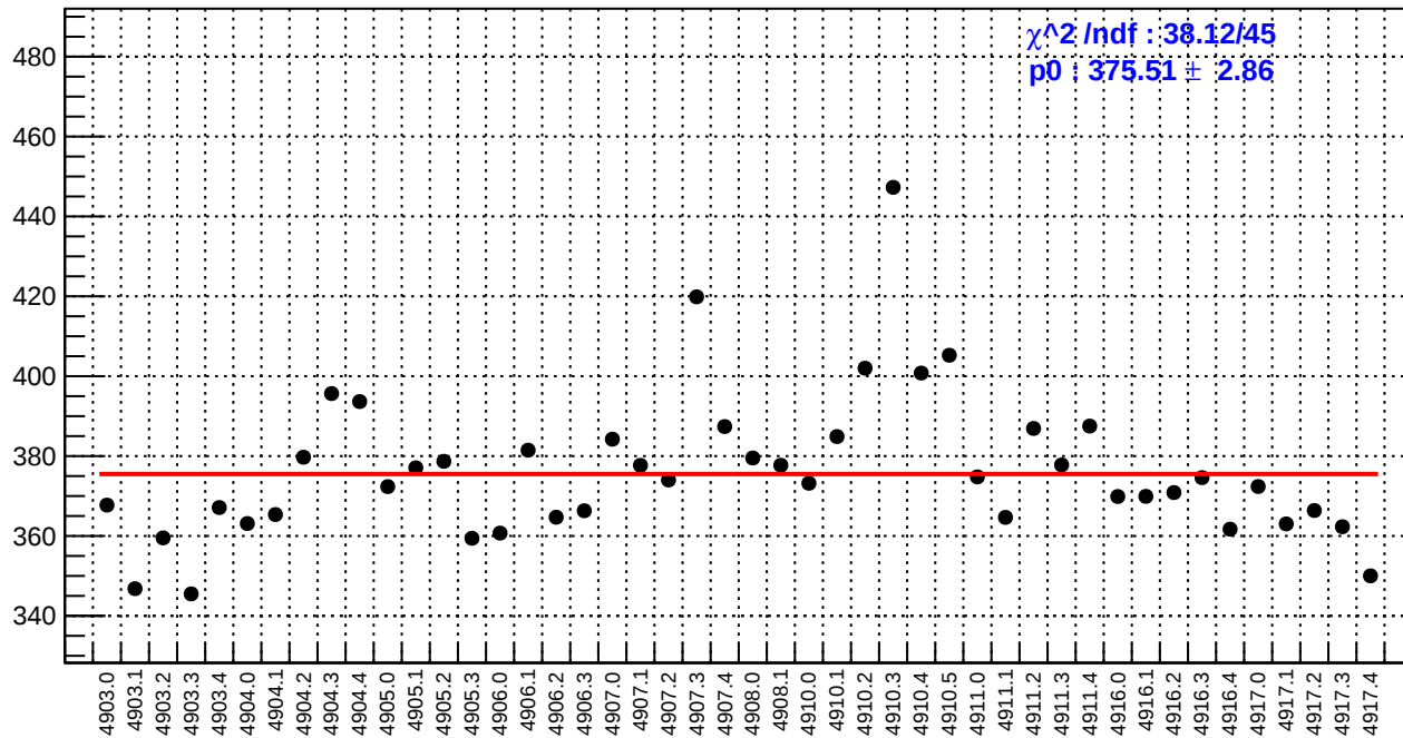
slug91: reg_asym_sam6.rms/ppm
