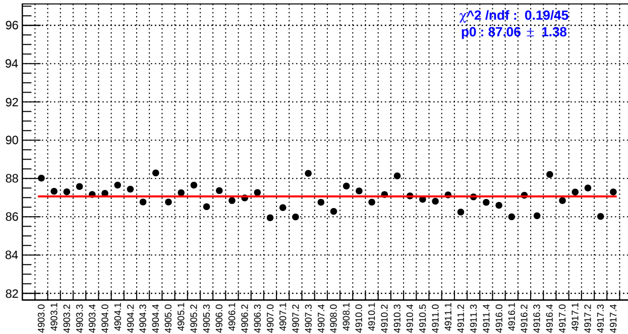
slug91: reg_asym_us_avg.rms/ppm
