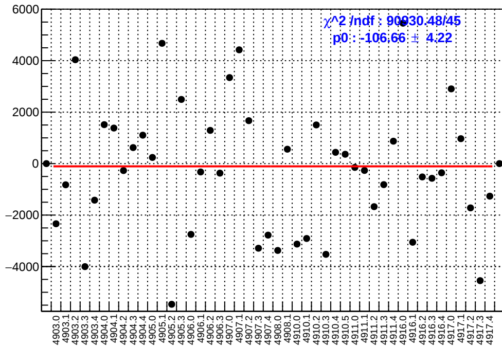
slug91: asym_at1_dd.mean/ppb-reg_asym_at1_dd.mean/ppb
