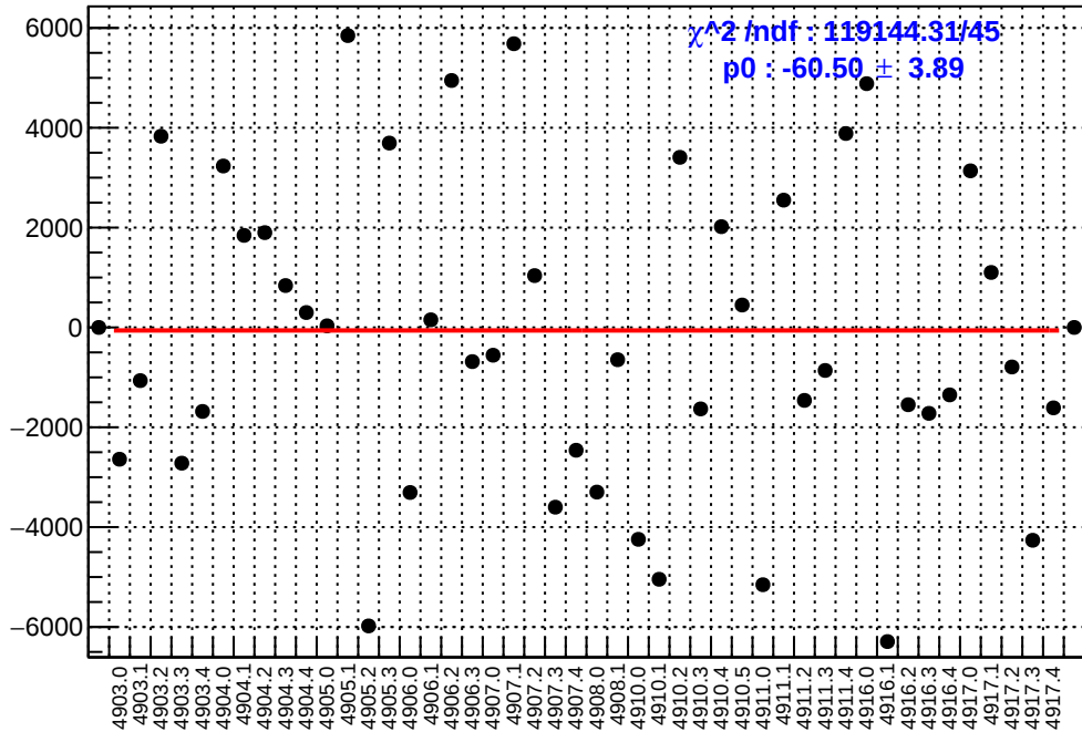
slug91: asym_us_dd.mean/ppb-reg_asym_us_dd.mean/ppb
