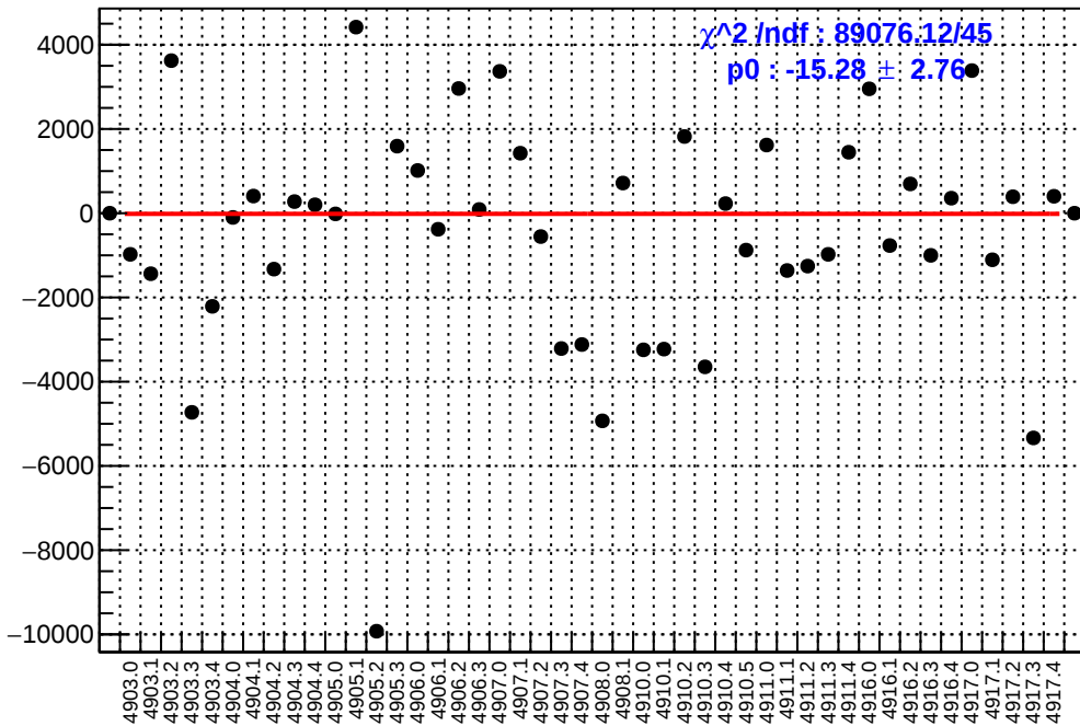
slug91: asym_atl1.mean/ppb-reg_asym_atl1.mean/ppb
