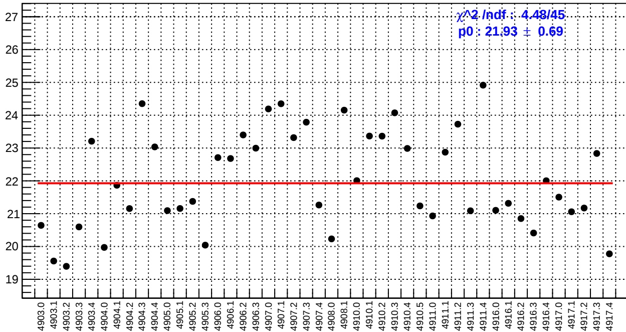
slug91: us_avg_bpm4aX/(ppb/nm)
