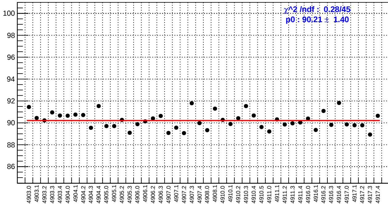
slug91: reg_asym_ds_avg.rms/ppm
