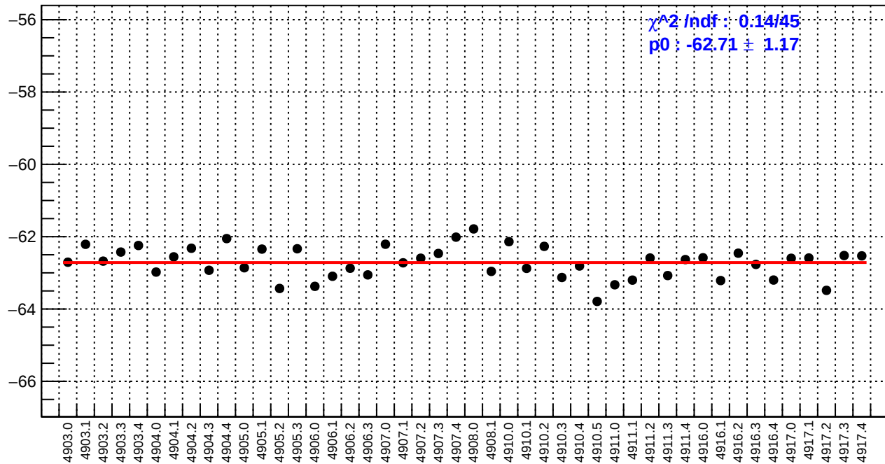
slug91: dsr_bpm12X/(ppb/nm)
