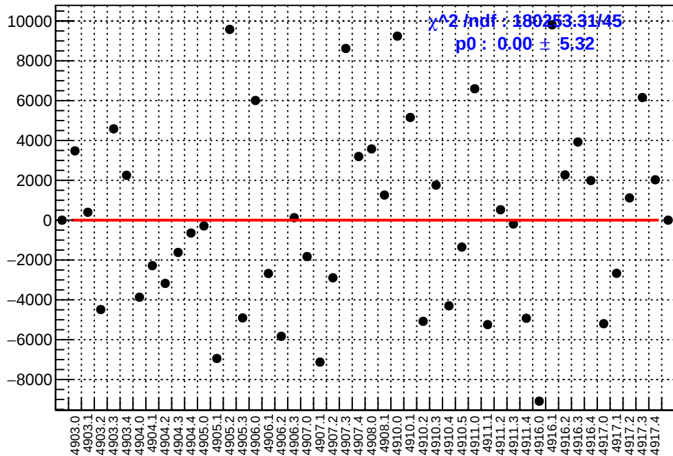
slug91: asym_at2_dd.mean/ppb-reg_asym_at2_dd.mean/ppb
