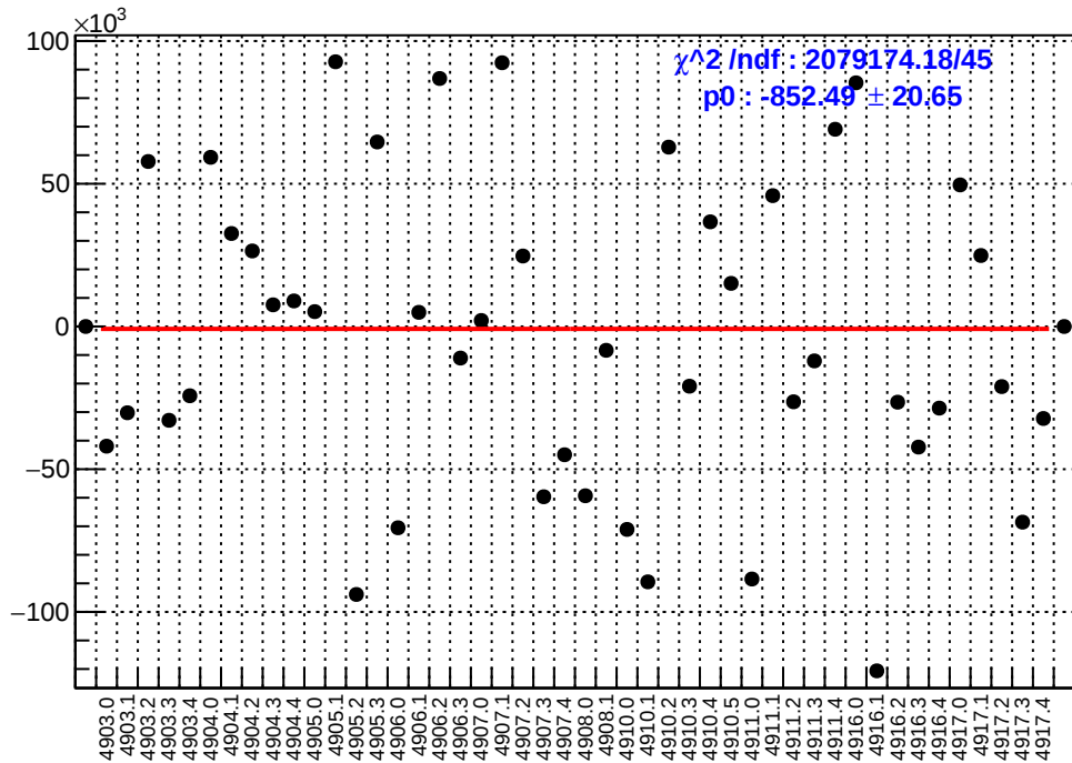
slug91: asym_sam3.mean/ppb-reg_asym_sam3.mean/ppb
