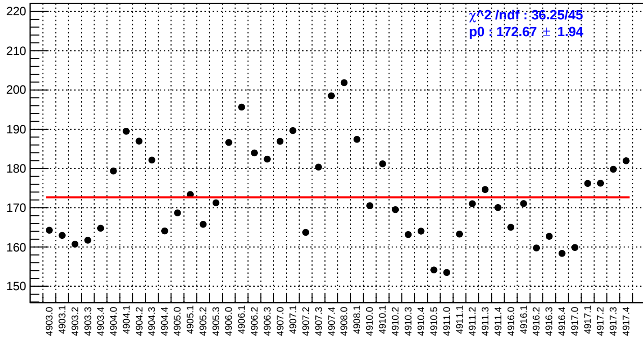
slug91: asym_bcm_an_ds.rms/ppm
