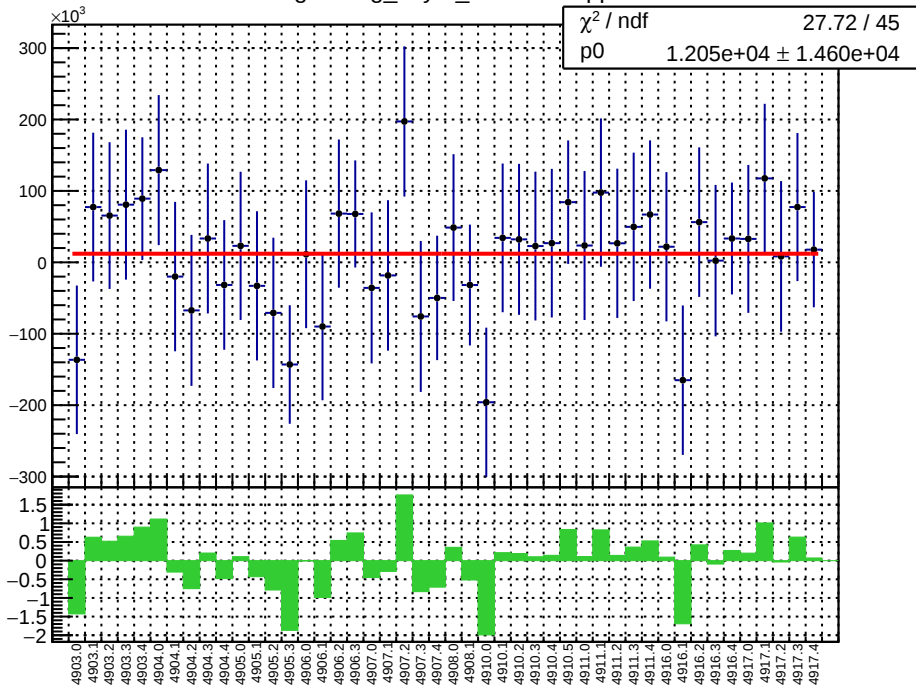
slug91: reg_asym_atr2.mean/ppb
