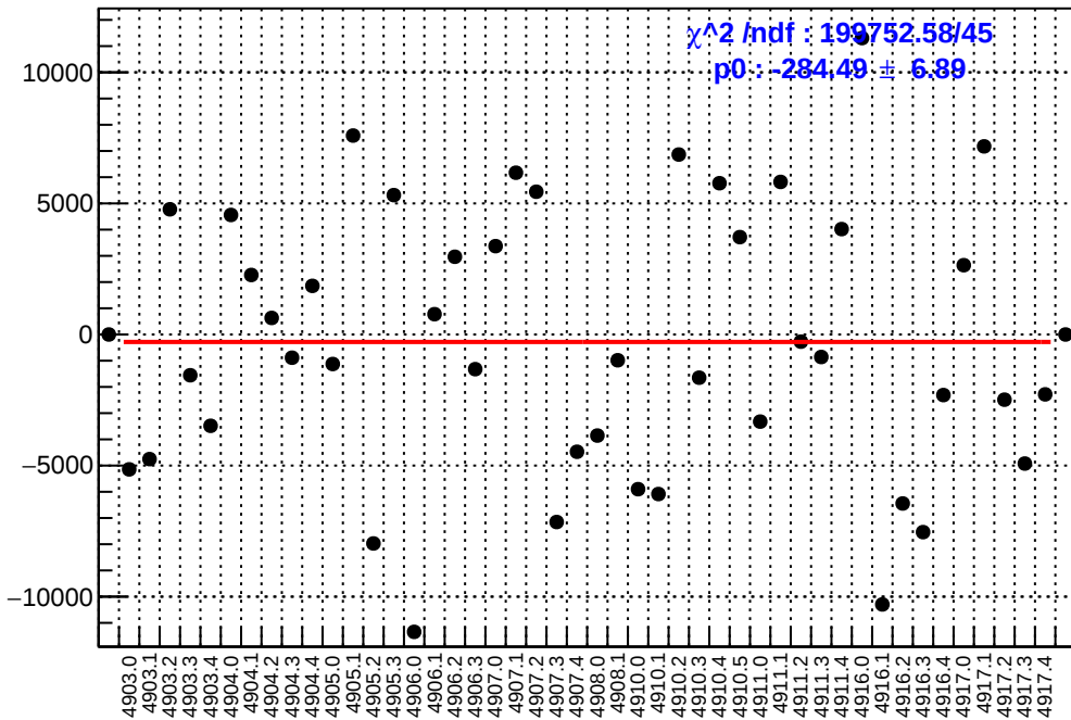
slug91: asym_atl2.mean/ppb-reg_asym_atl2.mean/ppb
