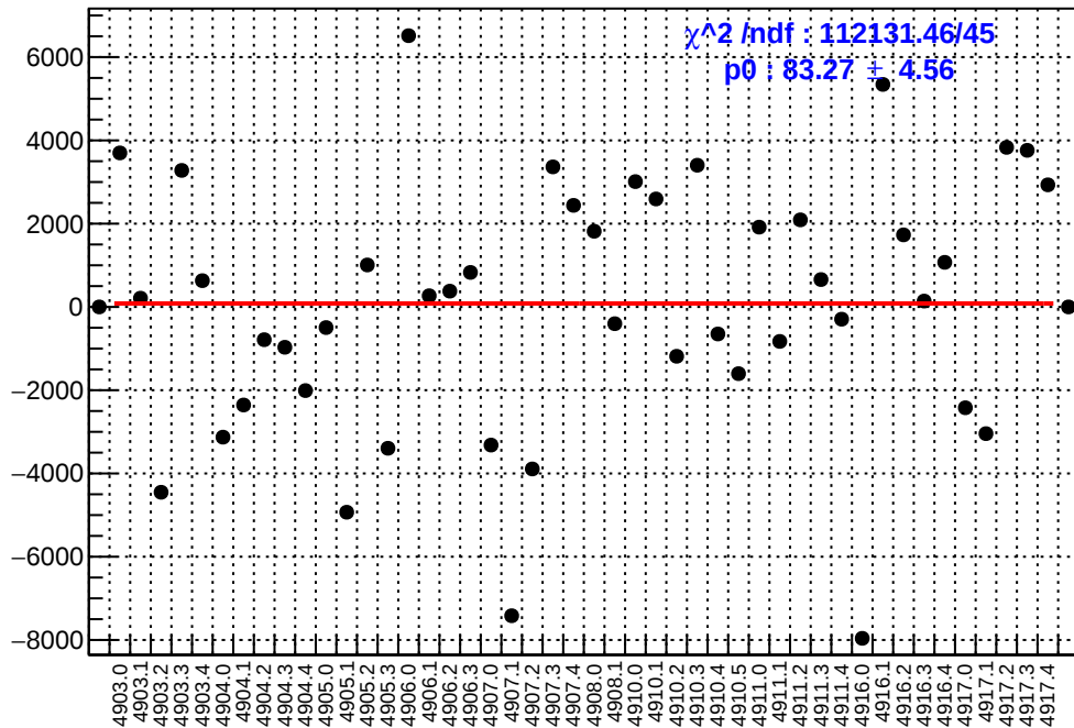
slug91: asym_atr1.mean/ppb-reg_asym_atr1.mean/ppb
