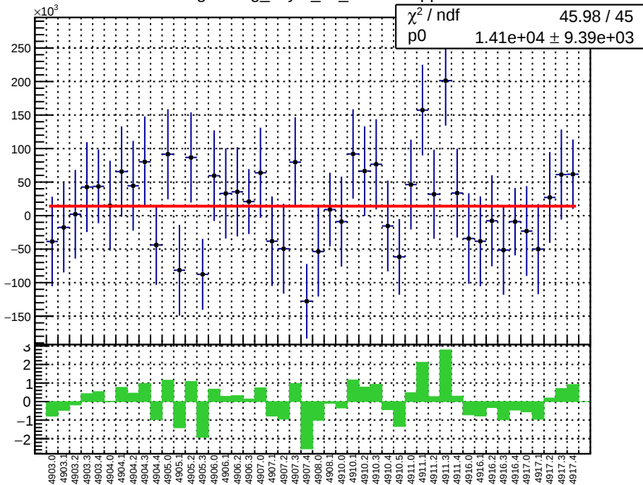
slug91: reg_asym_atl_dd.mean/ppb
