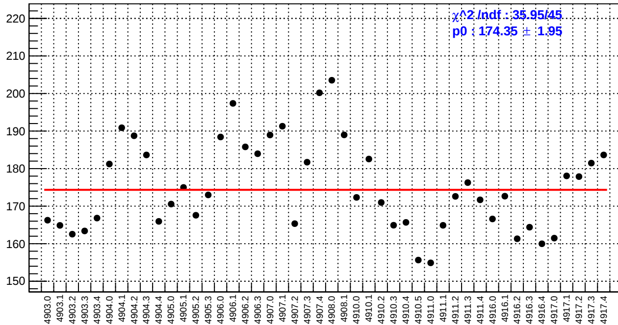
slug91: asym_bcm_an_ds3.rms/ppm
