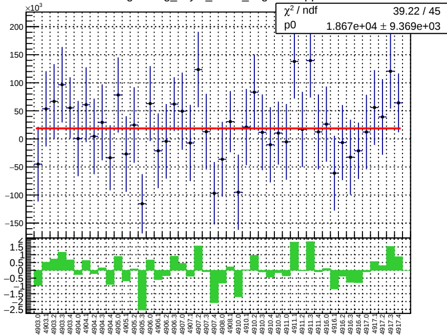
slug91: reg_asym_atl1r2_avg.mean/ppb
