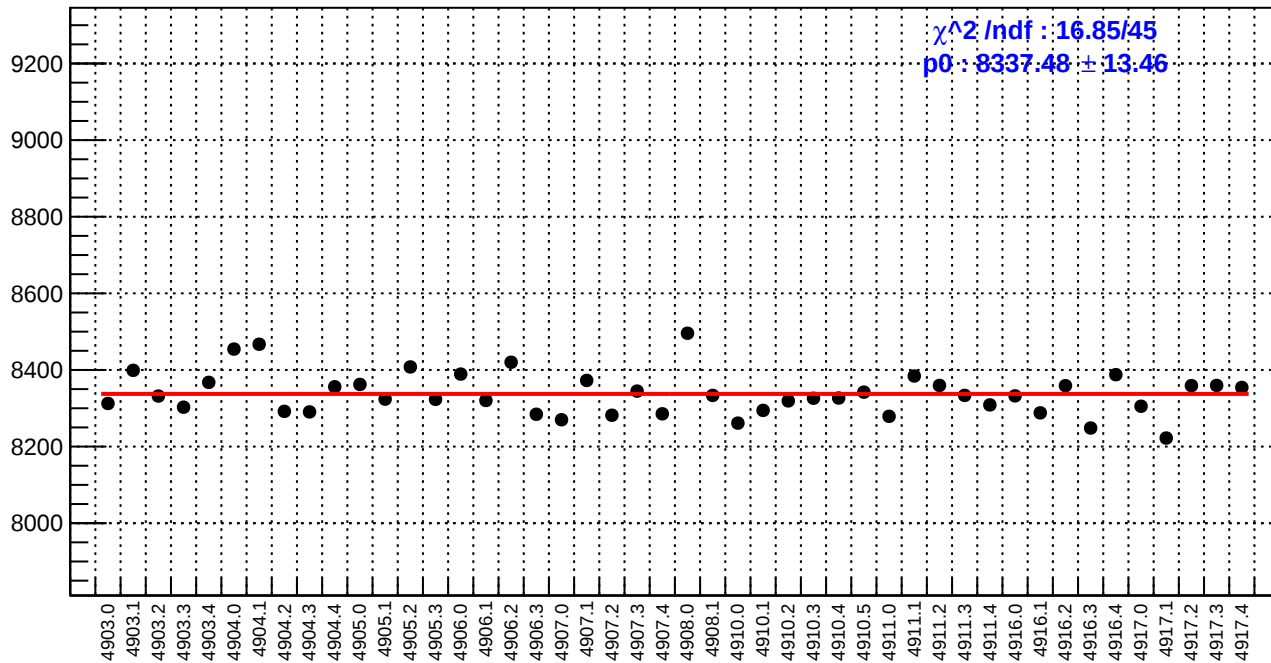
slug91: reg_asym_atr1.rms/ppm
