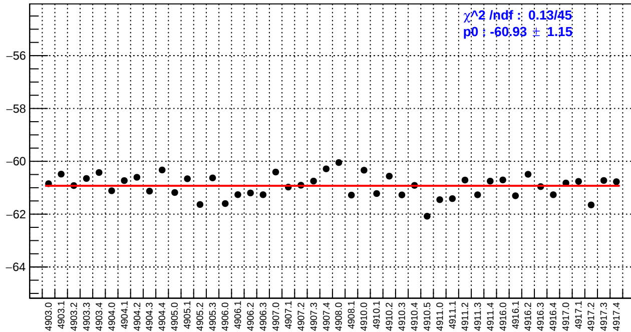
slug91: right_avg_bpm12X/(ppb/nm)
