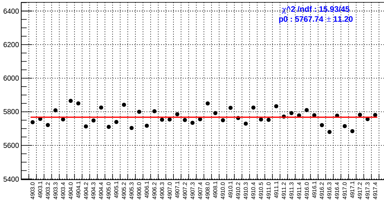
slug91: reg_asym_at1_avg.rms/ppm
