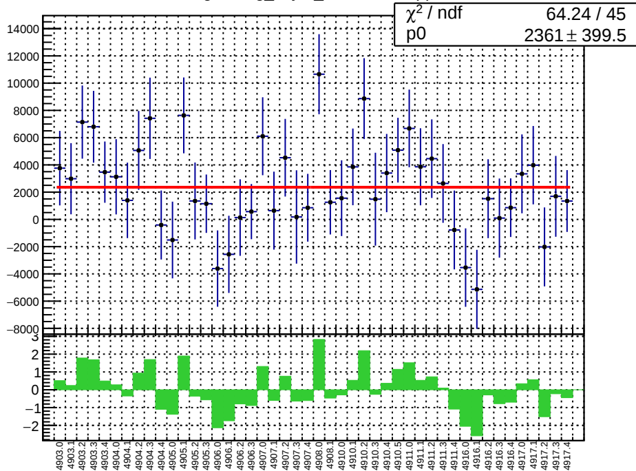
slug91: reg_asym_sam7.mean/ppb
