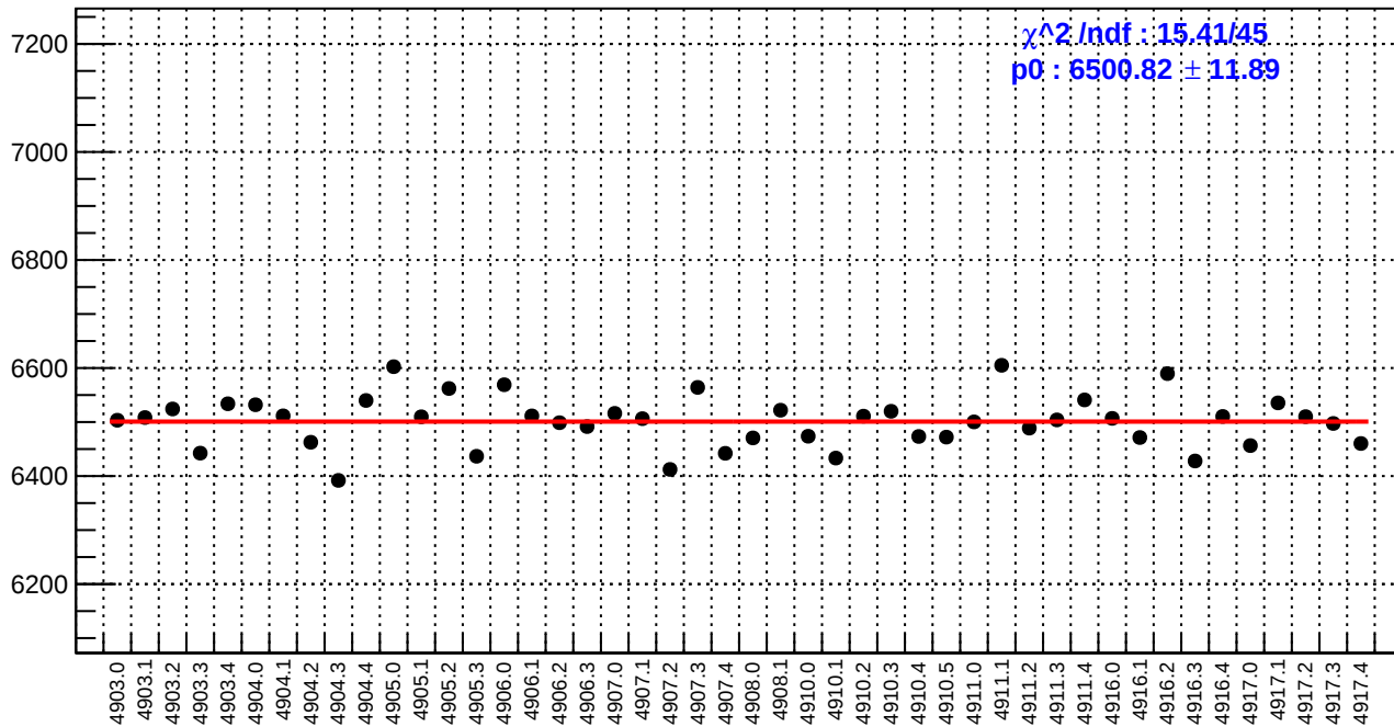
slug91: reg_asym_atr1l2_dd.rms/ppm
