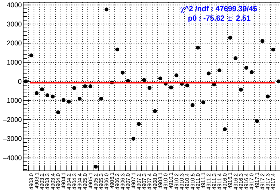
slug91: asym_at1_avg.mean/ppb-reg_asym_at1_avg.mean/ppb
