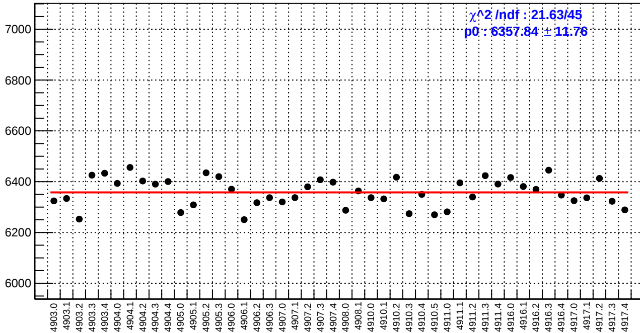
slug91: reg_asym_atl1r2_dd.rms/ppm
