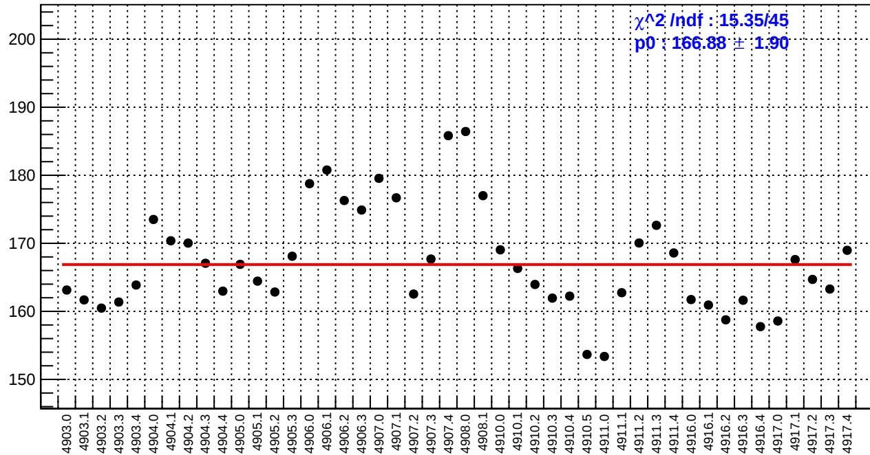
slug91: asym_bcm_an_us.rms/ppm
