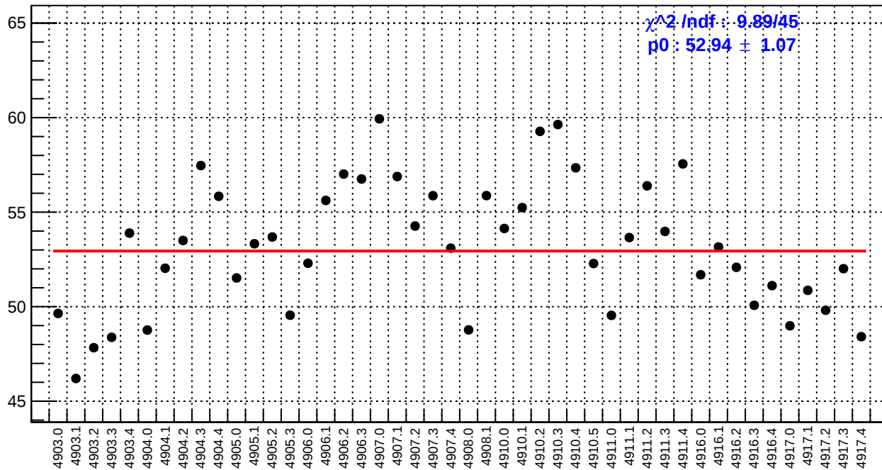
slug91: usl_bpm4aX/(ppb/nm)
