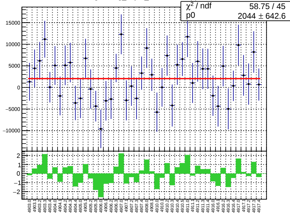
slug91: reg_asym_sam8.mean/ppb
