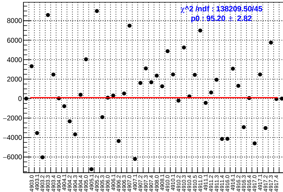
slug91: asym_right_avg.mean/ppb-reg_asym_right_avg.mean/ppb
