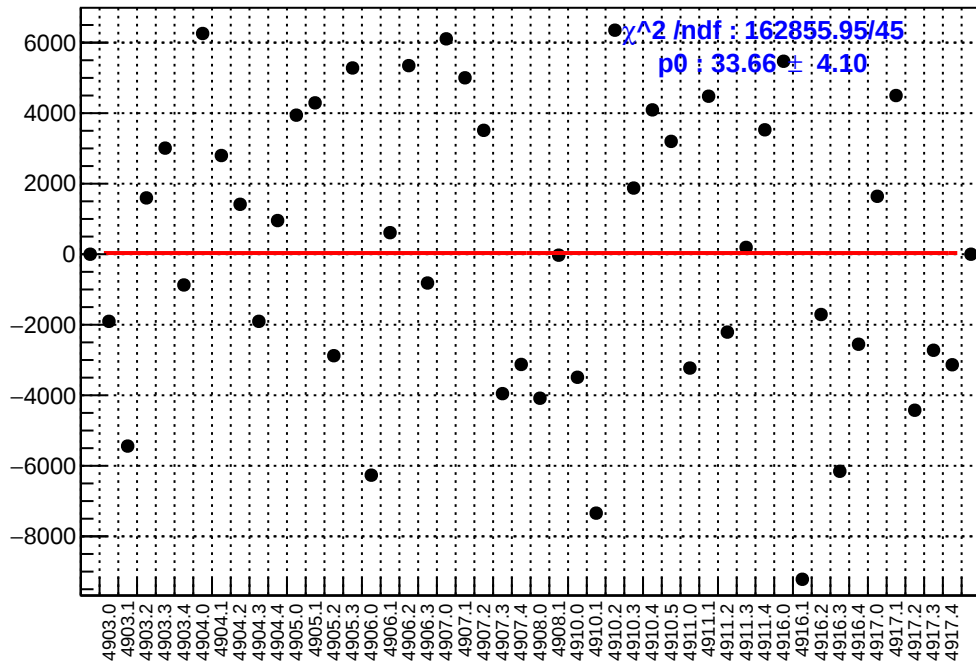
slug91: asym_left_avg.mean/ppb-reg_asym_left_avg.mean/ppb
