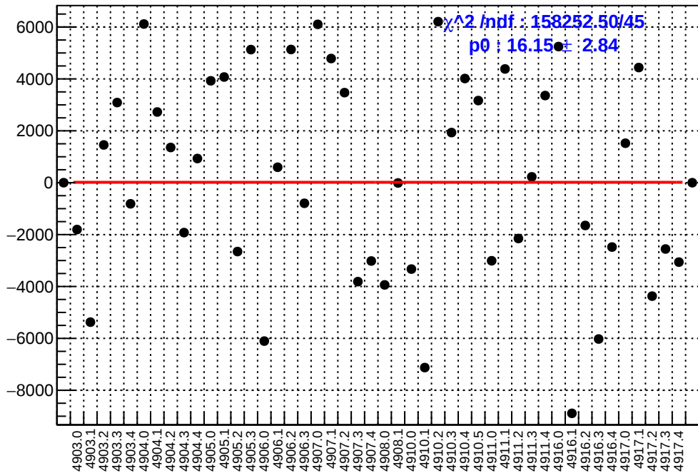
slug91: asym_usl.mean/ppb-reg_asym_usl.mean/ppb
