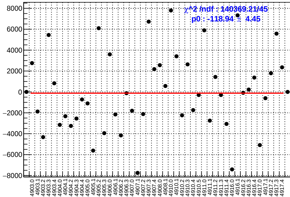
slug91: asym_atr_avg.mean/ppb-reg_asym_atr_avg.mean/ppb
