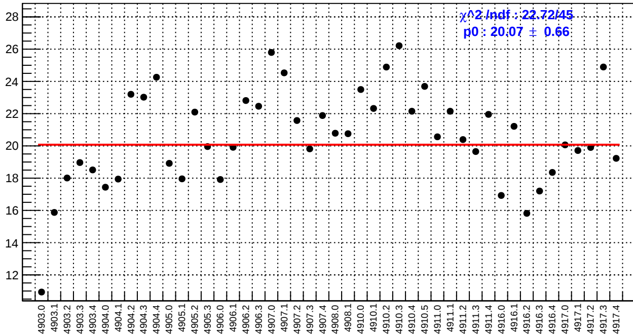
slug91: left_avg_bpm4eY/(ppb/nm)
