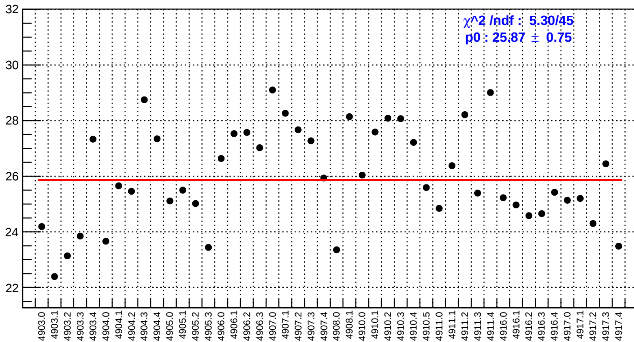
slug91: ds_avg_bpm4aX/(ppb/nm)
