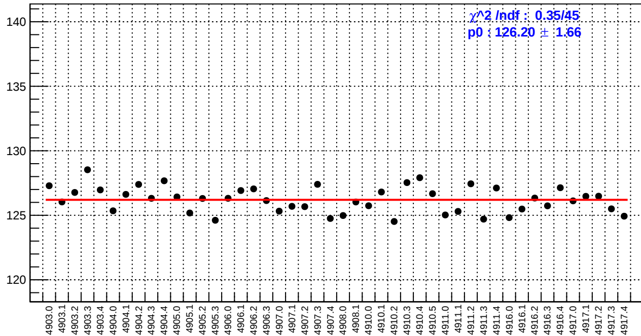
slug91: reg_asym_dsl.rms/ppm
