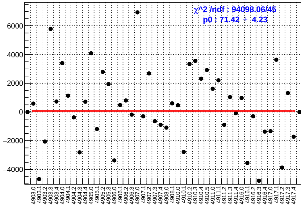
slug91: asym_ds_avg.mean/ppb-reg_asym_ds_avg.mean/ppb
