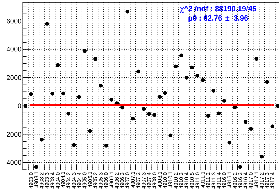
slug91: asym_us_avg.mean/ppb-reg_asym_us_avg.mean/ppb
