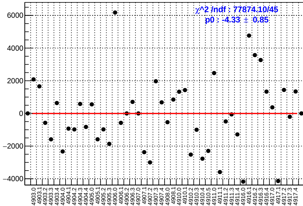
slug91: asym_atl_dd.mean/ppb-reg_asym_atl_dd.mean/ppb
