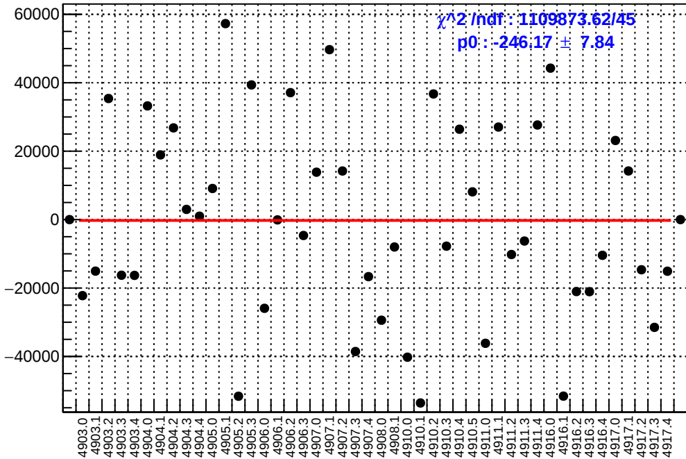
slug91: asym_sam4.mean/ppb-reg_asym_sam4.mean/ppb
