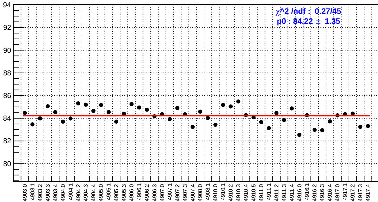
slug91: reg_asym_us_dd.rms/ppm
