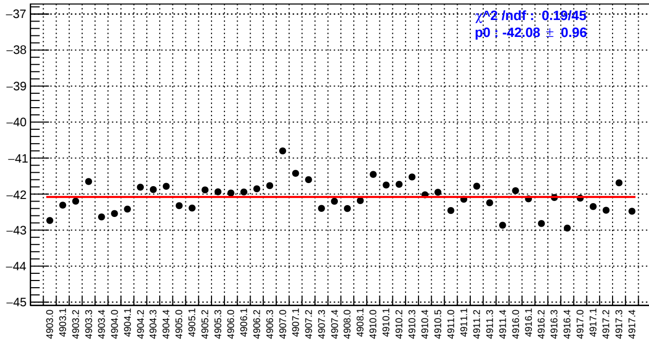
slug91: dsl_bpm12X/(ppb/nm)
