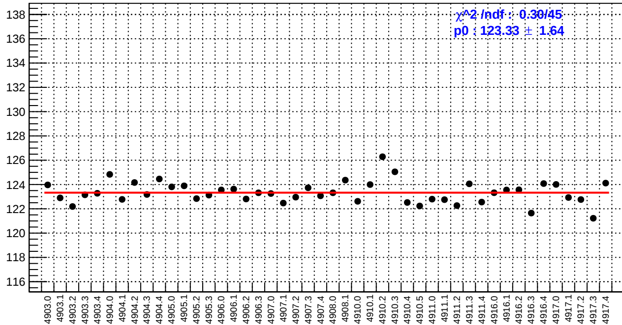
slug91: reg_asym_dsr.rms/ppm
