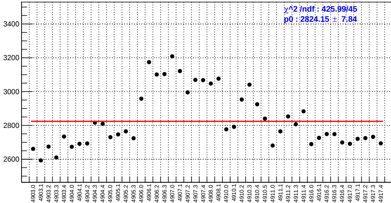
slug91: diff_bpm4aY.rms/nm
