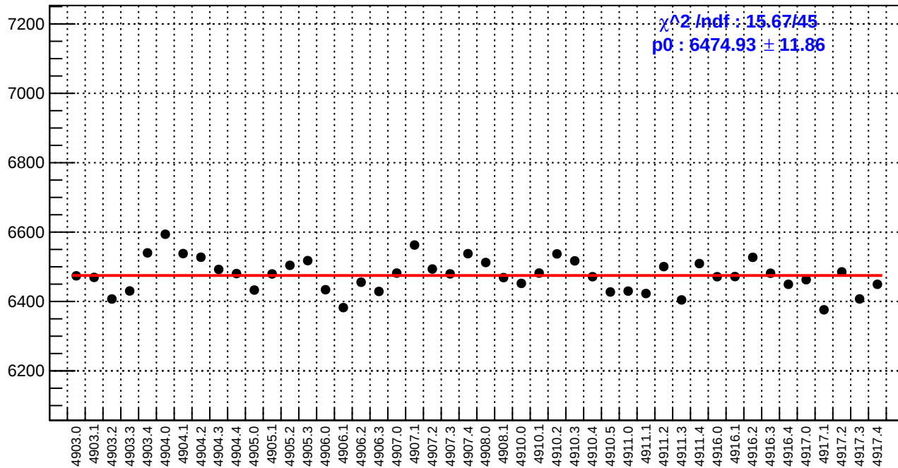
slug91: reg_asym_atr_dd.rms/ppm
