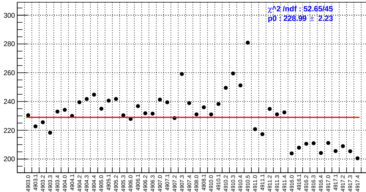
slug91: reg_asym_sam5.rms/ppm
