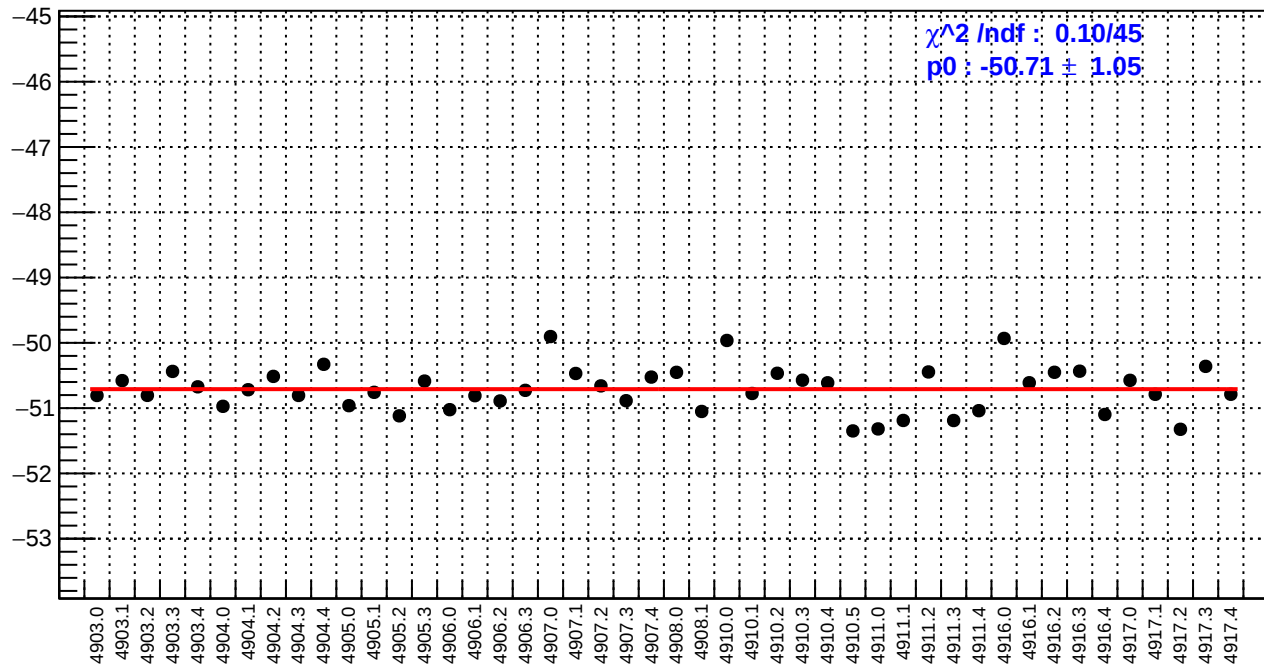
slug91: us_avg_bpm12X/(ppb/nm)
