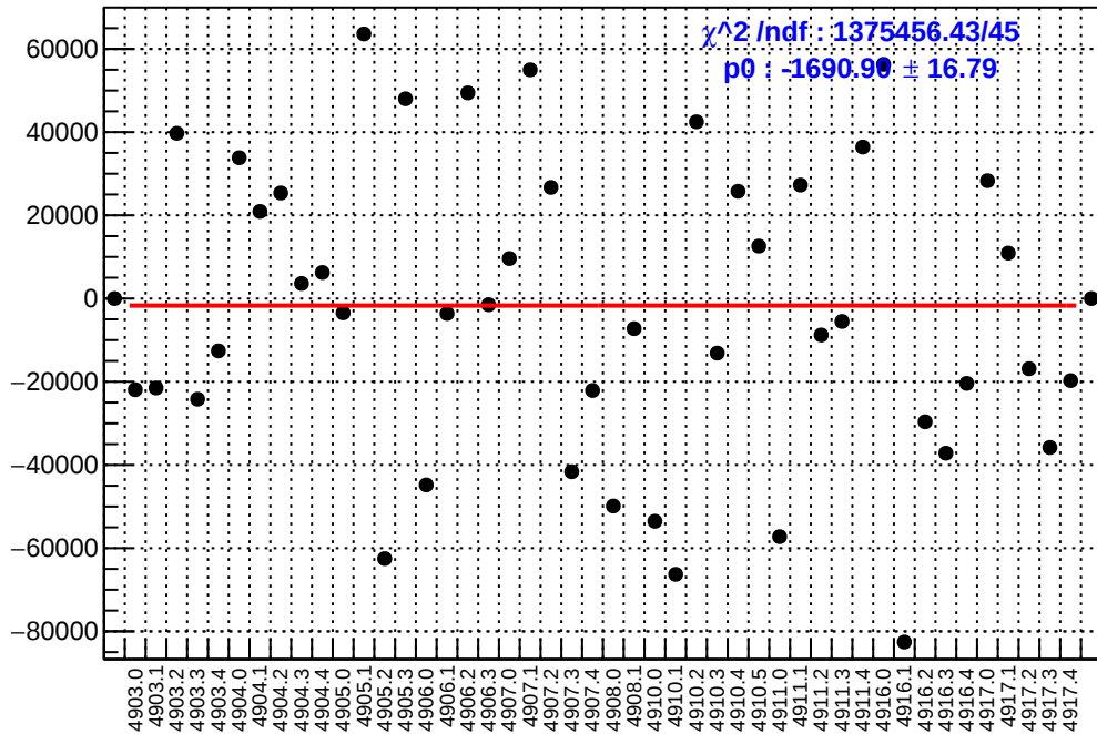
slug91: asym_sam2.mean/ppb-reg_asym_sam2.mean/ppb
