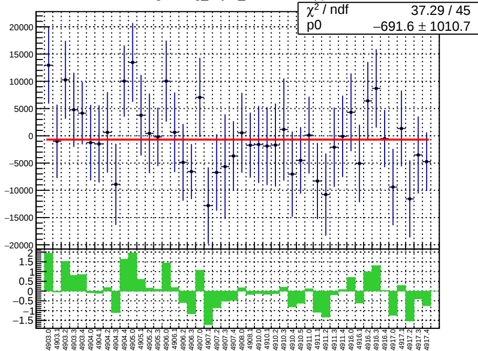
slug91: reg_asym_sam3.mean/ppb
