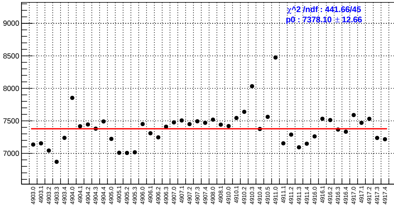
slug91: diff_bpm4eX.rms/nm
