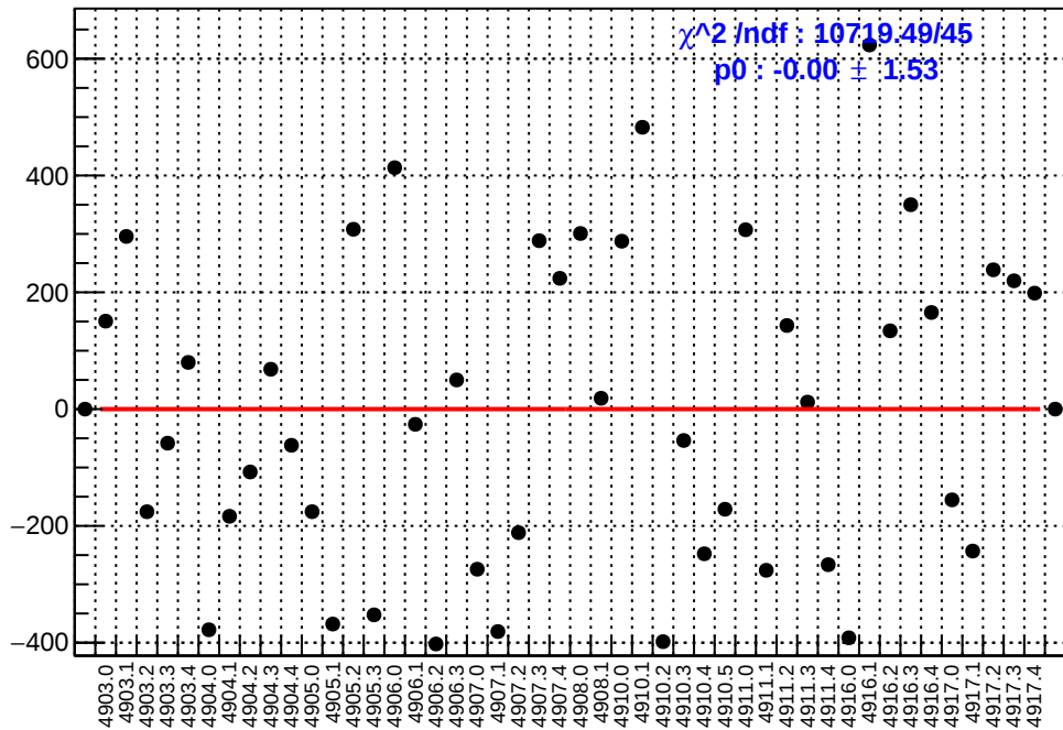
slug91: asym_right_dd.mean/ppb-reg_asym_right_dd.mean/ppb
