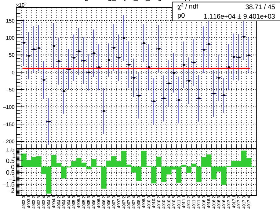
slug91: reg_asym_atl_avg.mean/ppb
