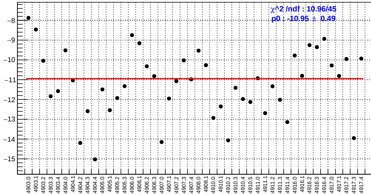
slug91: ds_avg_bpm4aY/(ppb/nm)
