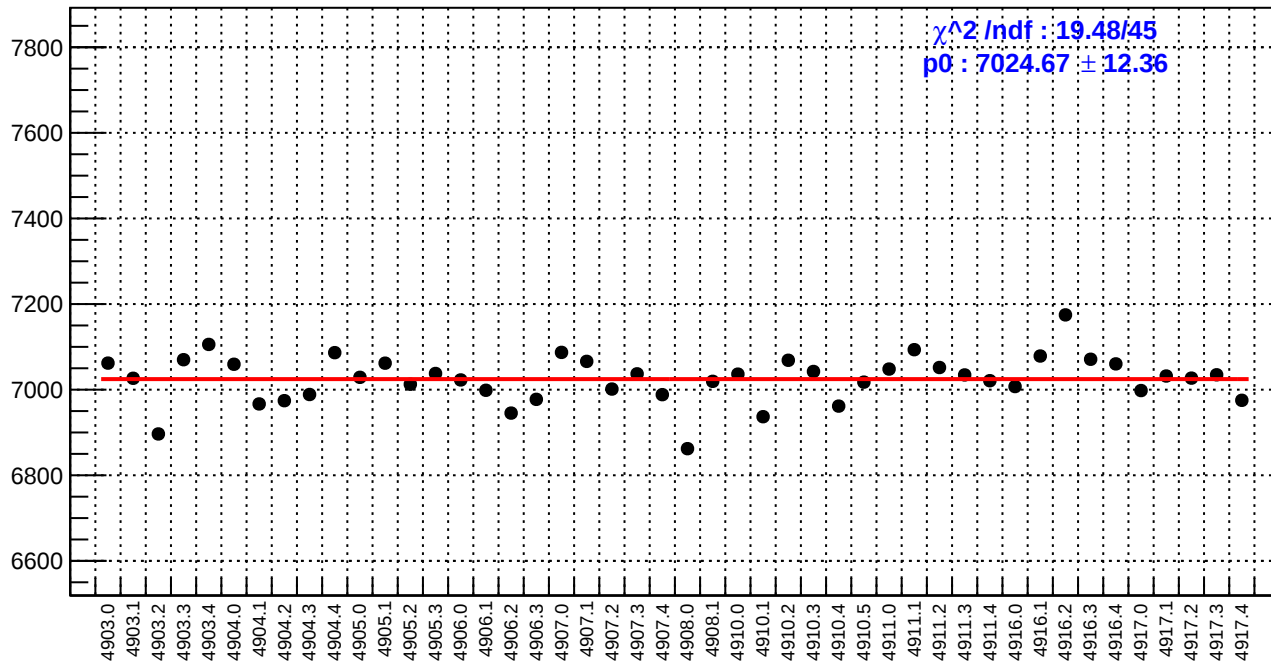
slug91: reg_asym_at2_avg.rms/ppm
