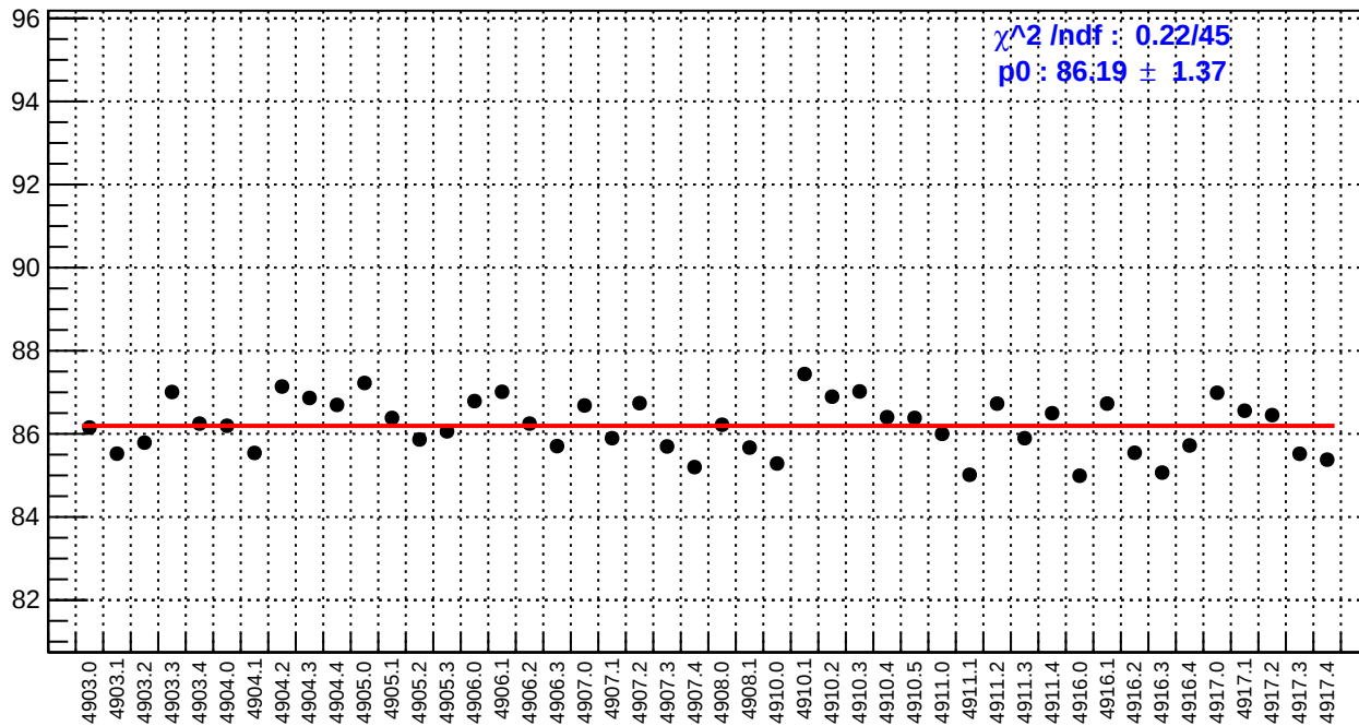
slug91: reg_asym_ds_dd.rms/ppm
