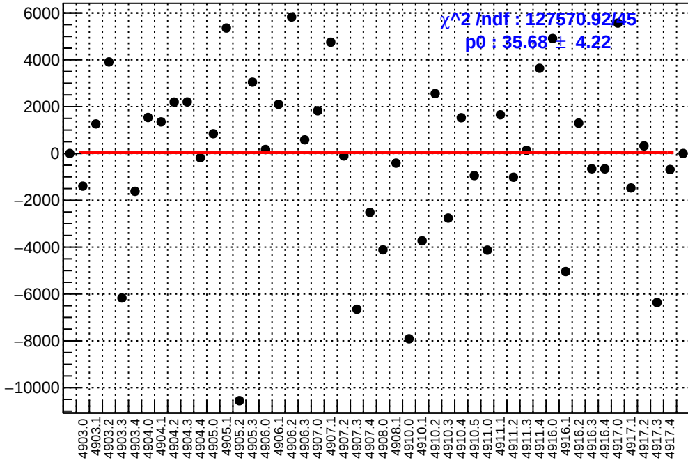
slug91: asym_atl1r2_dd.mean/ppb-reg_asym_atl1r2_dd.mean/ppb
