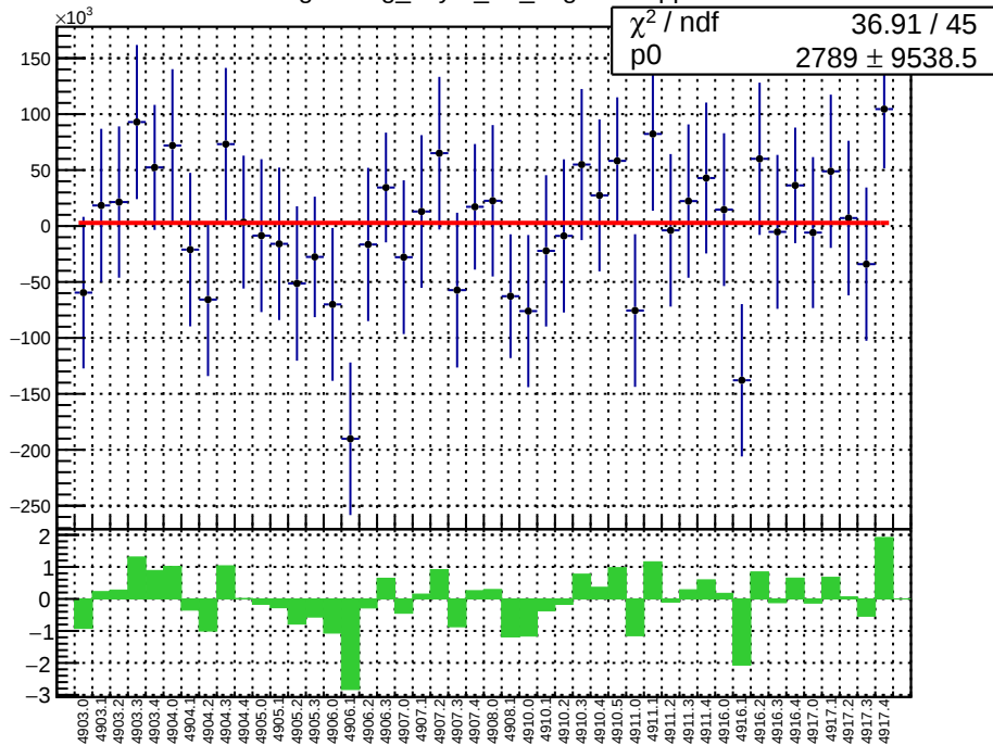
slug91: reg_asym_atr_avg.mean/ppb
