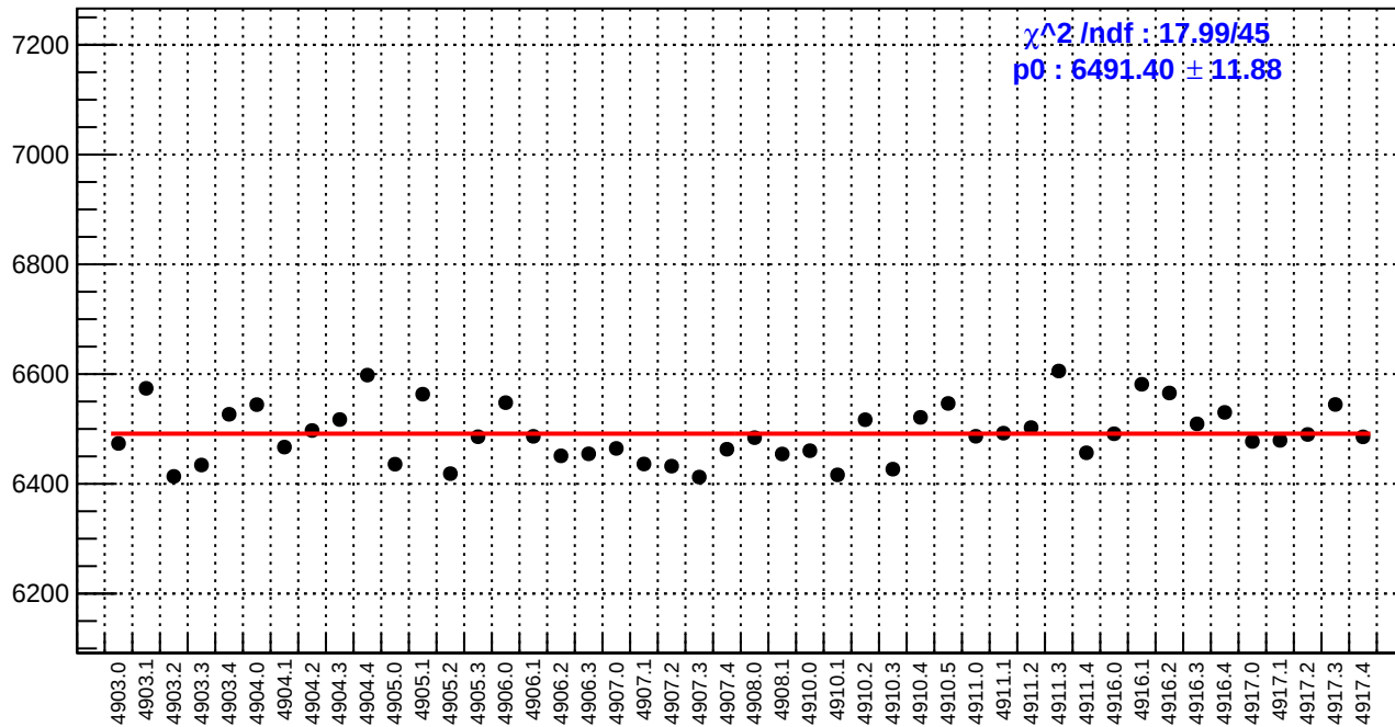
slug91: reg_asym_atr1l2_avg.rms/ppm
