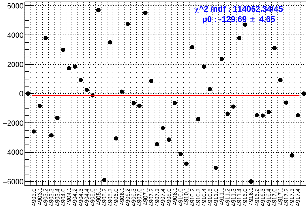
slug91: asym_ds_dd.mean/ppb-reg_asym_ds_dd.mean/ppb
