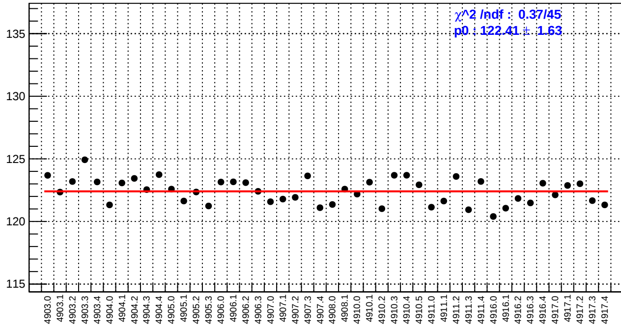
slug91: reg_asym_left_avg.rms/ppm
