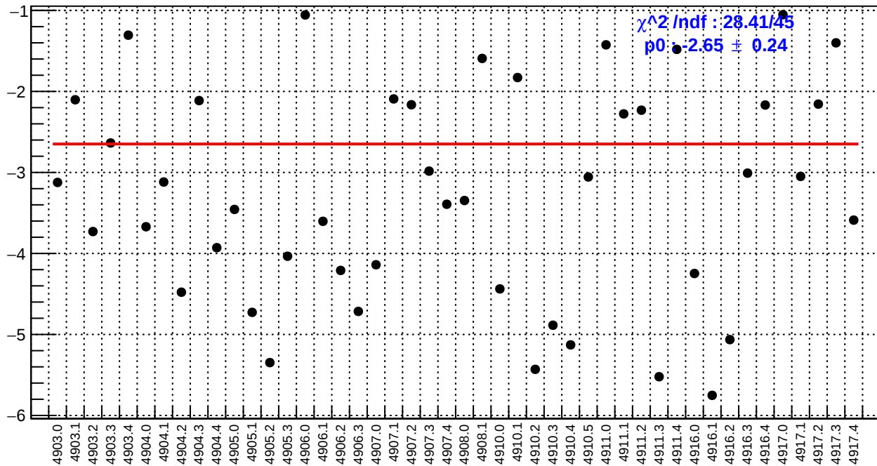
slug91: dsr_bpm4aX/(ppb/nm)
