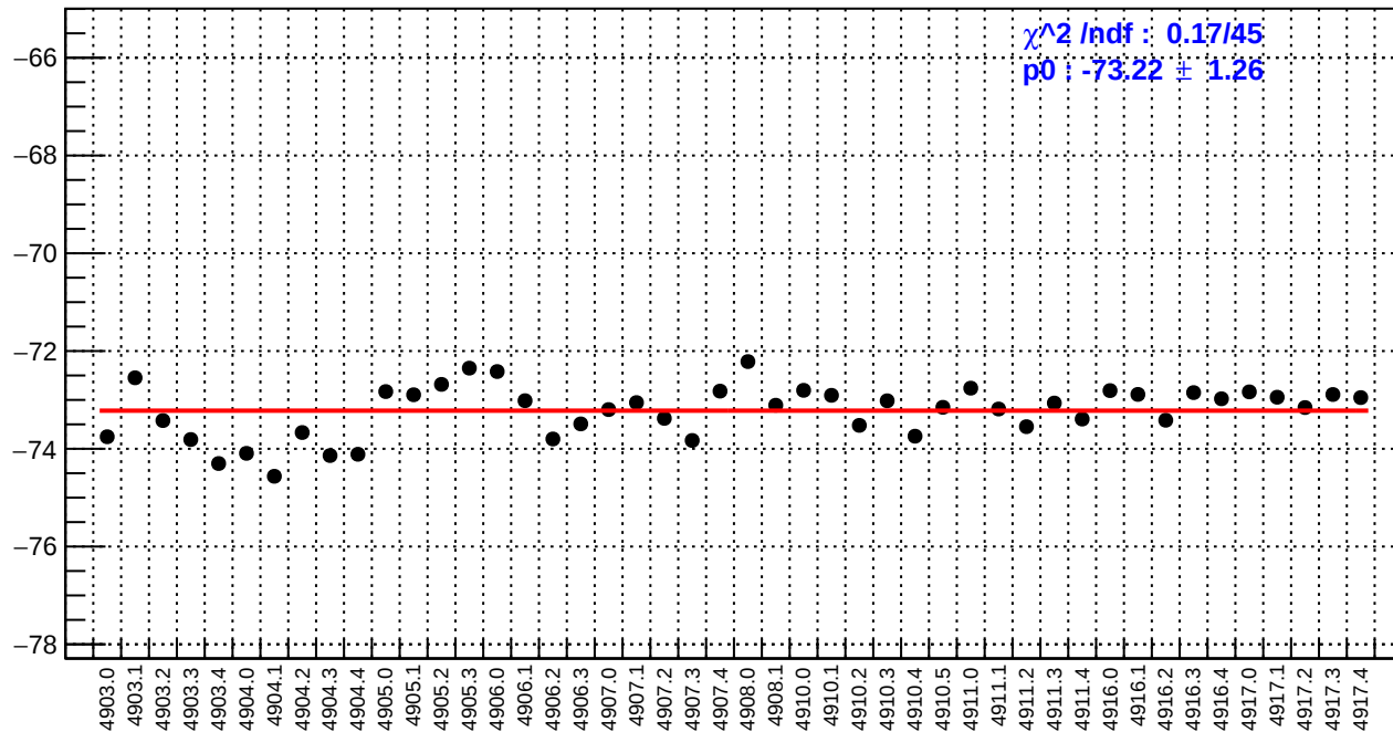
slug91: dsl_bpm4eX/(ppb/nm)
