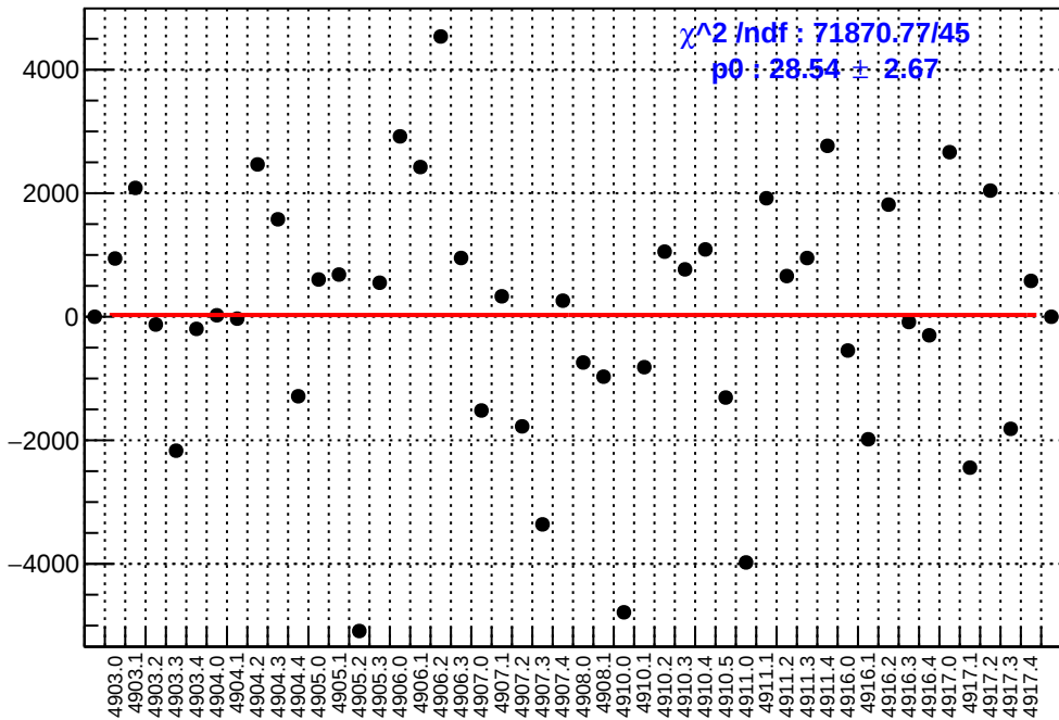
slug91: asym_atr_dd.mean/ppb-reg_asym_atr_dd.mean/ppb
