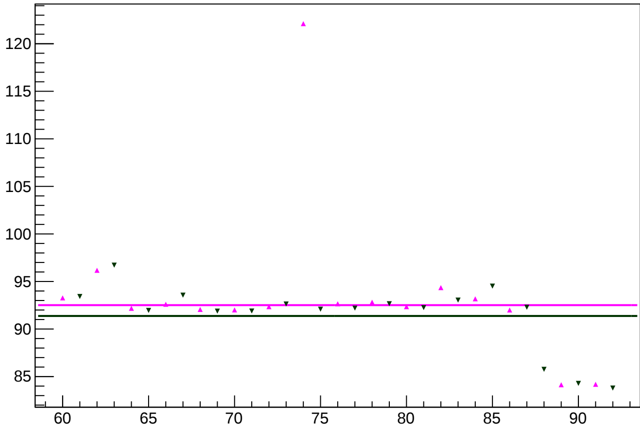
reg_asym_us_dd_rms vs slug
