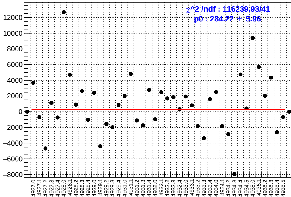
slug93: asym_atl_avg.mean/ppb-reg_asym_atl_avg.mean/ppb
