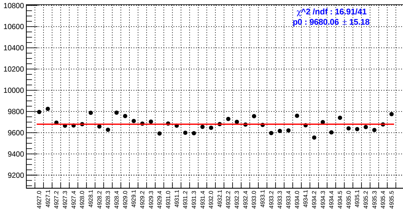
slug93: reg_asym_atr2.rms/ppm
