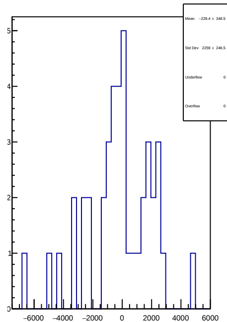
slug93: 1D Corr asym_atl_dd.mean/ppb-reg_asym_atl_dd.mean/ppb
