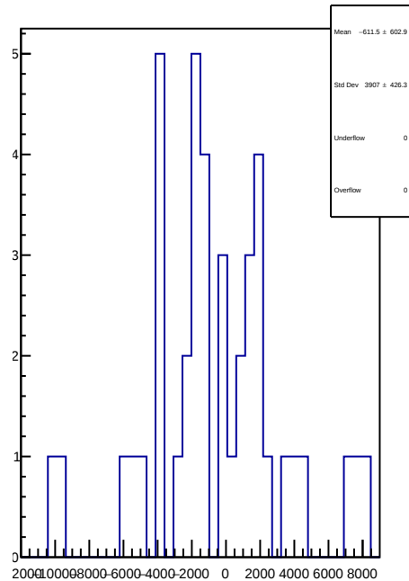
slug93: 1D Corr asym_atr1l2_dd.mean/ppb-reg_asym_atr1l2_dd.mean/ppb
