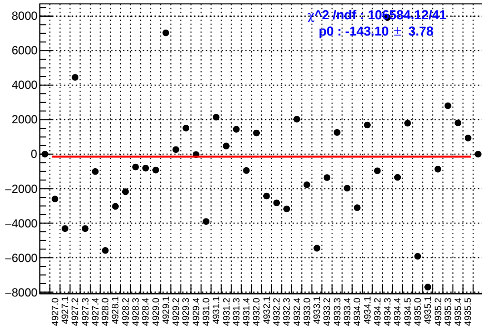
slug93: asym_usr.mean/ppb-reg_asym_usr.mean/ppb
