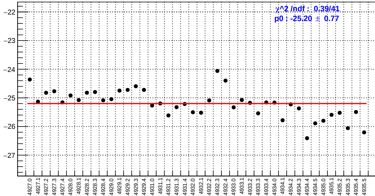
slug93: us_avg_bpm4eX/(ppb/nm)
