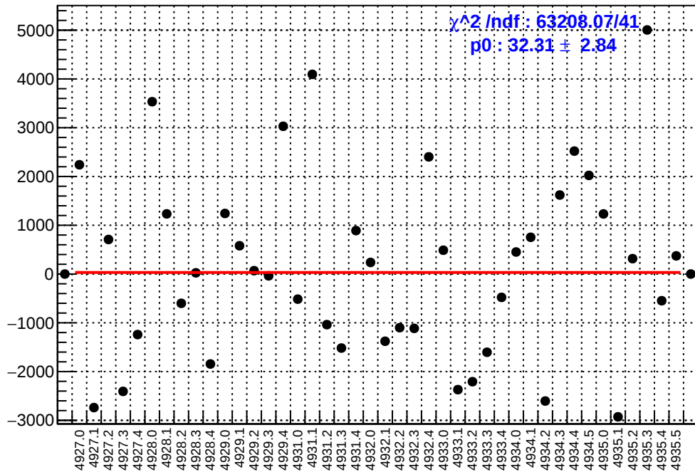
slug93: asym_us_avg.mean/ppb-reg_asym_us_avg.mean/ppb
