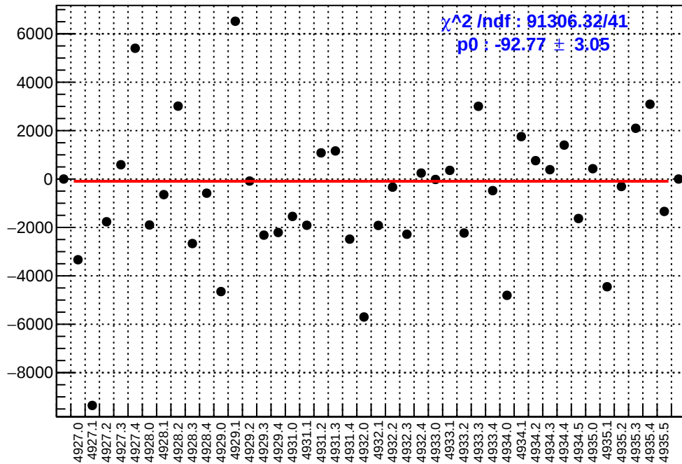
slug93: asym_sam1.mean/ppb-reg_asym_sam1.mean/ppb
