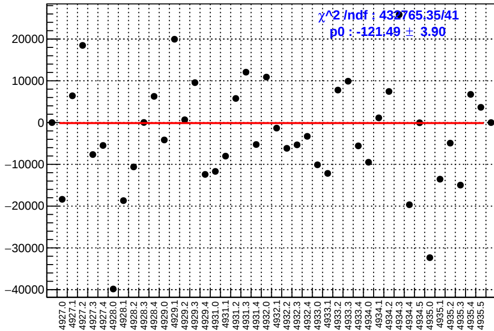
slug93: asym_sam6.mean/ppb-reg_asym_sam6.mean/ppb
