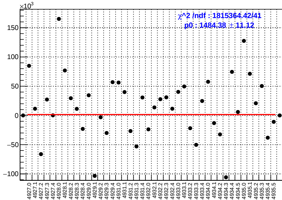
slug93: asym_sam3.mean/ppb-reg_asym_sam3.mean/ppb
