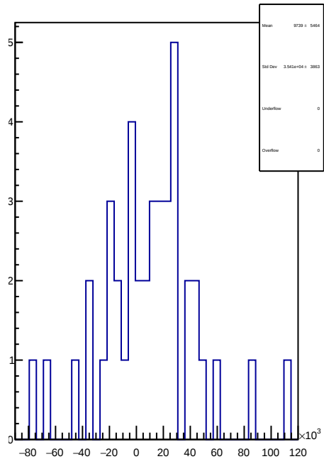
slug93: 1D Corr asym_sam2.mean/ppb-reg_asym_sam2.mean/ppb
