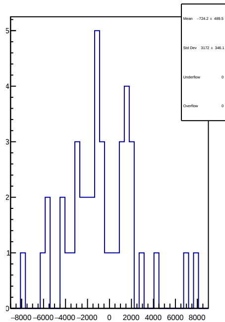
slug93: 1D Corr asym_usr.mean/ppb-reg_asym_usr.mean/ppb
