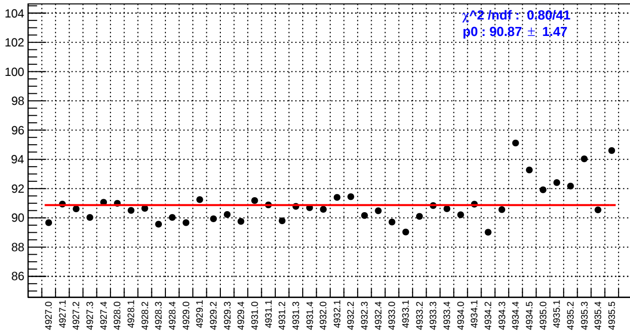
slug93: reg_asym_ds_avg.rms/ppm
