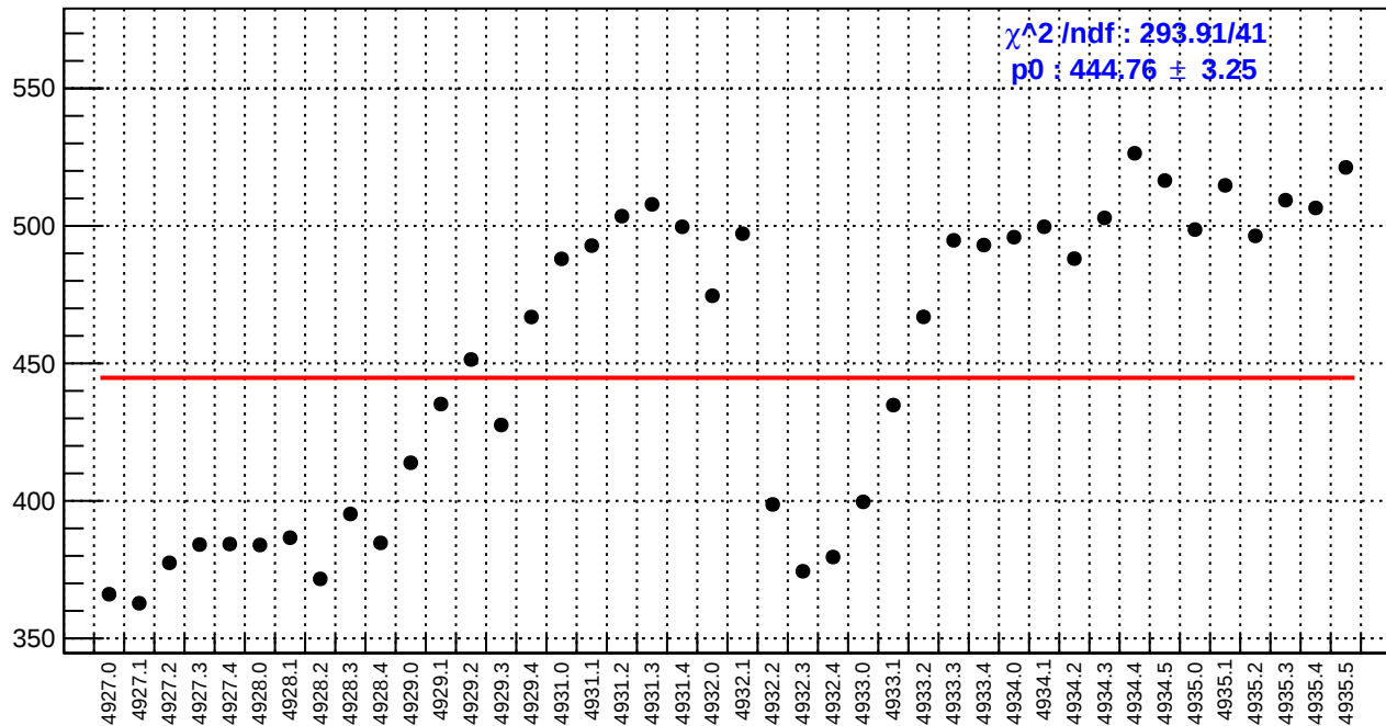
slug93: reg_asym_sam6.rms/ppm
