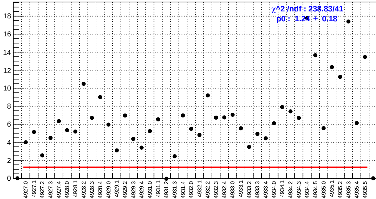
slug93: right_avg_bpm4eY/(ppb/nm)
