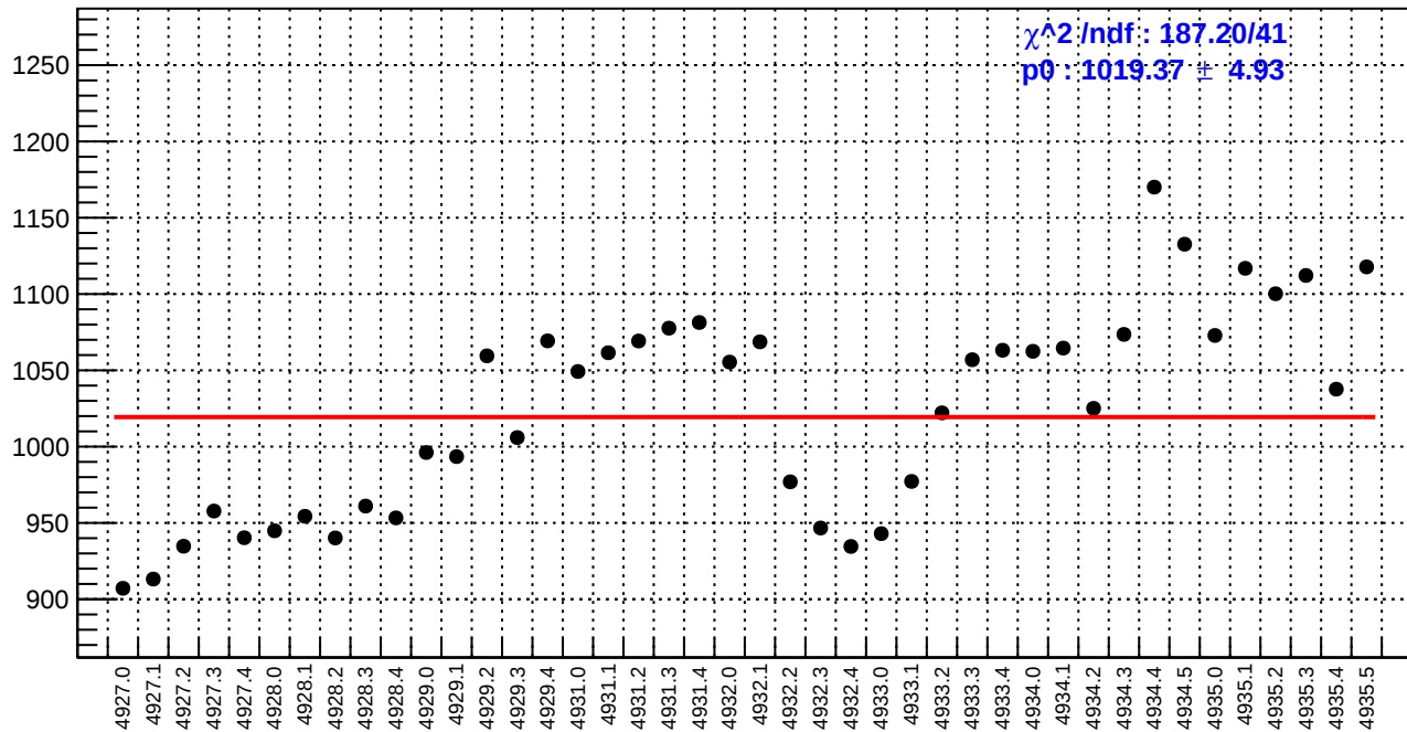
slug93: reg_asym_sam4.rms/ppm
