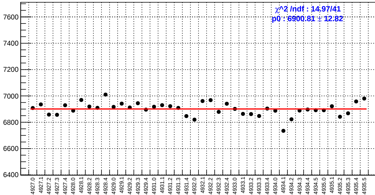
slug93: reg_asym_at2_avg.rms/ppm
