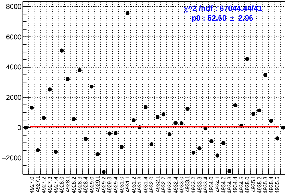
slug93: asym_atr1l2_avg.mean/ppb-reg_asym_atr1l2_avg.mean/ppb
