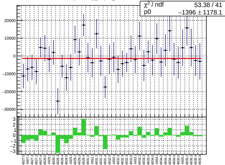
slug93: reg_asym_sam3.mean/ppb
