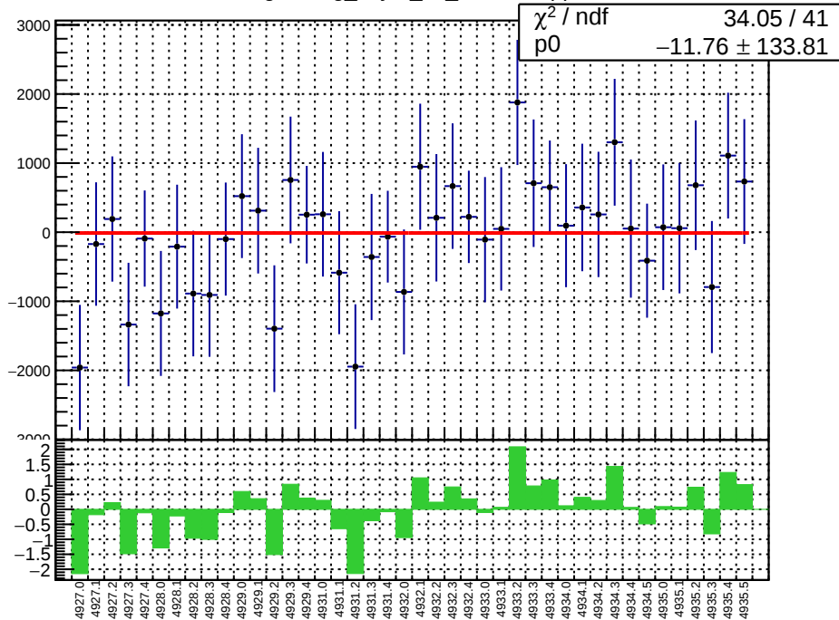
slug93: reg_asym_ds_dd.mean/ppb
