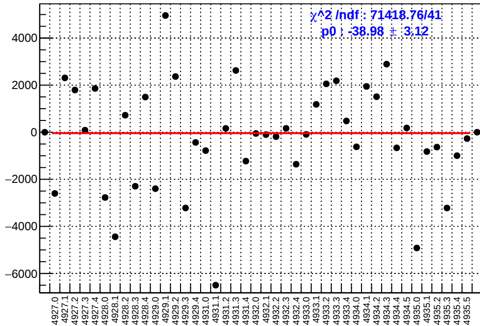
slug93: asym_atl_dd.mean/ppb-reg_asym_atl_dd.mean/ppb
