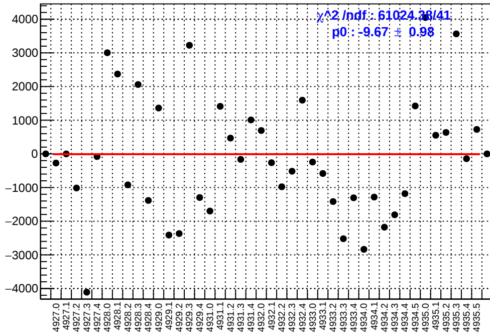
slug93: asym_at2_avg.mean/ppb-reg_asym_at2_avg.mean/ppb
