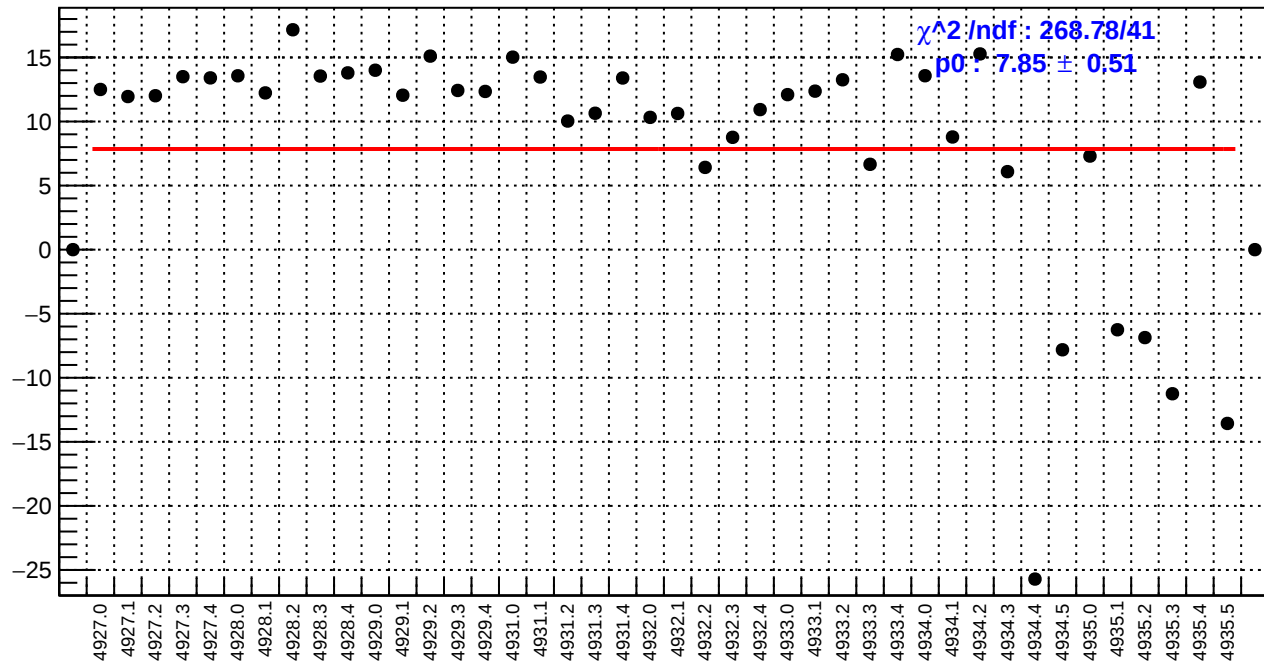
slug93: ds_avg_bpm4eY/(ppb/nm)
