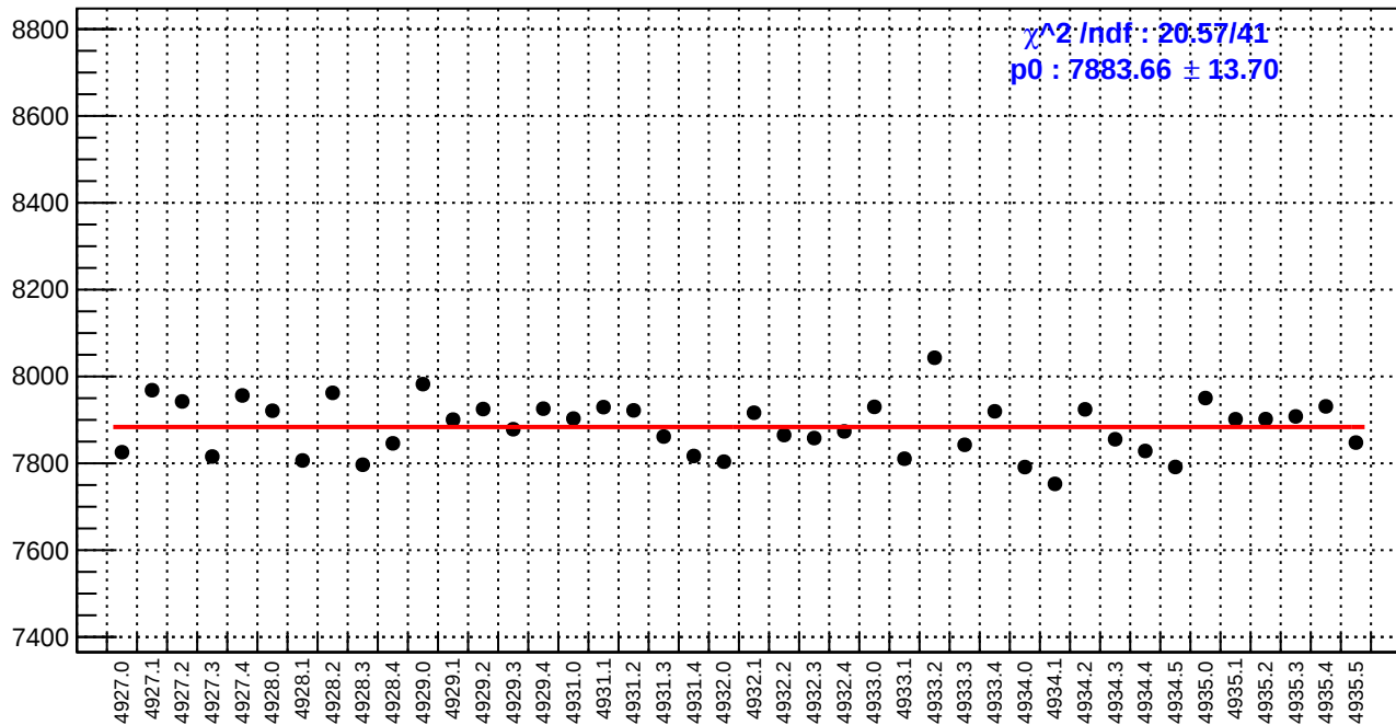
slug93: reg_asym_atl1.rms/ppm
