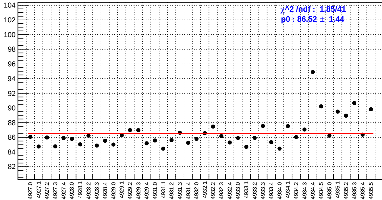
slug93: reg_asym_ds_dd.rms/ppm
