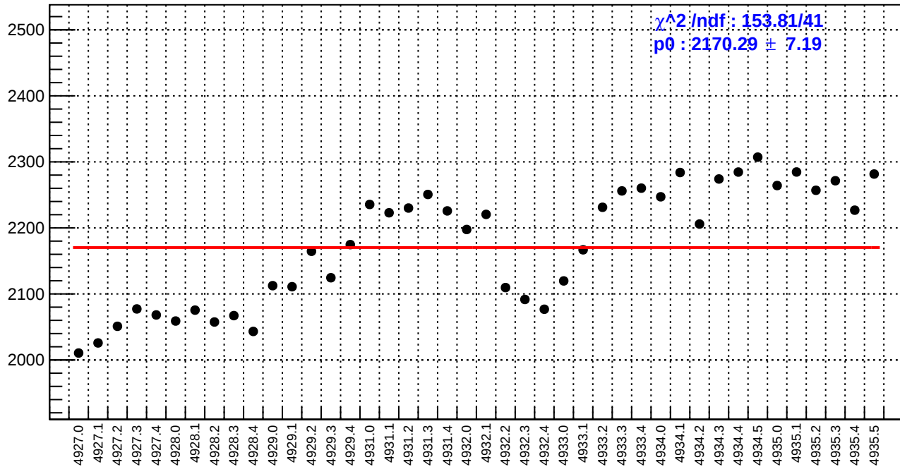
slug93: reg_asym_sam2.rms/ppm
