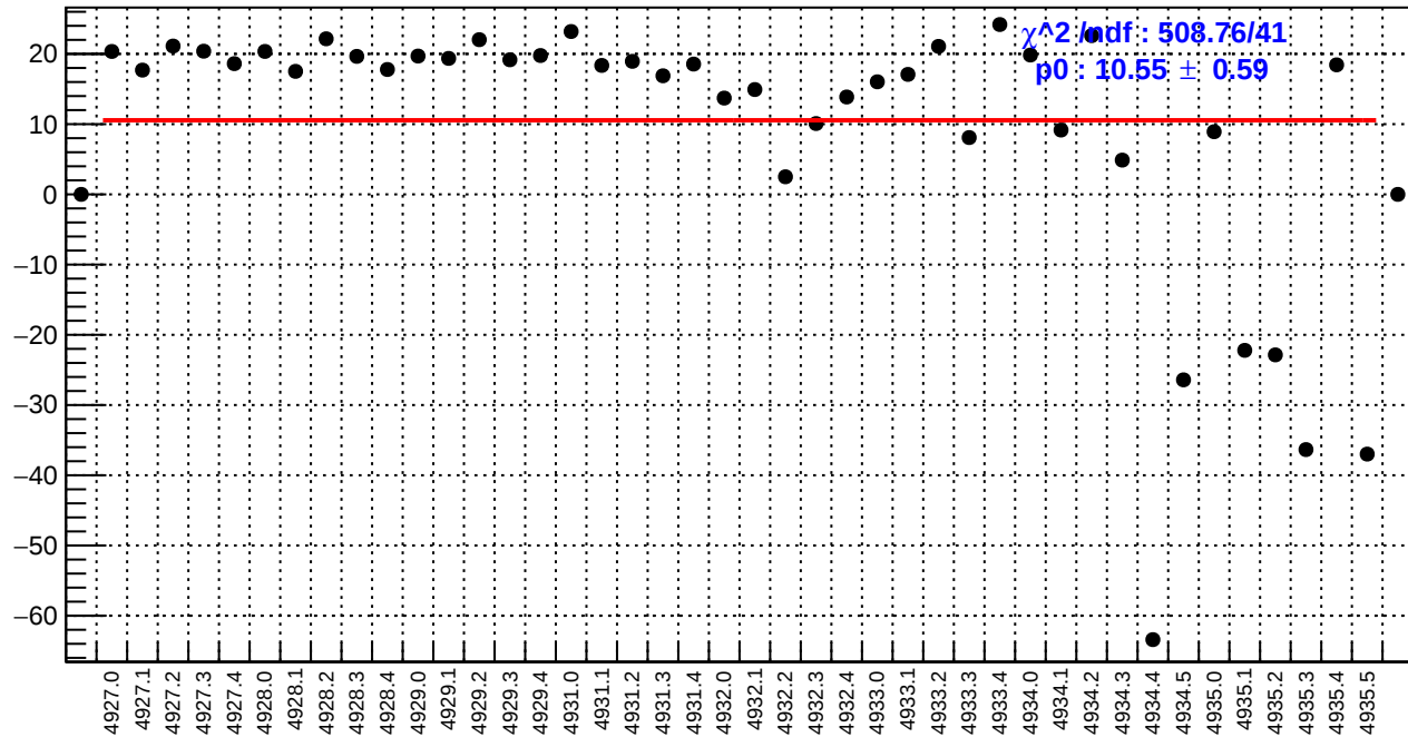
slug93: left_avg_bpm4eY/(ppb/nm)
