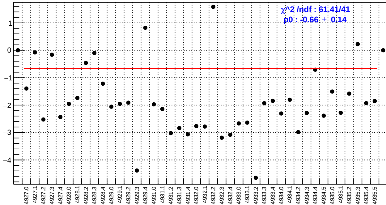
slug93: dsr_bpm4aX/(ppb/nm)
