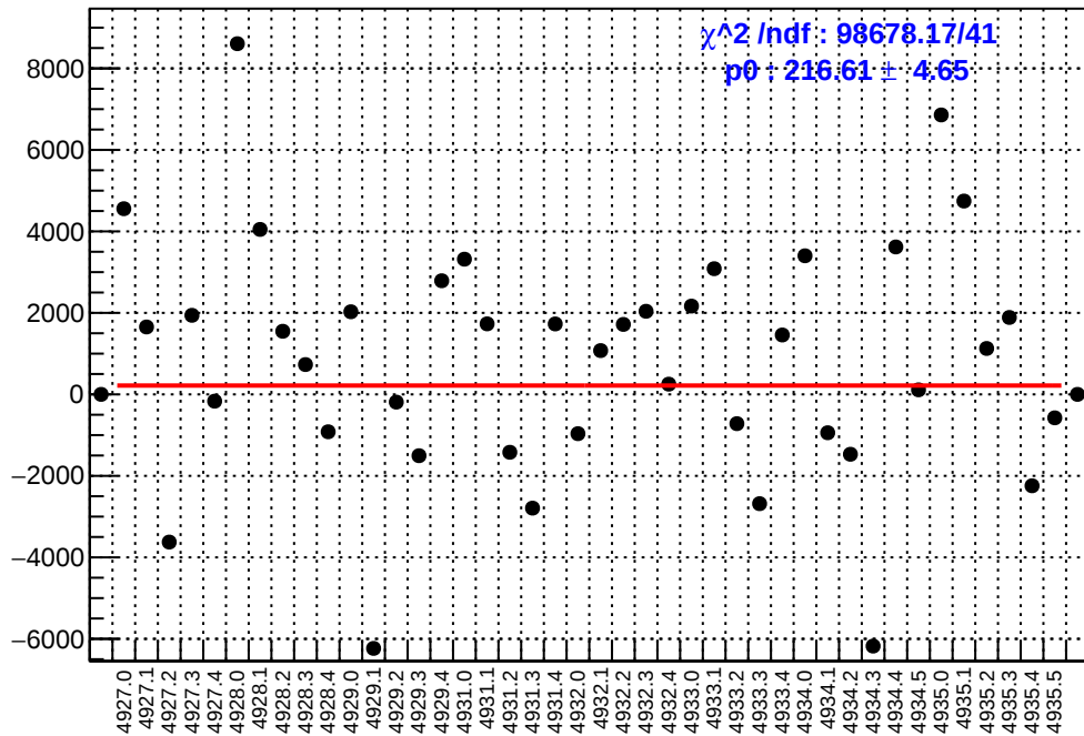
slug93: asym_ds_dd.mean/ppb-reg_asym_ds_dd.mean/ppb
