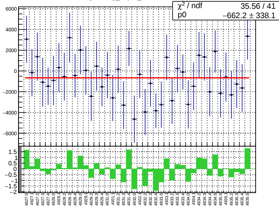
slug93: reg_asym_sam5.mean/ppb
