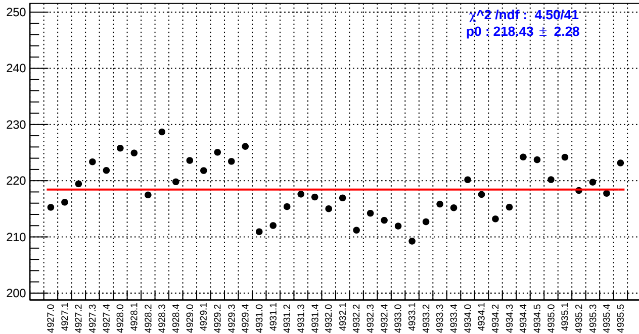
slug93: reg_asym_sam5.rms/ppm
