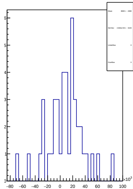
slug93: 1D Corr asym_sam4.mean/ppb-reg_asym_sam4.mean/ppb
