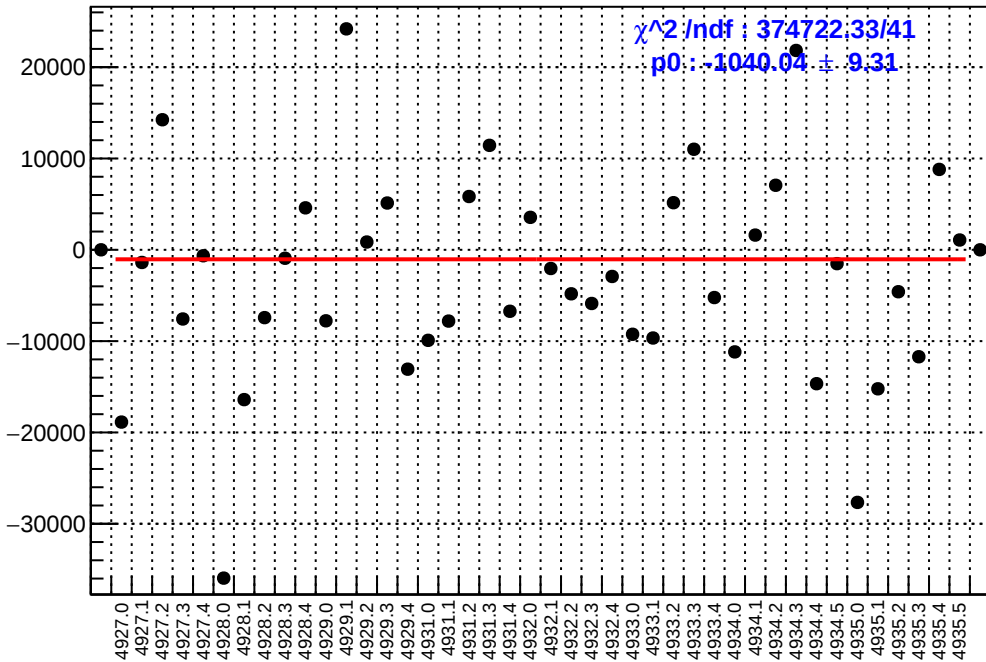
slug93: asym_sam7.mean/ppb-reg_asym_sam7.mean/ppb
