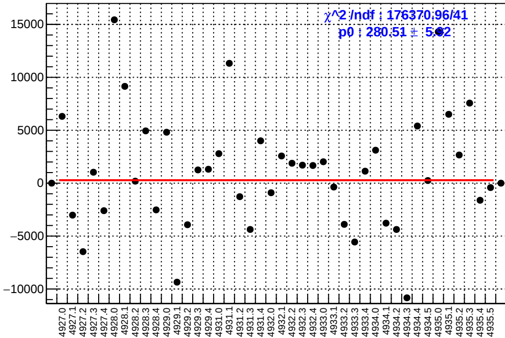
slug93: asym_atl2.mean/ppb-reg_asym_atl2.mean/ppb
