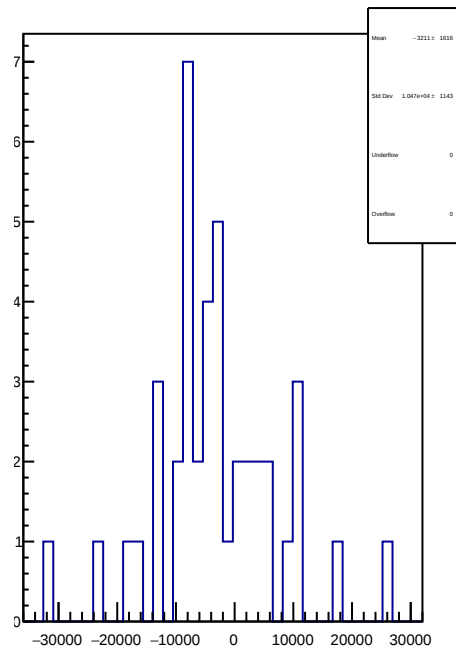
slug93: 1D Corr asym_sam8.mean/ppb-reg_asym_sam8.mean/ppb
