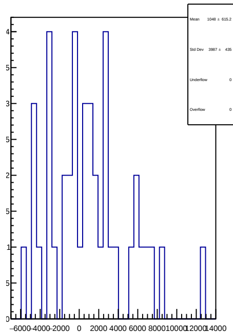
slug93: 1D Corr asym_usl.mean/ppb-reg_asym_usl.mean/ppb
