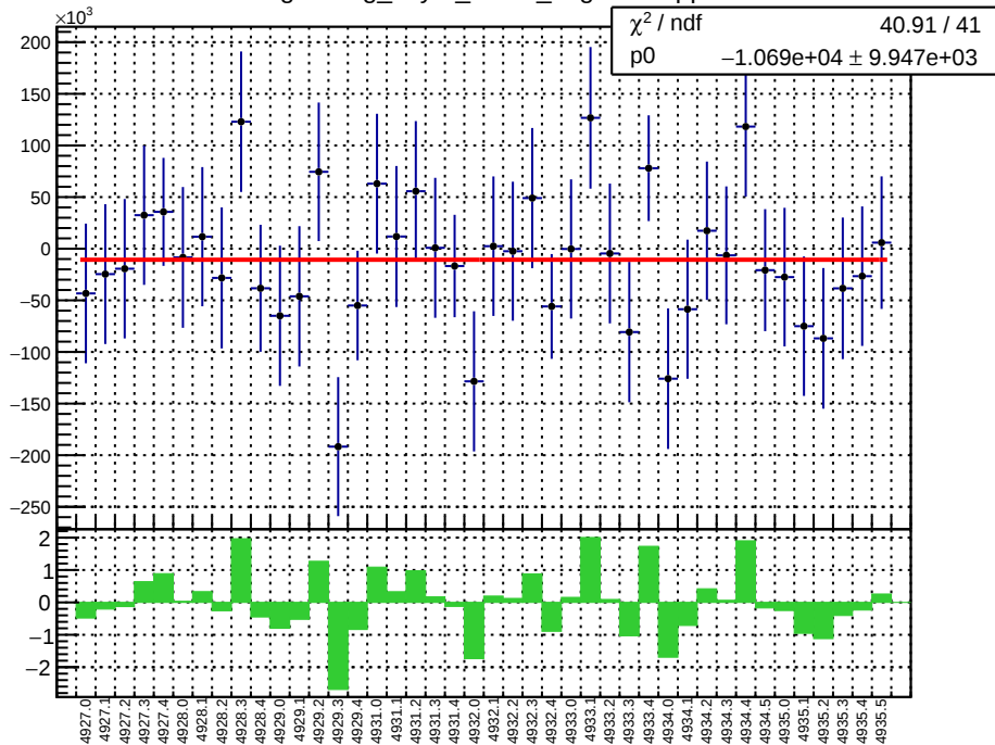
slug93: reg_asym_atr1l2_avg.mean/ppb
