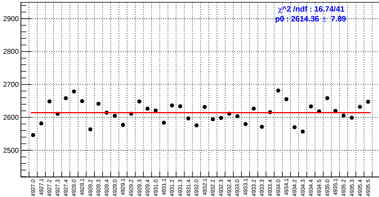
slug93: diff_bpm4aY.rms/nm
