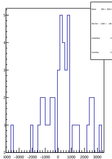
slug93: 1D Corr asym_at1_avg.mean/ppb-reg_asym_at1_avg.mean/ppb
