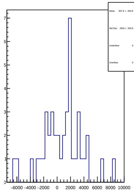
slug93: 1D Corr asym_ds_dd.mean/ppb-reg_asym_ds_dd.mean/ppb
