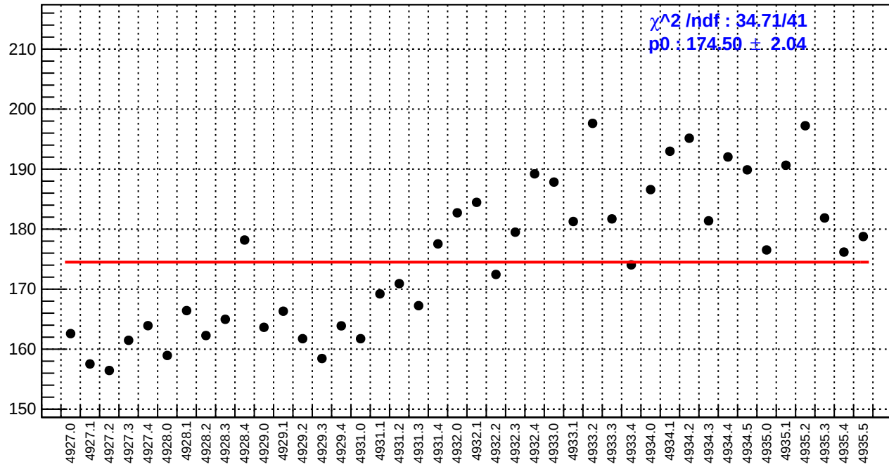
slug93: asym_bcm_an_us.rms/ppm
