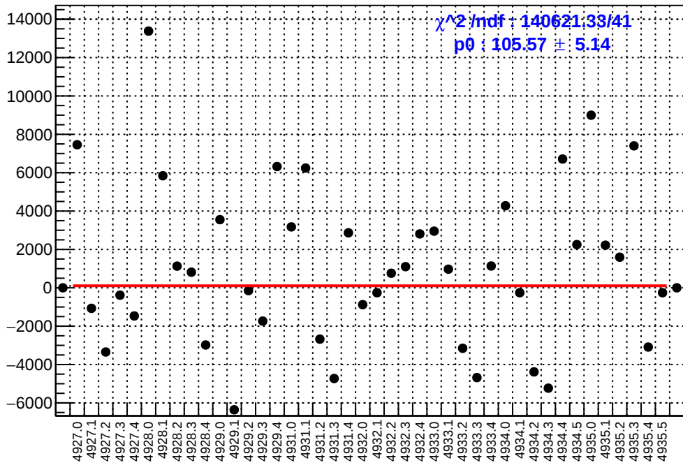
slug93: asym_dsl.mean/ppb-reg_asym_dsl.mean/ppb
