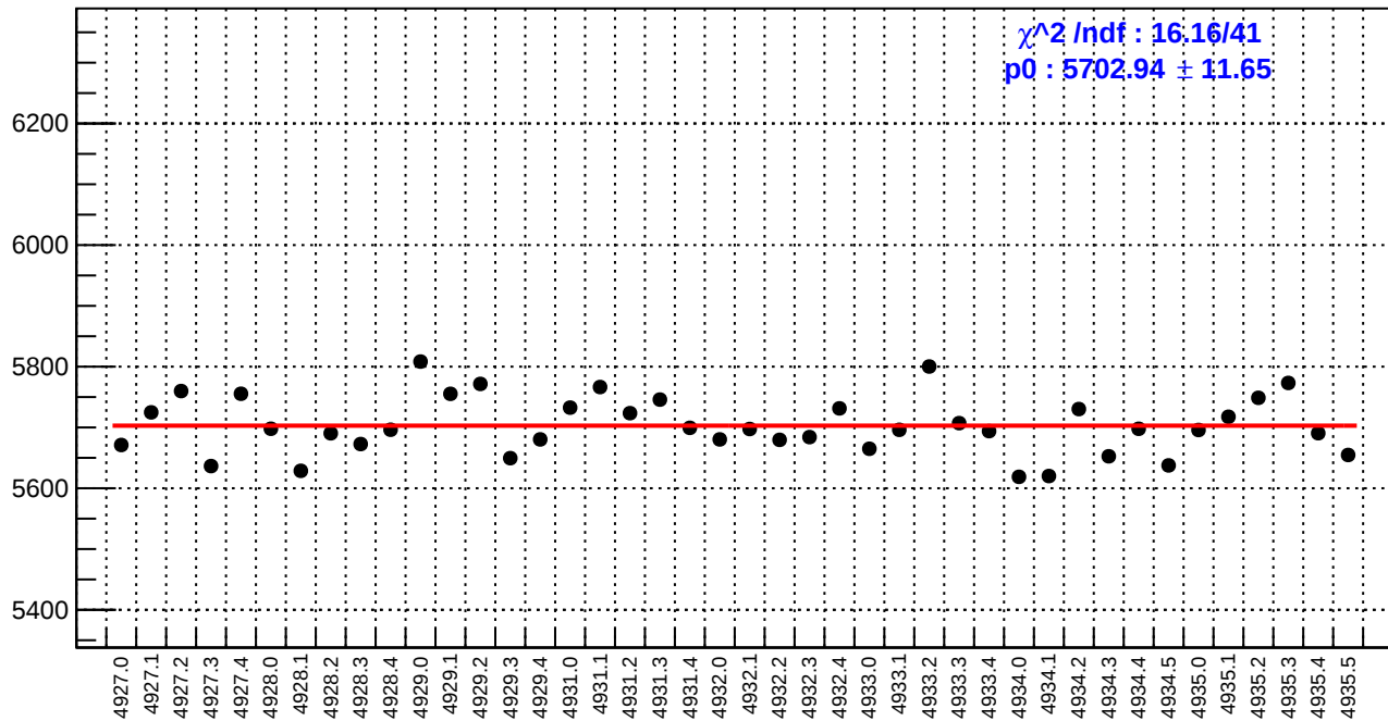
slug93: reg_asym_at1_avg.rms/ppm
