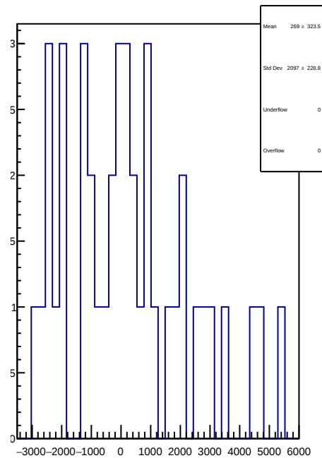
slug93: 1D Corr asym_ds_avg.mean/ppb-reg_asym_ds_avg.mean/ppb
