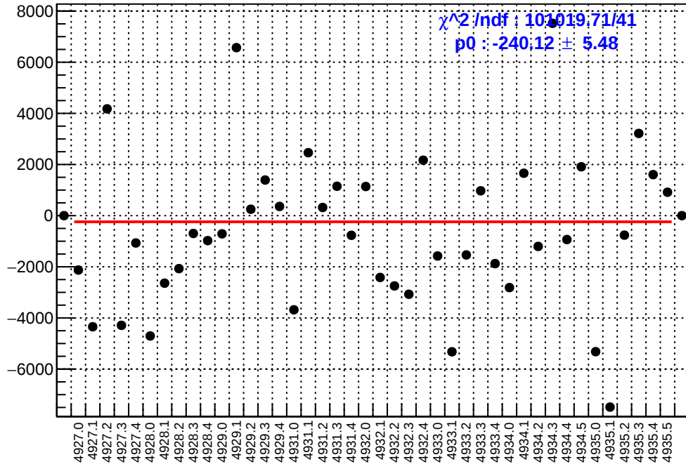
slug93: asym_right_avg.mean/ppb-reg_asym_right_avg.mean/ppb
