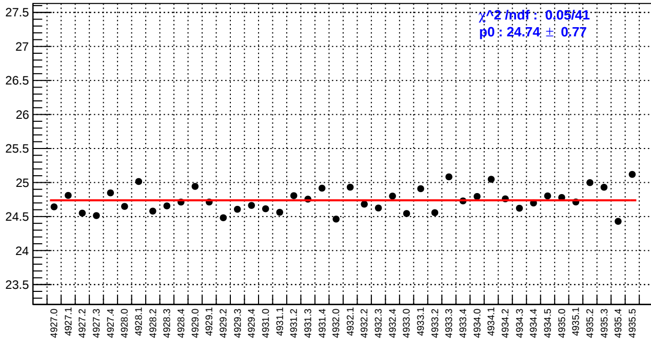
slug93: reg_asym_right_dd.rms/ppm
