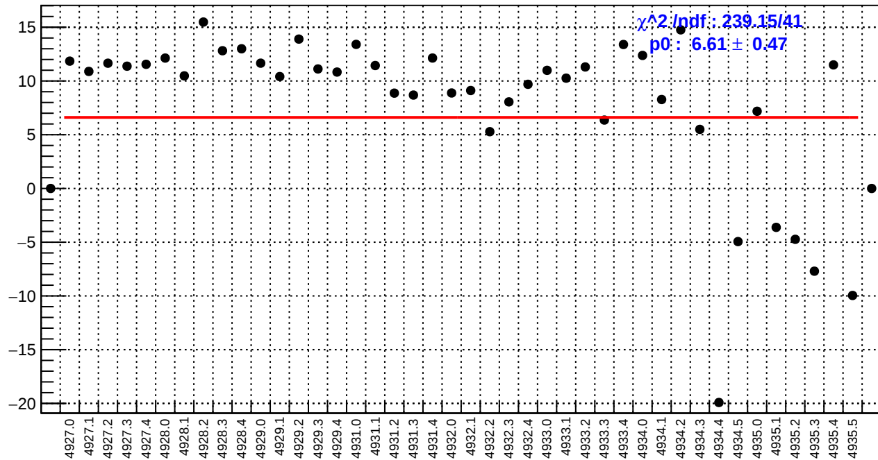
slug93: us_avg_bpm4eY/(ppb/nm)
