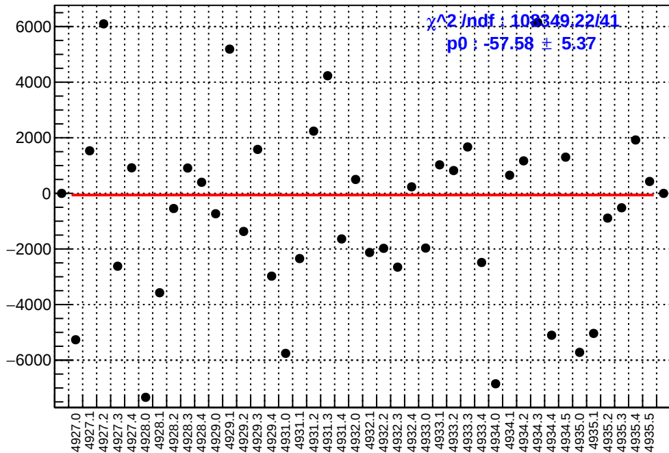
slug93: asym_atr_avg.mean/ppb-reg_asym_atr_avg.mean/ppb
