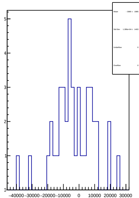
slug93: 1D Corr asym_sam6.mean/ppb-reg_asym_sam6.mean/ppb
