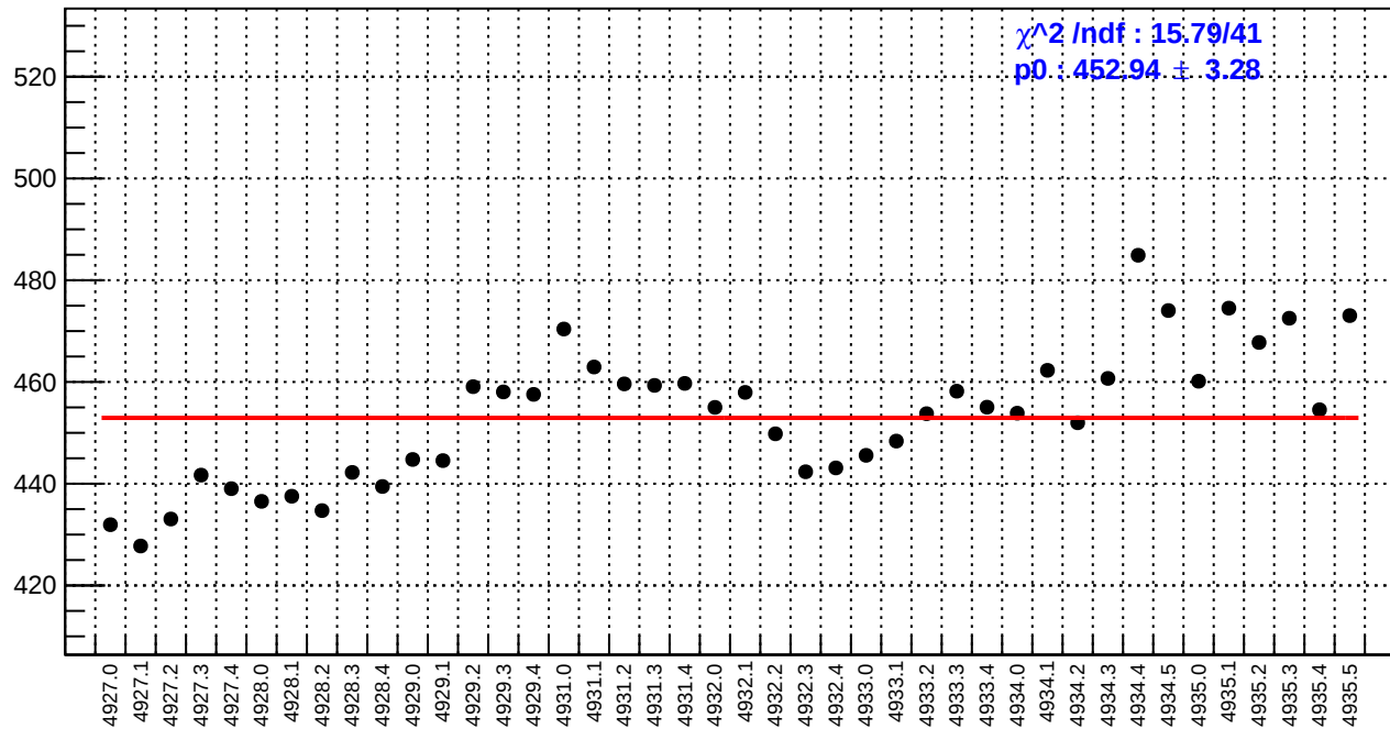
slug93: reg_asym_sam8.rms/ppm
