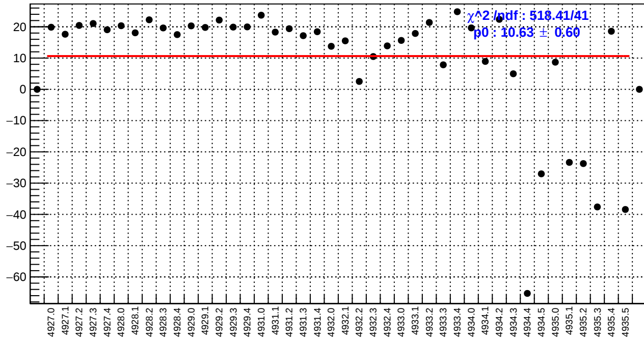
slug93: dsl_bpm4eY/(ppb/nm)
