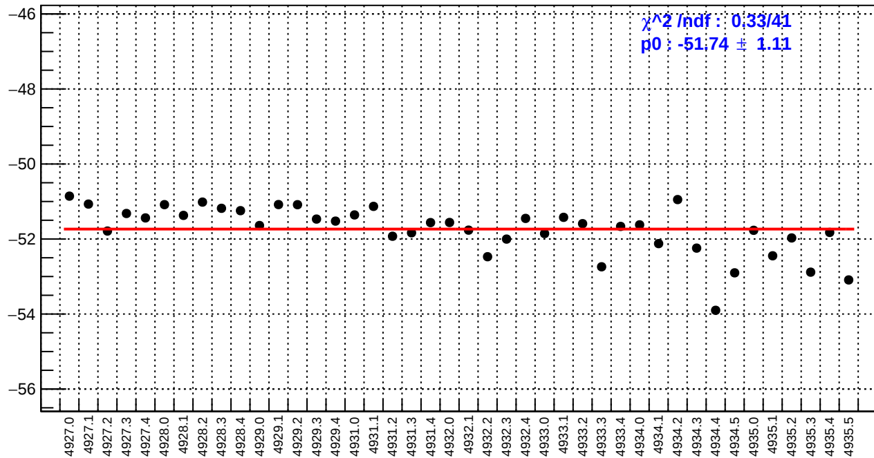
slug93: us_avg_bpm12X/(ppb/nm)
