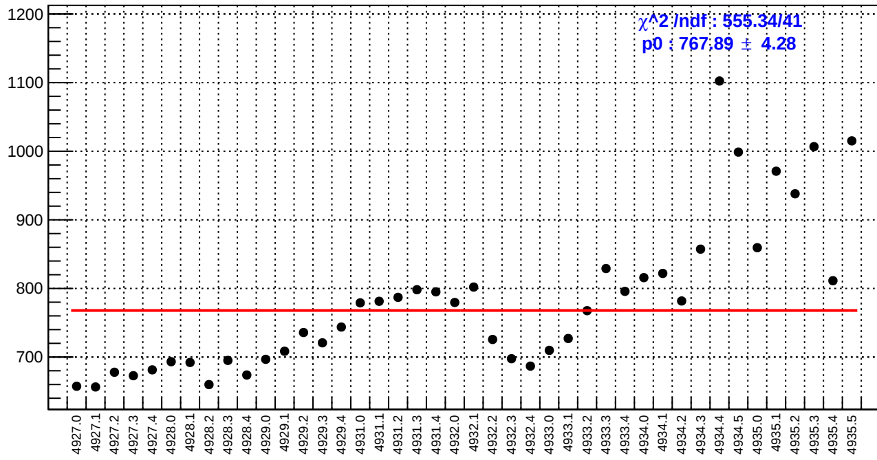
slug93: reg_asym_sam3.rms/ppm
