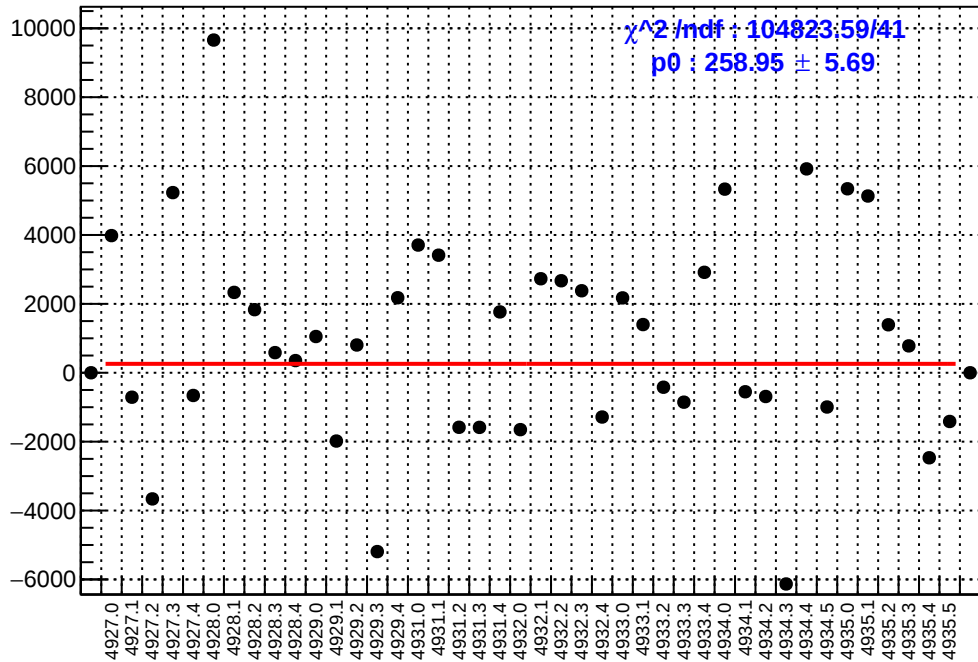
slug93: asym_atl1r2_dd.mean/ppb-reg_asym_atl1r2_dd.mean/ppb
