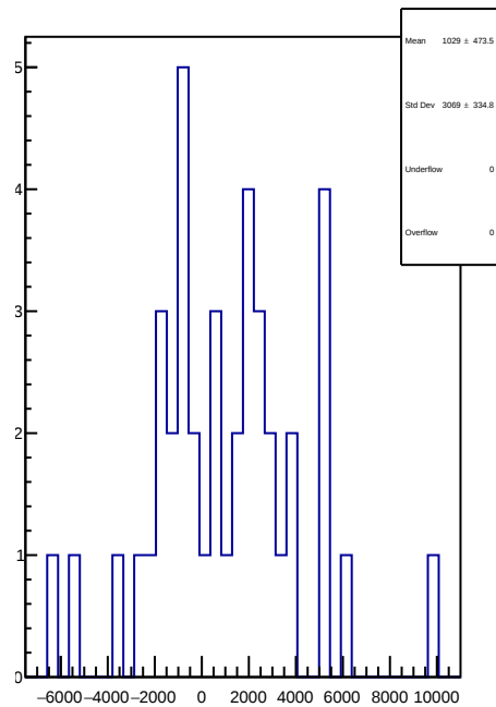
slug93: 1D Corr asym_atl1r2_dd.mean/ppb-reg_asym_atl1r2_dd.mean/ppb
