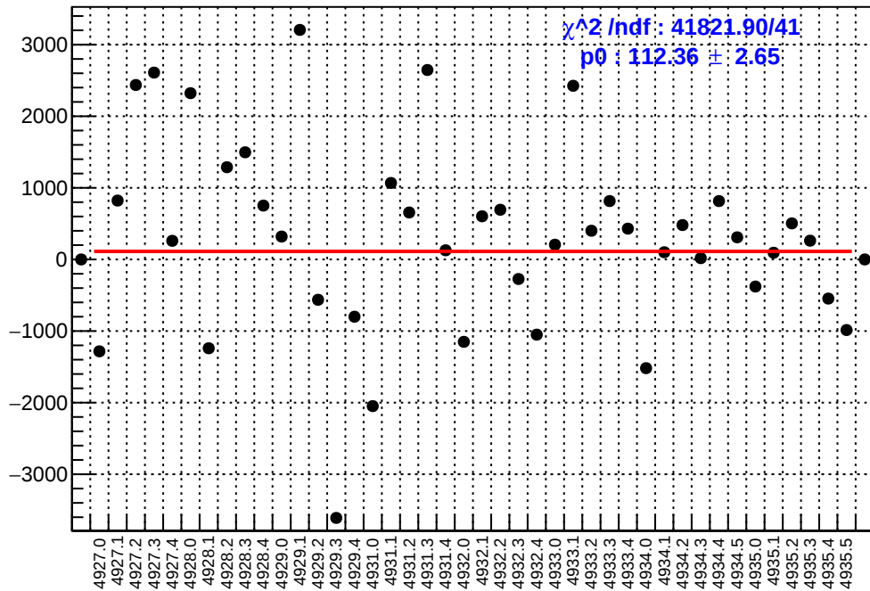
slug93: asym_at1_avg.mean/ppb-reg_asym_at1_avg.mean/ppb
