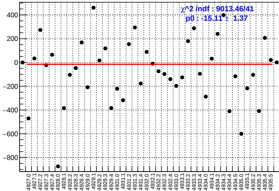
slug93: asym_right_dd.mean/ppb-reg_asym_right_dd.mean/ppb
