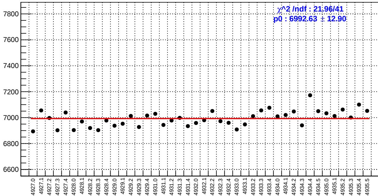
slug93: diff_bpm4eX.rms/nm
