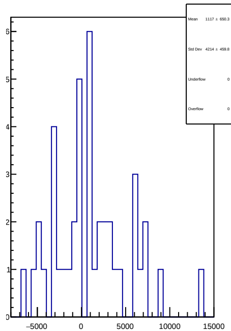
slug93: 1D Corr asym_dsl.mean/ppb-reg_asym_dsl.mean/ppb
