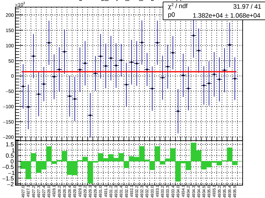
slug93: reg_asym_at2_avg.mean/ppb
