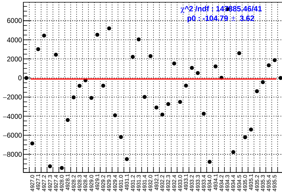
slug93: asym_atr2.mean/ppb-reg_asym_atr2.mean/ppb
