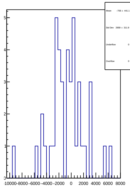
slug93: 1D Corr asym_sam1.mean/ppb-reg_asym_sam1.mean/ppb
