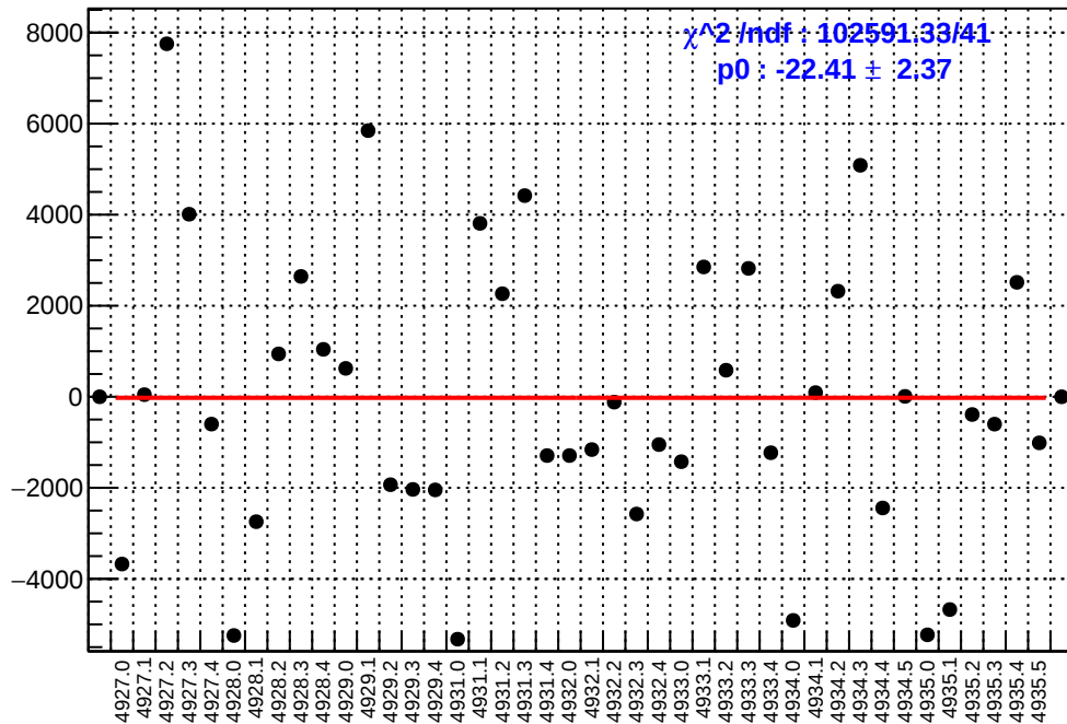
slug93: asym_atr1.mean/ppb-reg_asym_atr1.mean/ppb
