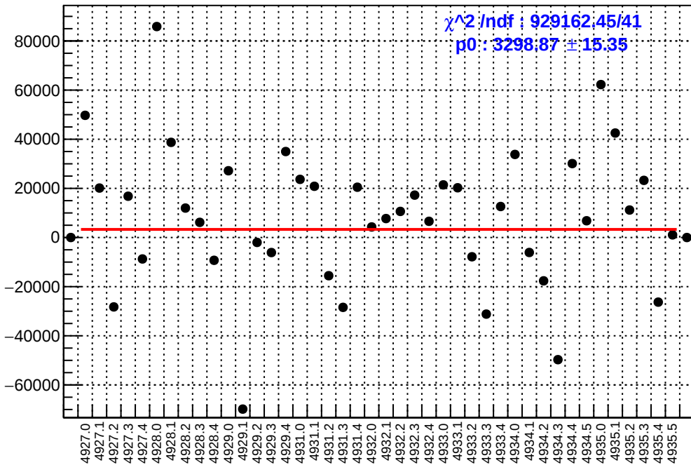
slug93: asym_sam4.mean/ppb-reg_asym_sam4.mean/ppb
