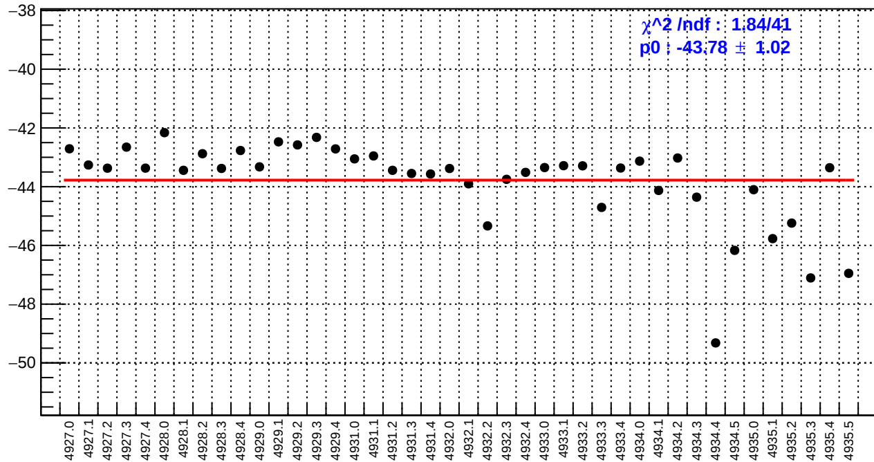
slug93: left_avg_bpm12X/(ppb/nm)
