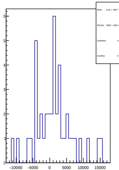
slug93: 1D Corr asym_atl2.mean/ppb-reg_asym_atl2.mean/ppb
