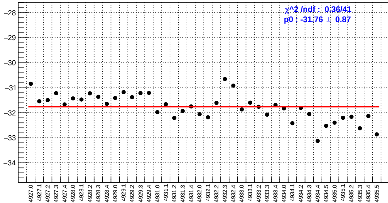
slug93: ds_avg_bpm4eX/(ppb/nm)
