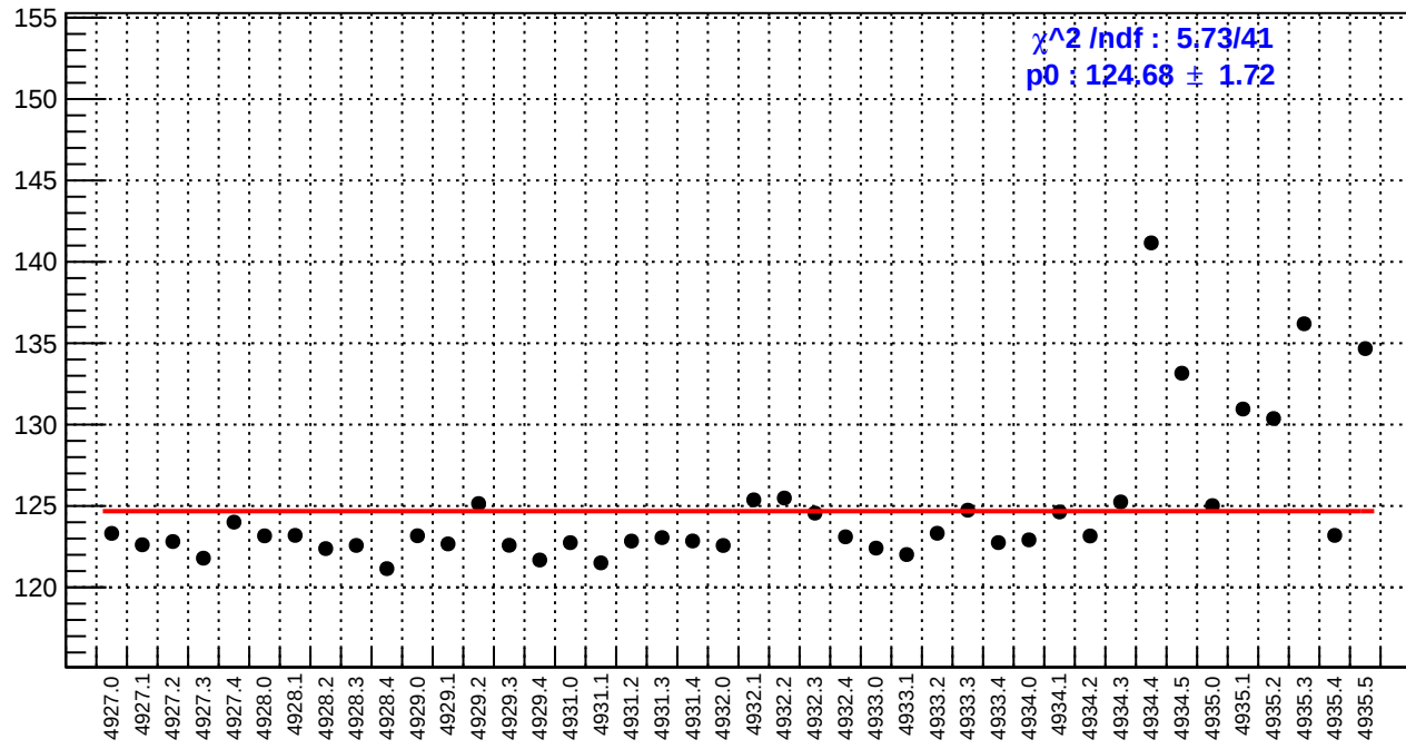
slug93: reg_asym_usl.rms/ppm
