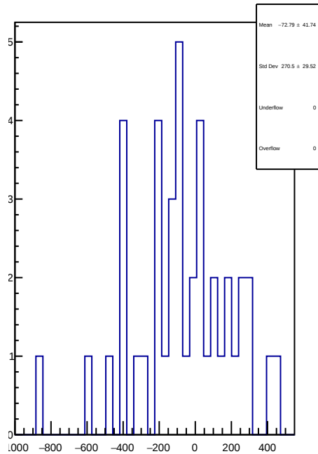
slug93: 1D Corr asym_right_dd.mean/ppb-reg_asym_right_dd.mean/ppb
