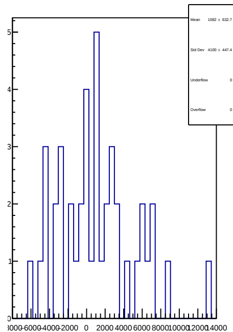
slug93: 1D Corr asym_left_avg.mean/ppb-reg_asym_left_avg.mean/ppb
