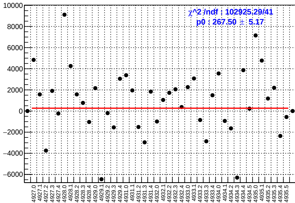
slug93: asym_us_dd.mean/ppb-reg_asym_us_dd.mean/ppb
