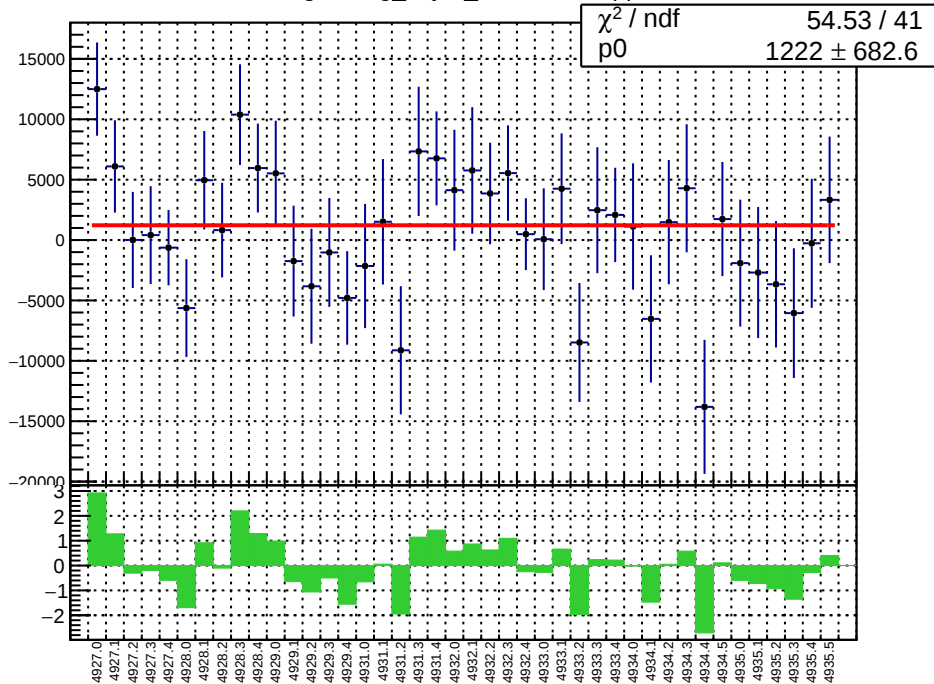
slug93: reg_asym_sam6.mean/ppb
