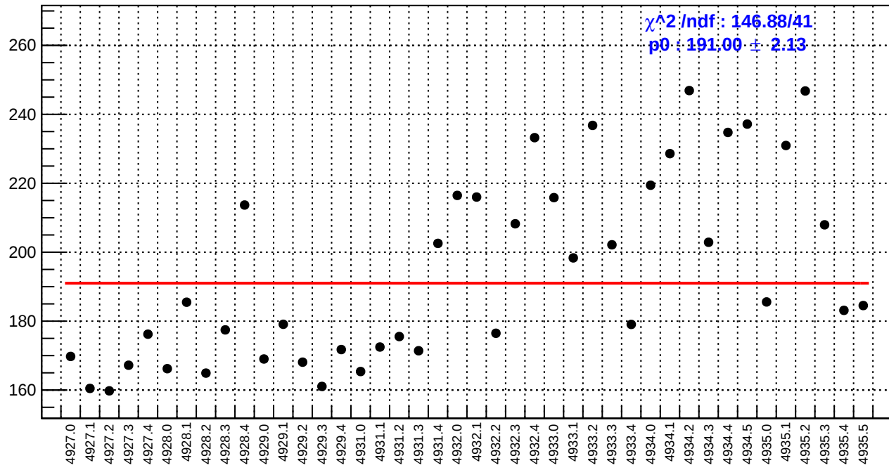
slug93: asym_bcm_an_ds3.rms/ppm
