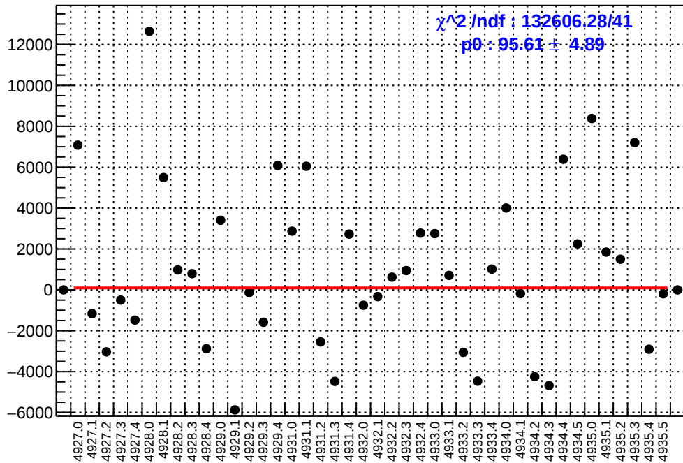
slug93: asym_usl.mean/ppb-reg_asym_usl.mean/ppb
