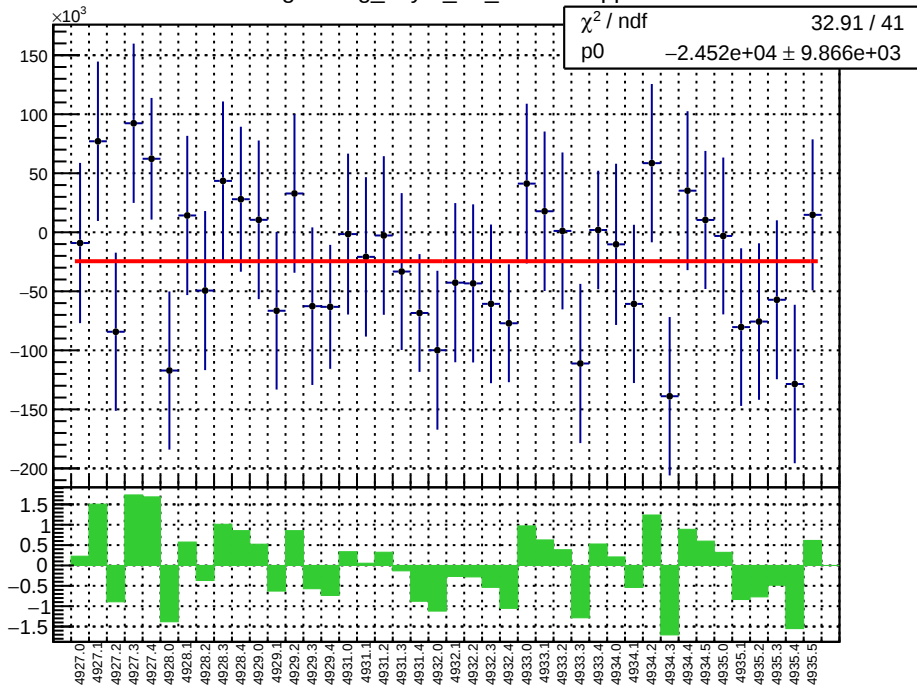
slug93: reg_asym_atr_dd.mean/ppb
