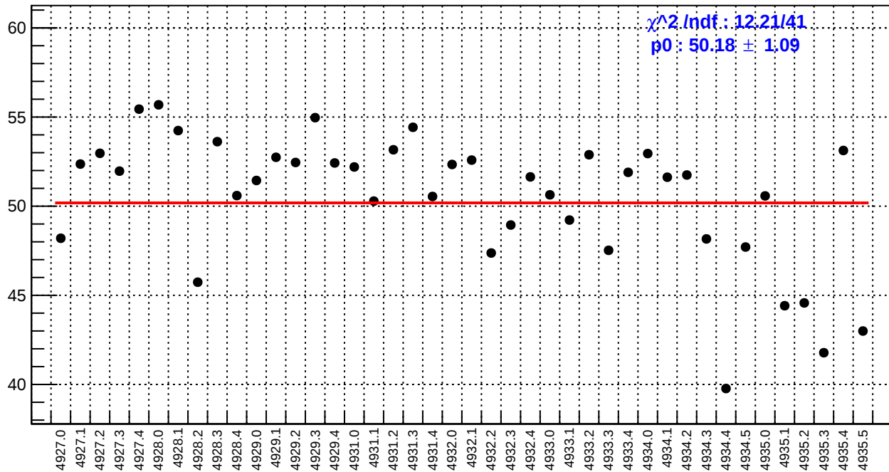
slug93: dsl_bpm4aX/(ppb/nm)
