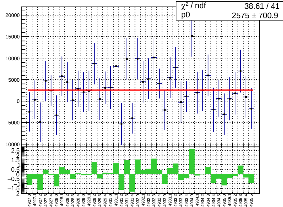
slug93: reg_asym_sam8.mean/ppb
