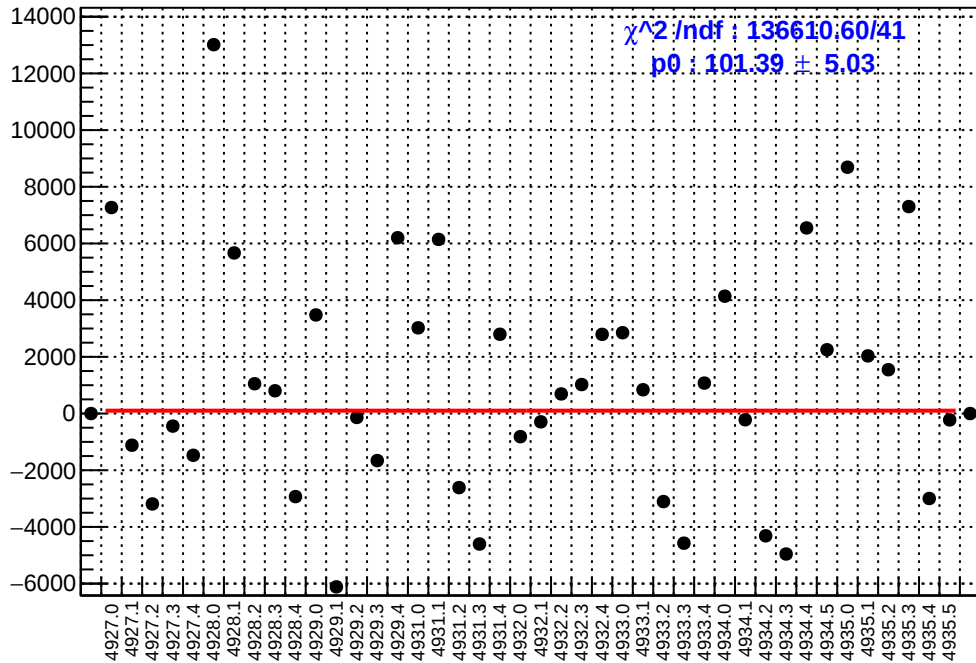
slug93: asym_left_avg.mean/ppb-reg_asym_left_avg.mean/ppb
