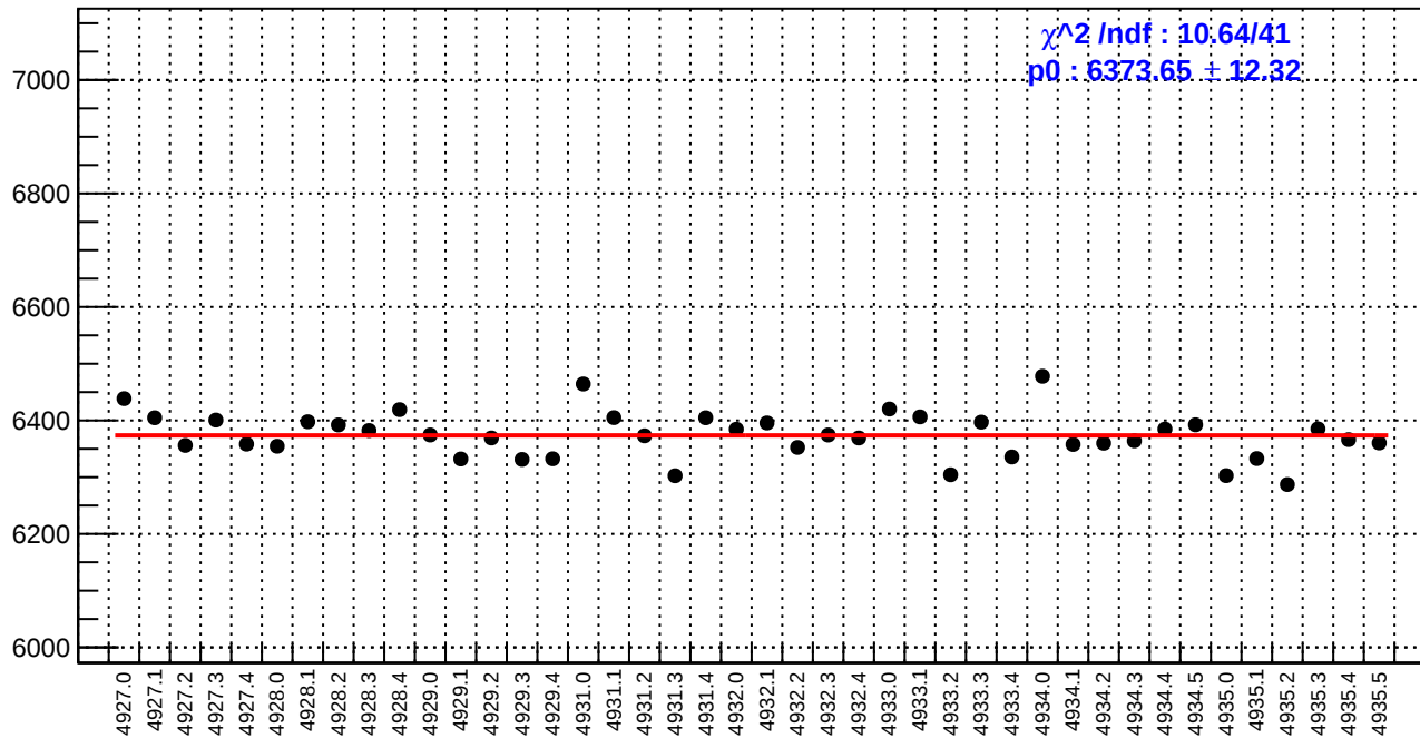
slug93: reg_asym_atr_dd.rms/ppm
