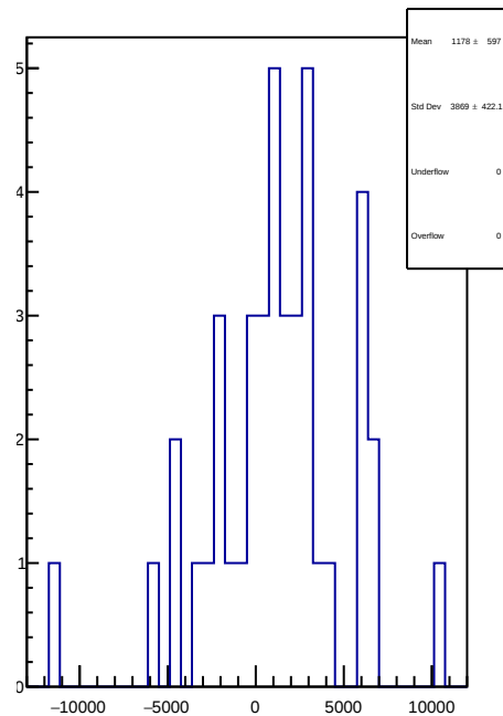
slug93: 1D Corr asym_sam5.mean/ppb-reg_asym_sam5.mean/ppb
