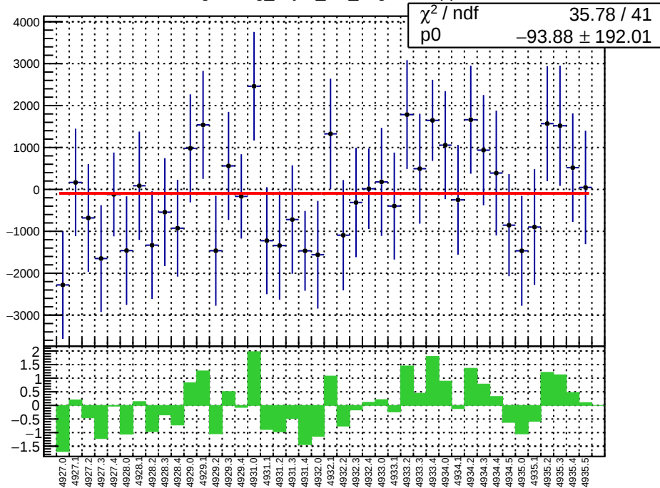
slug93: reg_asym_left_avg.mean/ppb
