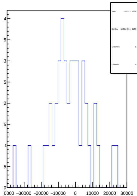
slug93: 1D Corr asym_sam7.mean/ppb-reg_asym_sam7.mean/ppb
