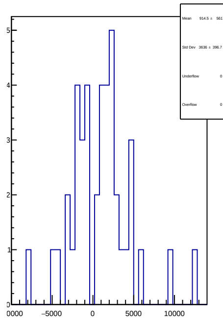
slug93: 1D Corr asym_atl_avg.mean/ppb-reg_asym_atl_avg.mean/ppb
