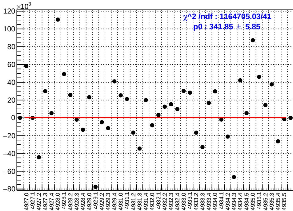
slug93: asym_sam2.mean/ppb-reg_asym_sam2.mean/ppb
