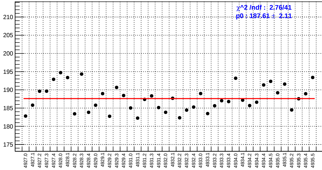
slug93: reg_asym_sam1.rms/ppm
