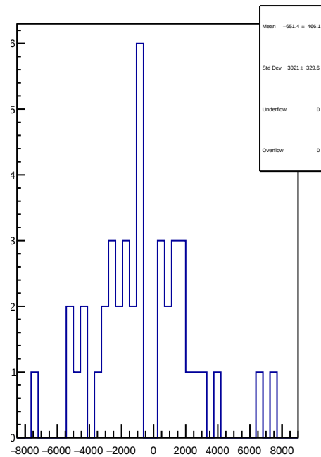
slug93: 1D Corr asym_right_avg.mean/ppb-reg_asym_right_avg.mean/ppb
