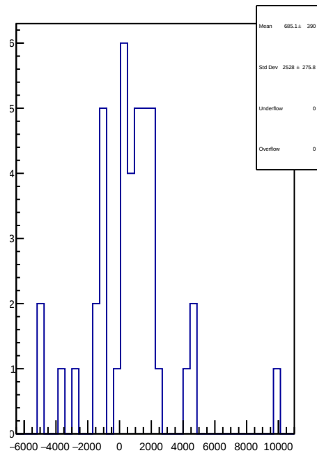
slug93: 1D Corr asym_atl1.mean/ppb-reg_asym_atl1.mean/ppb
