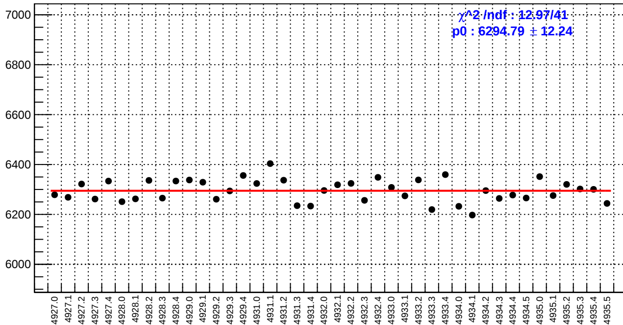
slug93: reg_asym_atl_dd.rms/ppm
