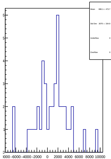
slug93: 1D Corr asym_us_dd.mean/ppb-reg_asym_us_dd.mean/ppb
