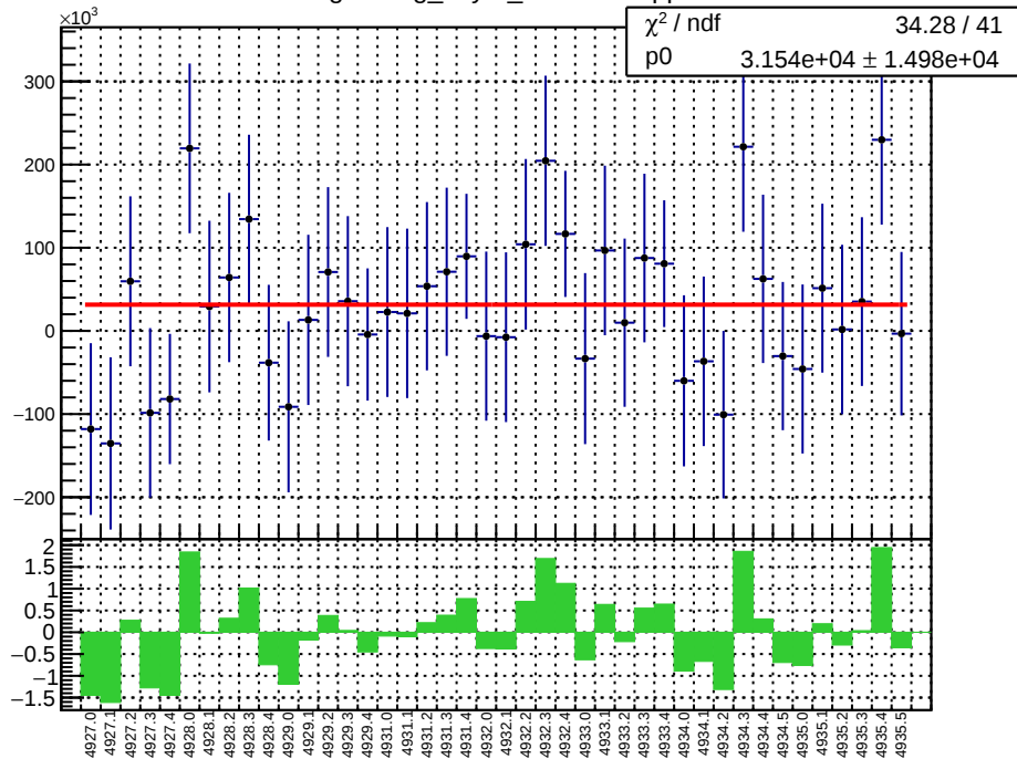
slug93: reg_asym_atr2.mean/ppb
