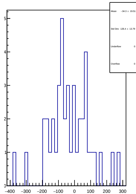
slug93: 1D Corr asym_left_dd.mean/ppb-reg_asym_left_dd.mean/ppb
