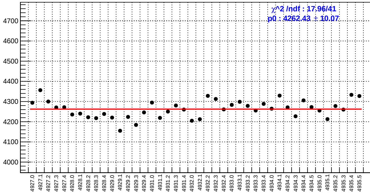
slug93: diff_bpm11X.rms/nm
