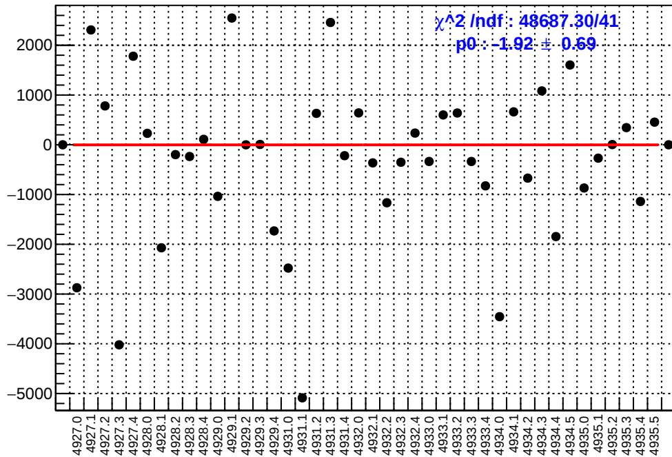
slug93: asym_atl1r2_avg.mean/ppb-reg_asym_atl1r2_avg.mean/ppb
