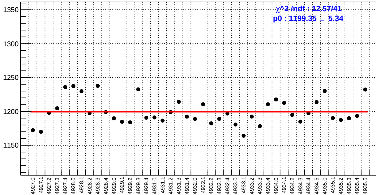
slug93: diff_bpm4aX.rms/nm
