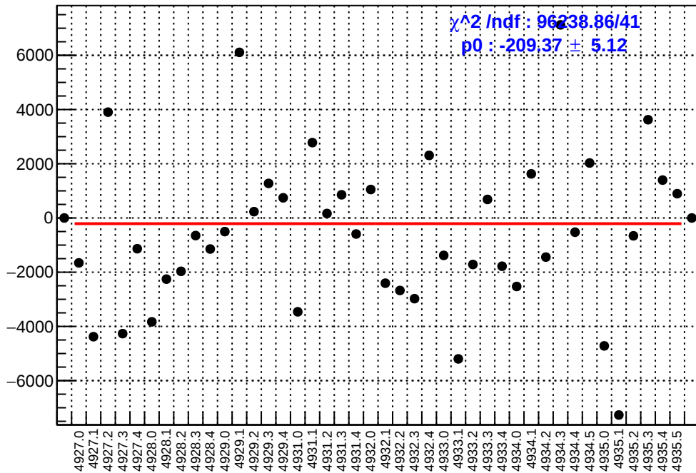
slug93: asym_dsr.mean/ppb-reg_asym_dsr.mean/ppb
