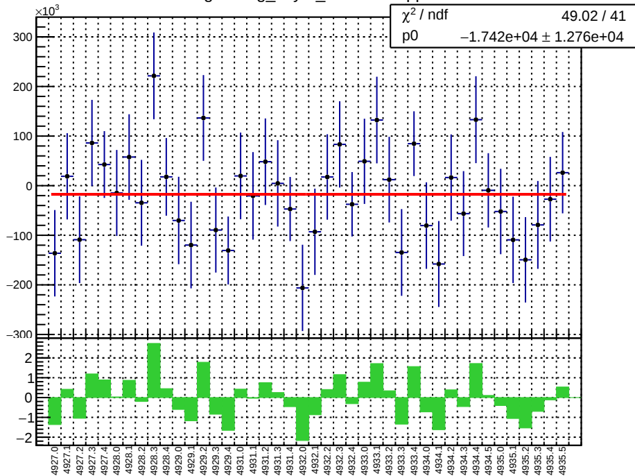
slug93: reg_asym_atr1.mean/ppb
