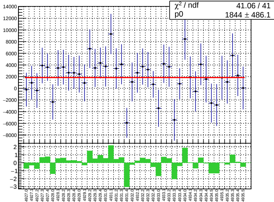
slug93: reg_asym_sam7.mean/ppb
