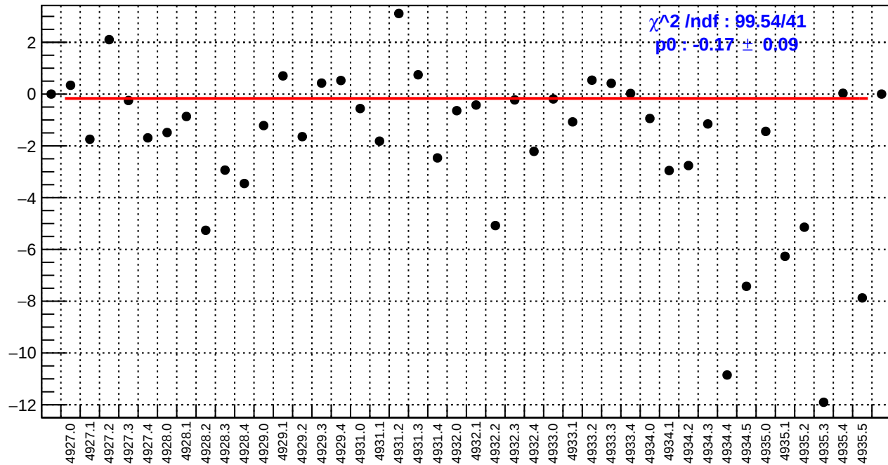
slug93: right_avg_bpm4aY/(ppb/nm)
