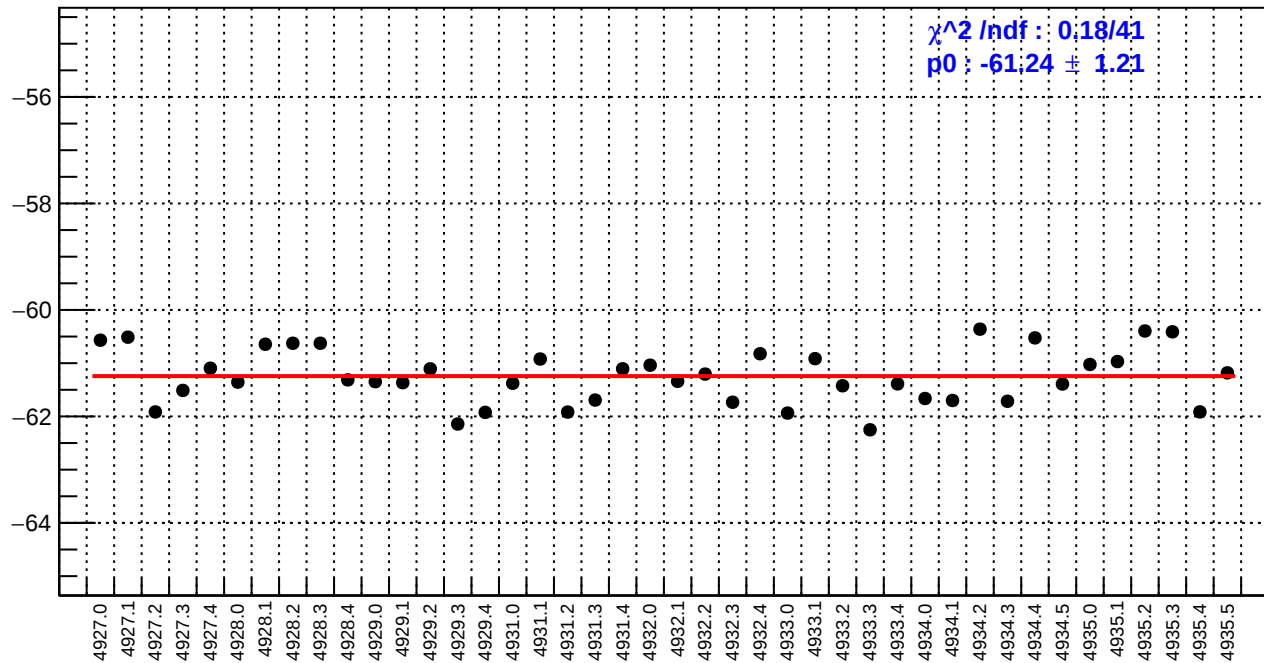
slug93: right_avg_bpm12X/(ppb/nm)
