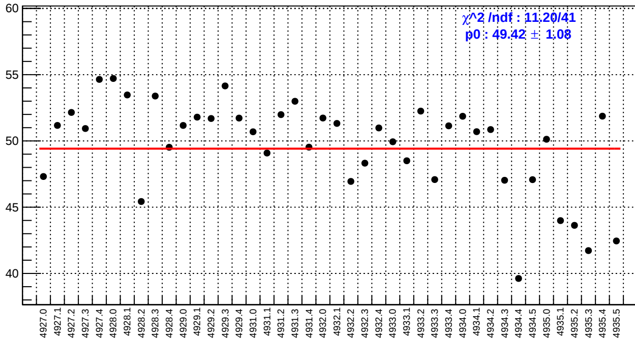
slug93: left_avg_bpm4aX/(ppb/nm)
