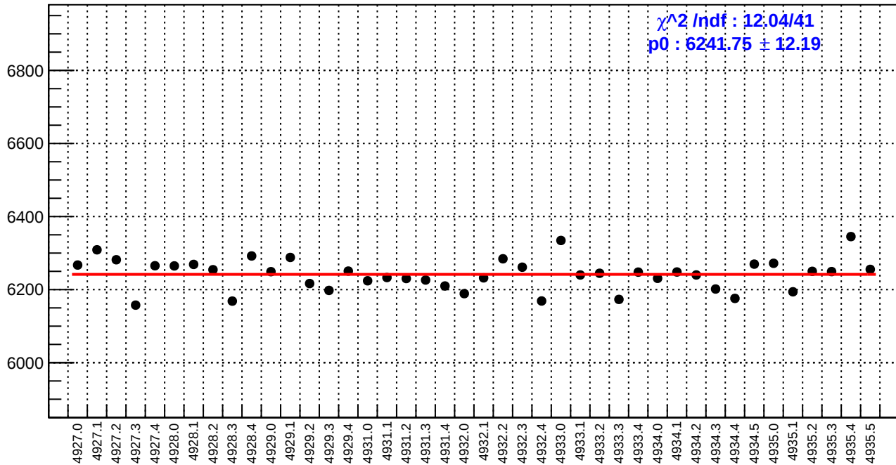
slug93: reg_asym_atl1r2_dd.rms/ppm
