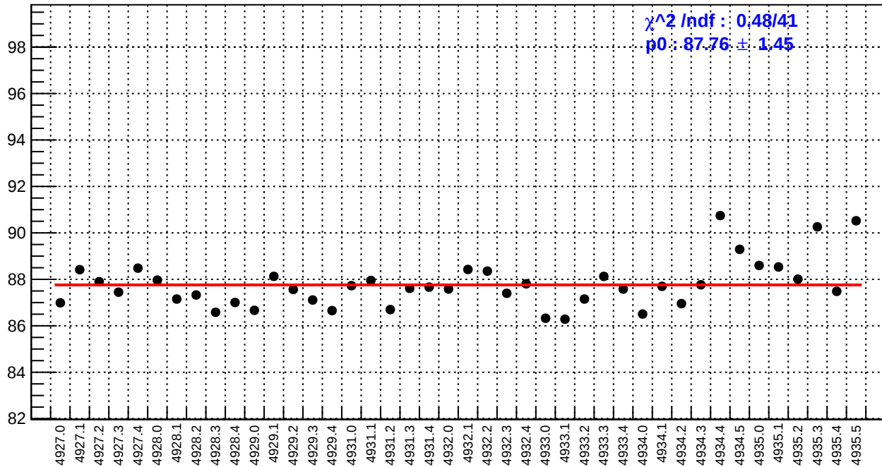
slug93: reg_asym_us_avg.rms/ppm
