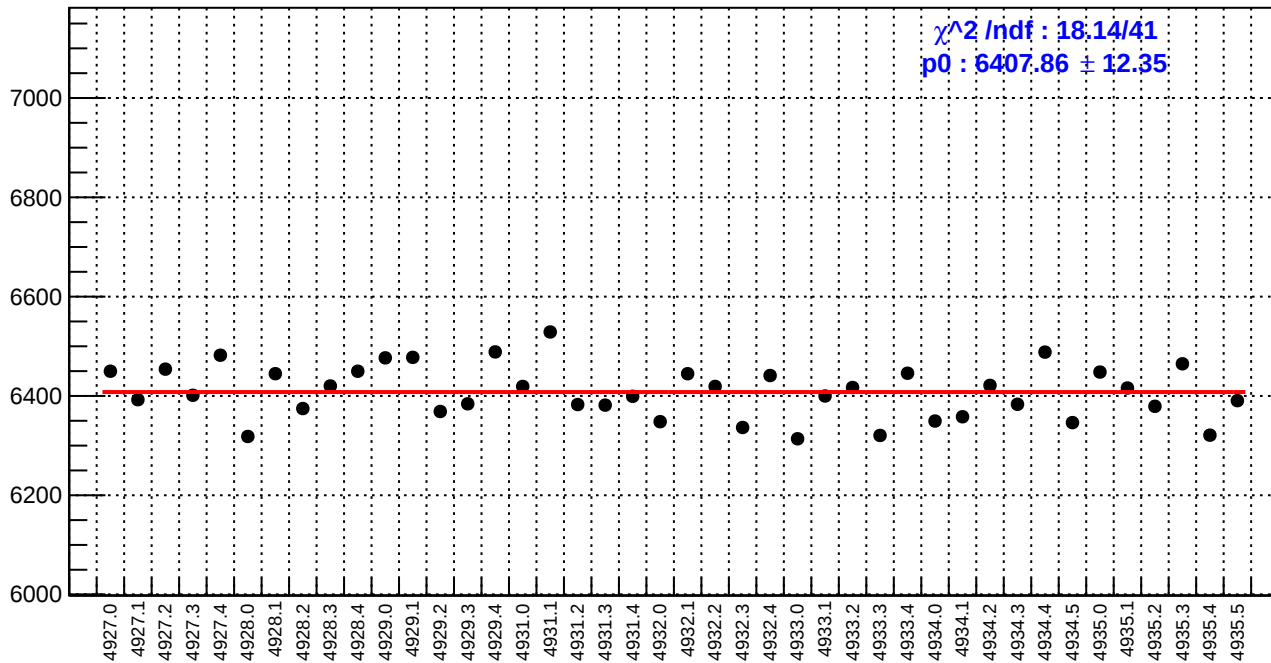
slug93: reg_asym_atr1l2_dd.rms/ppm
