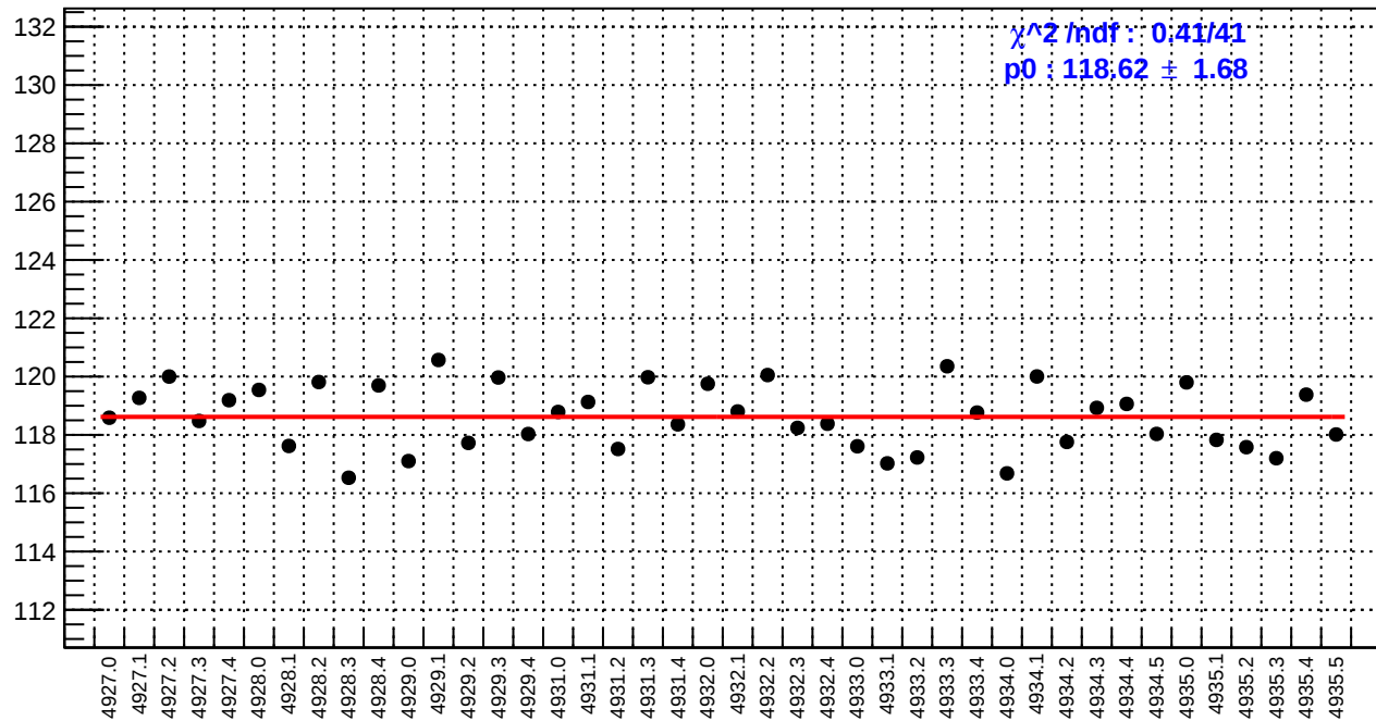
slug93: reg_asym_right_avg.rms/ppm
