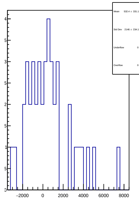
slug93: 1D Corr asym_atr1l2_avg.mean/ppb-reg_asym_atr1l2_avg.mean/ppb
