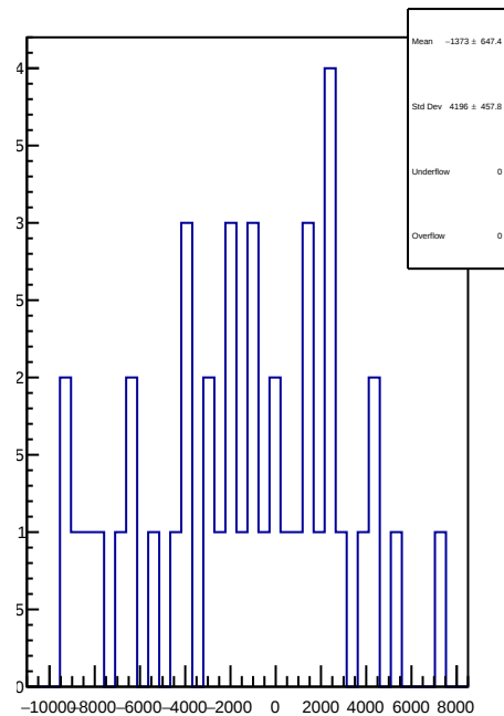
slug93: 1D Corr asym_atr2.mean/ppb-reg_asym_atr2.mean/ppb
