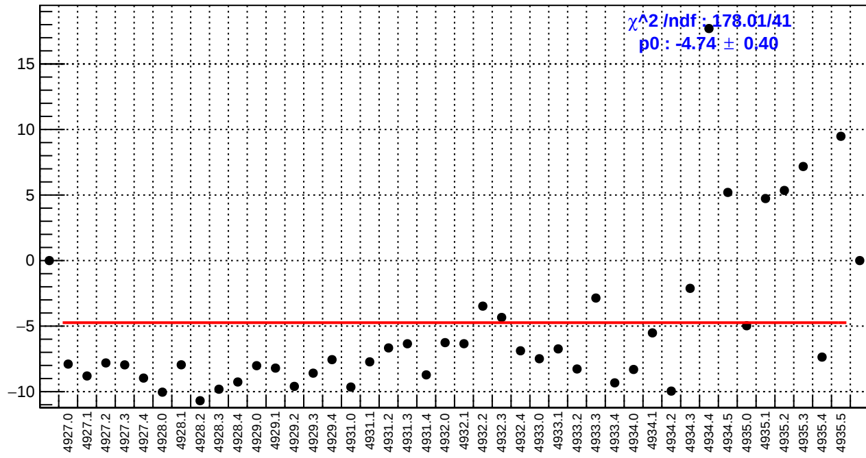
slug93: us_avg_bpm4aY/(ppb/nm)
