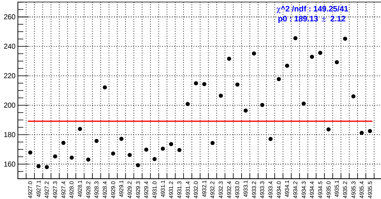
slug93: asym_bcm_an_ds.rms/ppm
