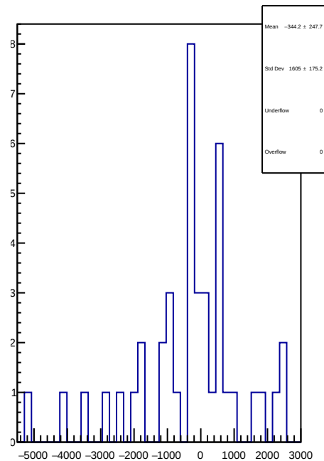
slug93: 1D Corr asym_atl1r2_avg.mean/ppb-reg_asym_atl1r2_avg.mean/ppb
