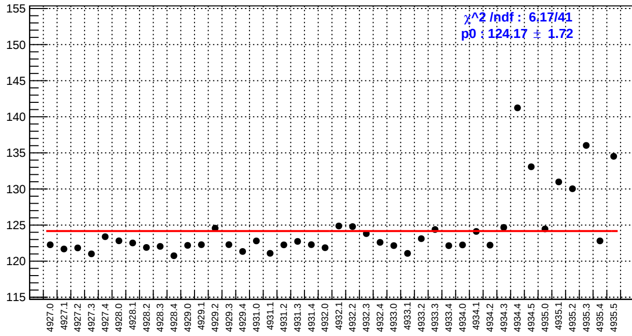
slug93: reg_asym_left_avg.rms/ppm
