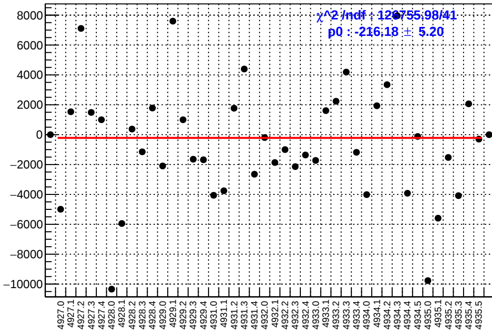
slug93: asym_atr1l2_dd.mean/ppb-reg_asym_atr1l2_dd.mean/ppb
