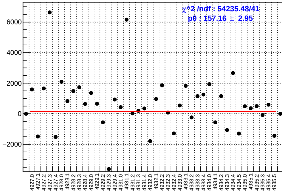
slug93: asym_atr_dd.mean/ppb-reg_asym_atr_dd.mean/ppb
