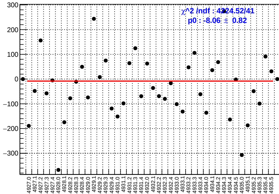
slug93: asym_left_dd.mean/ppb-reg_asym_left_dd.mean/ppb
