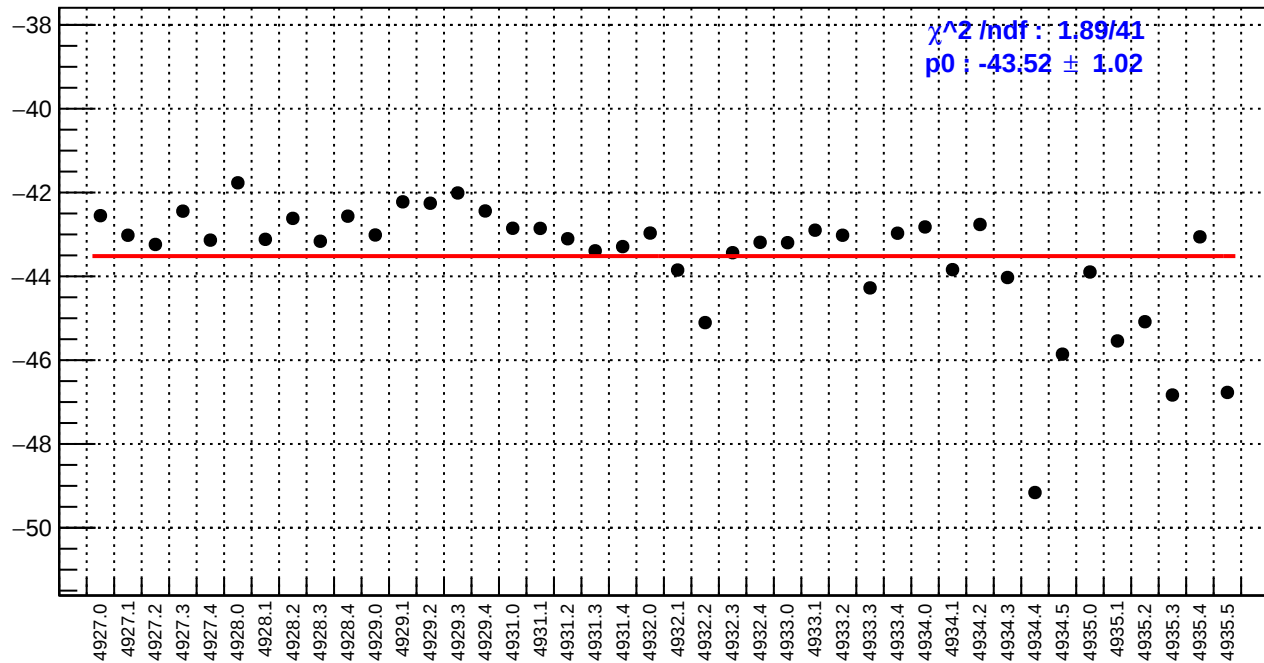
slug93: dsl_bpm12X/(ppb/nm)
