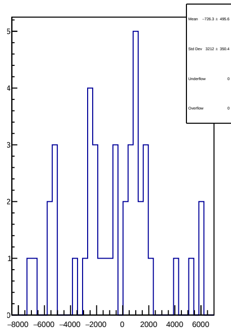
slug93: 1D Corr asym_atr_avg.mean/ppb-reg_asym_atr_avg.mean/ppb
