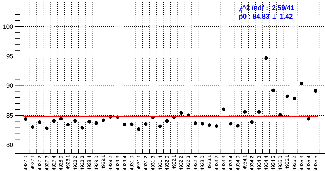
slug93: reg_asym_us_dd.rms/ppm
