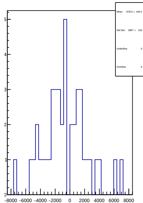
slug93: 1D Corr asym_dsr.mean/ppb-reg_asym_dsr.mean/ppb
