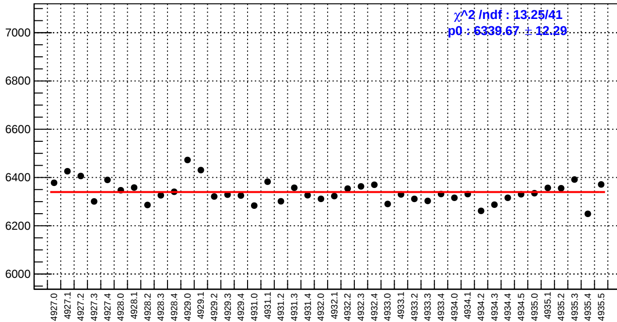
slug93: reg_asym_atr_avg.rms/ppm
