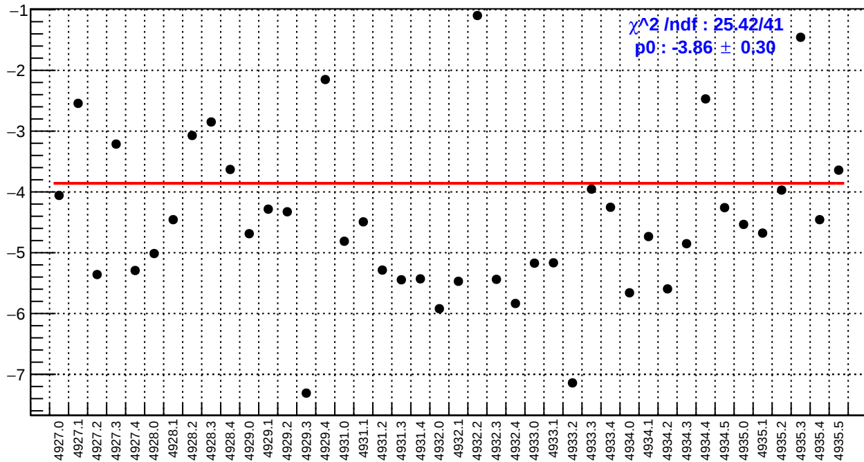
slug93: right_avg_bpm4aX/(ppb/nm)
