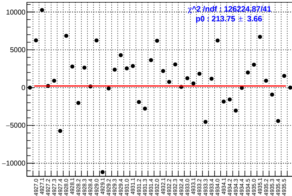
slug93: asym_sam5.mean/ppb-reg_asym_sam5.mean/ppb
