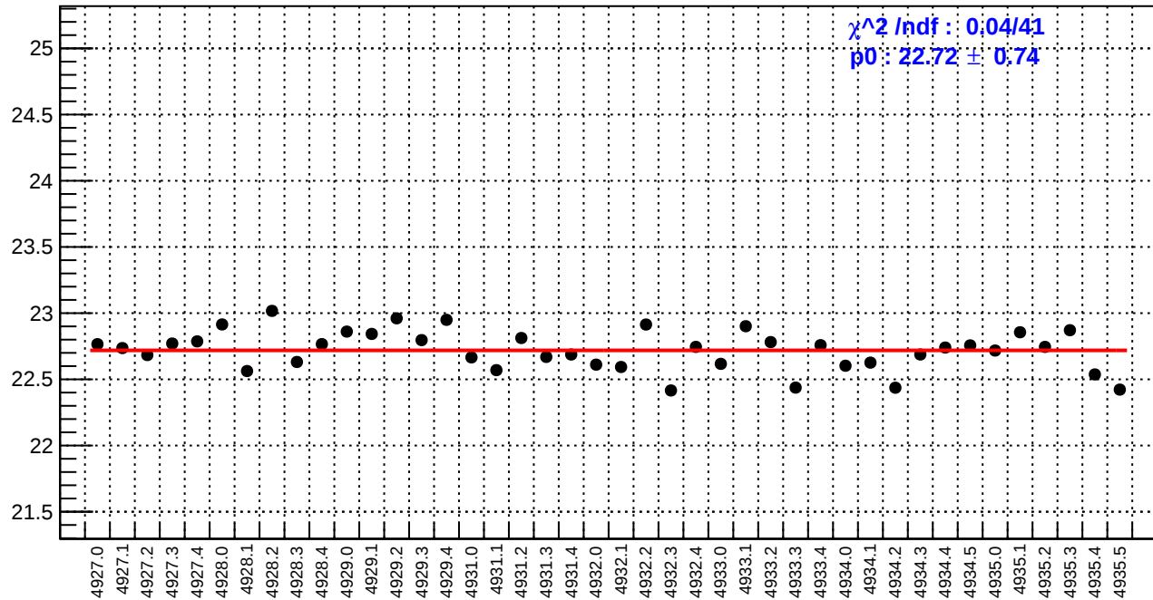
slug93: reg_asym_left_dd.rms/ppm
