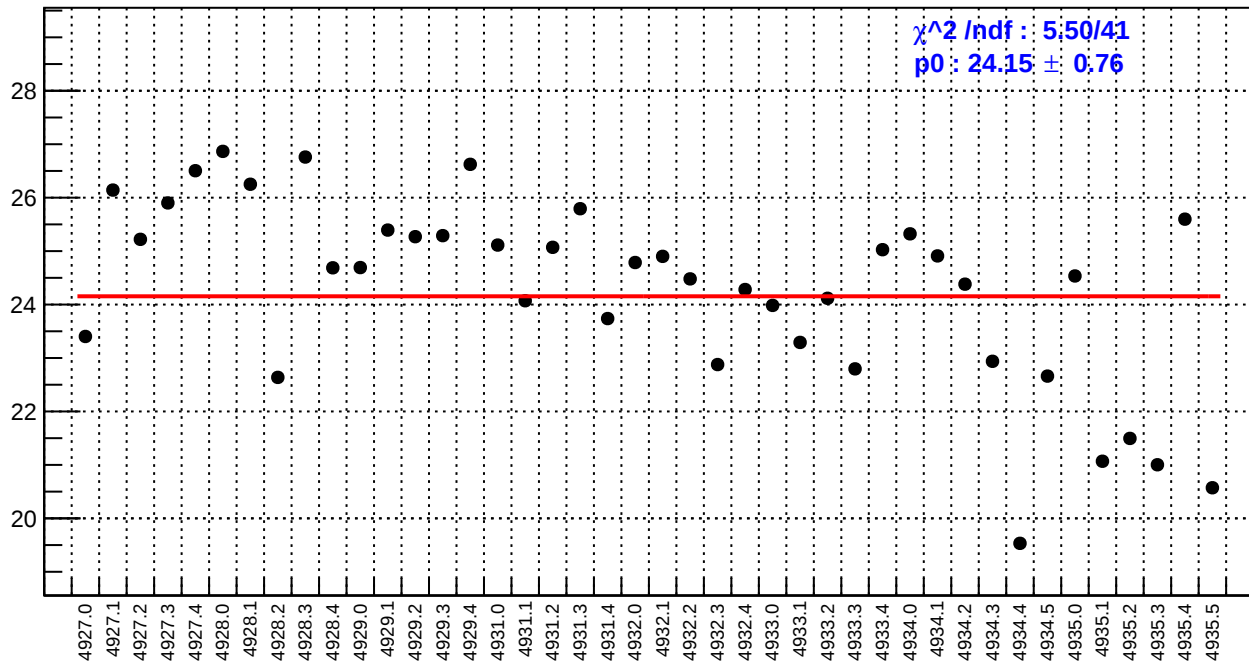
slug93: ds_avg_bpm4aX/(ppb/nm)
