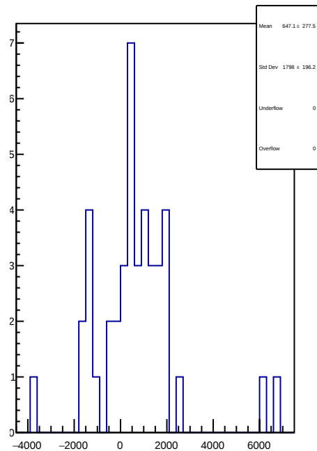
slug93: 1D Corr asym_atr_dd.mean/ppb-reg_asym_atr_dd.mean/ppb
