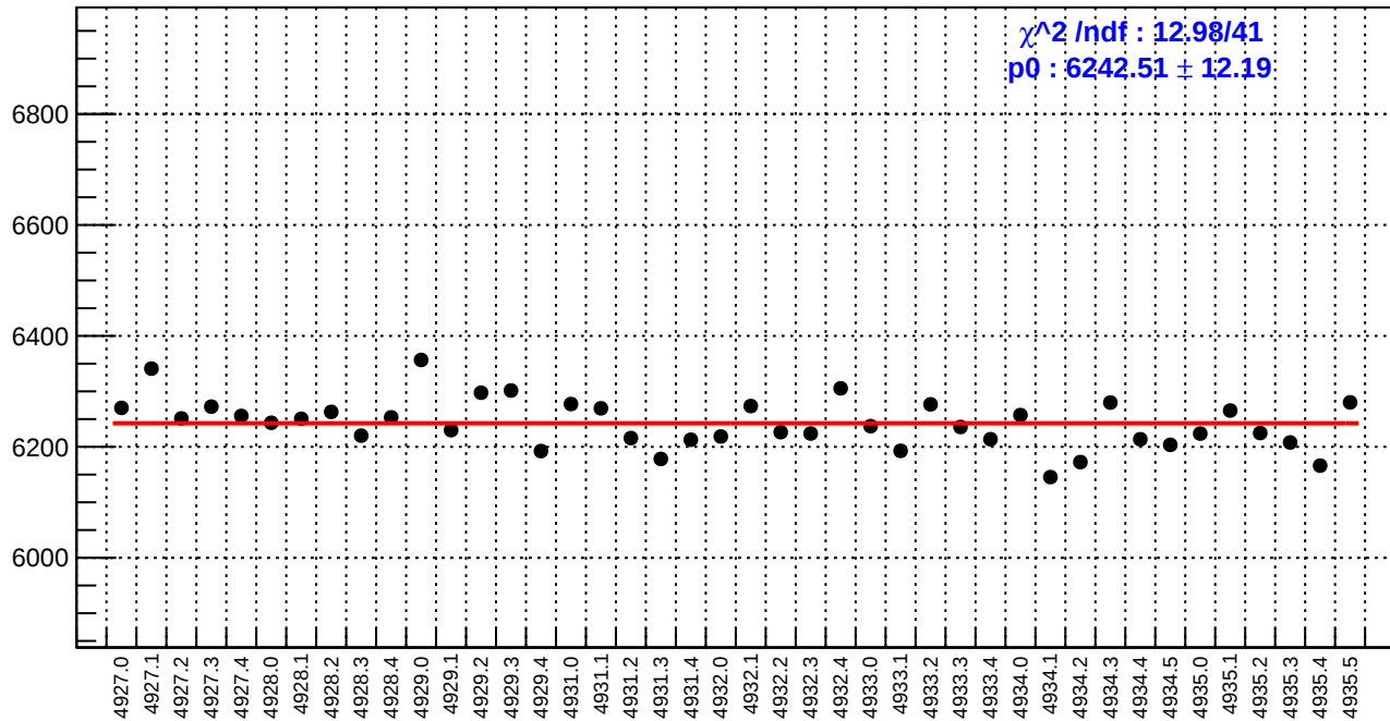
slug93: reg_asym_atl1r2_avg.rms/ppm
