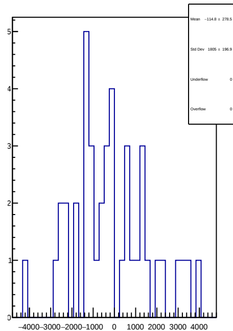
slug93: 1D Corr asym_at2_avg.mean/ppb-reg_asym_at2_avg.mean/ppb
