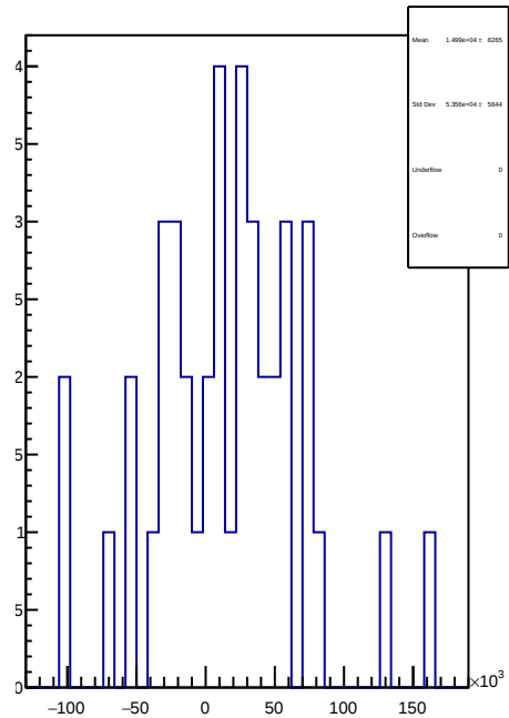
slug93: 1D Corr asym_sam3.mean/ppb-reg_asym_sam3.mean/ppb
