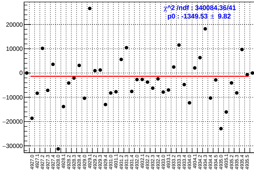
slug93: asym_sam8.mean/ppb-reg_asym_sam8.mean/ppb
