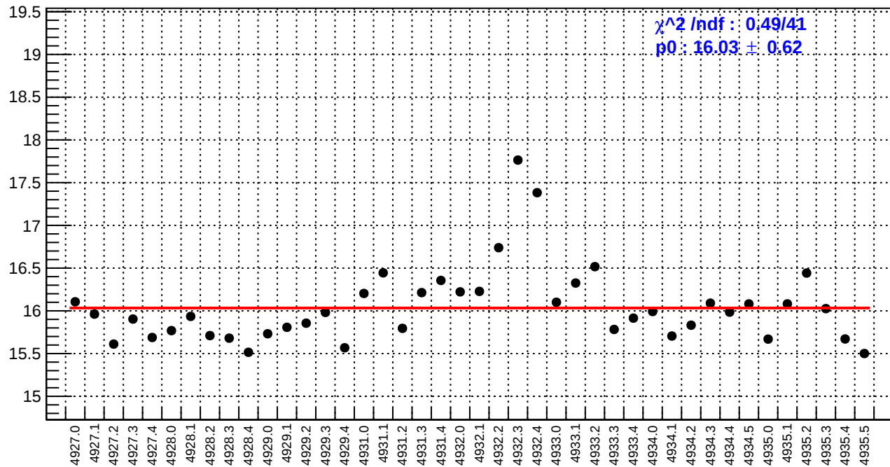
slug93: right_avg_bpm4eX/(ppb/nm)
