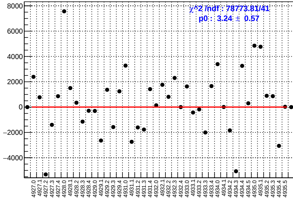
slug93: asym_at1_dd.mean/ppb-reg_asym_at1_dd.mean/ppb
