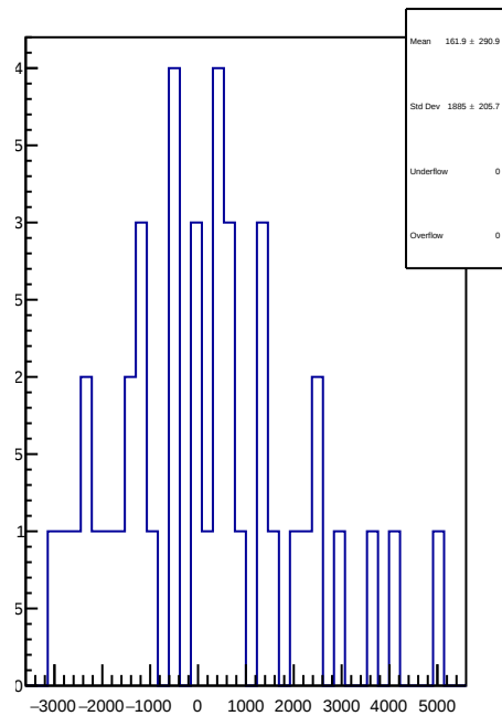
slug93: 1D Corr asym_us_avg.mean/ppb-reg_asym_us_avg.mean/ppb
