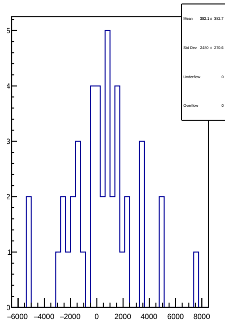
slug93: 1D Corr asym_at1_dd.mean/ppb-reg_asym_at1_dd.mean/ppb
