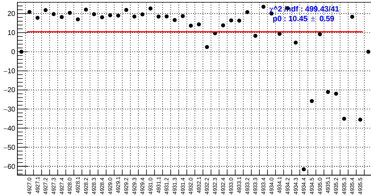
slug93: usl_bpm4eY/(ppb/nm)
