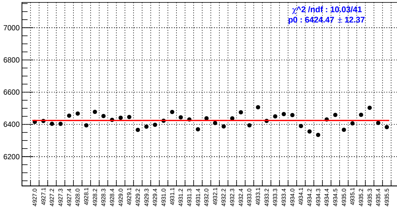
slug93: reg_asym_atr1l2_avg.rms/ppm
