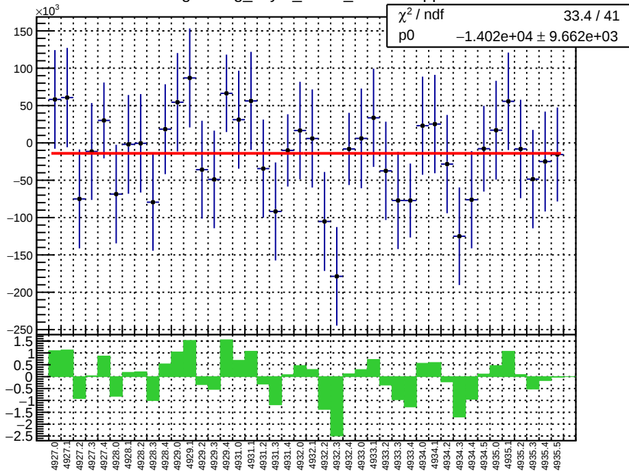
slug93: reg_asym_atl1r2_dd.mean/ppb
