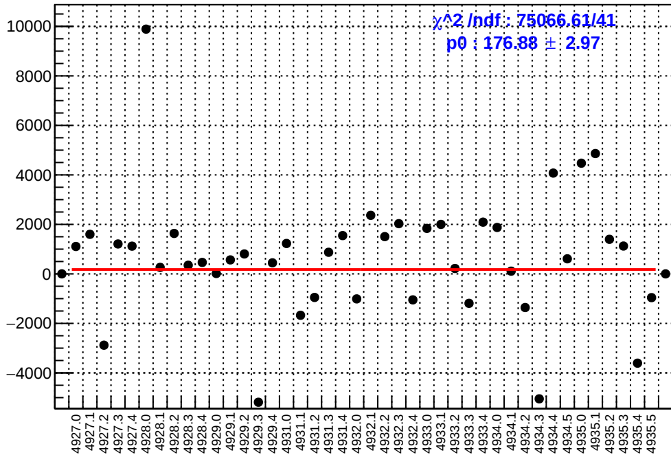
slug93: asym_atl1.mean/ppb-reg_asym_atl1.mean/ppb
