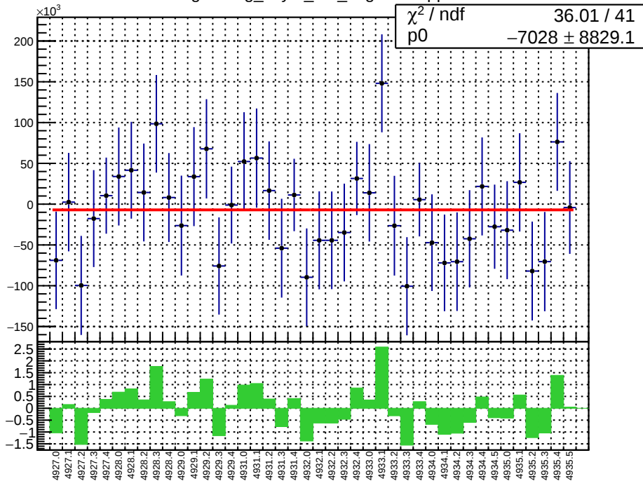
slug93: reg_asym_at1_avg.mean/ppb
