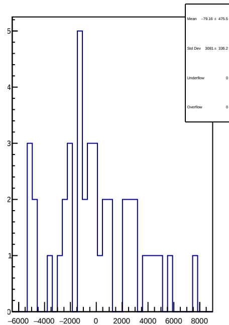
slug93: 1D Corr asym_atr1.mean/ppb-reg_asym_atr1.mean/ppb
