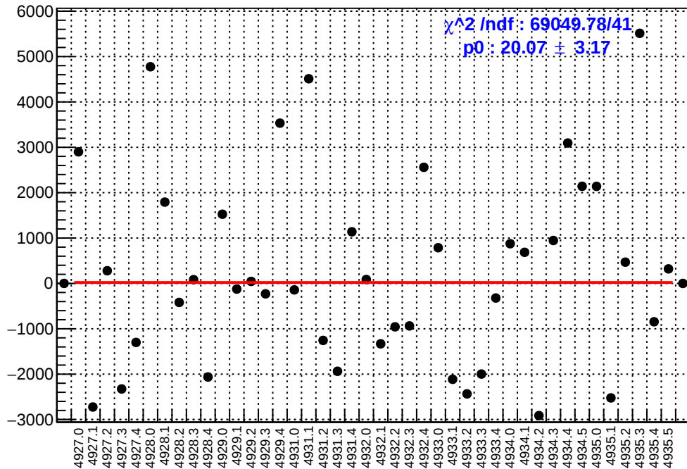
slug93: asym_ds_avg.mean/ppb-reg_asym_ds_avg.mean/ppb
