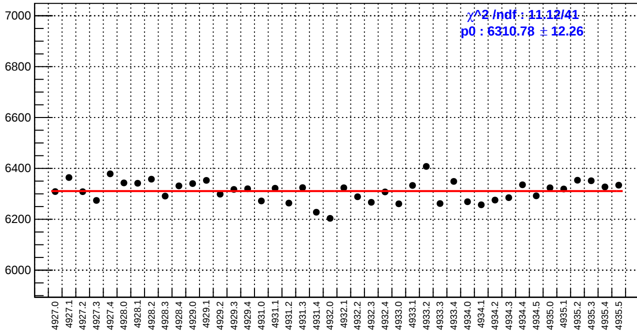
slug93: reg_asym_atl_avg.rms/ppm
