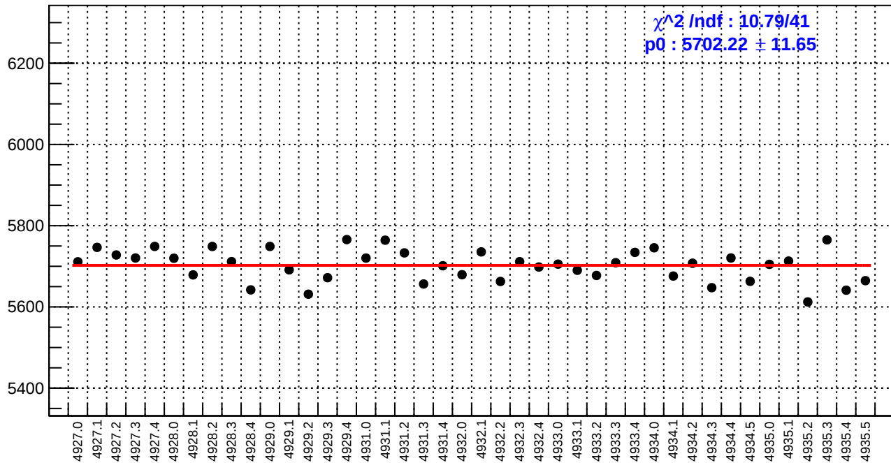
slug93: reg_asym_at1_dd.rms/ppm
