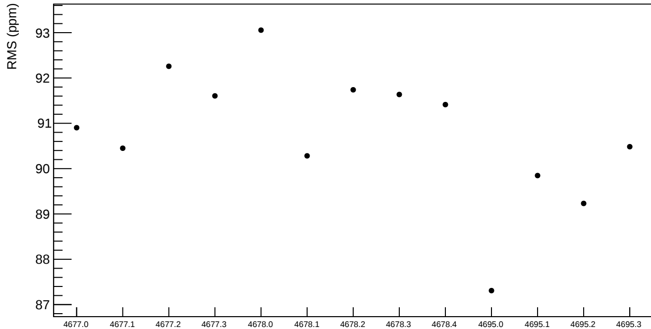
lgr_asym_us_dd RMS (ppm)
