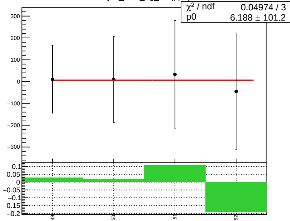
asym_bcm_dg_ds (ppb)
