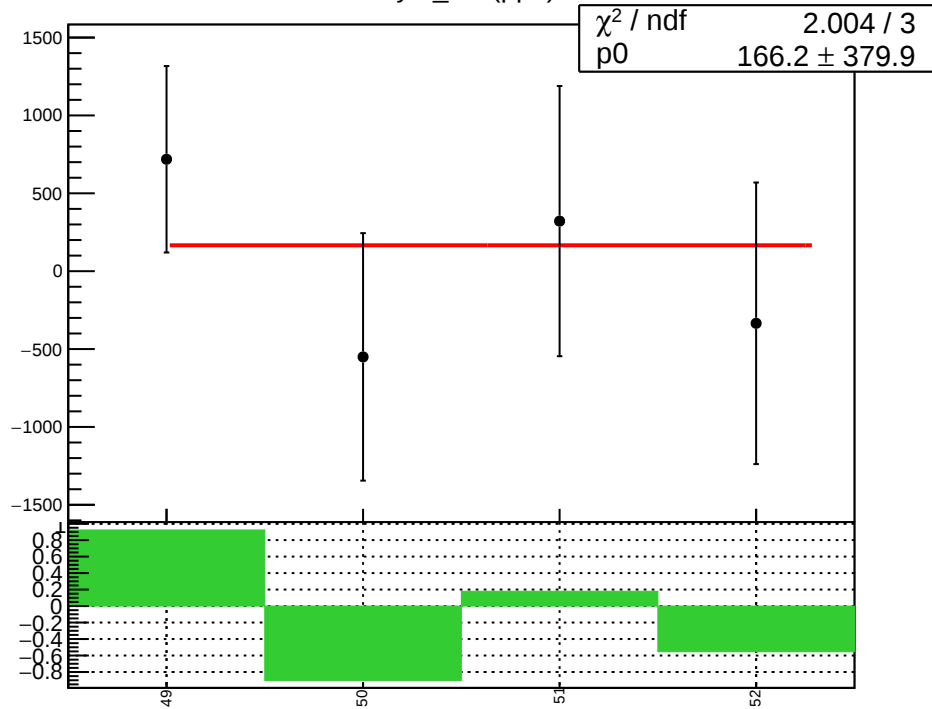
asym_dsl (ppb)
