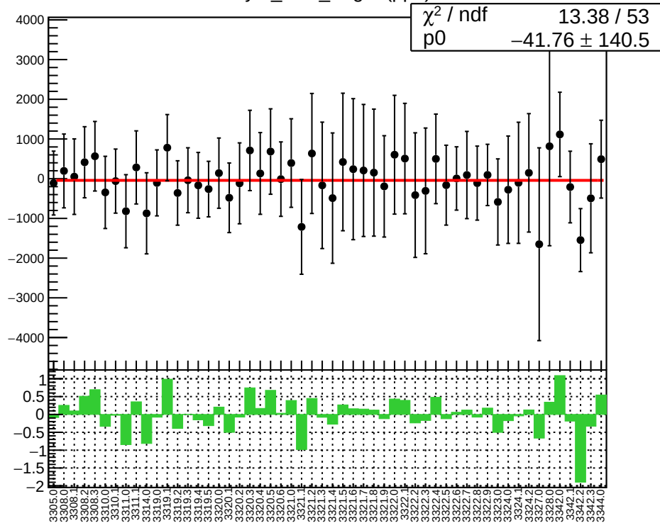
asym_bcm_target (ppb)
