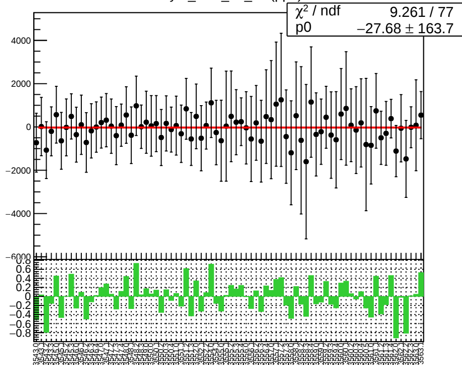
asym_bcm_an_ds (ppb)
