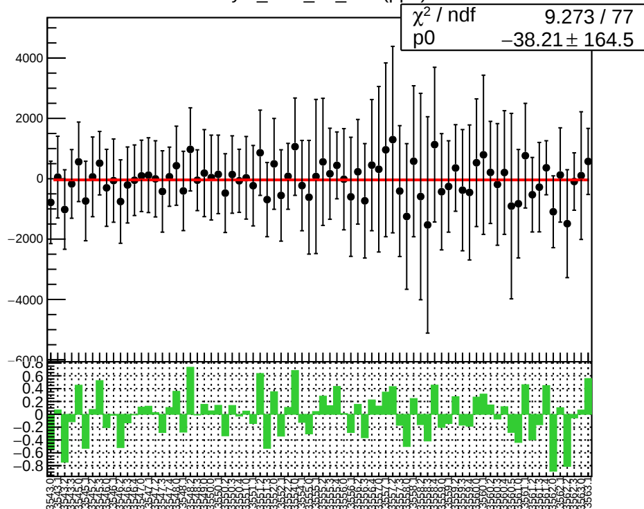
asym_bcm_an_ds3 (ppb)
