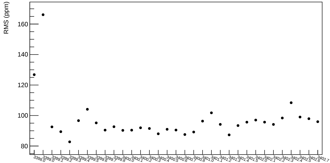
asym_bcm_dg_us RMS (ppm)
