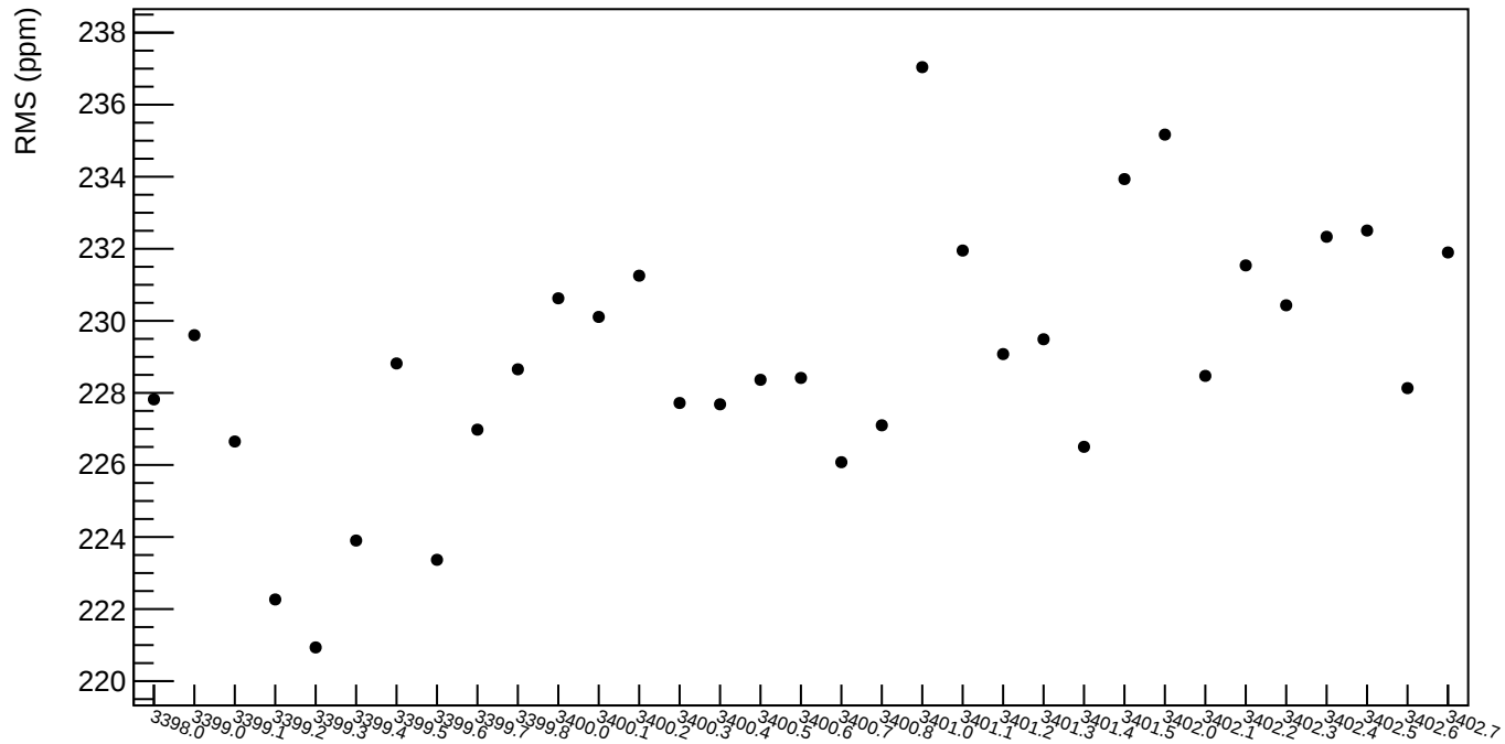
asym_ds_avg RMS (ppm)
