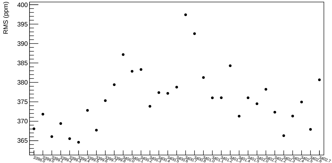
asym_ds_dd RMS (ppm)
