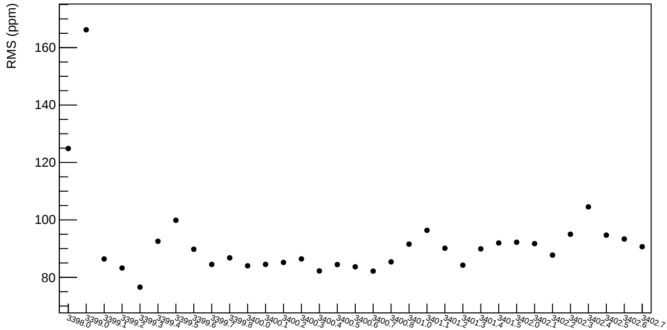
asym_bcm_dg_ds RMS (ppm)
