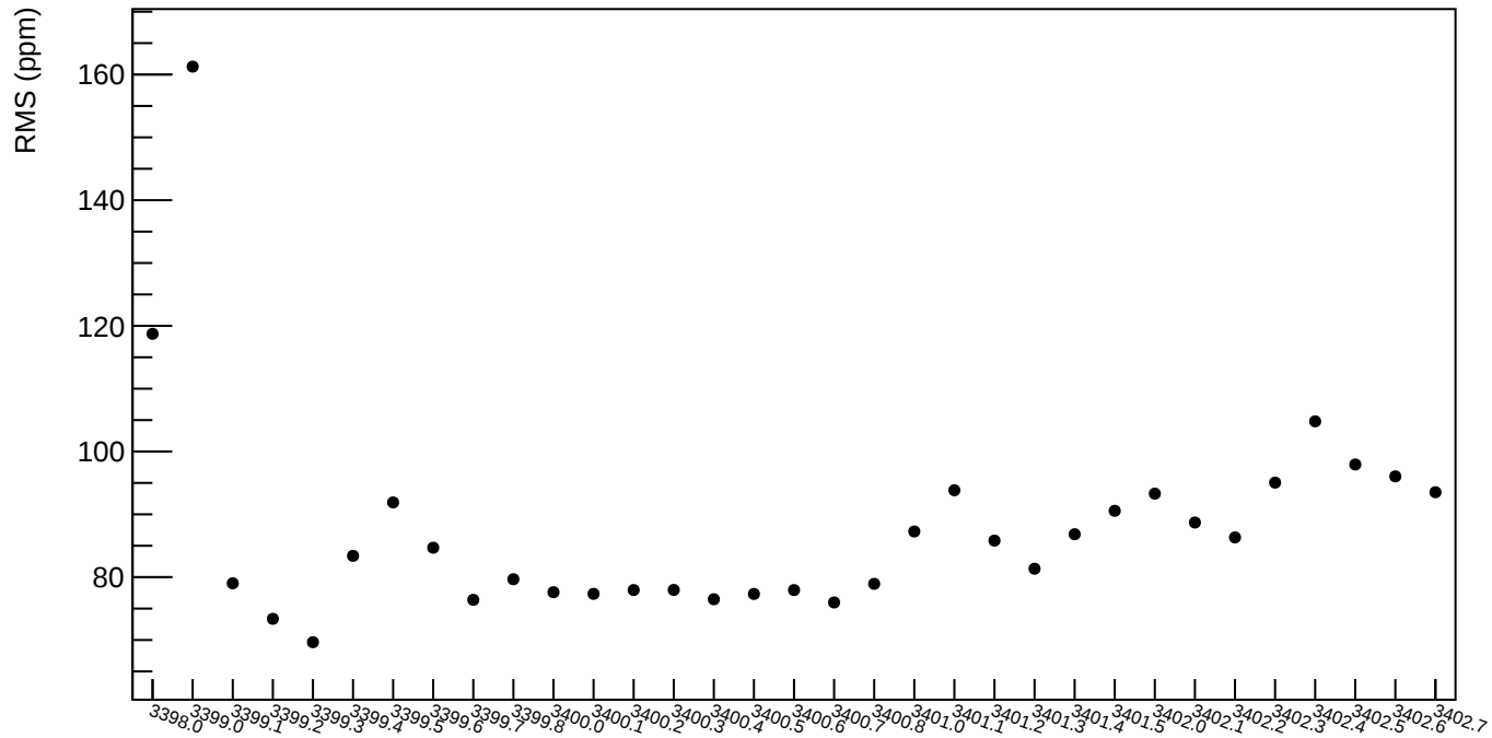
asym_bcm_an_us RMS (ppm)
