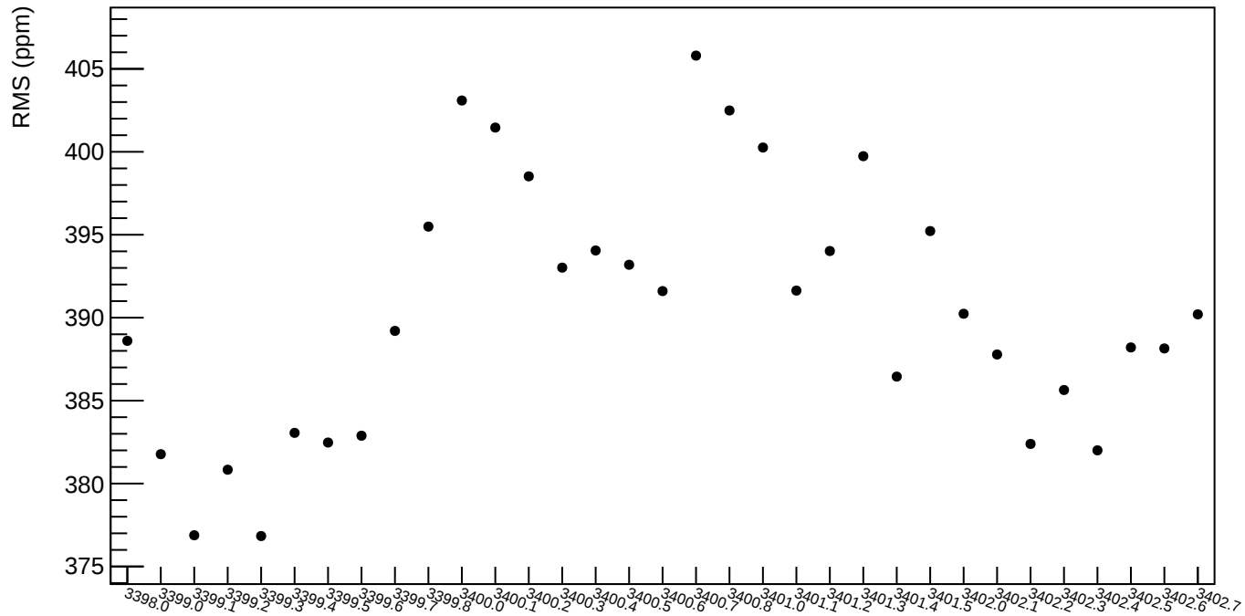
asym_dsr RMS (ppm)
