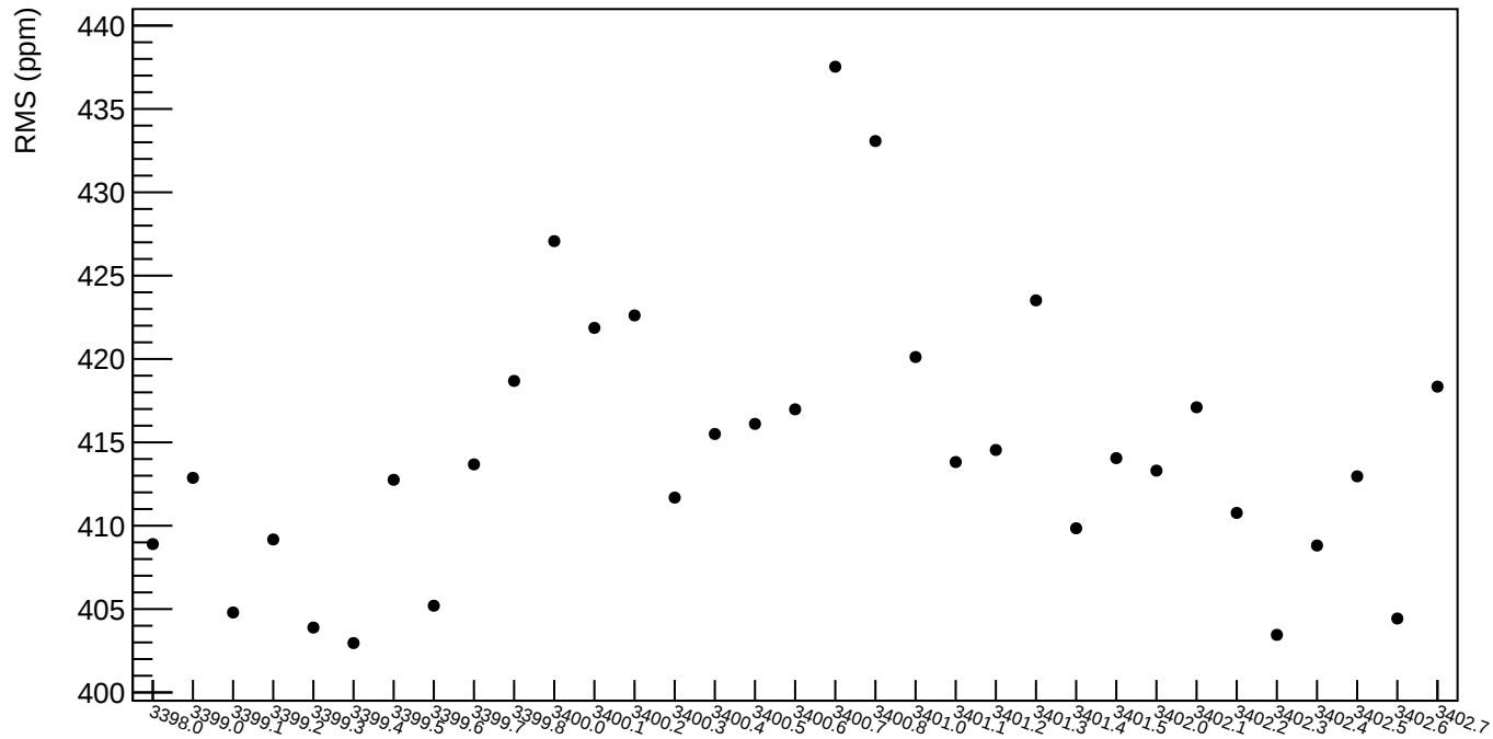
asym_us_dd RMS (ppm)
