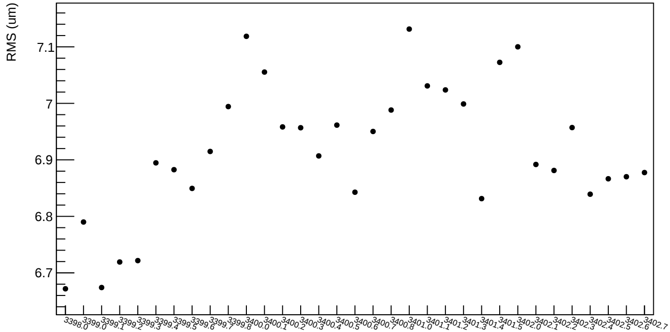
diff_bpme RMS ( \mu\text{m} )
