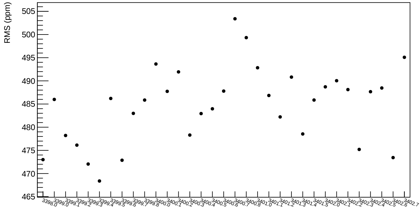
asym_dsl RMS (ppm)
