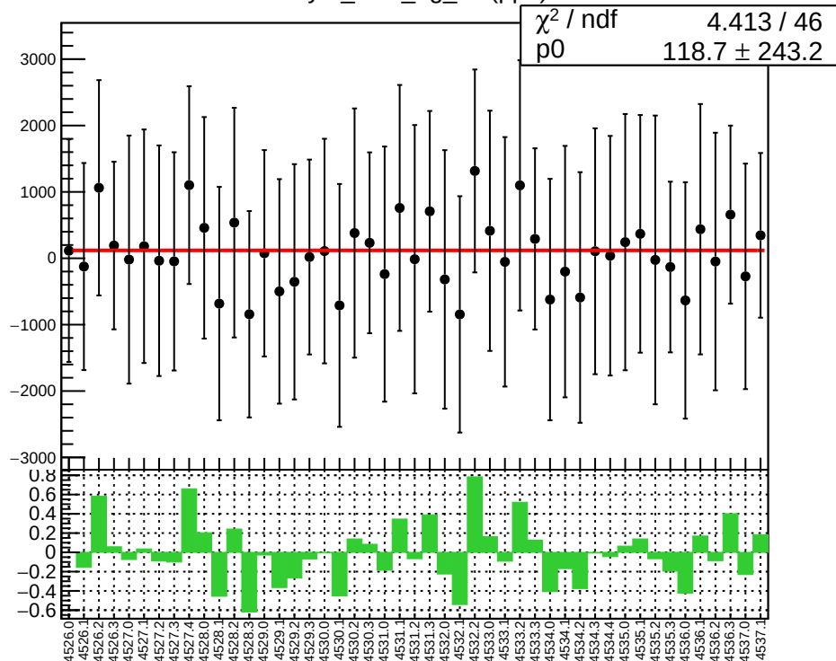
asym_bcm_dg_ds (ppb)
