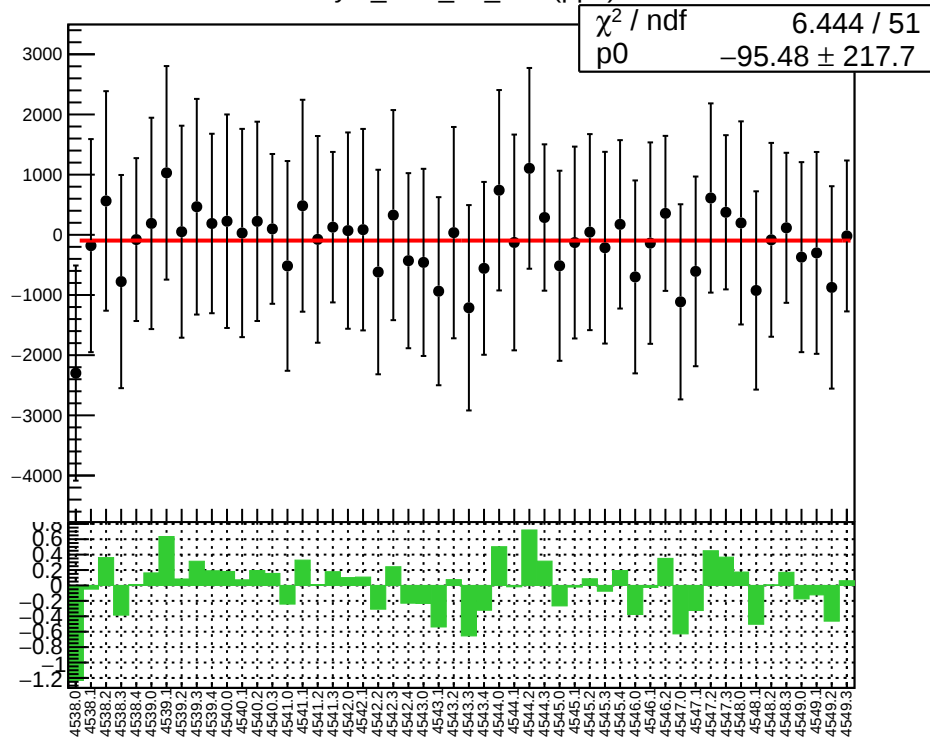
asym_bcm_an_ds3 (ppb)
