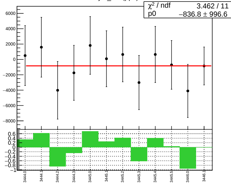
asym_dsr (ppb)
