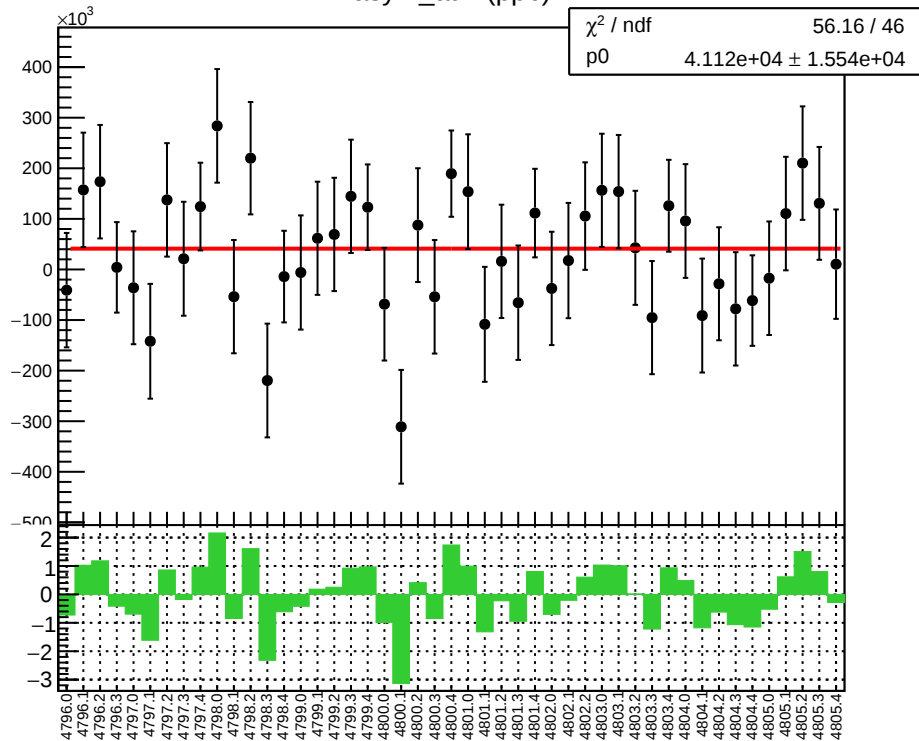
asym_atl2 (ppb)
