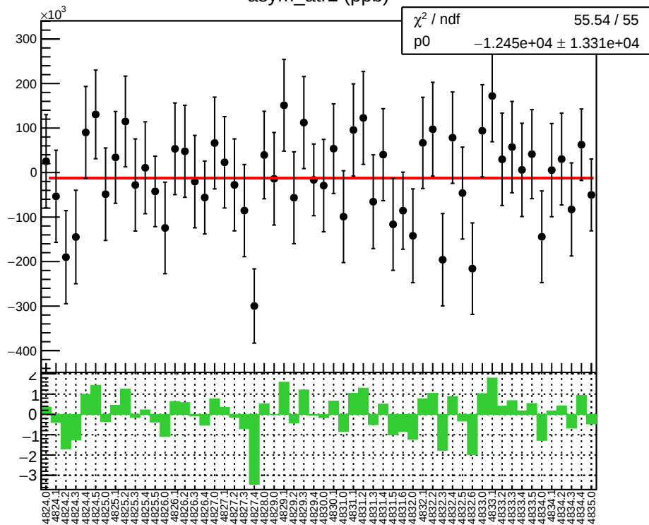
asym_atr2 (ppb)
