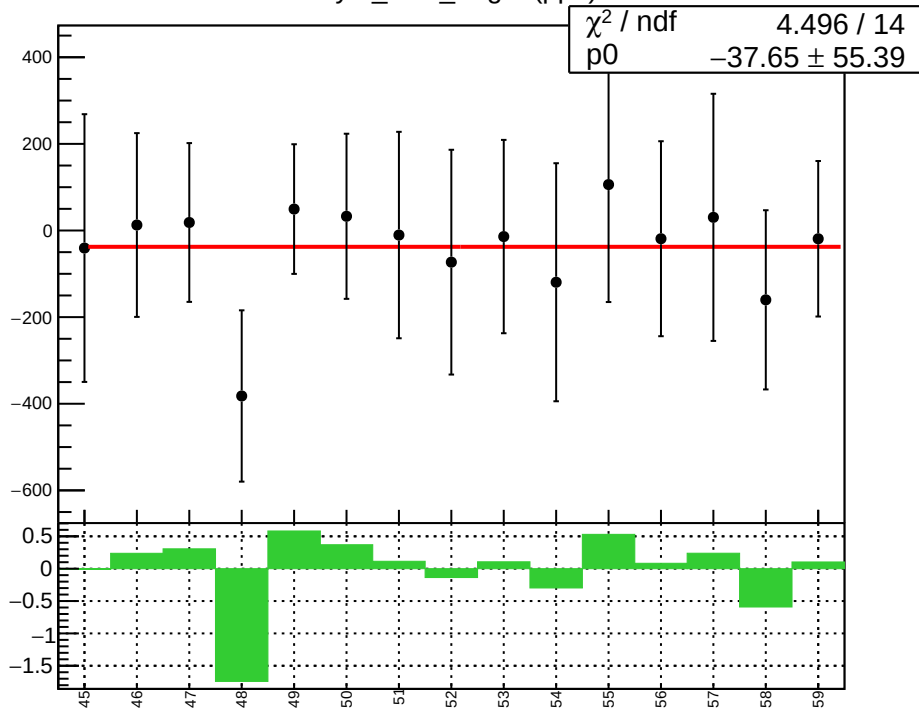
asym_bcm_target (ppb)
