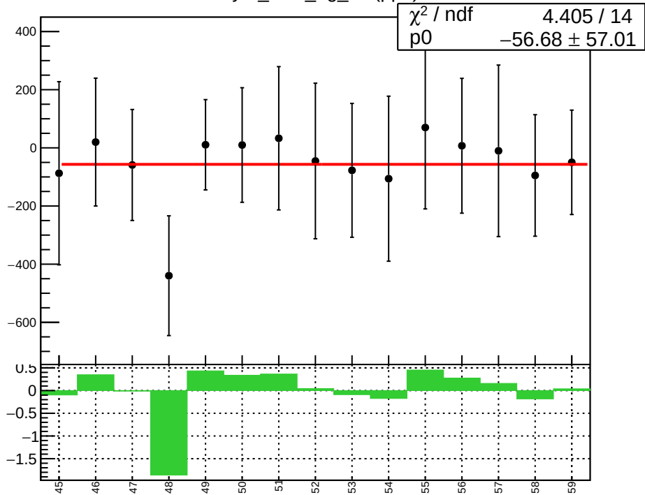
asym_bcm_dg_ds (ppb)
