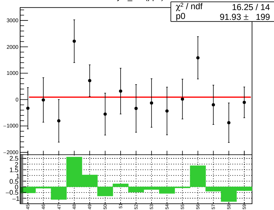
asym_dsl (ppb)
