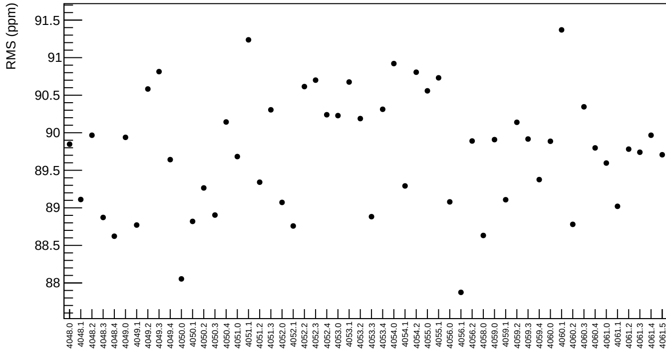
reg_asym_us_dd RMS (ppm)
