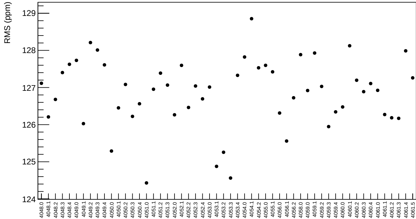
reg_asym_usr RMS (ppm)
