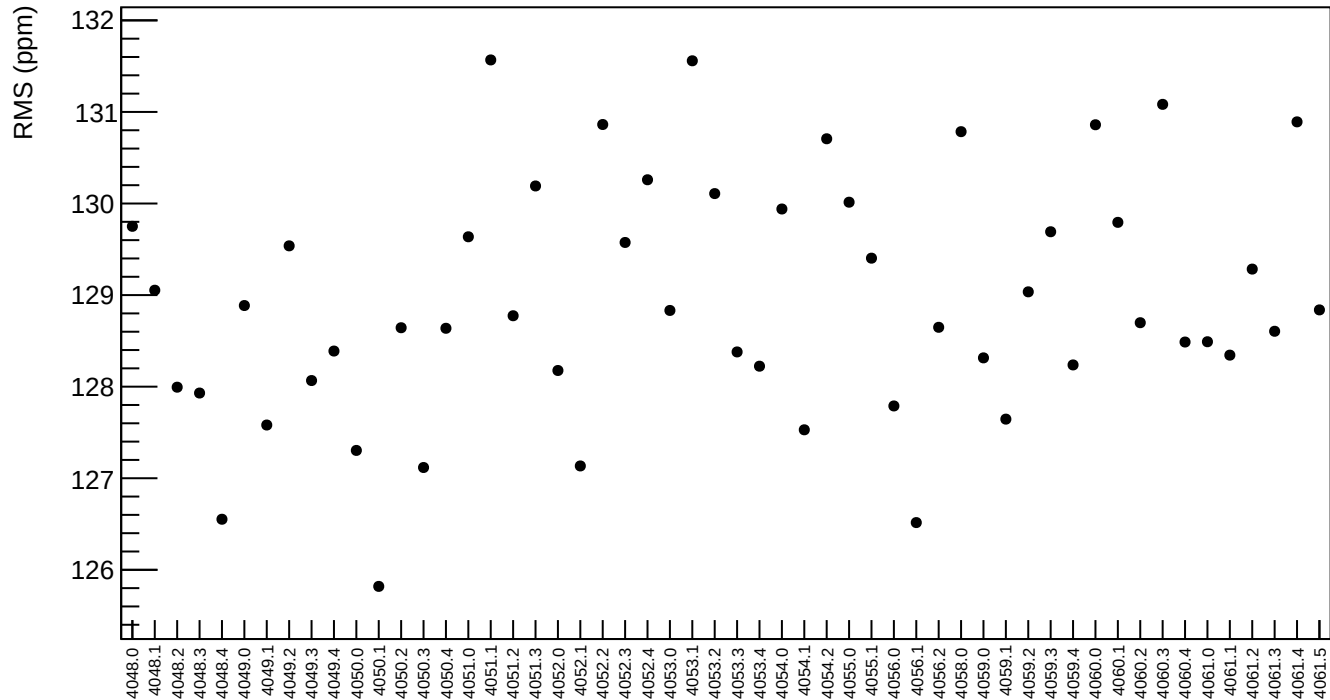
reg_asym_usl RMS (ppm)
