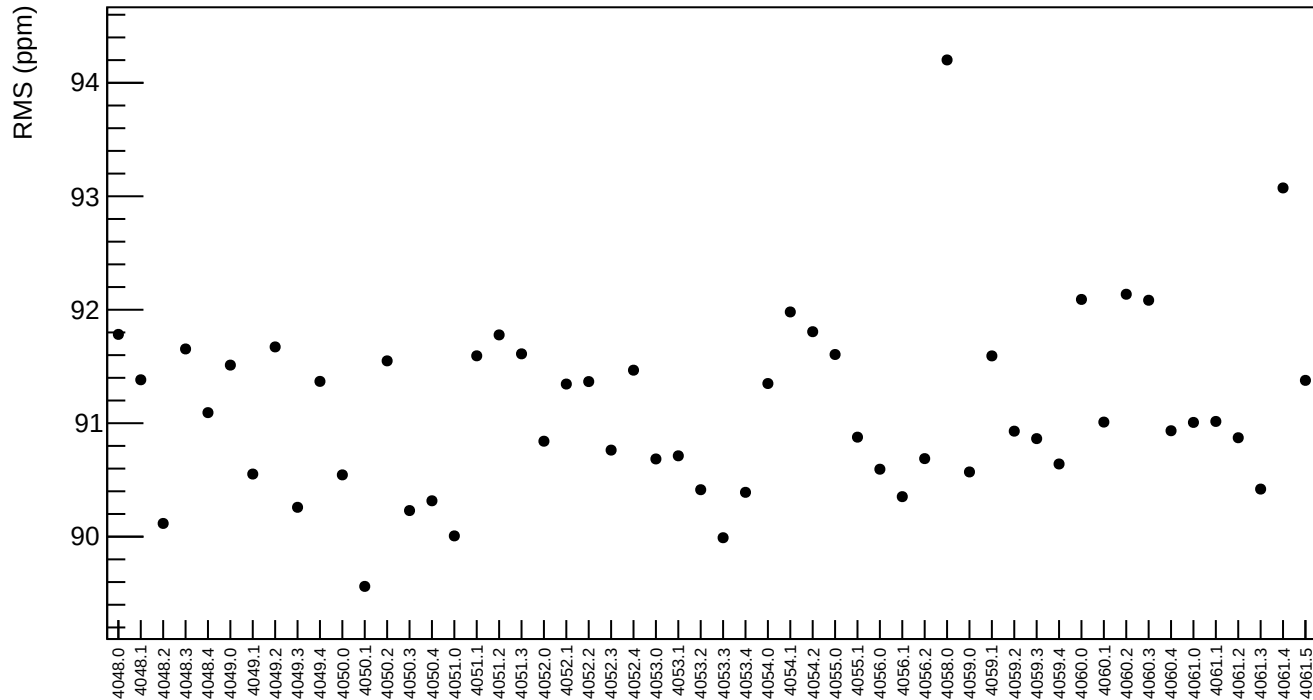
reg_asym_us_avg RMS (ppm)
