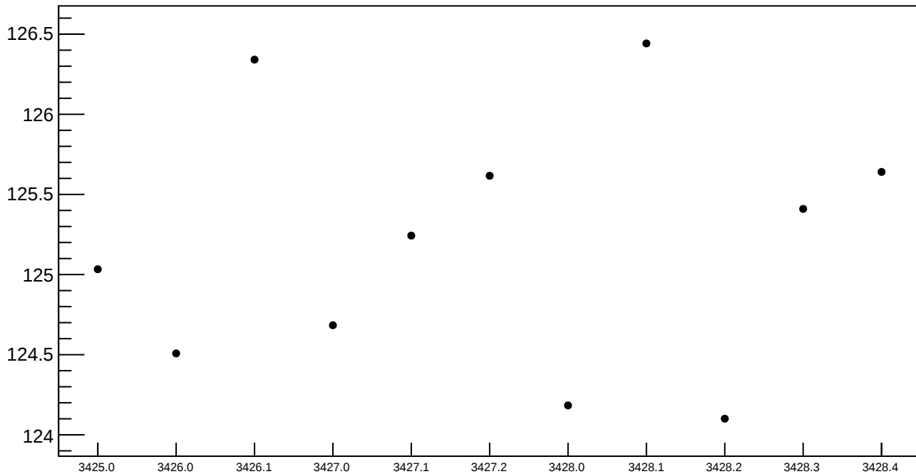
reg_asym_usl RMS (ppm)
