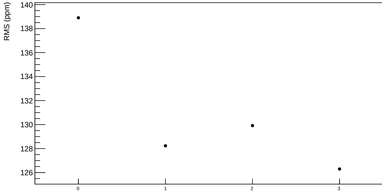
reg_asym_usr RMS (ppm)
