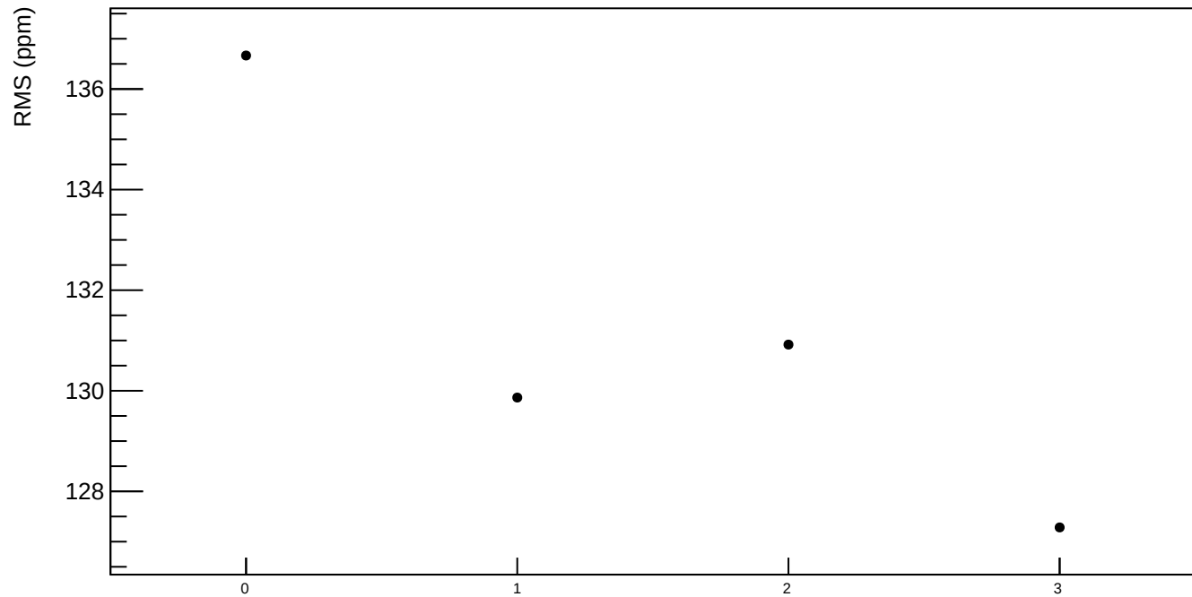
reg_asym_usl RMS (ppm)
