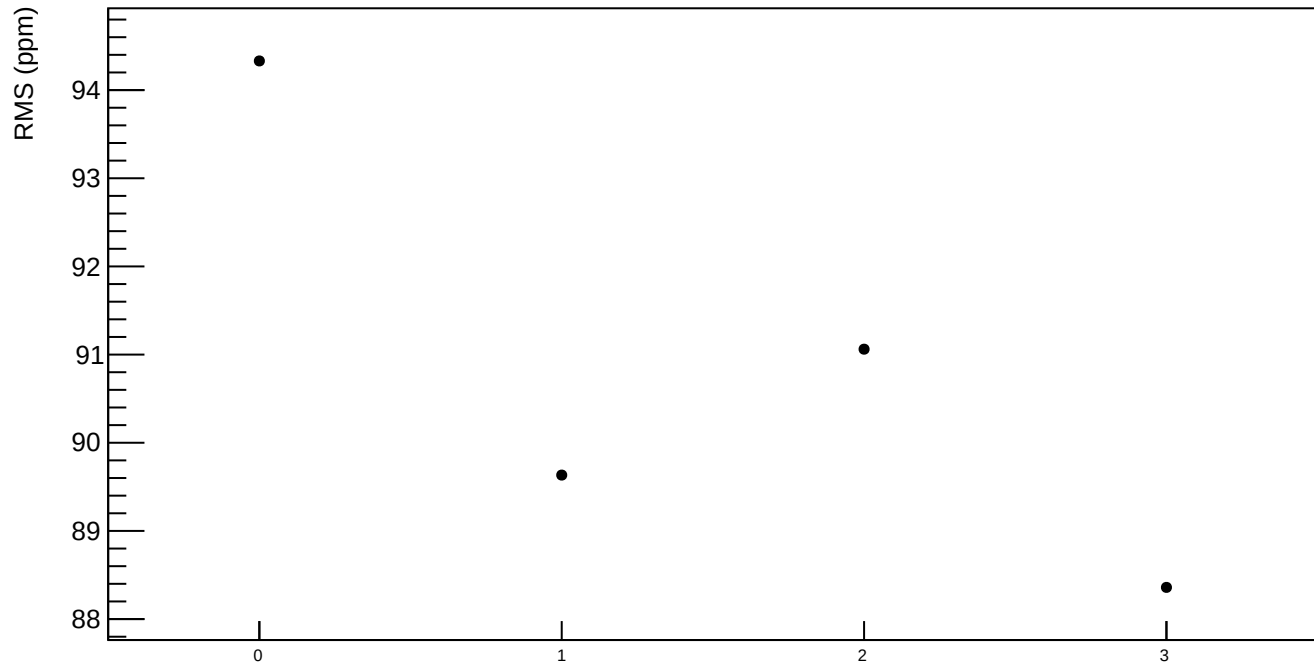
reg_asym_us_dd RMS (ppm)
