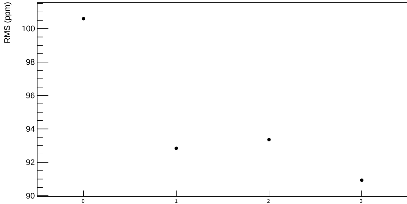
reg_asym_us_avg RMS (ppm)
