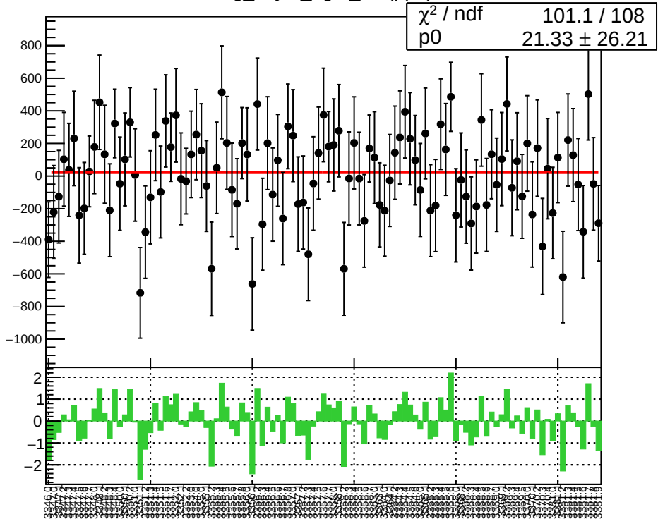
reg_asym_right_dd (ppb)
