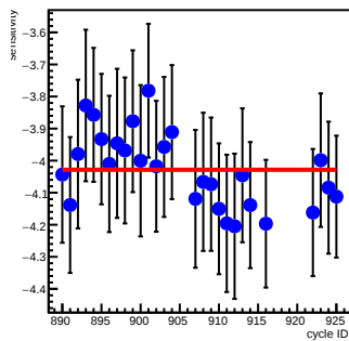
dsr_coil2(ppm/count)
