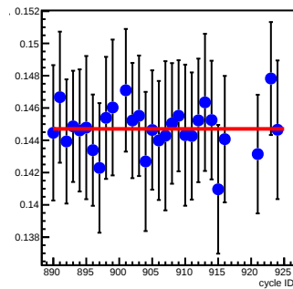
bpm12Y_coil6(um/count)
