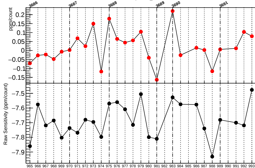
Residual Sensitivity in us1_coil3
