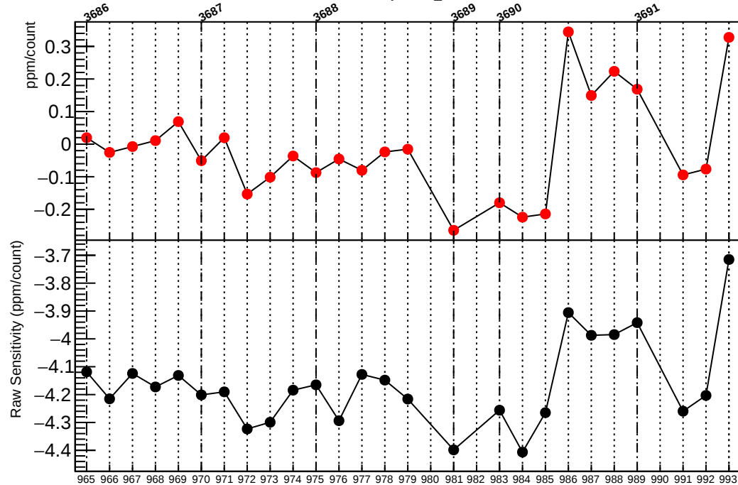
Residual Sensitivity in dsr_coil2
