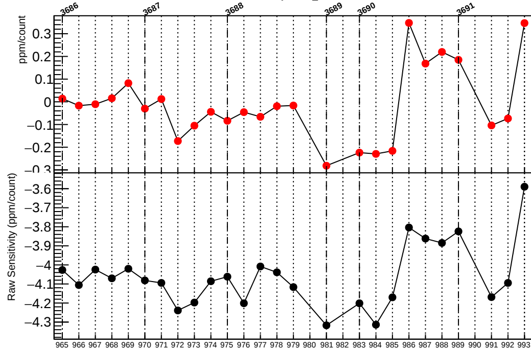
Residual Sensitivity in usr_coil2
