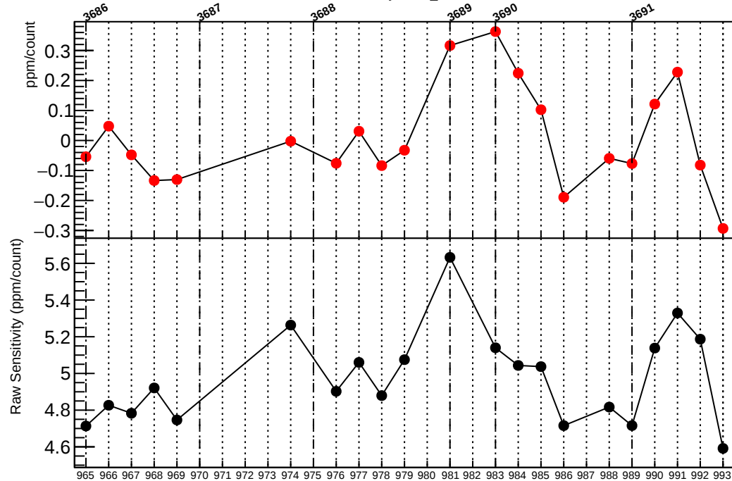
Residual Sensitivity in us1_coil6
