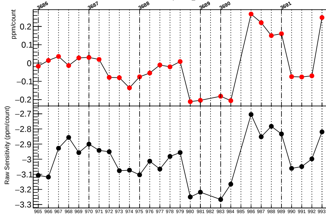
Residual Sensitivity in usr_coil4
