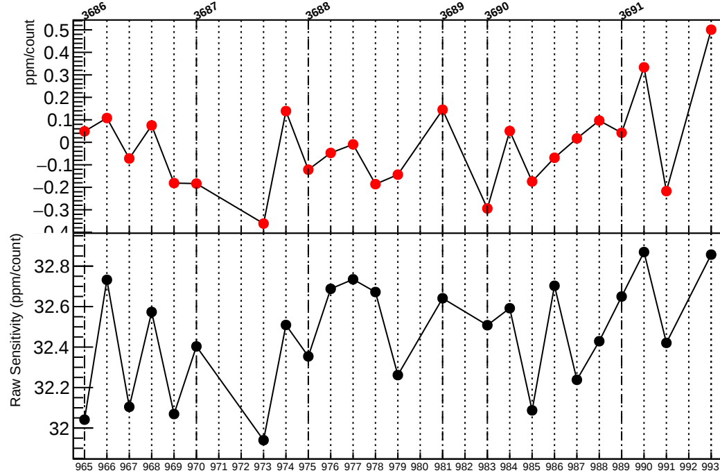
Residual Sensitivity in us1_coil7
