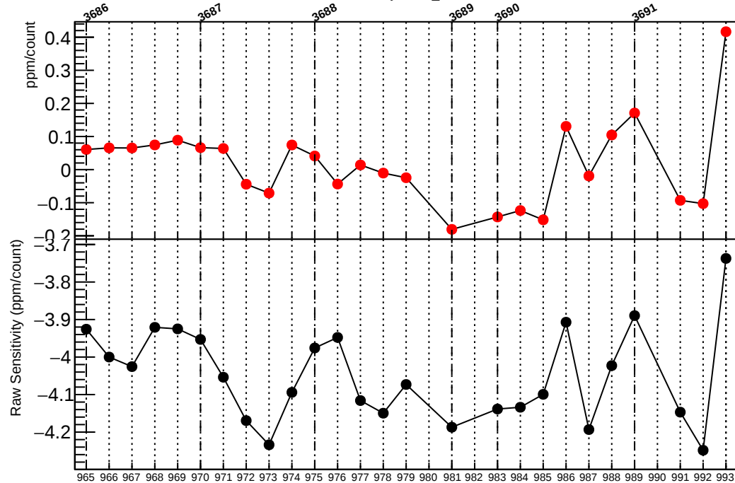
Residual Sensitivity in usl_coil2
