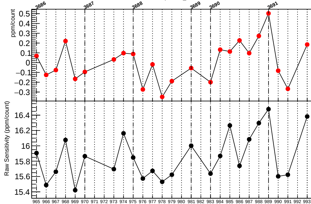
Residual Sensitivity in dsr_coil7
