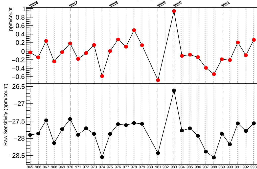
Residual Sensitivity in dsl_coil1
