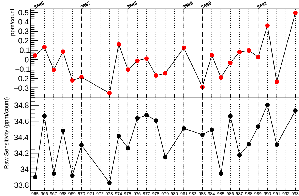
Residual Sensitivity in dsl_coil7
