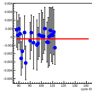
bpm8Y_coil7(um/count)
