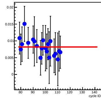
bpm8Y_coil7(um/count)
