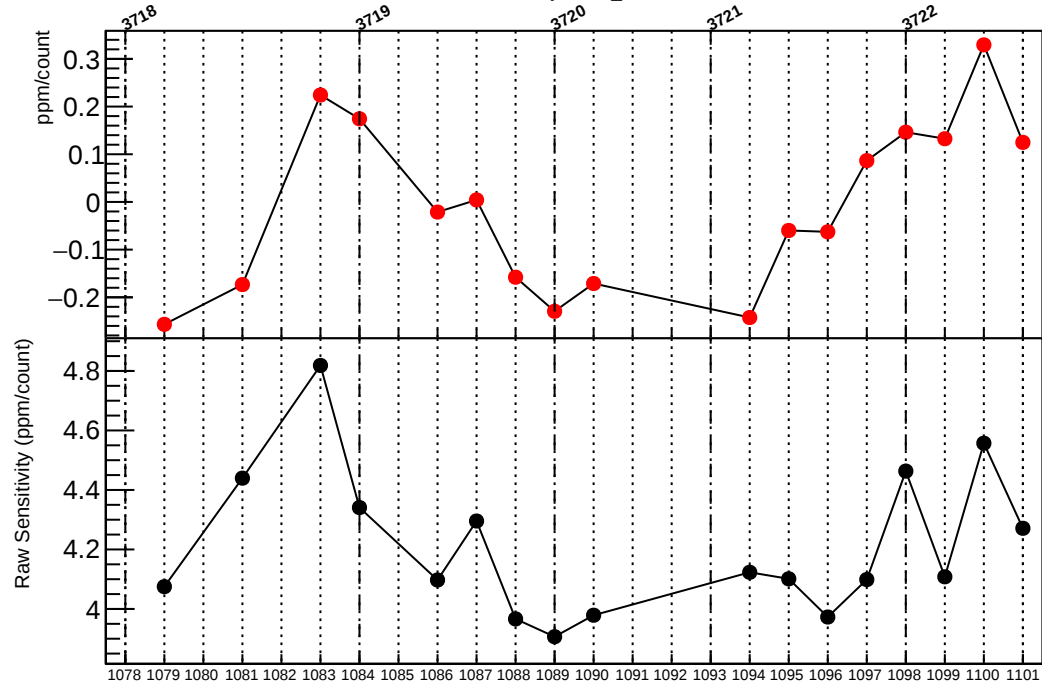
Residual Sensitivity in dsr_coil6
