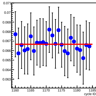
bpm16X_coil2(um/count)
