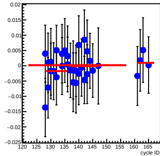
bpm8X_coil6(um/count)
