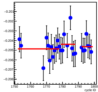
bpm16Y_coil6(um/count)
