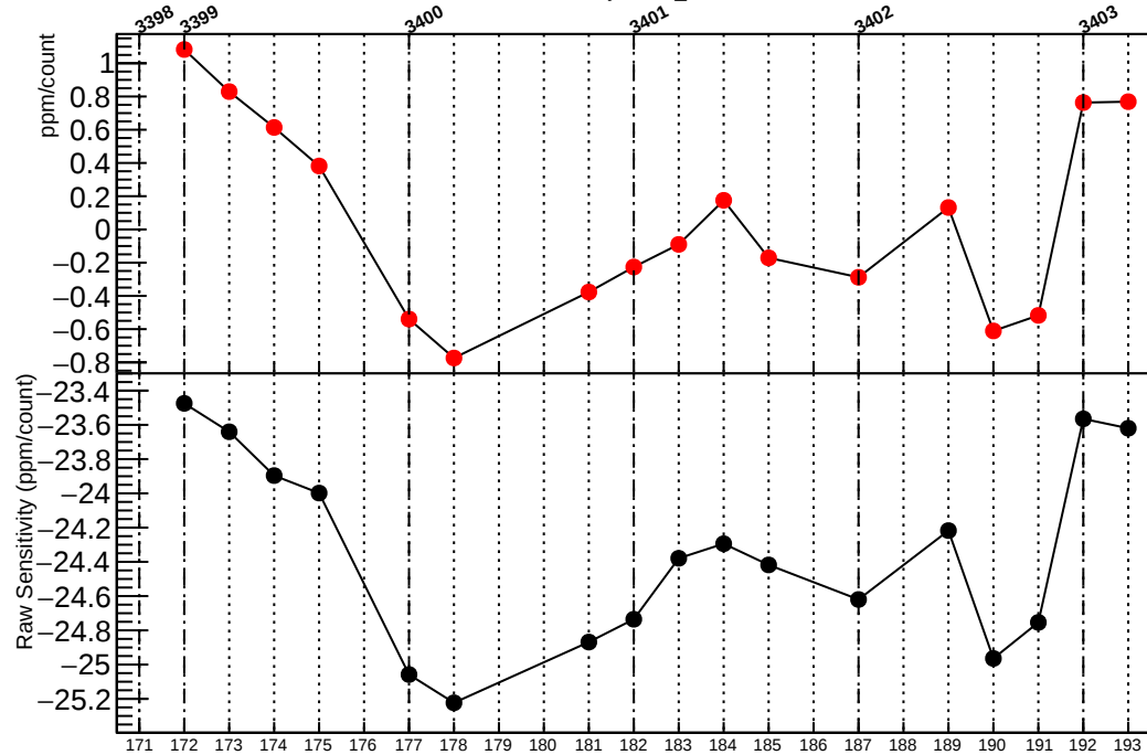
Residual Sensitivity in dsr_coil5
