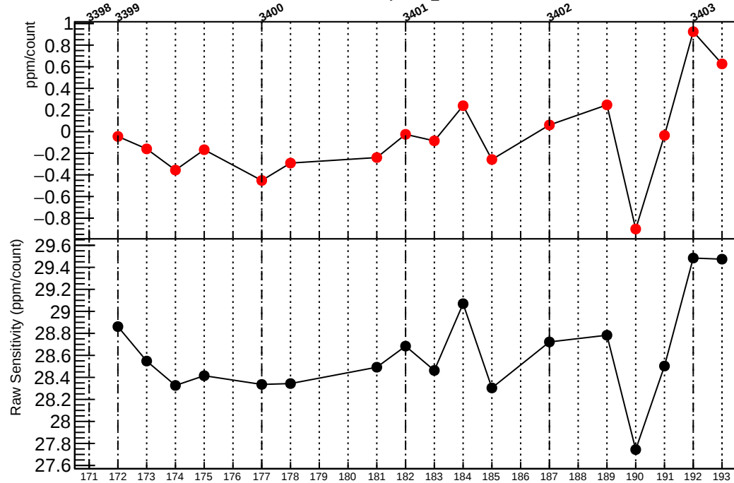
Residual Sensitivity in dsl_coil5
