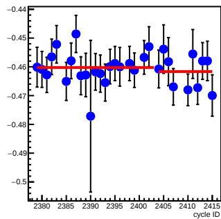
bpm11X_coil7(um/count)
