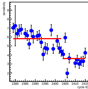
at1_coil2(ppm/count)
