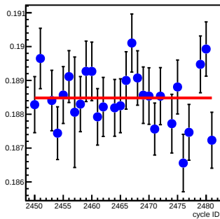
bpm16Y_coil2(um/count)
