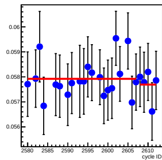
bpm16Y_coil5(um/count)
