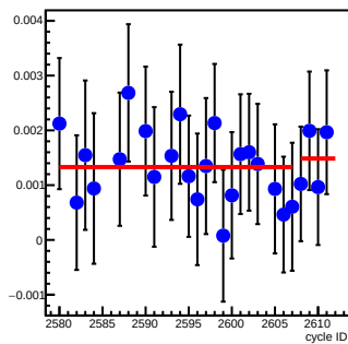
bpm16Y_coil2(um/count)
