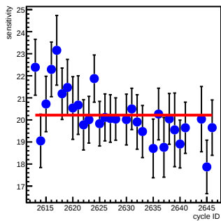
at1_coil2(ppm/count)
