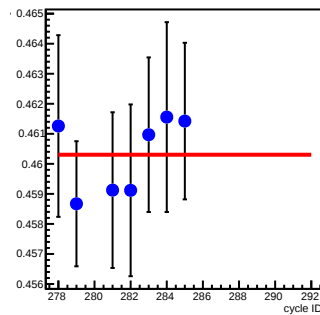
bpm4aY_coil6(um/count)
