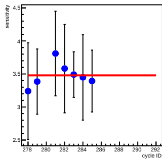
dsl_coil6(ppm/count)
