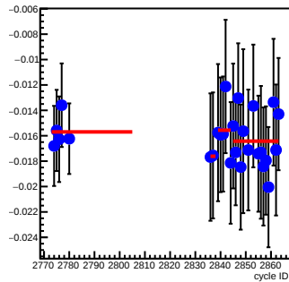
bpm12Y_coil2(um/count)
