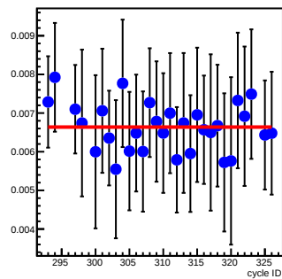
bpm16X_coil5(um/count)
