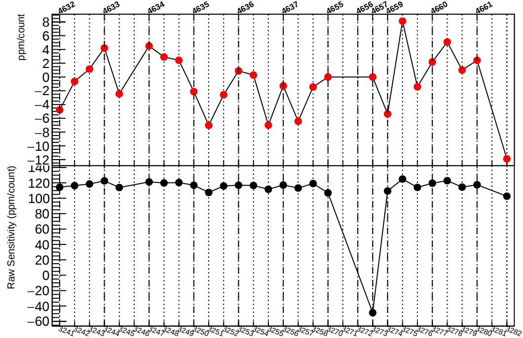
Residual Sensitivity in atl1_coil7
