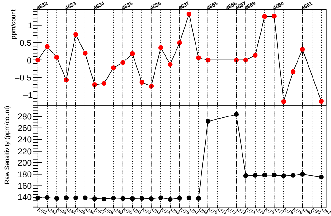
Residual Sensitivity in at11_coil1
