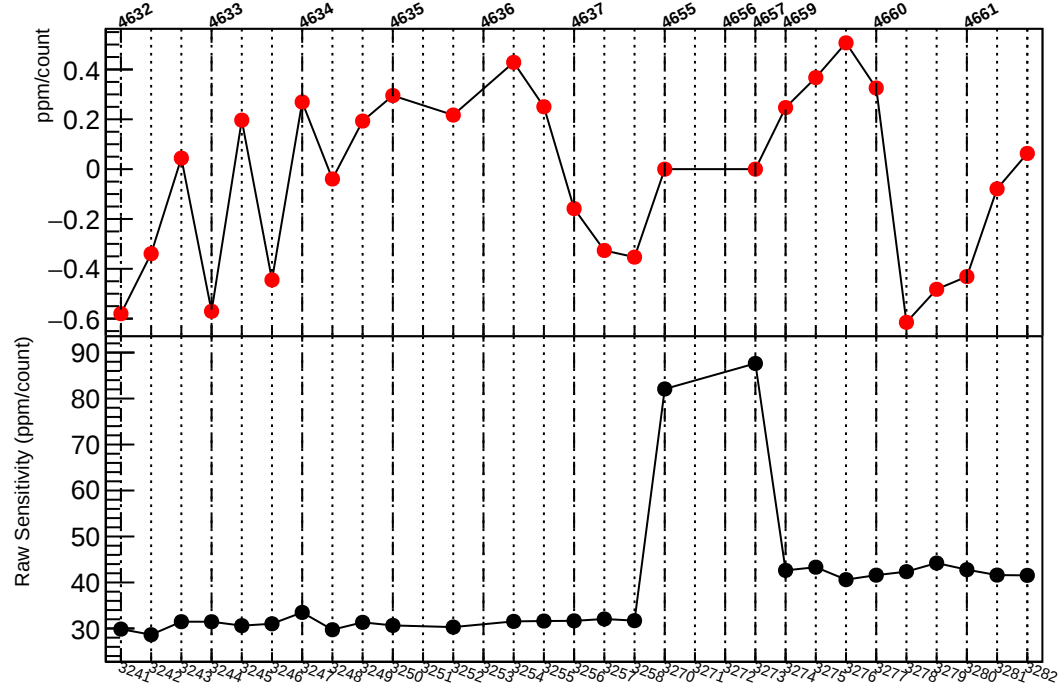
Residual Sensitivity in atr2_coil3
