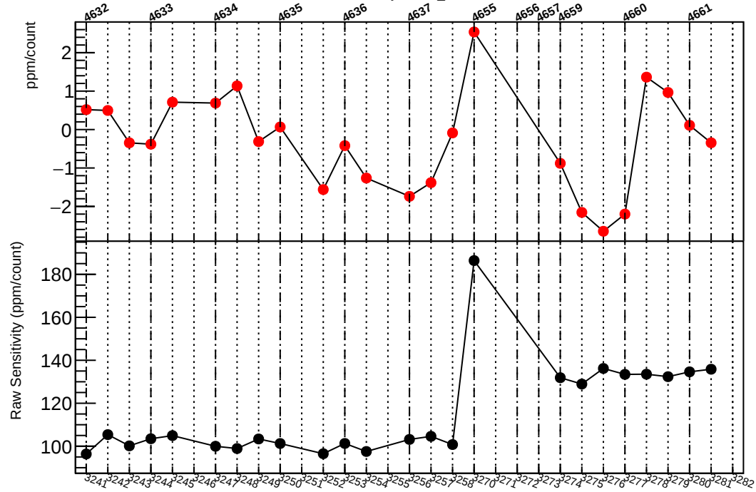
Residual Sensitivity in atl2_coil5
