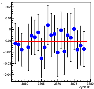
bpm11X12X_coil6(um/count)
