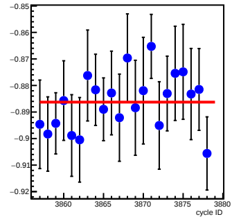
bpm11X_coil7(um/count)
