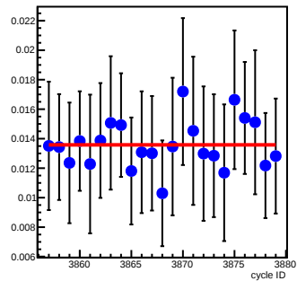
bpm16X_coil5(um/count)
