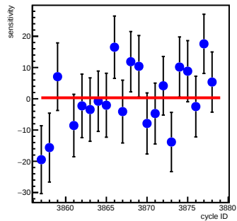
atr2_coil6(ppm/count)
