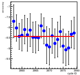
dsl_coil5(ppm/count)
