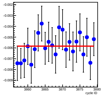
bpm4aX_coil5(um/count)
