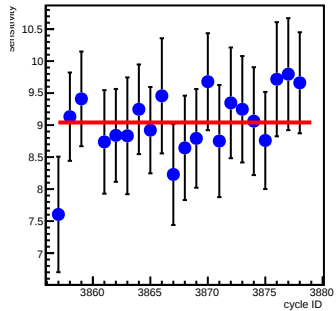
usr_coil6(ppm/count)
