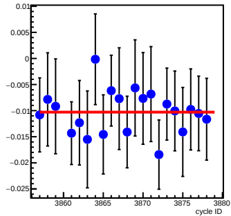
bpm16X_coil6(um/count)
