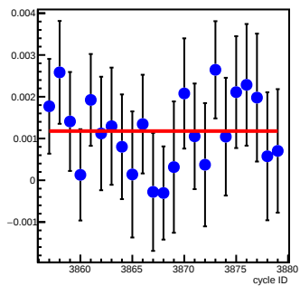
bpm16Y_coil2(um/count)
