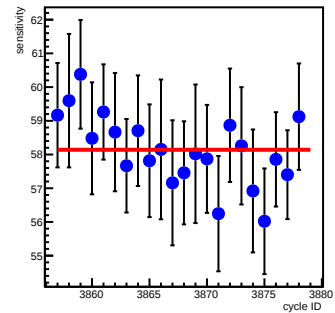
dsl_coil7(ppm/count)
