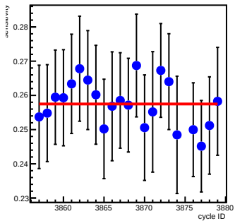
bpm12X_coil5(um/count)
