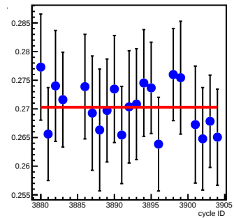
bpm12Y_coil6(um/count)
