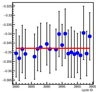
bpm1X_coil2(um/count)
