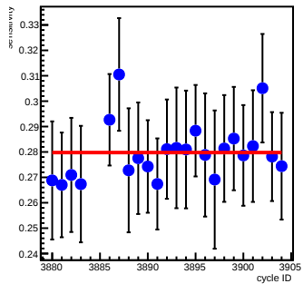
bpm1X_coil7(um/count)
