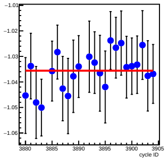
bpm1X_coil7(um/count)
