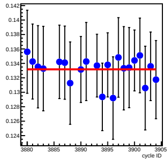
bpm16X_coil2(um/count)
