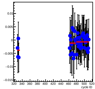
bpm11X12X_coil6(um/count)
