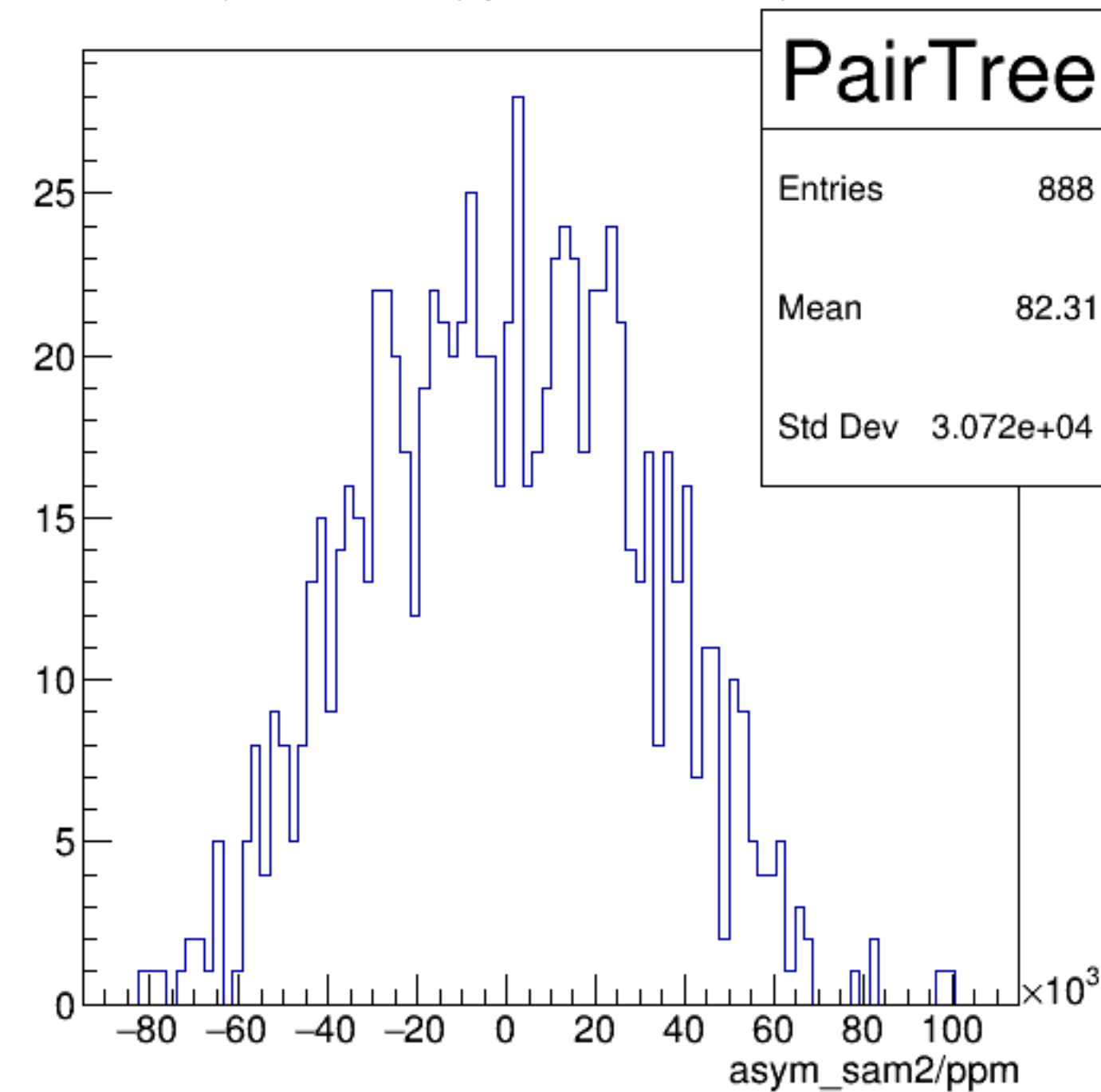
asym_sam2/ppm {ErrorFlag==0}
