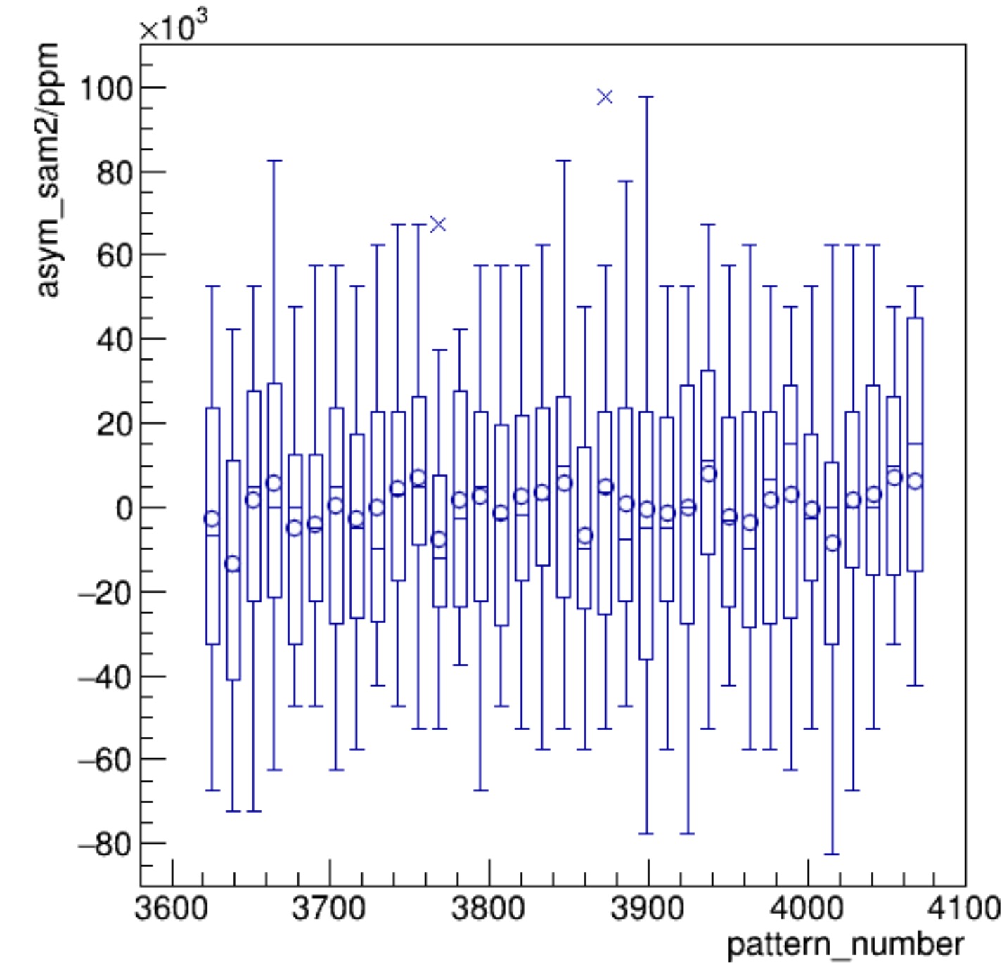
asym_sam2/ppm:pattern_number {ErrorFlag==0}
