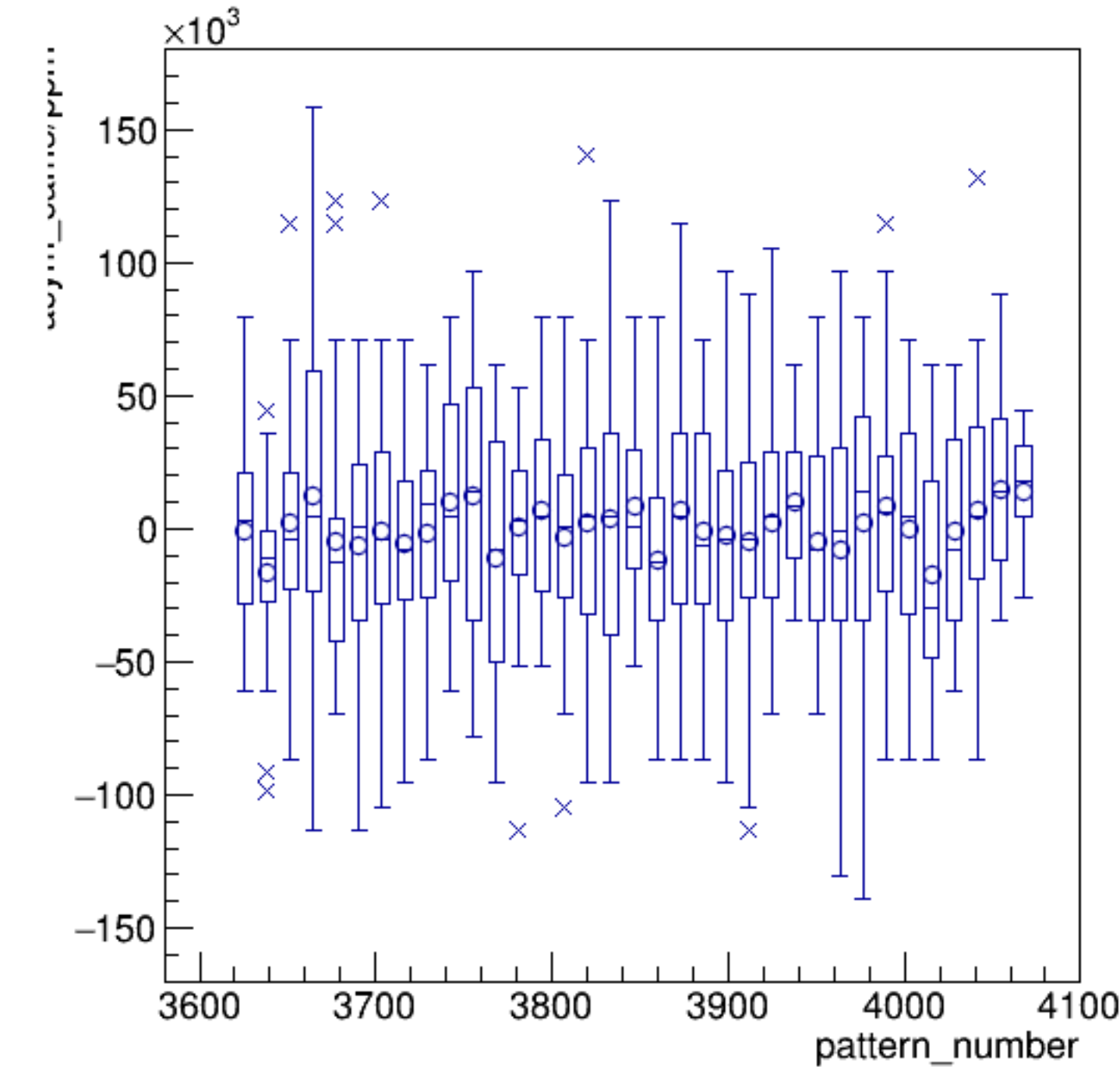
asym_sam3/ppm:pattern_number {ErrorFlag==0}
