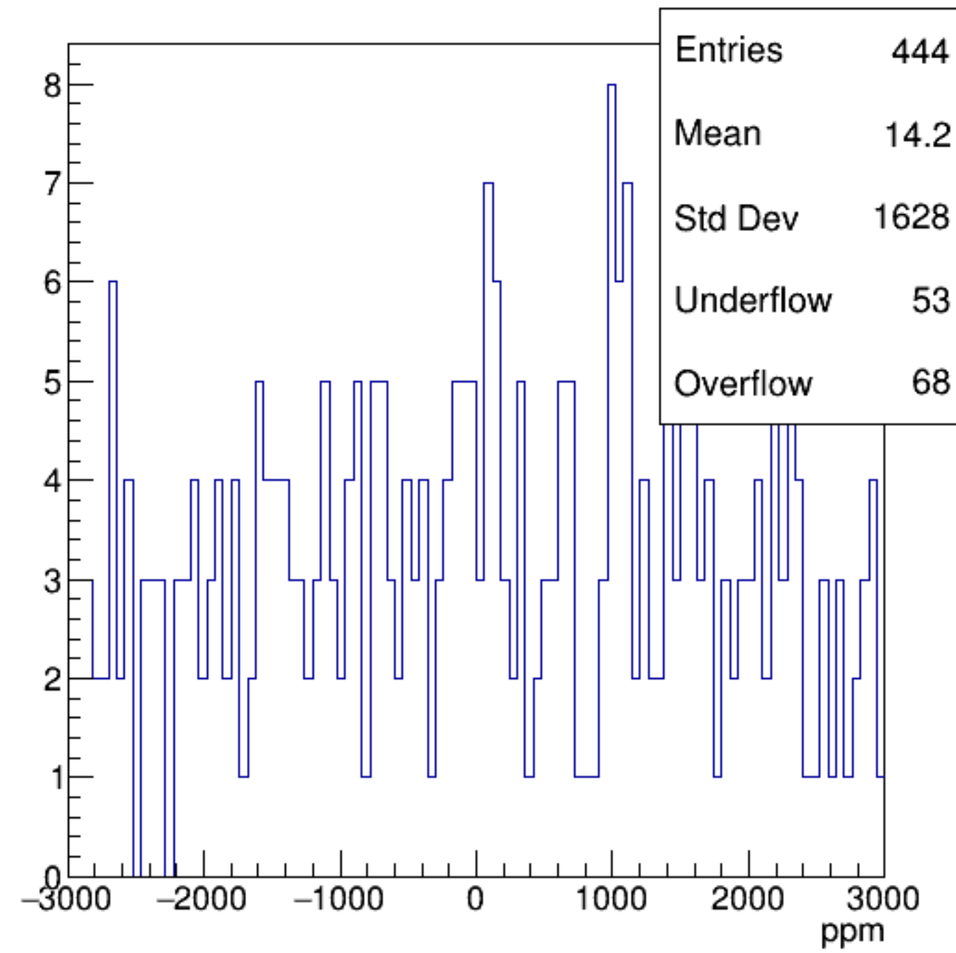
asym_sam5
