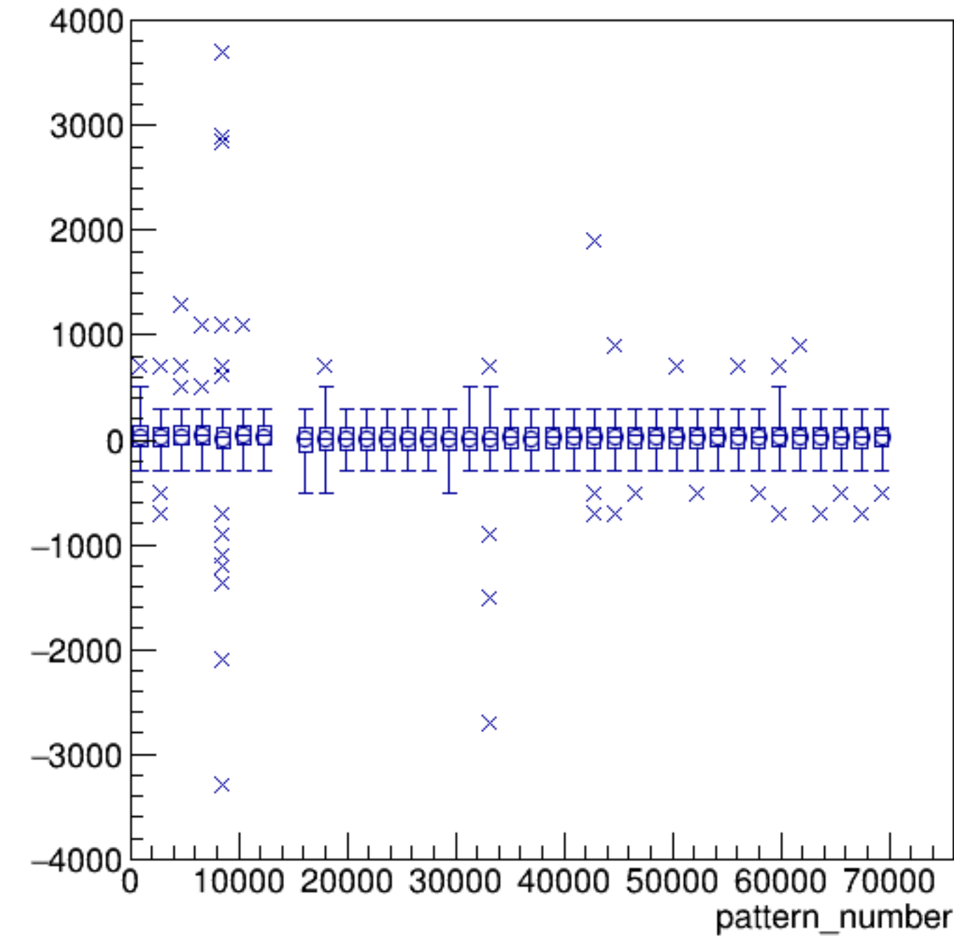
asym_bcm0l02/ppm:pattern_number {ErrorFlag==0}
