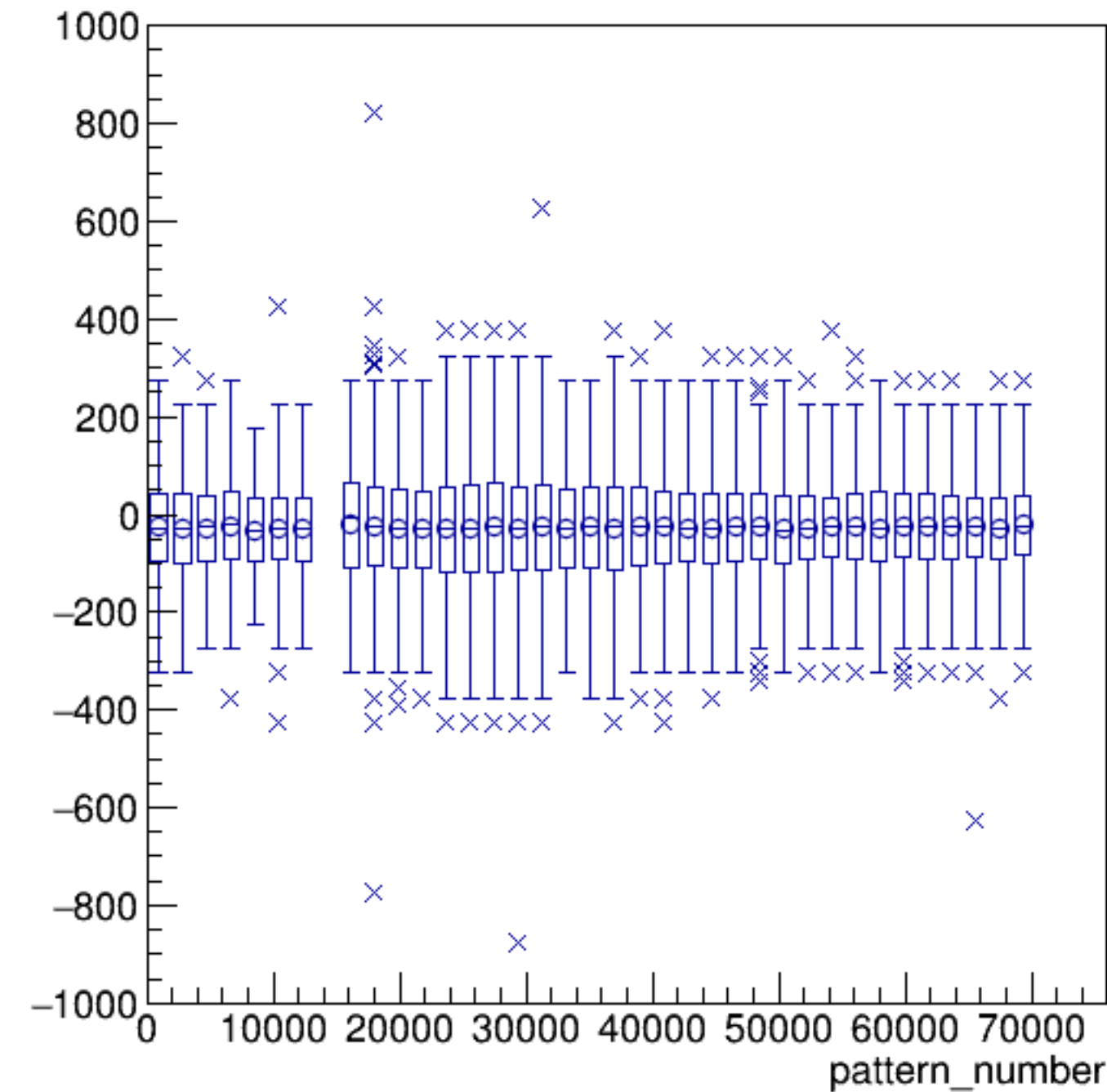
asym_bcm_an_ds/ppm:pattern_number {ErrorFlag==0}
