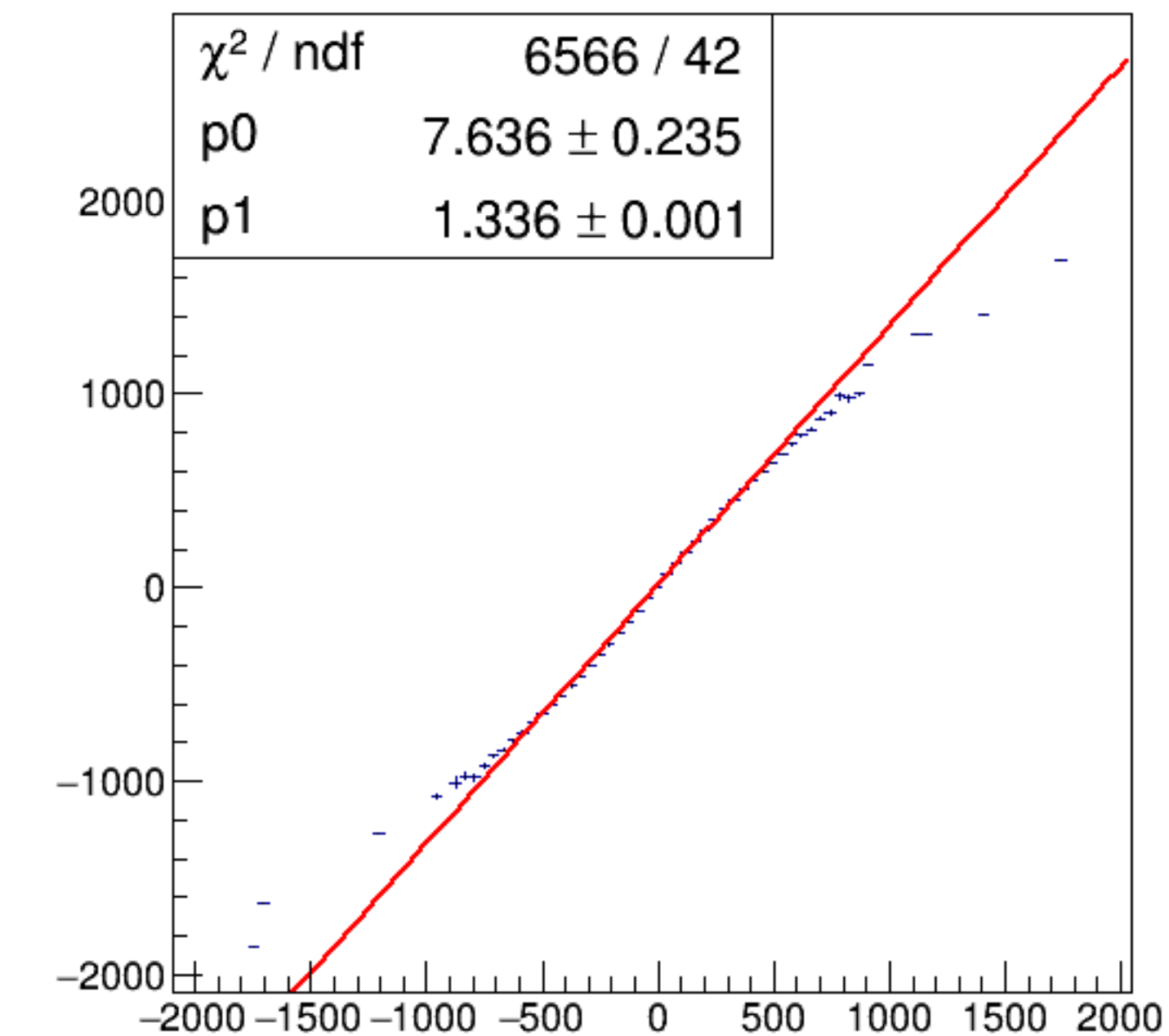
run3291_000_asym_bcm_dg_us_vs_asym_bcm_dg_ds_pr.png
