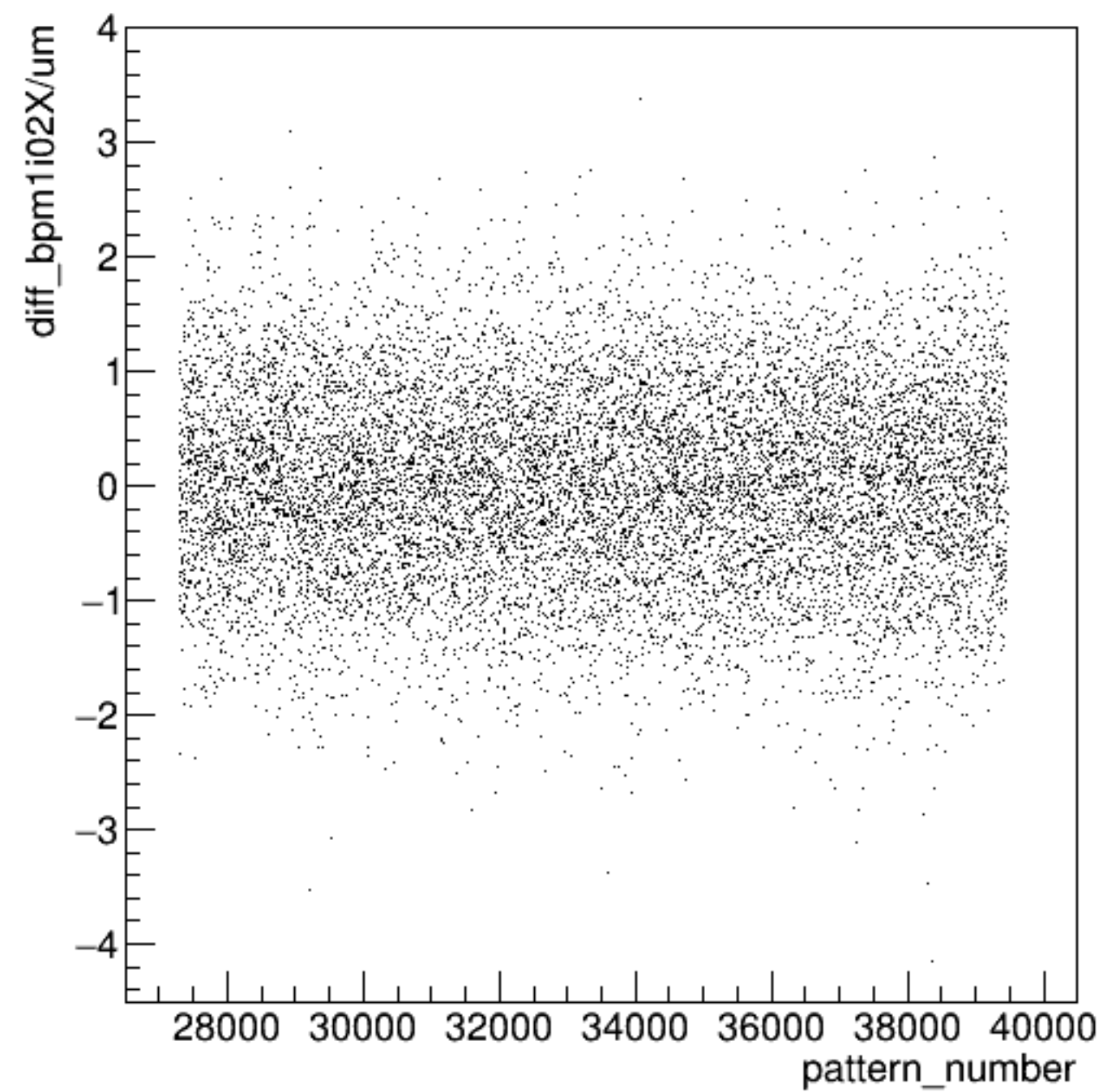
diff_bpm1i02X/um:pattern_number {ErrorFlag==0}
