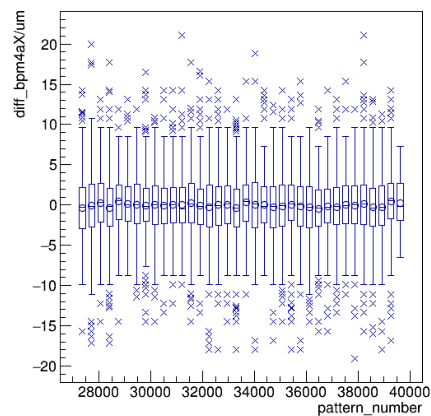
diff_bpm4aX/um:pattern_number {ErrorFlag==0}
