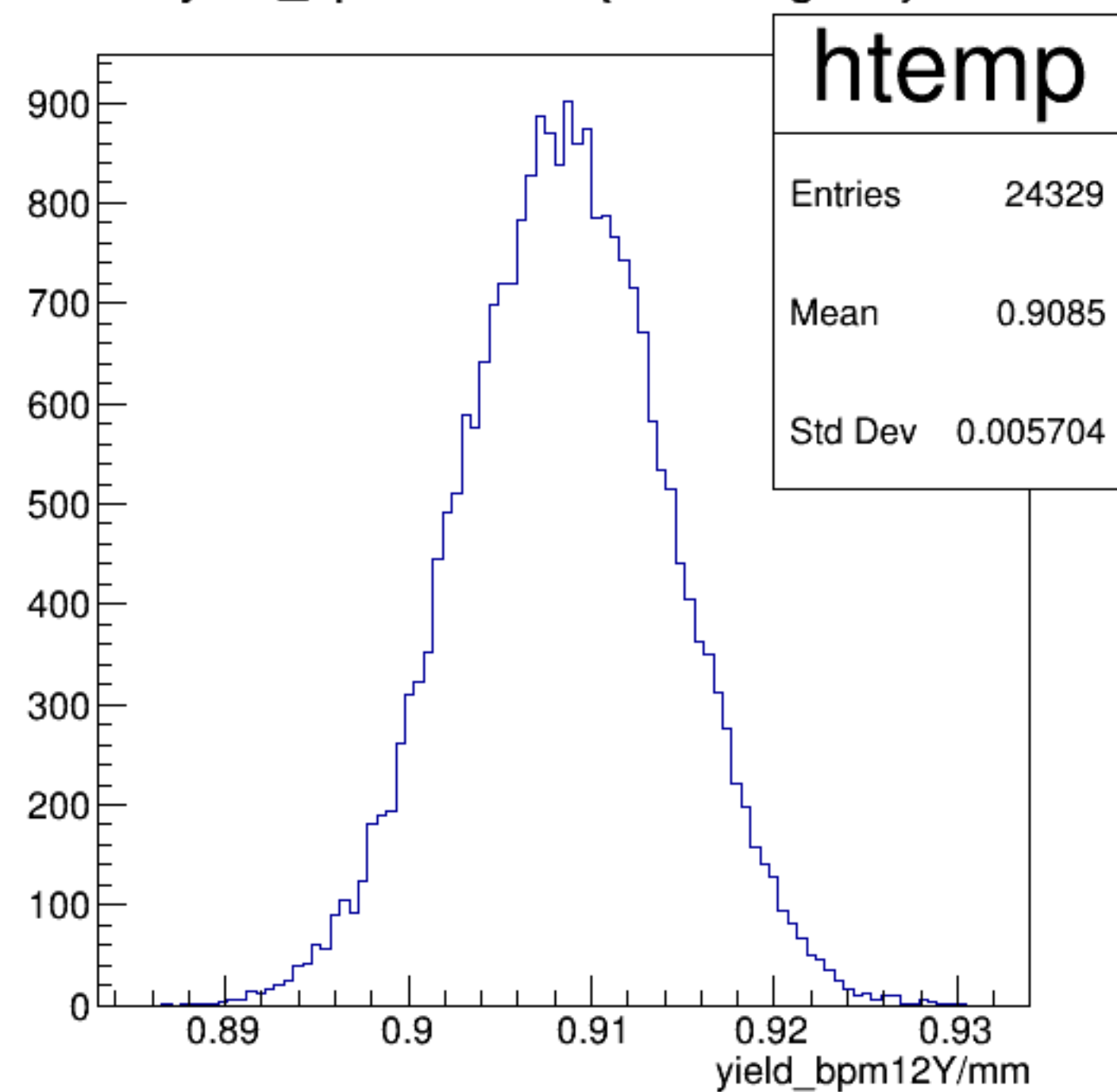
yield_bpm12Y/mm {ErrorFlag==0}
