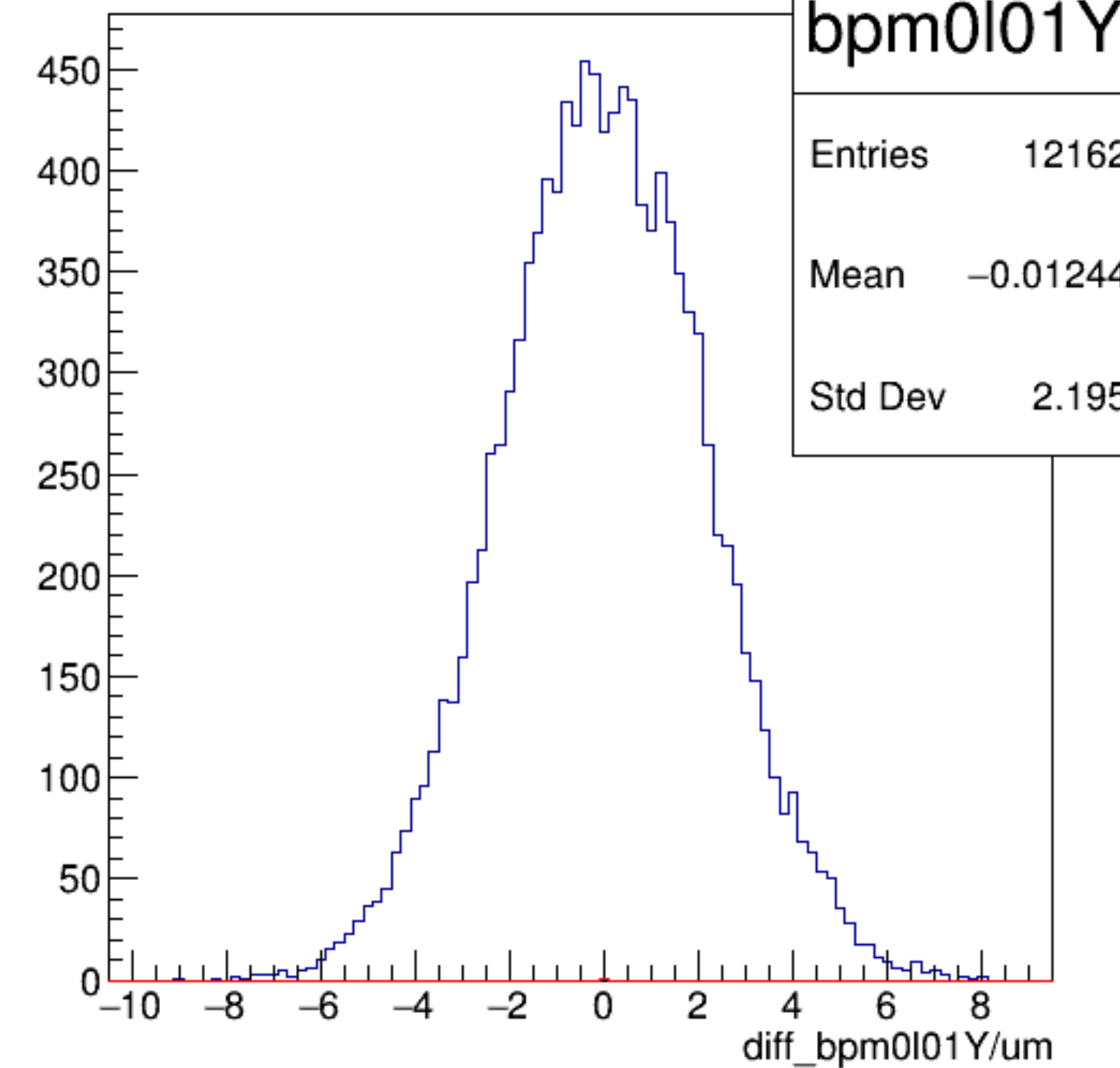
diff_bpm0l01Y/um {ErrorFlag==0}
