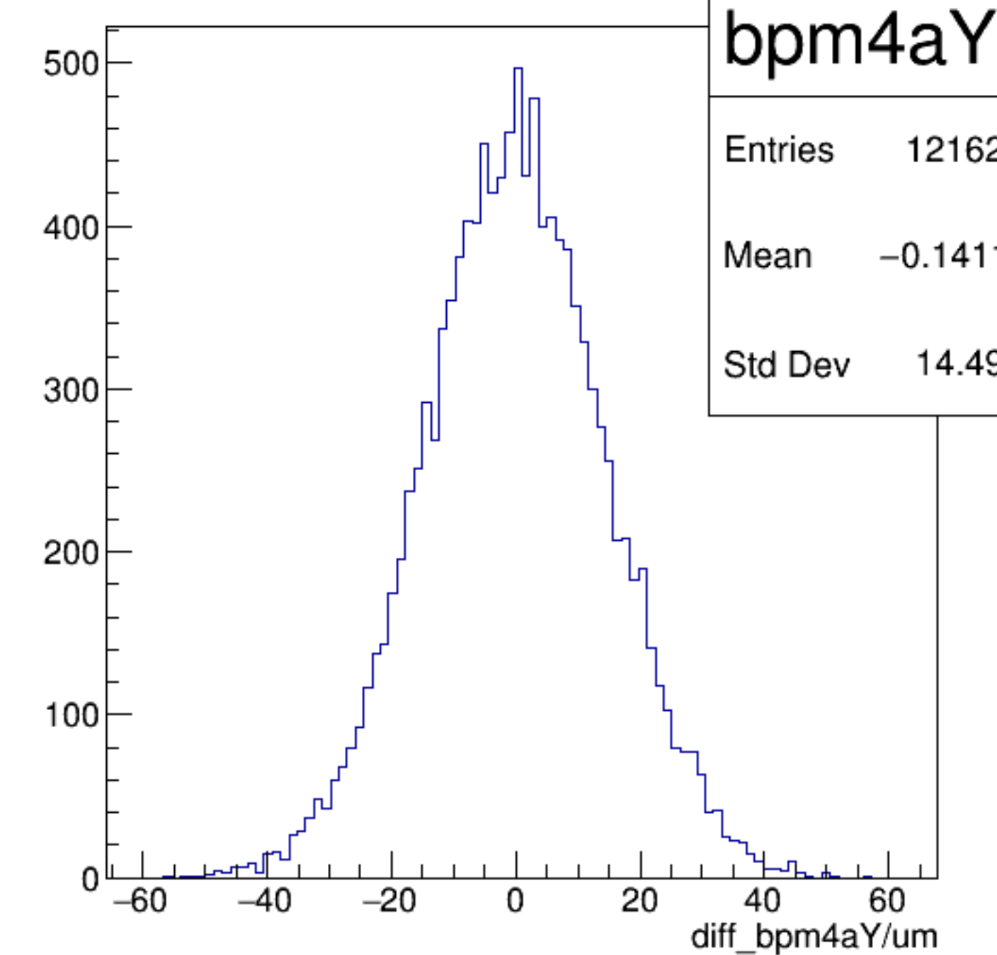
diff_bpm4aY/um {ErrorFlag==0}
