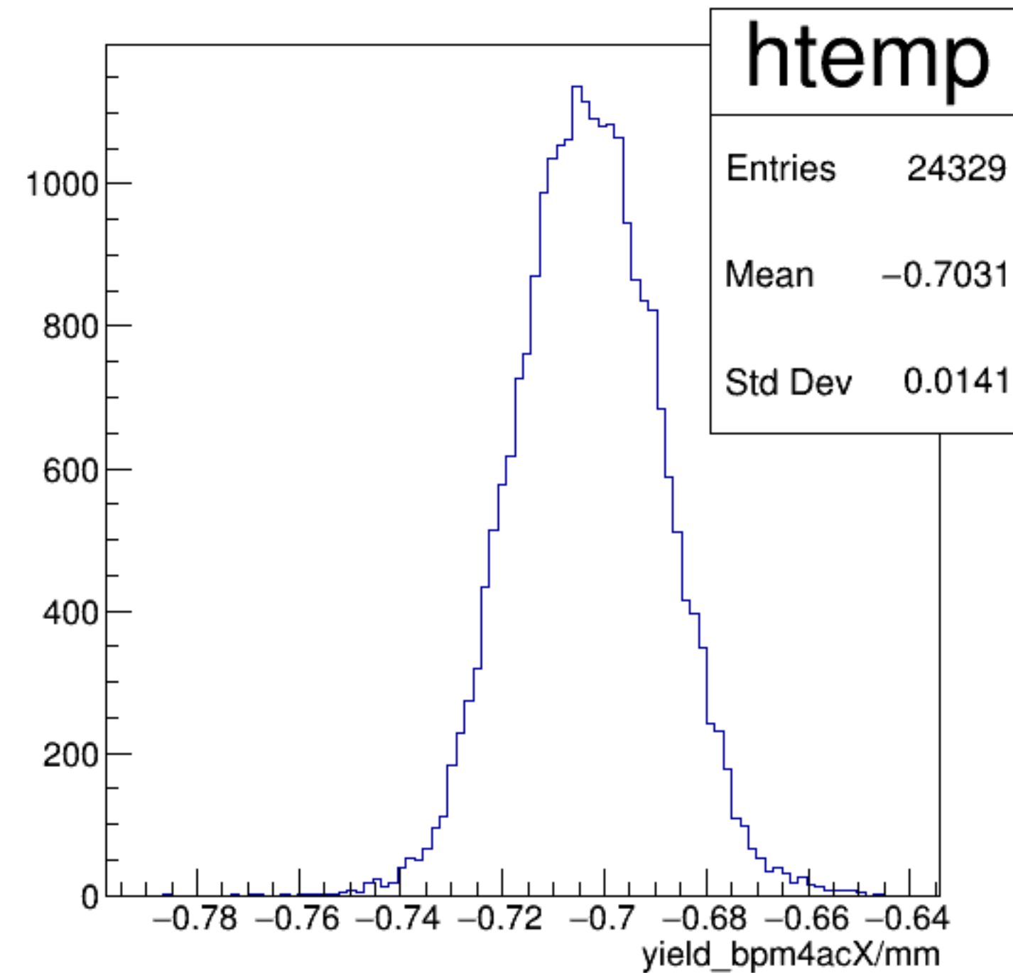
yield_bpm4acX/mm {ErrorFlag==0}
