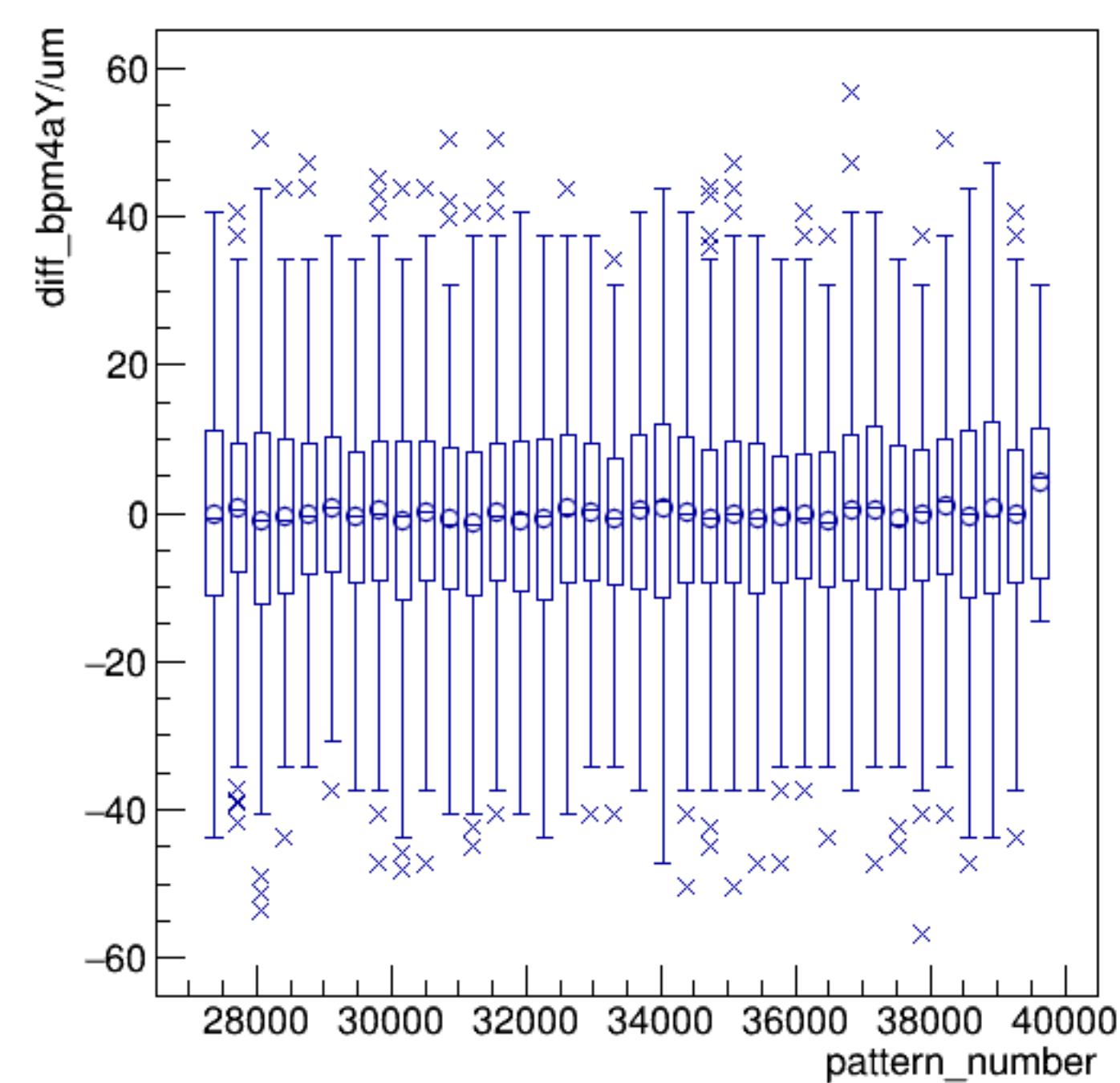
diff_bpm4aY/um:pattern_number {ErrorFlag==0}
