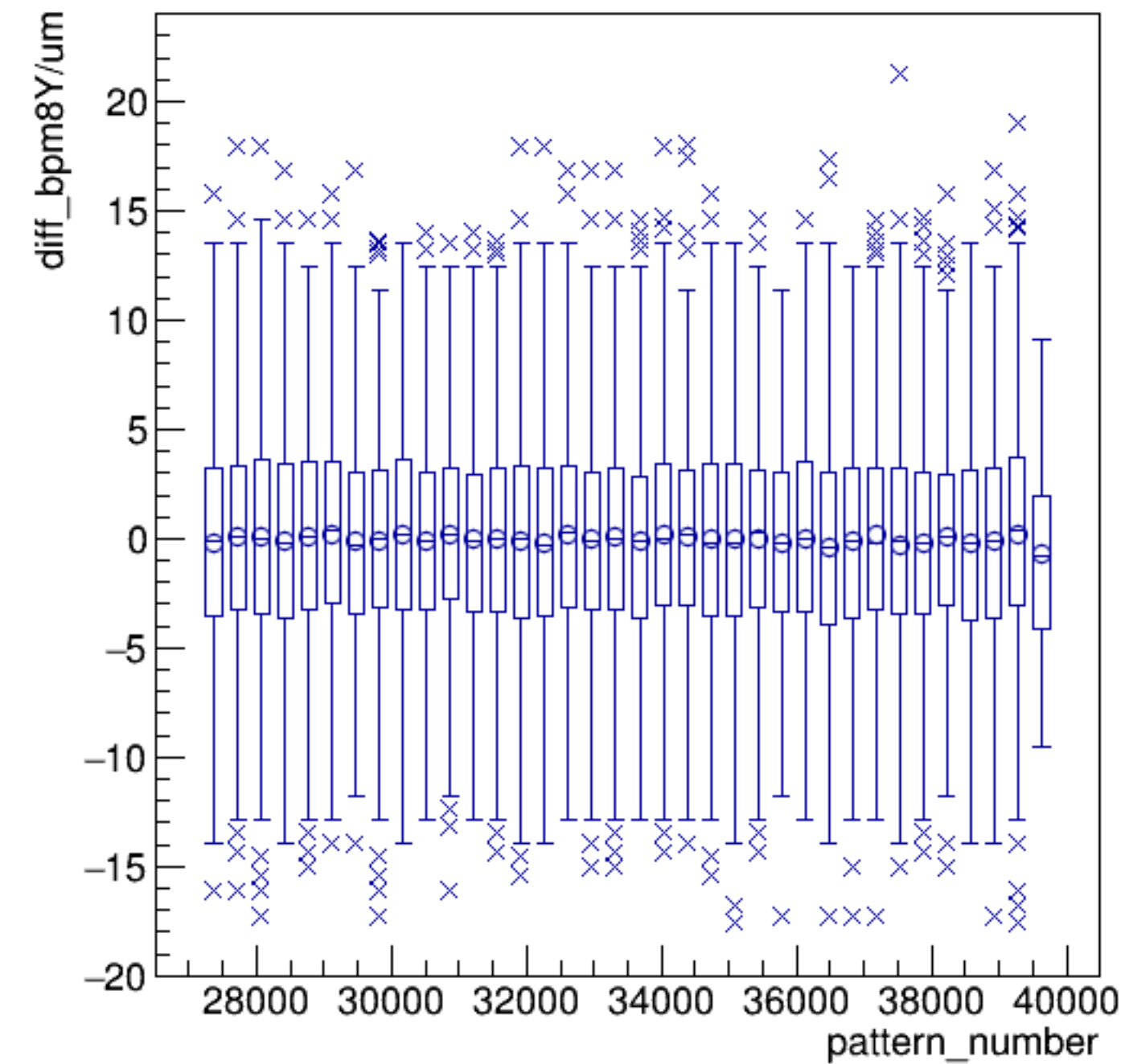
diff_bpm8Y/um:pattern_number {ErrorFlag==0}
