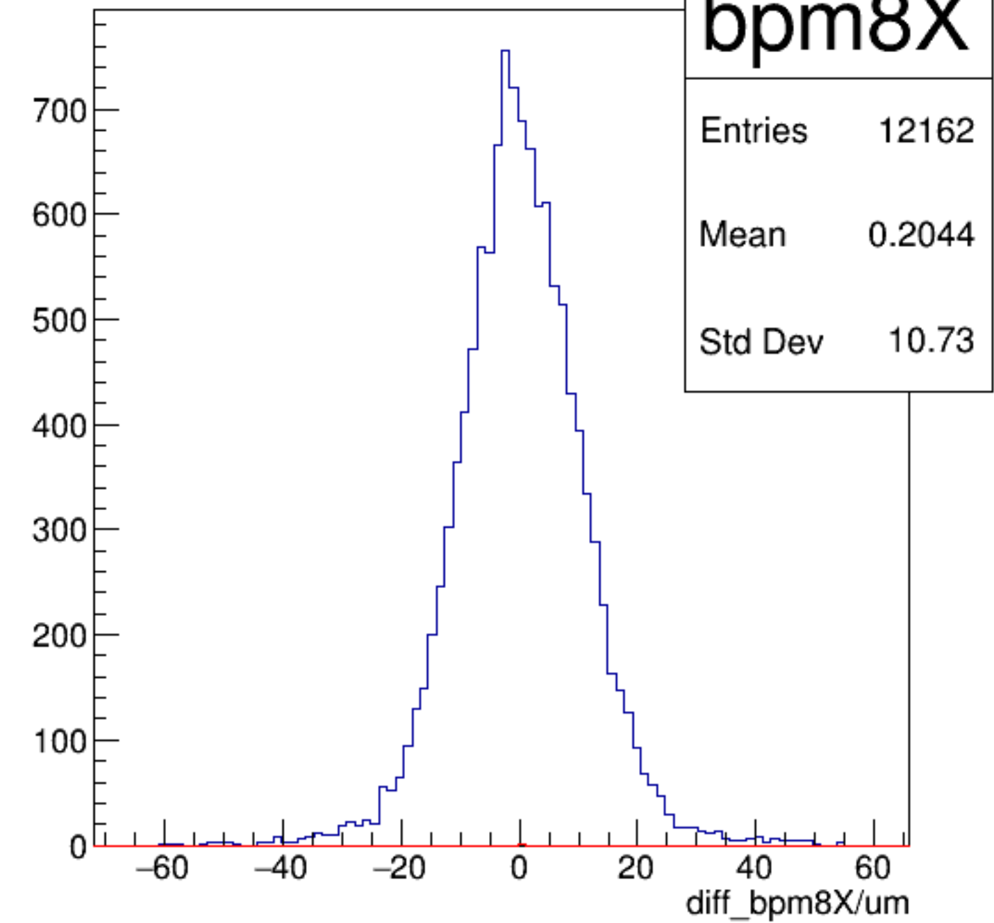
diff_bpm8X/um {ErrorFlag==0}
