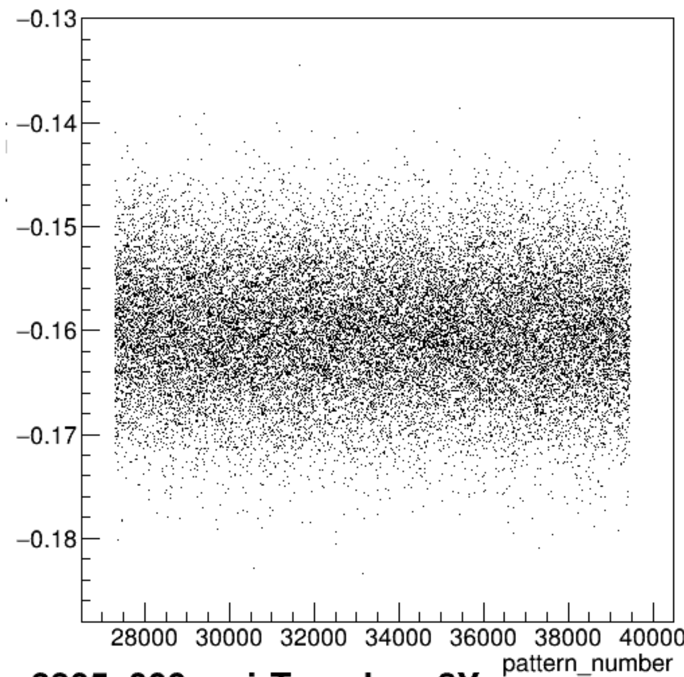
yield_bpm8Y/mm:pattern_number {ErrorFlag==0}
