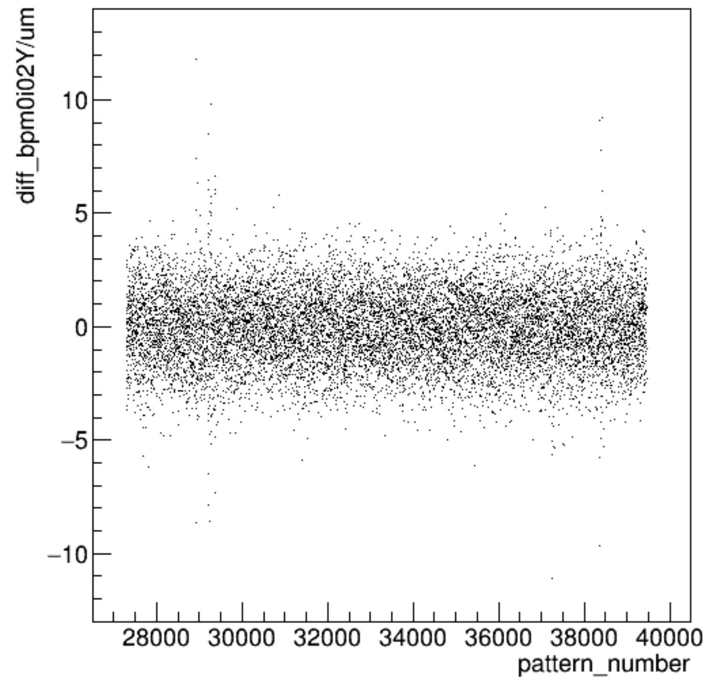
diff_bpm0i02Y/um:pattern_number {ErrorFlag==0}
