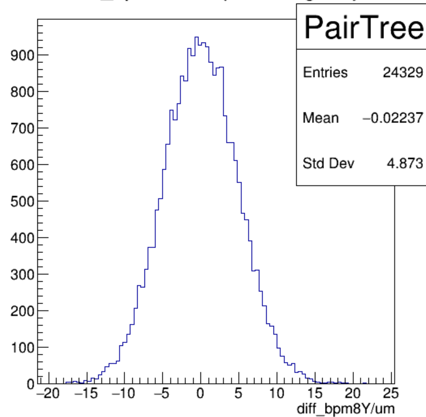
diff_bpm8Y/um {ErrorFlag==0}
