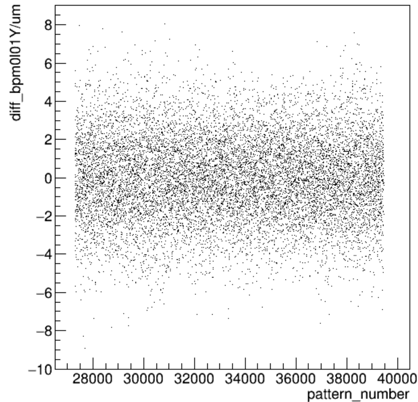
diff_bpm0l01Y/um:pattern_number {ErrorFlag==0}
