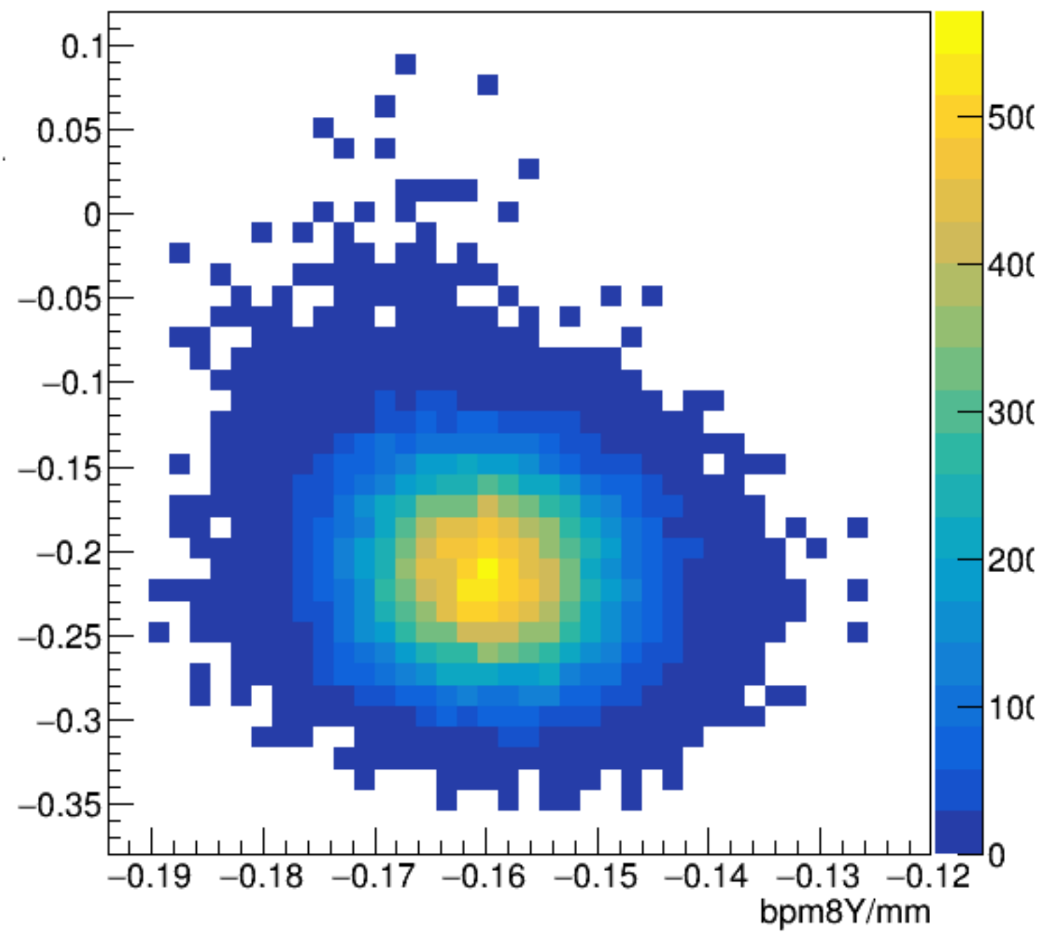
bpm8X/mm:bpm8Y/mm {ErrorFlag==0}
