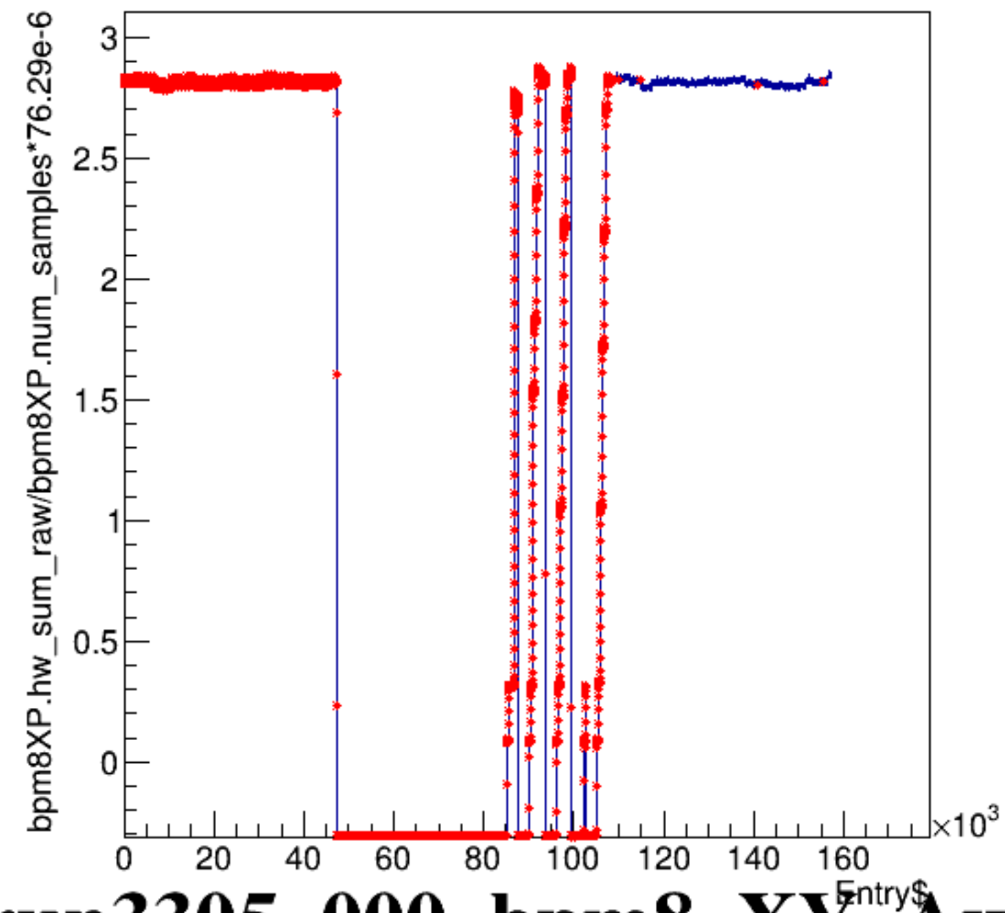
bpm8XP.hw_sum_raw/bpm8XP.num_samples*76.29e-6:Entry$
