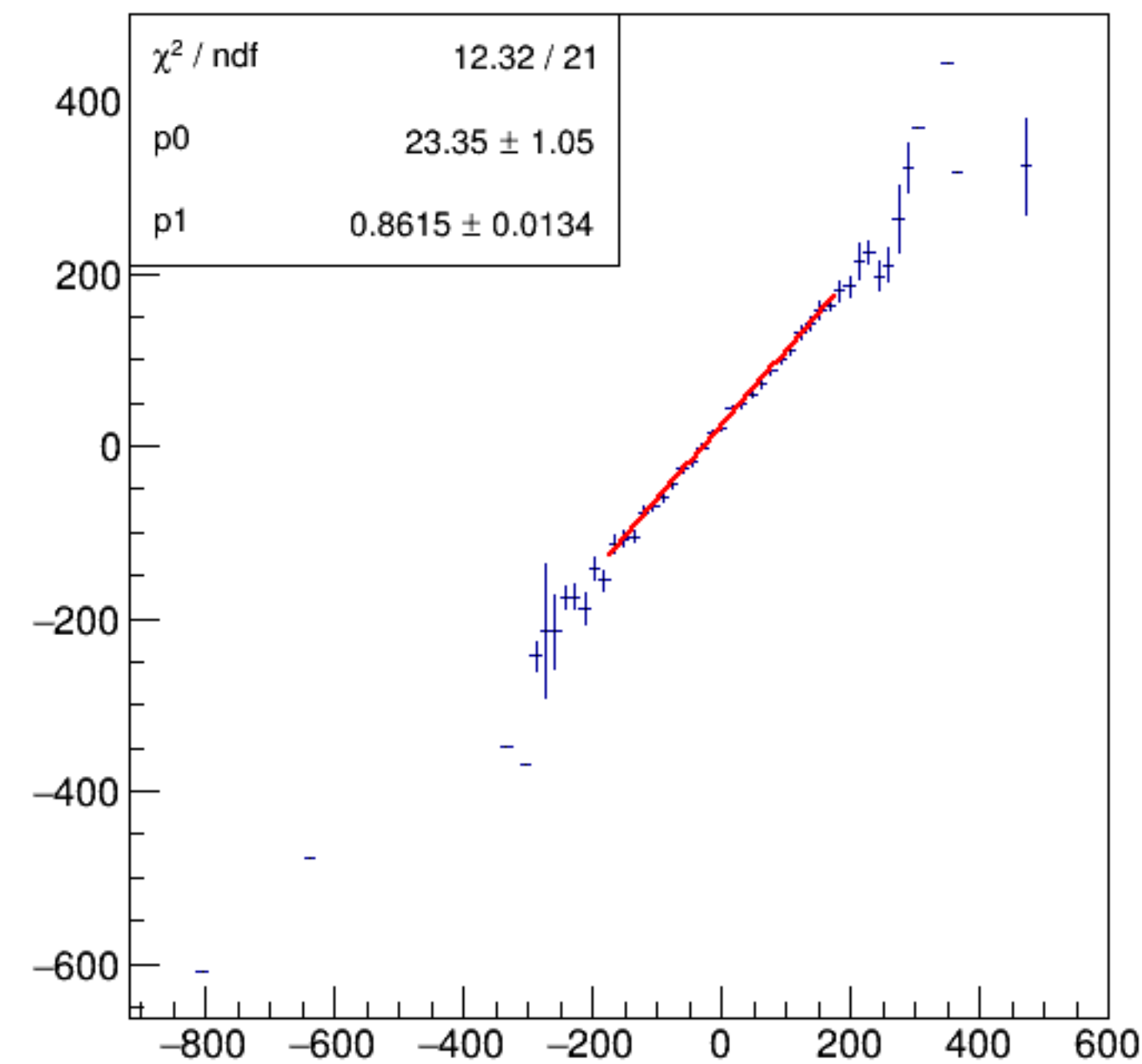
asym_bpm0l01WS/ppm:Aq/ppm {ErrorFlag==0}
