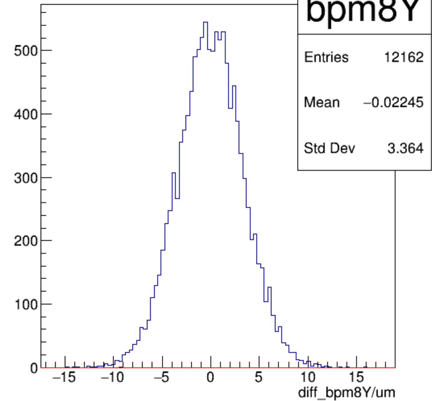
diff_bpm8Y/um {ErrorFlag==0}
