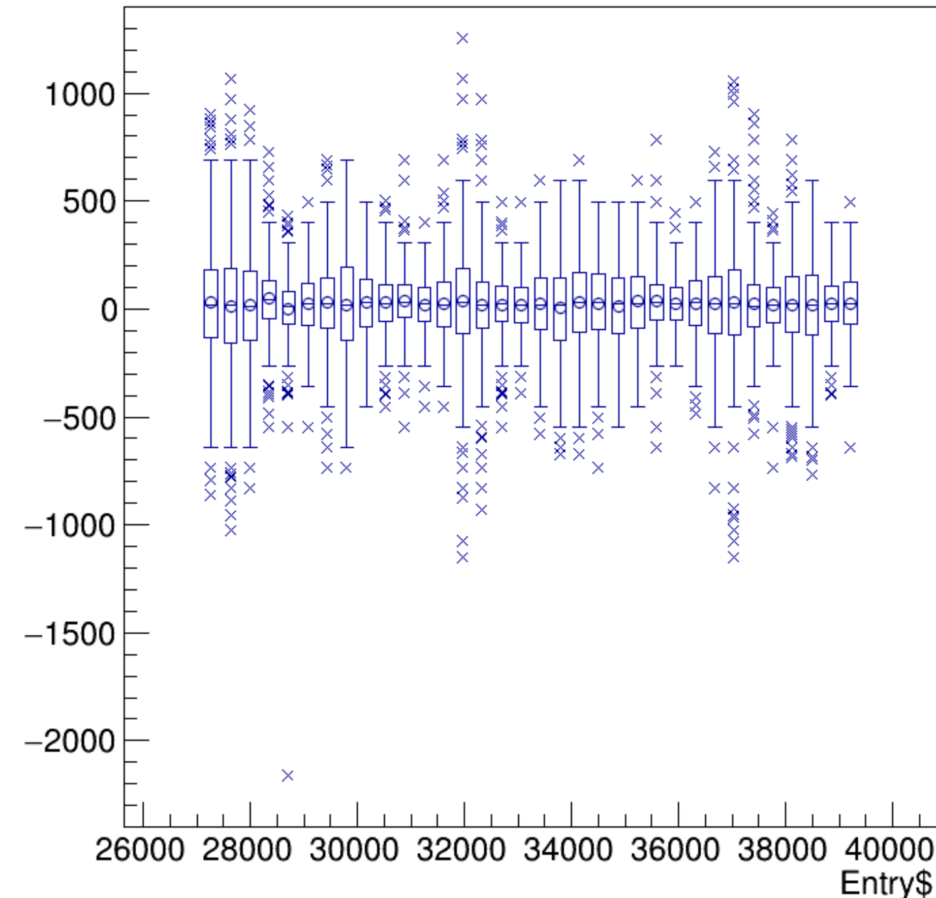
asym_bpm0i07WS/ppm:Entry$ {ErrorFlag==0}
