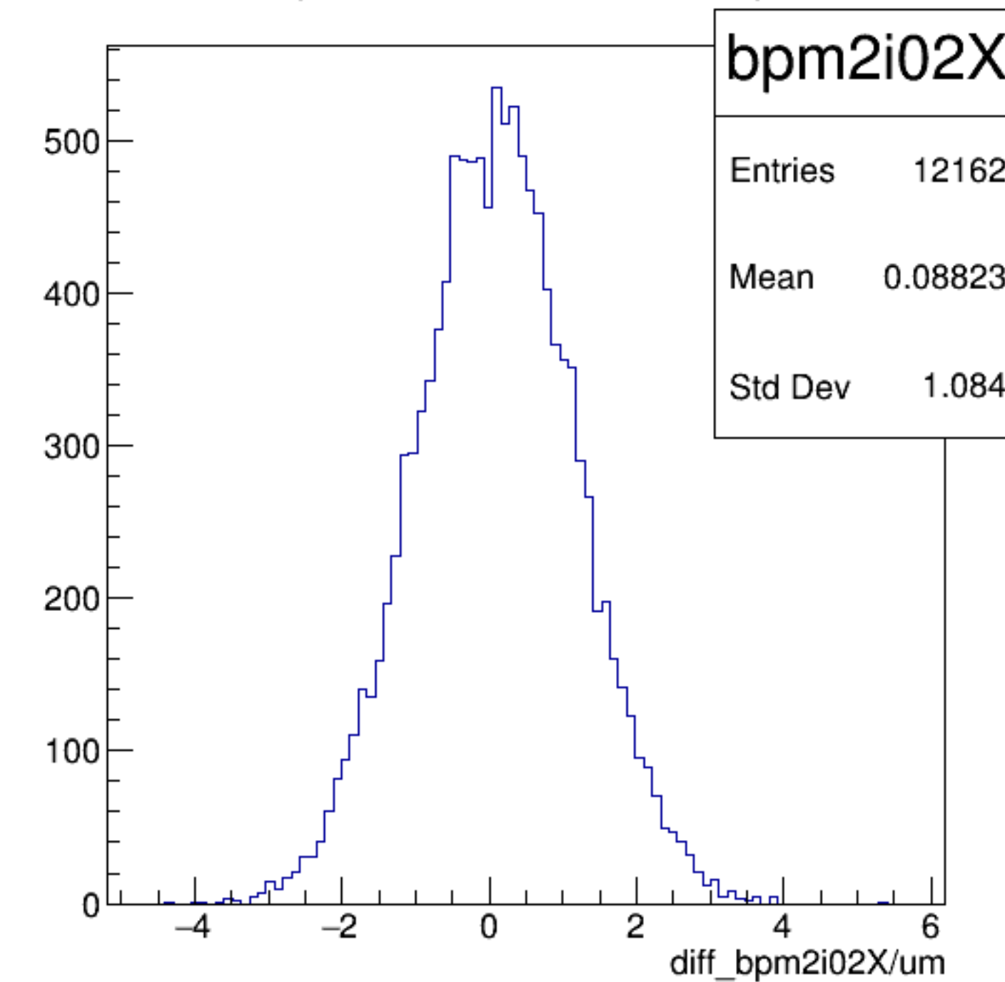
diff_bpm2i02X/um {ErrorFlag==0}
