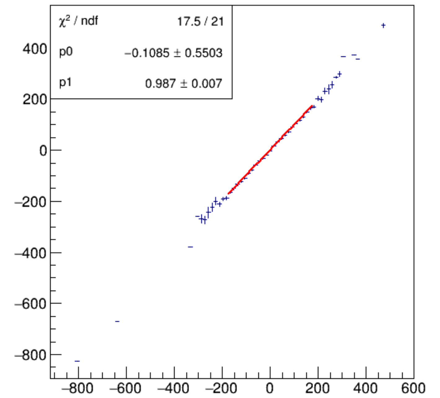
asym_bpm8WS/ppm:Aq/ppm {ErrorFlag==0}
