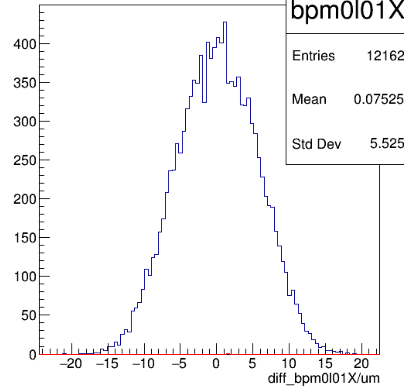
diff_bpm0l01X/um {ErrorFlag==0}
