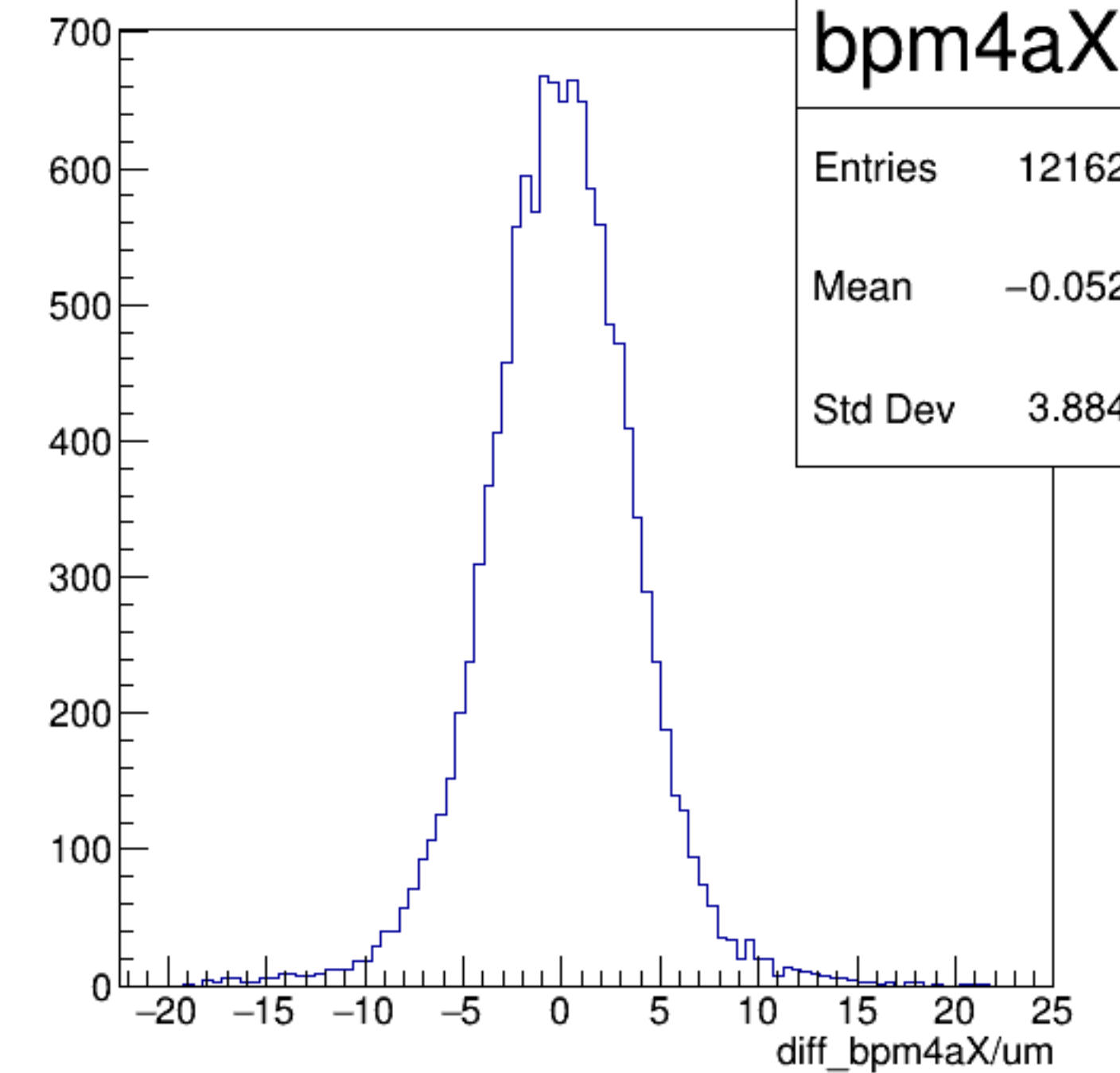
diff_bpm4aX/um {ErrorFlag==0}
