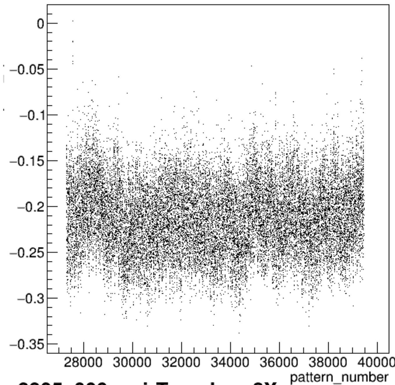
yield_bpm8X/mm:pattern_number {ErrorFlag==0}
