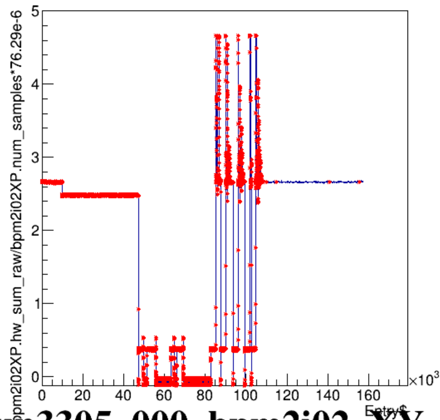
bpm2i02XP.hw_sum_raw/bpm2i02XP.num_samples*76.29e-6:Entry$
