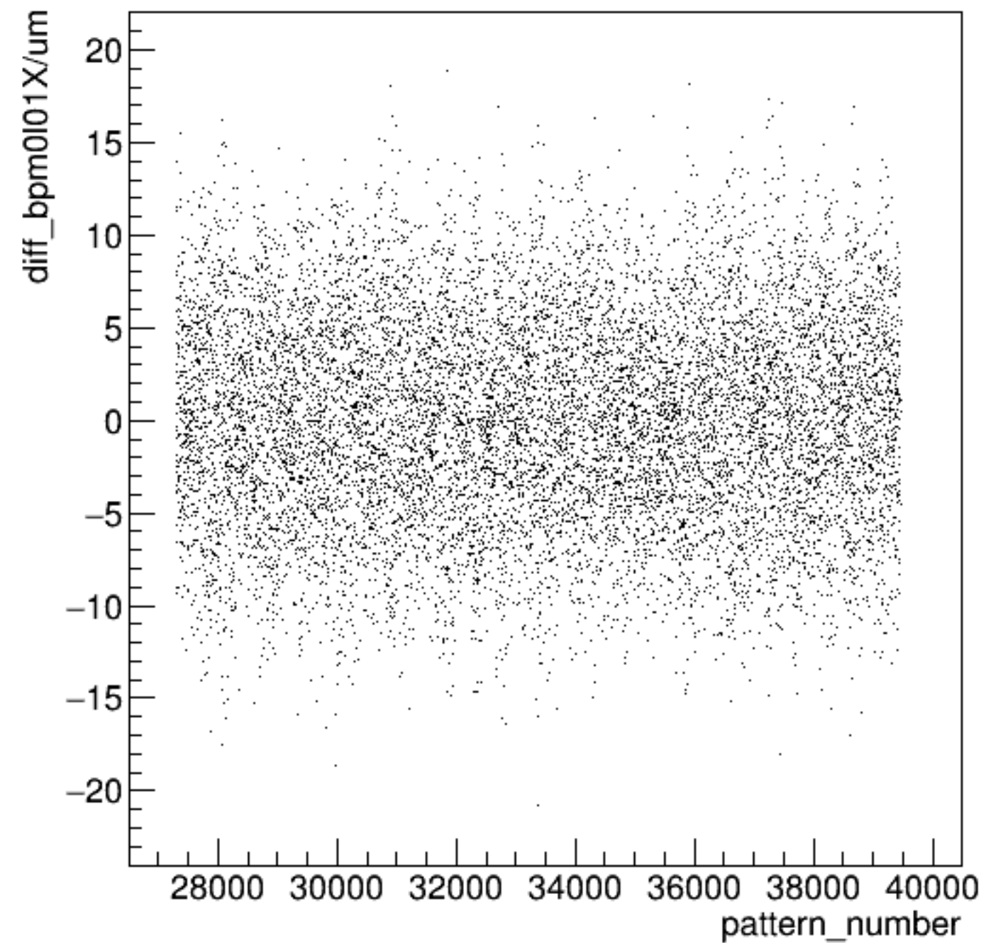
diff_bpm0l01X/um:pattern_number {ErrorFlag==0}
