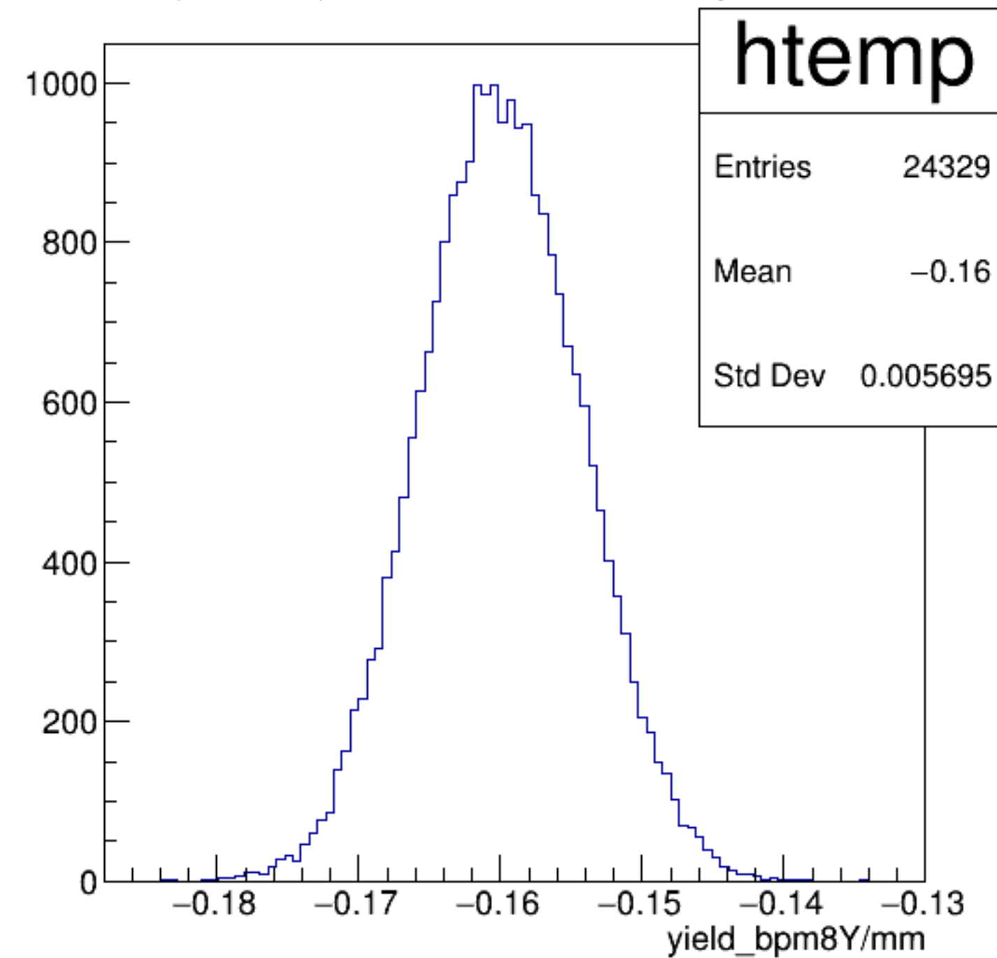
yield_bpm8Y/mm {ErrorFlag==0}
