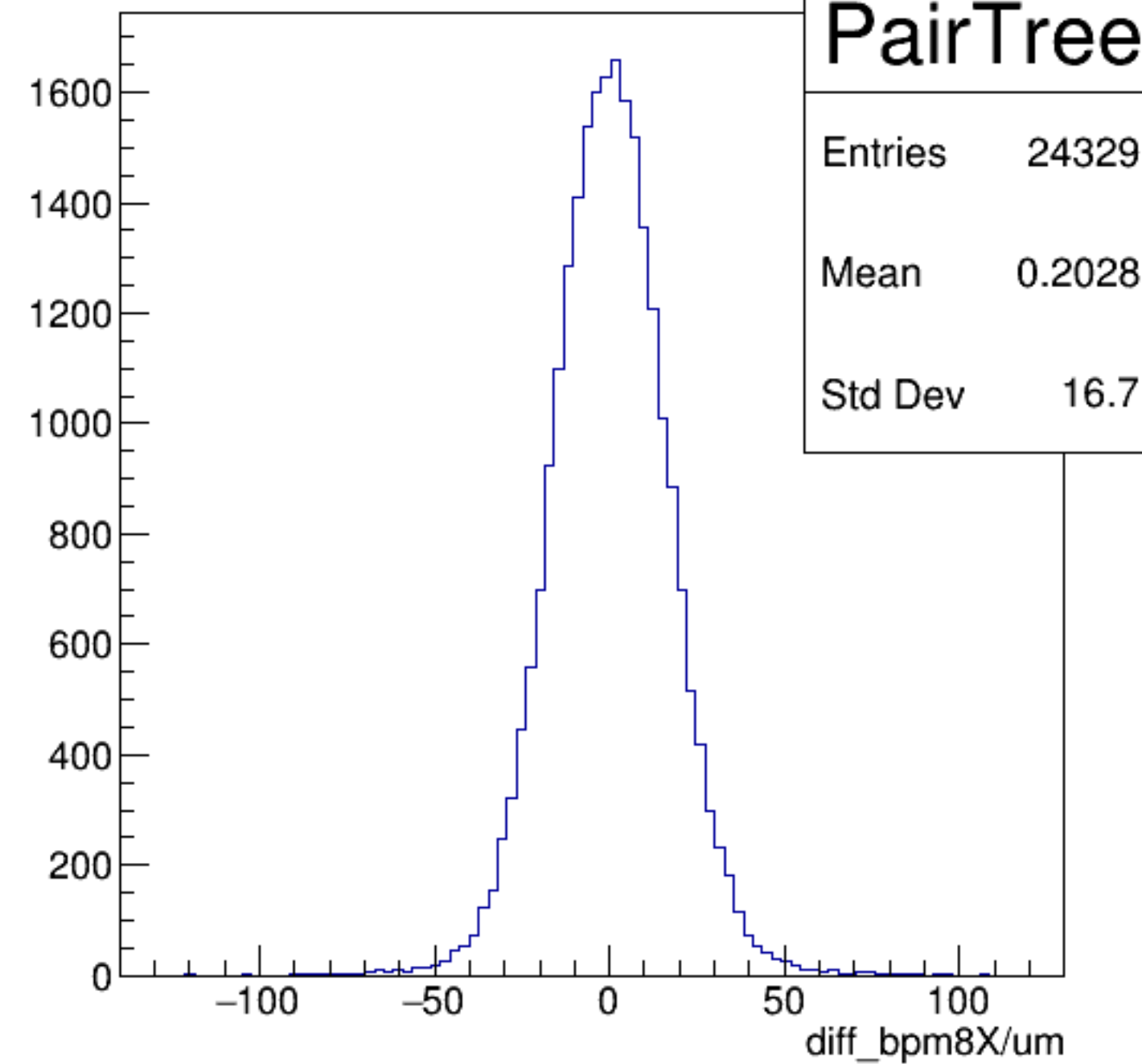
diff_bpm8X/um {ErrorFlag==0}
