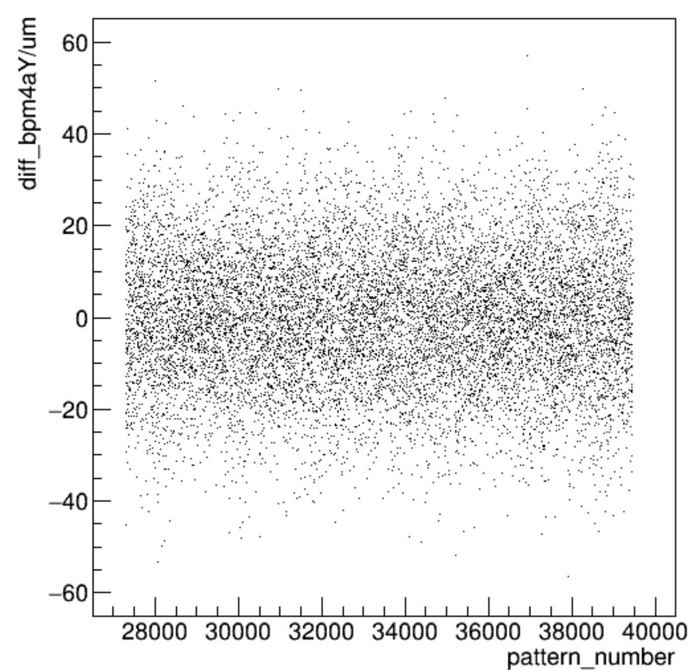
diff_bpm4aY/um:pattern_number {ErrorFlag==0}
