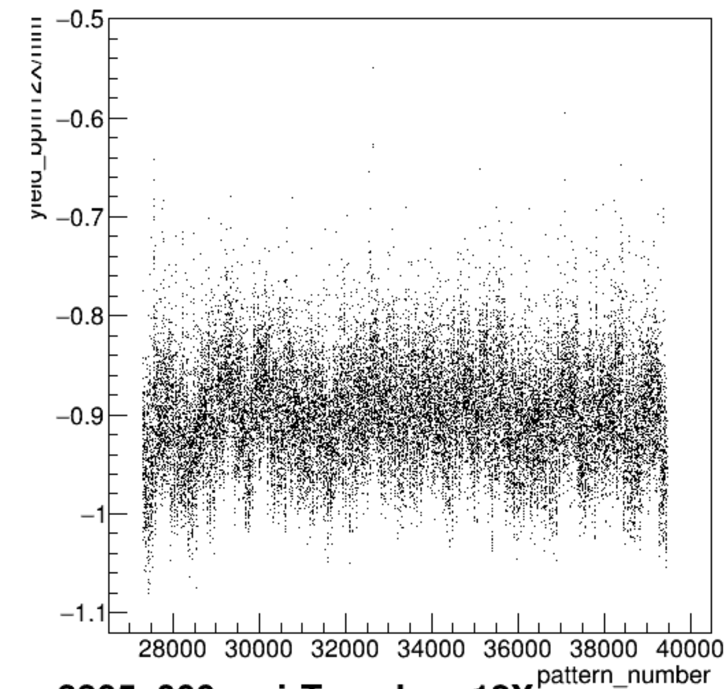
yield_bpm12X/mm:pattern_number {ErrorFlag==0}
