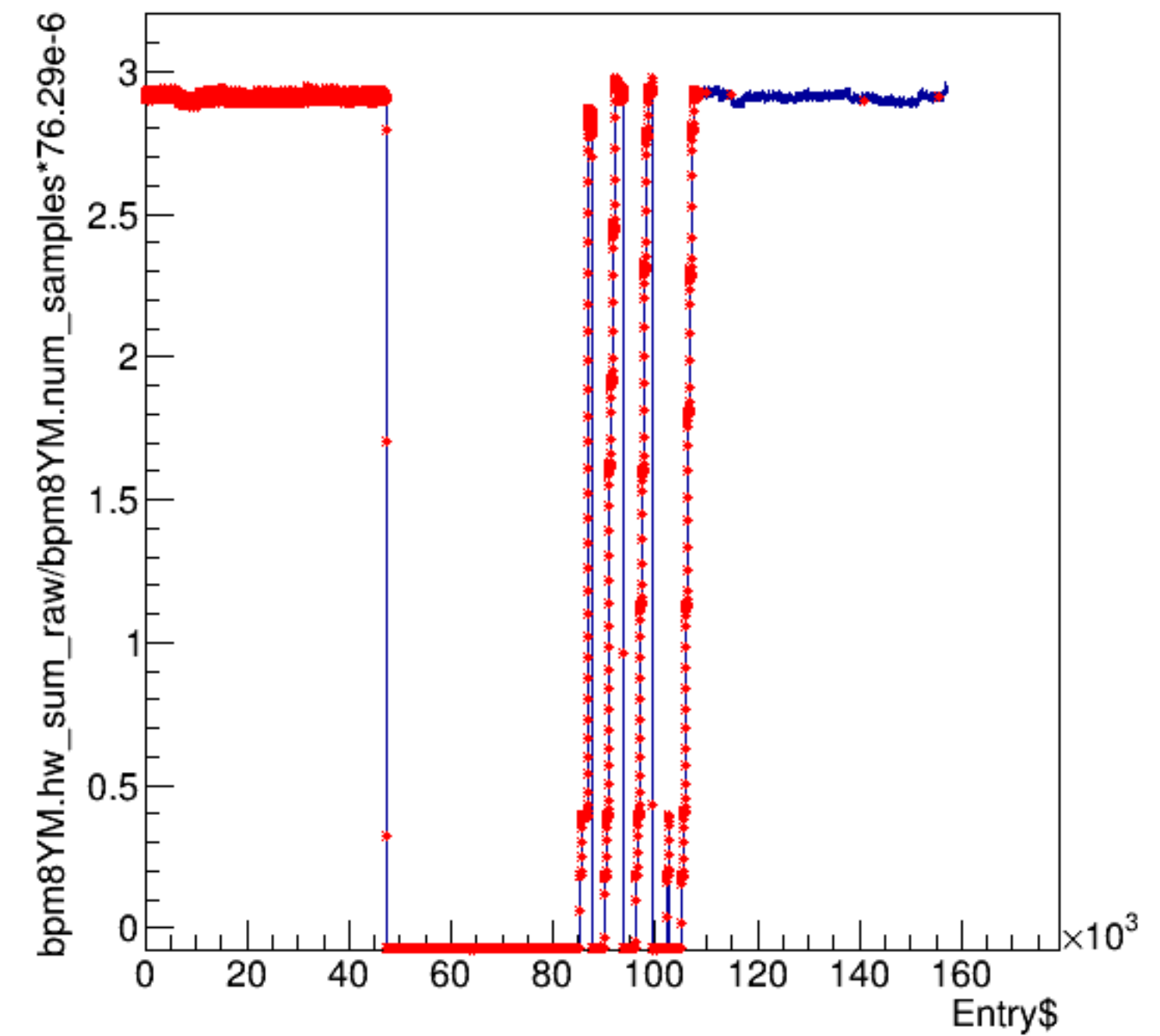
bpm8YM.hw_sum_raw/bpm8YM.num_samples*76.29e-6:Entry$
