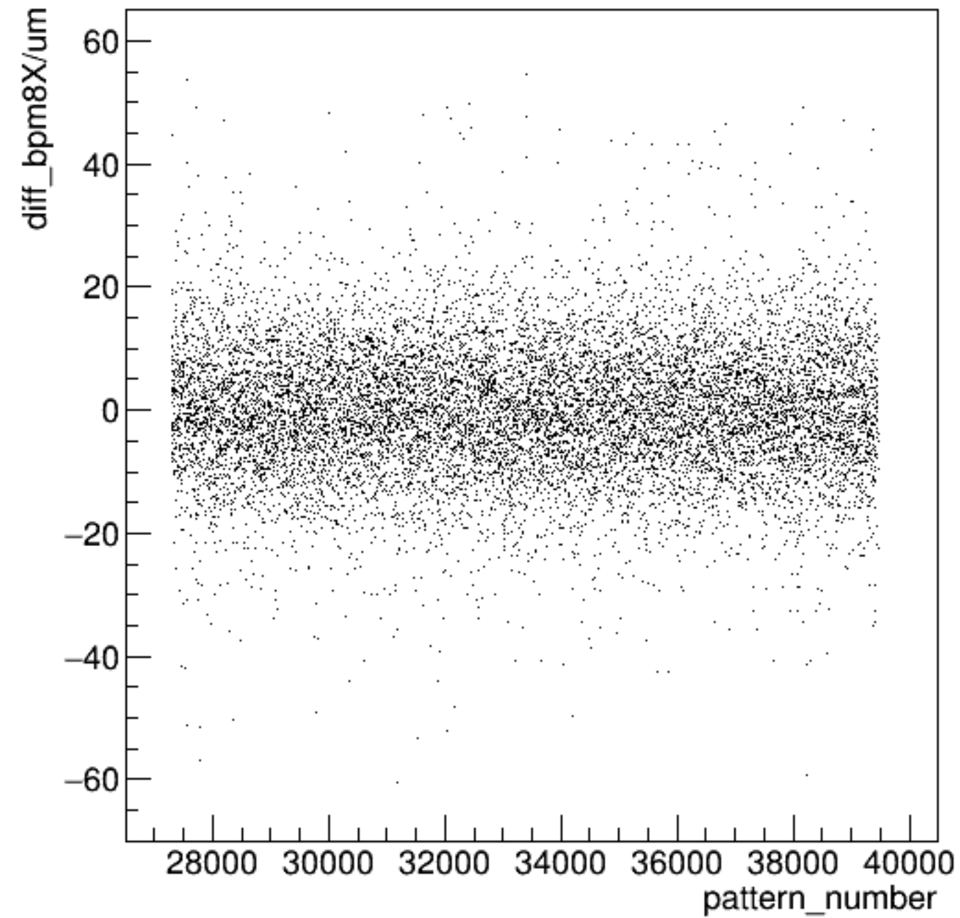
diff_bpm8X/um:pattern_number {ErrorFlag==0}
