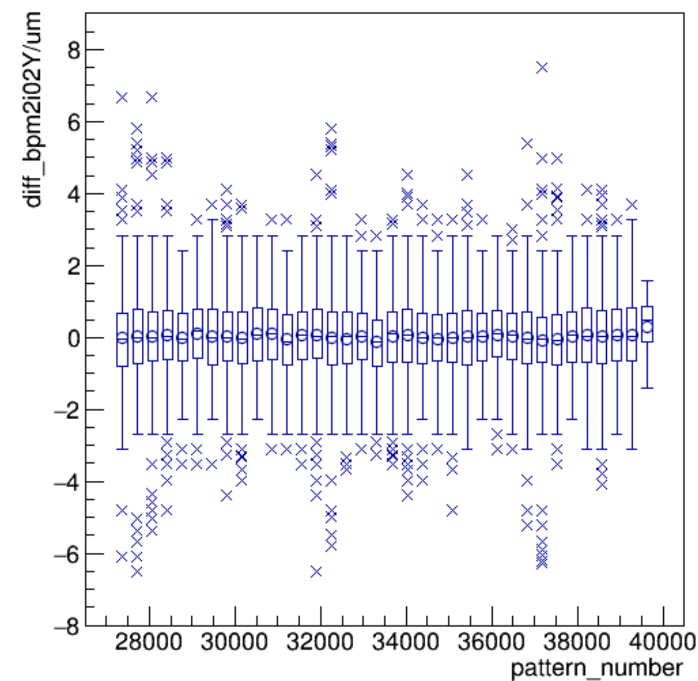
diff_bpm2i02Y/um:pattern_number {ErrorFlag==0}
