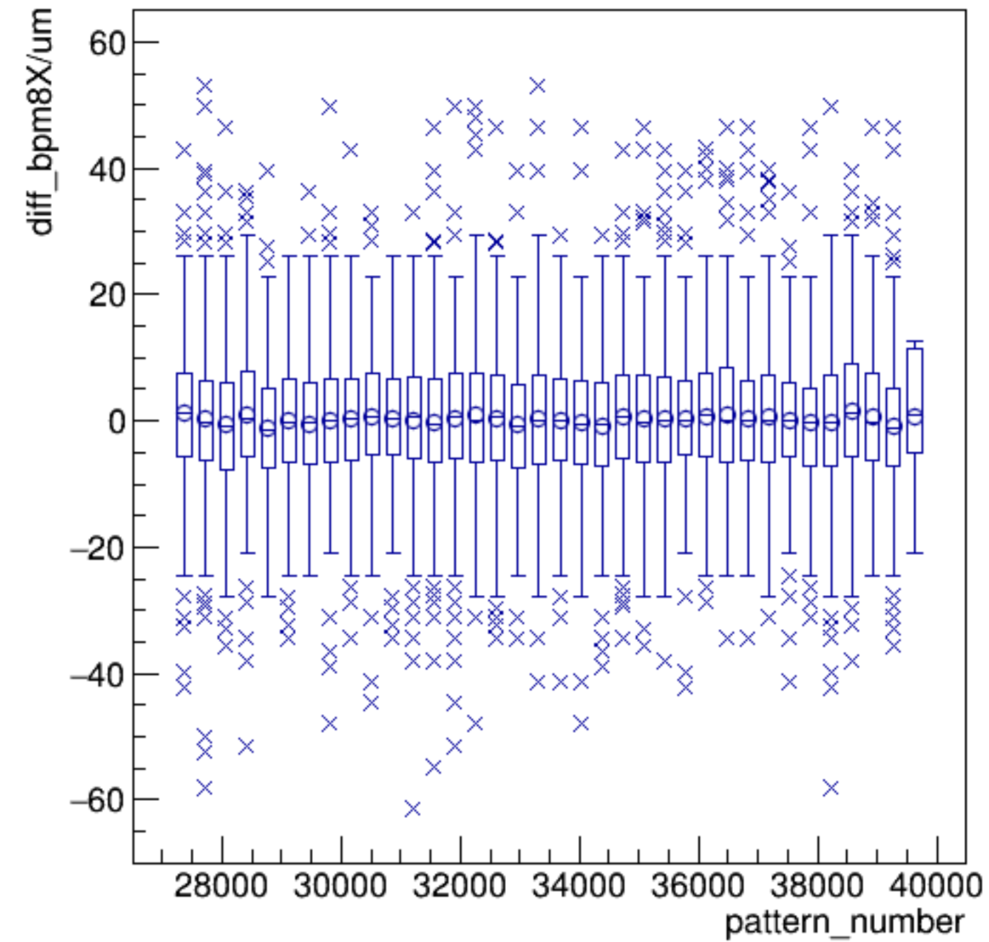
diff_bpm8X/um:pattern_number {ErrorFlag==0}
