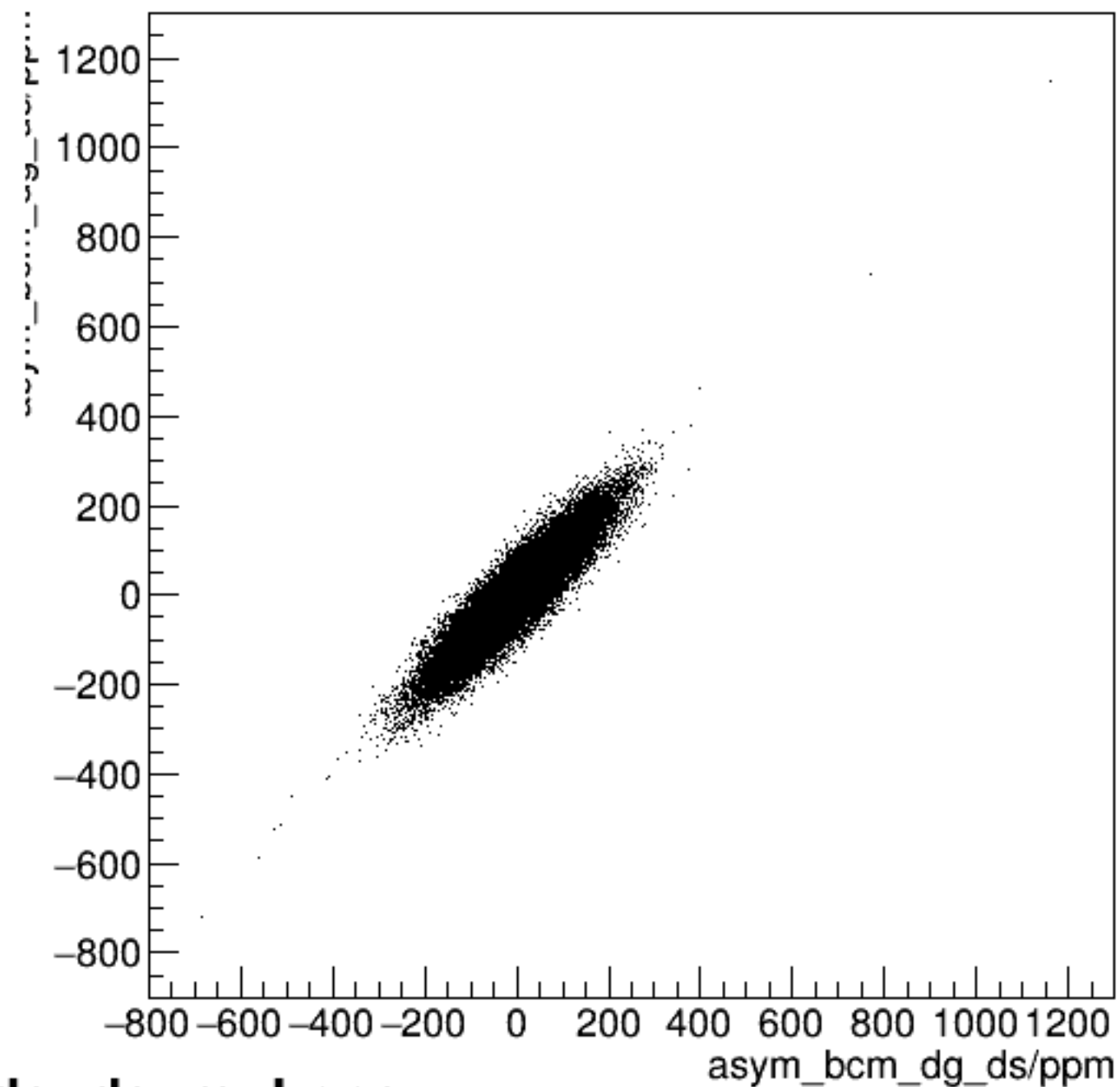
run3308_000_asym_bcm_dg_us_vs_asym_bcm_dg_ds_mul.png
