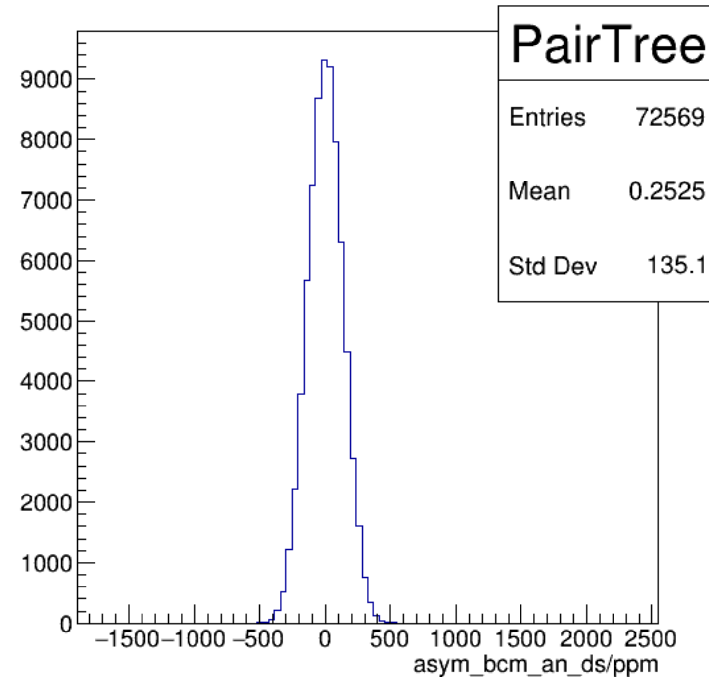
asym_bcm_an_ds/ppm {ErrorFlag==0}
