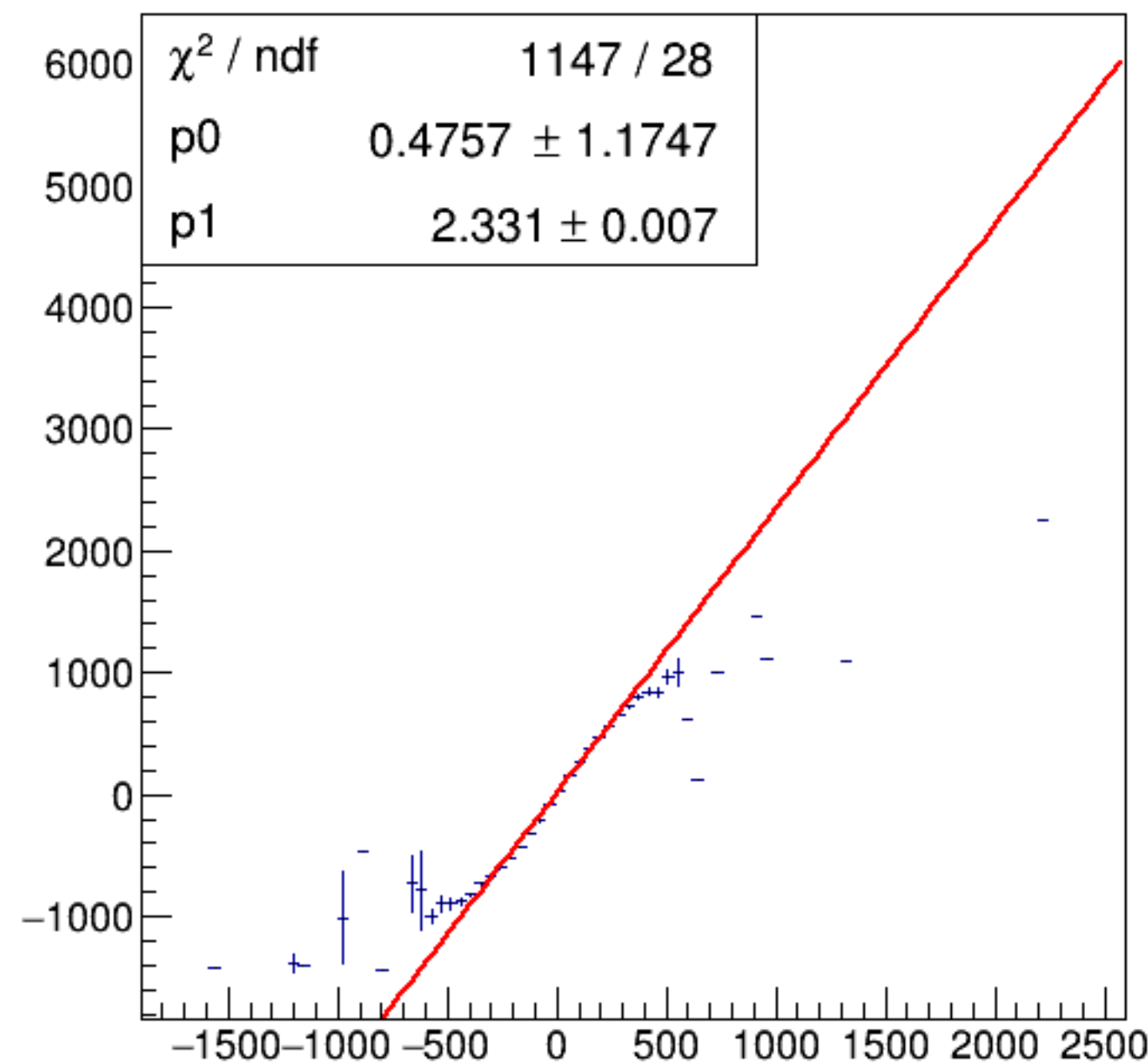
run3308_000_asym_bcm_dg_us_vs_asym_bcm_an_ds3_pr.png
