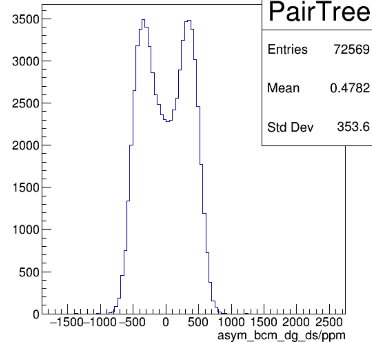
asym_bcm_dg_ds/ppm {ErrorFlag==0}
