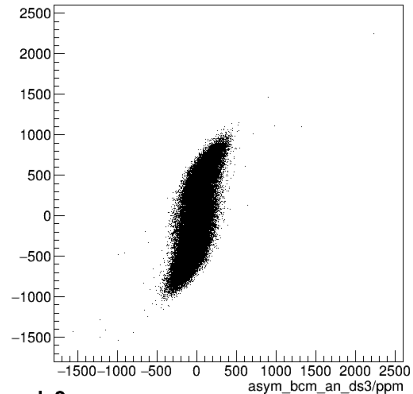
run3308_000_asym_bcm_dg_us_vs_asym_bcm_an_ds3_pr.png
