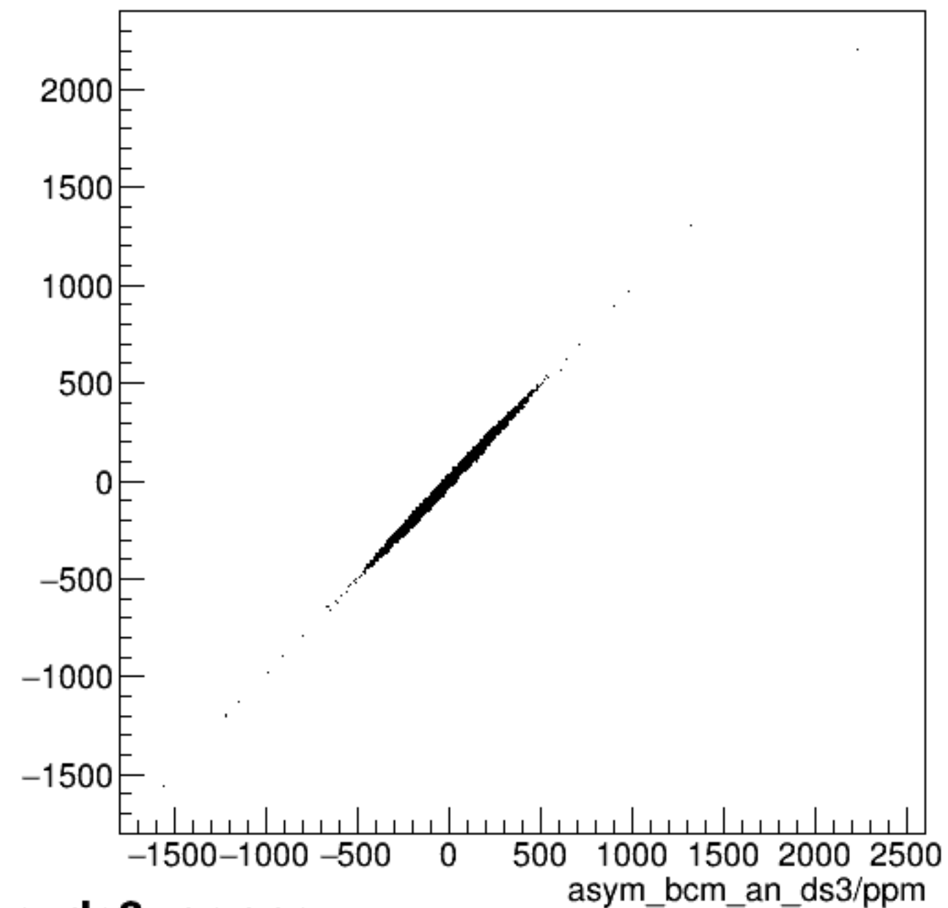
run3308_000_asym_bcm_an_ds_vs_asym_bcm_an_ds3_pr.png
