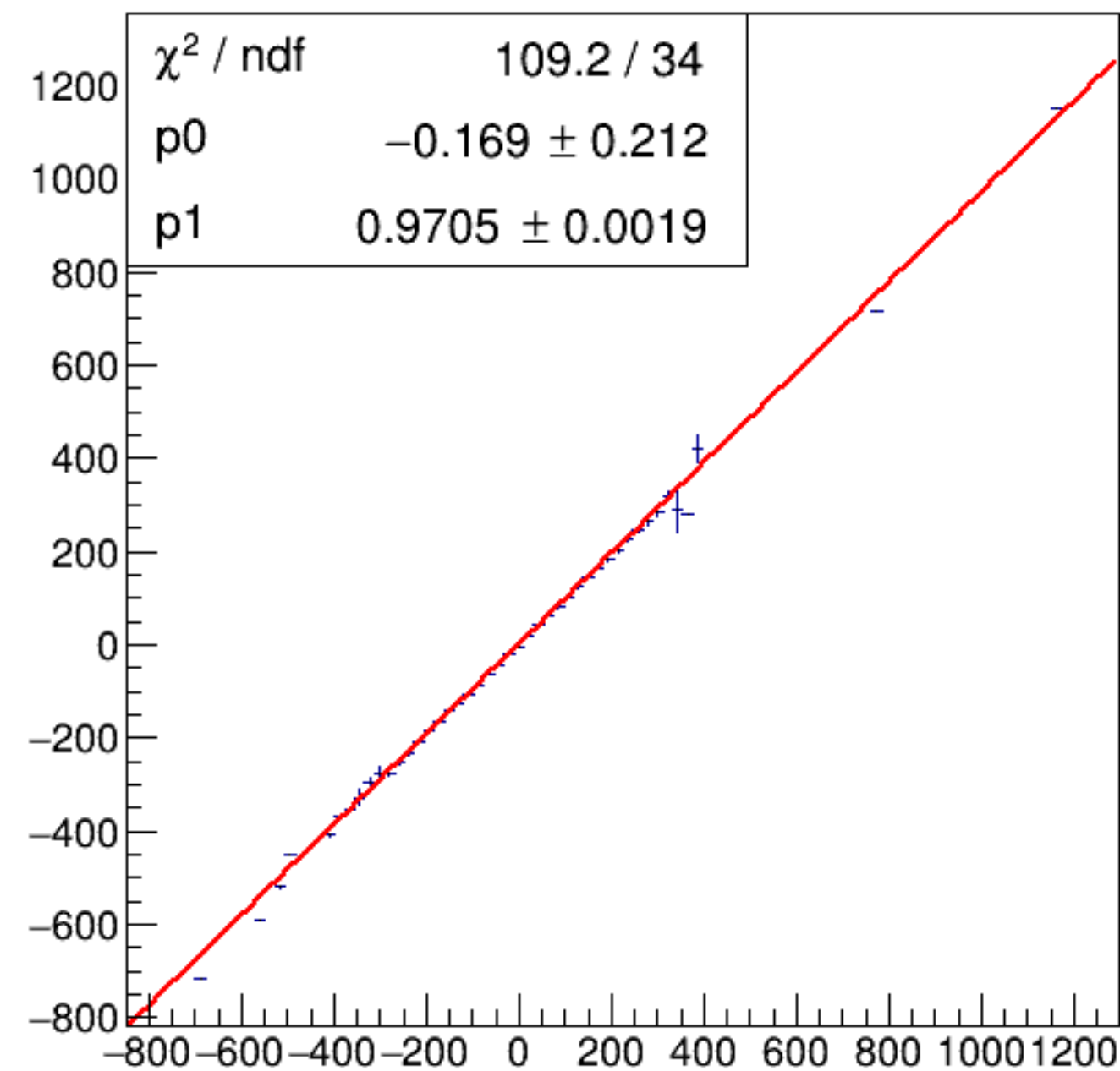
run3308_000_asym_bcm_dg_us_vs_asym_bcm_dg_ds_mul.png
