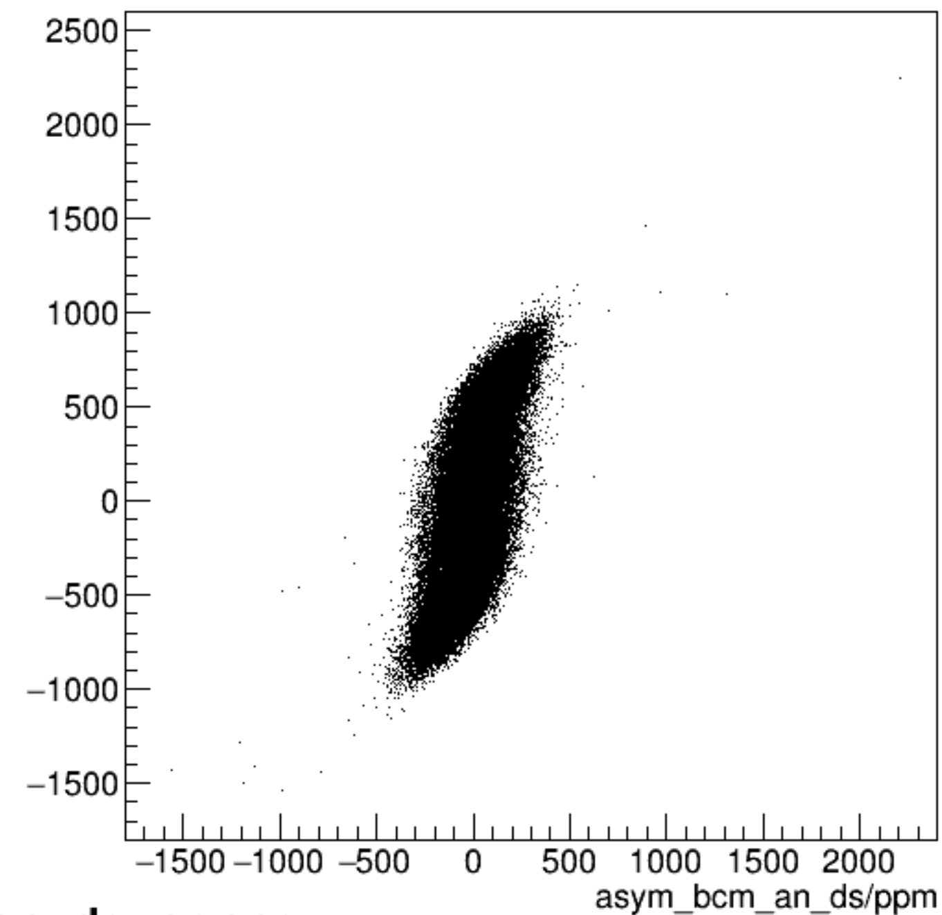
run3308_000_asym_bcm_dg_us_vs_asym_bcm_an_ds_pr.png
