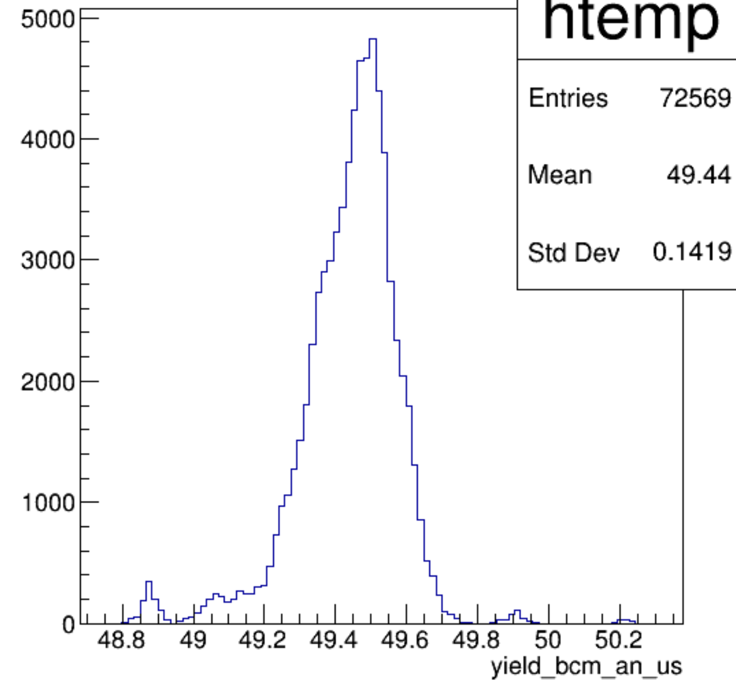
yield_bcm_an_us {ErrorFlag==0}
