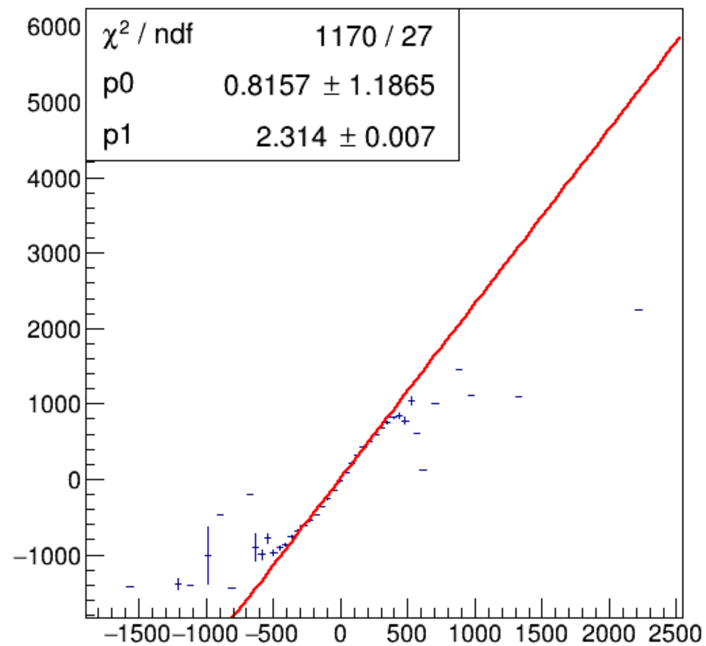
run3308_000_asym_bcm_dg_us_vs_asym_bcm_an_ds_pr.png
