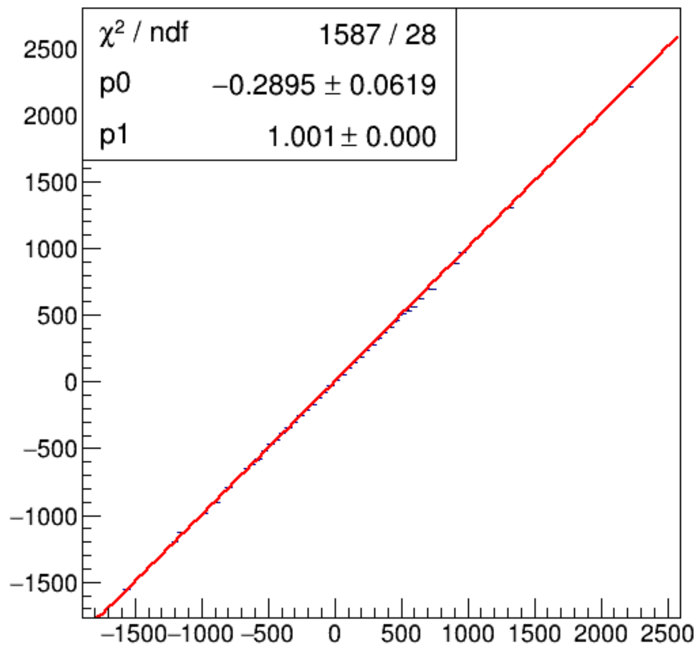
run3308_000_asym_bcm_an_ds_vs_asym_bcm_an_ds3_pr.png
