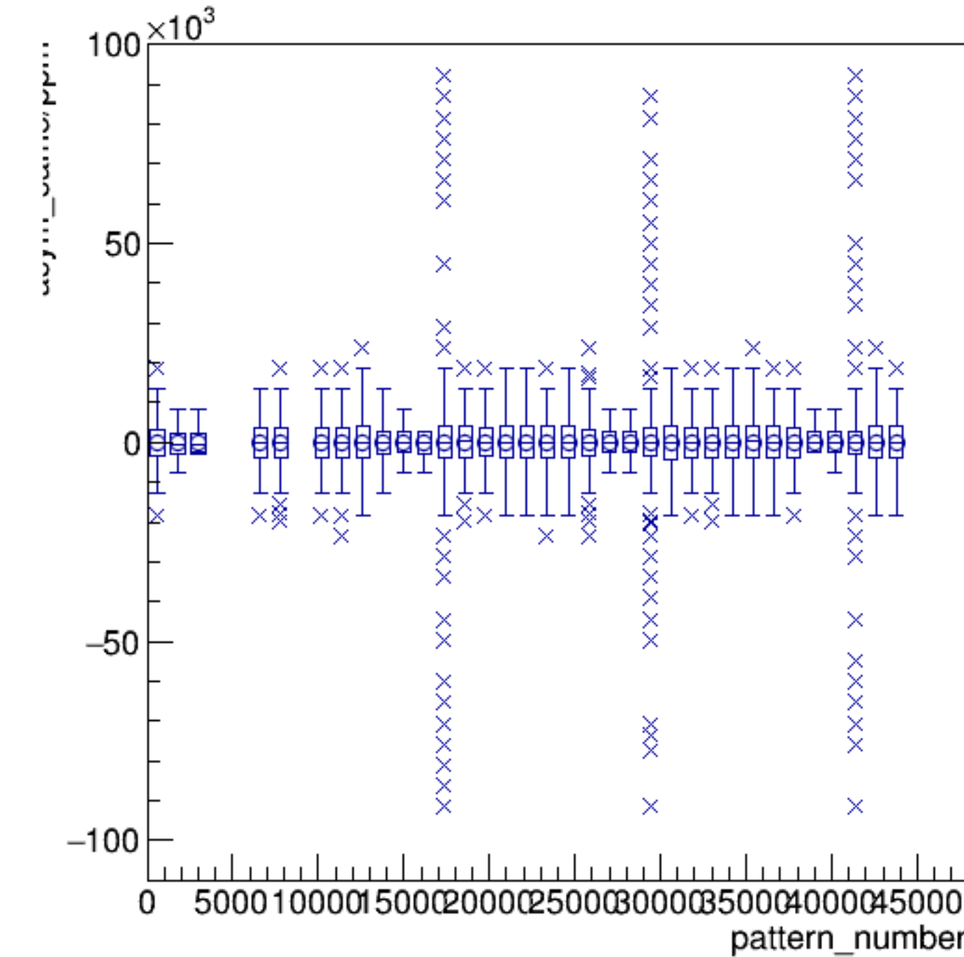
asym_sam5/ppm:pattern_number {ErrorFlag==0}
