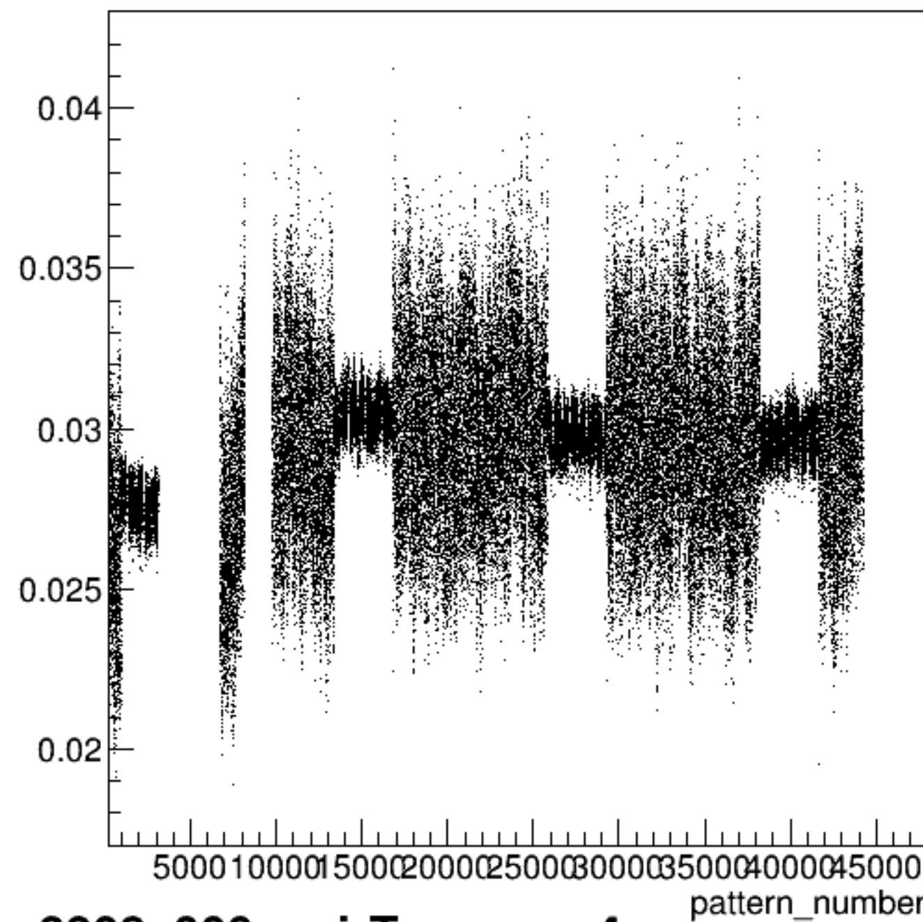
yield_sam4:pattern_number {ErrorFlag==0}
