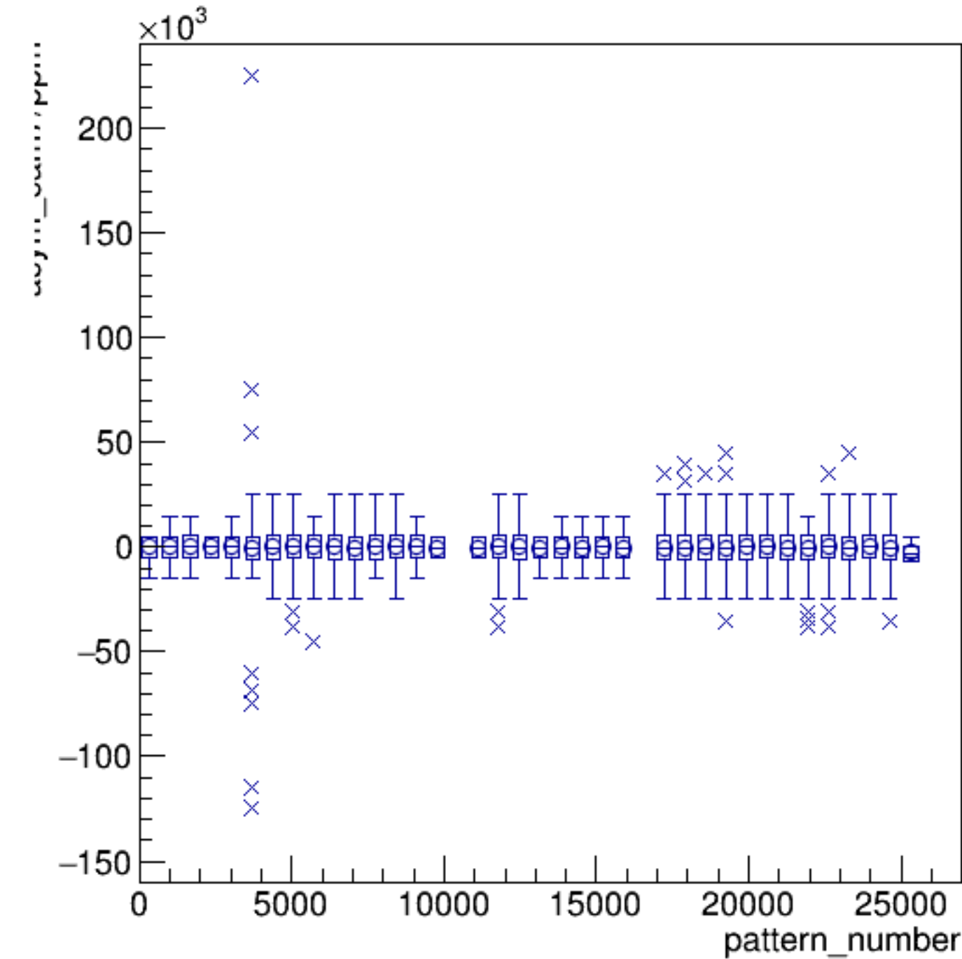
asym_sam7/ppm:pattern_number {ErrorFlag==0}
