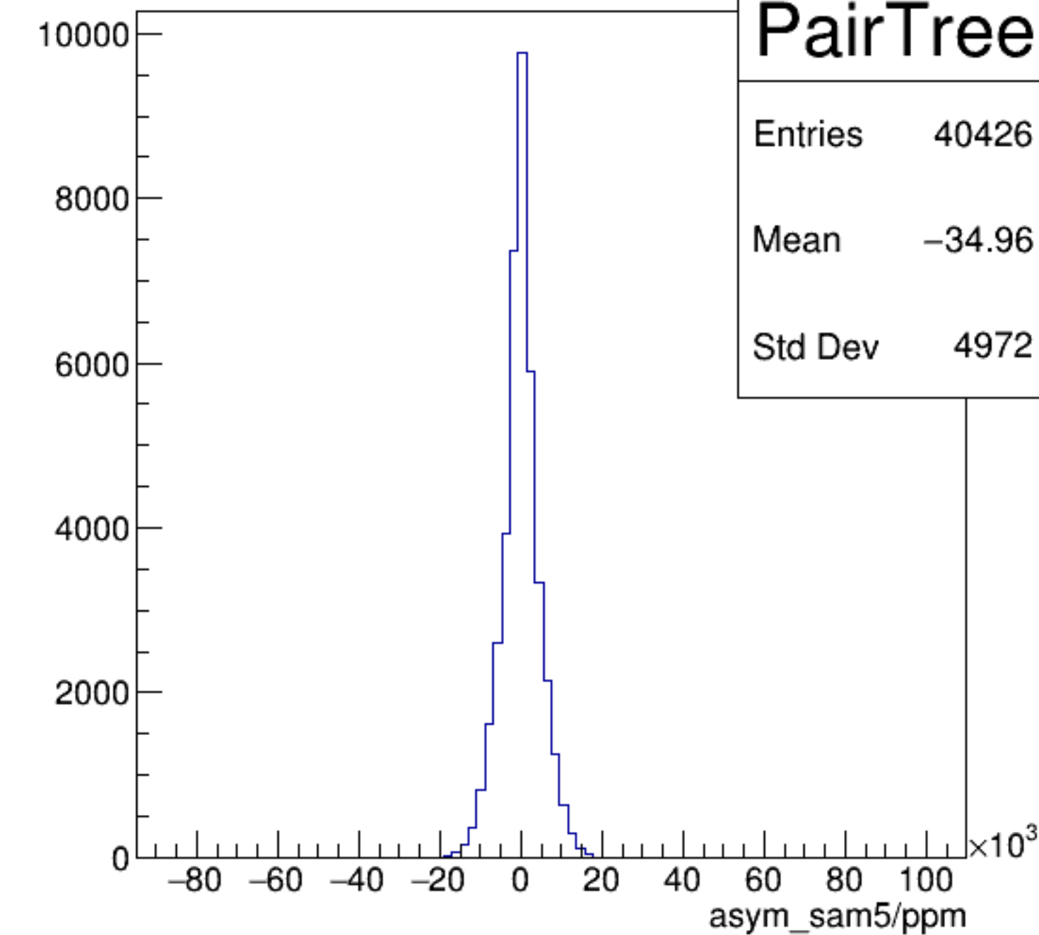
asym_sam5/ppm {ErrorFlag==0}
