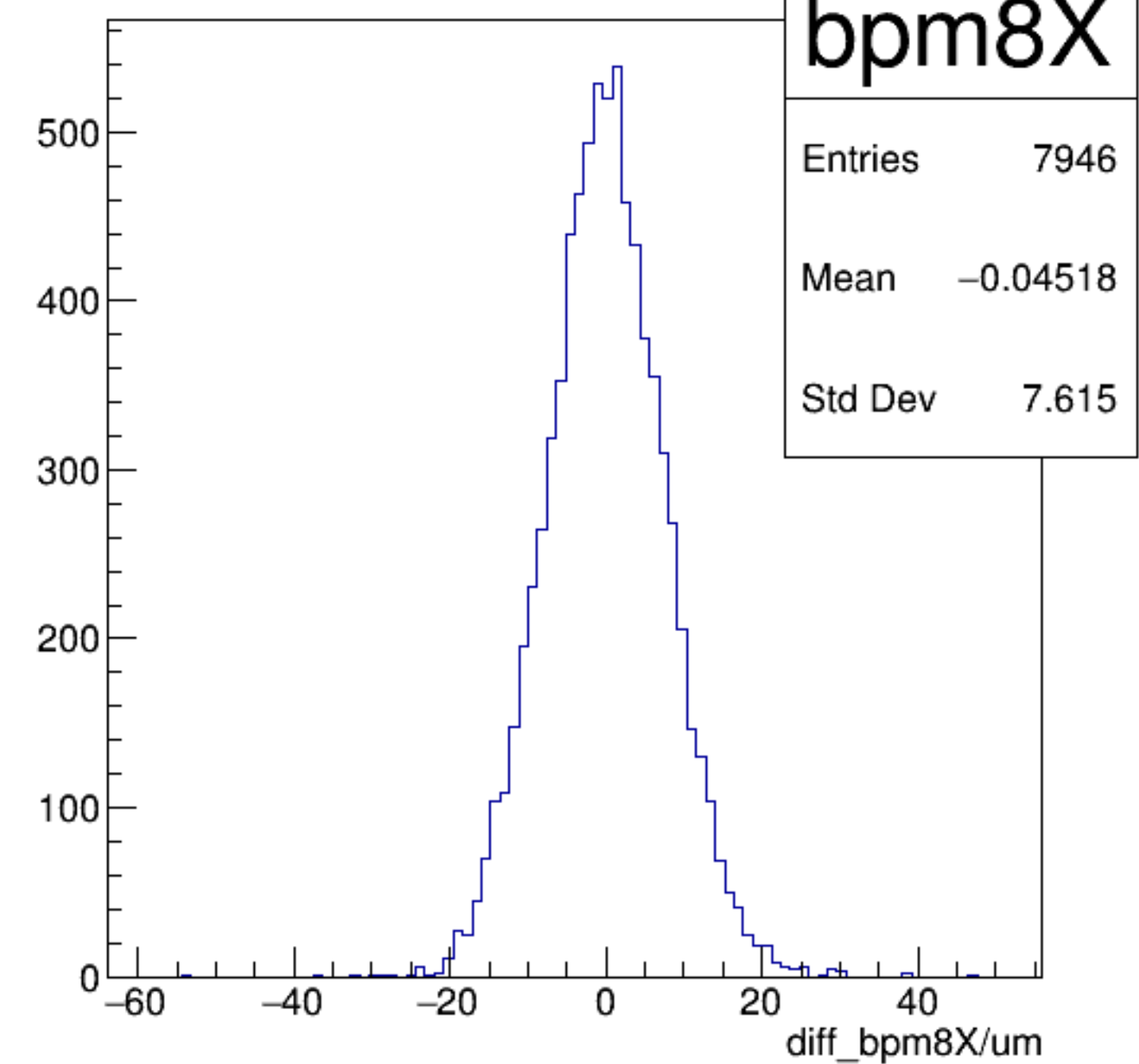
diff_bpm8X/um {ErrorFlag==0}
