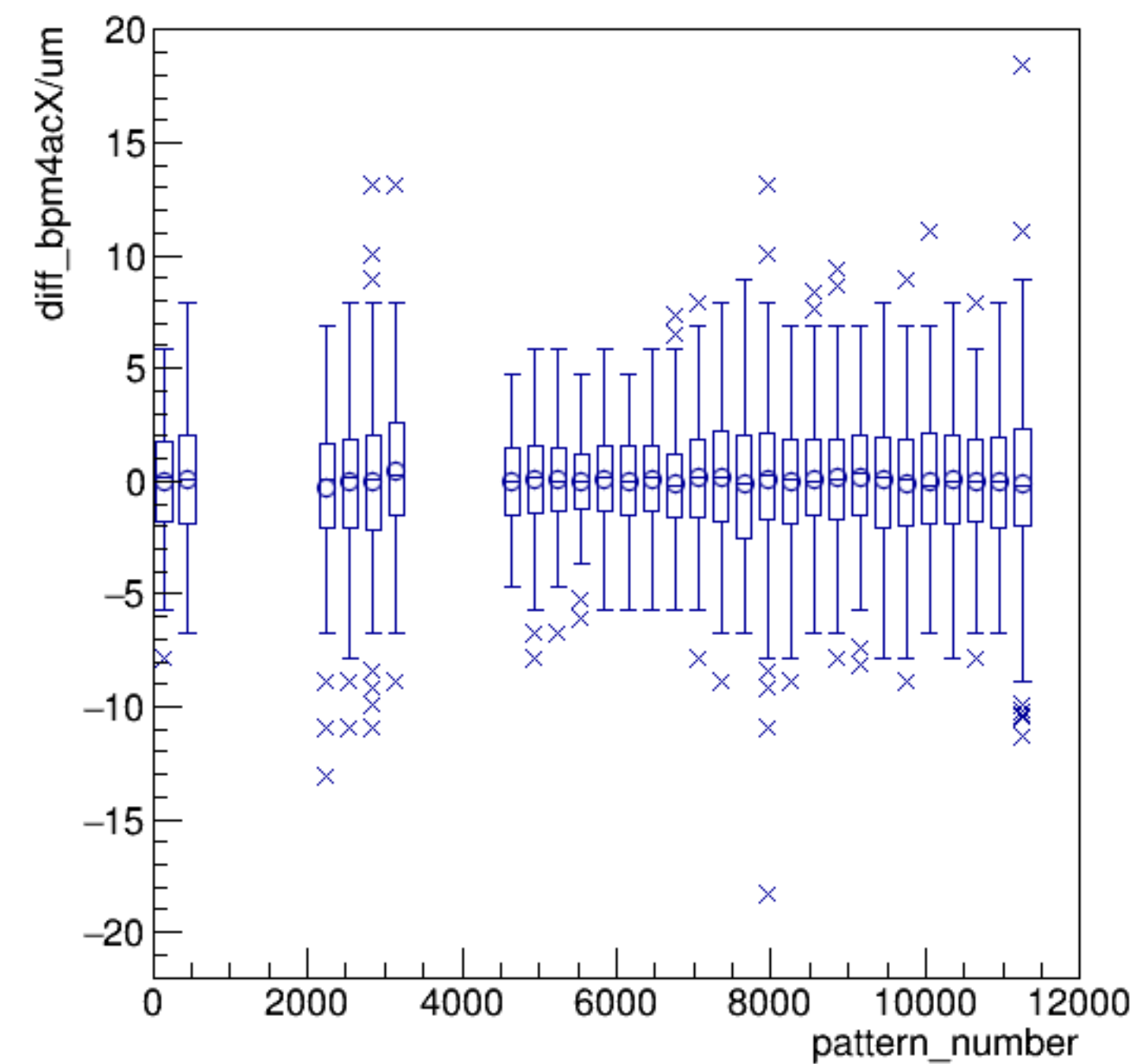
diff_bpm4acX/um:pattern_number {ErrorFlag==0}
