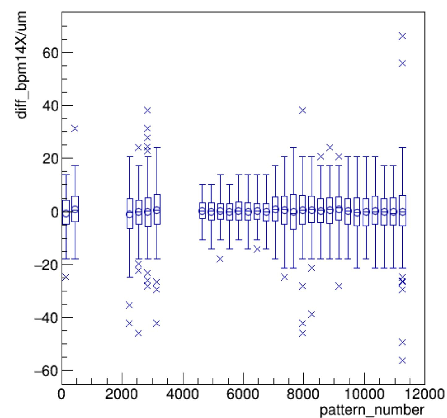
diff_bpm14X/um:pattern_number {ErrorFlag==0}
