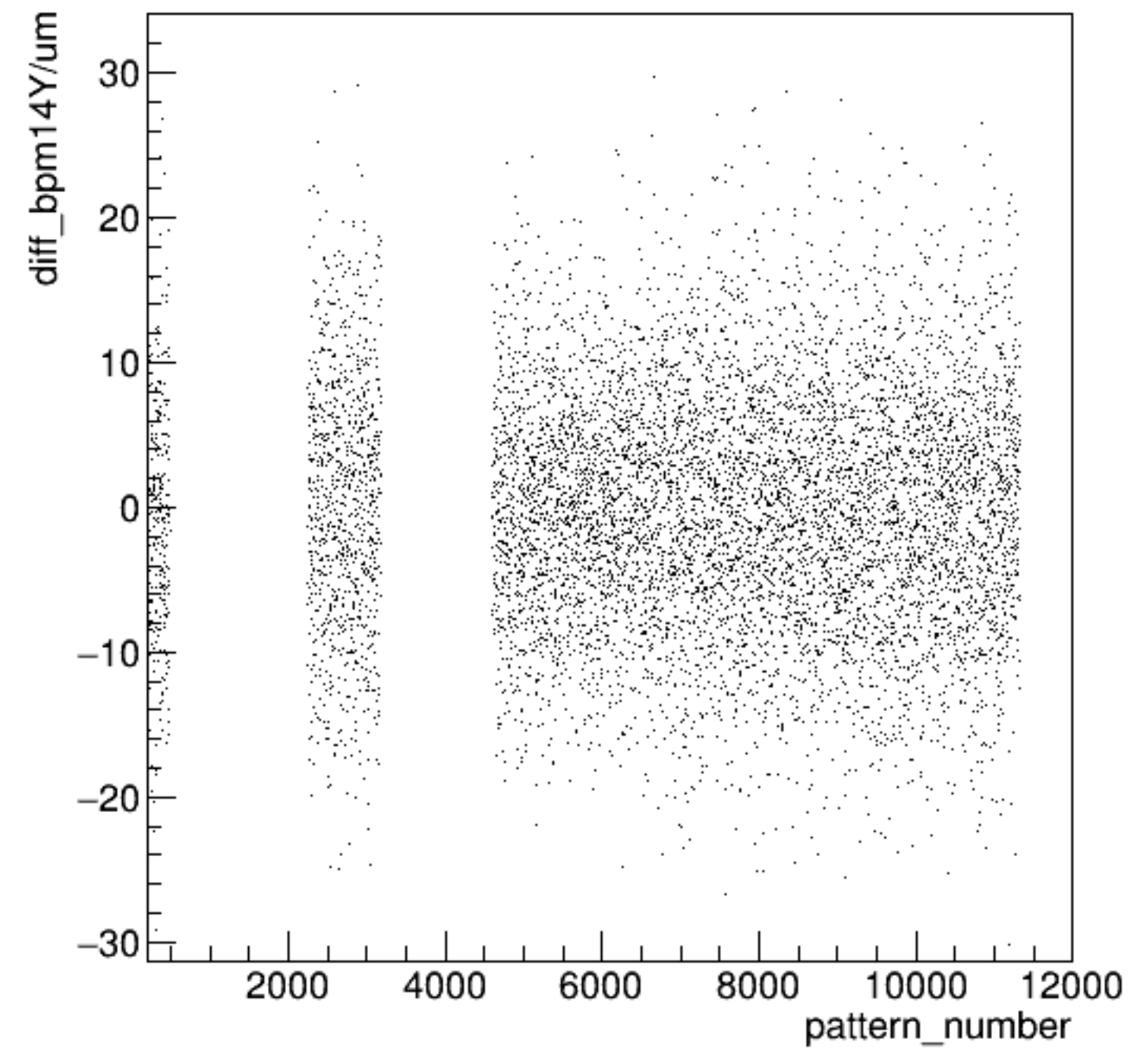
diff_bpm14Y/um:pattern_number {ErrorFlag==0}
