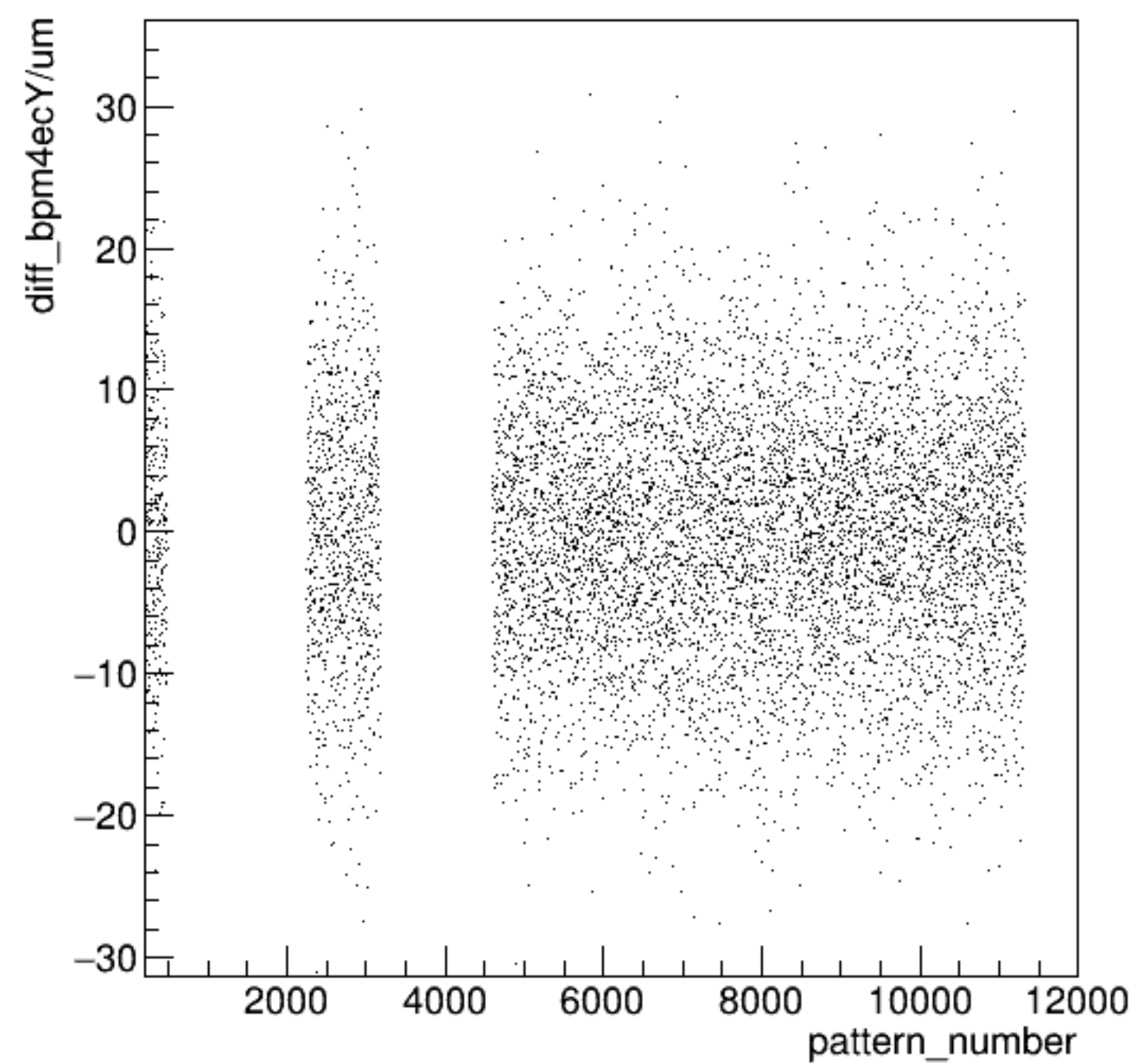
diff_bpm4ecY/um:pattern_number {ErrorFlag==0}
