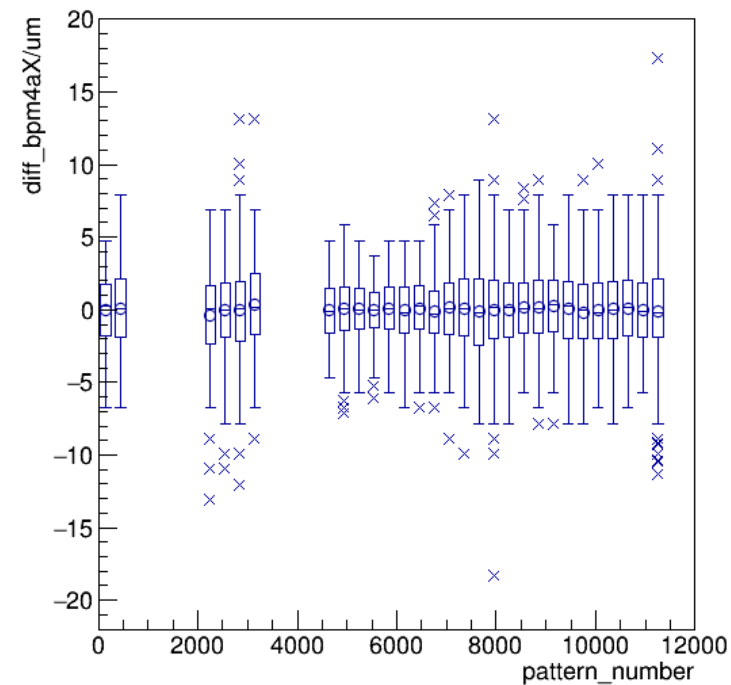
diff_bpm4aX/um:pattern_number {ErrorFlag==0}
