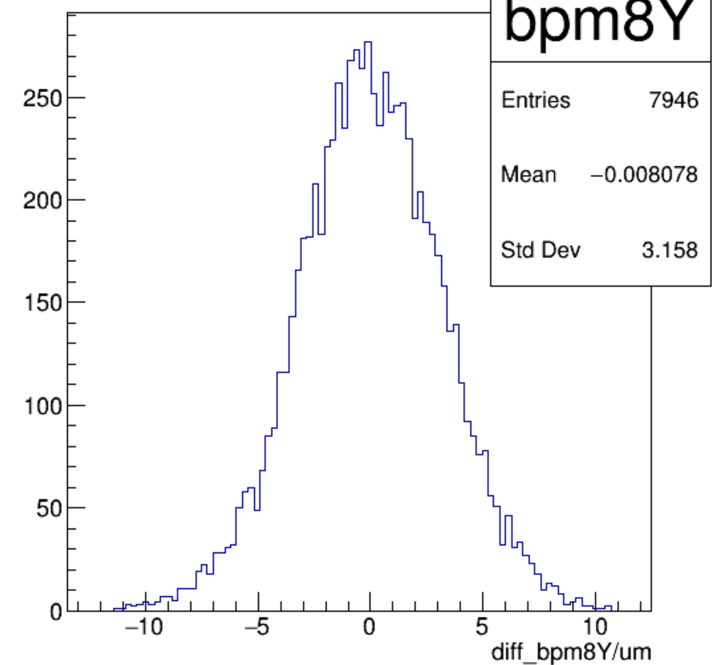
diff_bpm8Y/um {ErrorFlag==0}
