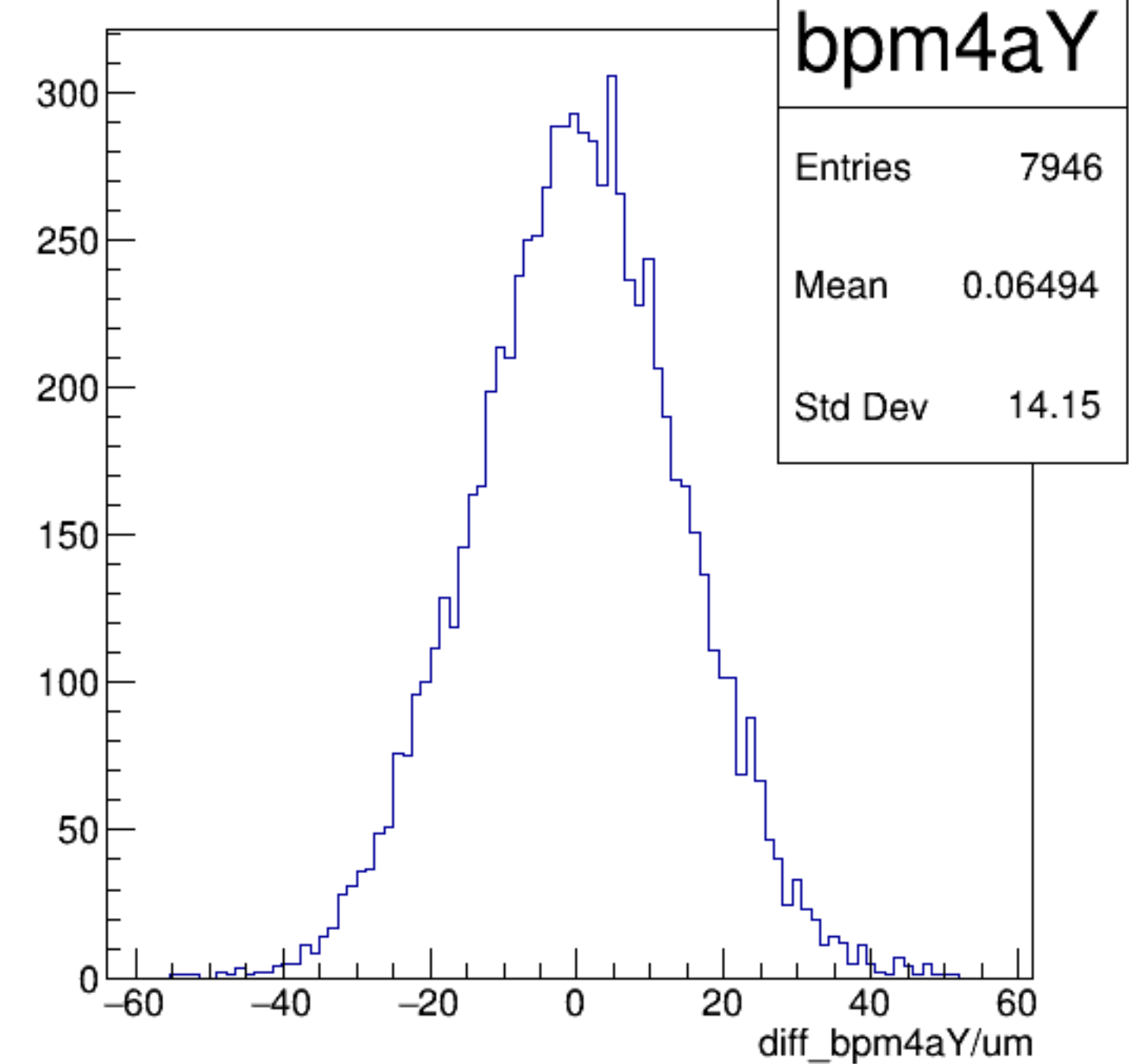
diff_bpm4aY/um {ErrorFlag==0}
