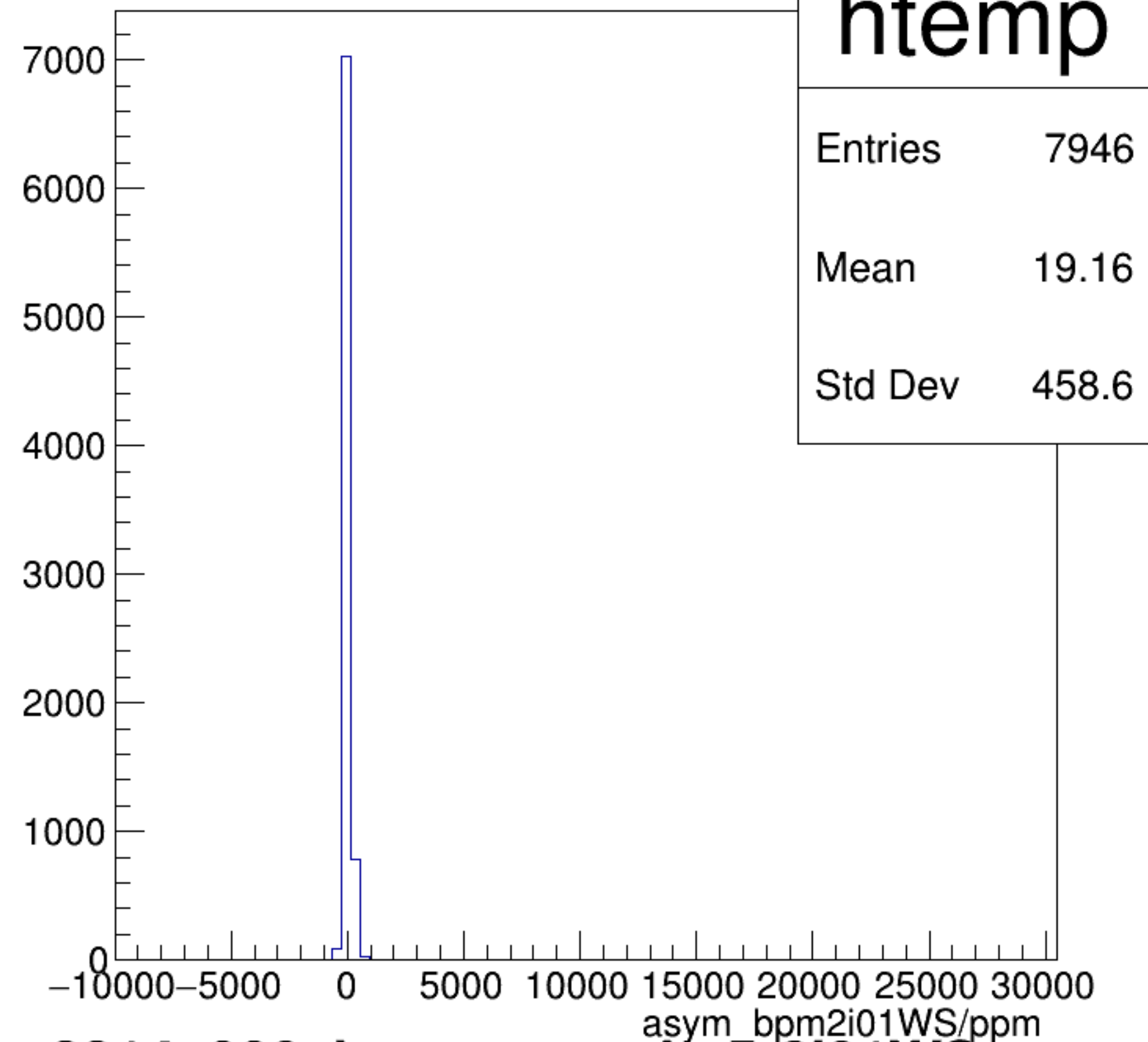
asym_bpm2i01WS/ppm {ErrorFlag==0}
