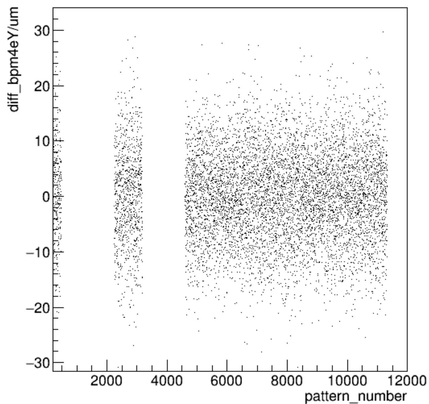
diff_bpm4eY/um:pattern_number {ErrorFlag==0}
