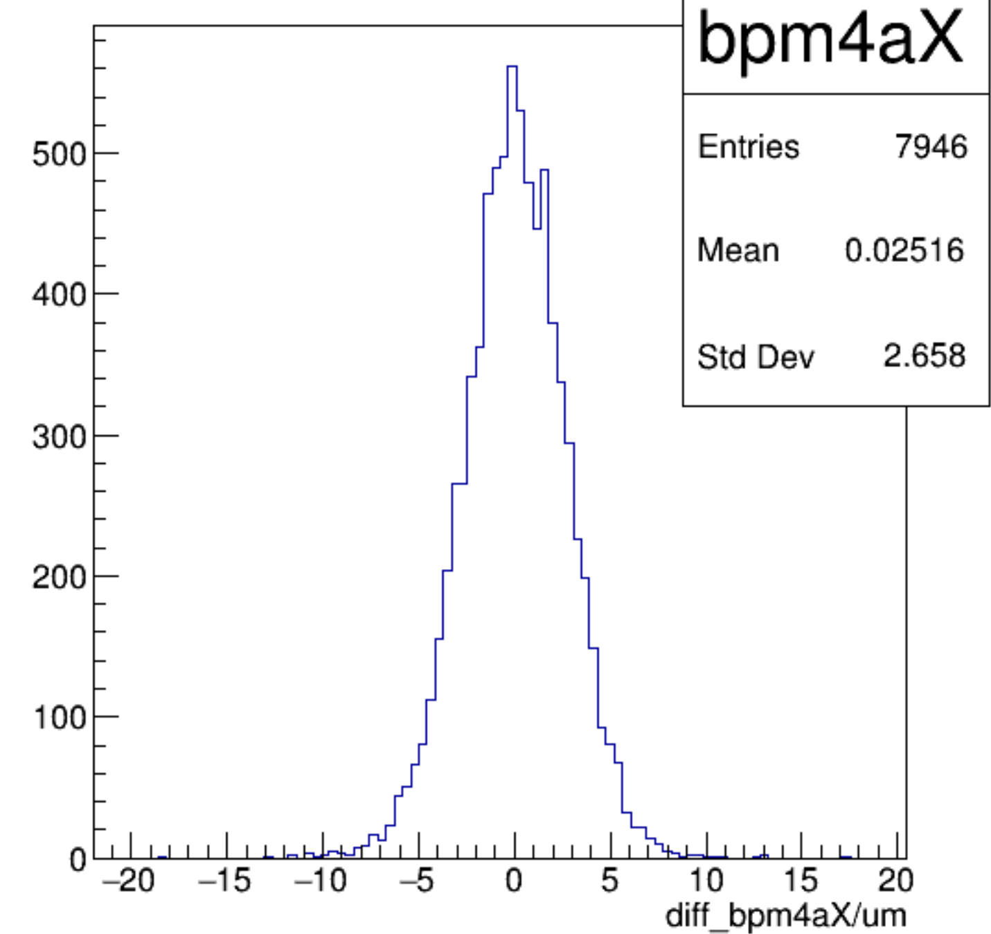
diff_bpm4aX/um {ErrorFlag==0}
