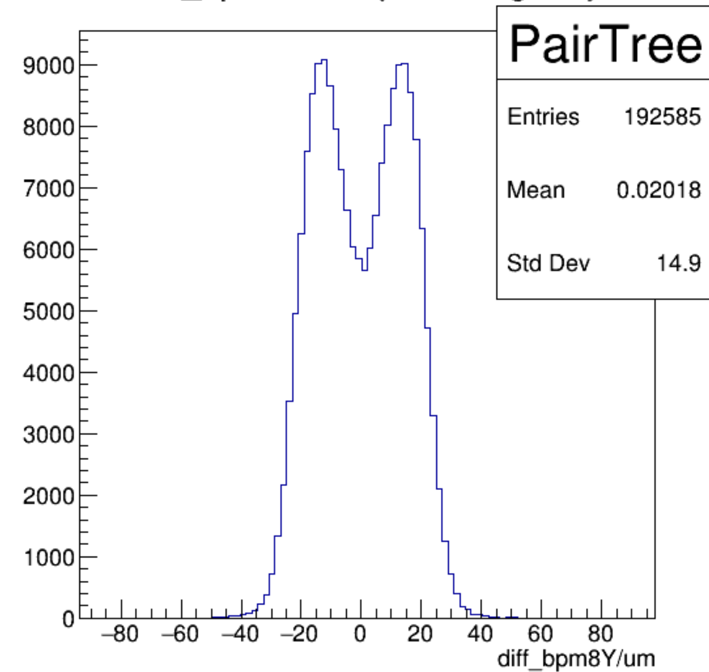
diff_bpm8Y/um {ErrorFlag==0}
