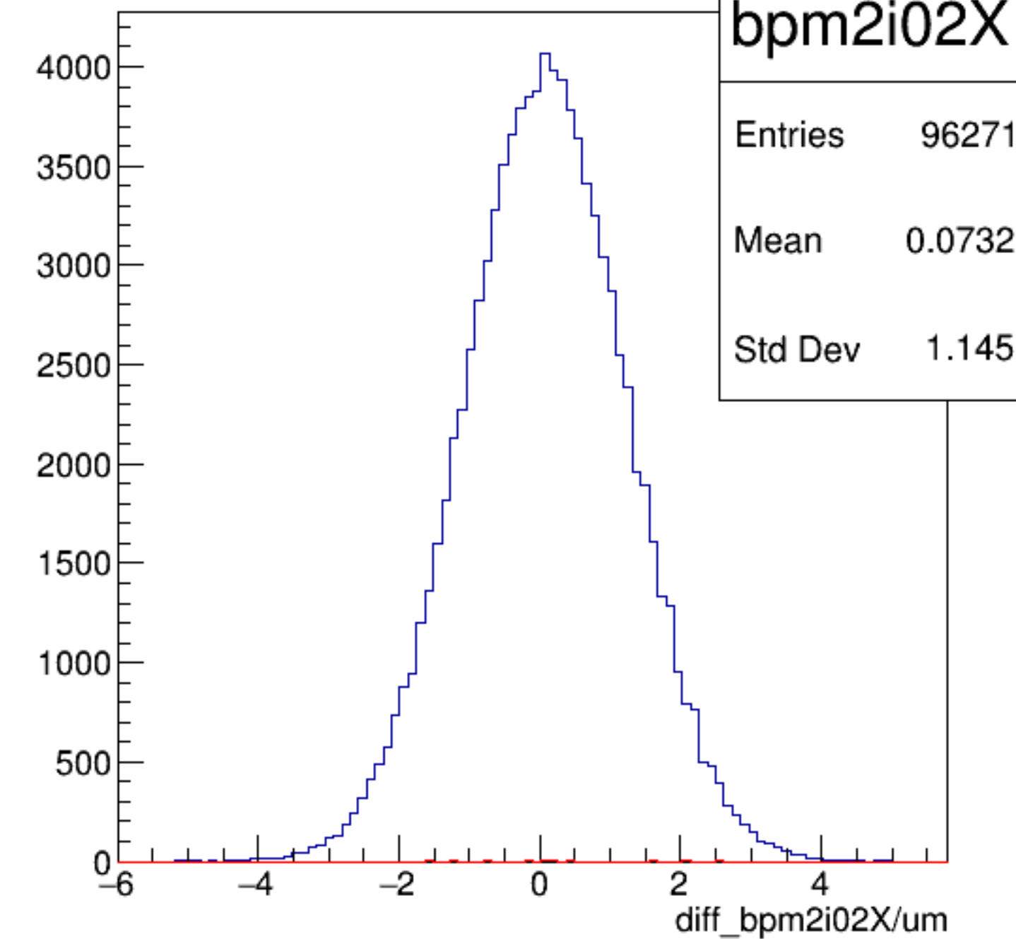
diff_bpm2i02X/um {ErrorFlag==0}
