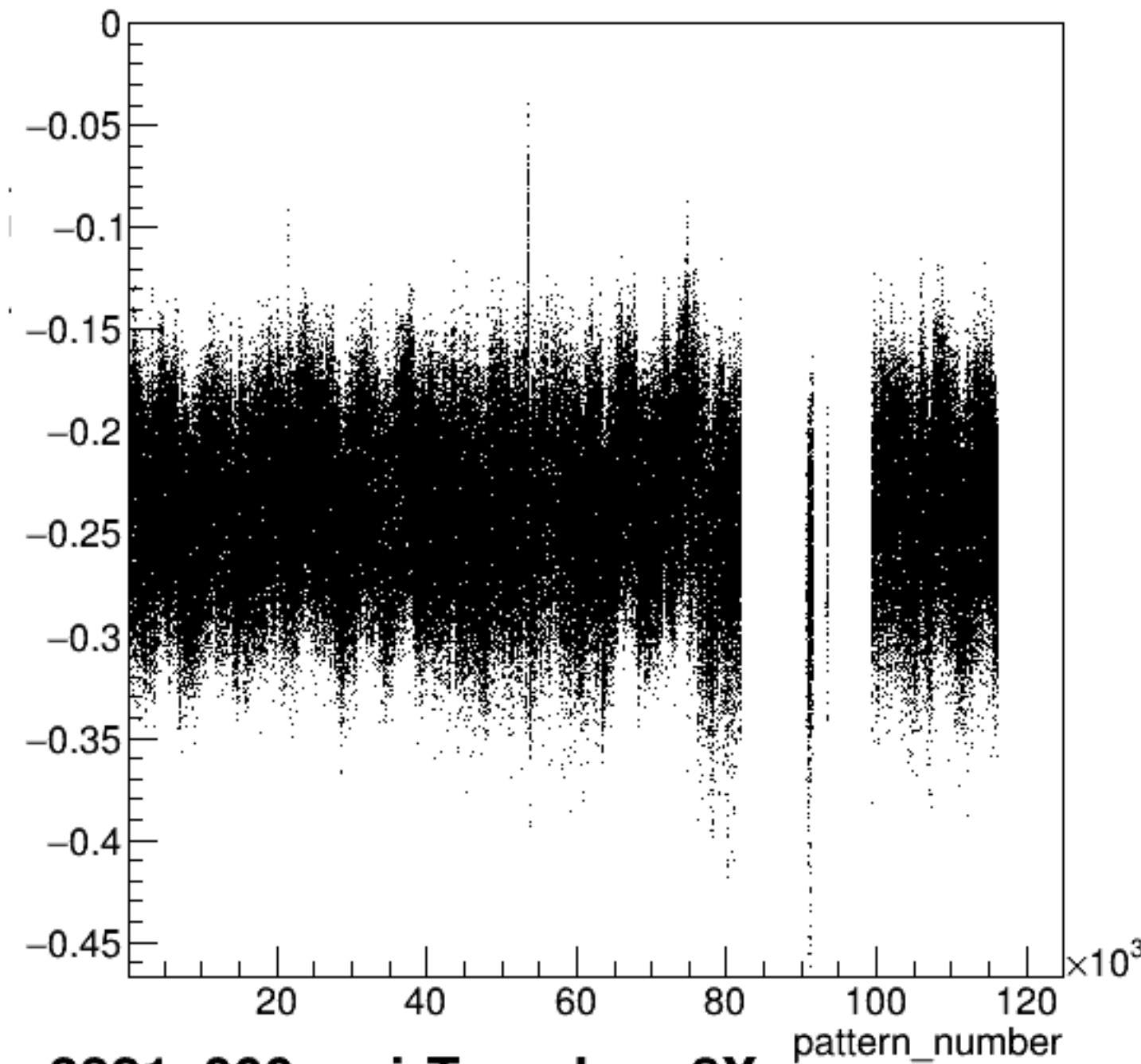
yield_bpm8X/mm:pattern_number {ErrorFlag==0}
