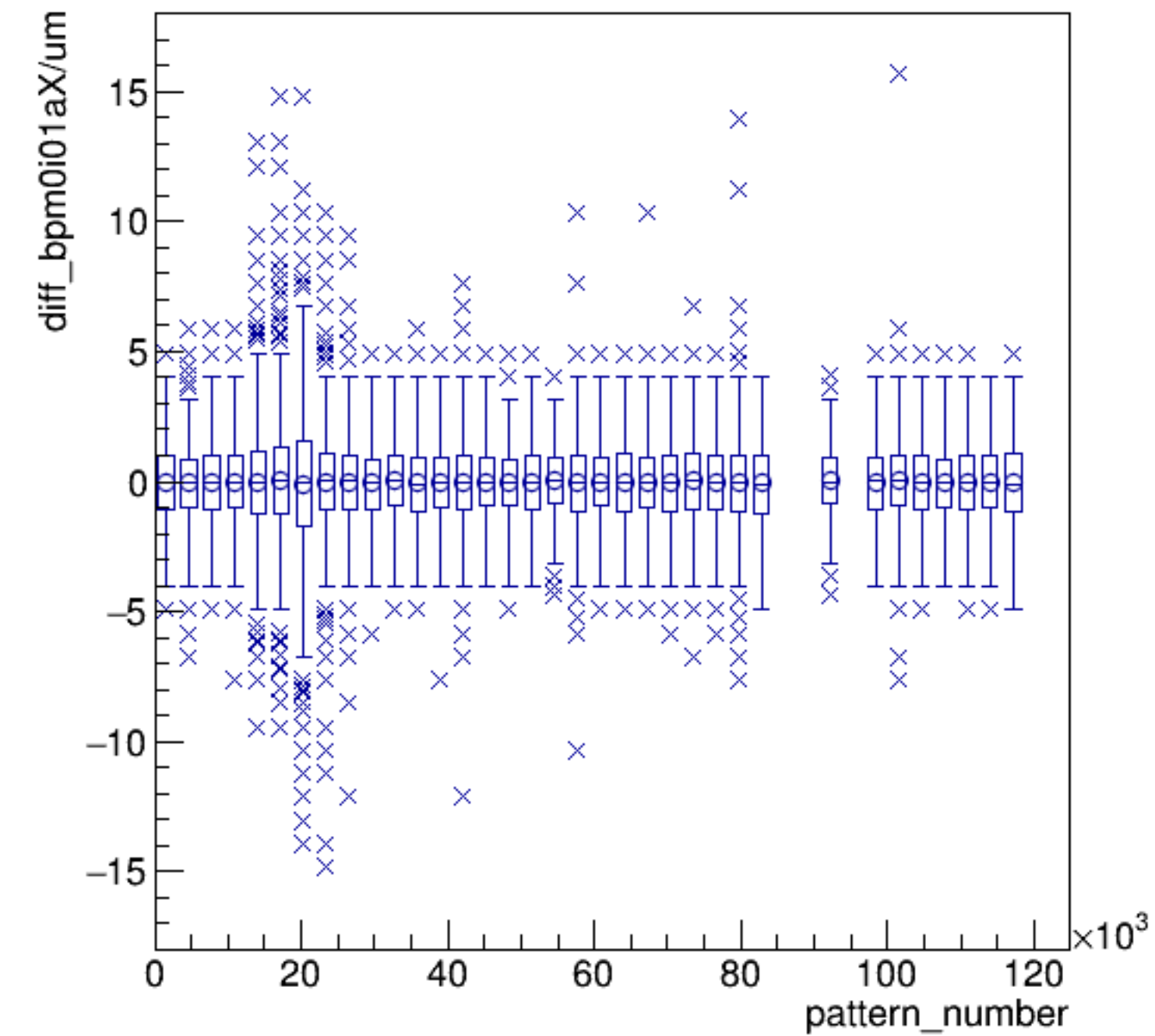
diff_bpm0i01aX/um:pattern_number {ErrorFlag==0}
