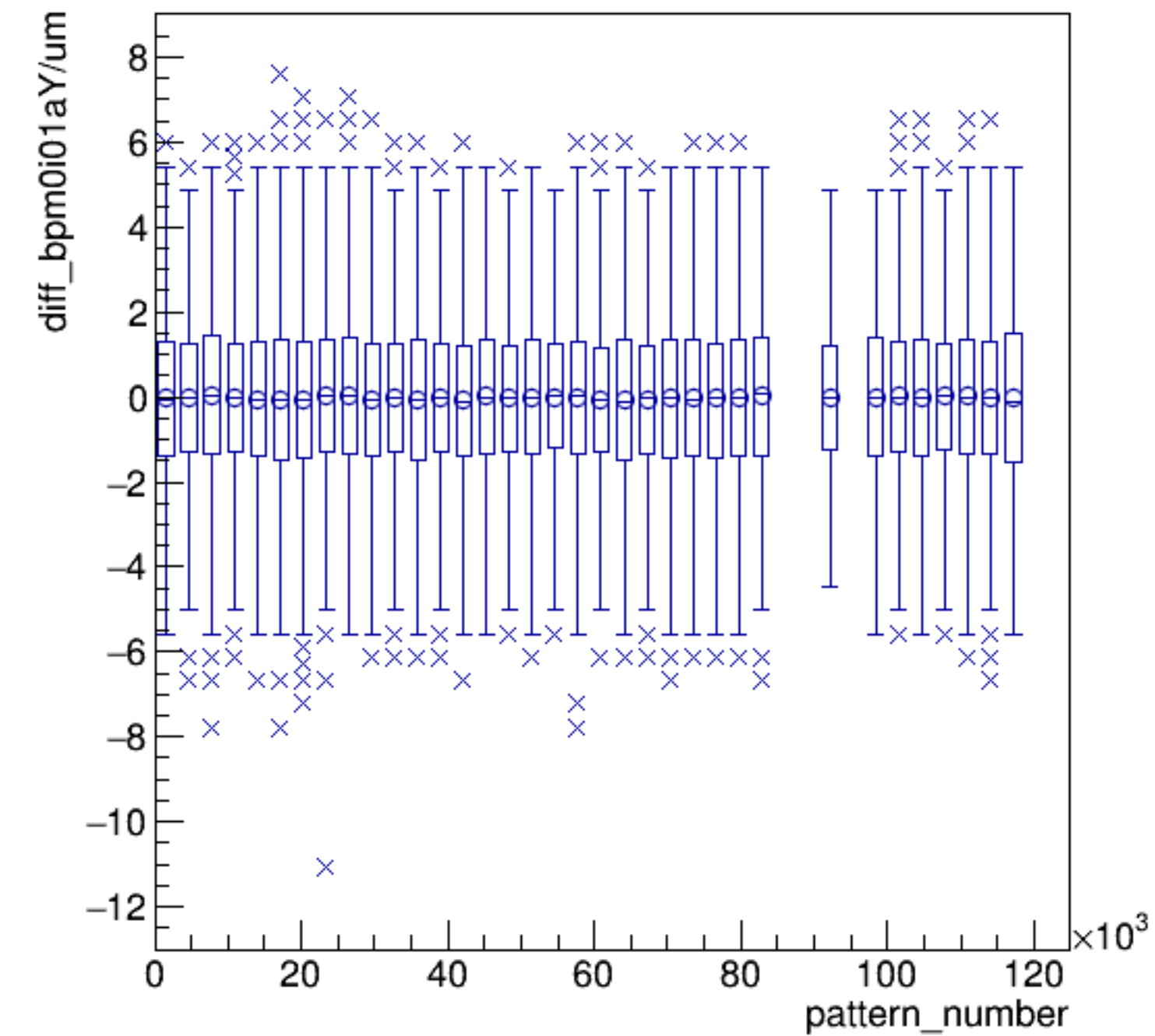
diff_bpm0i01aY/um:pattern_number {ErrorFlag==0}
