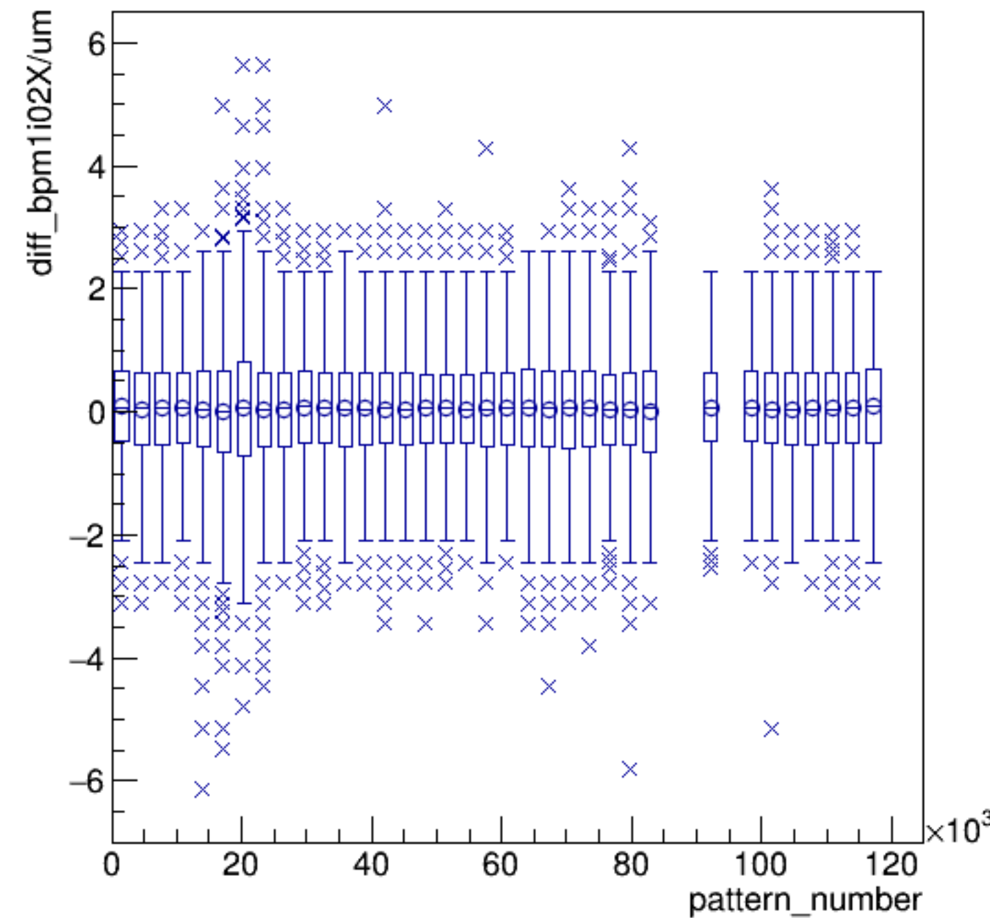
diff_bpm1i02X/um:pattern_number {ErrorFlag==0}
