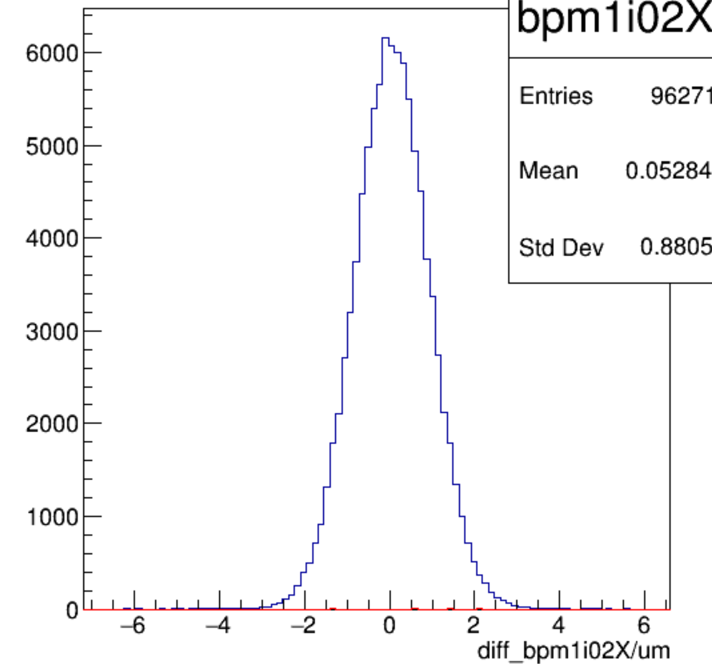
diff_bpm1i02X/um {ErrorFlag==0}
