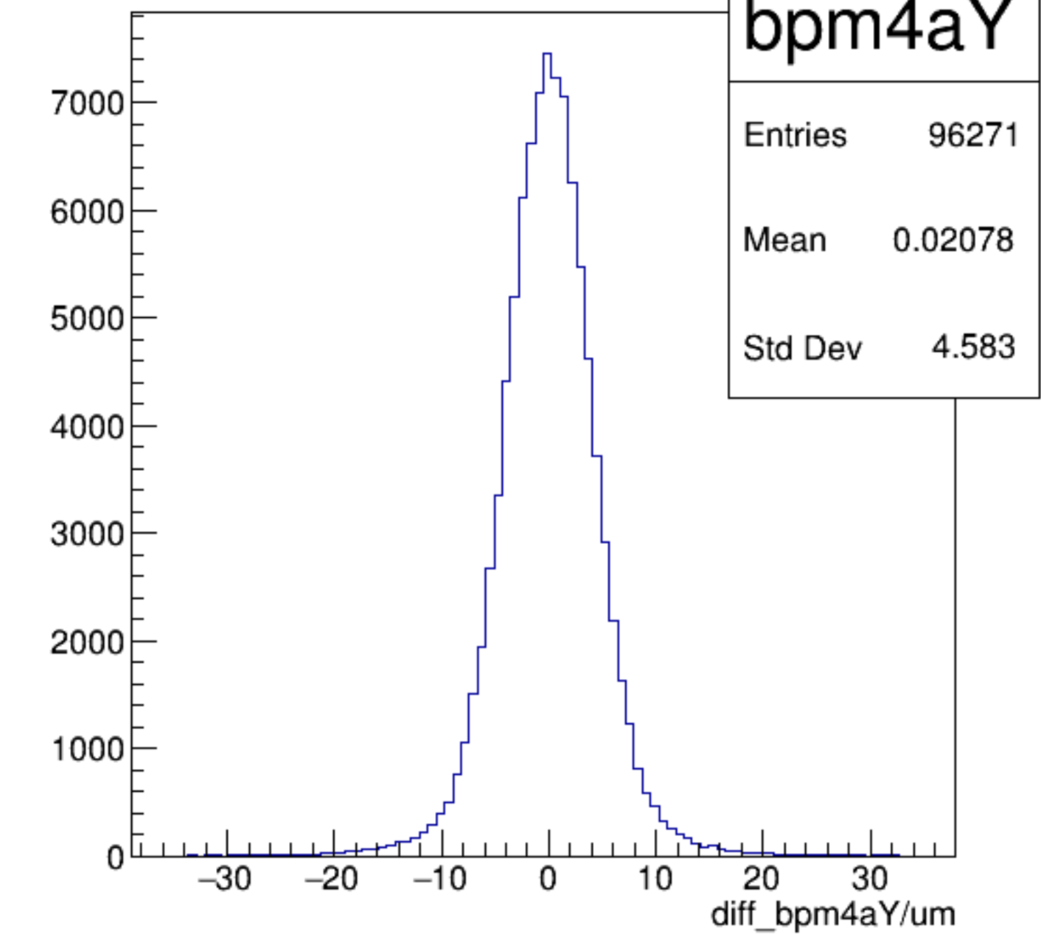
diff_bpm4aY/um {ErrorFlag==0}
