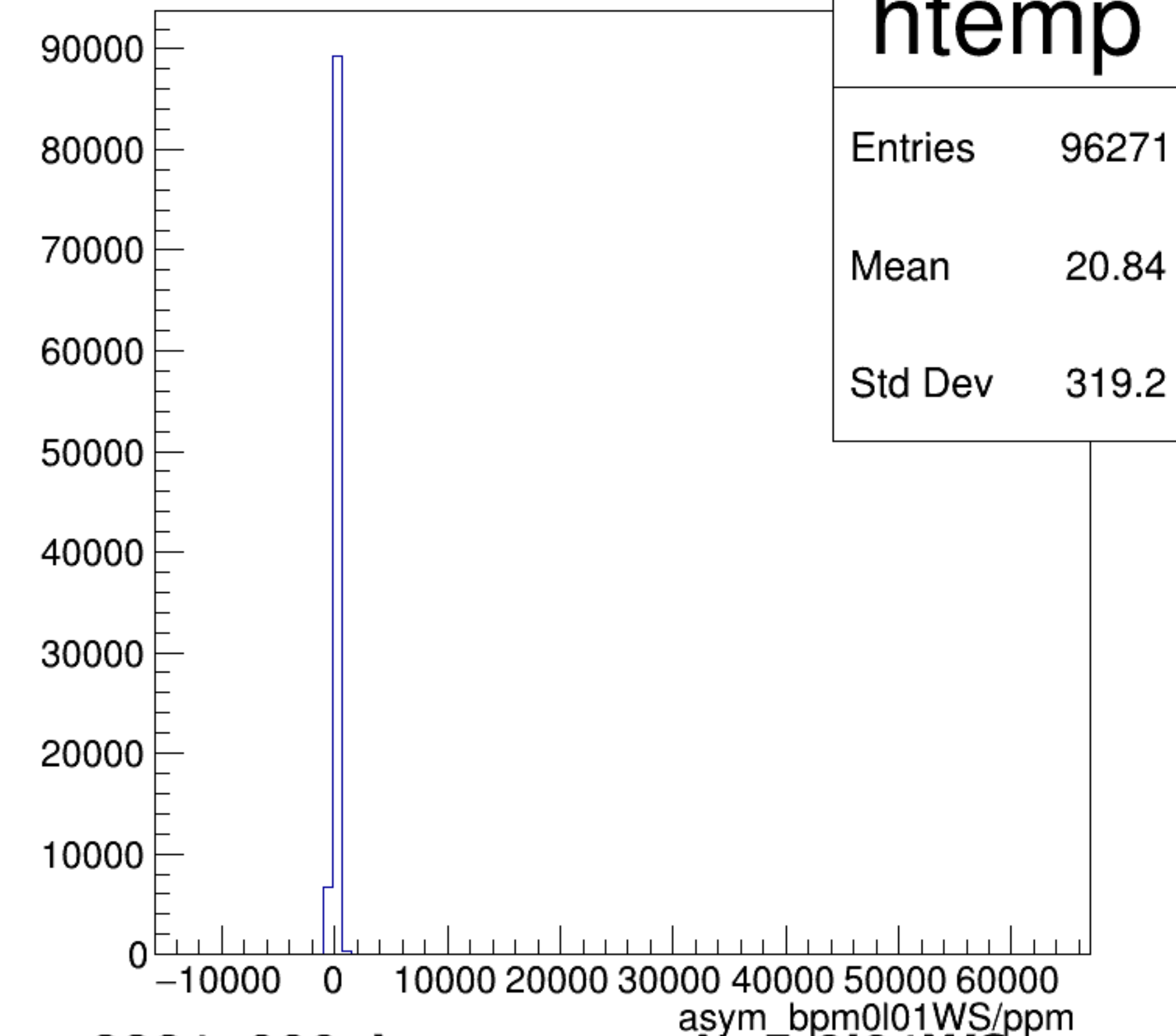
asym_bpm0l01WS/ppm {ErrorFlag==0}
