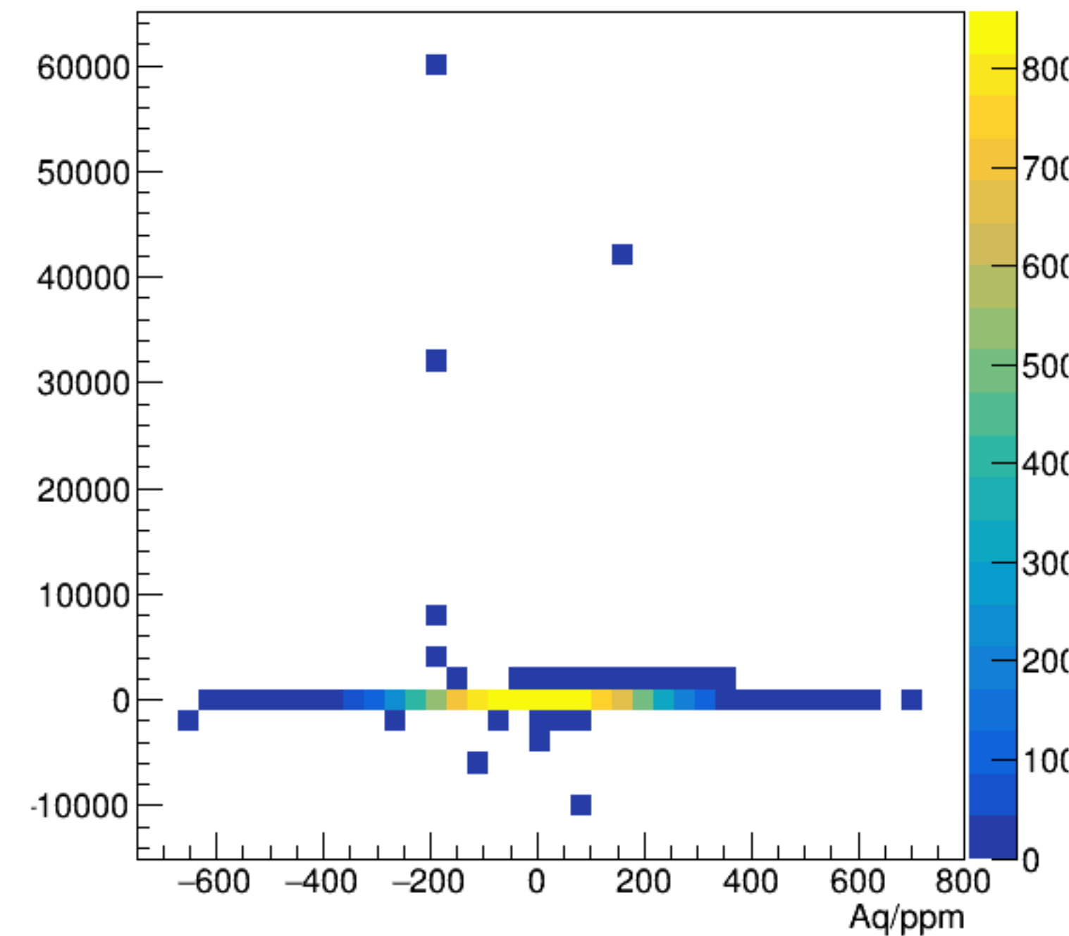
asym_bpm0l01WS/ppm:Aq/ppm {ErrorFlag==0}
