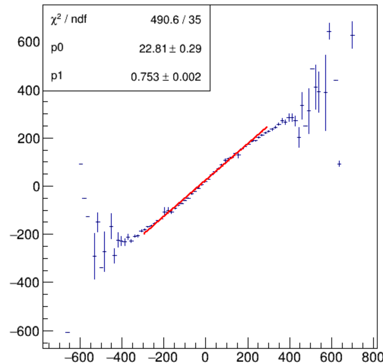
asym_bpm2i02WS/ppm:Aq/ppm {ErrorFlag==0}
