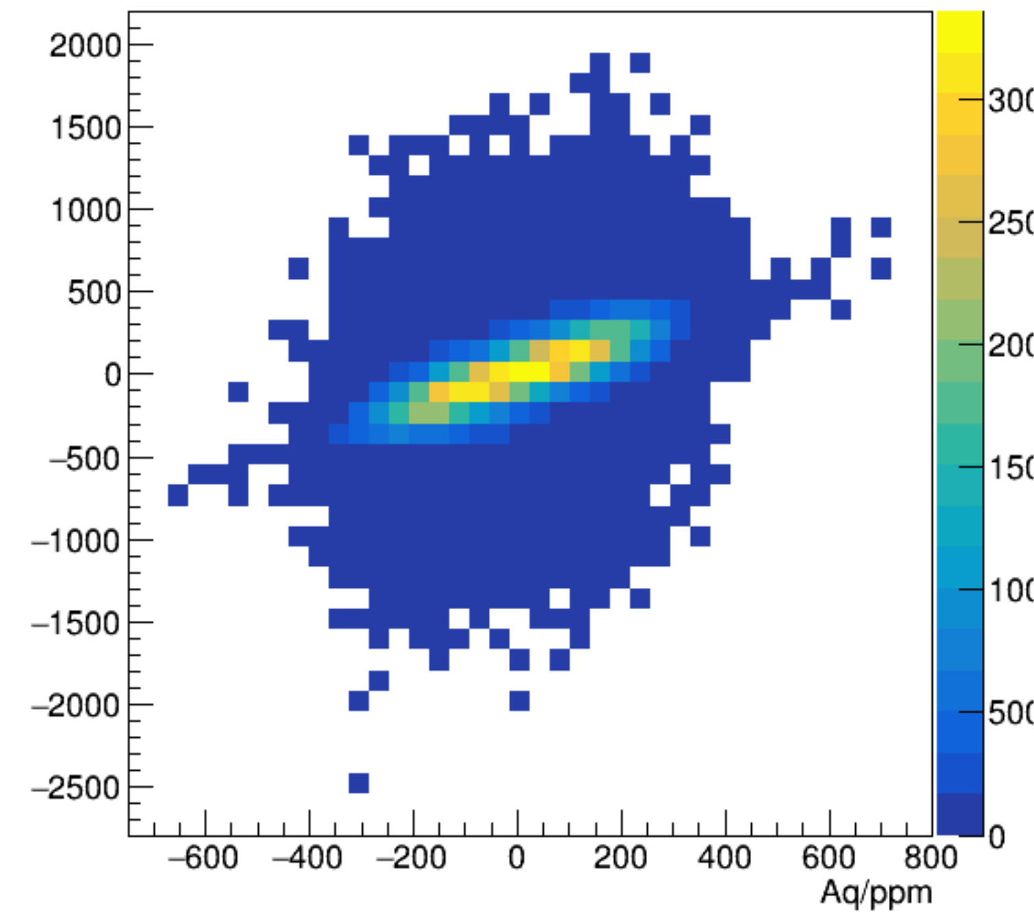
asym_bpm4aWS/ppm:Aq/ppm {ErrorFlag==0}
