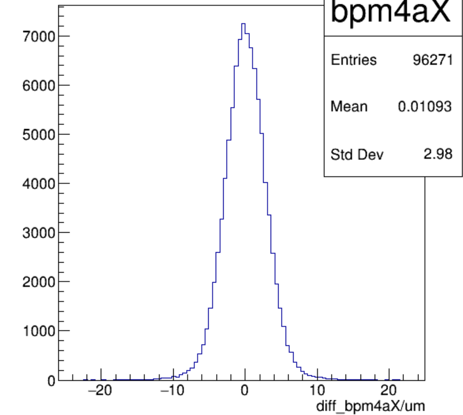
diff_bpm4aX/um {ErrorFlag==0}
