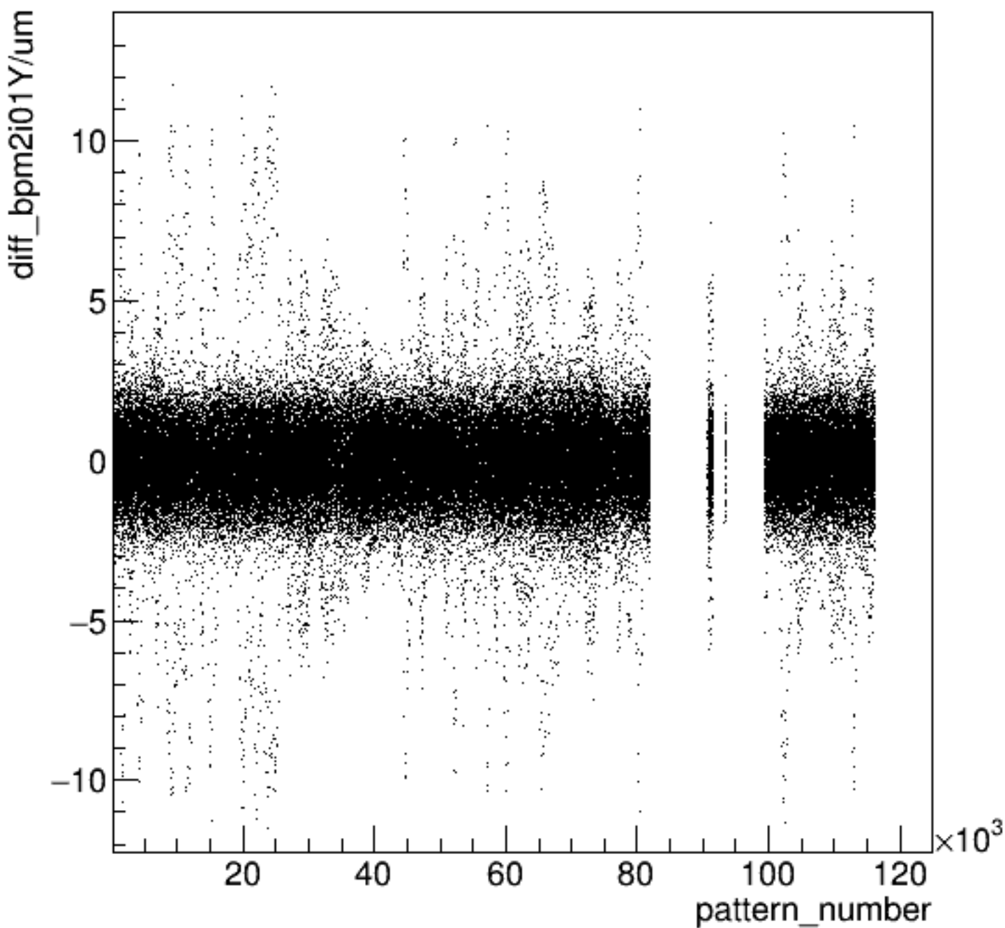
diff_bpm2i01Y/um:pattern_number {ErrorFlag==0}
