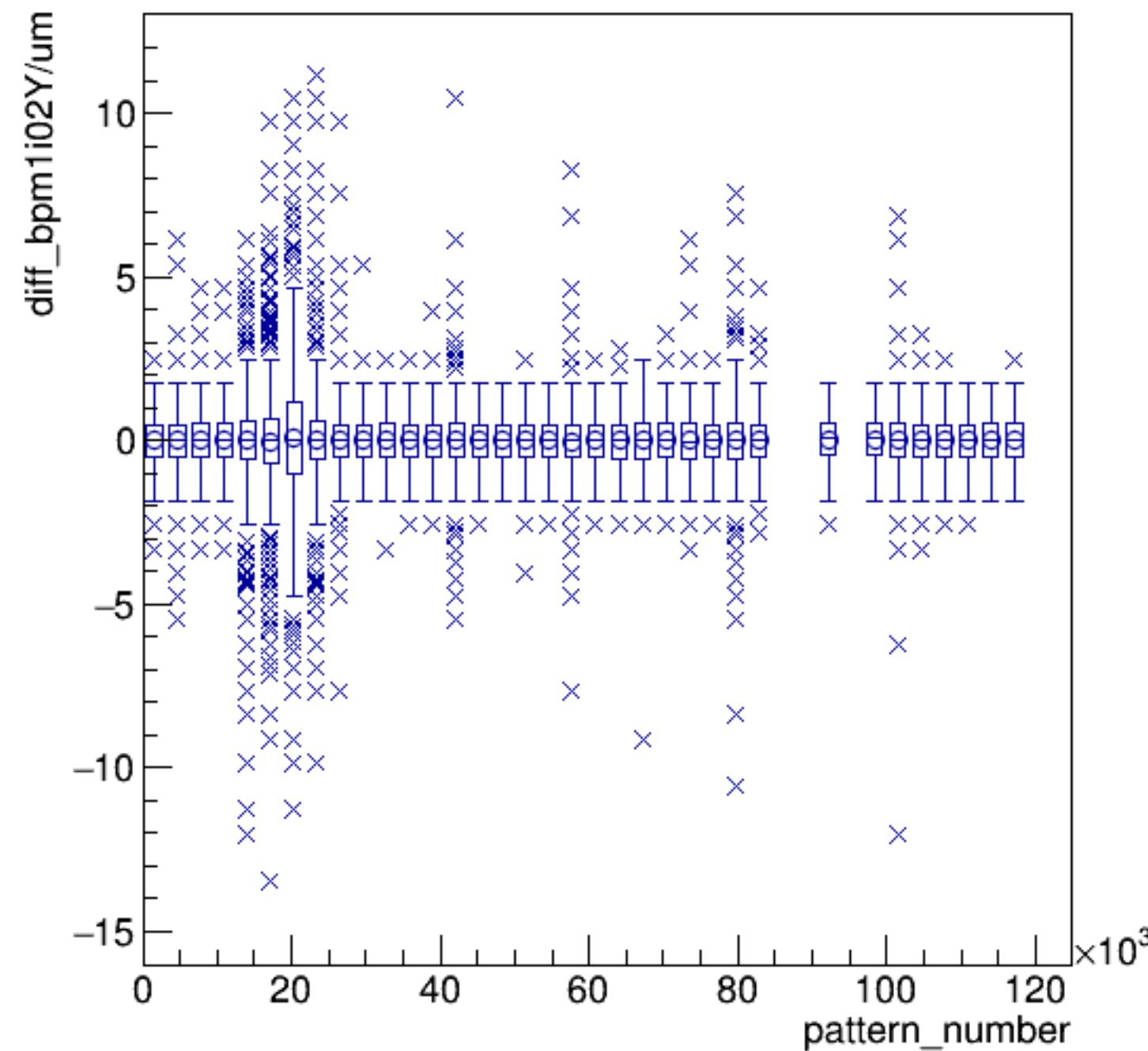
diff_bpm1i02Y/um:pattern_number {ErrorFlag==0}
