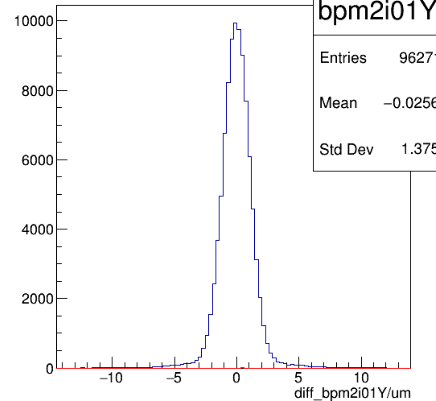
diff_bpm2i01Y/um {ErrorFlag==0}
