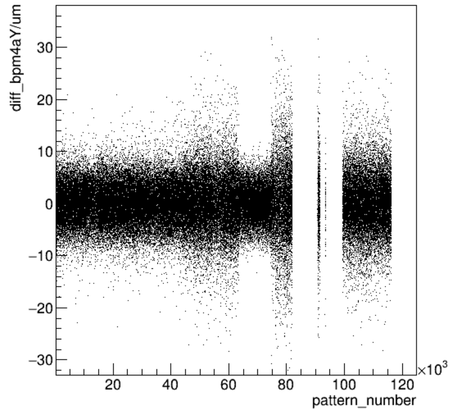
diff_bpm4aY/um:pattern_number {ErrorFlag==0}
