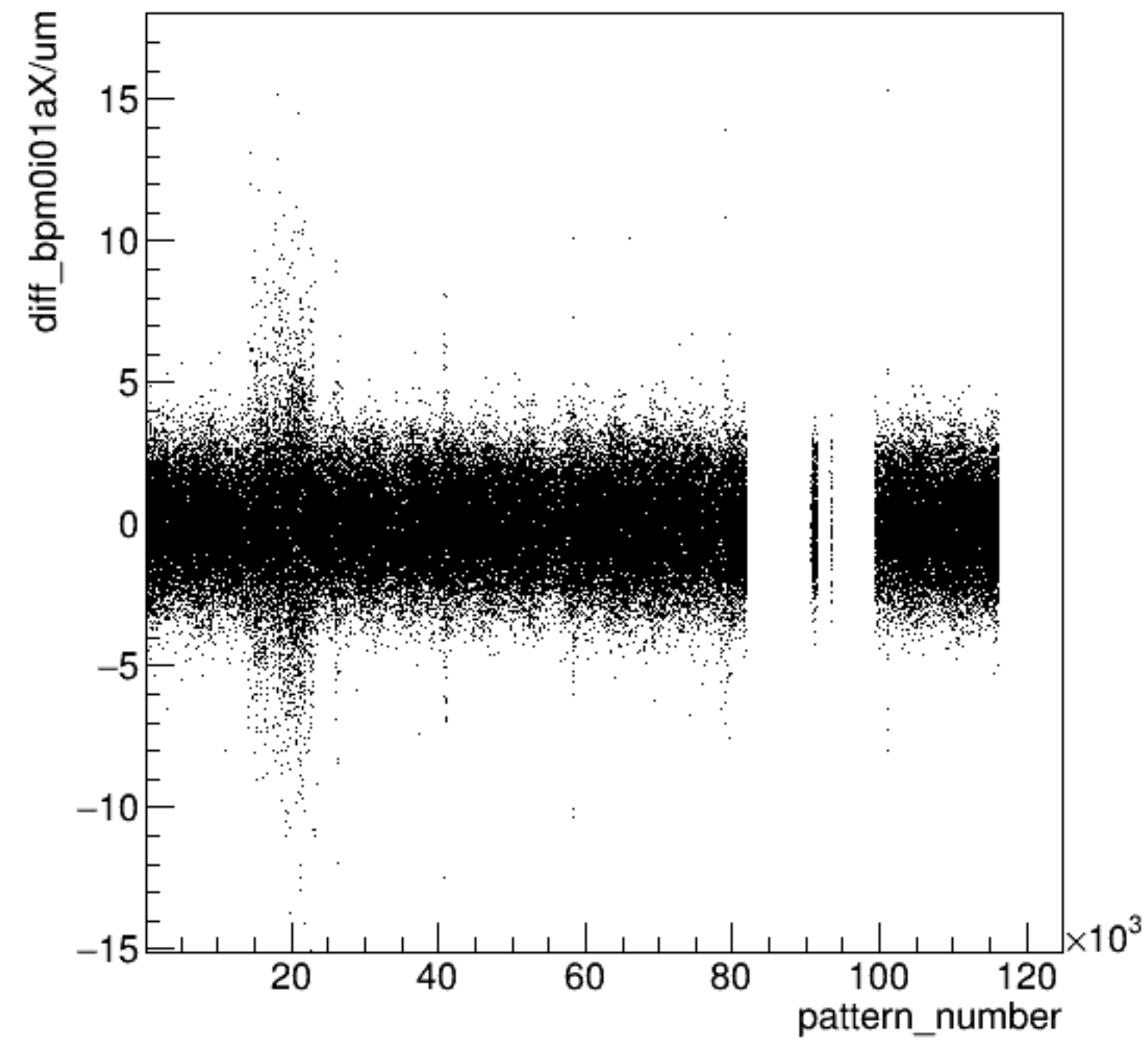
diff_bpm0i01aX/um:pattern_number {ErrorFlag==0}
