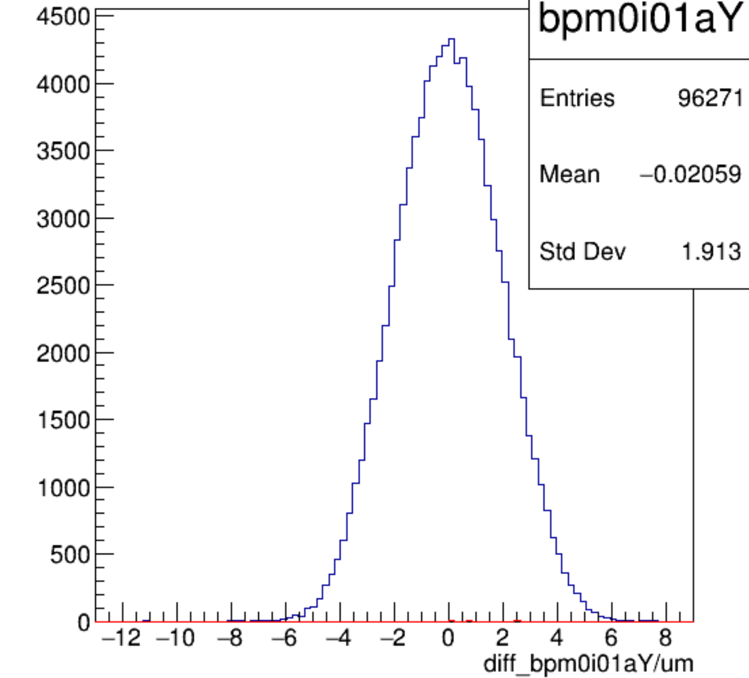
diff_bpm0i01aY/um {ErrorFlag==0}
