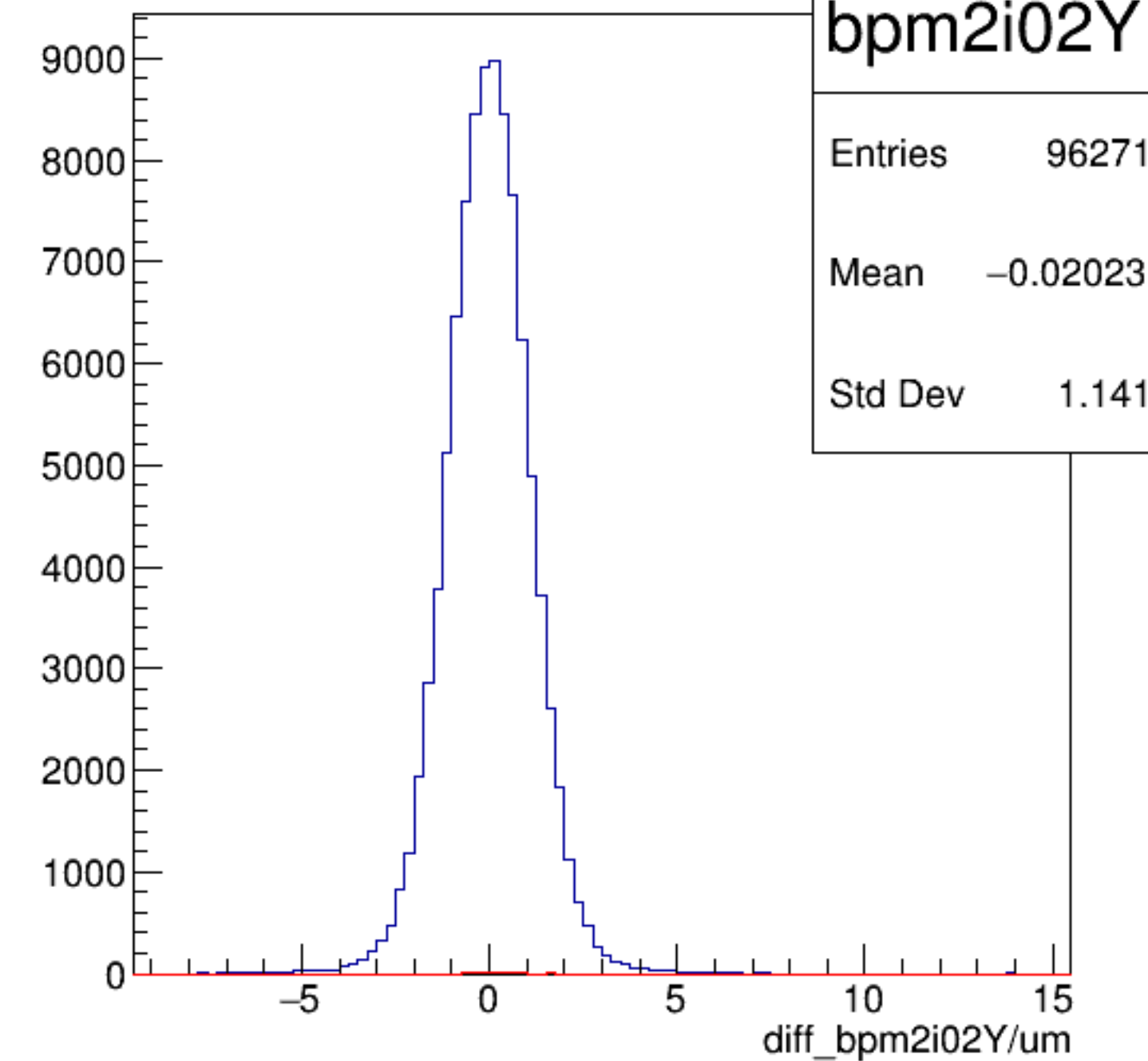
diff_bpm2i02Y/um {ErrorFlag==0}
