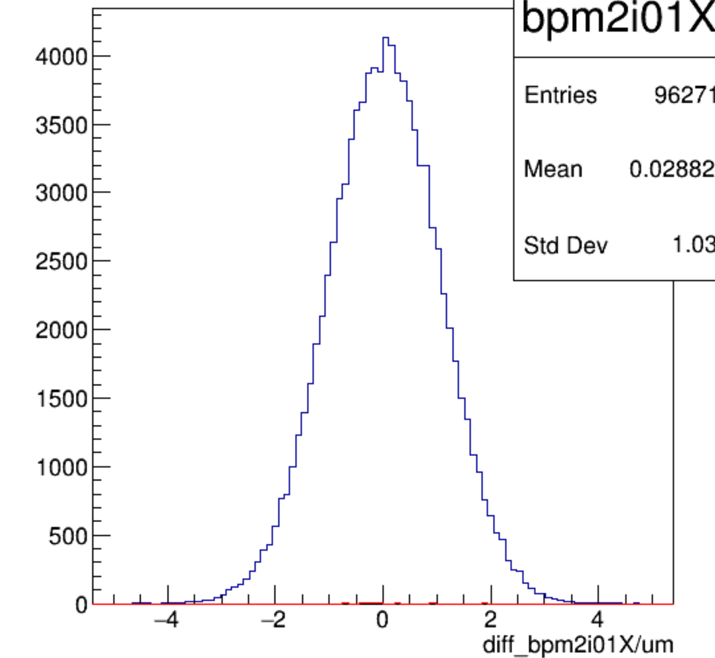
diff_bpm2i01X/um {ErrorFlag==0}
