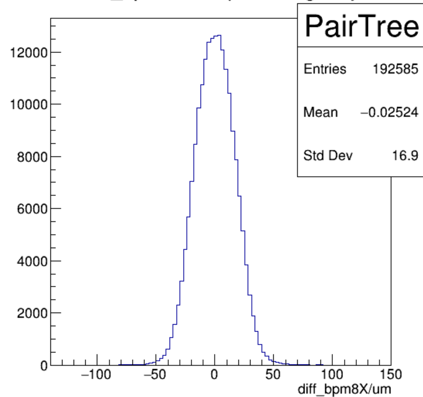
diff_bpm8X/um {ErrorFlag==0}
