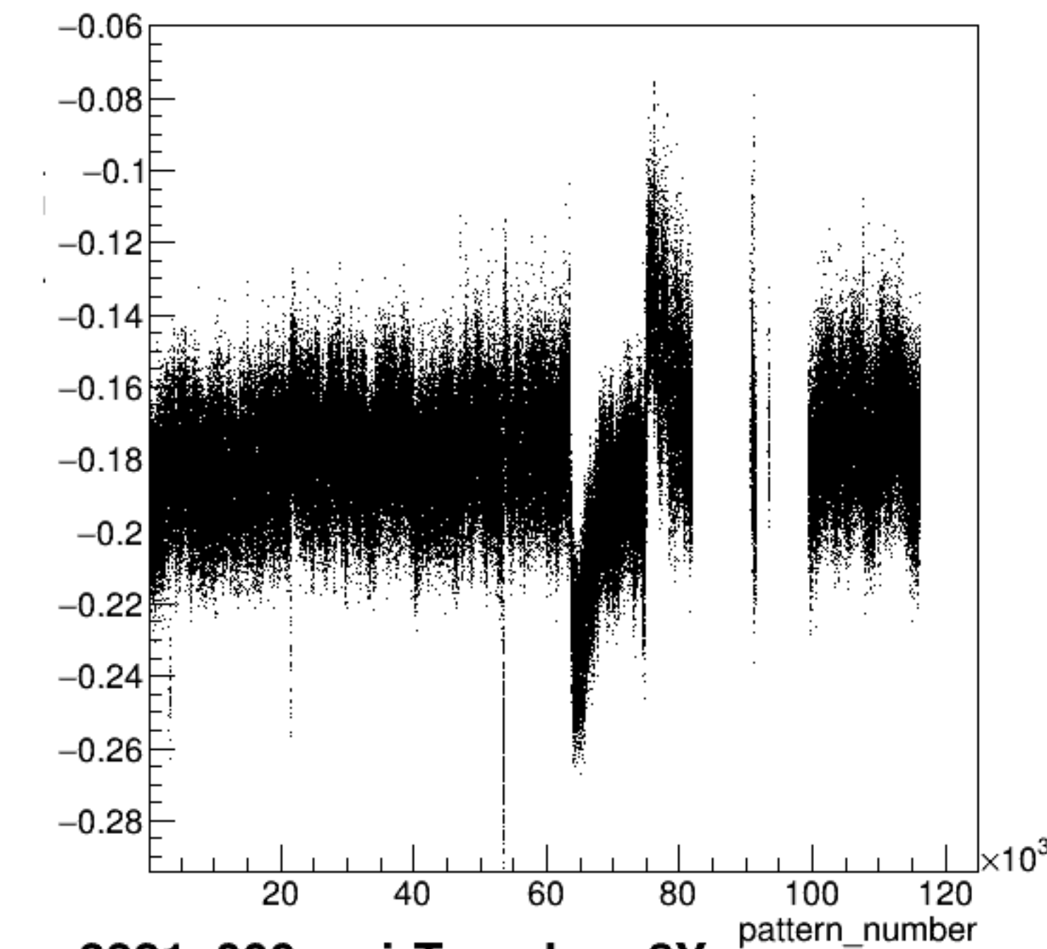
yield_bpm8Y/mm:pattern_number {ErrorFlag==0}
