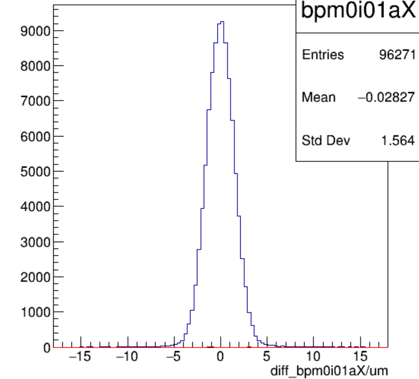
diff_bpm0i01aX/um {ErrorFlag==0}
