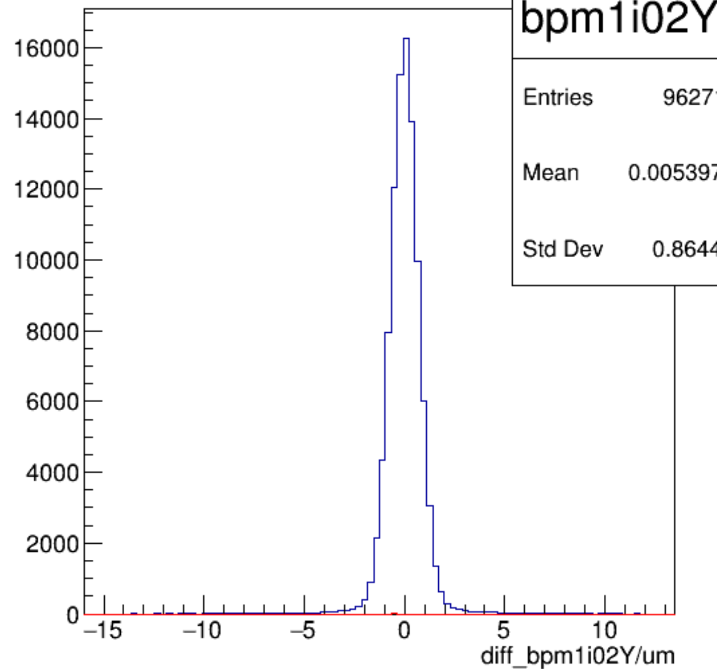
diff_bpm1i02Y/um {ErrorFlag==0}
