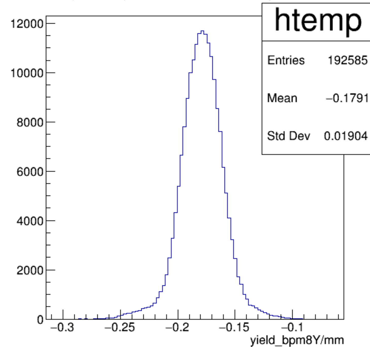
yield_bpm8Y/mm {ErrorFlag==0}
