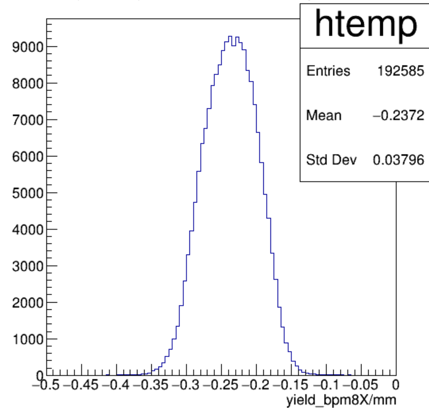
yield_bpm8X/mm {ErrorFlag==0}
